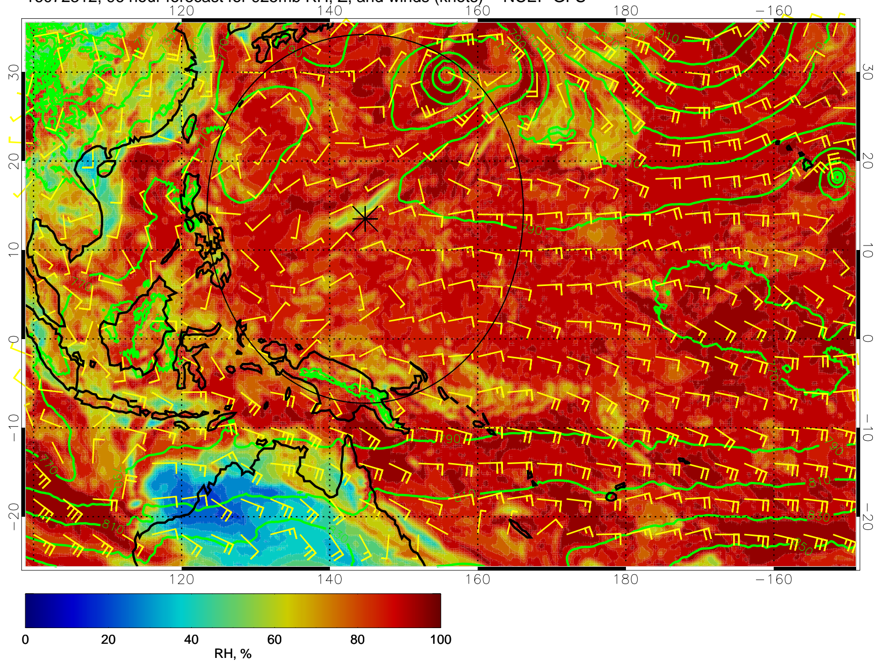
16072312, 96 hour forecast for 925mb RH, Z, and winds (knots) -- NCEP GFS
