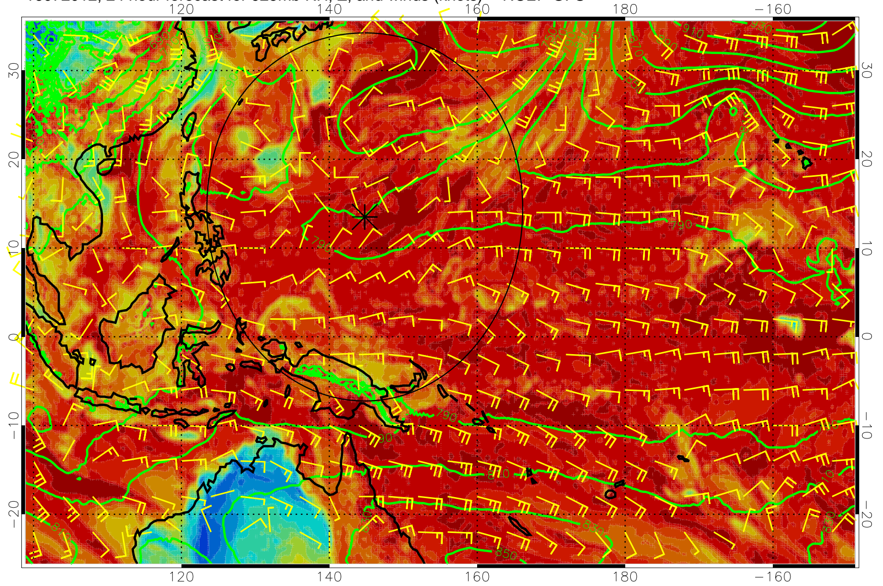
16072012, 24 hour forecast for 925mb RH, Z, and winds (knots) -- NCEP GFS
