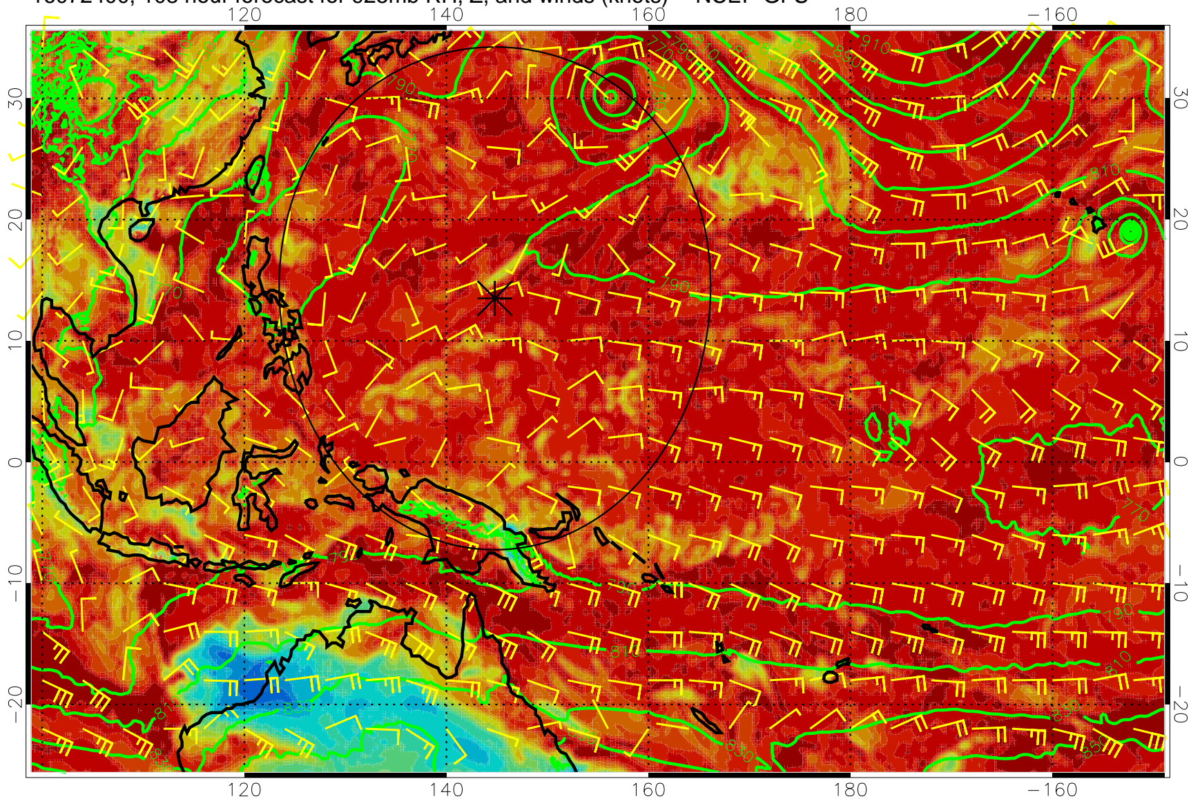
16072400, 108 hour forecast for 925mb RH, Z, and winds (knots) -- NCEP GFS
