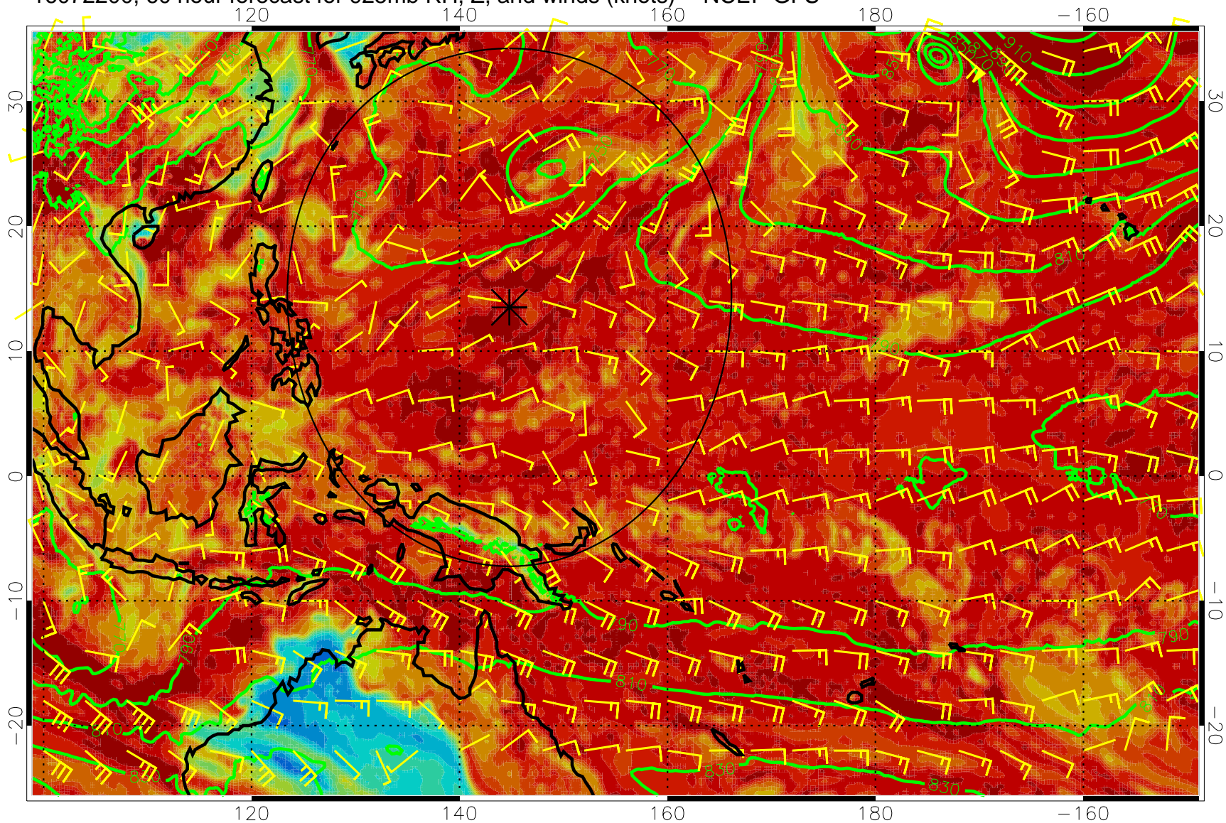
16072200, 60 hour forecast for 925mb RH, Z, and winds (knots) -- NCEP GFS
