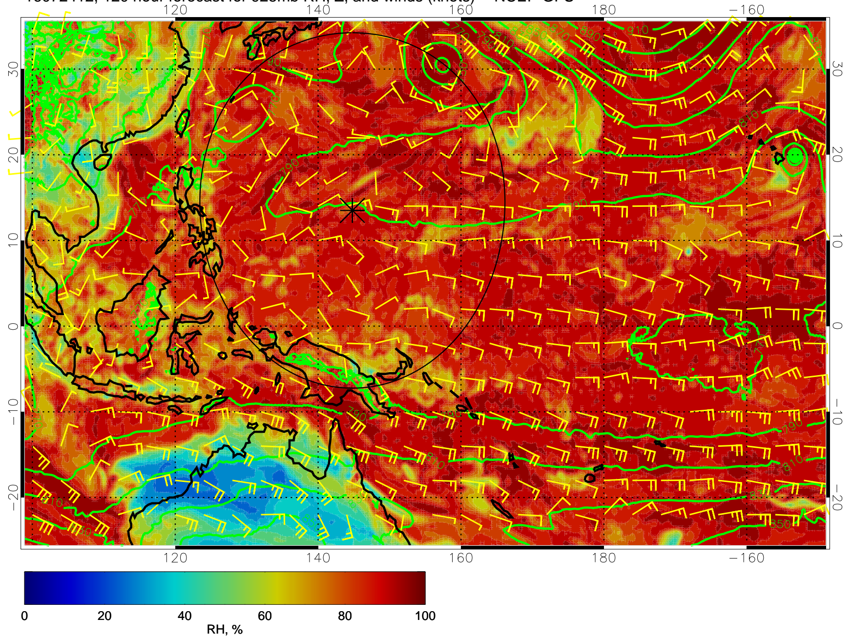
16072412, 120 hour forecast for 925mb RH, Z, and winds (knots) -- NCEP GFS
