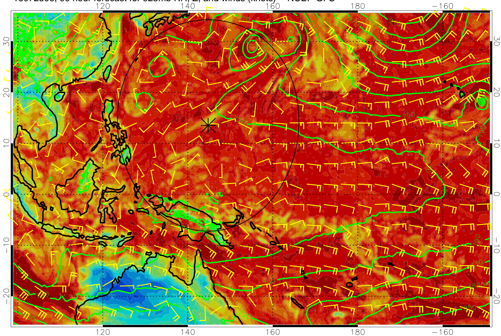
16072306, 90 hour forecast for 925mb RH, Z, and winds (knots) -- NCEP GFS
