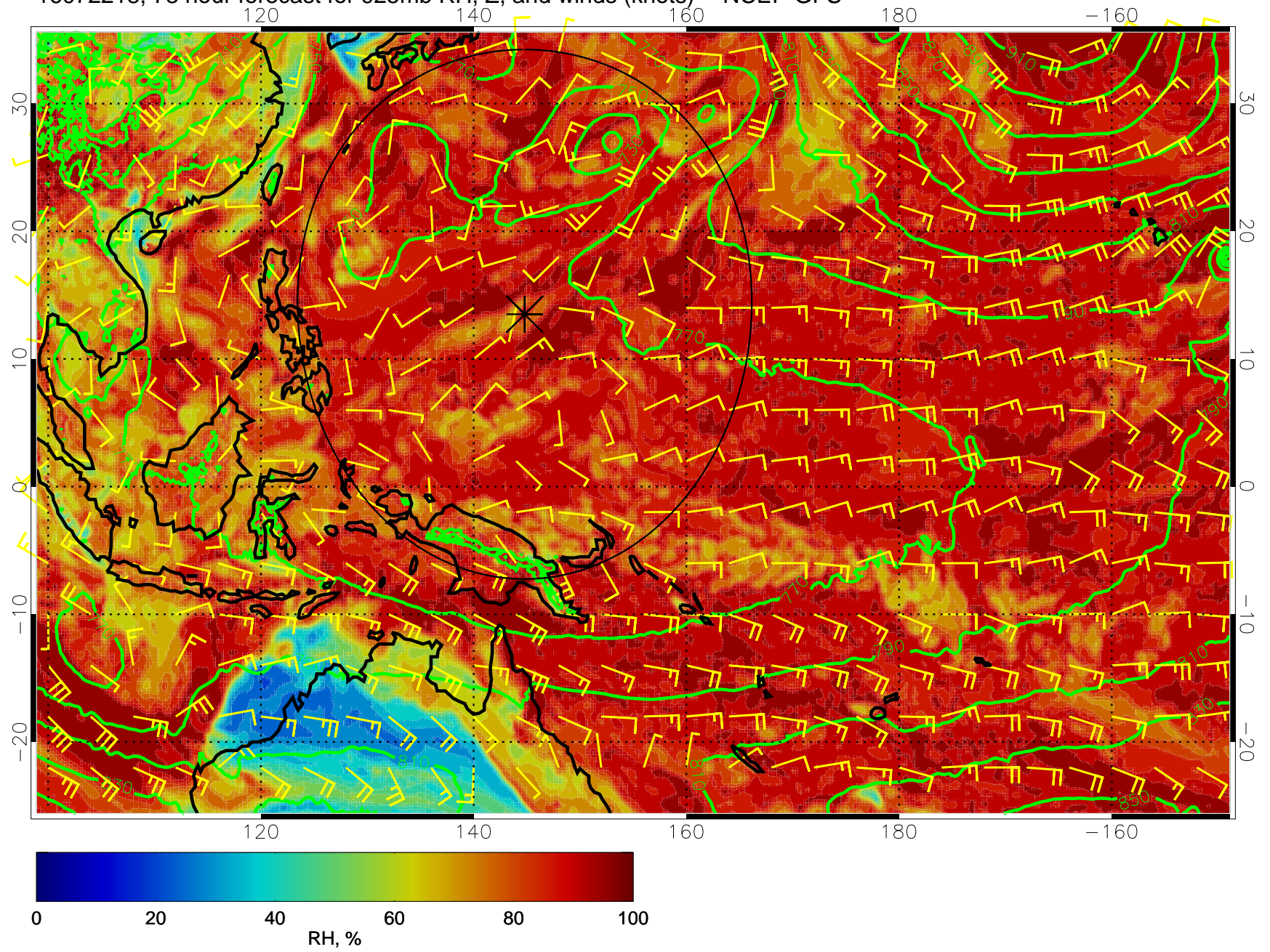
16072218, 78 hour forecast for 925mb RH, Z, and winds (knots) -- NCEP GFS
