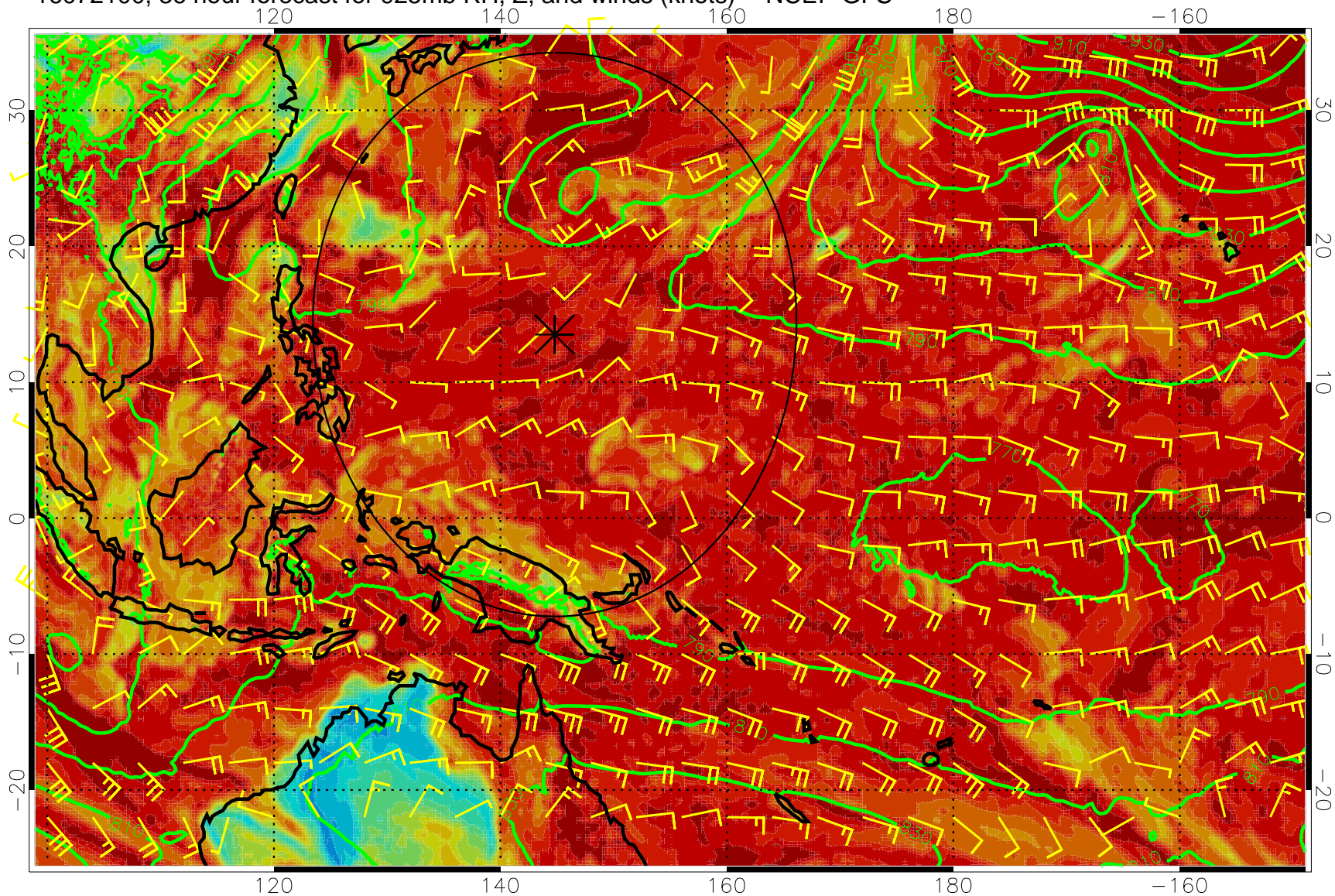
16072100, 36 hour forecast for 925mb RH, Z, and winds (knots) -- NCEP GFS
