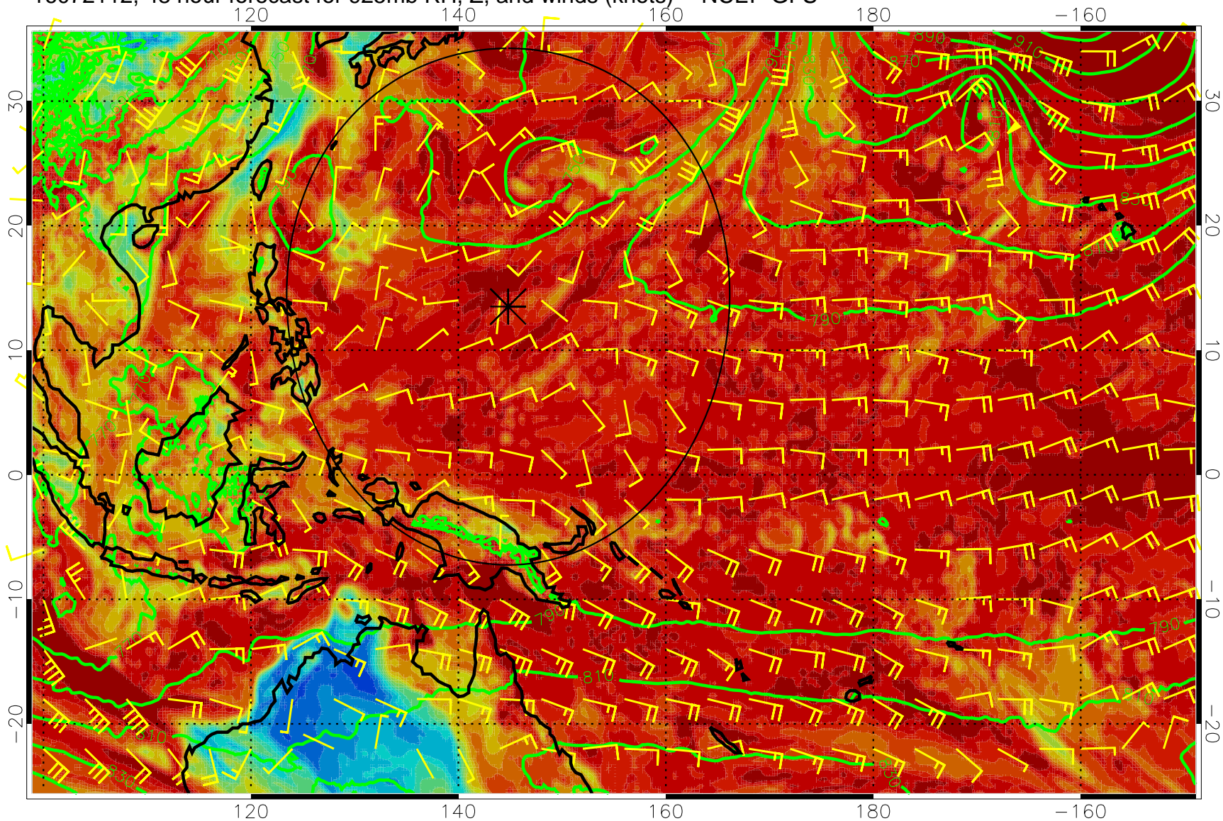
16072112, 48 hour forecast for 925mb RH, Z, and winds (knots) -- NCEP GFS
