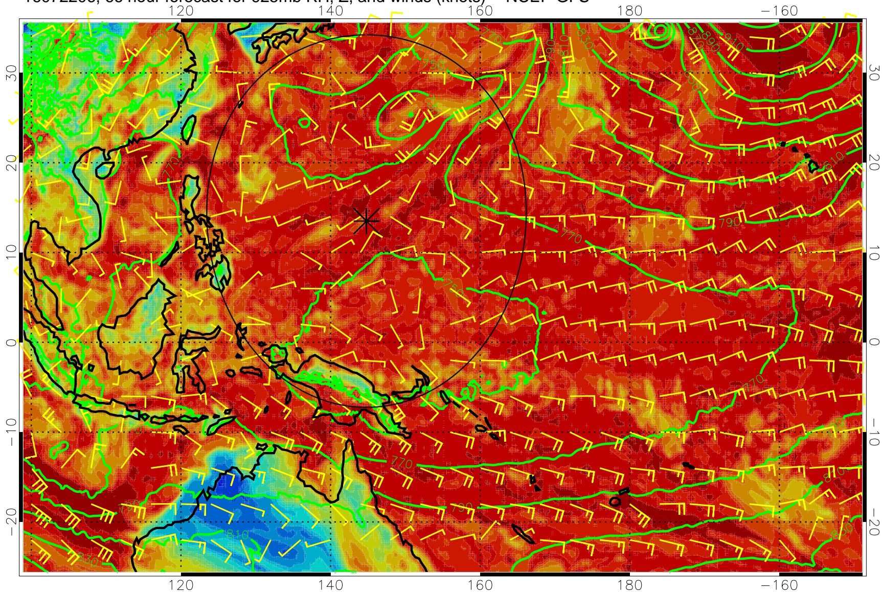
16072206, 66 hour forecast for 925mb RH, Z, and winds (knots) -- NCEP GFS
