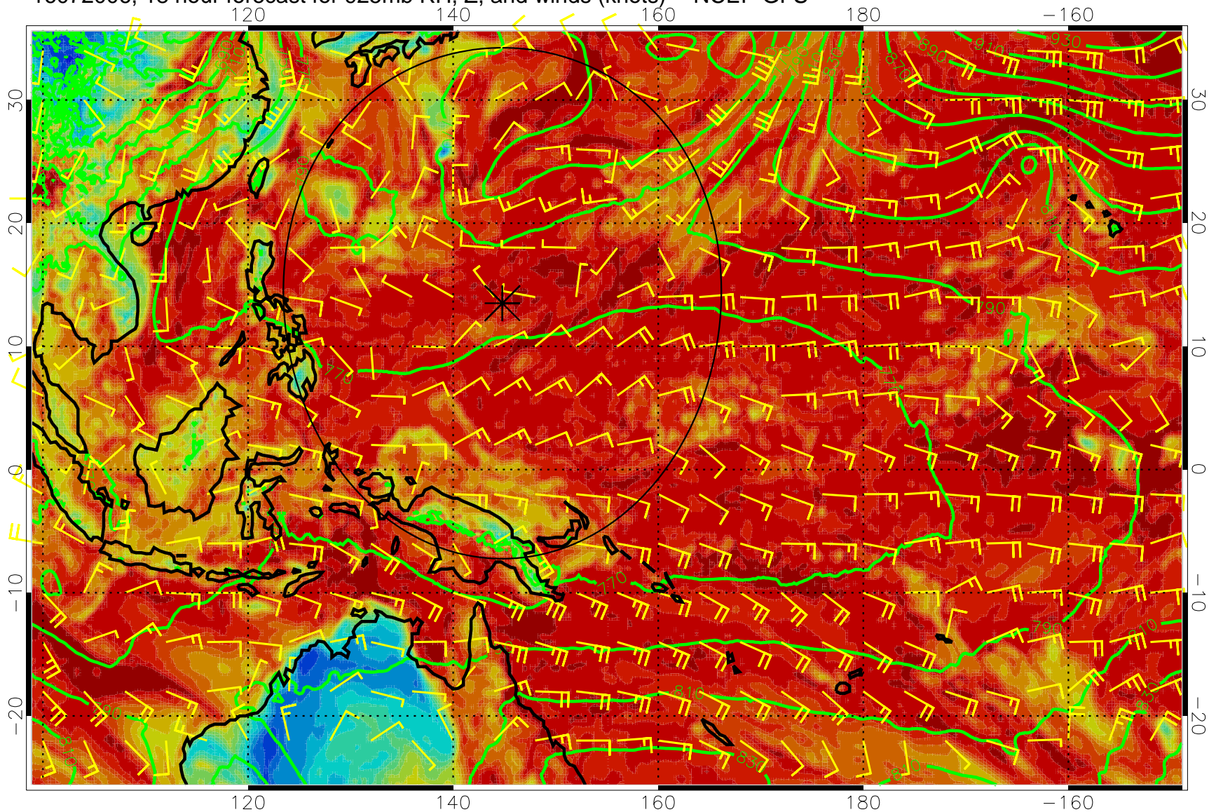
16072006, 18 hour forecast for 925mb RH, Z, and winds (knots) -- NCEP GFS
