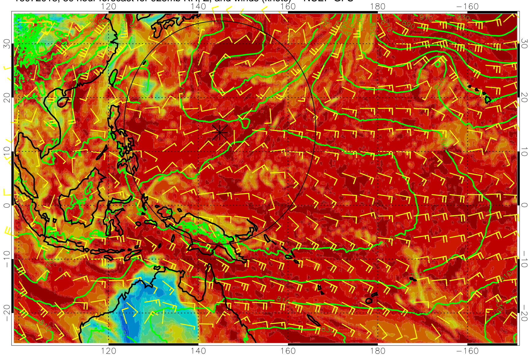
16072018, 30 hour forecast for 925mb RH, Z, and winds (knots) -- NCEP GFS
