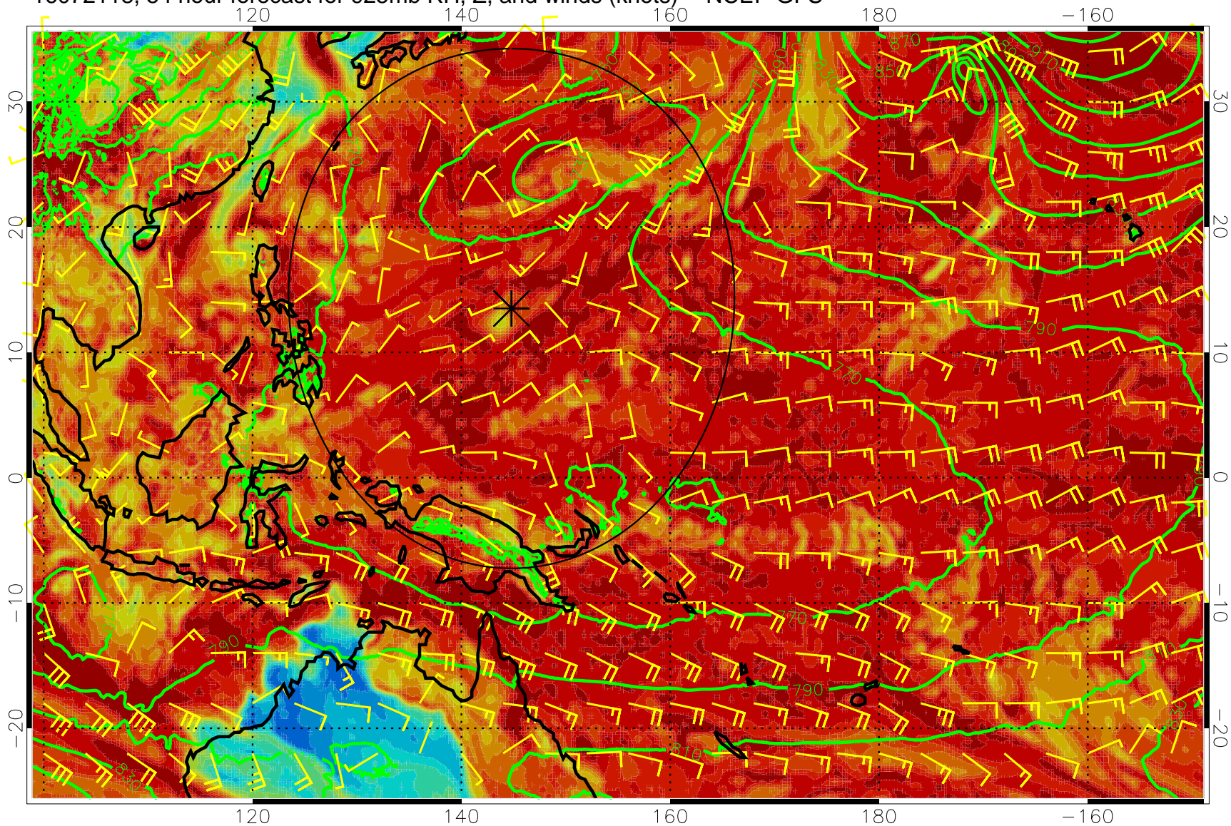
16072118, 54 hour forecast for 925mb RH, Z, and winds (knots) -- NCEP GFS
