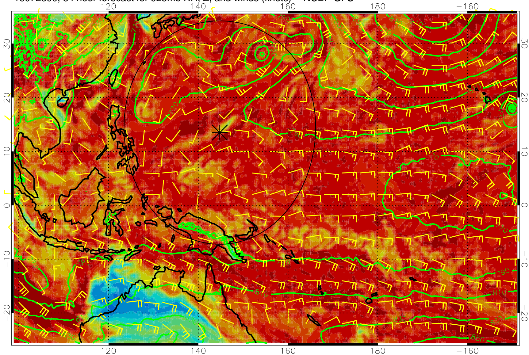
16072300, 84 hour forecast for 925mb RH, Z, and winds (knots) -- NCEP GFS
