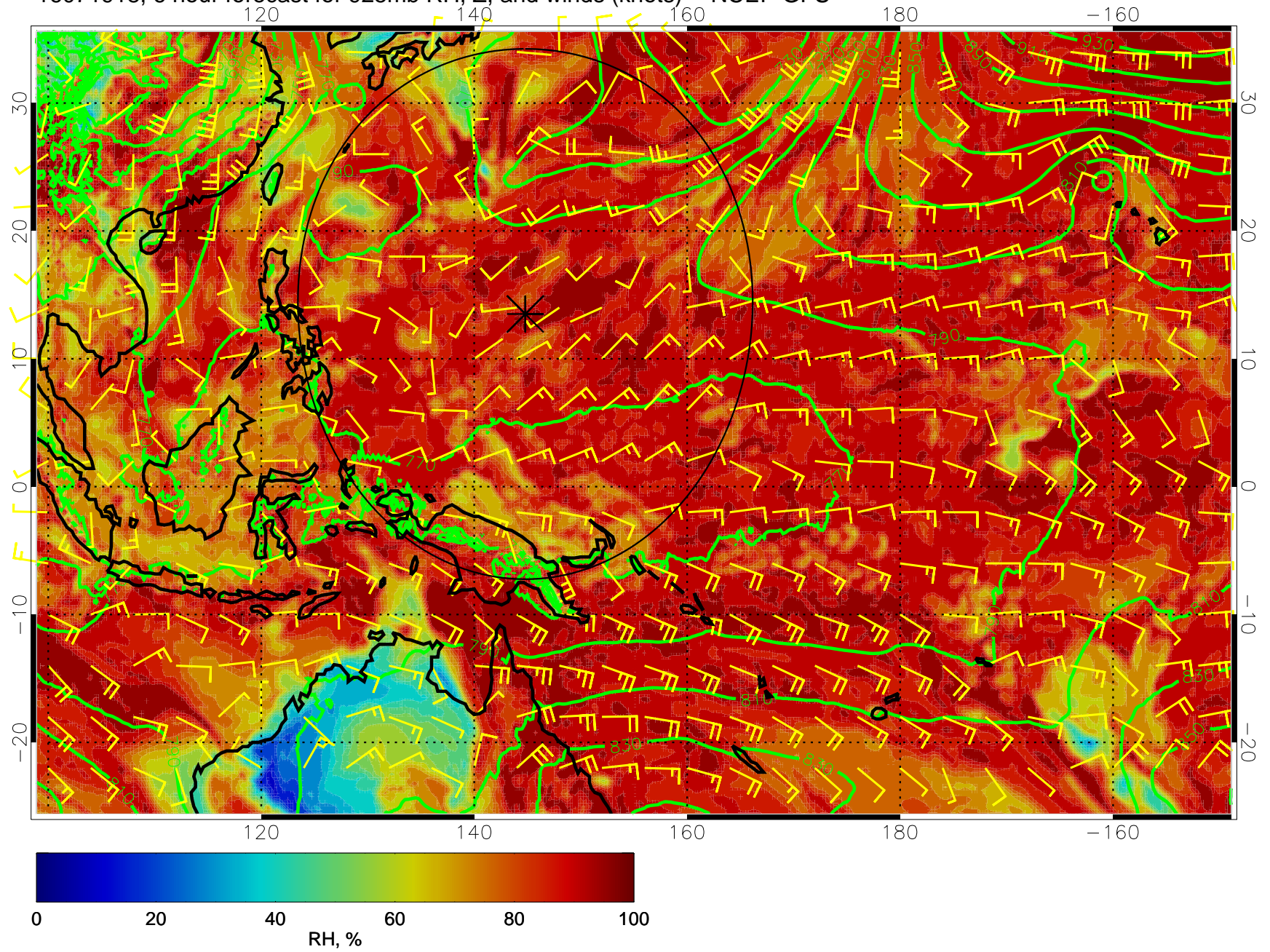
16071918, 6 hour forecast for 925mb RH, Z, and winds (knots) -- NCEP GFS
