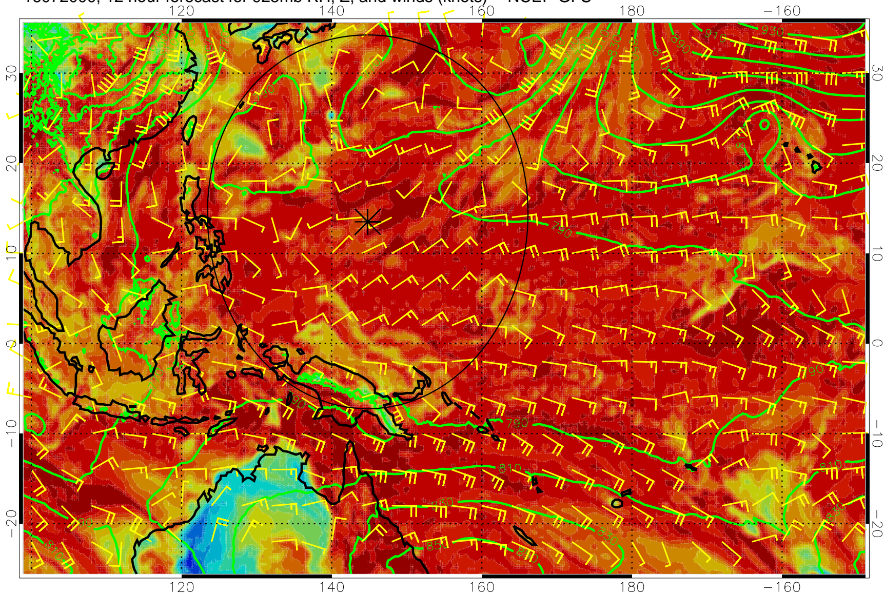
16072000, 12 hour forecast for 925mb RH, Z, and winds (knots) -- NCEP GFS
