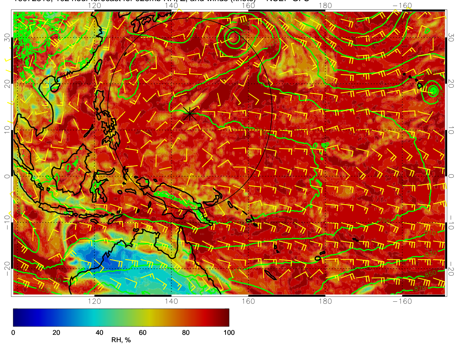
16072318, 102 hour forecast for 925mb RH, Z, and winds (knots) -- NCEP GFS
