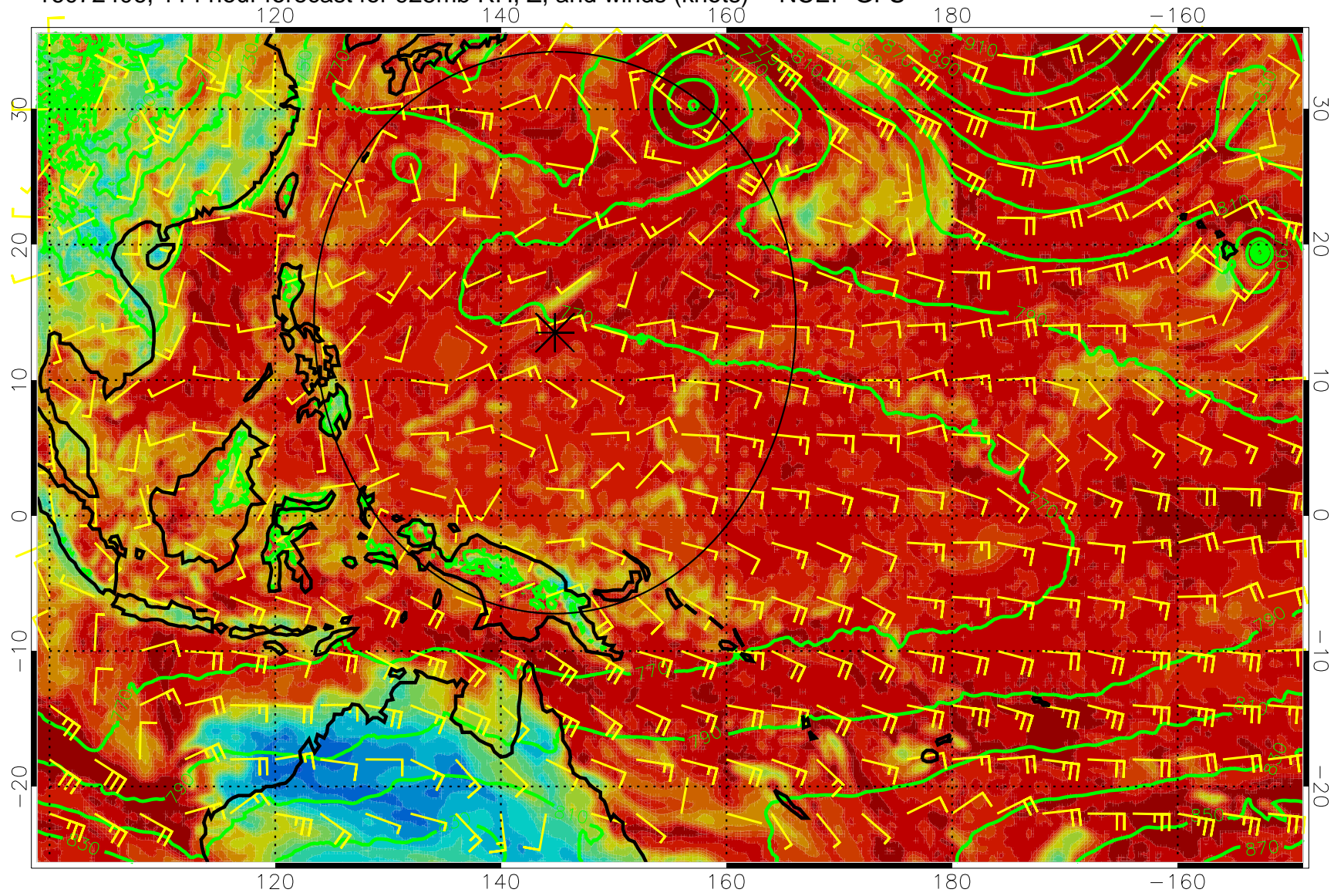
16072406, 114 hour forecast for 925mb RH, Z, and winds (knots) -- NCEP GFS
