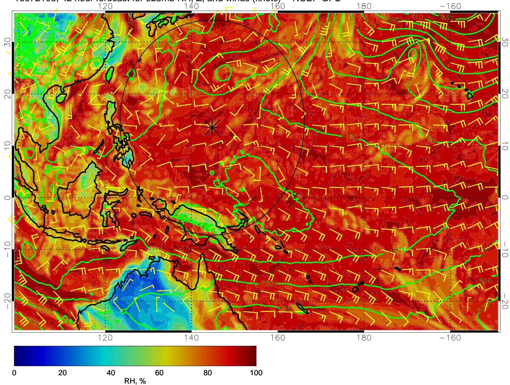
16072106, 42 hour forecast for 925mb RH, Z, and winds (knots) -- NCEP GFS
