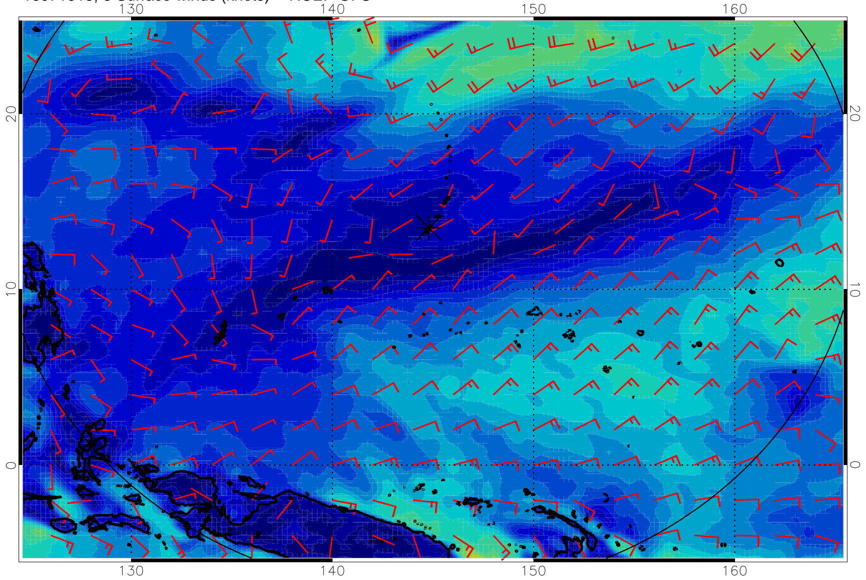
16071918, 6 Surface winds (knots) -- NCEP GFS
