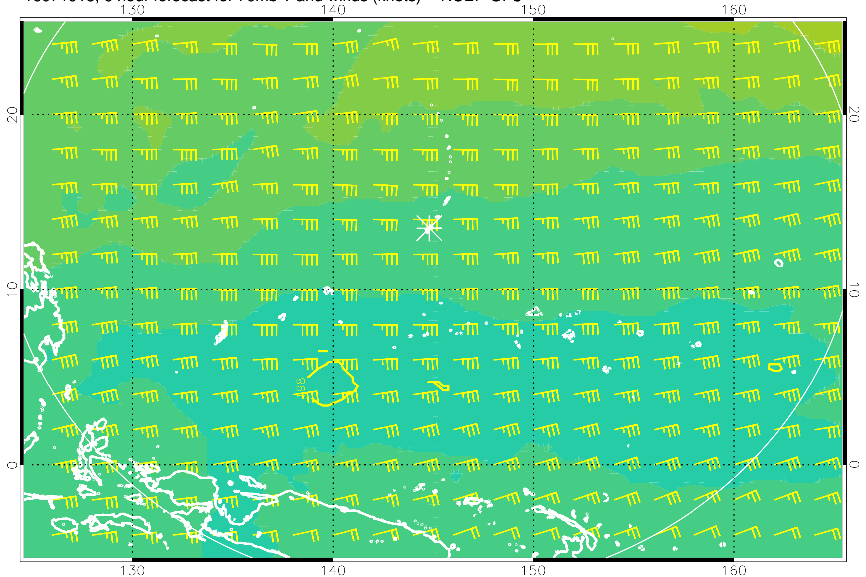
16071918, 6 hour forecast for 70mb T and winds (knots) -- NCEP GFS
