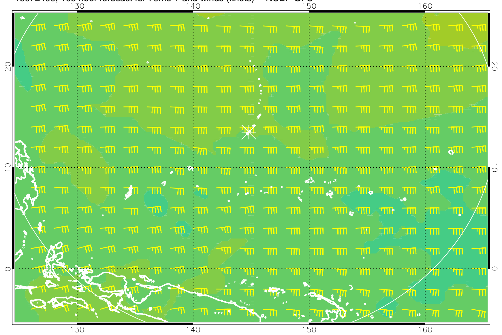
16072400, 108 hour forecast for 70mb T and winds (knots) -- NCEP GFS
