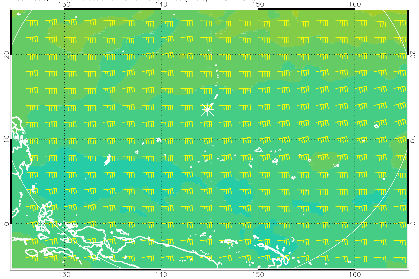
16072000, 12 hour forecast for 70mb T and winds (knots) -- NCEP GFS
