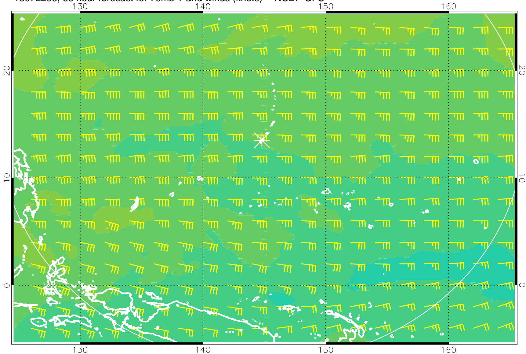
16072206, 66 hour forecast for 70mb T and winds (knots) -- NCEP GFS
