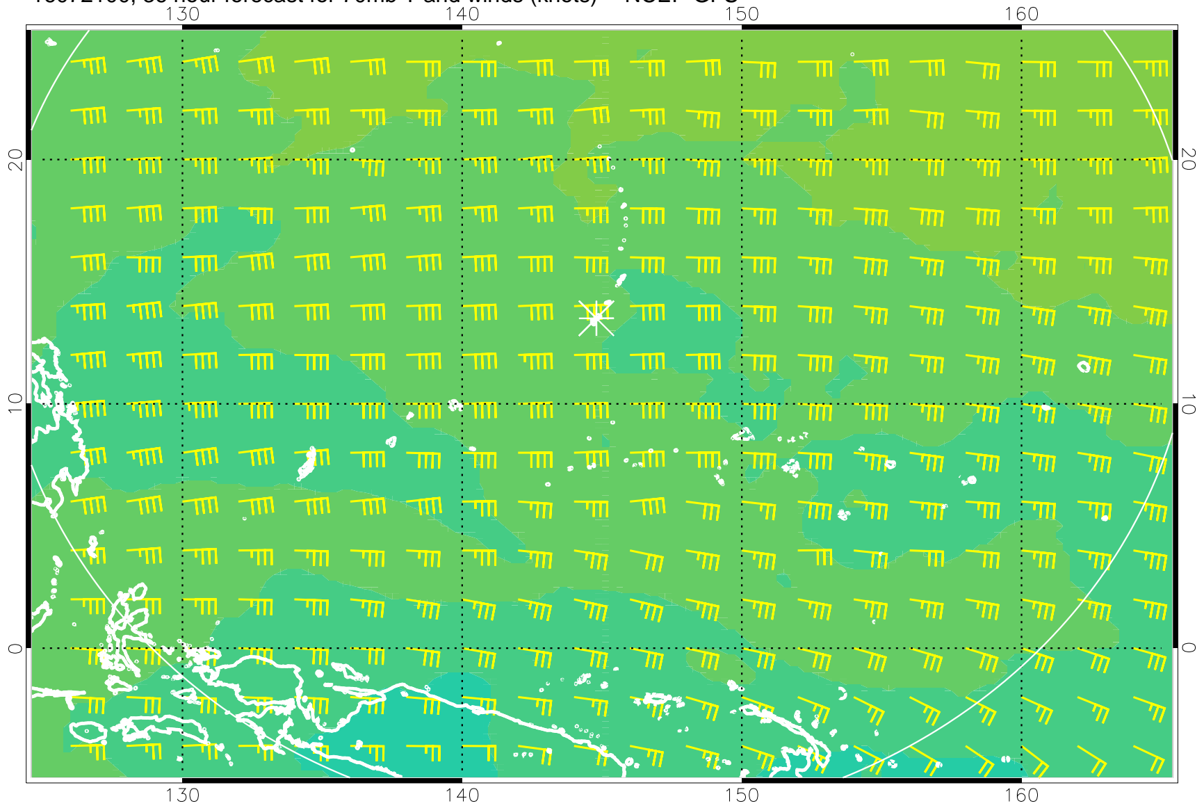
16072100, 36 hour forecast for 70mb T and winds (knots) -- NCEP GFS
