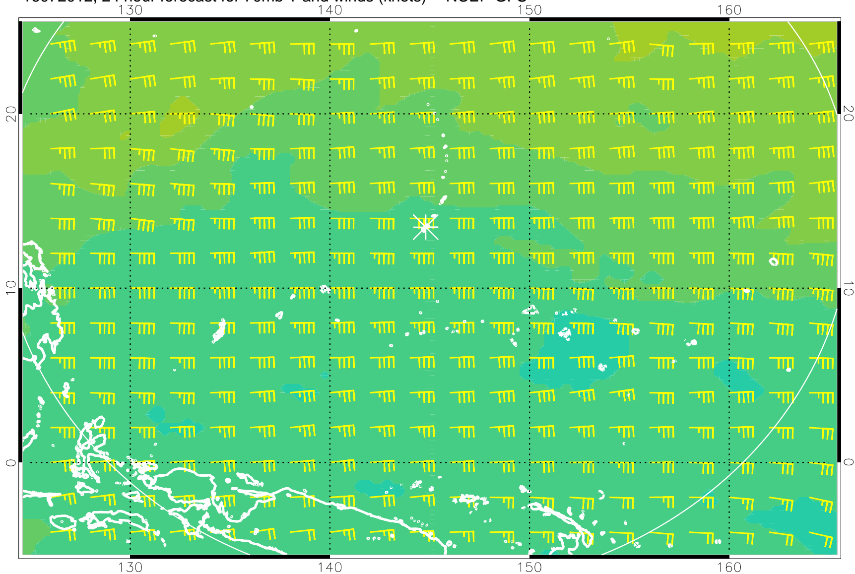
16072012, 24 hour forecast for 70mb T and winds (knots) -- NCEP GFS
