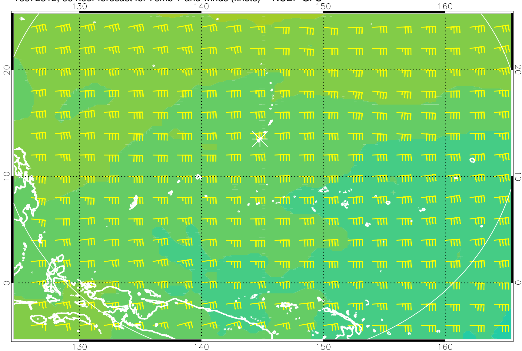
16072312, 96 hour forecast for 70mb T and winds (knots) -- NCEP GFS
