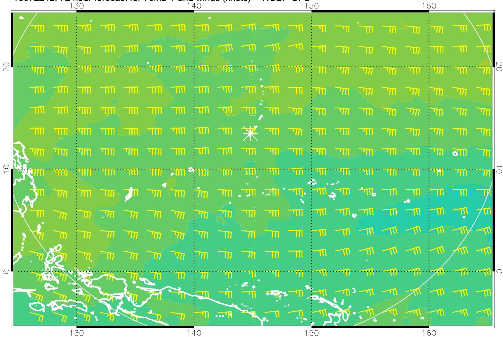
16072212, 72 hour forecast for 70mb T and winds (knots) -- NCEP GFS
