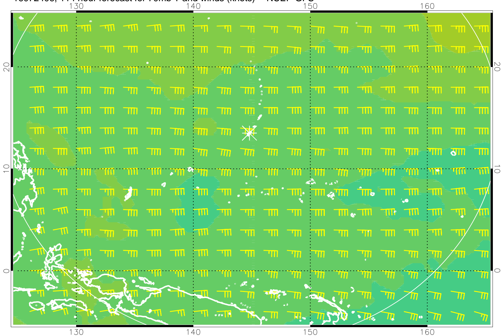
16072406, 114 hour forecast for 70mb T and winds (knots) -- NCEP GFS
