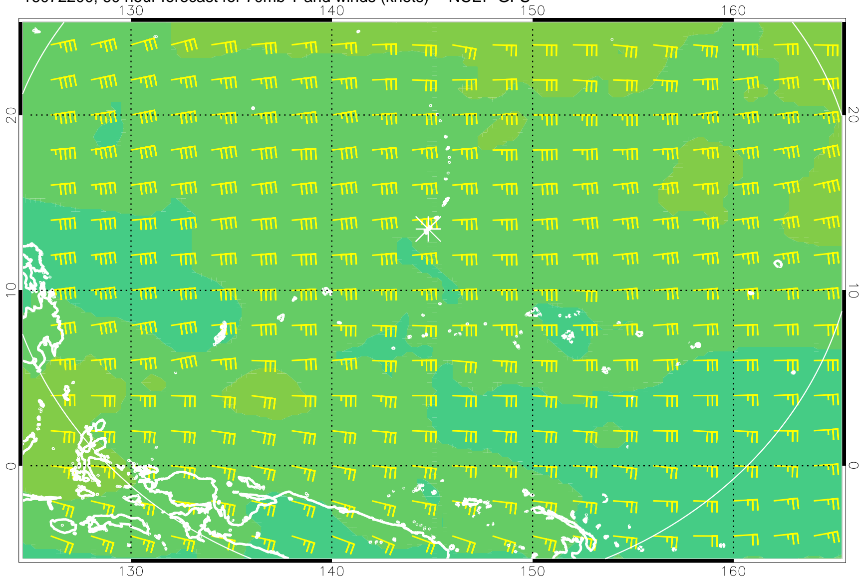
16072200, 60 hour forecast for 70mb T and winds (knots) -- NCEP GFS
