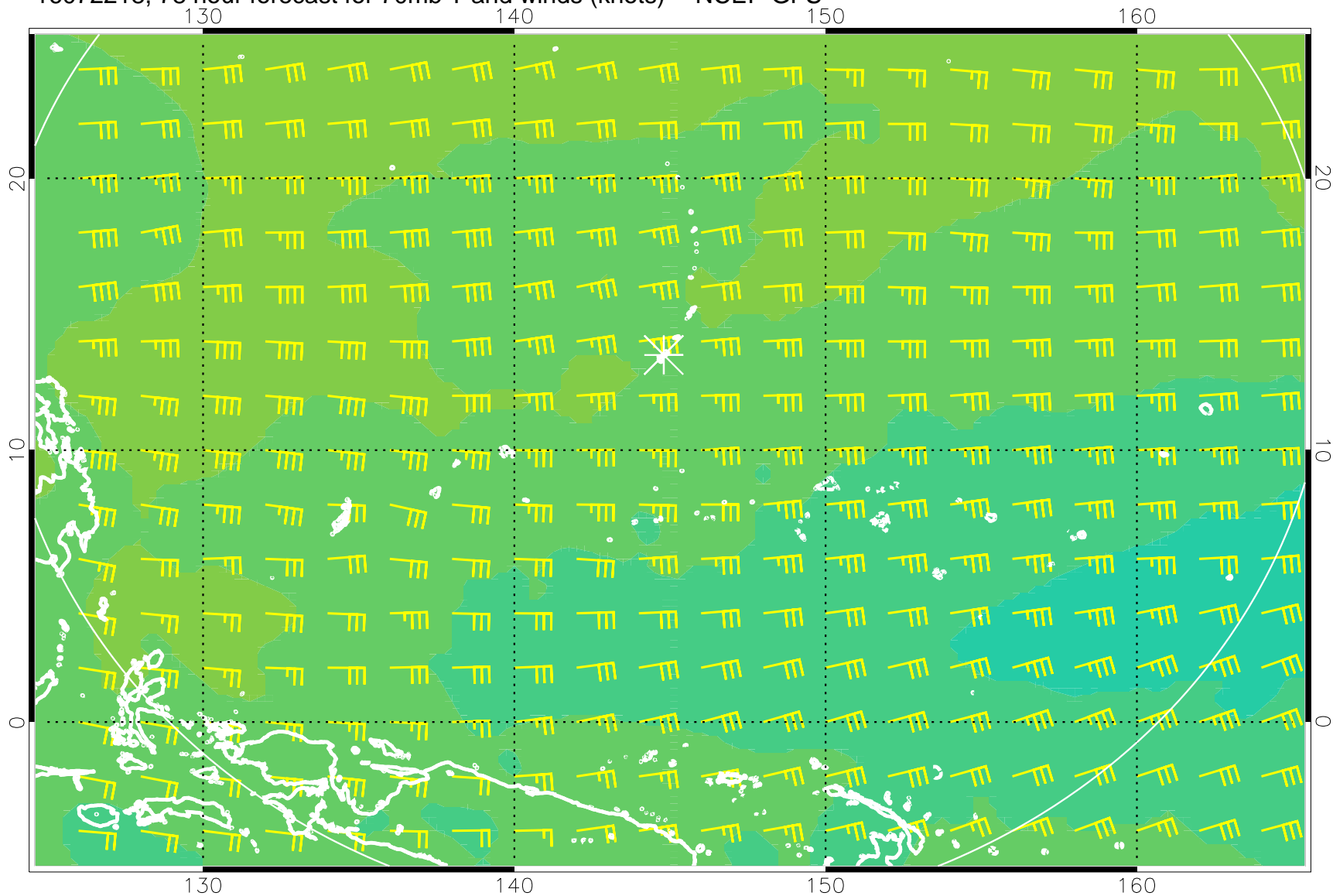
16072218, 78 hour forecast for 70mb T and winds (knots) -- NCEP GFS
