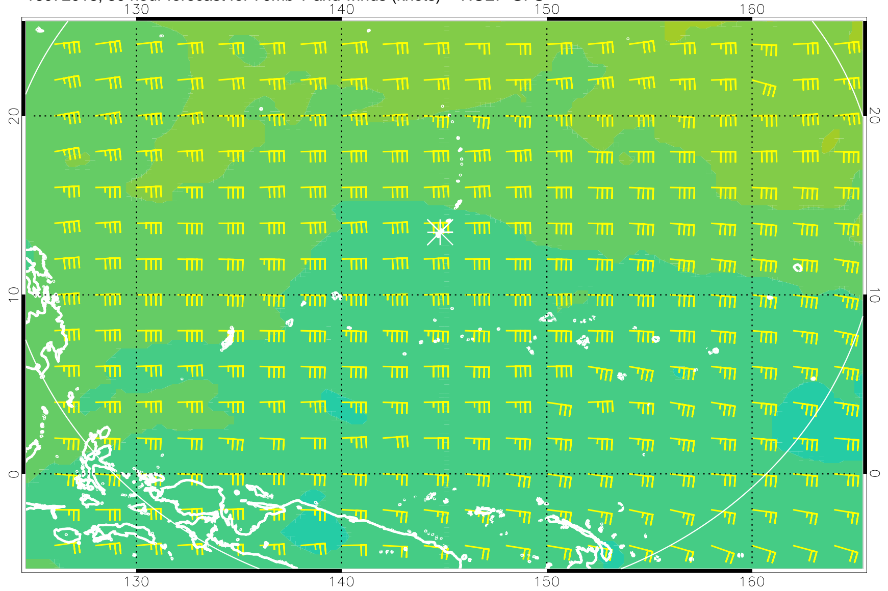
16072018, 30 hour forecast for 70mb T and winds (knots) -- NCEP GFS
