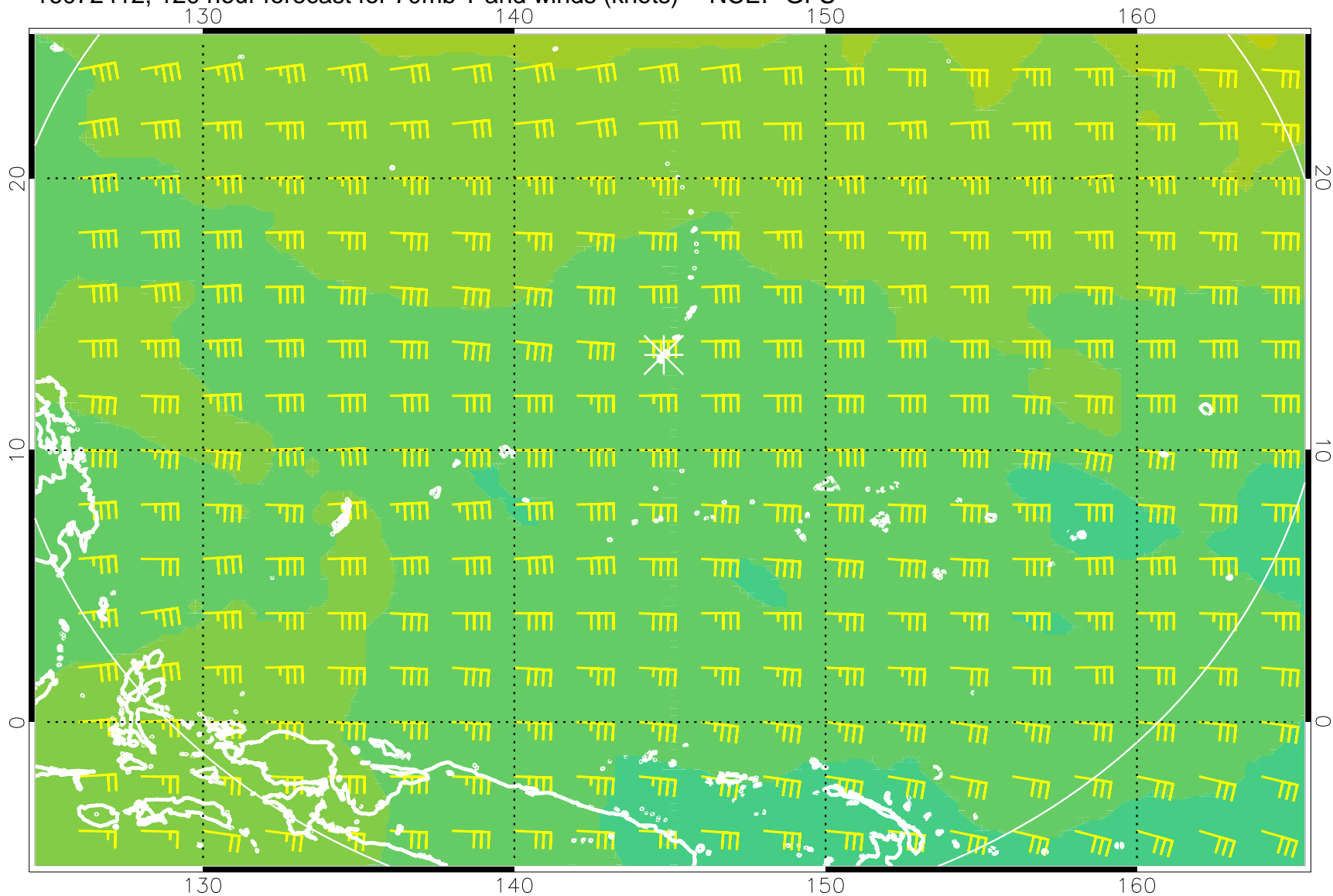
16072412, 120 hour forecast for 70mb T and winds (knots) -- NCEP GFS
