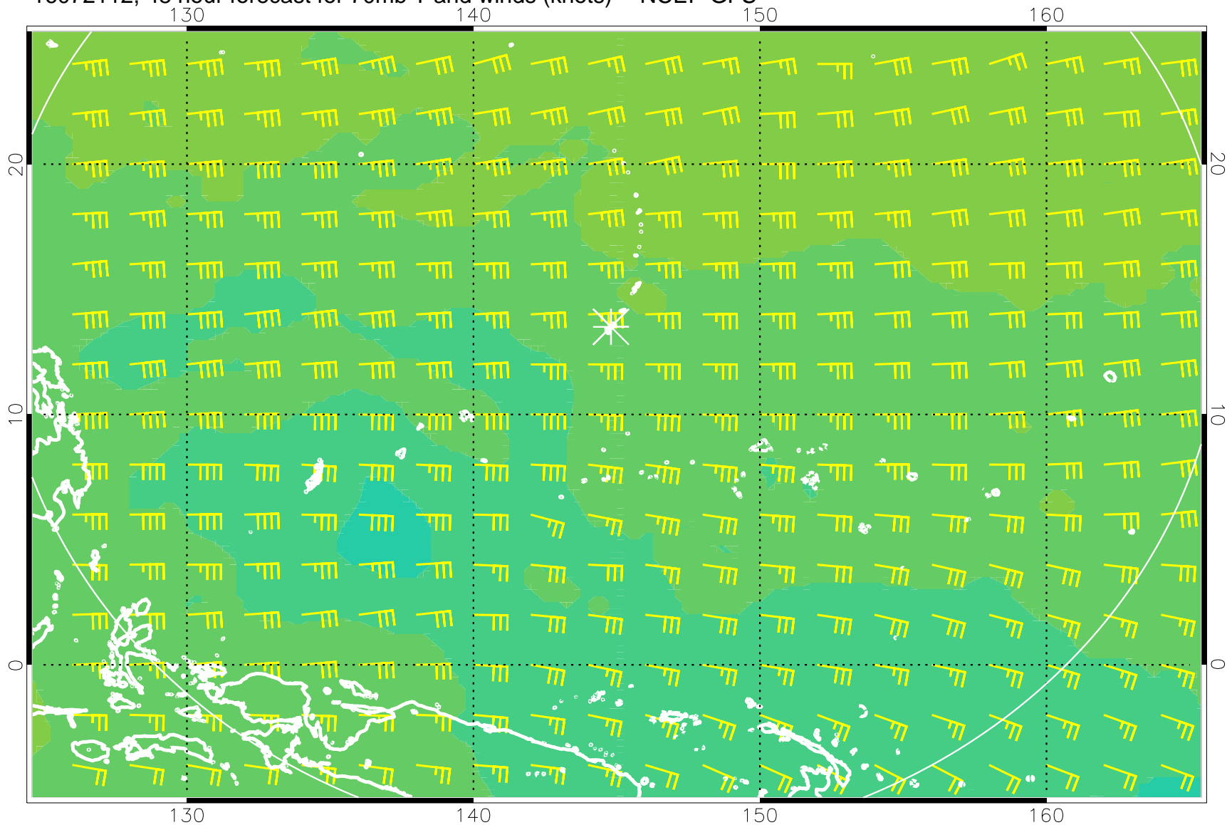
16072112, 48 hour forecast for 70mb T and winds (knots) -- NCEP GFS
