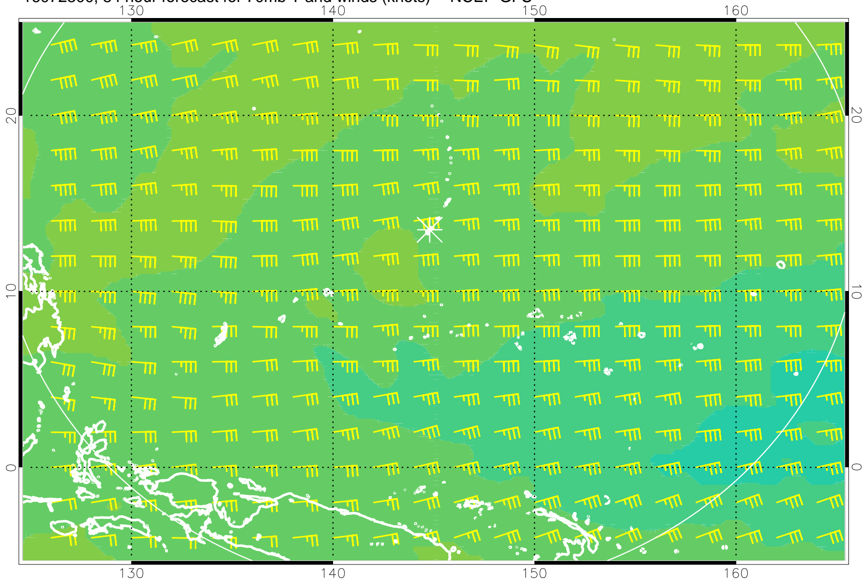
16072300, 84 hour forecast for 70mb T and winds (knots) -- NCEP GFS
