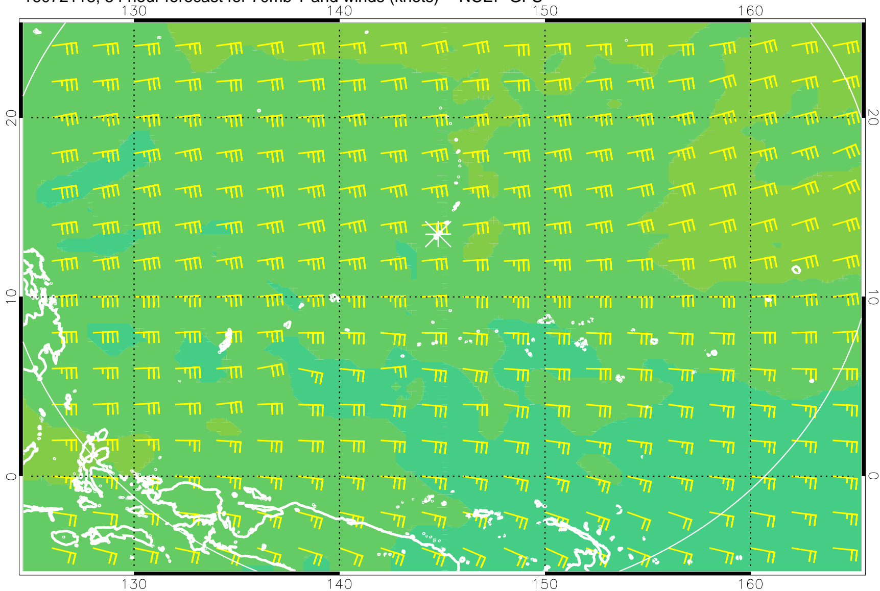
16072118, 54 hour forecast for 70mb T and winds (knots) -- NCEP GFS
