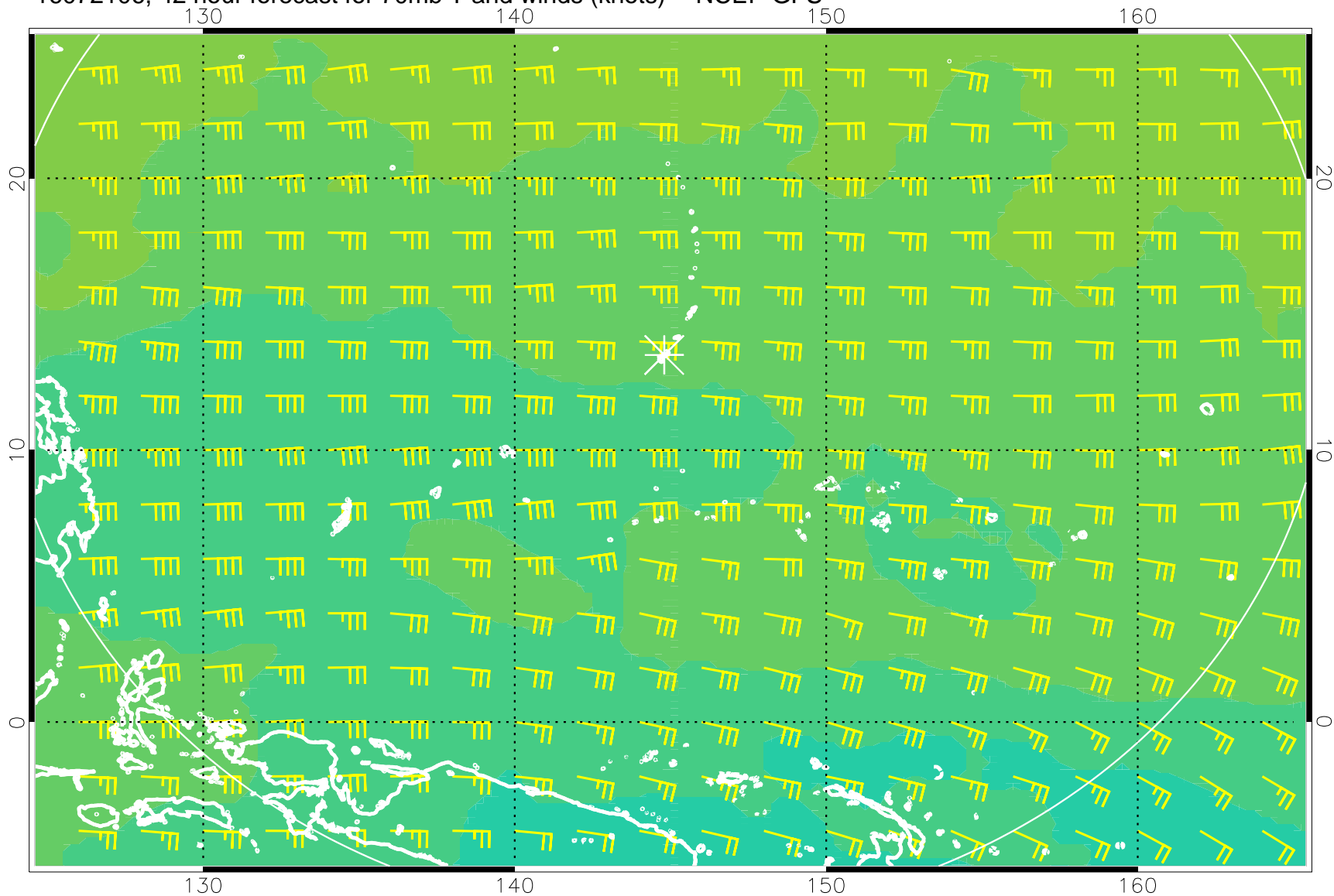
16072106, 42 hour forecast for 70mb T and winds (knots) -- NCEP GFS
