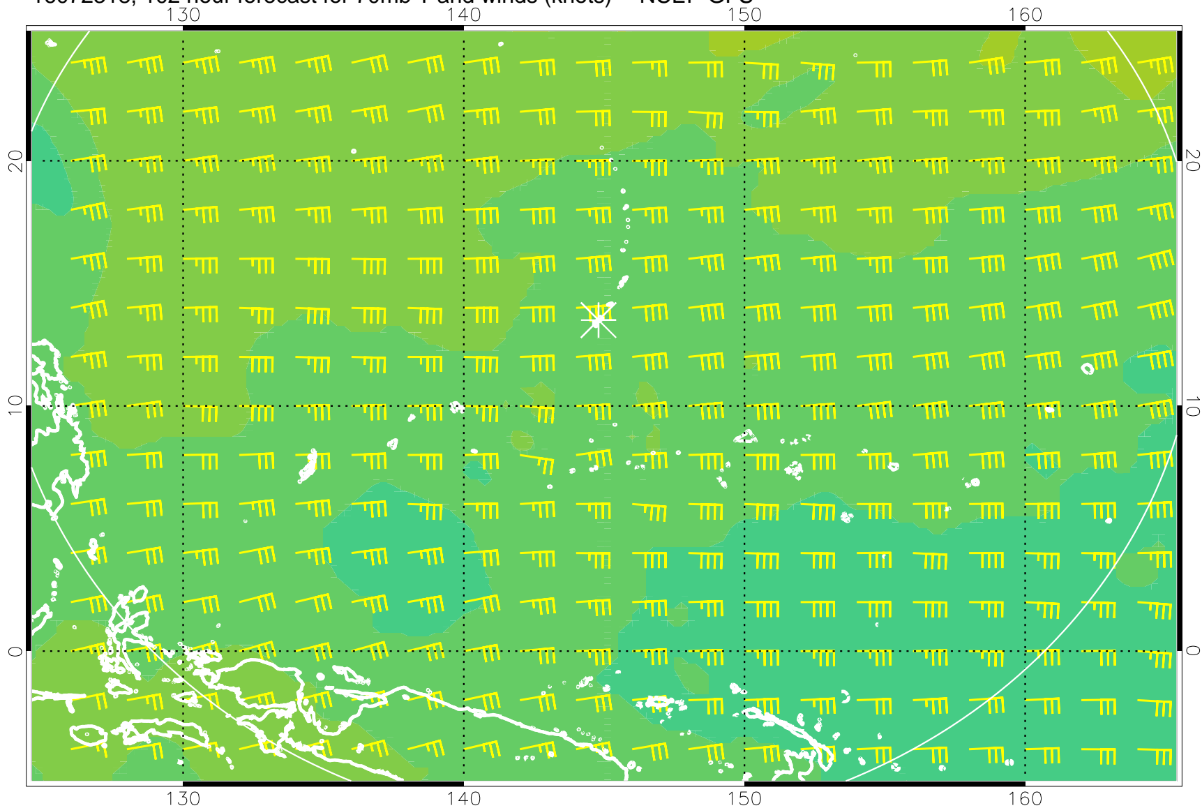
16072318, 102 hour forecast for 70mb T and winds (knots) -- NCEP GFS
