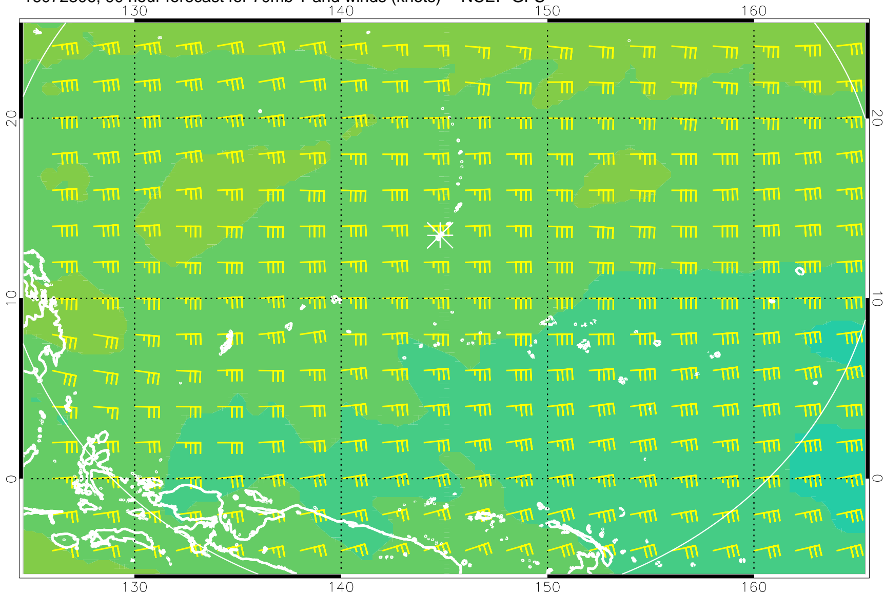
16072306, 90 hour forecast for 70mb T and winds (knots) -- NCEP GFS
