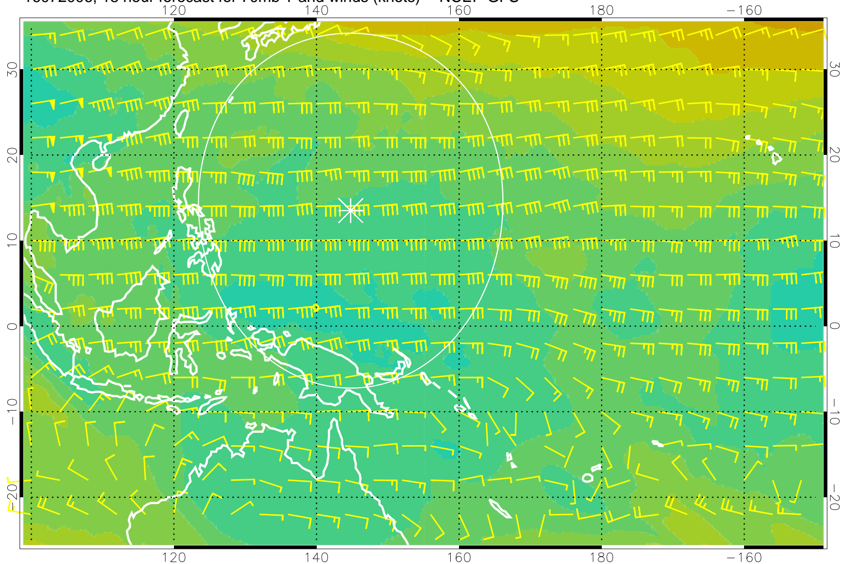
16072006, 18 hour forecast for 70mb T and winds (knots) -- NCEP GFS
