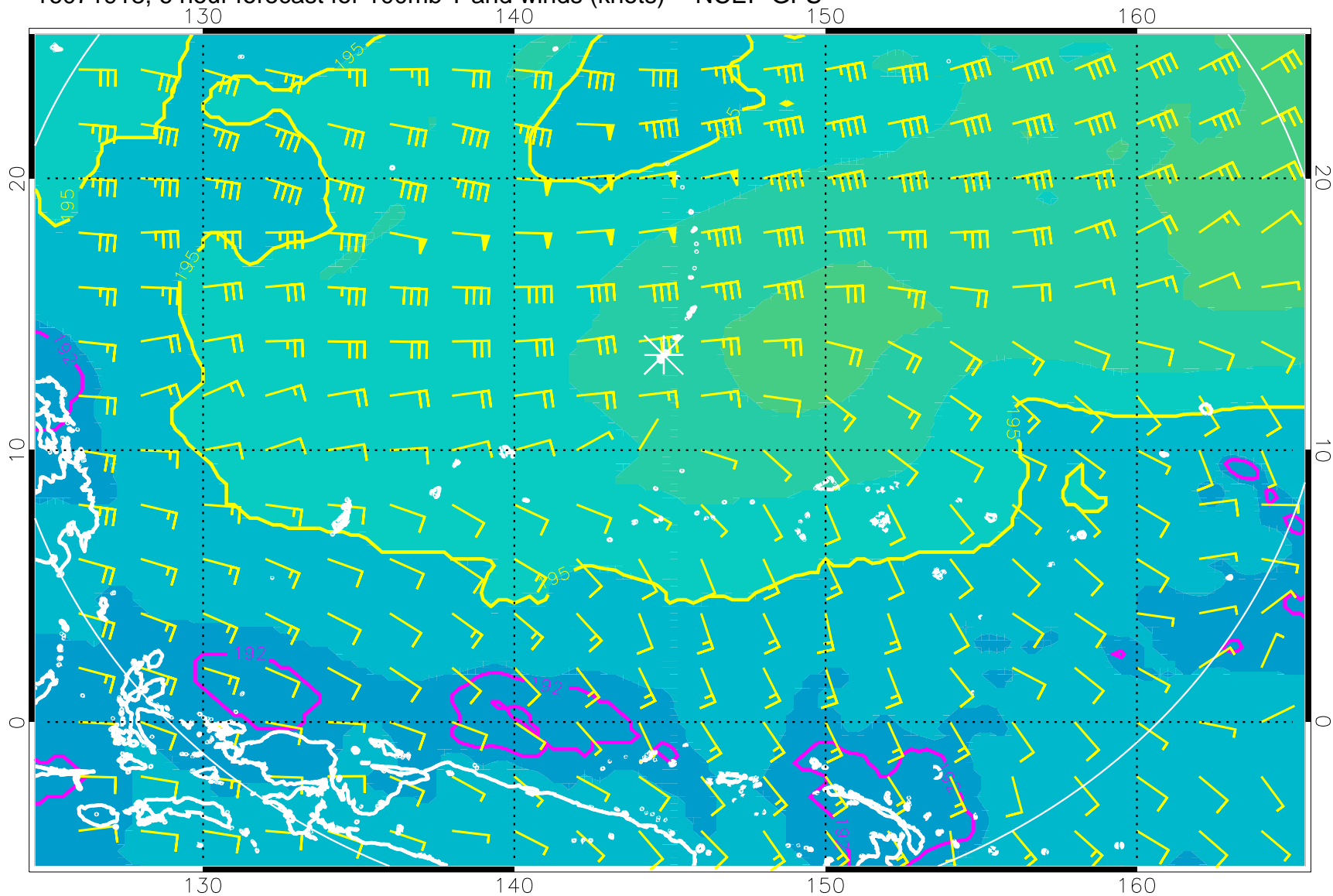
16071918, 6 hour forecast for 100mb T and winds (knots) -- NCEP GFS
