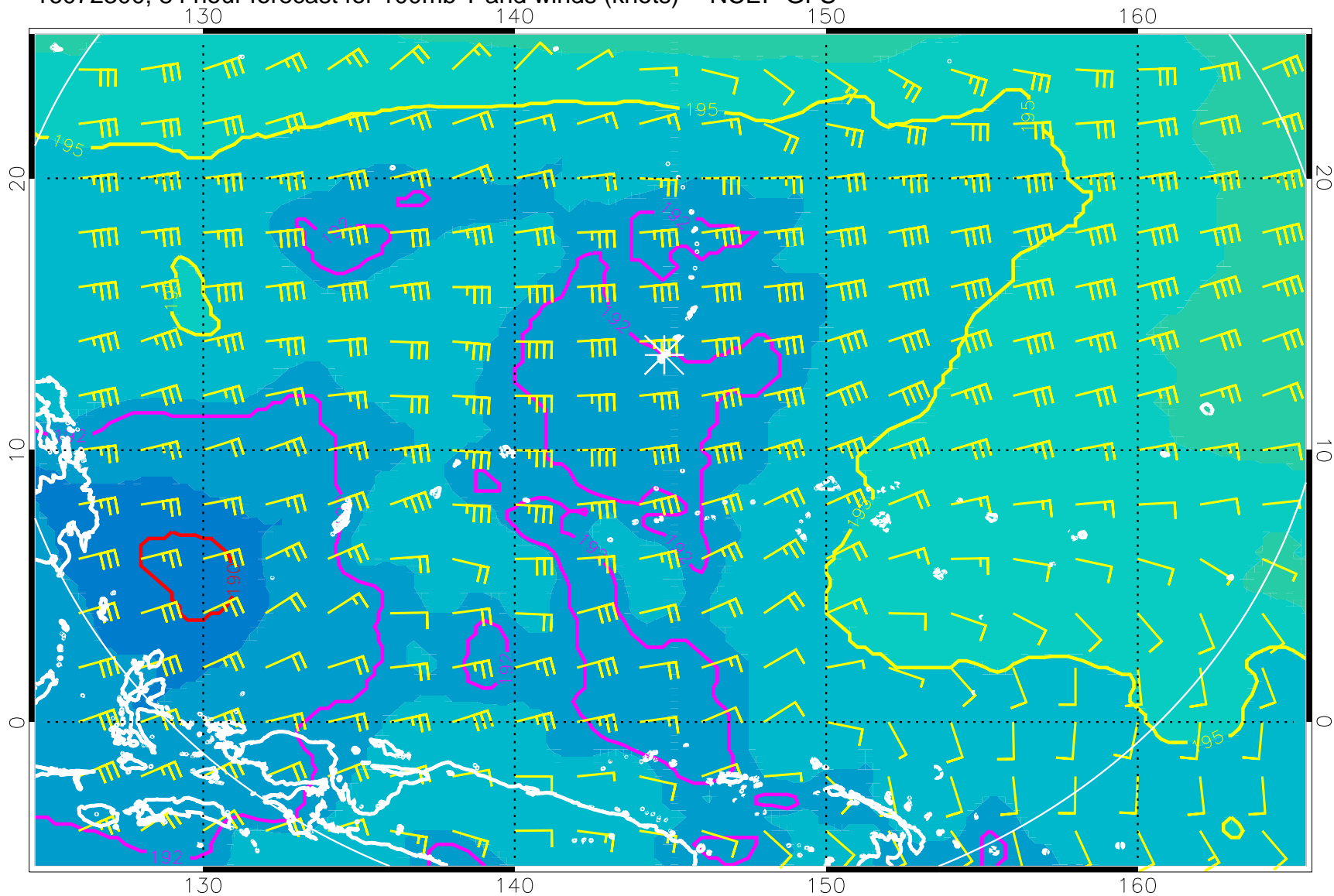
16072300, 84 hour forecast for 100mb T and winds (knots) -- NCEP GFS
