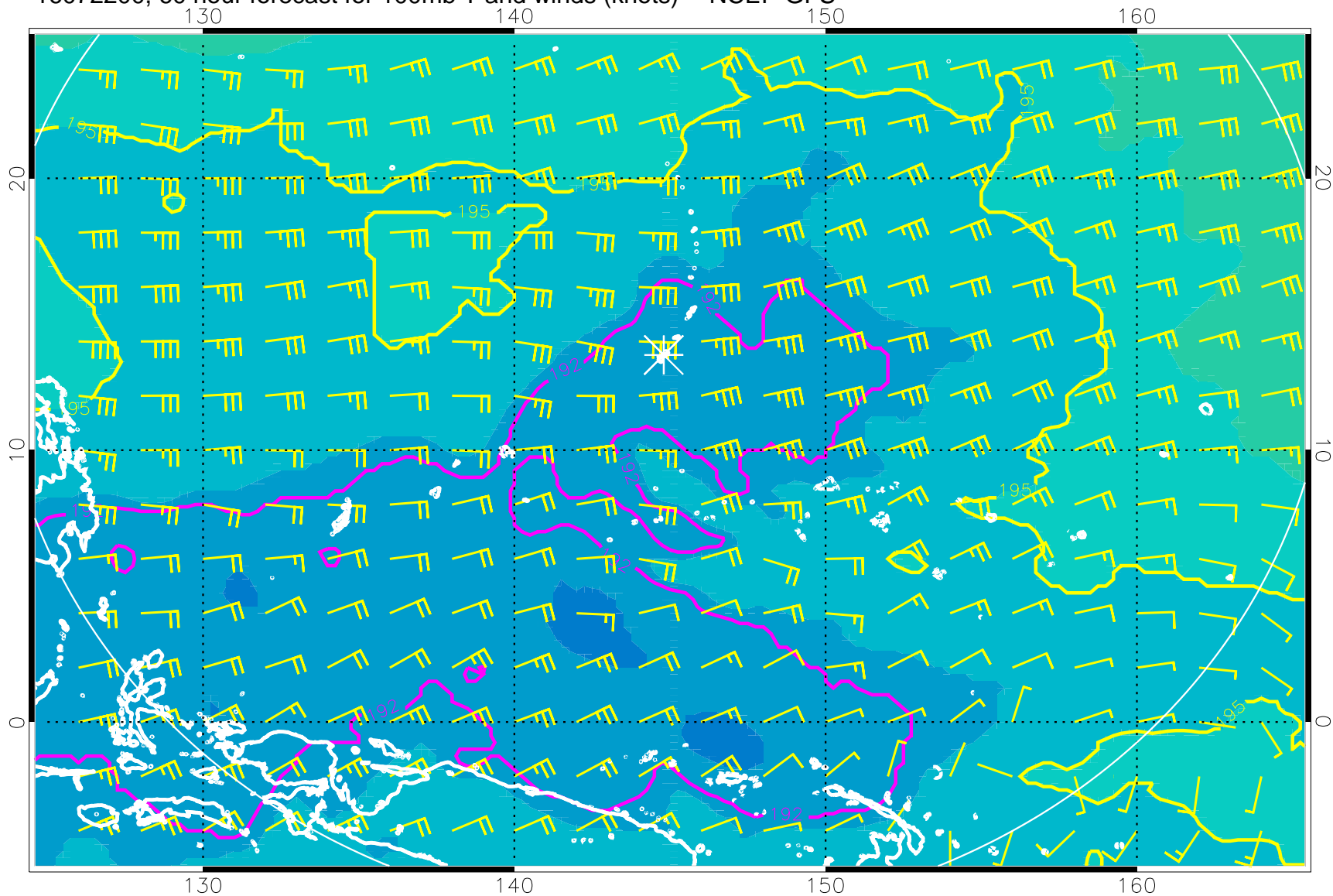
16072200, 60 hour forecast for 100mb T and winds (knots) -- NCEP GFS
