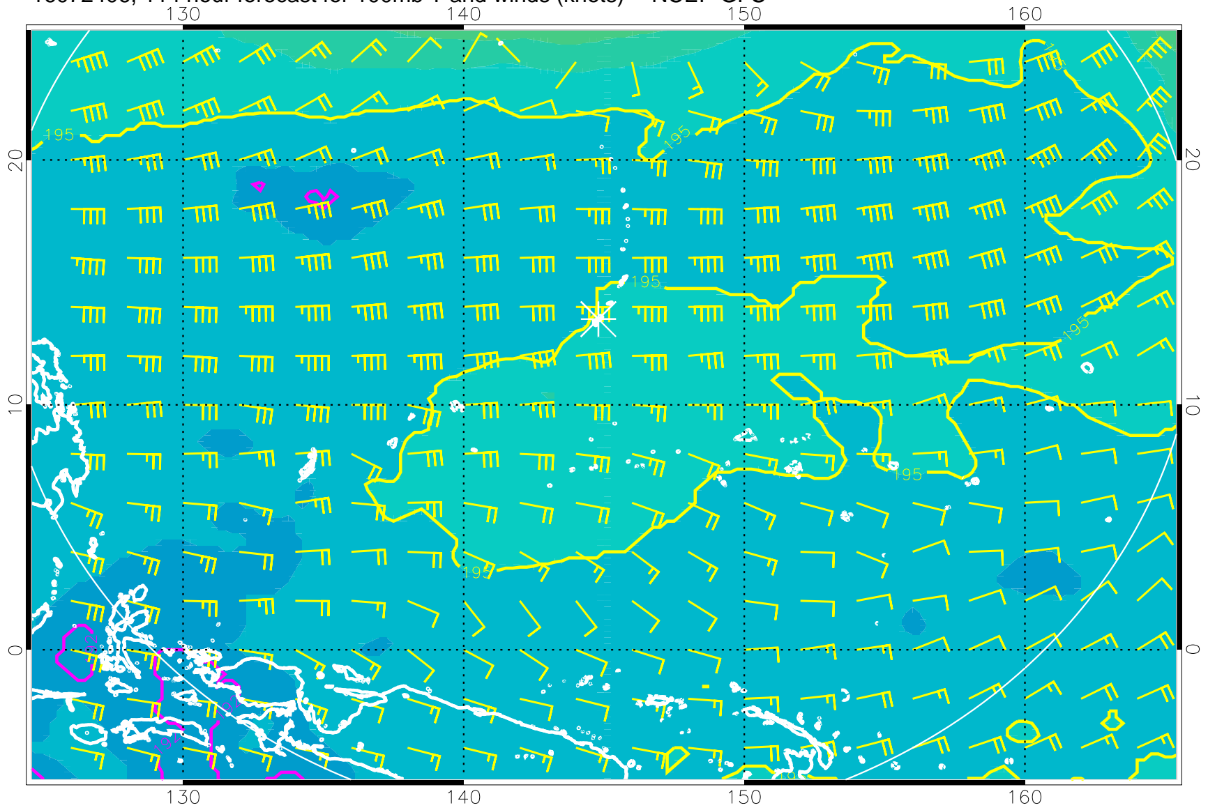
16072406, 114 hour forecast for 100mb T and winds (knots) -- NCEP GFS
