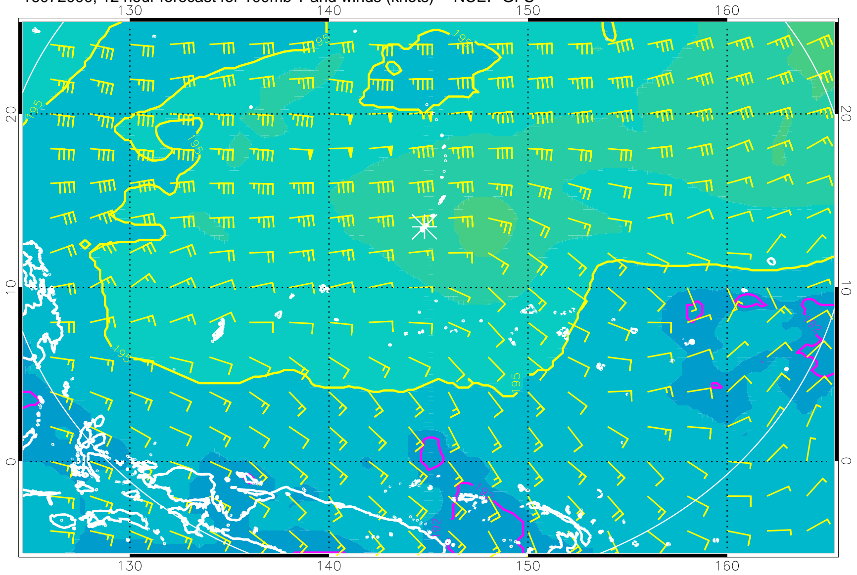
16072000, 12 hour forecast for 100mb T and winds (knots) -- NCEP GFS
