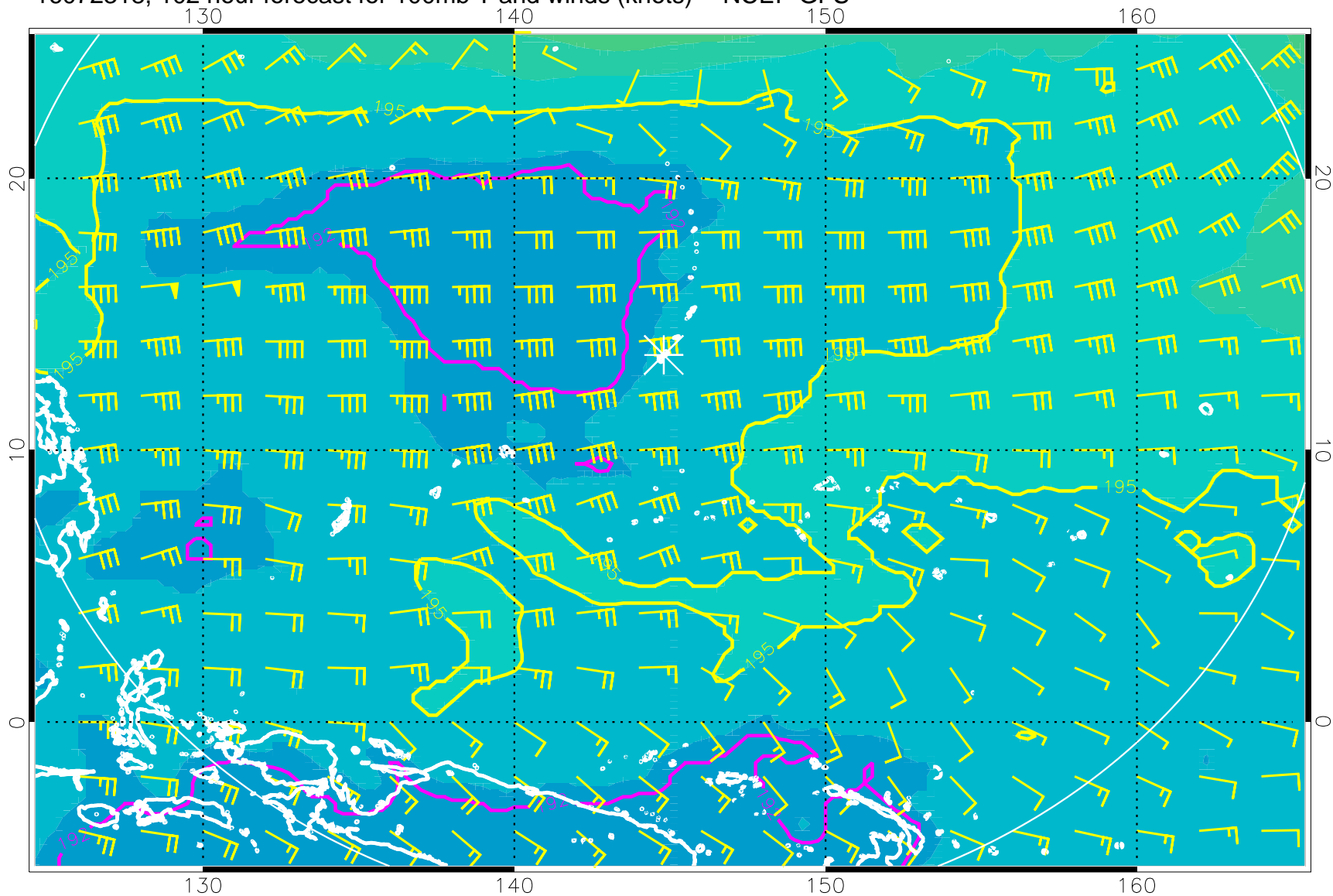
16072318, 102 hour forecast for 100mb T and winds (knots) -- NCEP GFS
