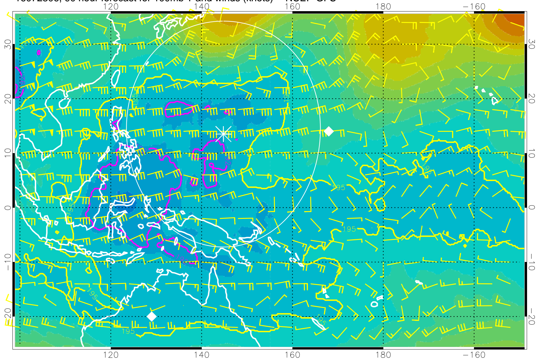
16072306, 90 hour forecast for 100mb T and winds (knots) -- NCEP GFS
