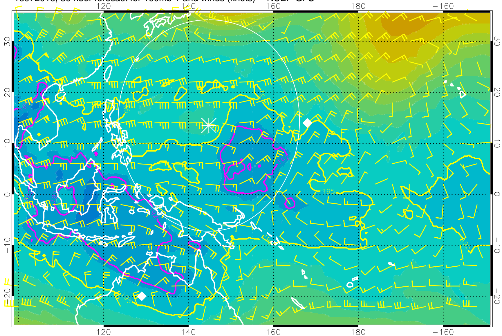
16072018, 30 hour forecast for 100mb T and winds (knots) -- NCEP GFS
