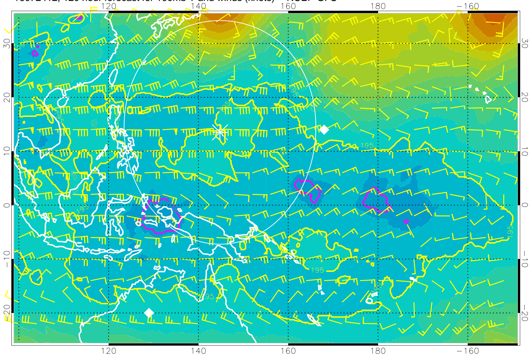
16072412, 120 hour forecast for 100mb T and winds (knots) -- NCEP GFS
