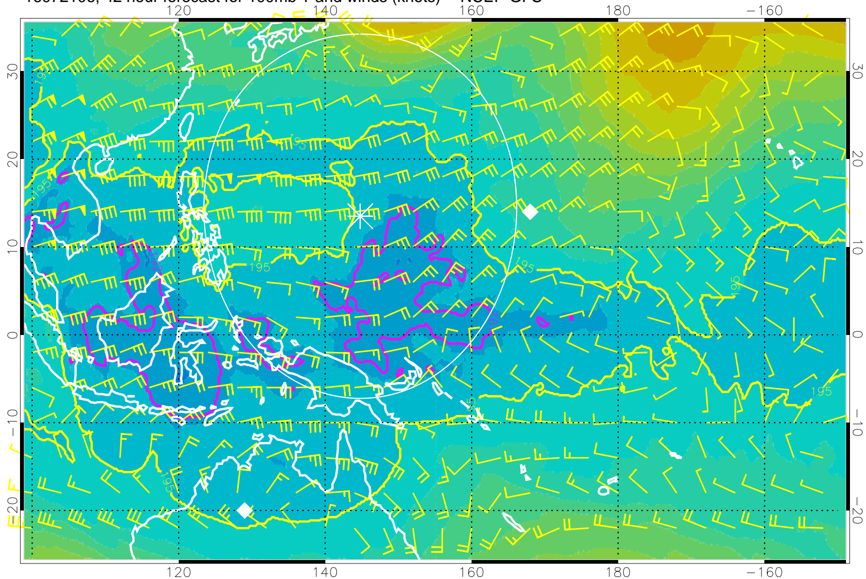
16072106, 42 hour forecast for 100mb T and winds (knots) -- NCEP GFS
