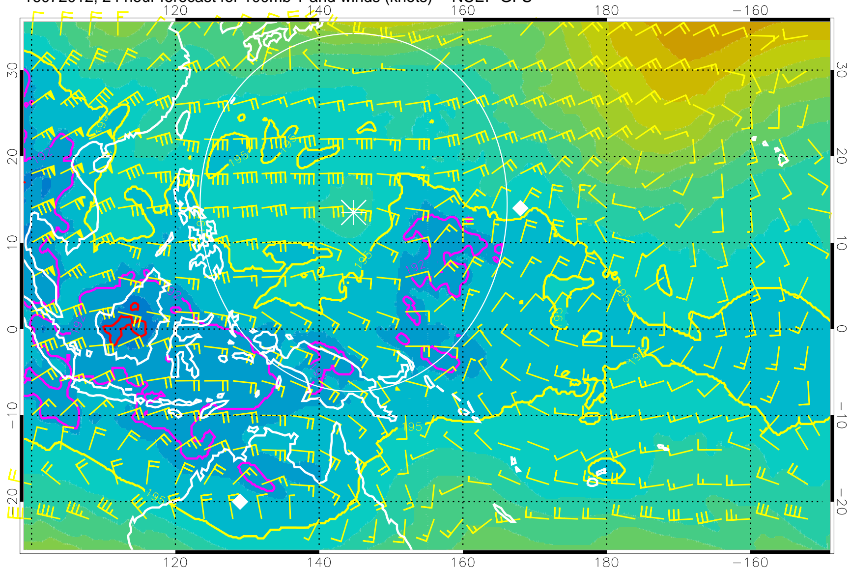
16072012, 24 hour forecast for 100mb T and winds (knots) -- NCEP GFS
