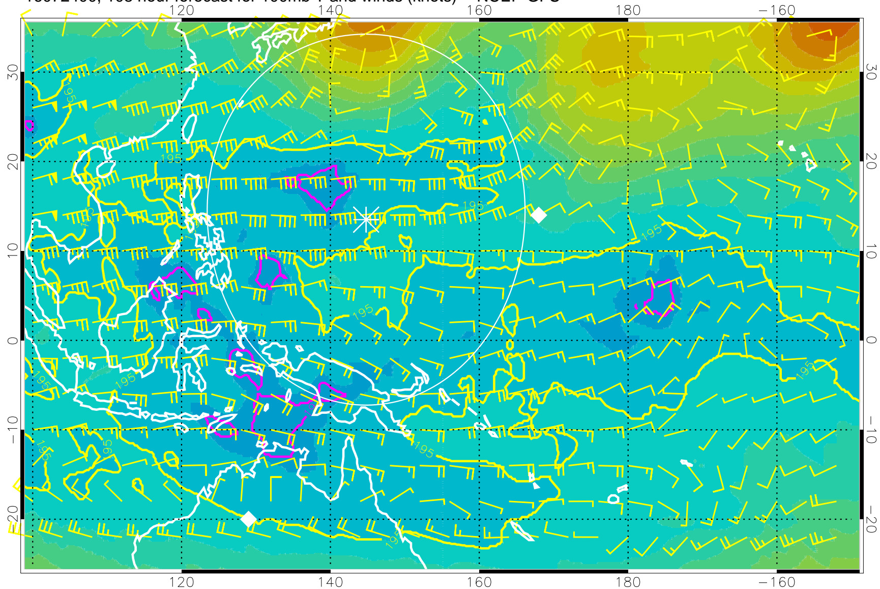
16072400, 108 hour forecast for 100mb T and winds (knots) -- NCEP GFS
