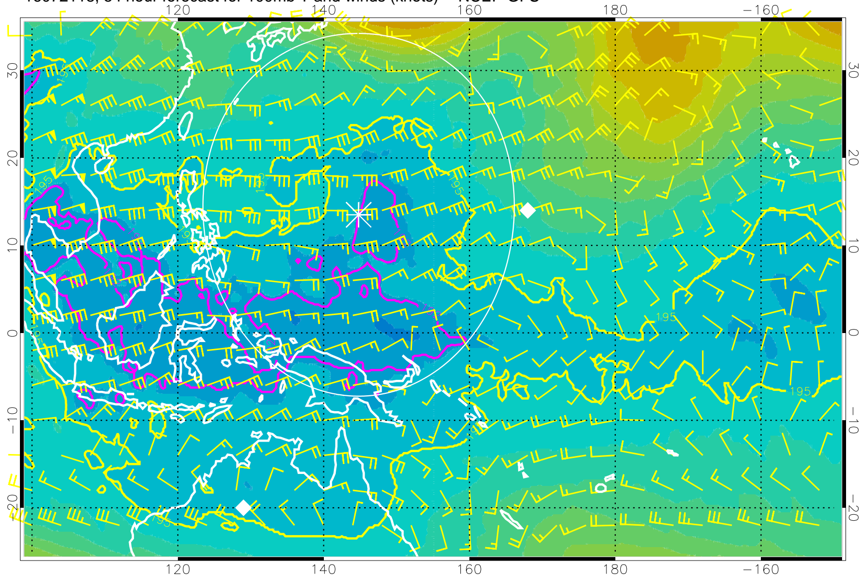
16072118, 54 hour forecast for 100mb T and winds (knots) -- NCEP GFS
