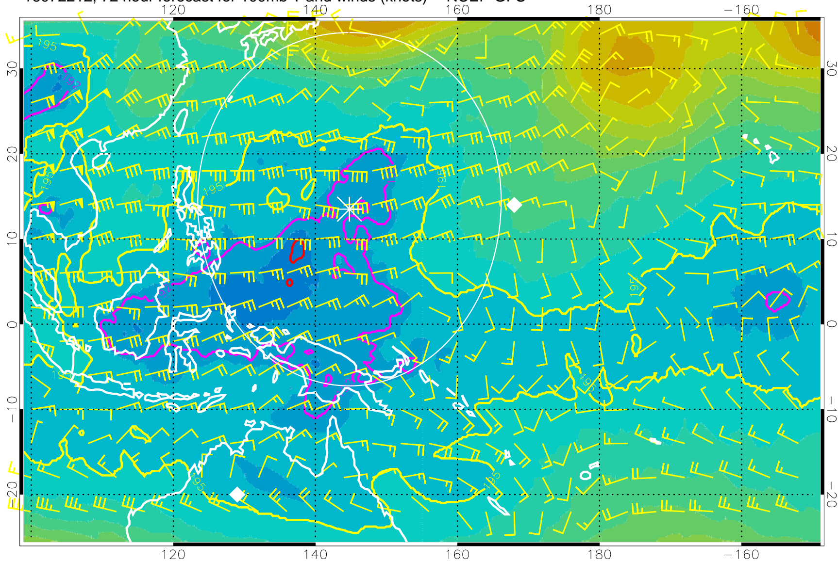
16072212, 72 hour forecast for 100mb T and winds (knots) -- NCEP GFS
