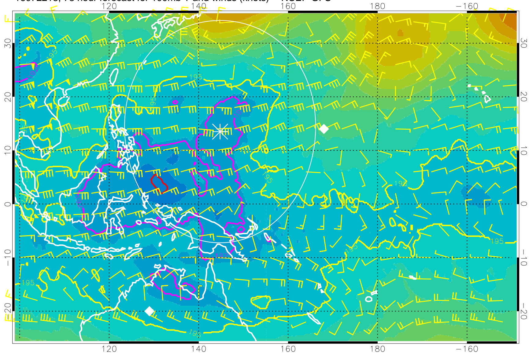
16072218, 78 hour forecast for 100mb T and winds (knots) -- NCEP GFS
