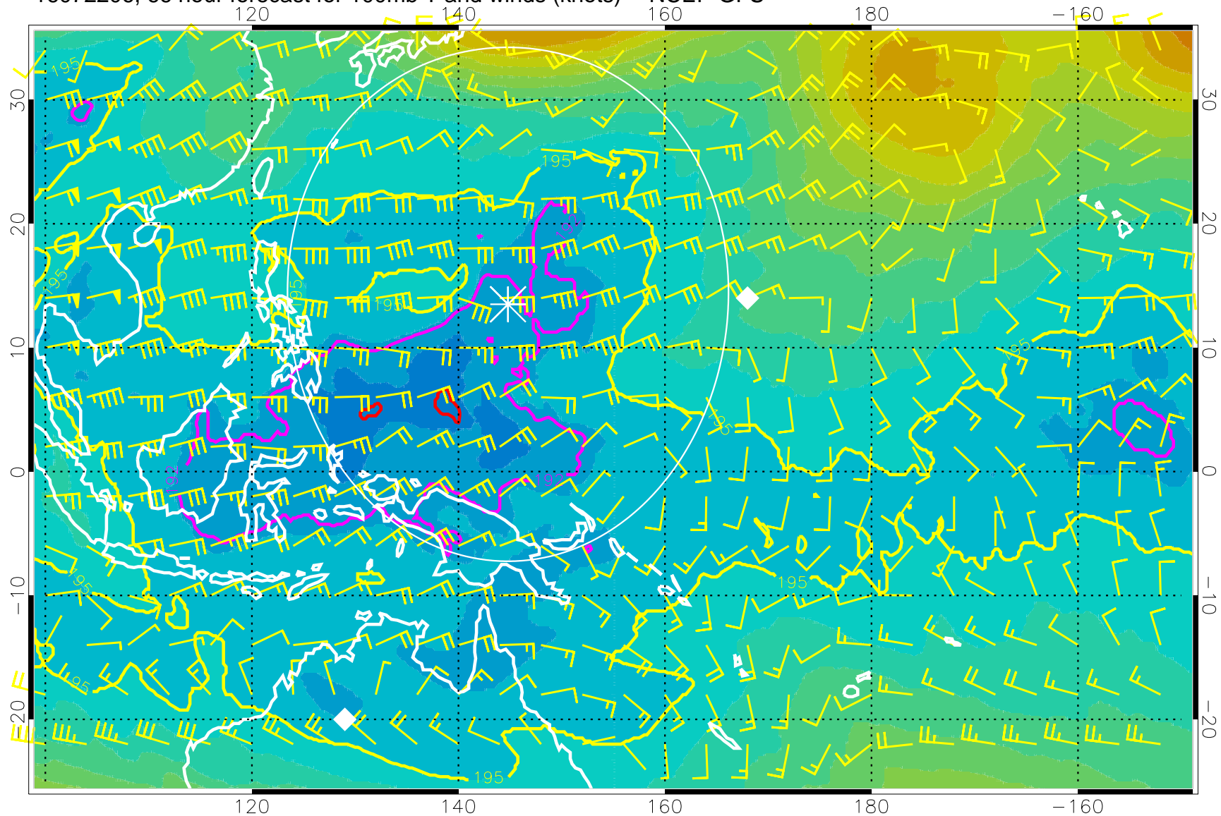
16072206, 66 hour forecast for 100mb T and winds (knots) -- NCEP GFS
