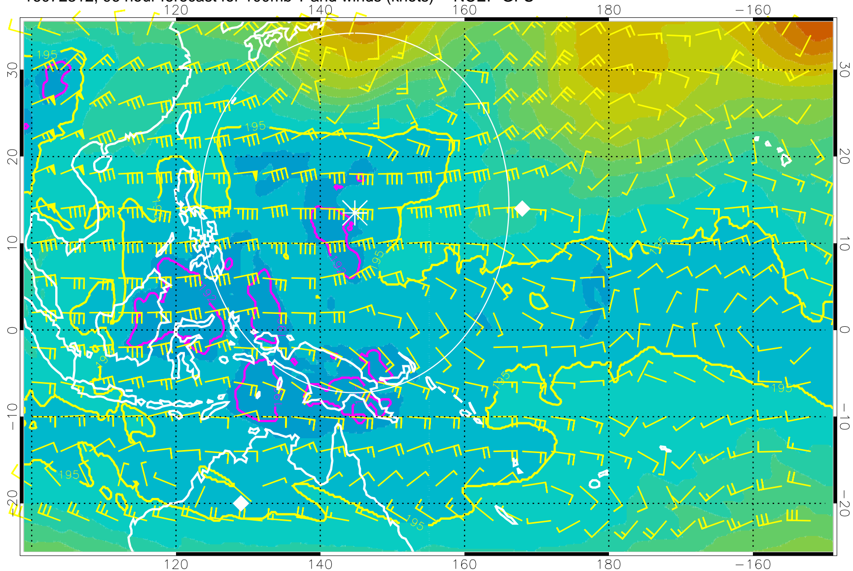
16072312, 96 hour forecast for 100mb T and winds (knots) -- NCEP GFS
