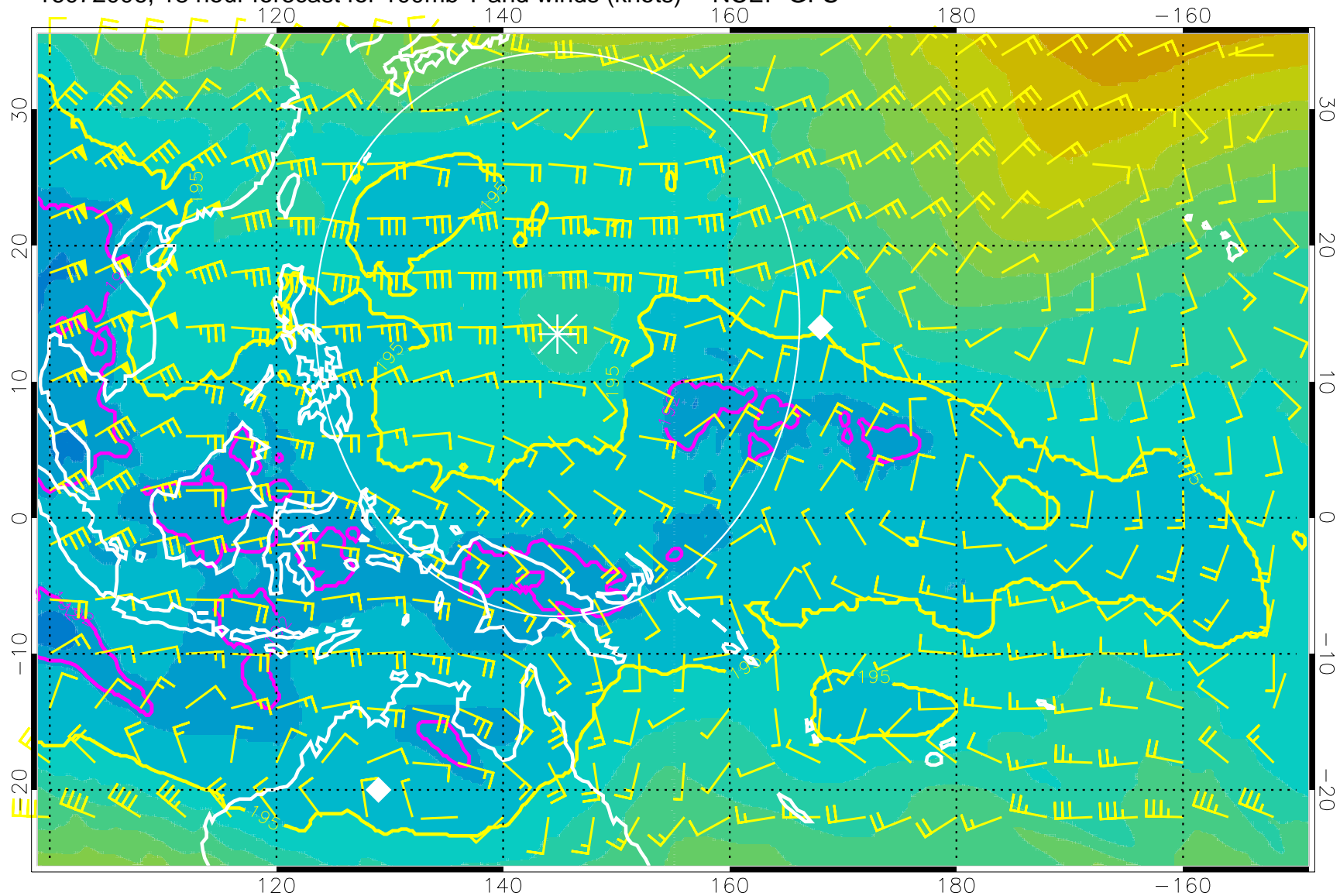
16072006, 18 hour forecast for 100mb T and winds (knots) -- NCEP GFS
