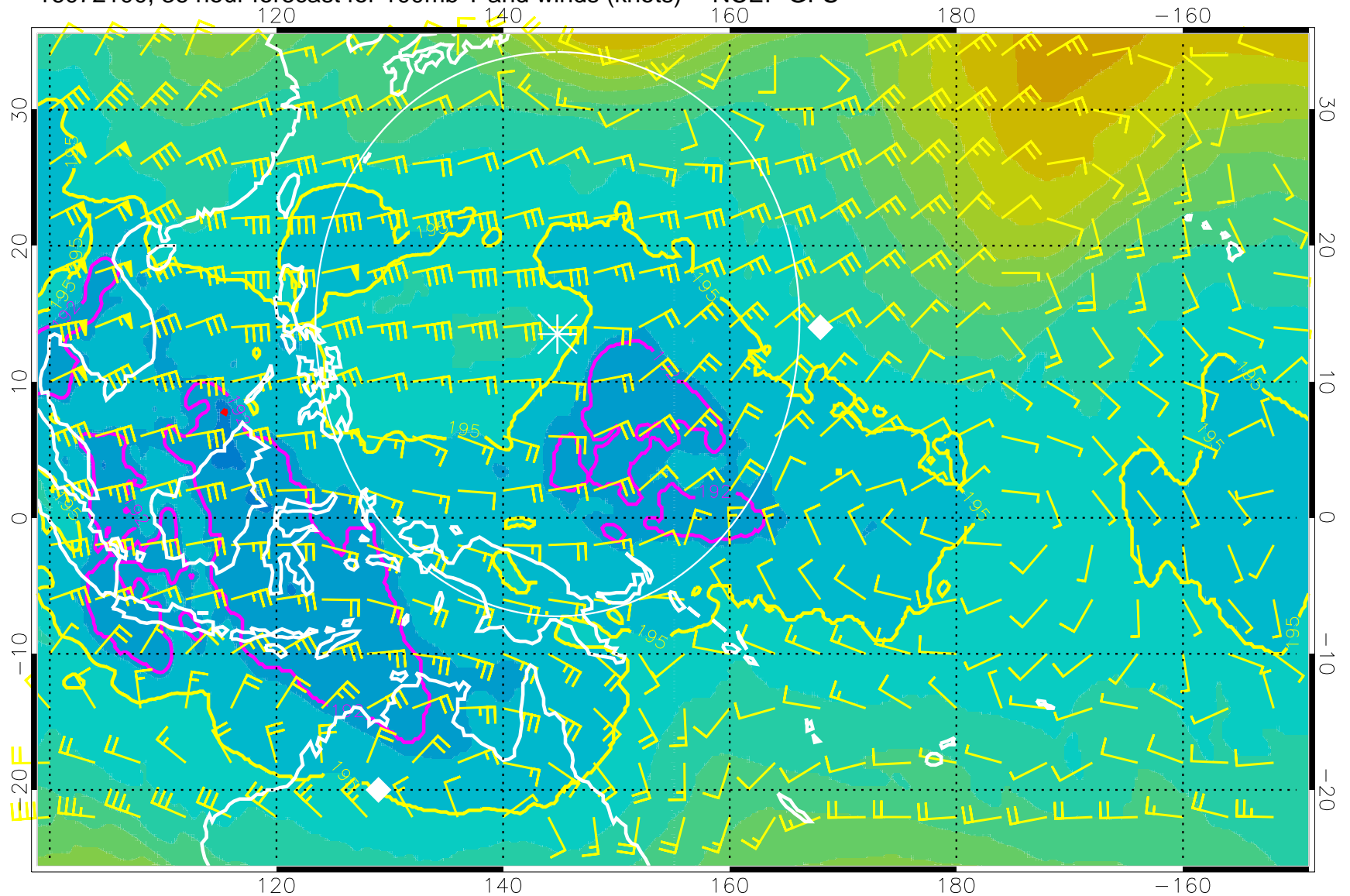
16072100, 36 hour forecast for 100mb T and winds (knots) -- NCEP GFS
