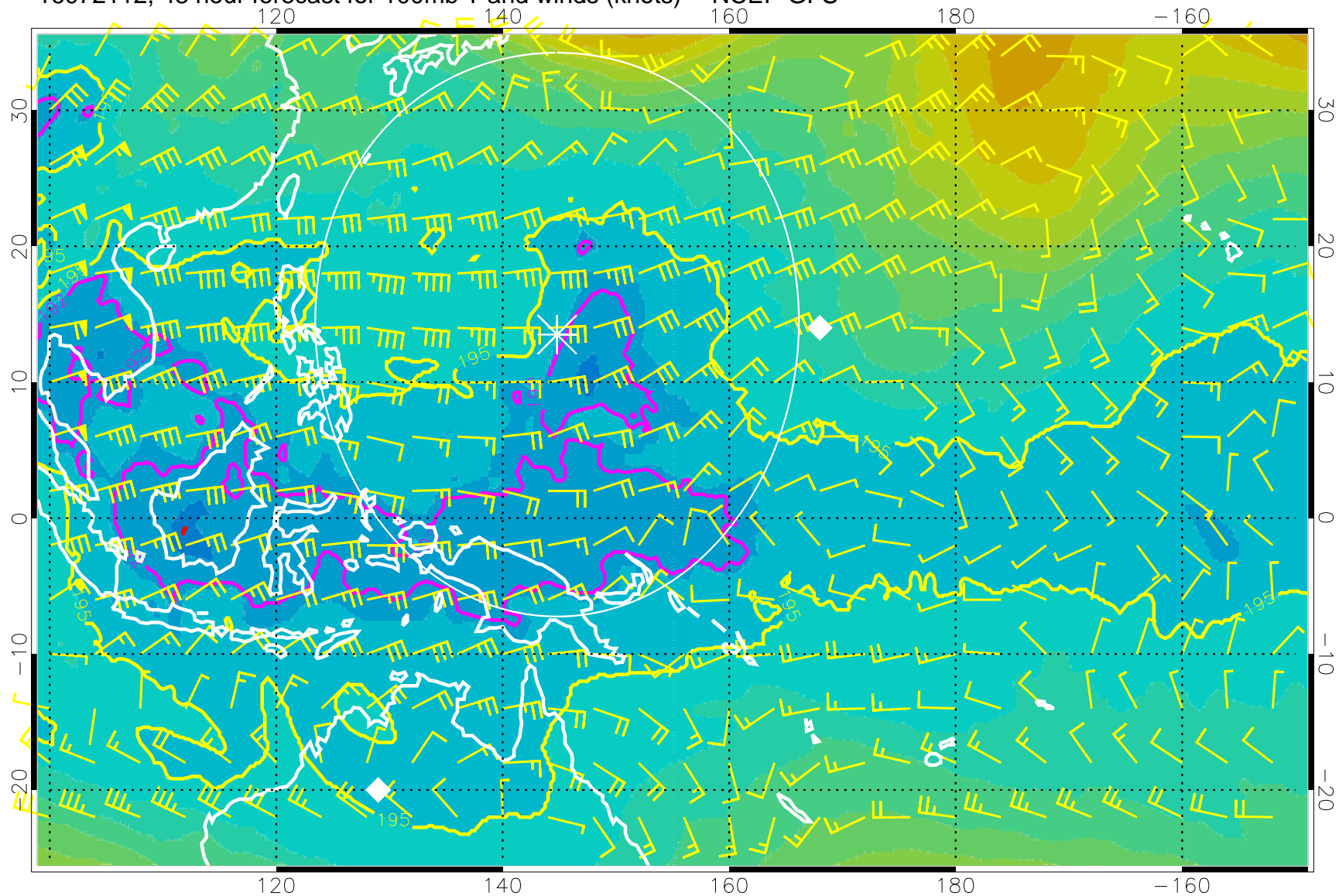
16072112, 48 hour forecast for 100mb T and winds (knots) -- NCEP GFS
