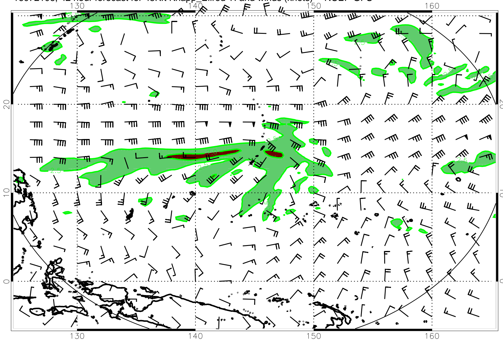
16072106, 42 hour forecast for 45Kft Knapp_Ellrod TI and winds (knots) -- NCEP GFS
