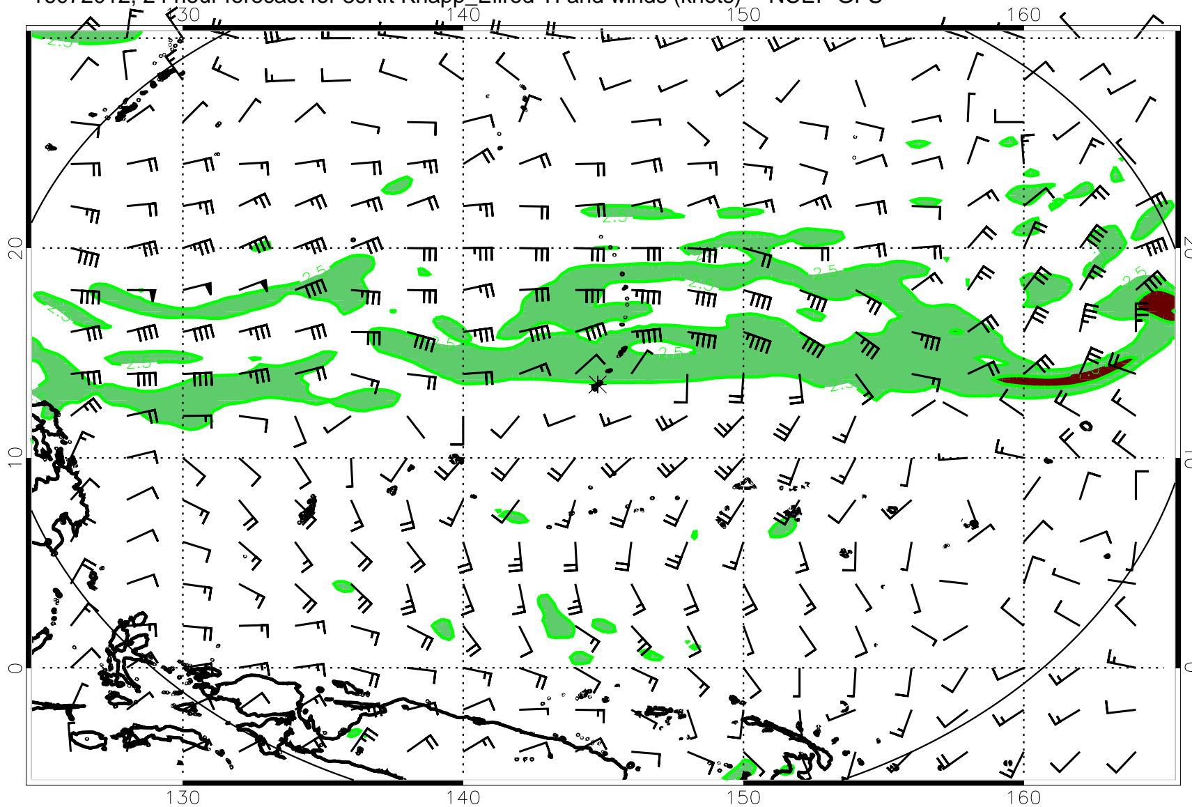
16072012, 24 hour forecast for 39Kft Knapp_Ellrod TI and winds (knots) -- NCEP GFS
