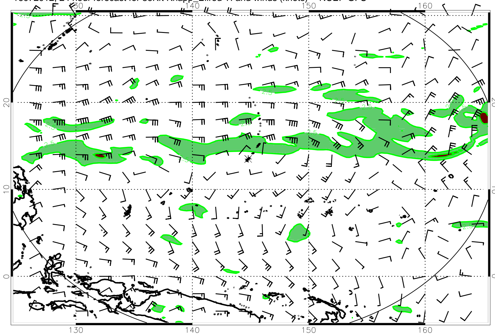
16072012, 24 hour forecast for 36Kft Knapp_Ellrod TI and winds (knots) -- NCEP GFS
