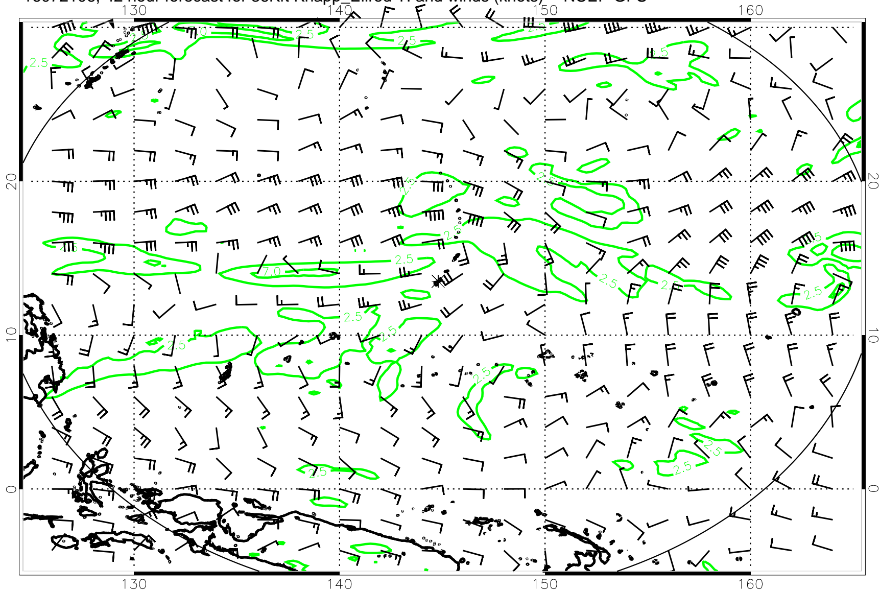
16072106, 42 hour forecast for 36Kft Knapp_Ellrod TI and winds (knots) -- NCEP GFS
