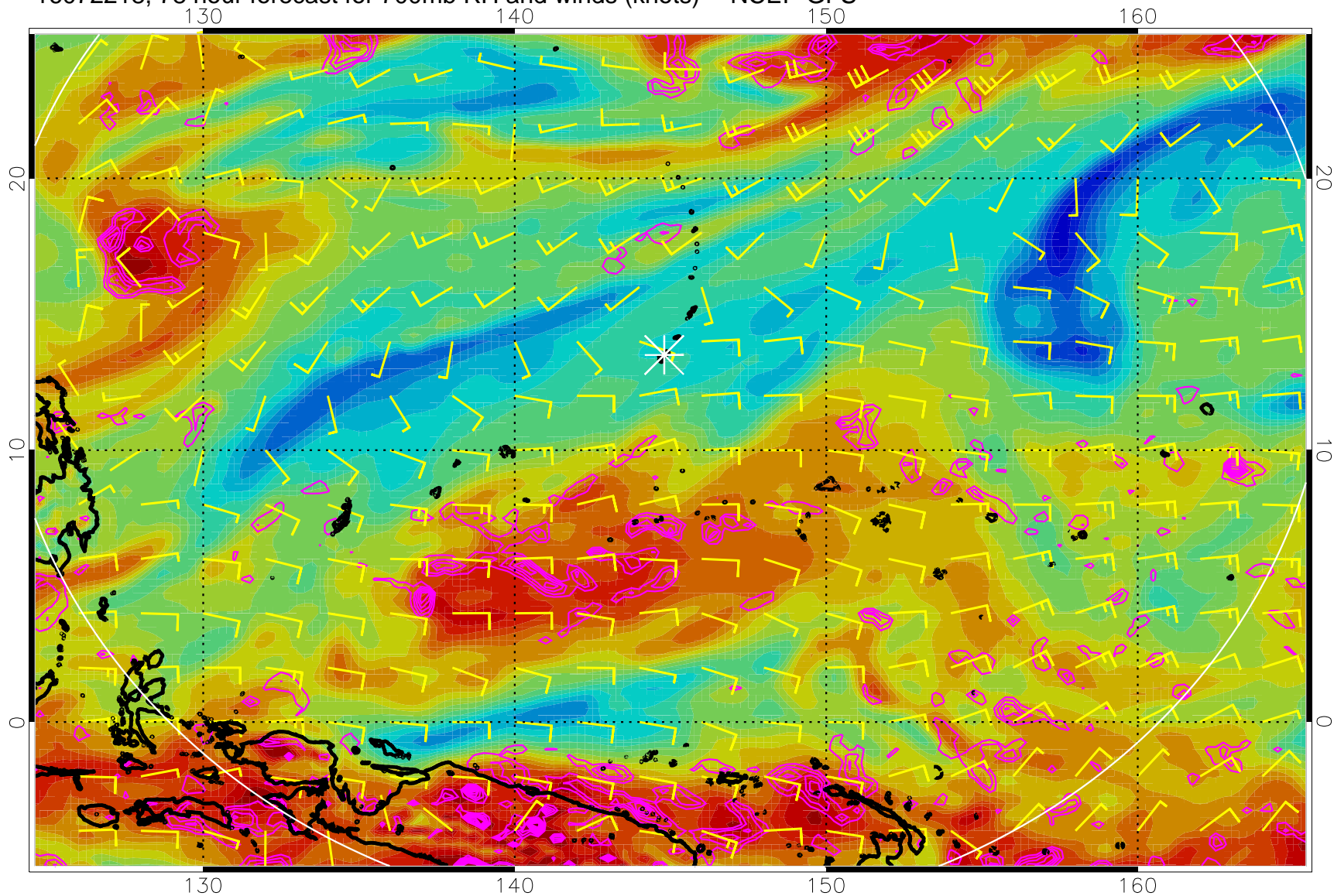
16072218, 78 hour forecast for 700mb RH and winds (knots) -- NCEP GFS
