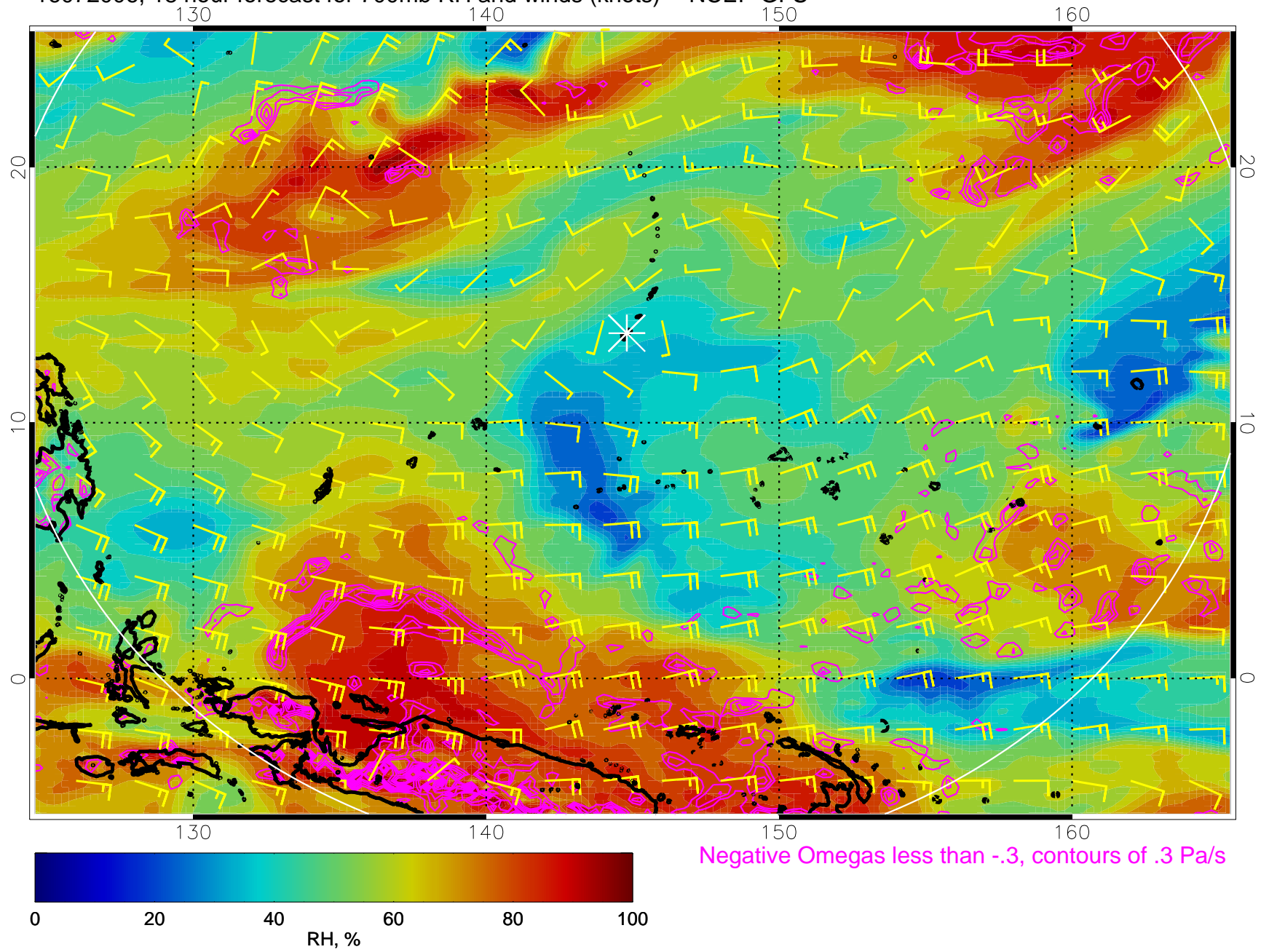
16072006, 18 hour forecast for 700mb RH and winds (knots) -- NCEP GFS
