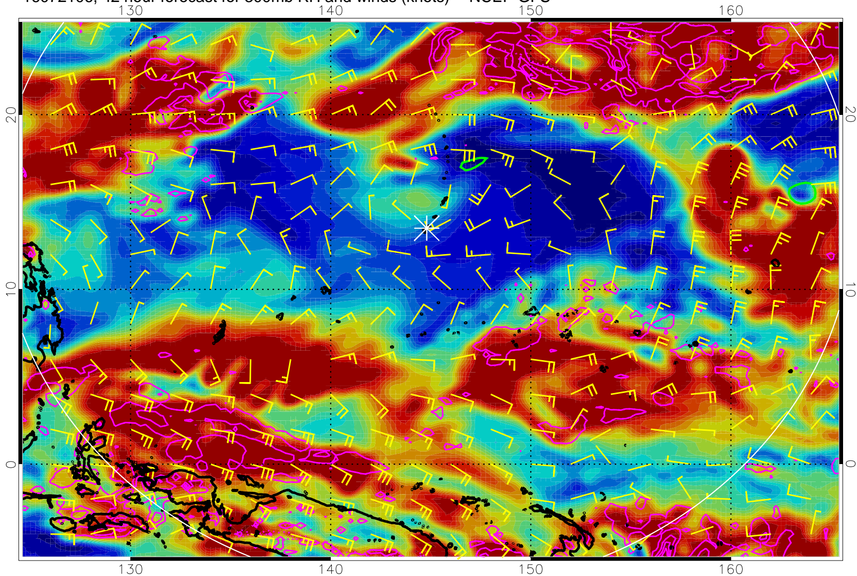
16072106, 42 hour forecast for 300mb RH and winds (knots) -- NCEP GFS
