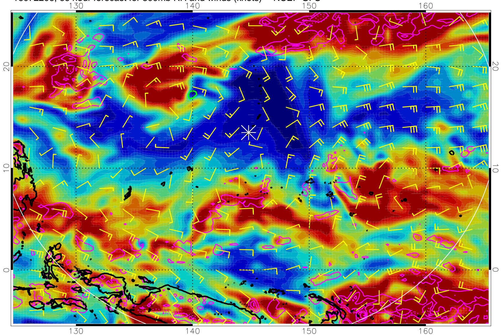
16072206, 66 hour forecast for 300mb RH and winds (knots) -- NCEP GFS
