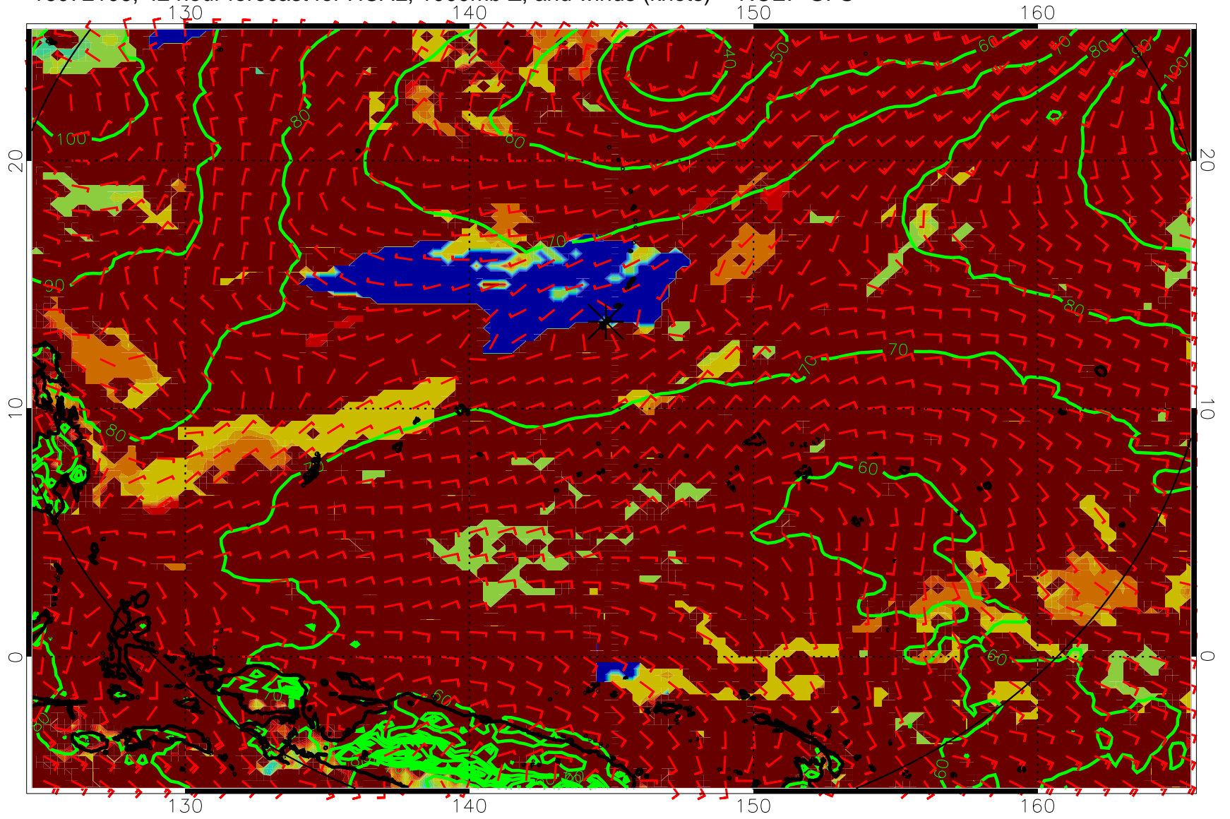
16072106, 42 hour forecast for HCAL, 1000mb Z, and winds (knots) -- NCEP GFS
