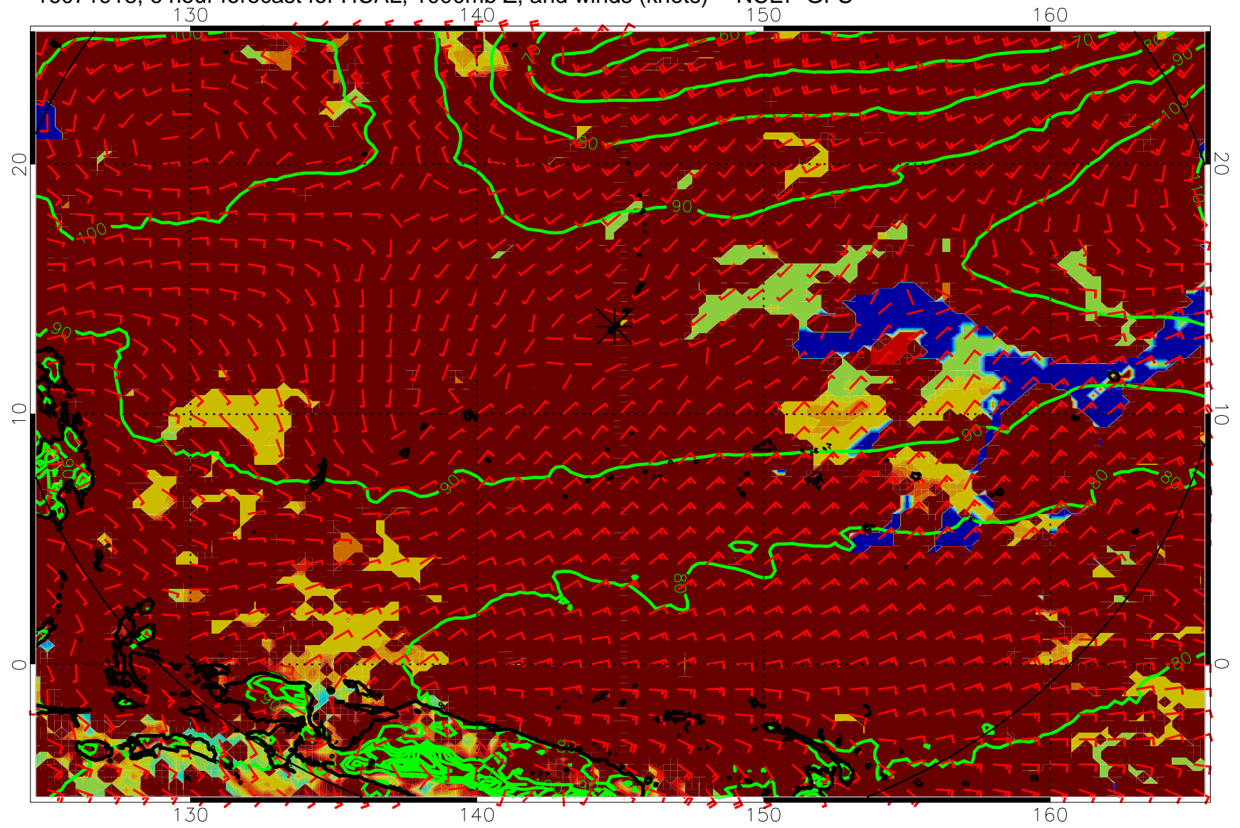
16071918, 6 hour forecast for HCAL, 1000mb Z, and winds (knots) -- NCEP GFS
