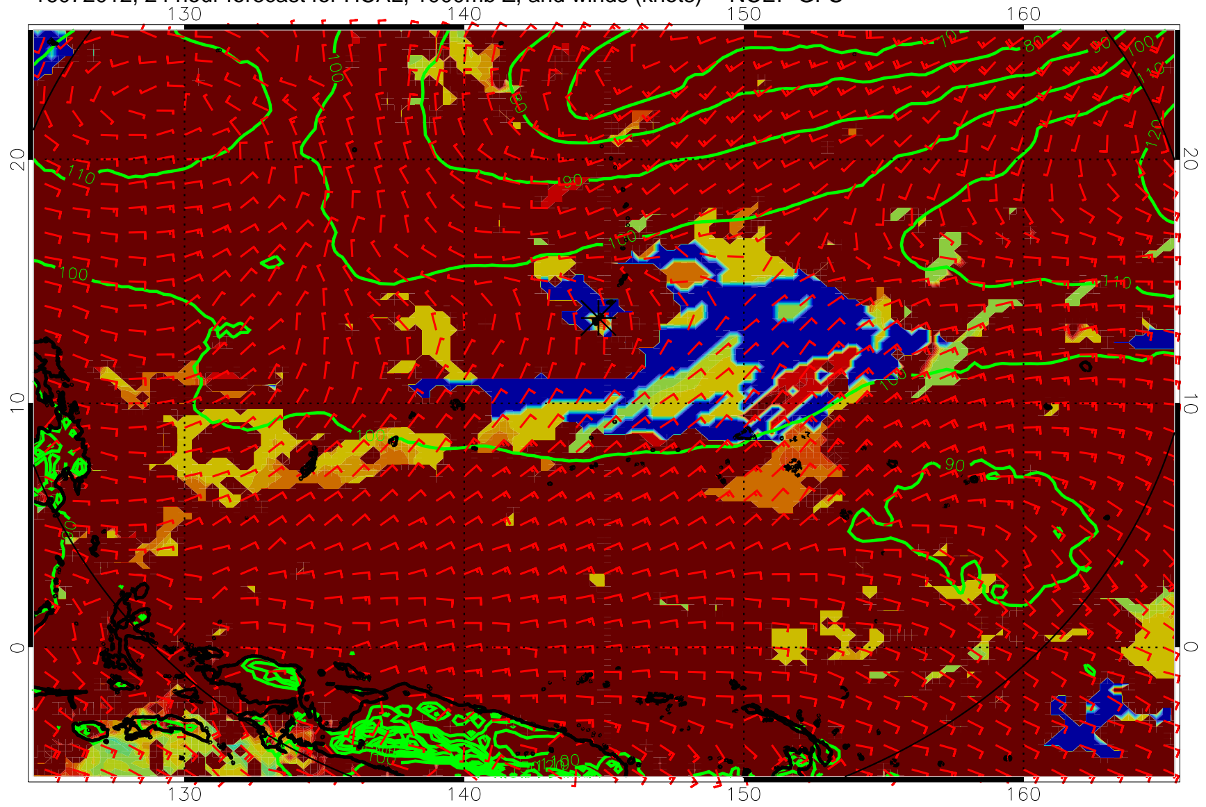
16072012, 24 hour forecast for HCAL, 1000mb Z, and winds (knots) -- NCEP GFS
