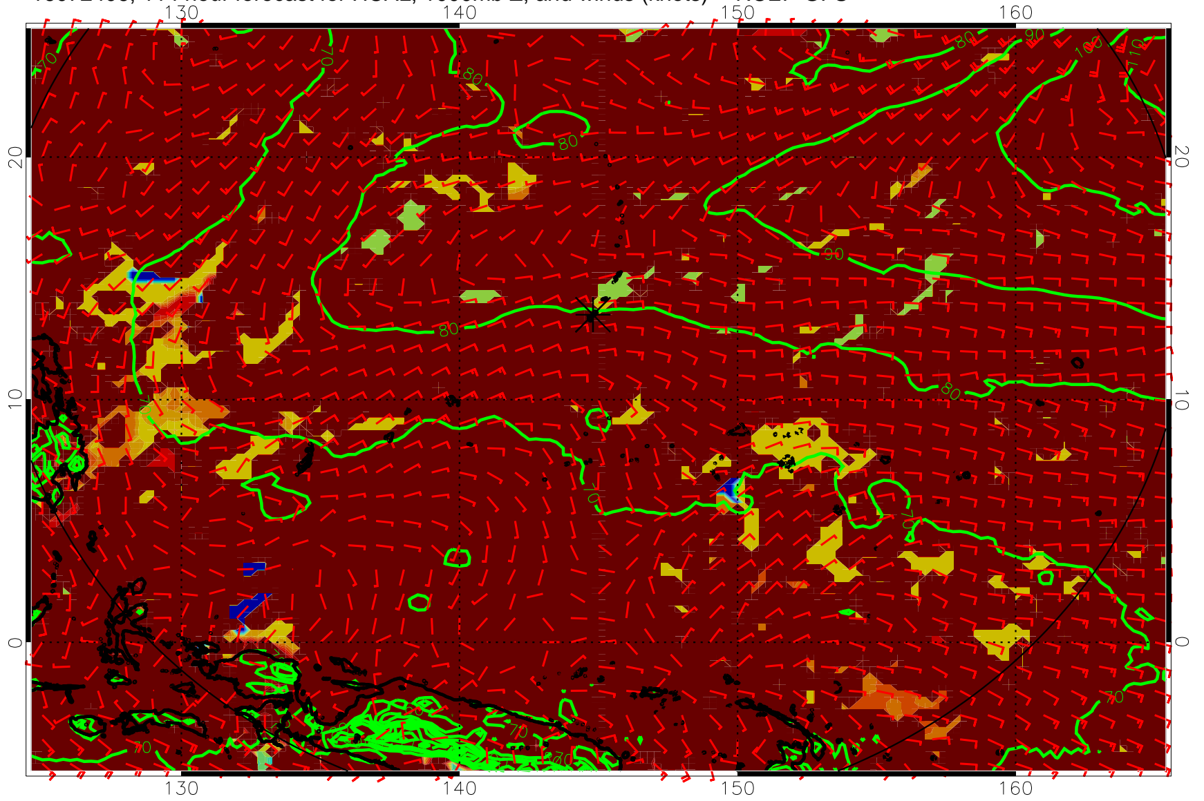
16072406, 114 hour forecast for HCAL, 1000mb Z, and winds (knots) -- NCEP GFS
