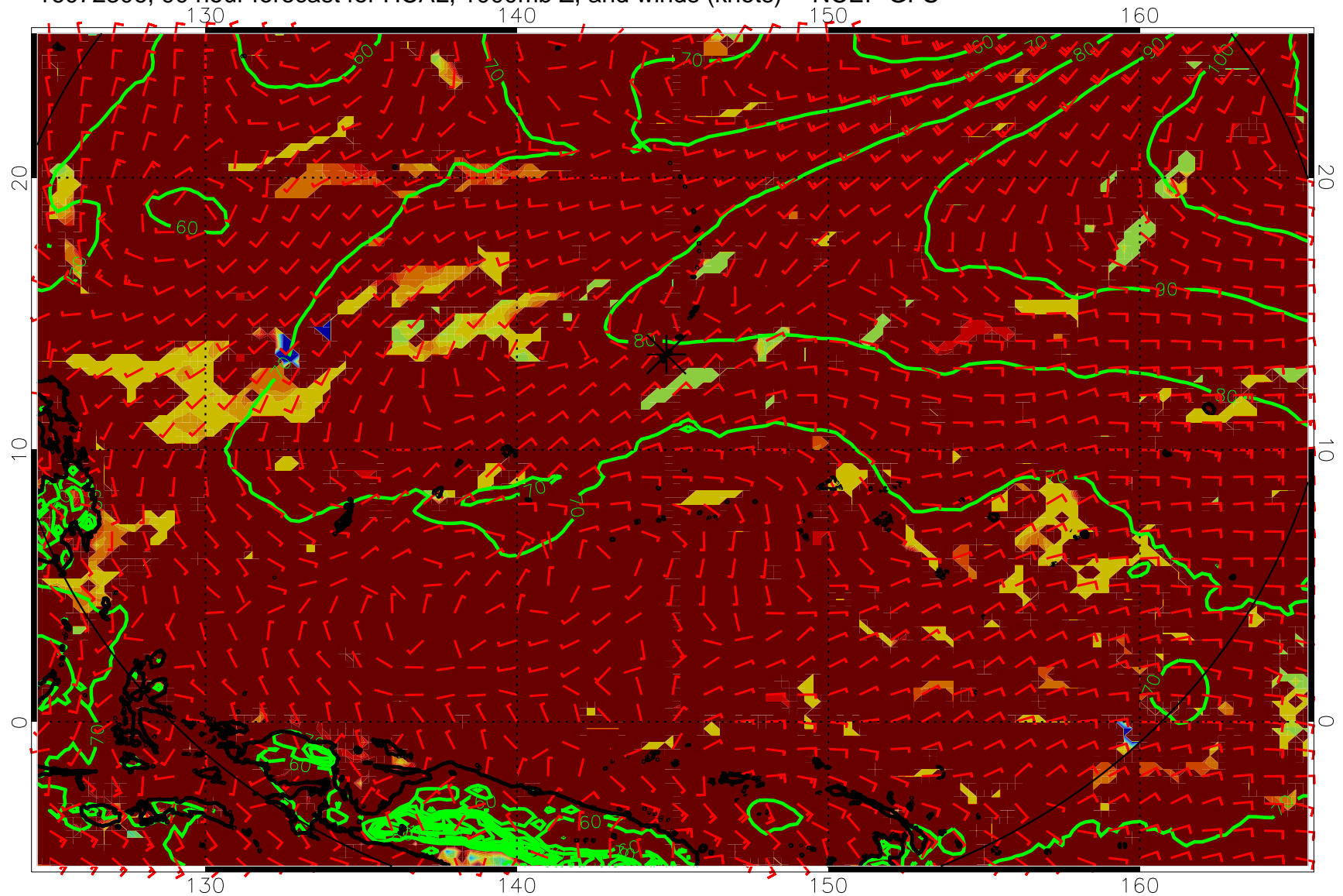
16072306, 90 hour forecast for HCAL, 1000mb Z, and winds (knots) -- NCEP GFS
