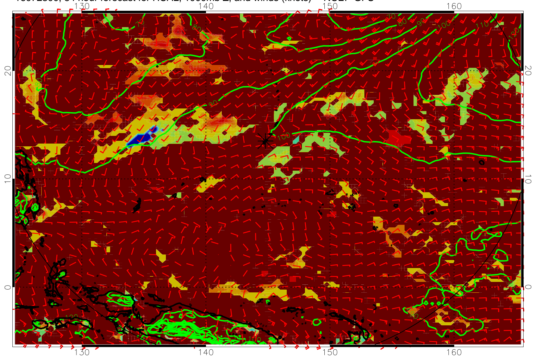
16072300, 84 hour forecast for HCAL, 1000mb Z, and winds (knots) -- NCEP GFS
