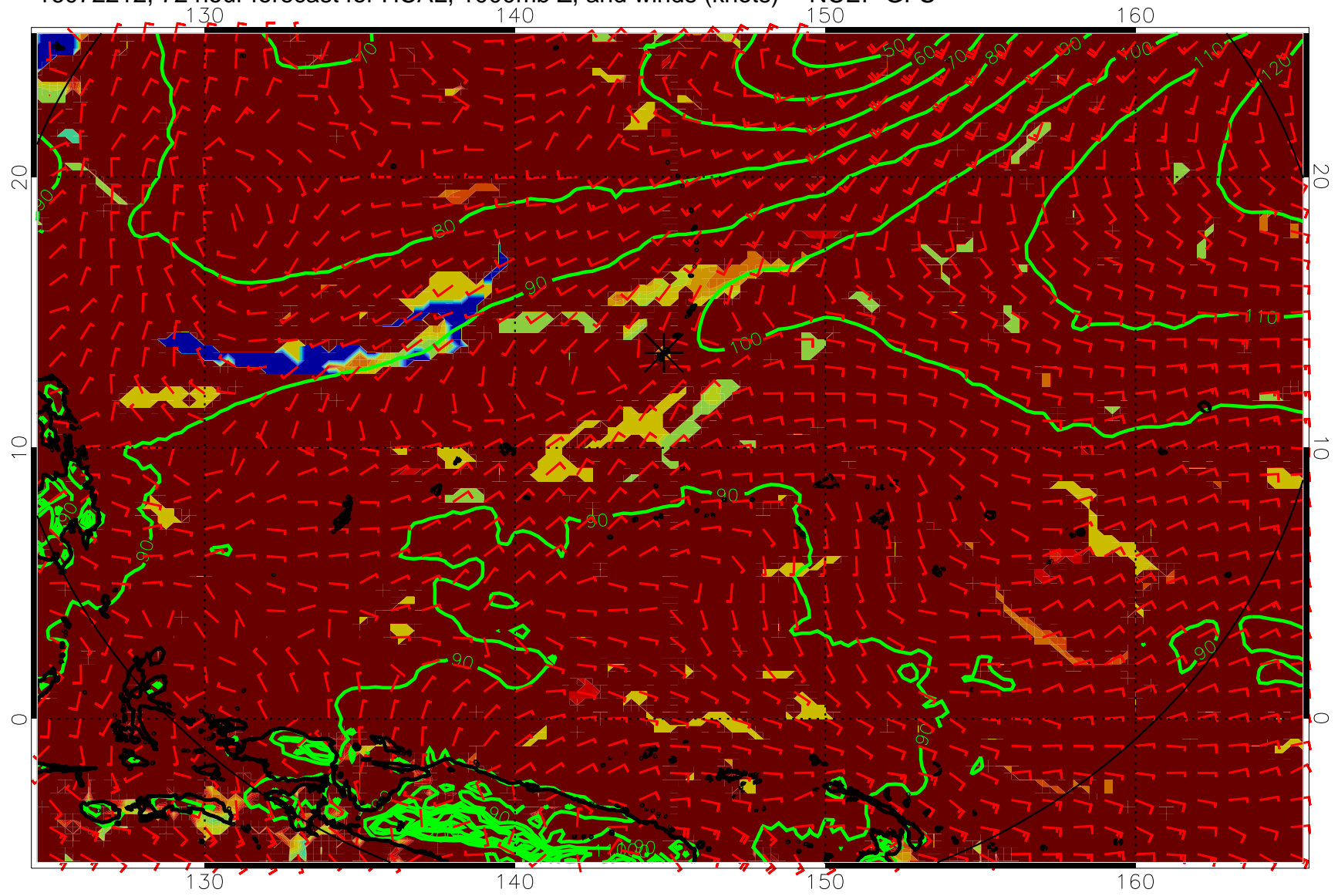
16072212, 72 hour forecast for HCAL, 1000mb Z, and winds (knots) -- NCEP GFS
