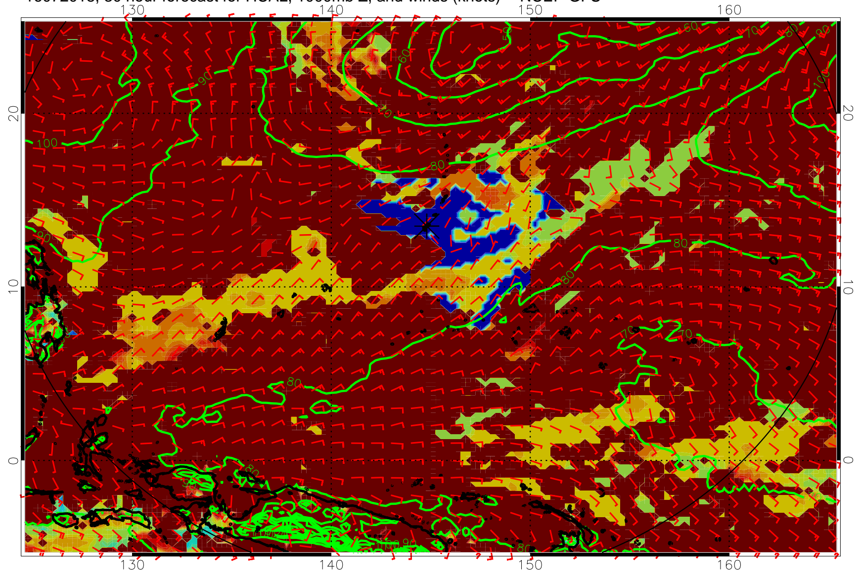
16072018, 30 hour forecast for HCAL, 1000mb Z, and winds (knots) -- NCEP GFS
