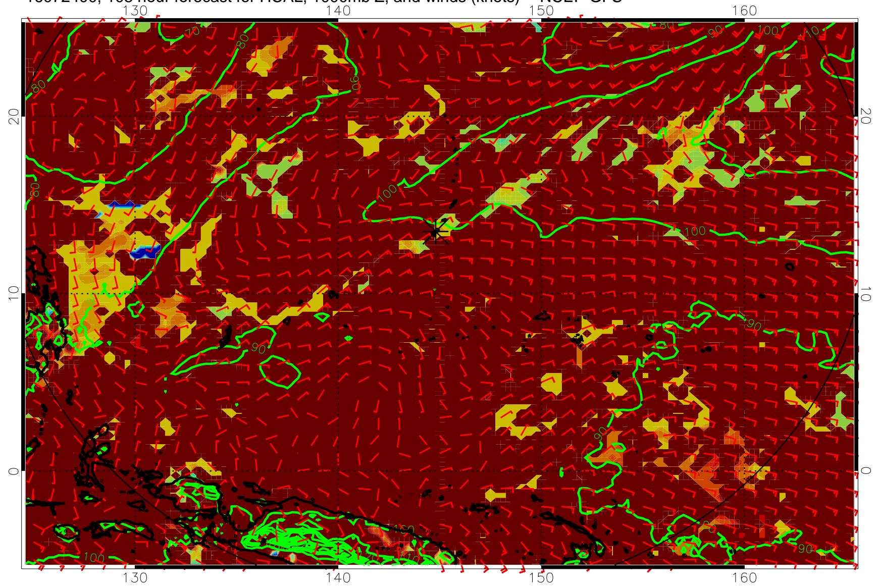
16072400, 108 hour forecast for HCAL, 1000mb Z, and winds (knots) -- NCEP GFS
