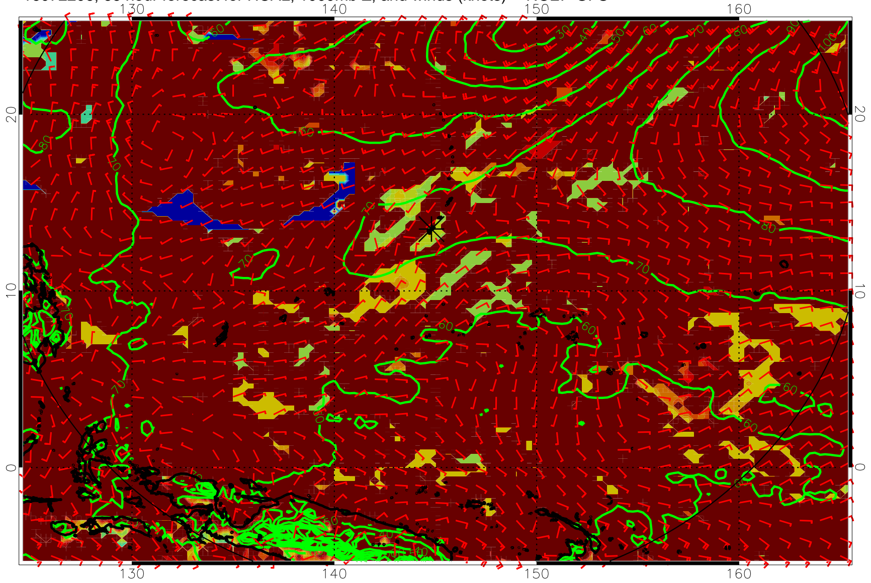
16072206, 66 hour forecast for HCAL, 1000mb Z, and winds (knots) -- NCEP GFS
