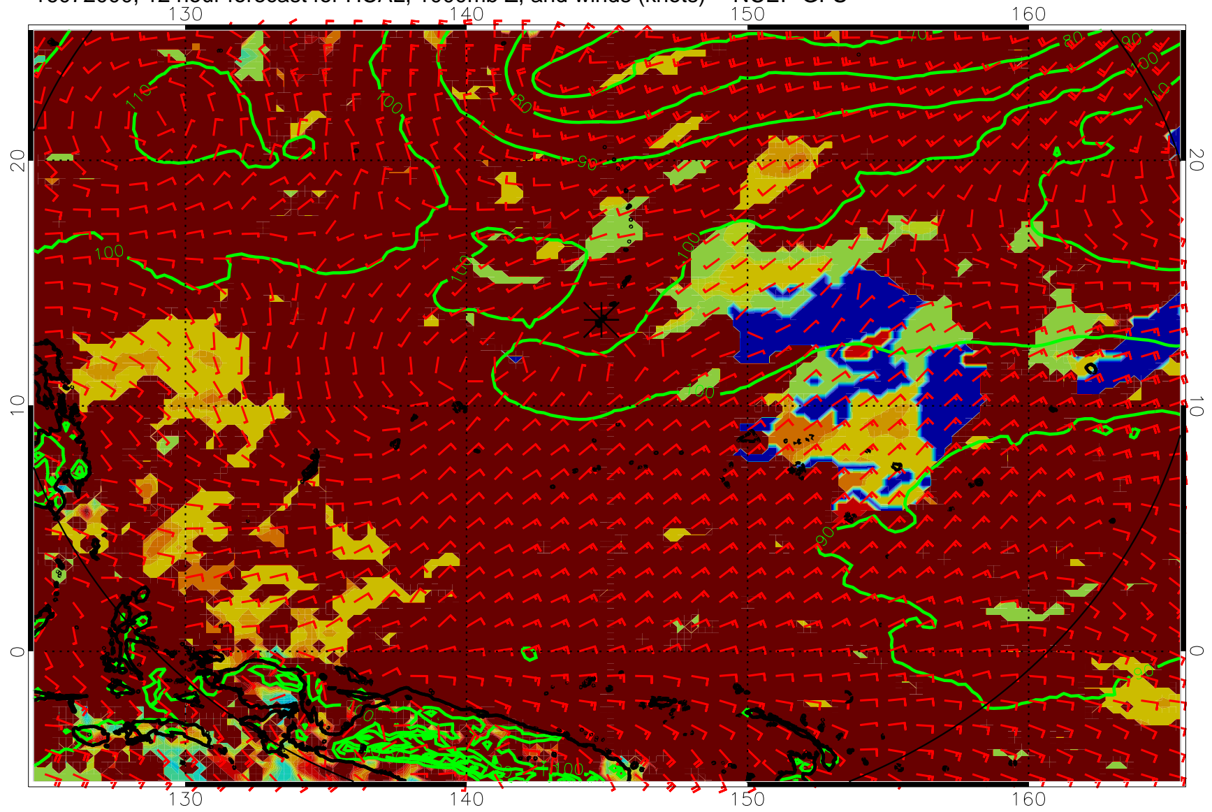
16072000, 12 hour forecast for HCAL, 1000mb Z, and winds (knots) -- NCEP GFS
