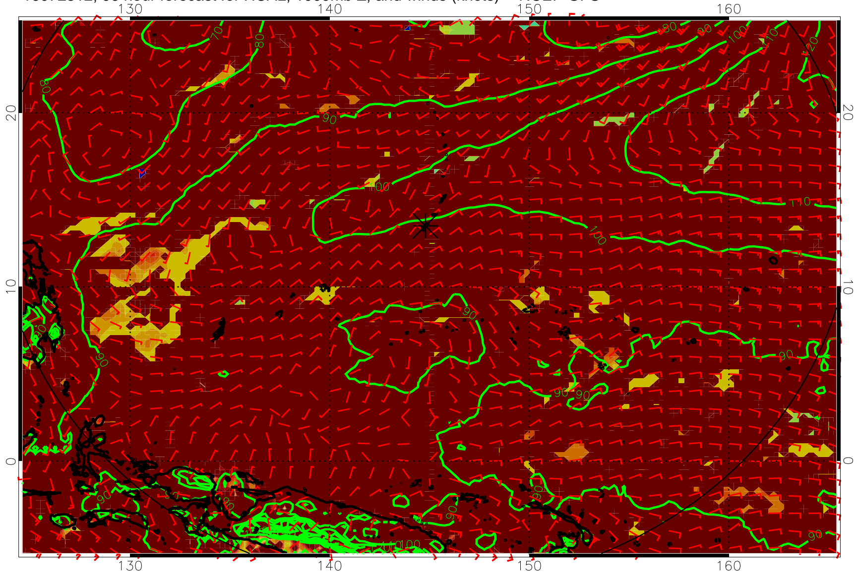
16072312, 96 hour forecast for HCAL, 1000mb Z, and winds (knots) -- NCEP GFS
