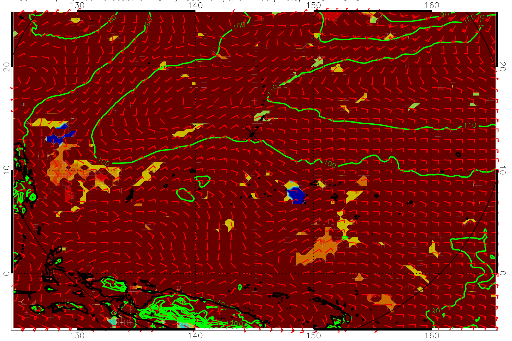
16072412, 120 hour forecast for HCAL, 1000mb Z, and winds (knots) -- NCEP GFS
