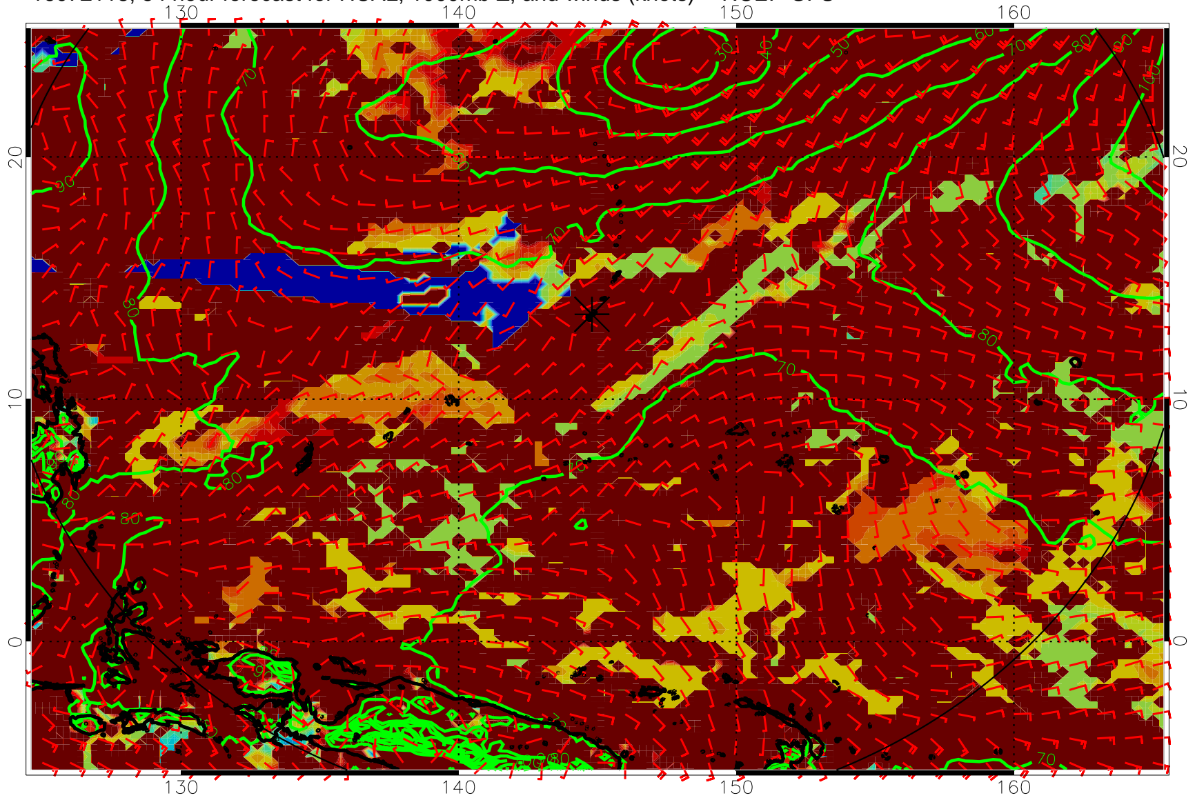
16072118, 54 hour forecast for HCAL, 1000mb Z, and winds (knots) -- NCEP GFS
