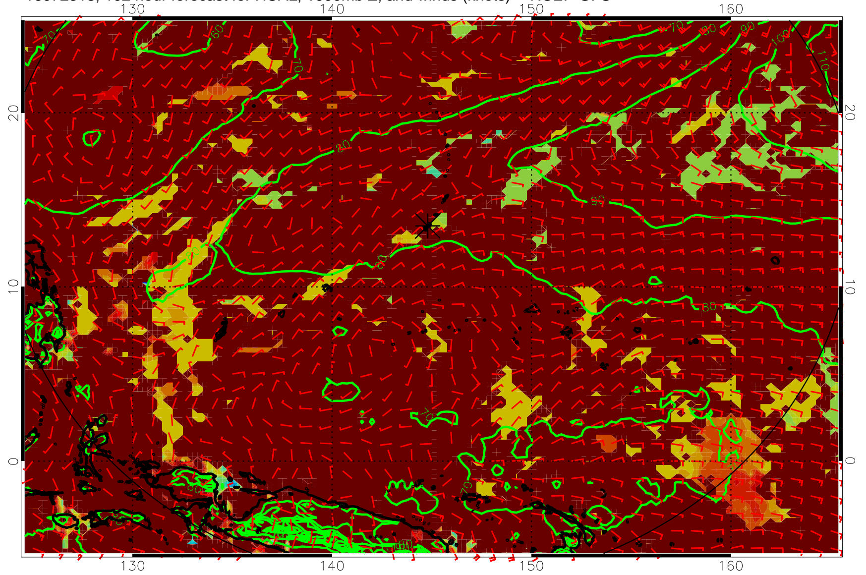
16072318, 102 hour forecast for HCAL, 1000mb Z, and winds (knots) -- NCEP GFS
