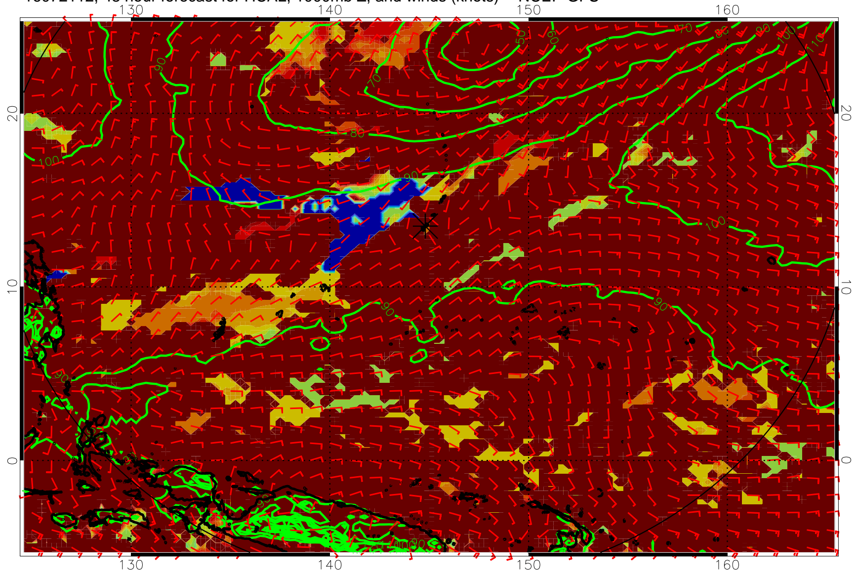
16072112, 48 hour forecast for HCAL, 1000mb Z, and winds (knots) -- NCEP GFS
