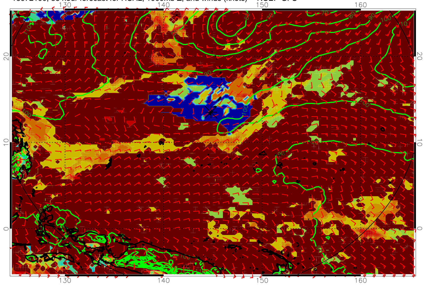
16072100, 36 hour forecast for HCAL, 1000mb Z, and winds (knots) -- NCEP GFS
