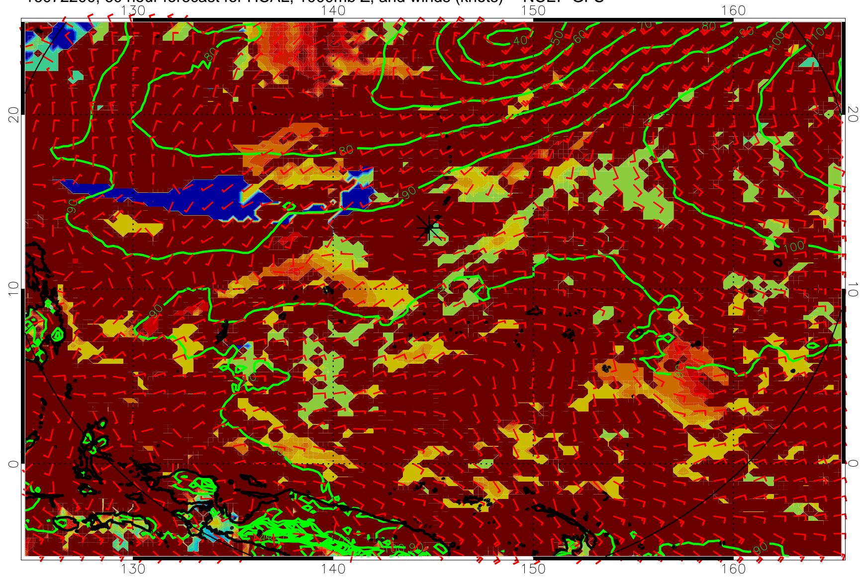
16072200, 60 hour forecast for HCAL, 1000mb Z, and winds (knots) -- NCEP GFS
