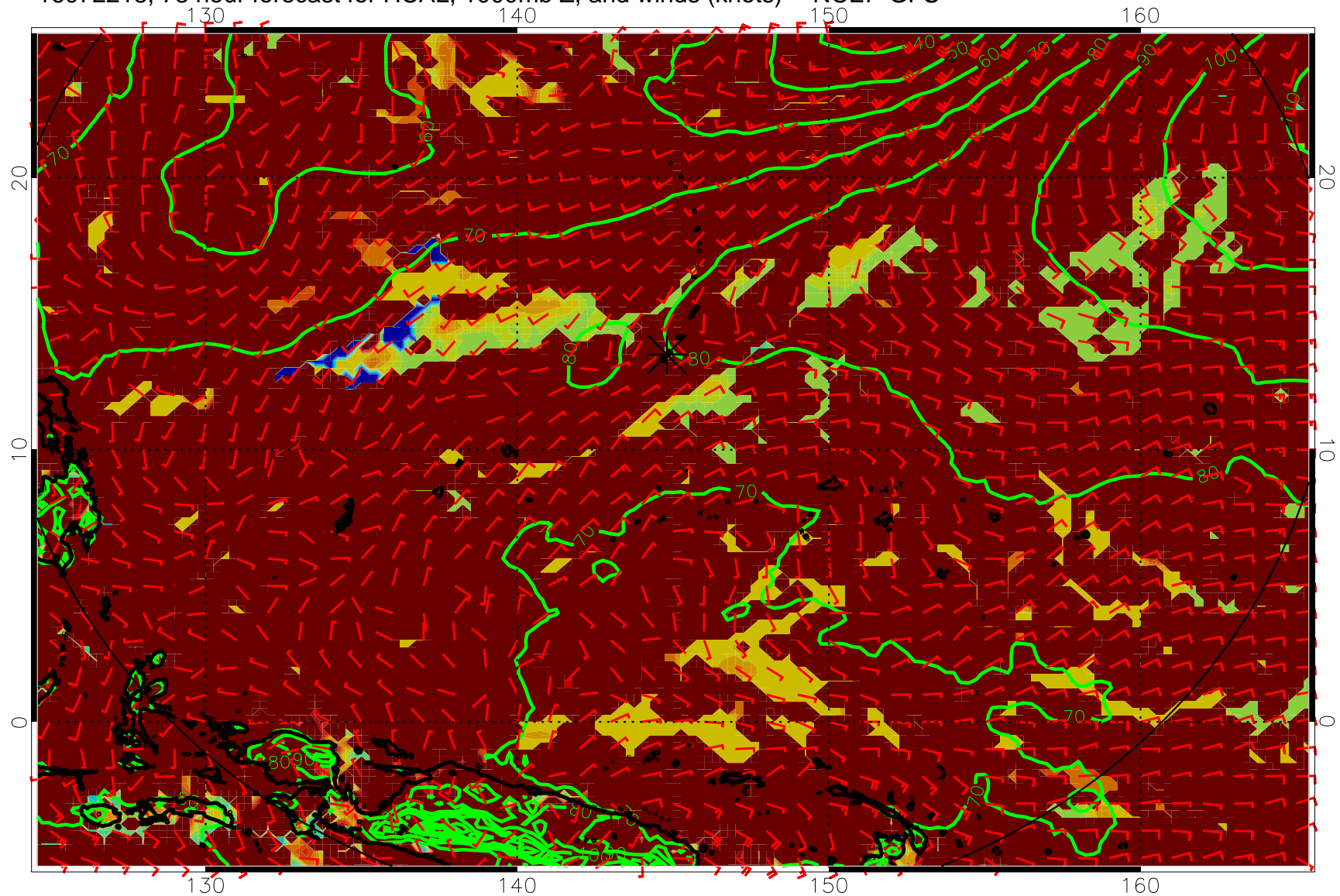
16072218, 78 hour forecast for HCAL, 1000mb Z, and winds (knots) -- NCEP GFS
