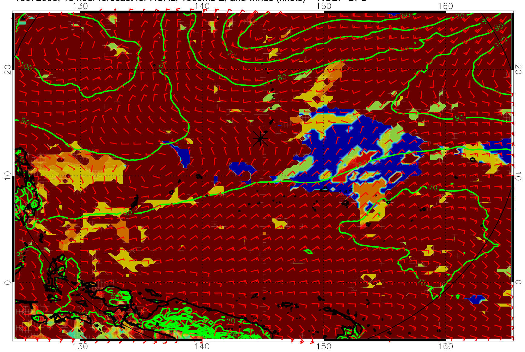
16072006, 18 hour forecast for HCAL, 1000mb Z, and winds (knots) -- NCEP GFS
