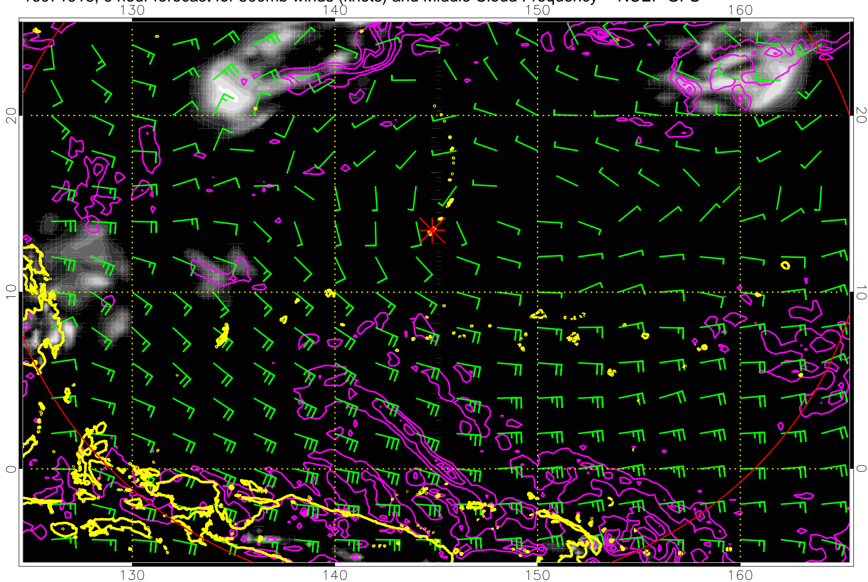
16071918, 6 hour forecast for 500mb winds (knots) and Middle Cloud Frequency -- NCEP GFS
