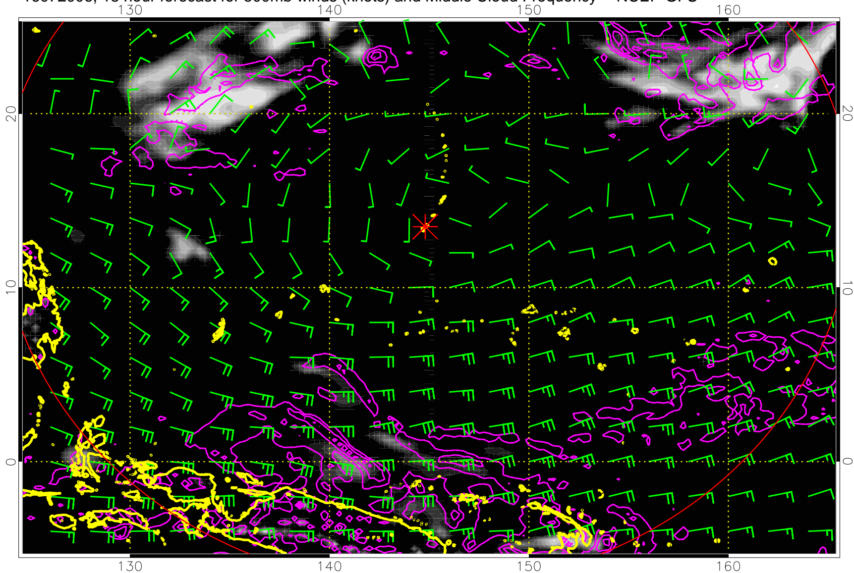
16072006, 18 hour forecast for 500mb winds (knots) and Middle Cloud Frequency -- NCEP GFS
