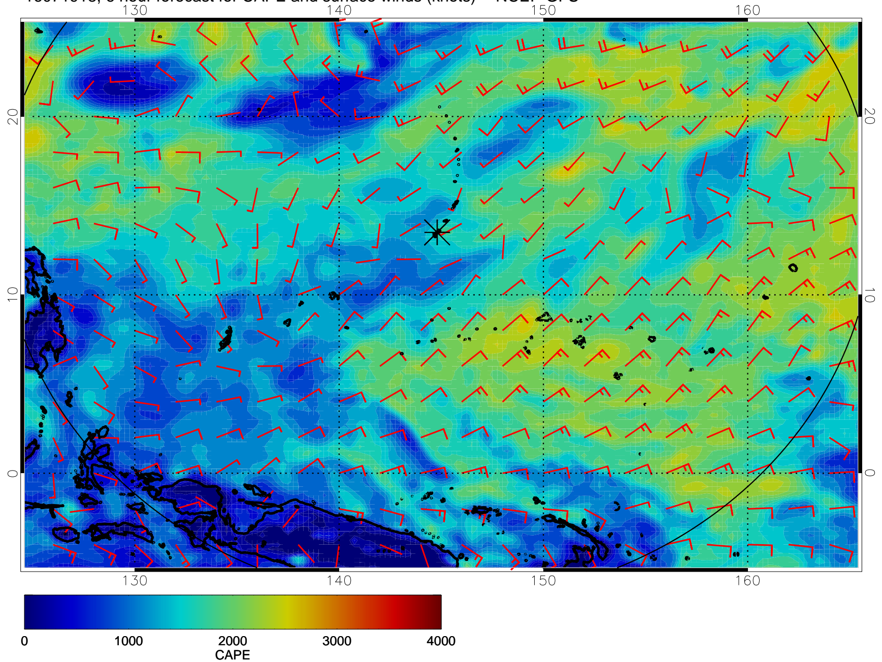
16071918, 6 hour forecast for CAPE and surface winds (knots) -- NCEP GFS
