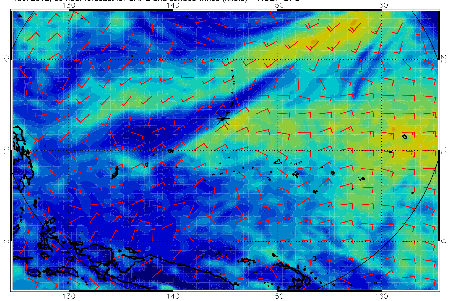
16072312, 96 hour forecast for CAPE and surface winds (knots) -- NCEP GFS
