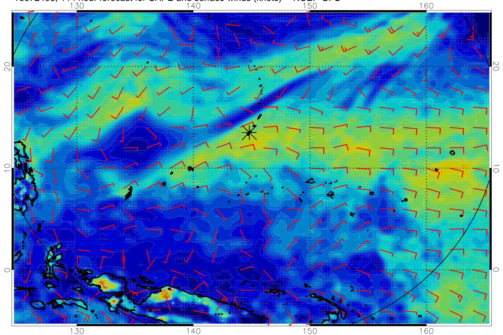
16072406, 114 hour forecast for CAPE and surface winds (knots) -- NCEP GFS
