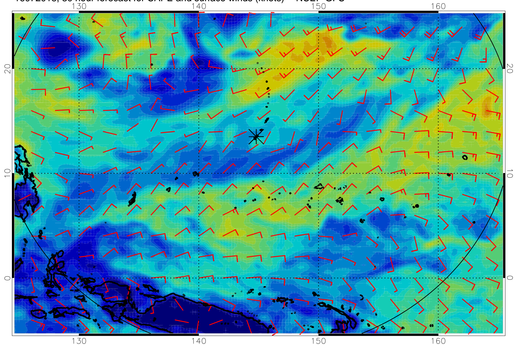
16072018, 30 hour forecast for CAPE and surface winds (knots) -- NCEP GFS
