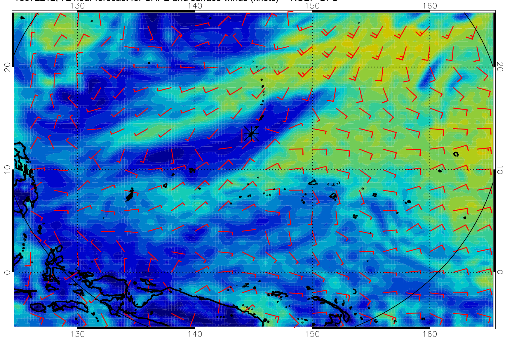
16072212, 72 hour forecast for CAPE and surface winds (knots) -- NCEP GFS
