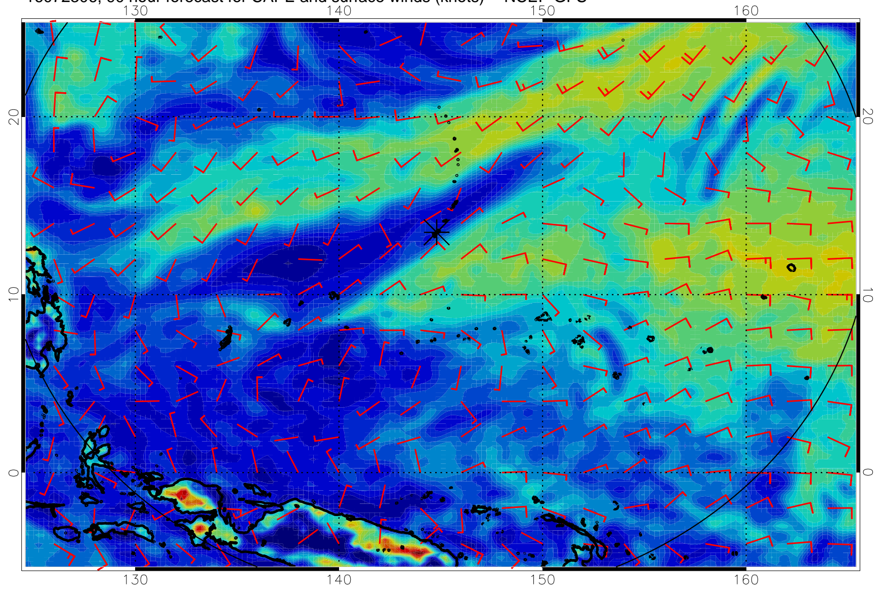
16072306, 90 hour forecast for CAPE and surface winds (knots) -- NCEP GFS
