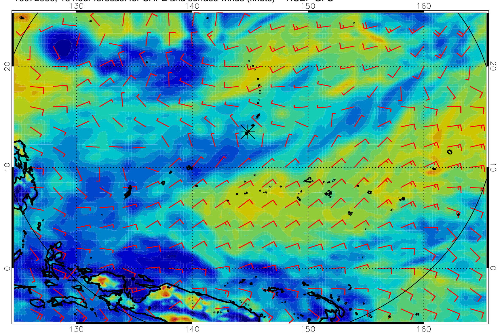
16072006, 18 hour forecast for CAPE and surface winds (knots) -- NCEP GFS
