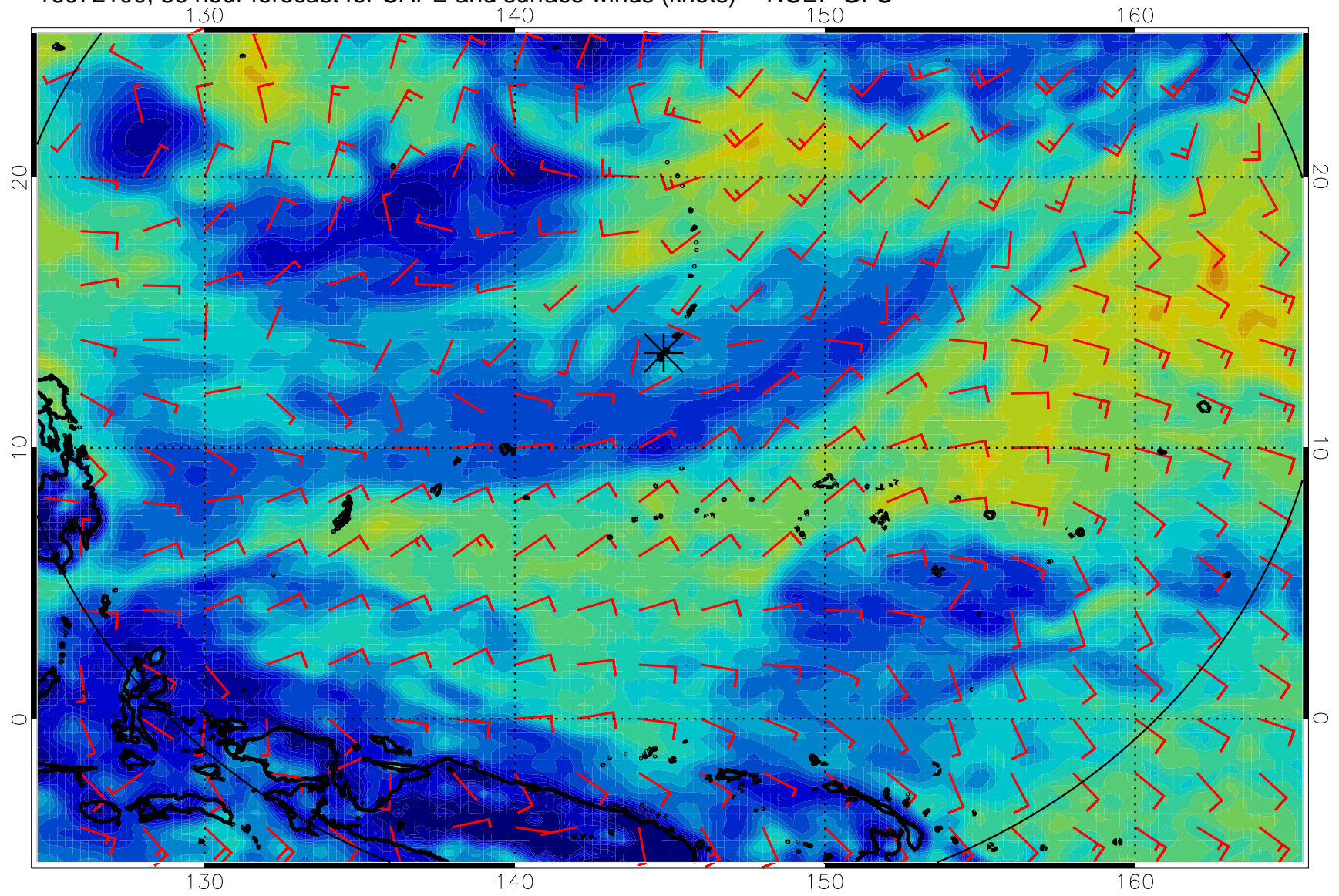
16072100, 36 hour forecast for CAPE and surface winds (knots) -- NCEP GFS
