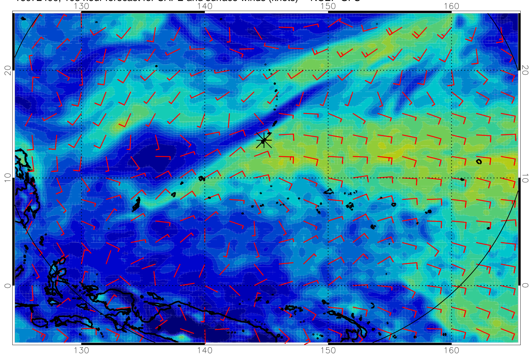
16072400, 108 hour forecast for CAPE and surface winds (knots) -- NCEP GFS
