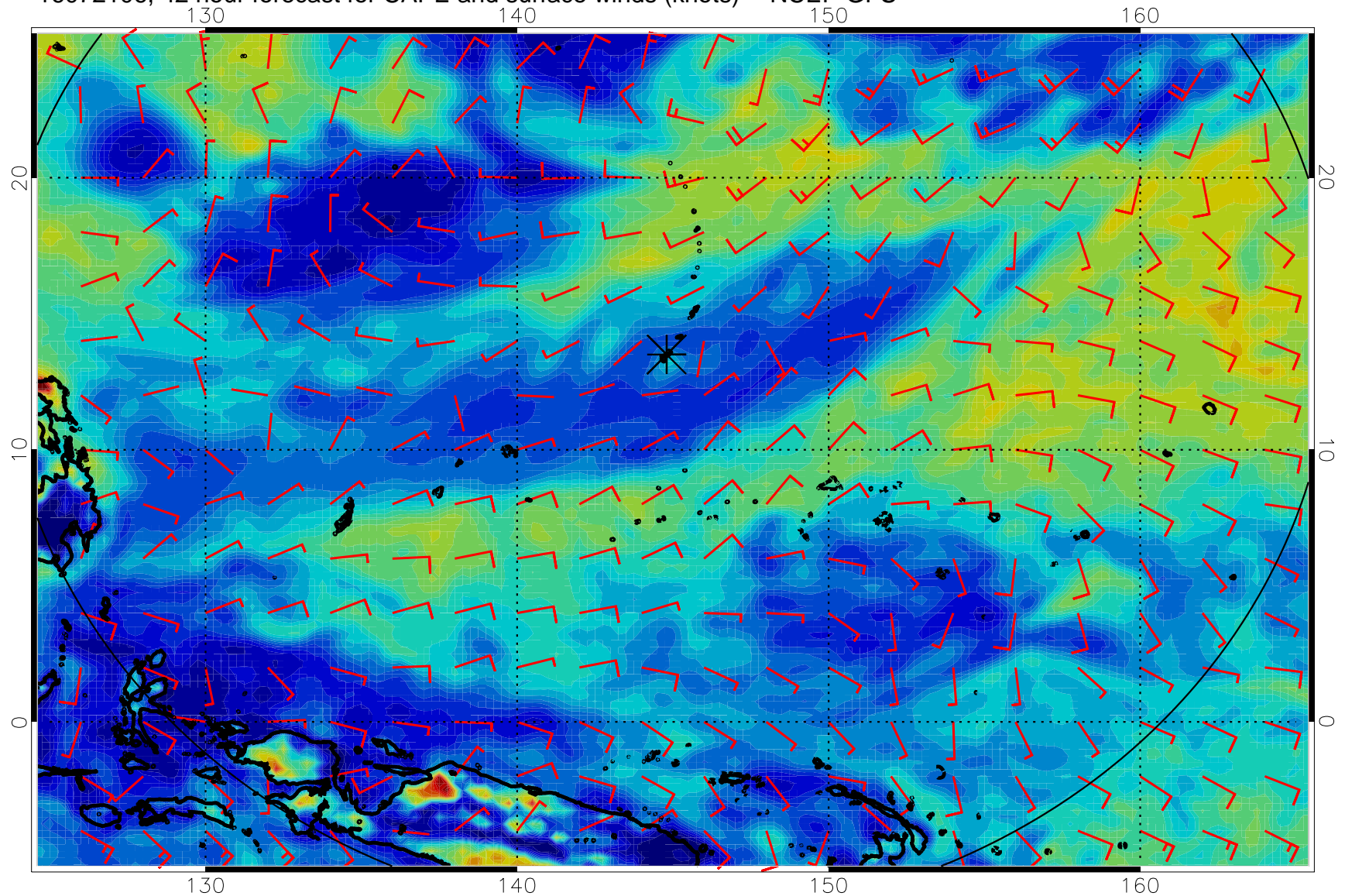
16072106, 42 hour forecast for CAPE and surface winds (knots) -- NCEP GFS
