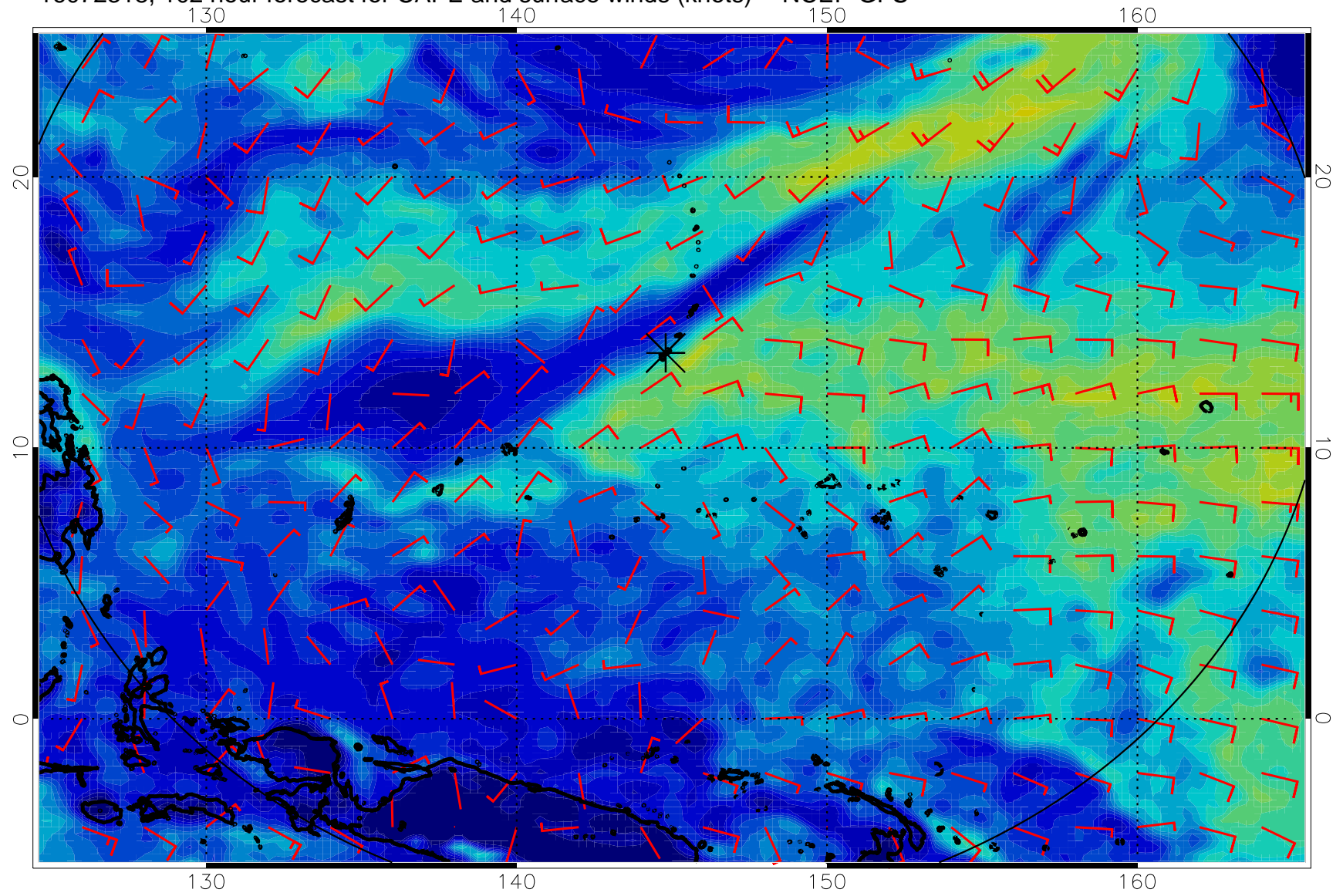
16072318, 102 hour forecast for CAPE and surface winds (knots) -- NCEP GFS
