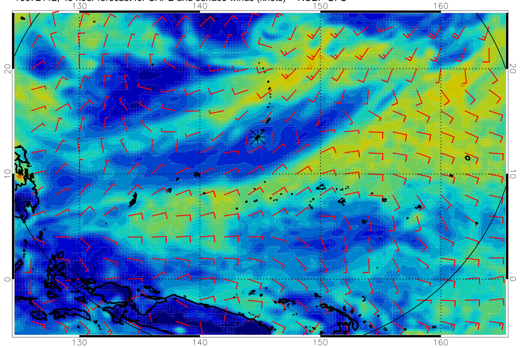
16072112, 48 hour forecast for CAPE and surface winds (knots) -- NCEP GFS
