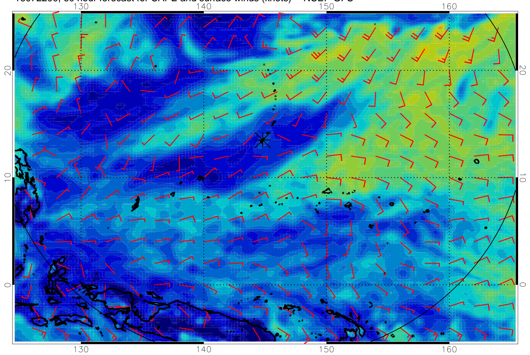
16072200, 60 hour forecast for CAPE and surface winds (knots) -- NCEP GFS
