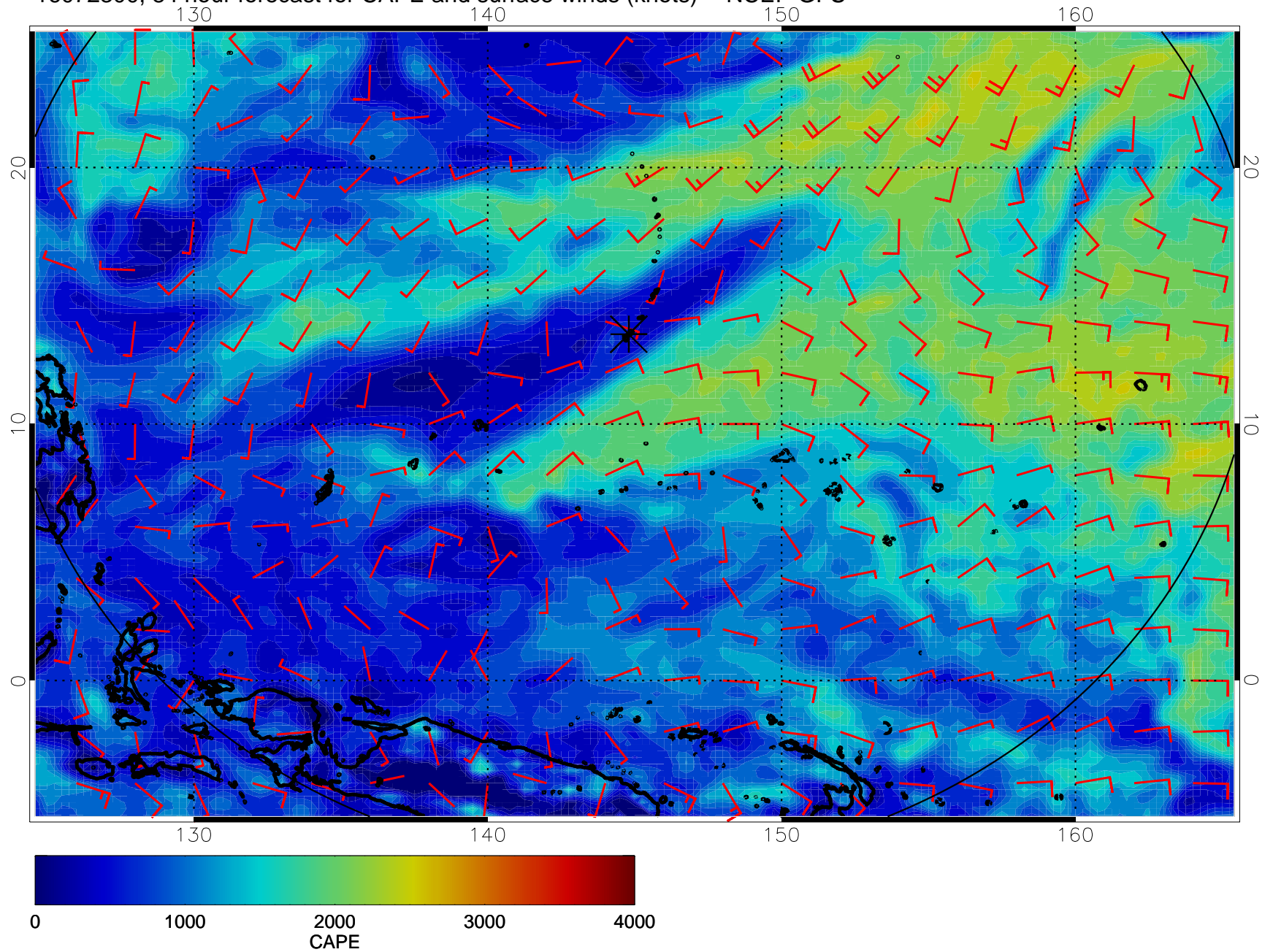
16072300, 84 hour forecast for CAPE and surface winds (knots) -- NCEP GFS
