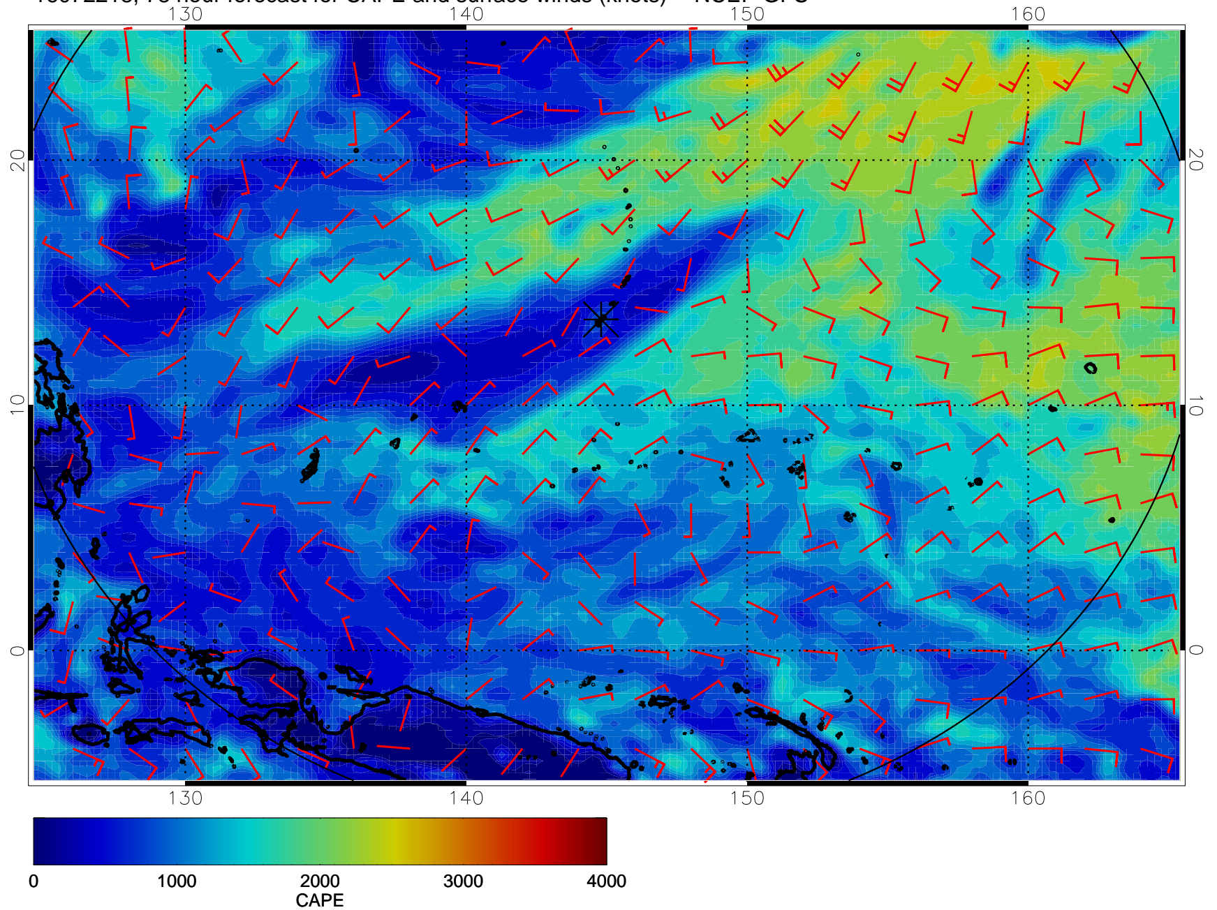
16072218, 78 hour forecast for CAPE and surface winds (knots) -- NCEP GFS
