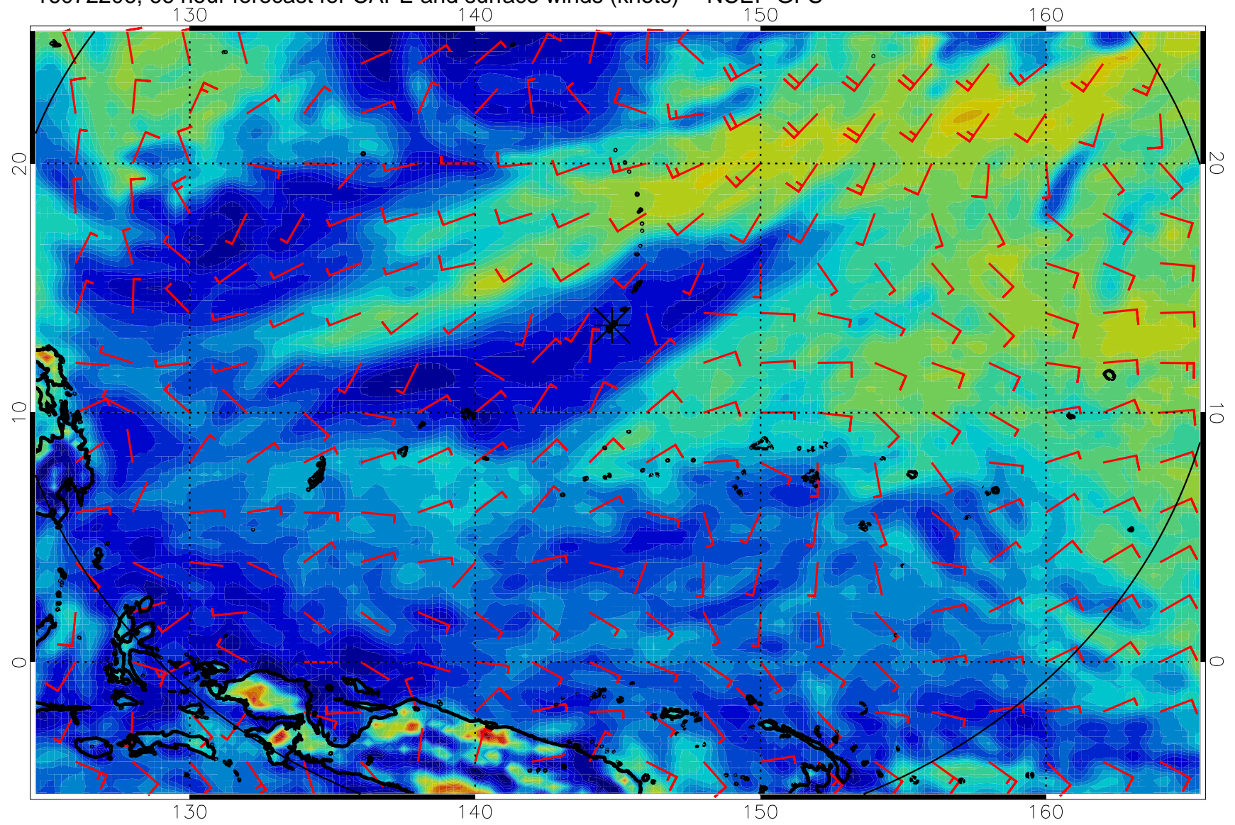
16072206, 66 hour forecast for CAPE and surface winds (knots) -- NCEP GFS
