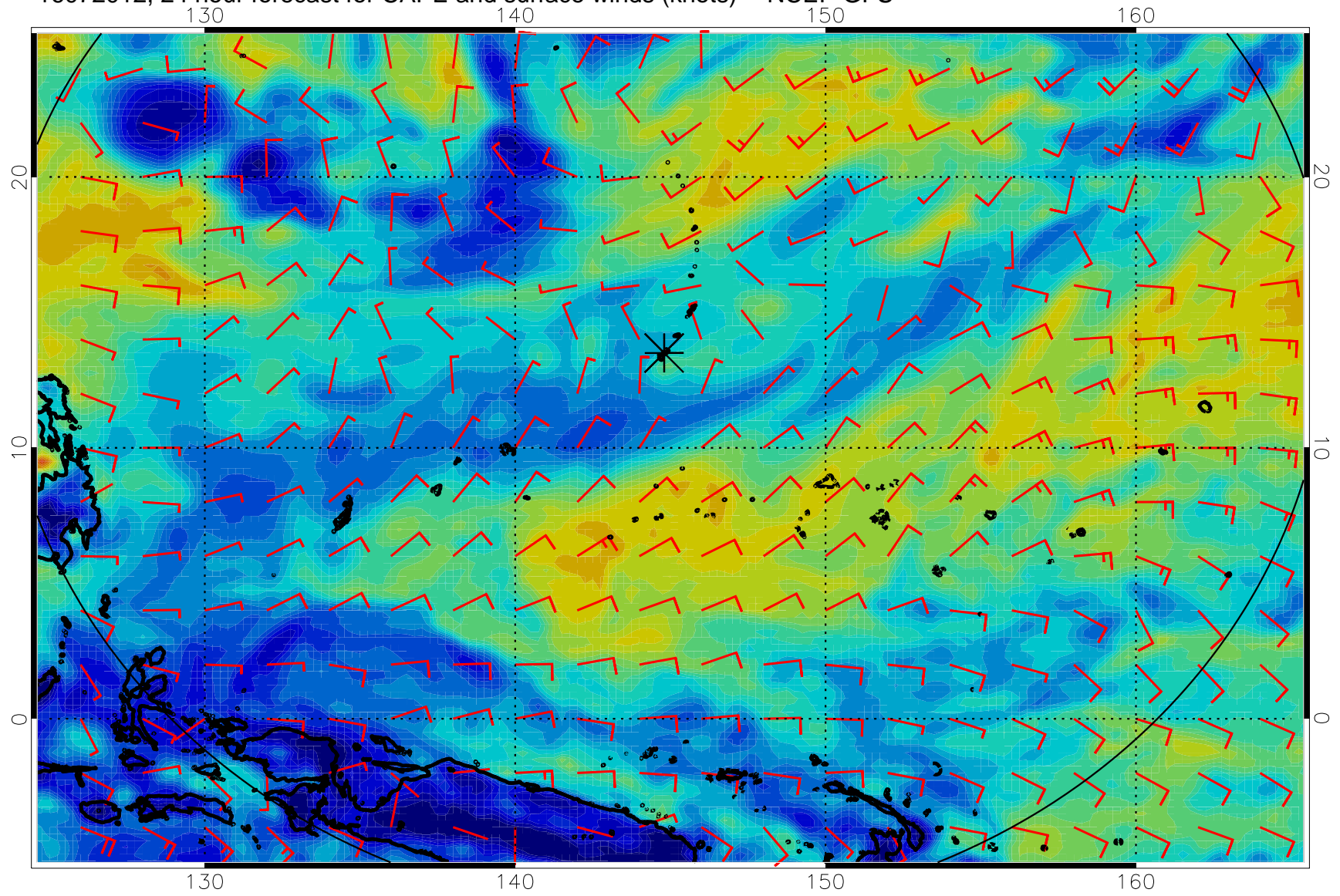
16072012, 24 hour forecast for CAPE and surface winds (knots) -- NCEP GFS
