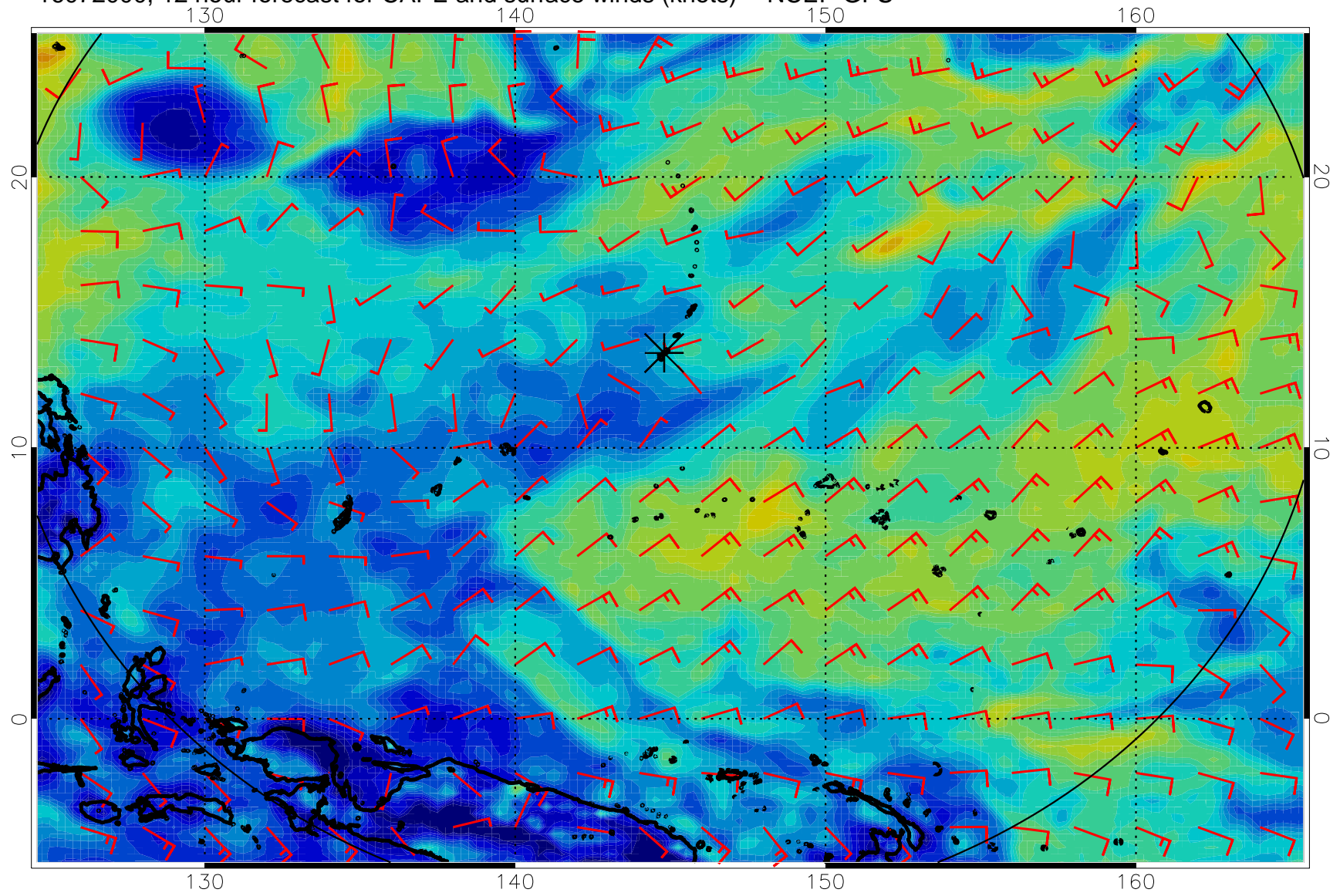
16072000, 12 hour forecast for CAPE and surface winds (knots) -- NCEP GFS
