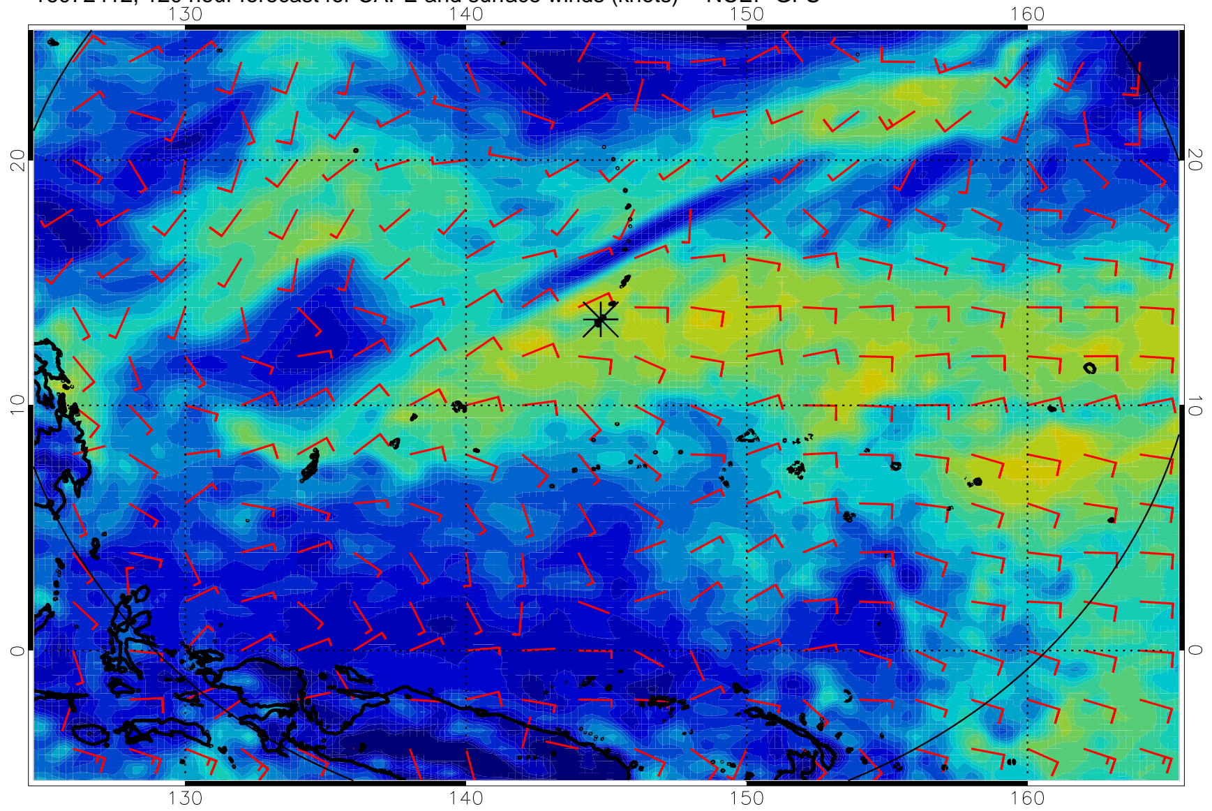
16072412, 120 hour forecast for CAPE and surface winds (knots) -- NCEP GFS
