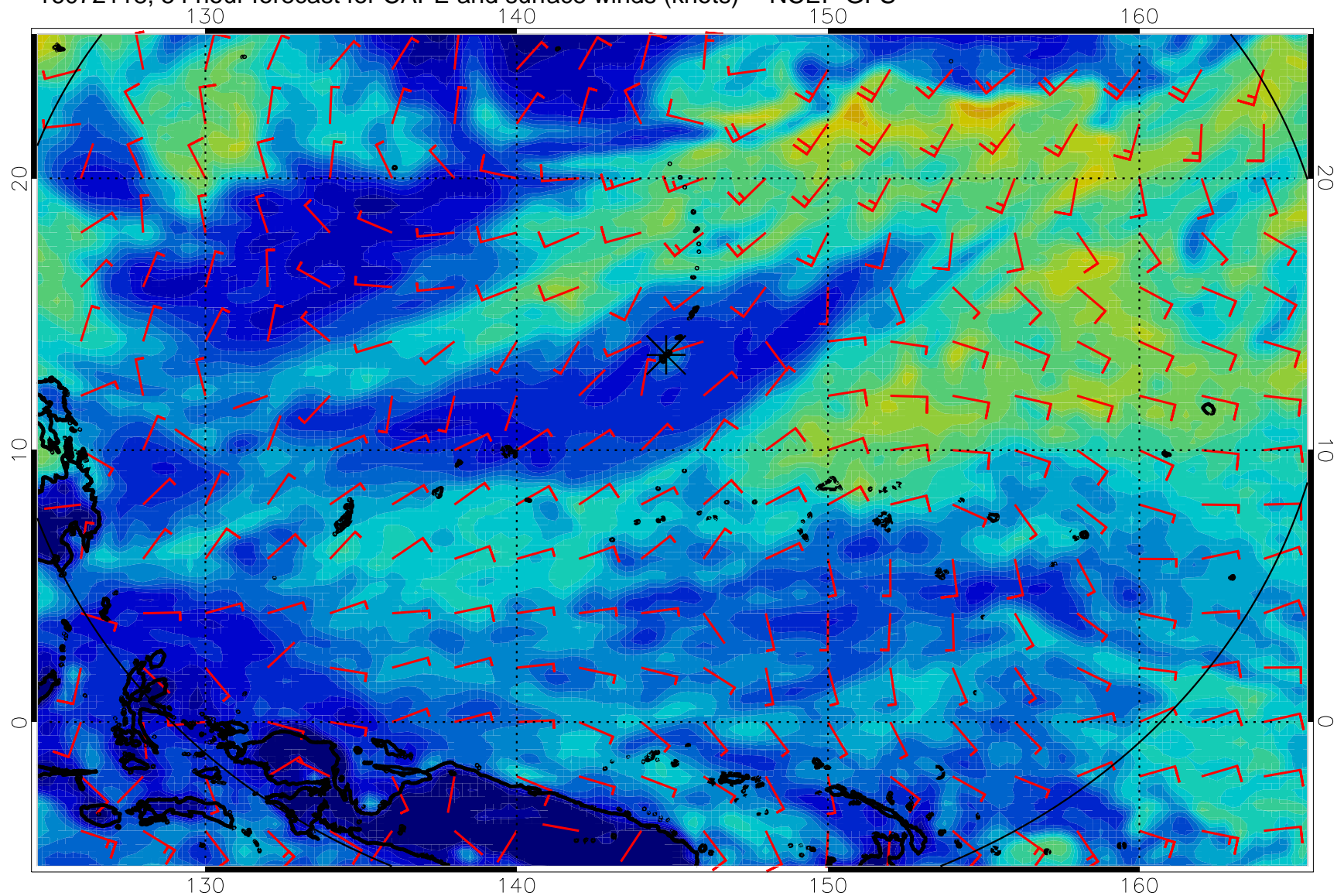
16072118, 54 hour forecast for CAPE and surface winds (knots) -- NCEP GFS
