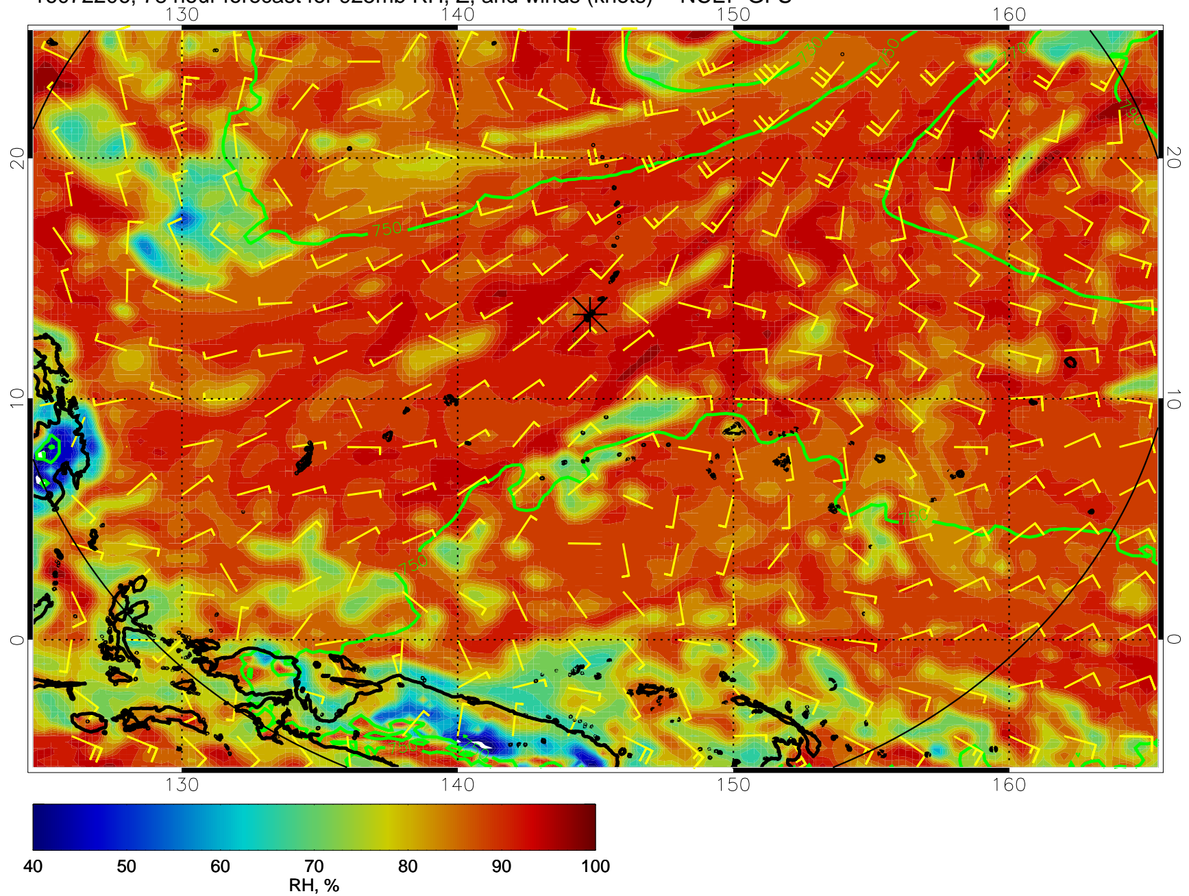
16072206, 78 hour forecast for 925mb RH, Z, and winds (knots) -- NCEP GFS
