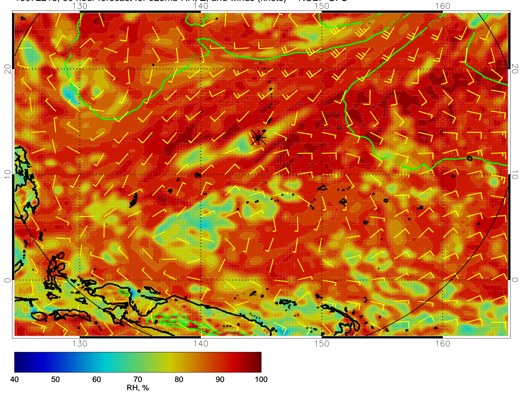
16072218, 90 hour forecast for 925mb RH, Z, and winds (knots) -- NCEP GFS
