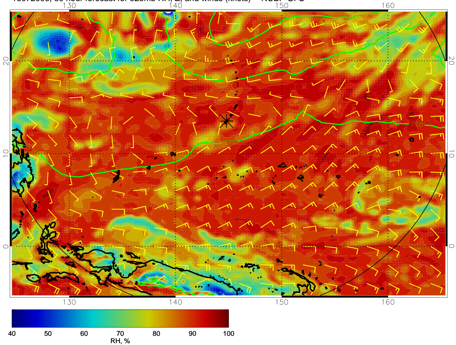
16072006, 30 hour forecast for 925mb RH, Z, and winds (knots) -- NCEP GFS
