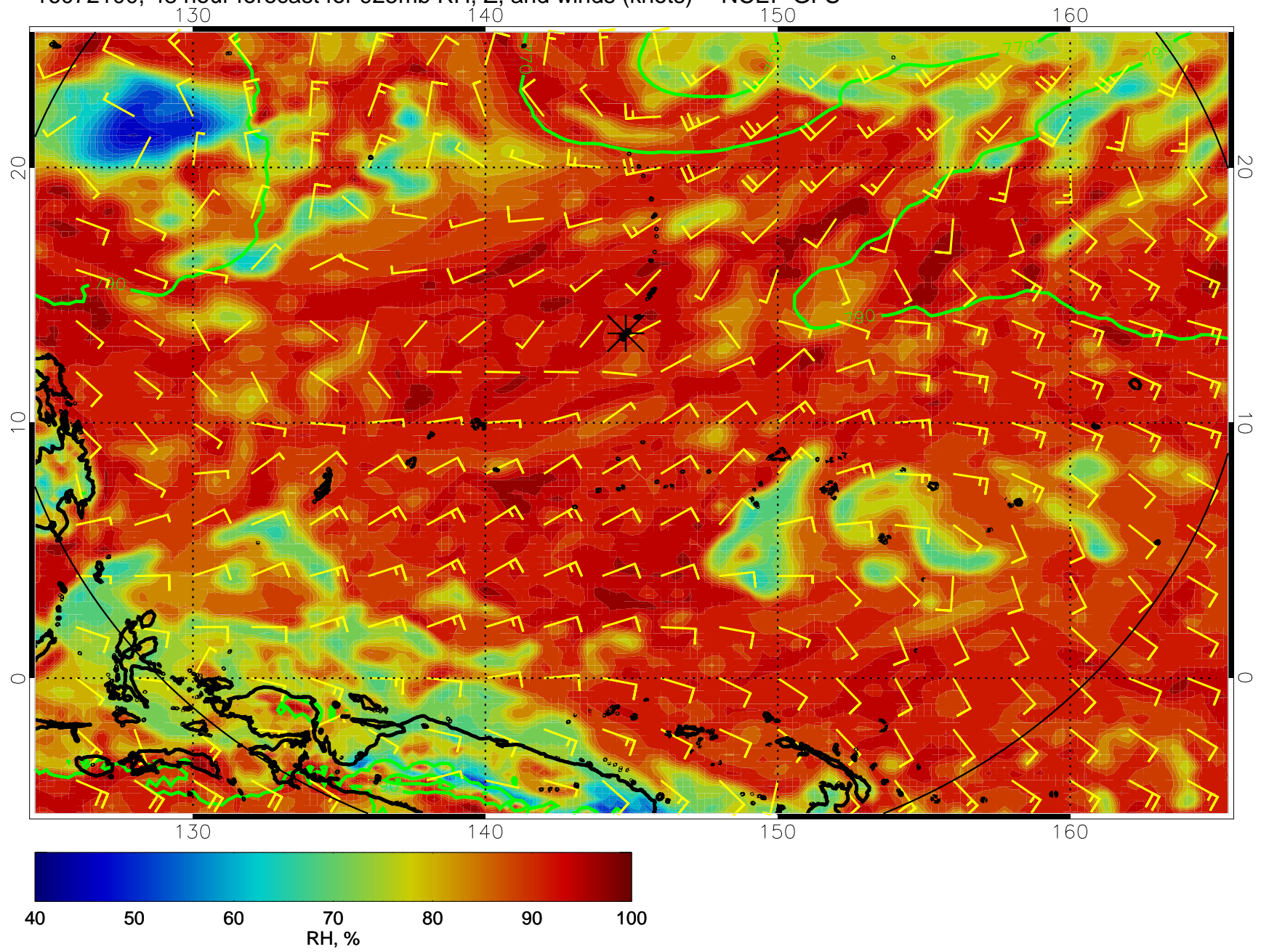
16072100, 48 hour forecast for 925mb RH, Z, and winds (knots) -- NCEP GFS
