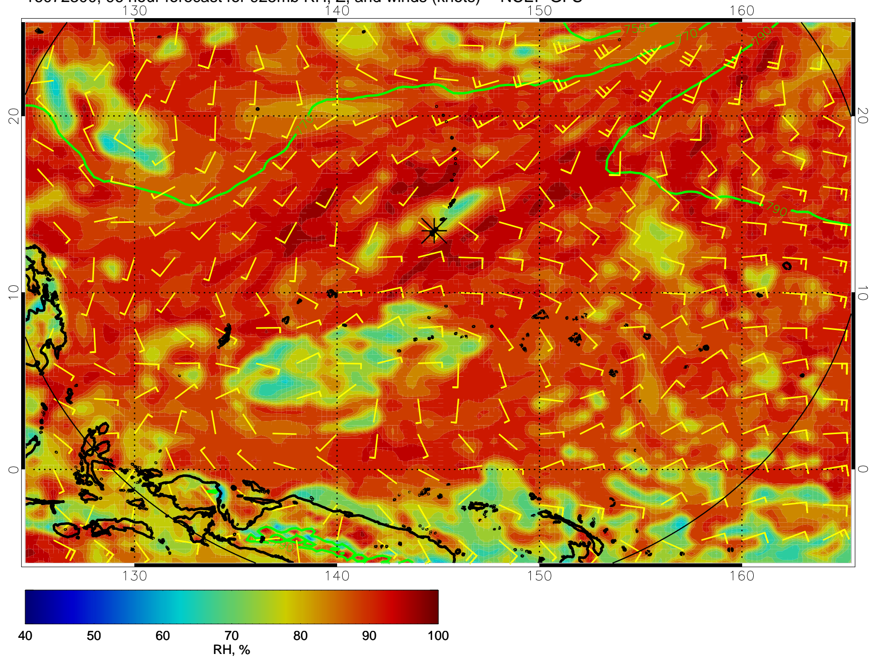
16072300, 96 hour forecast for 925mb RH, Z, and winds (knots) -- NCEP GFS
