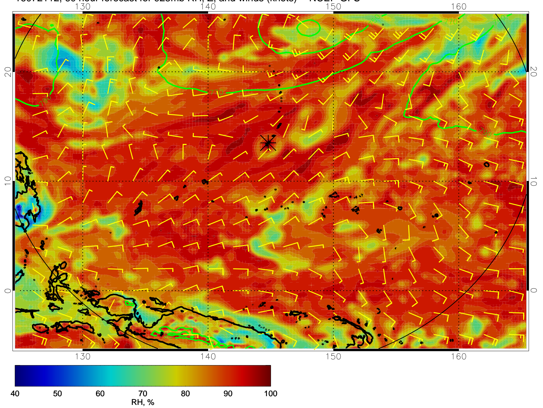
16072112, 60 hour forecast for 925mb RH, Z, and winds (knots) -- NCEP GFS
