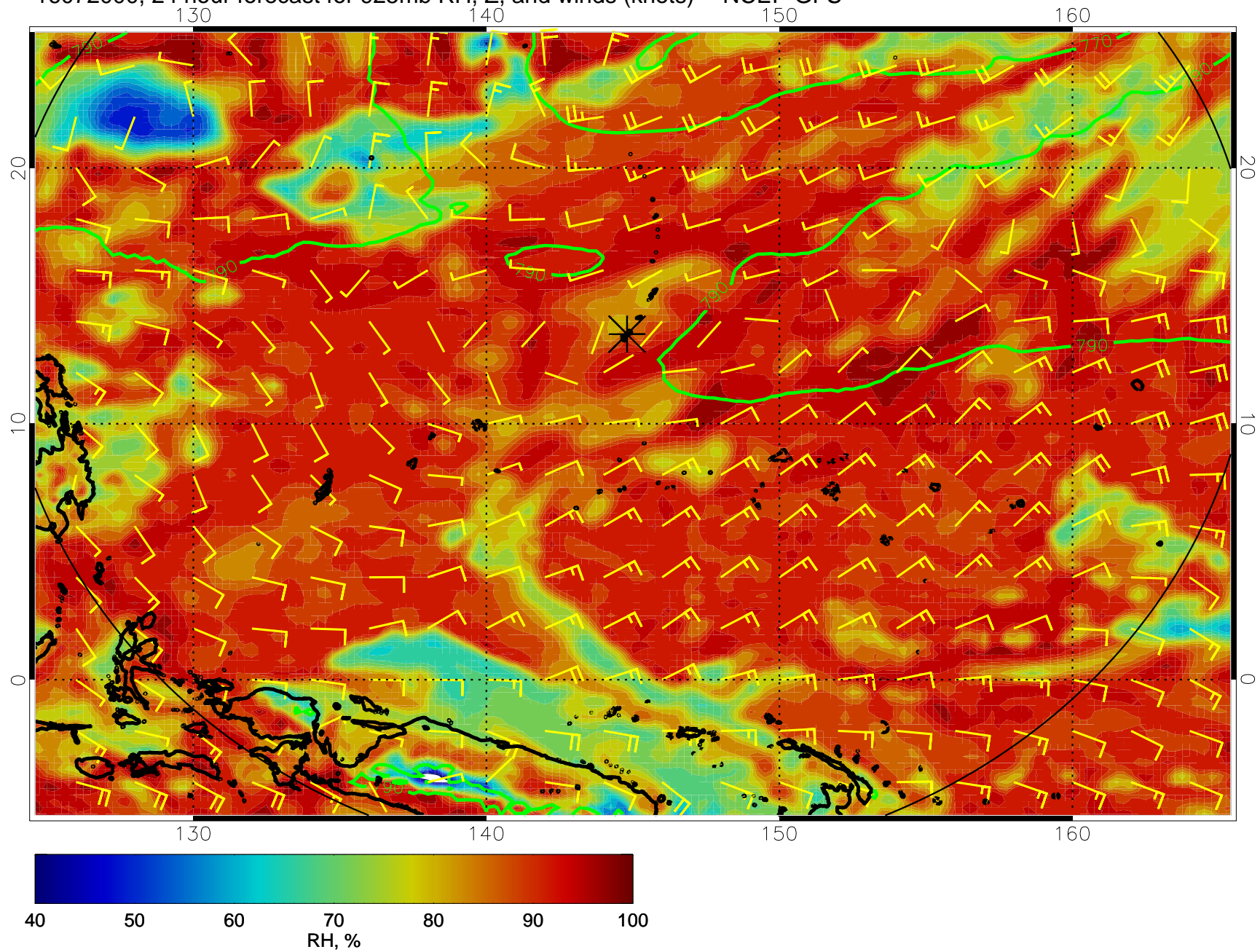
16072000, 24 hour forecast for 925mb RH, Z, and winds (knots) -- NCEP GFS
