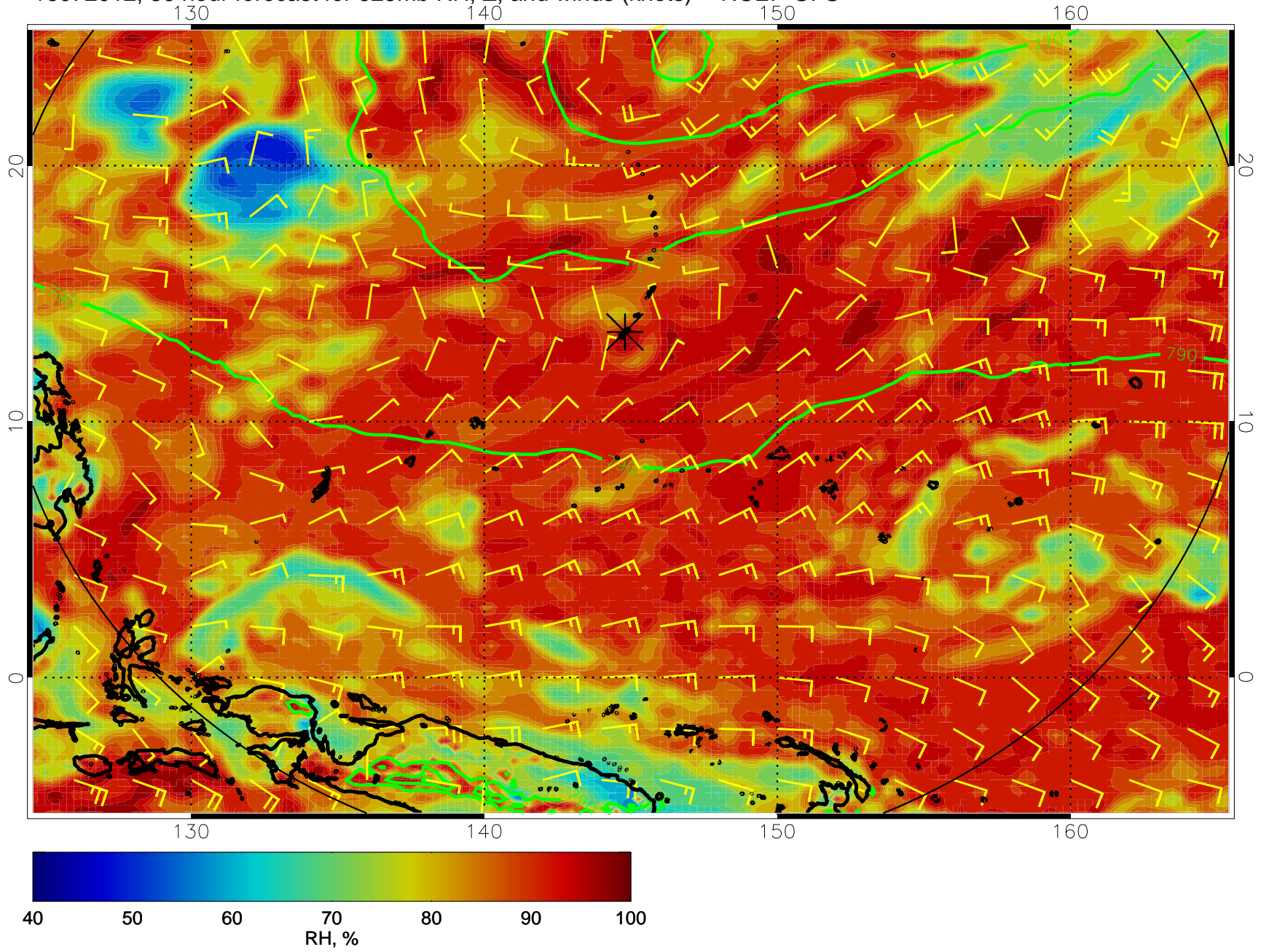
16072012, 36 hour forecast for 925mb RH, Z, and winds (knots) -- NCEP GFS
