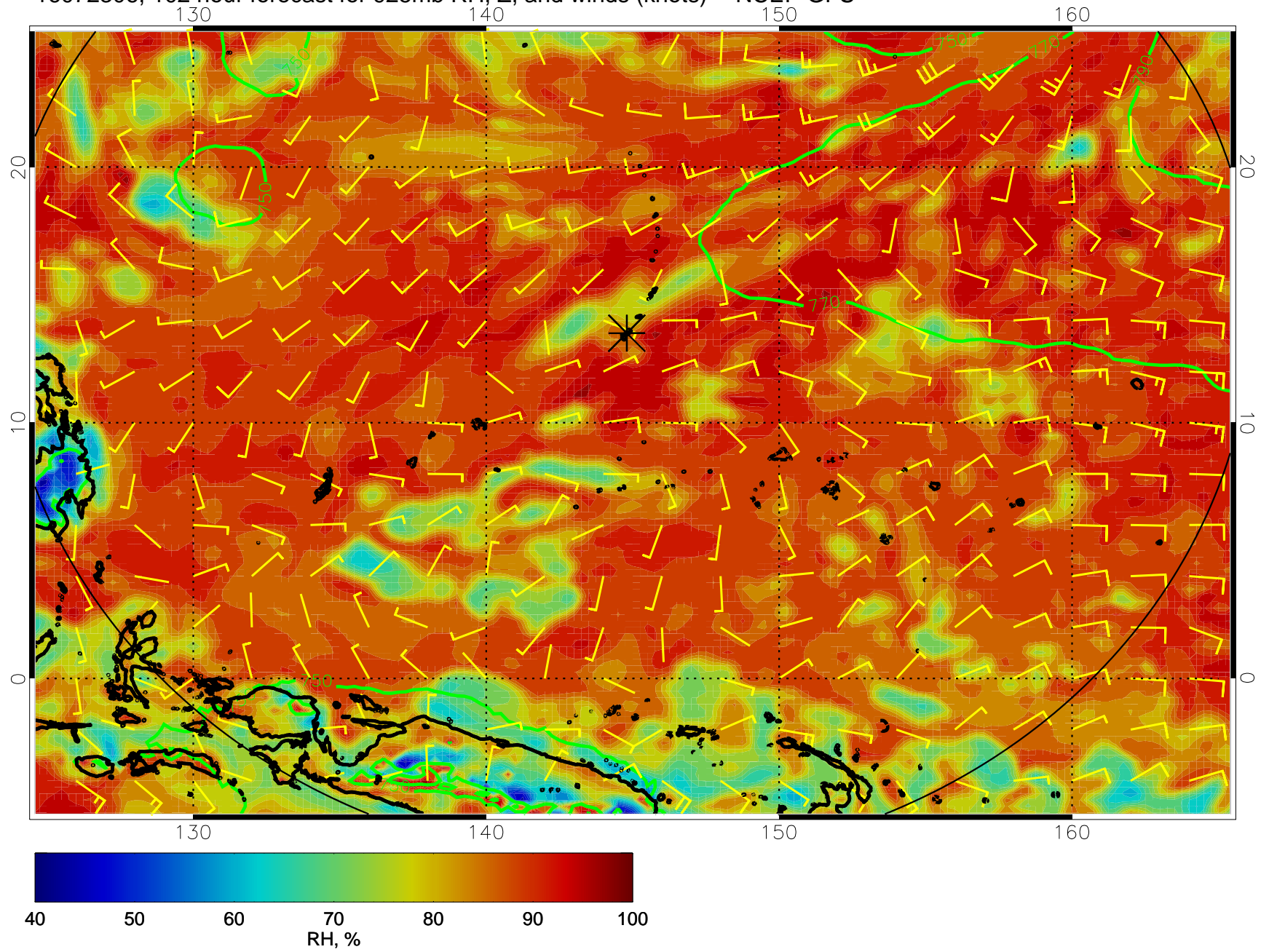
16072306, 102 hour forecast for 925mb RH, Z, and winds (knots) -- NCEP GFS
