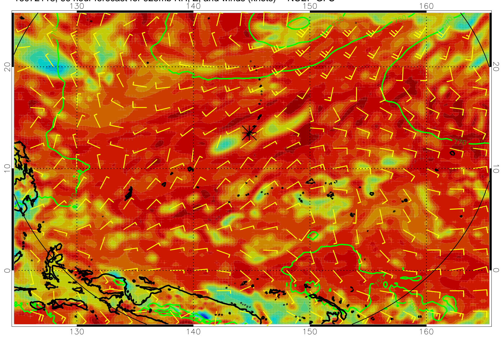
16072118, 66 hour forecast for 925mb RH, Z, and winds (knots) -- NCEP GFS
