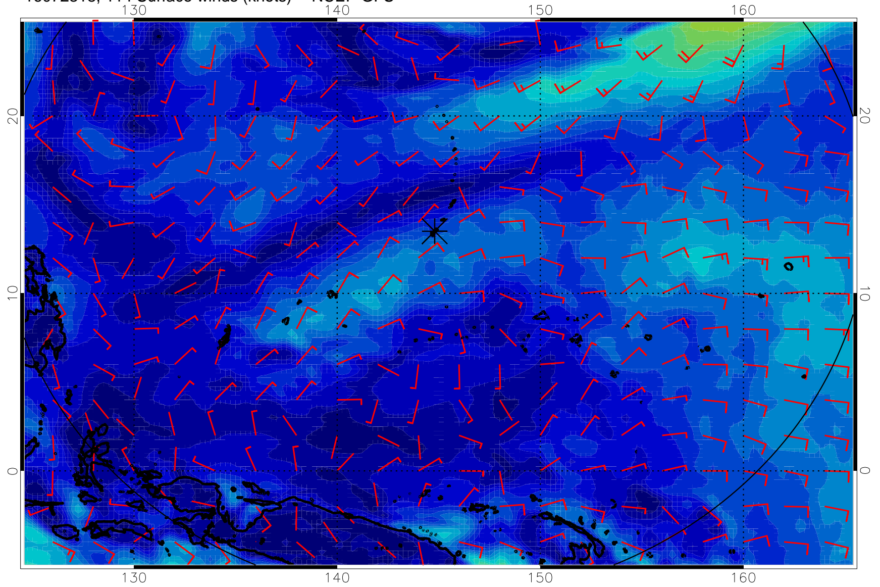
16072318, 114 Surface winds (knots) -- NCEP GFS
