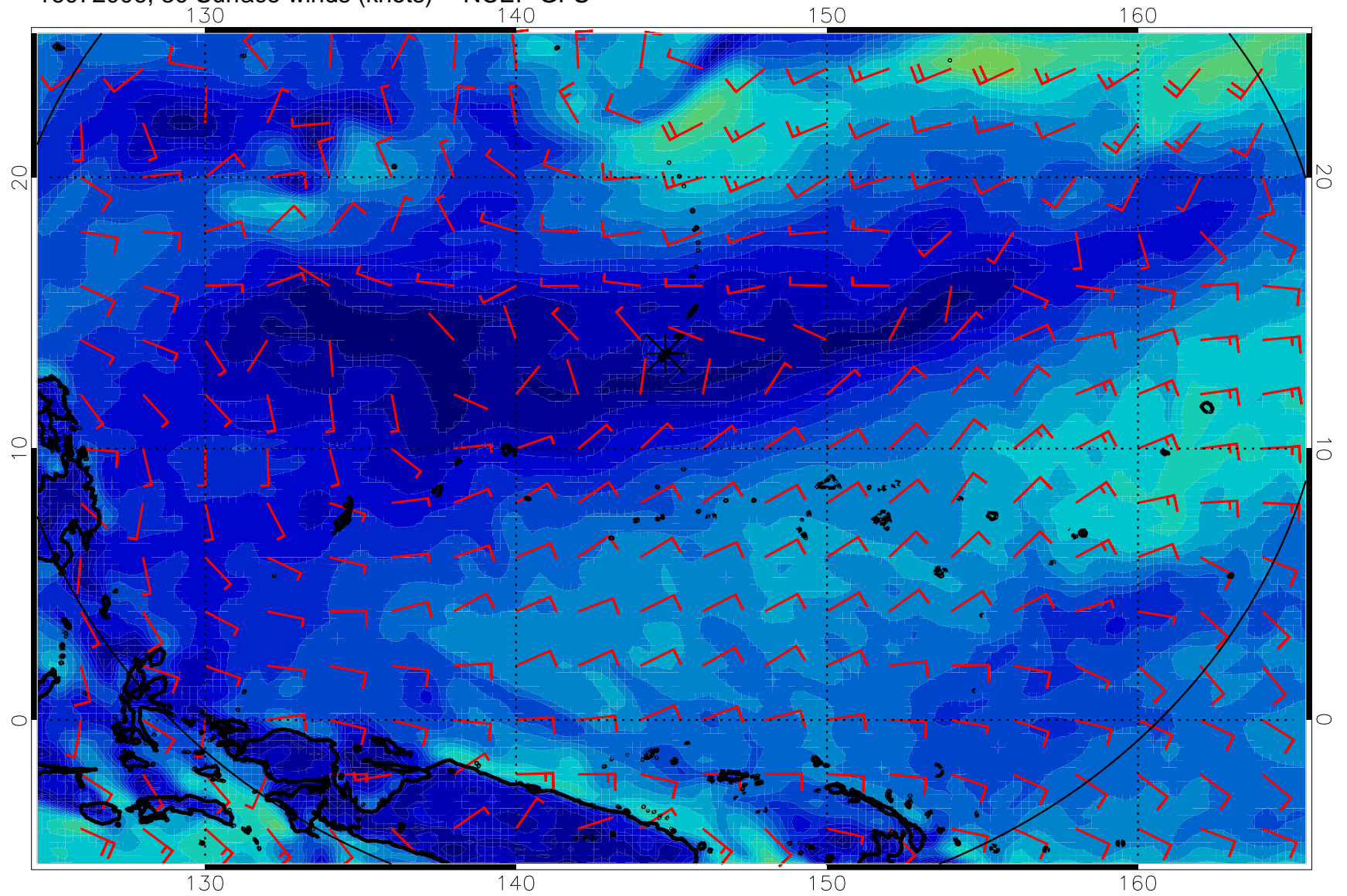
16072006, 30 Surface winds (knots) -- NCEP GFS
