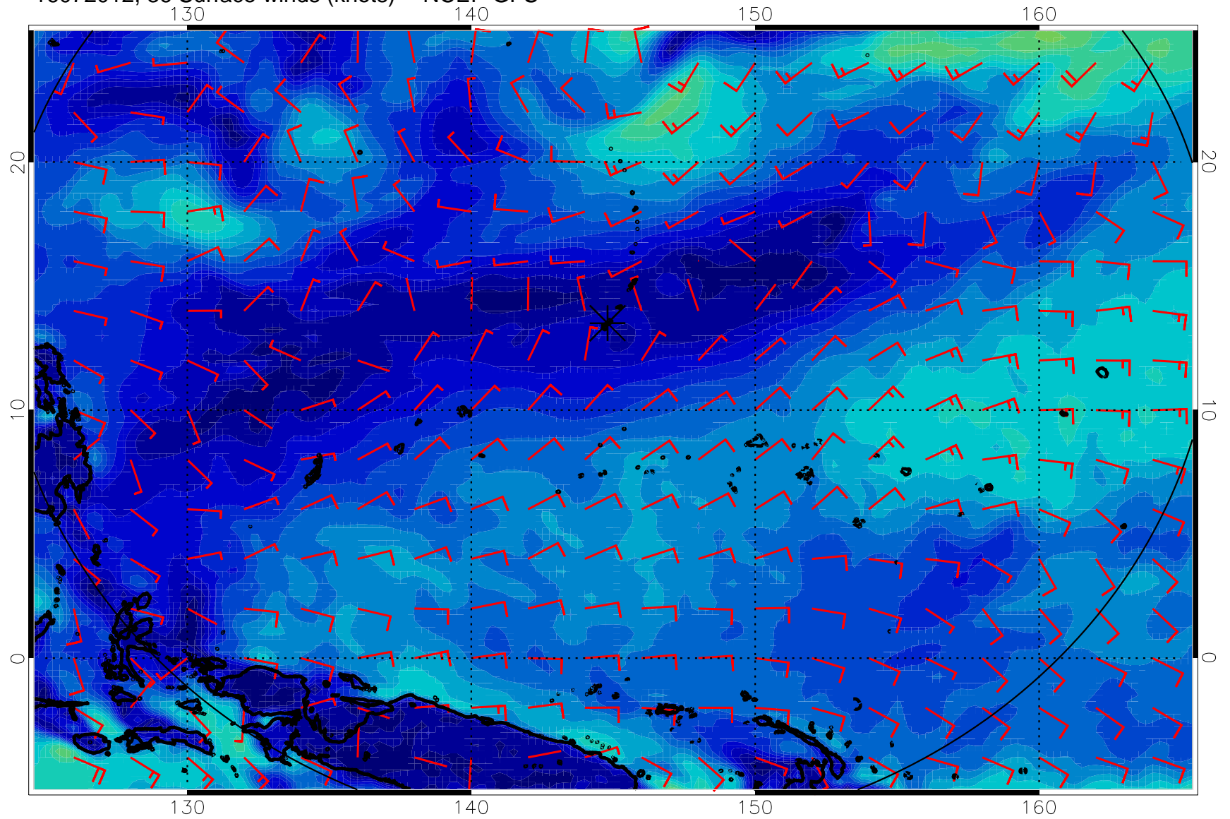
16072012, 36 Surface winds (knots) -- NCEP GFS
