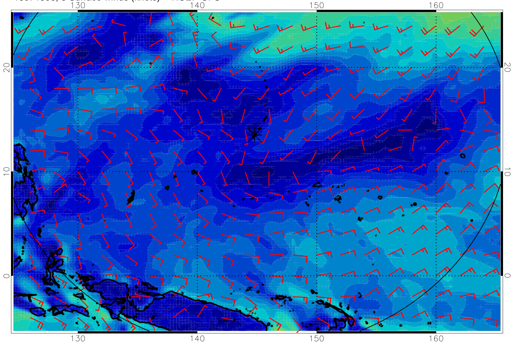
16071906, 6 Surface winds (knots) -- NCEP GFS
