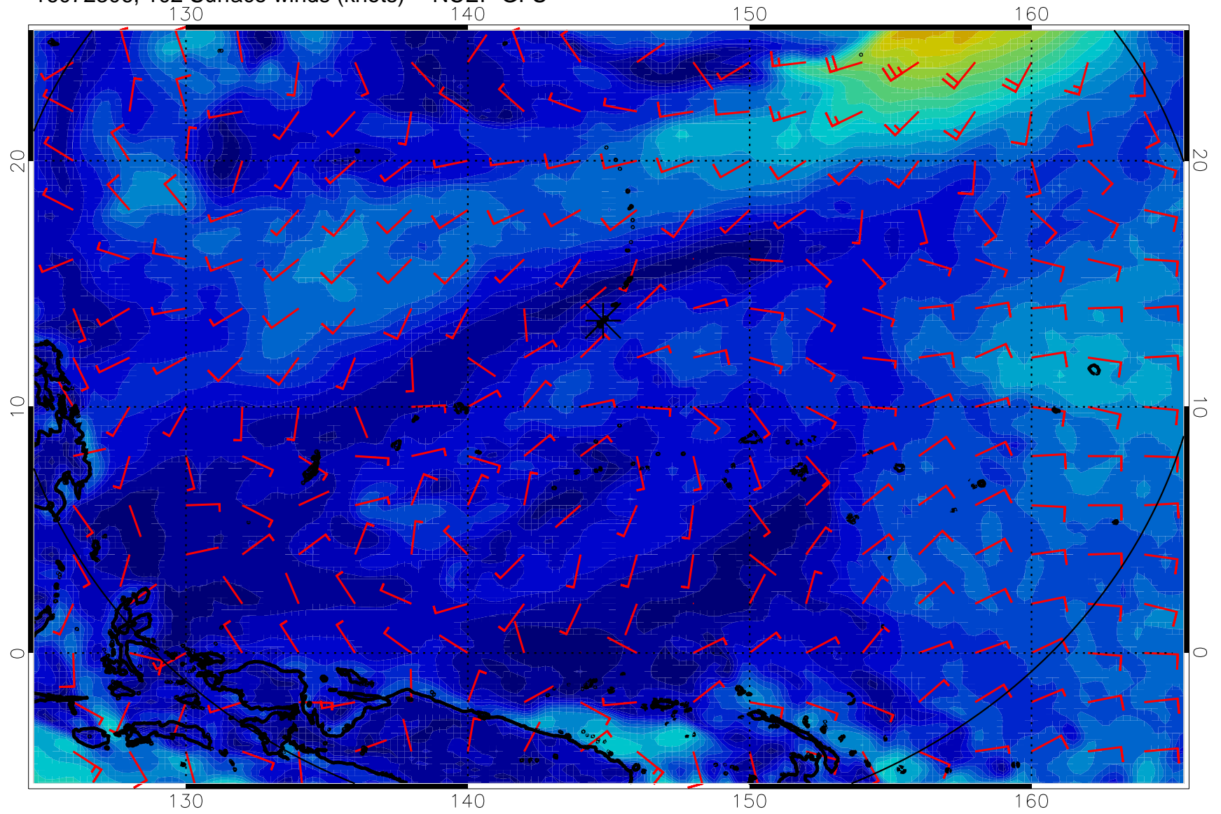
16072306, 102 Surface winds (knots) -- NCEP GFS
