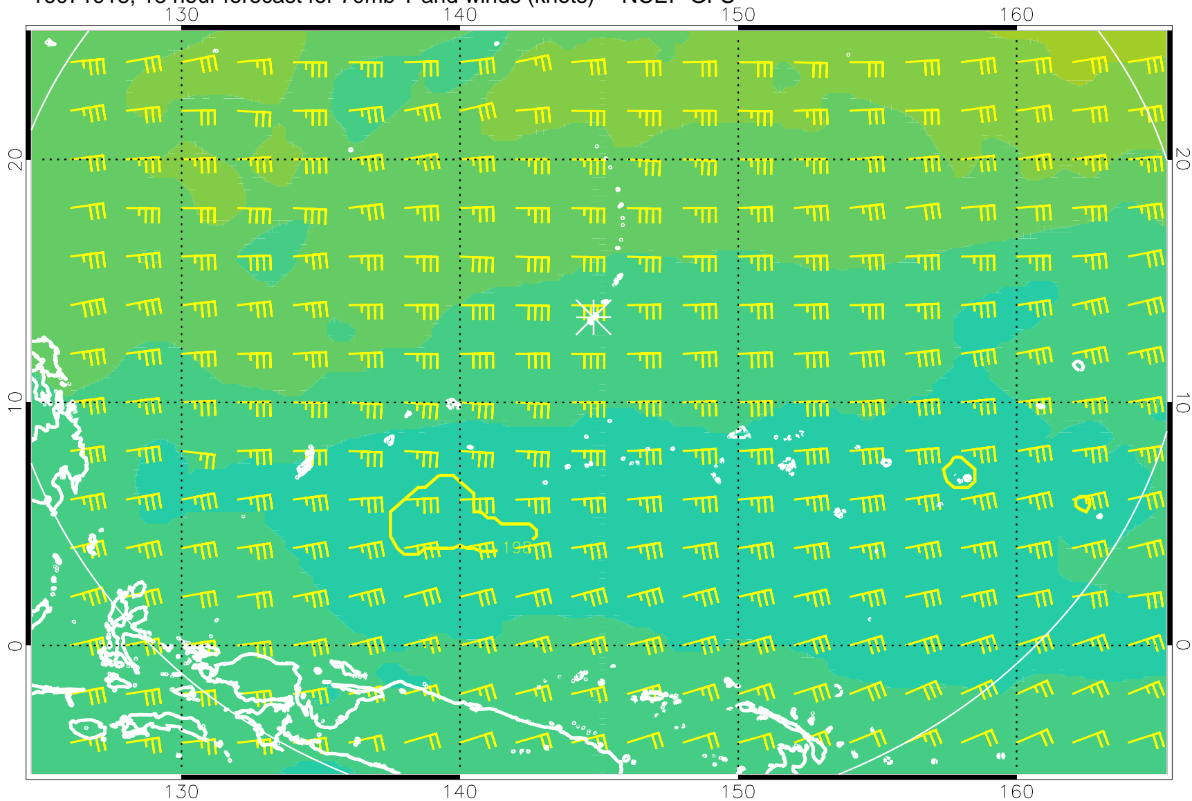
16071918, 18 hour forecast for 70mb T and winds (knots) -- NCEP GFS
