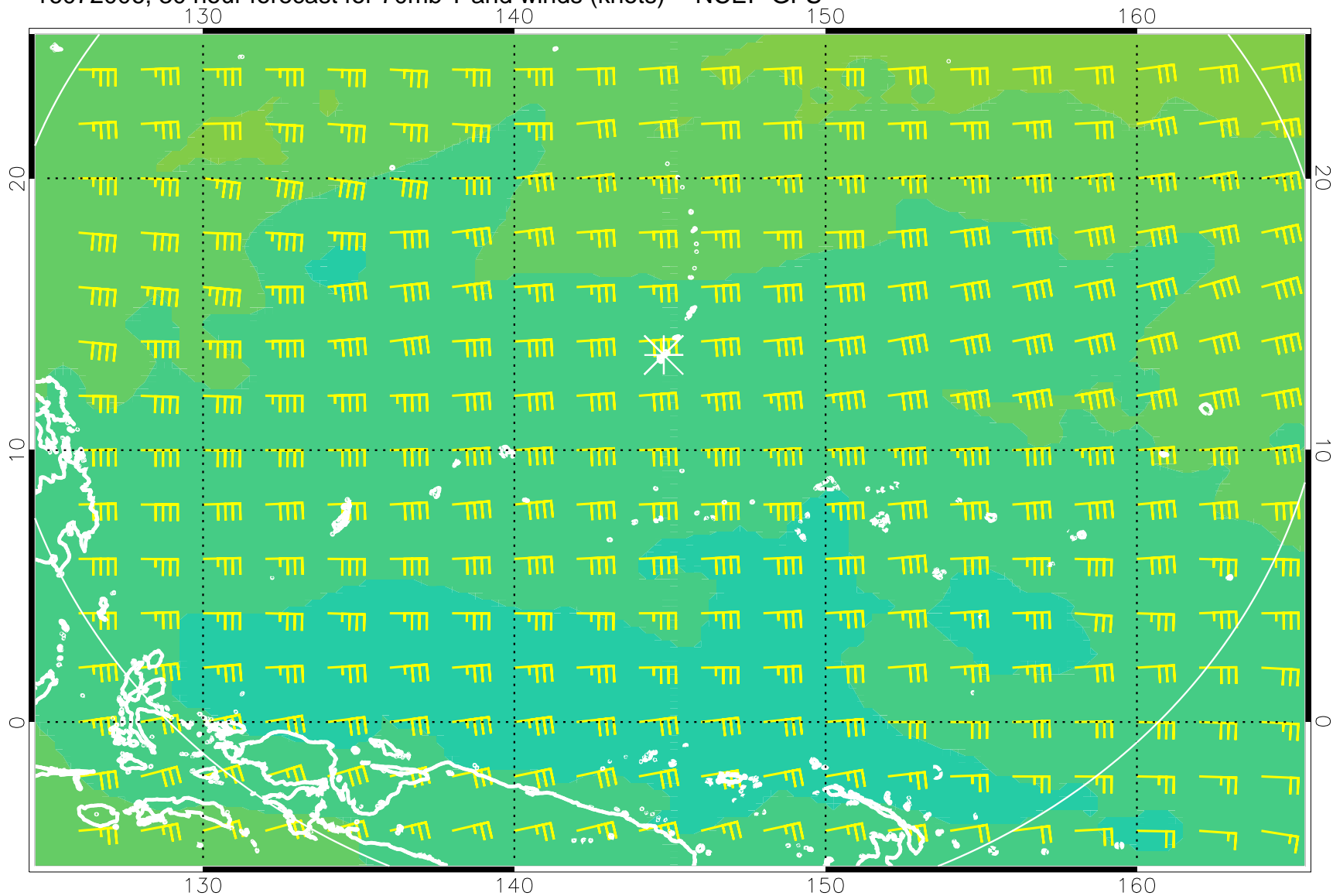
16072006, 30 hour forecast for 70mb T and winds (knots) -- NCEP GFS
