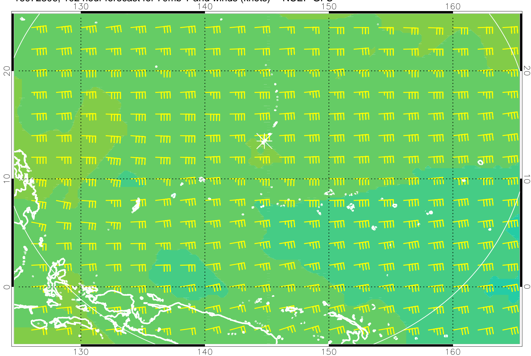
16072306, 102 hour forecast for 70mb T and winds (knots) -- NCEP GFS
