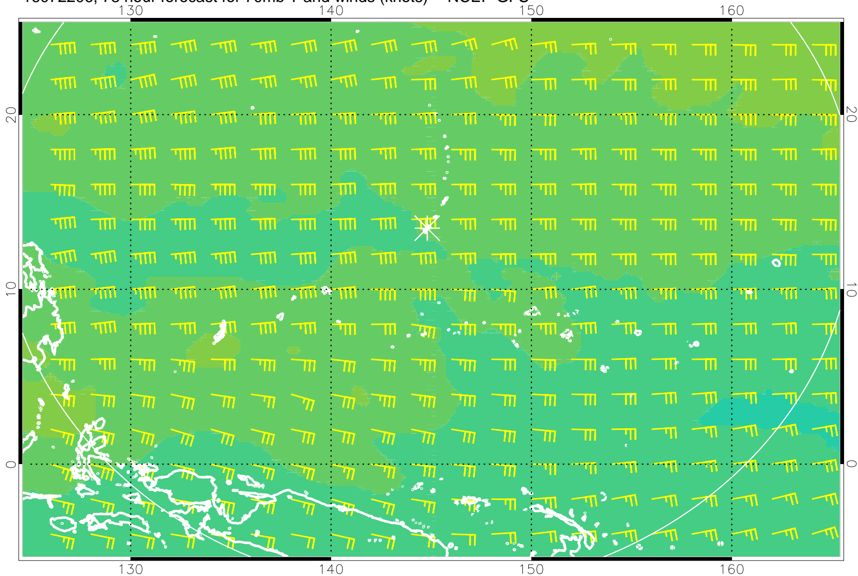
16072206, 78 hour forecast for 70mb T and winds (knots) -- NCEP GFS
