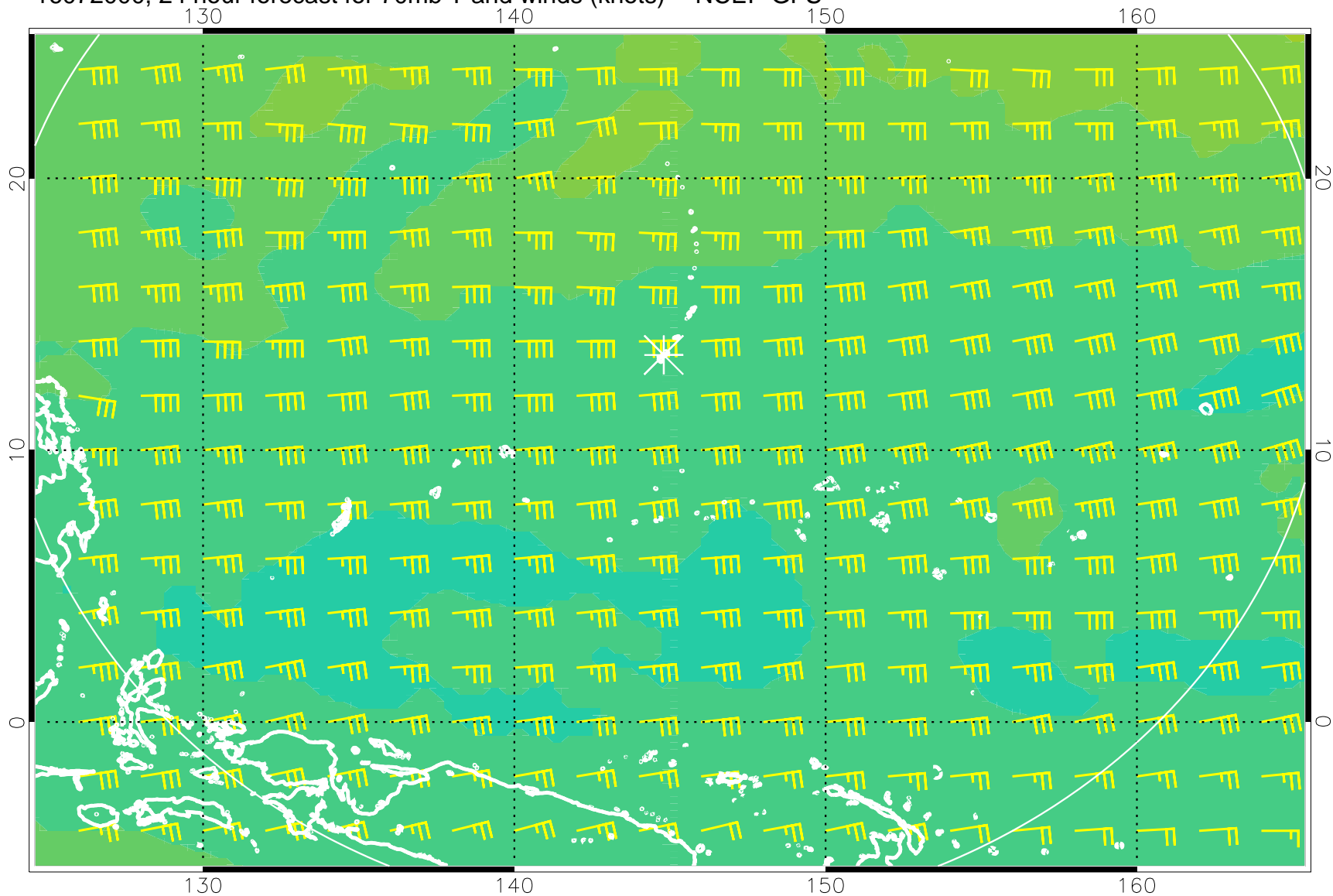
16072000, 24 hour forecast for 70mb T and winds (knots) -- NCEP GFS
