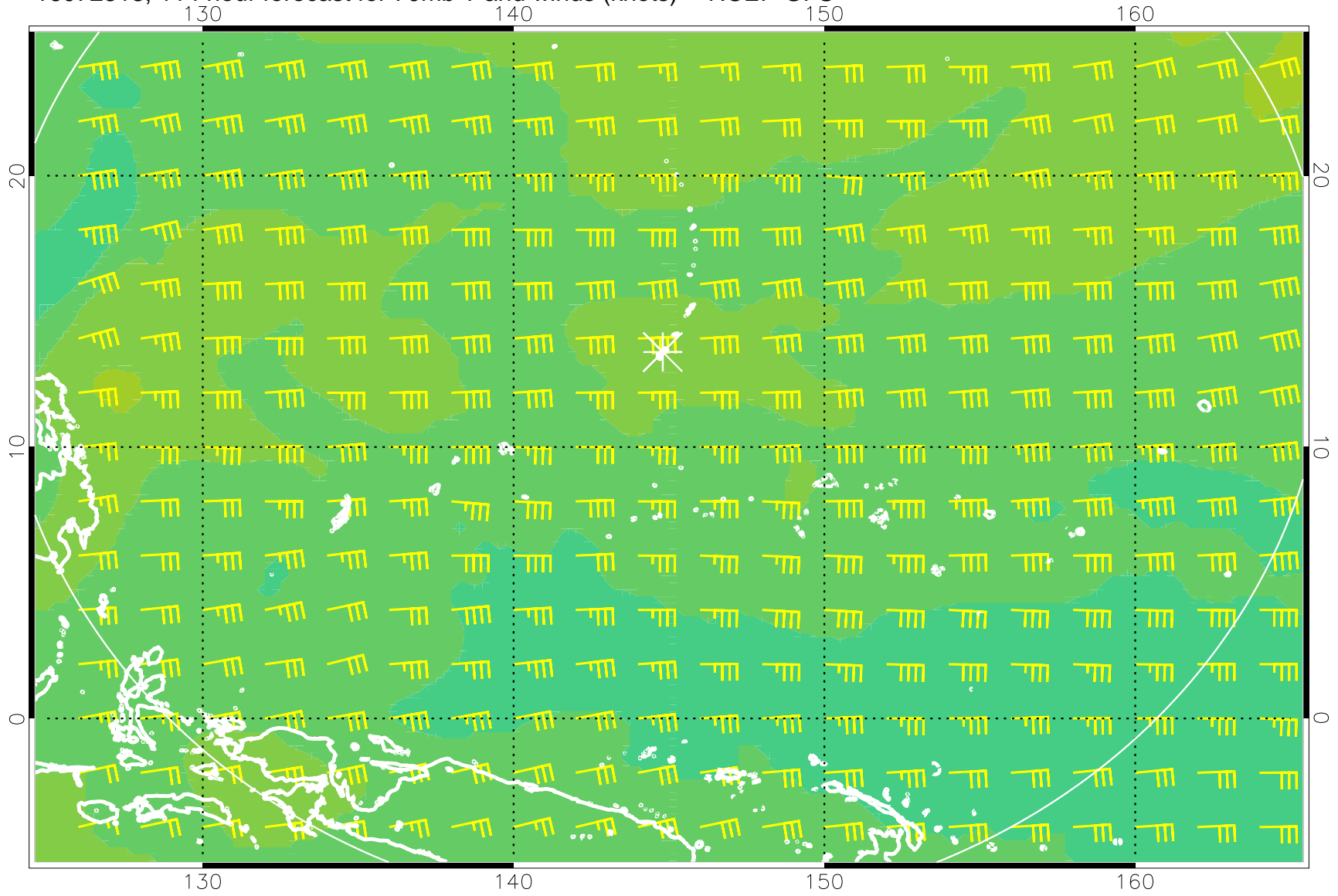
16072318, 114 hour forecast for 70mb T and winds (knots) -- NCEP GFS
