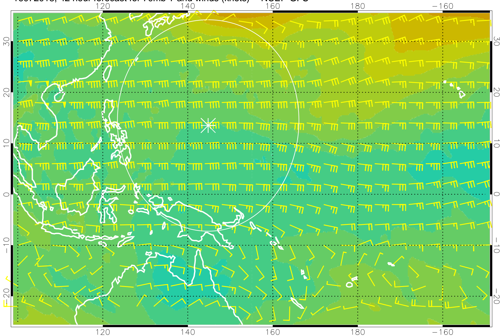
16072018, 42 hour forecast for 70mb T and winds (knots) -- NCEP GFS
