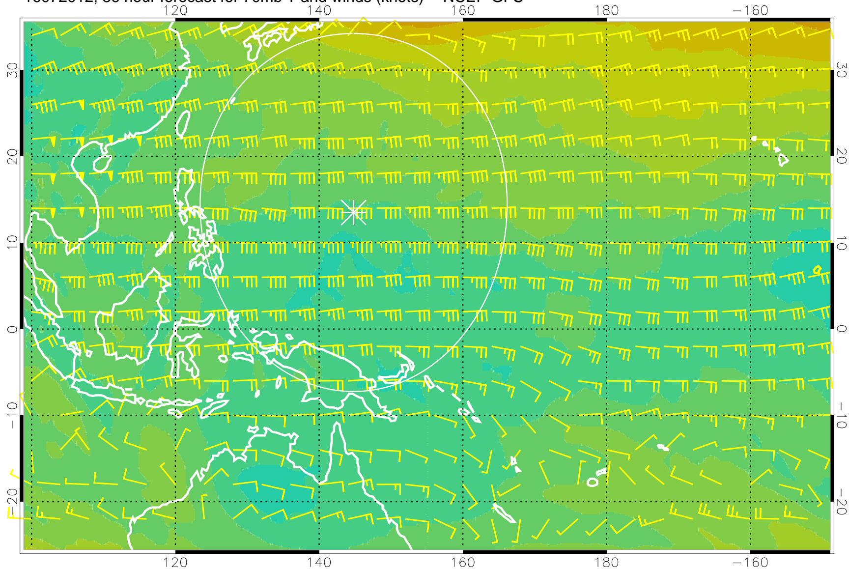
16072012, 36 hour forecast for 70mb T and winds (knots) -- NCEP GFS
