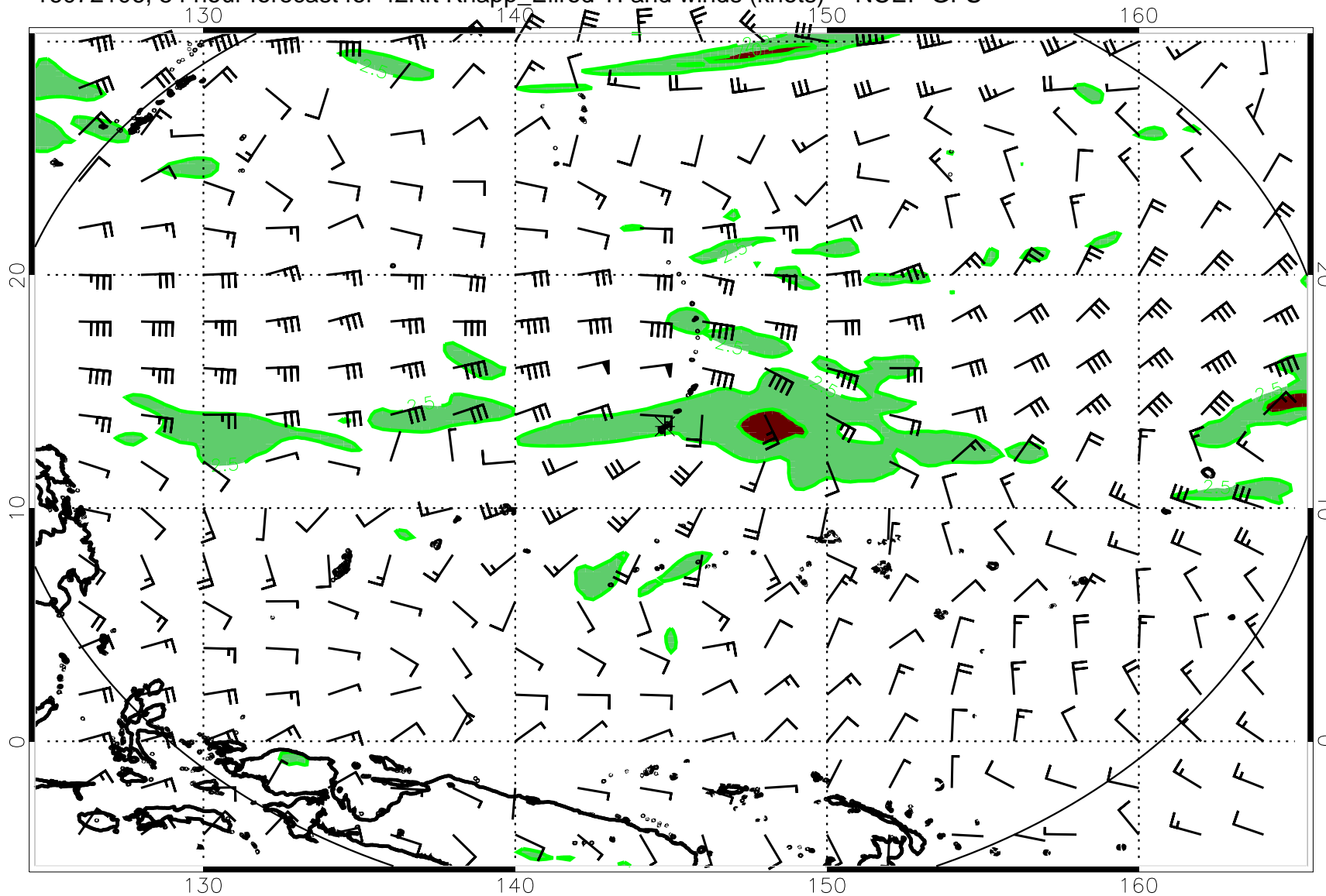
16072106, 54 hour forecast for 42Kft Knapp_Ellrod TI and winds (knots) -- NCEP GFS
