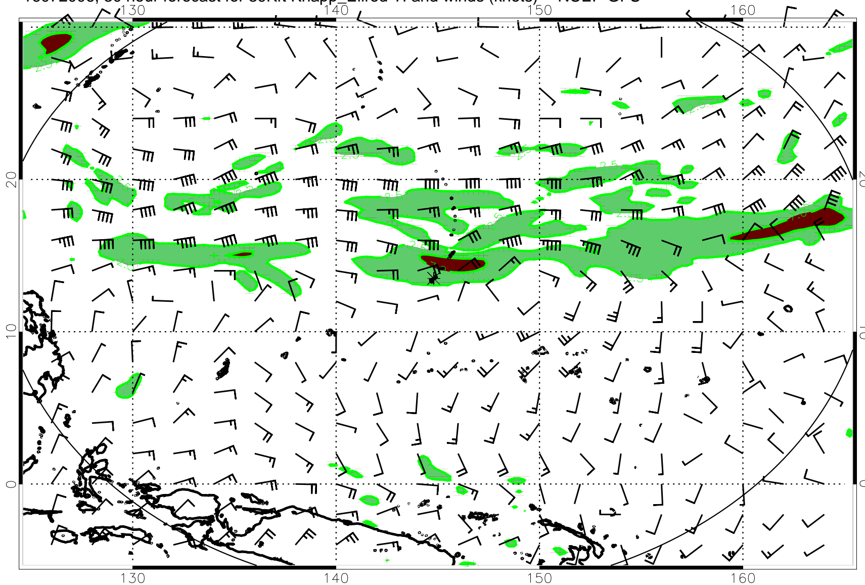
16072006, 30 hour forecast for 39Kft Knapp_Ellrod TI and winds (knots) -- NCEP GFS
