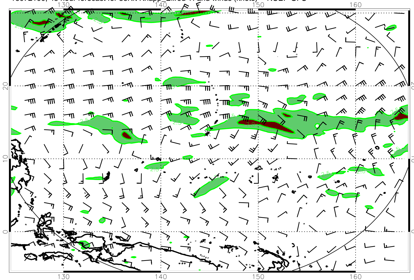
16072100, 48 hour forecast for 36Kft Knapp_Ellrod TI and winds (knots) -- NCEP GFS
