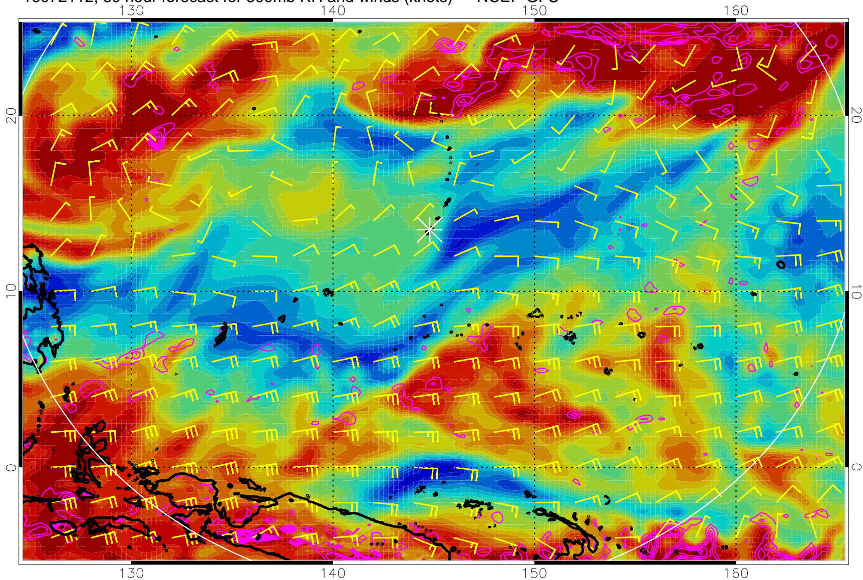
16072112, 60 hour forecast for 500mb RH and winds (knots) -- NCEP GFS
