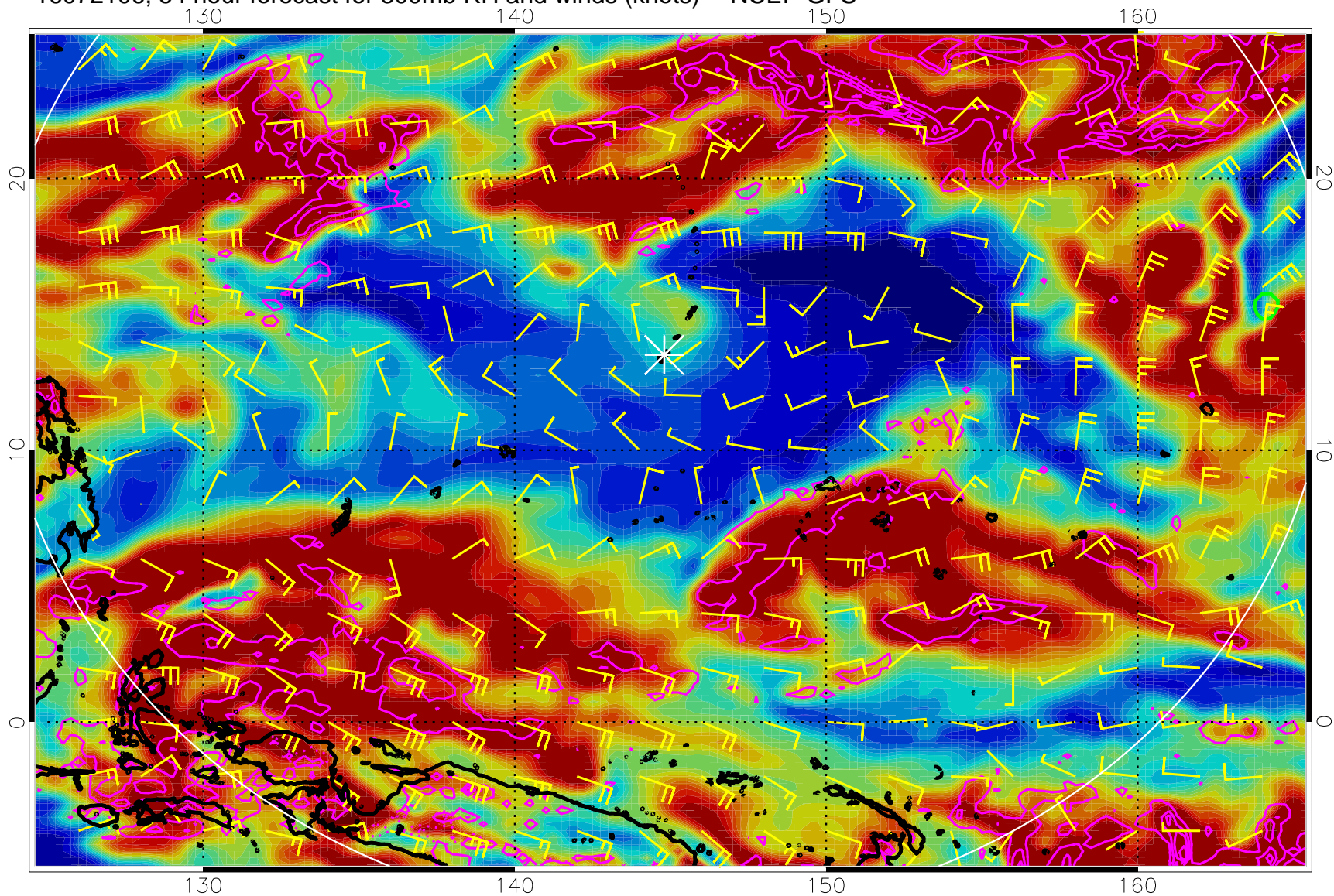
16072106, 54 hour forecast for 300mb RH and winds (knots) -- NCEP GFS
