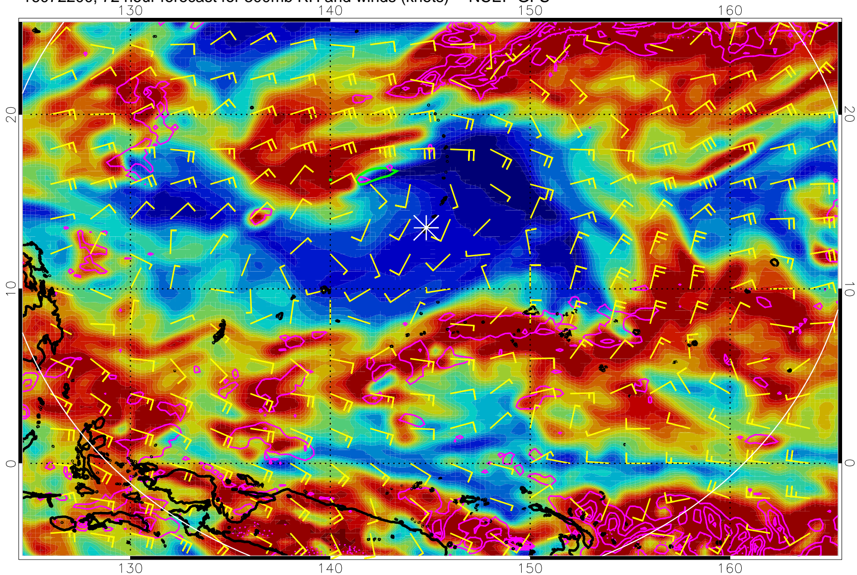
16072200, 72 hour forecast for 300mb RH and winds (knots) -- NCEP GFS
