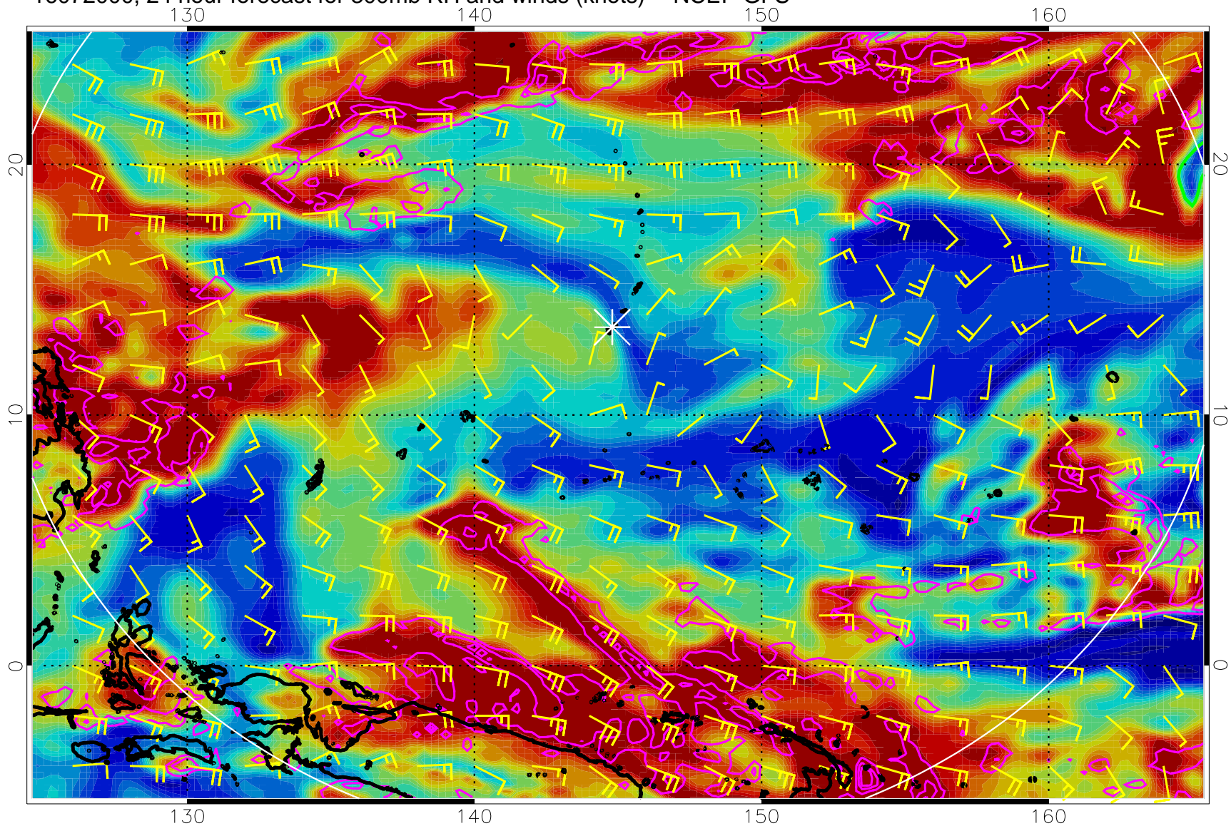
16072000, 24 hour forecast for 300mb RH and winds (knots) -- NCEP GFS
