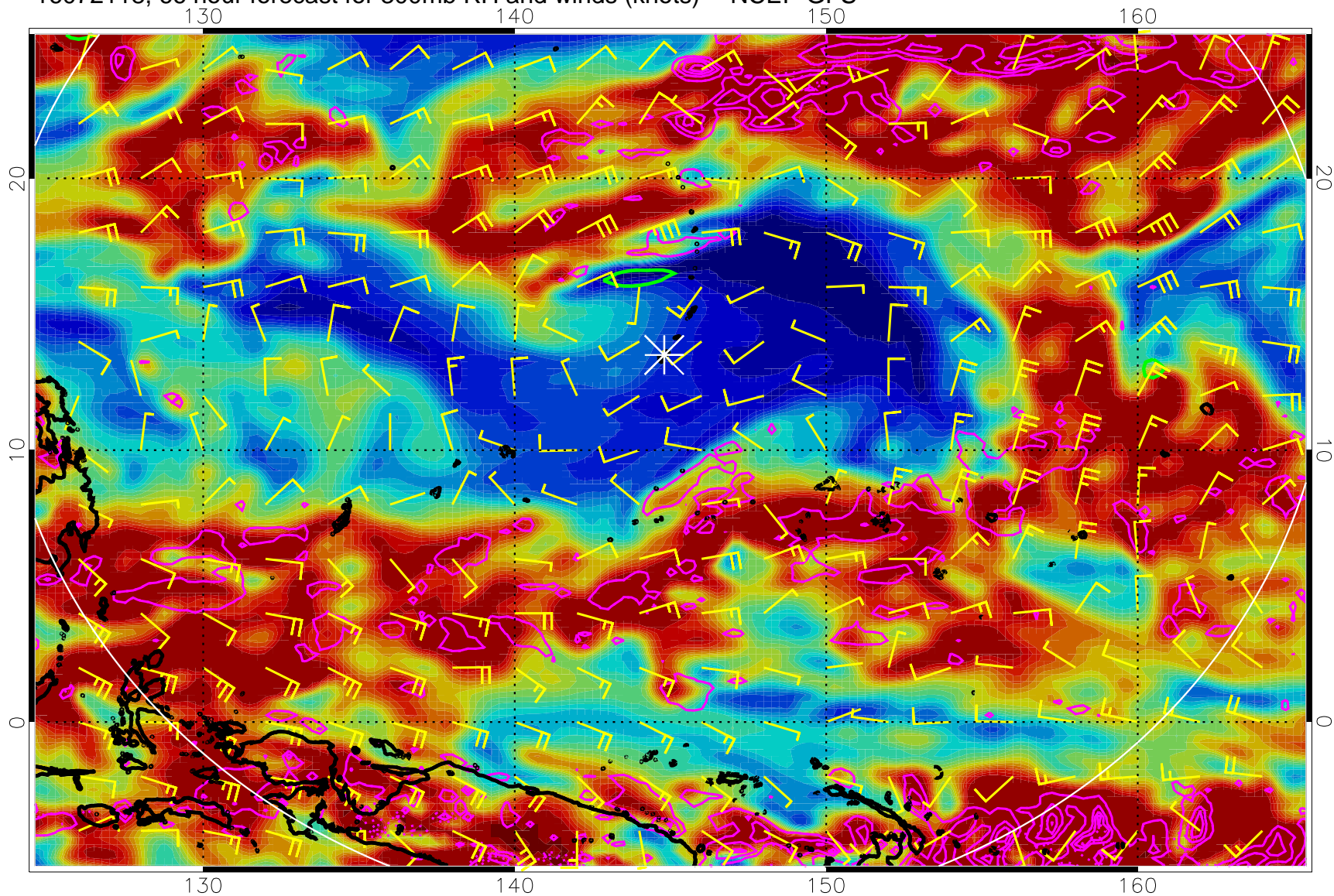
16072118, 66 hour forecast for 300mb RH and winds (knots) -- NCEP GFS
