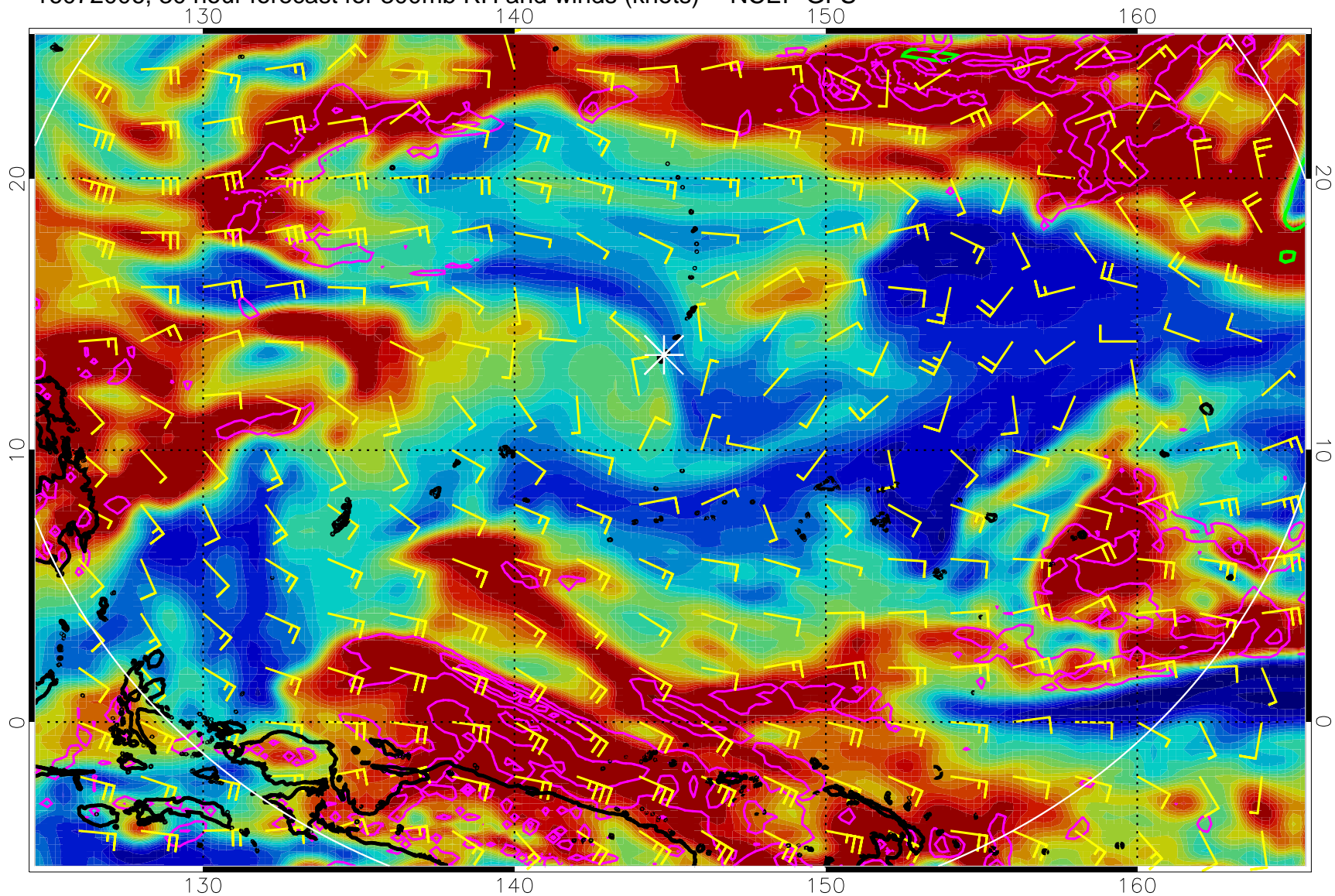
16072006, 30 hour forecast for 300mb RH and winds (knots) -- NCEP GFS
