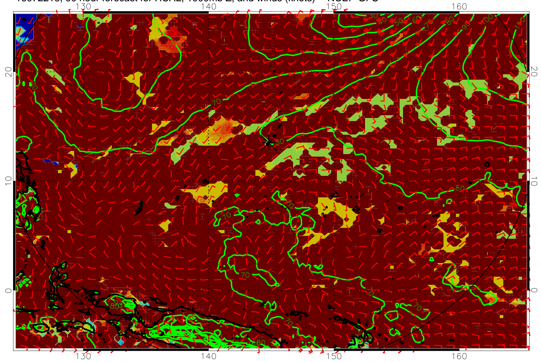
16072218, 90 hour forecast for HCAL, 1000mb Z, and winds (knots) -- NCEP GFS
