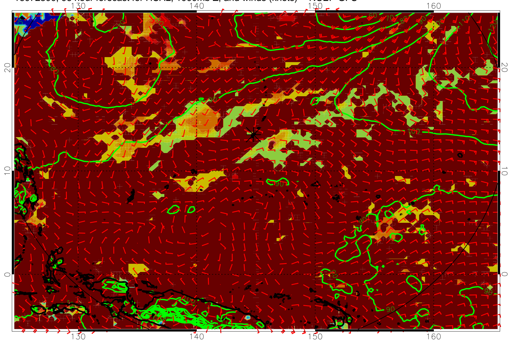
16072300, 96 hour forecast for HCAL, 1000mb Z, and winds (knots) -- NCEP GFS
