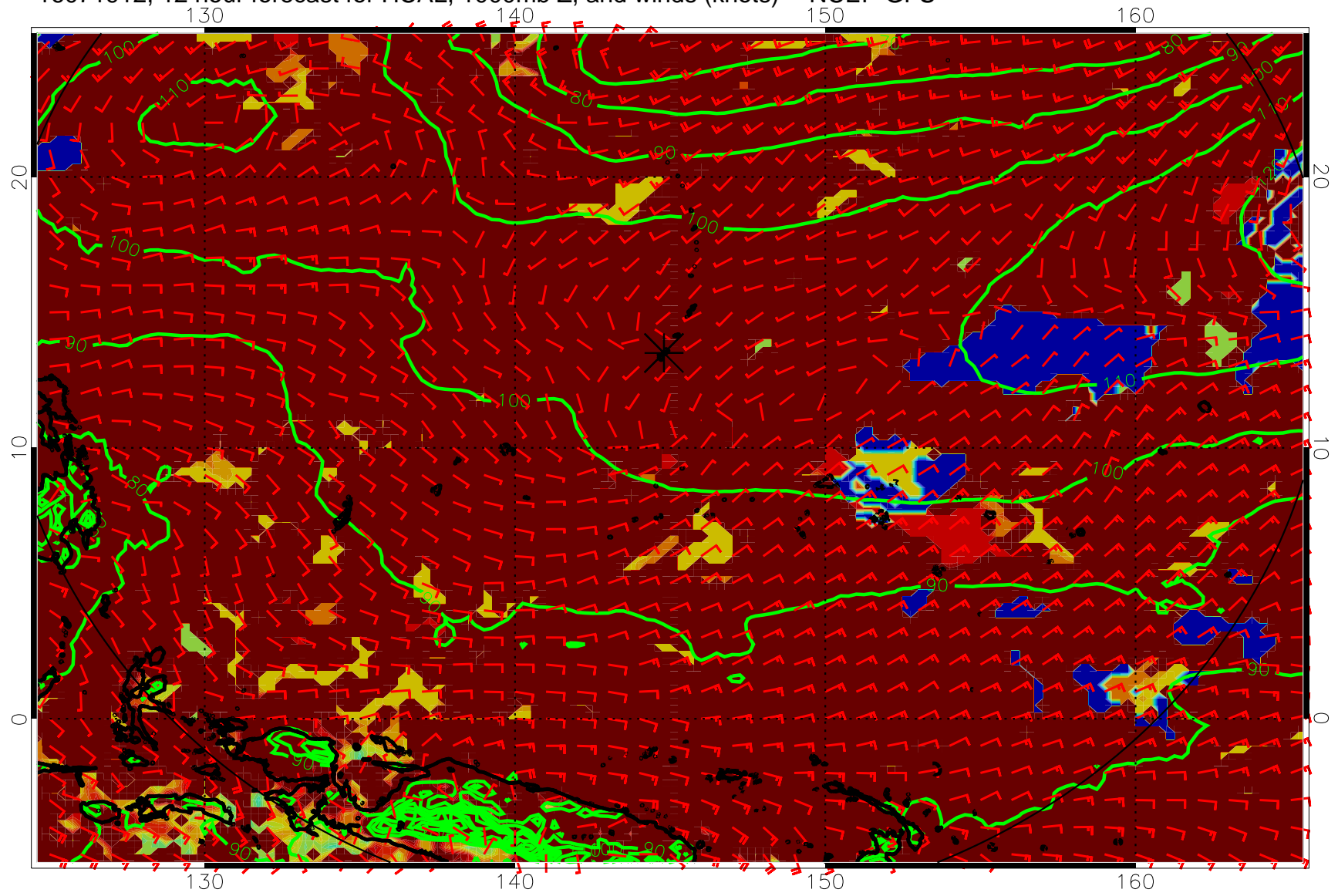
16071912, 12 hour forecast for HCAL, 1000mb Z, and winds (knots) -- NCEP GFS
