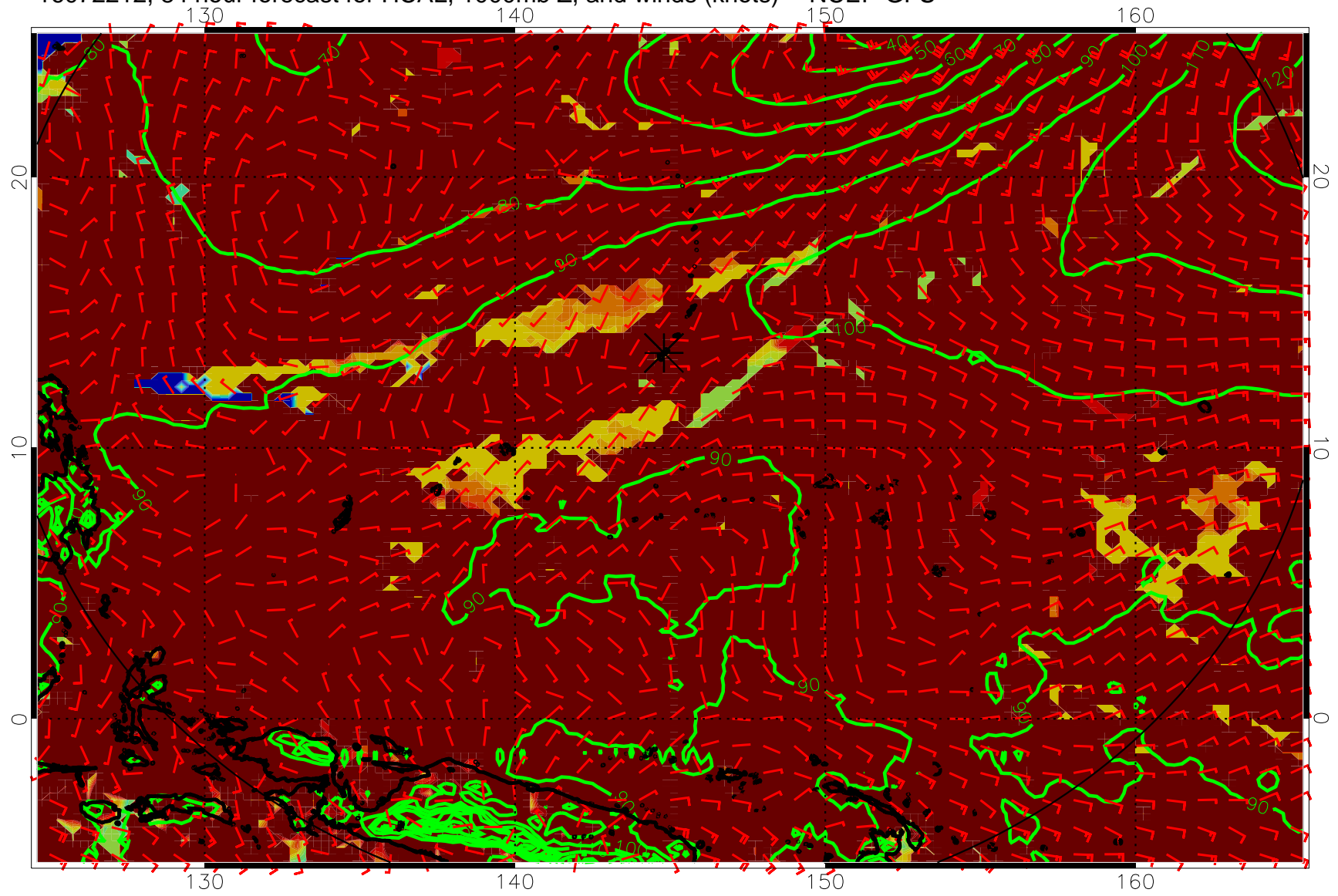
16072212, 84 hour forecast for HCAL, 1000mb Z, and winds (knots) -- NCEP GFS
