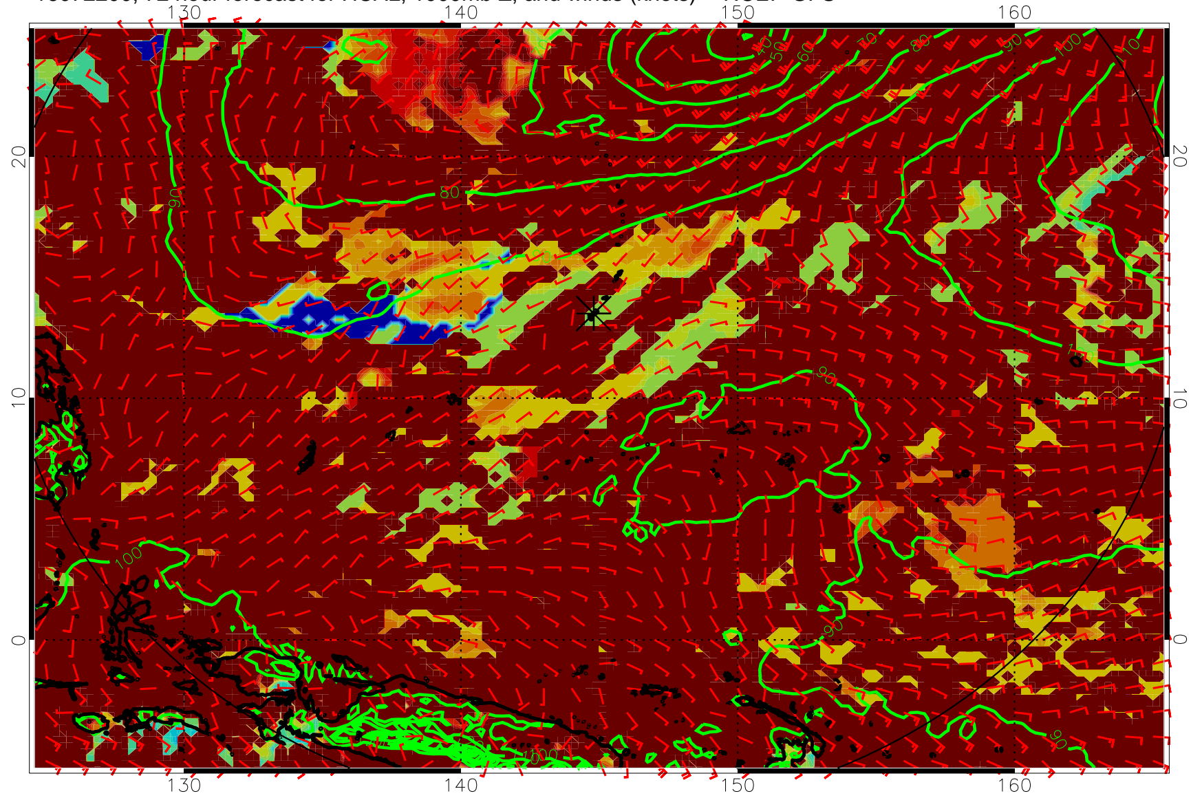
16072200, 72 hour forecast for HCAL, 1000mb Z, and winds (knots) -- NCEP GFS
