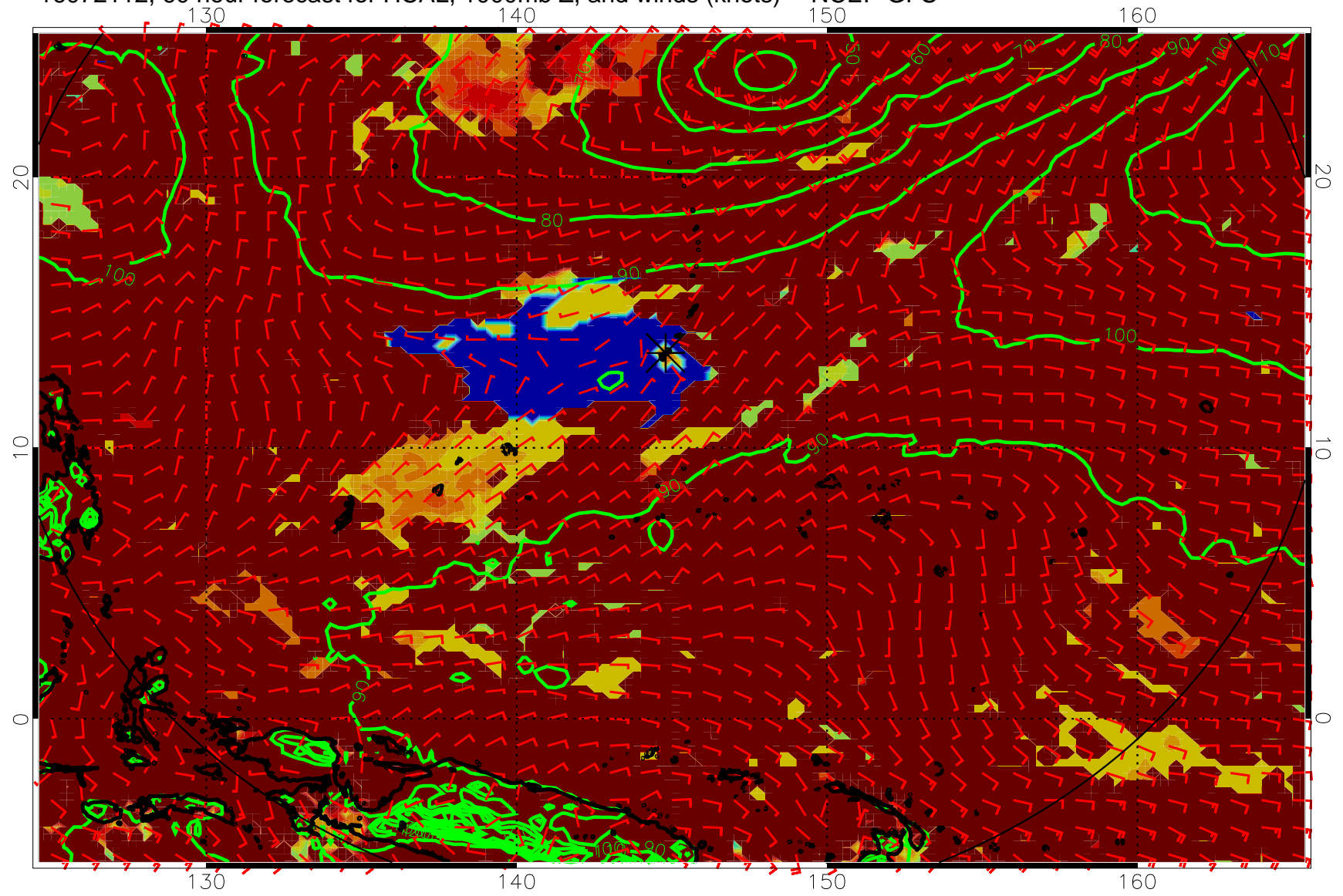
16072112, 60 hour forecast for HCAL, 1000mb Z, and winds (knots) -- NCEP GFS
