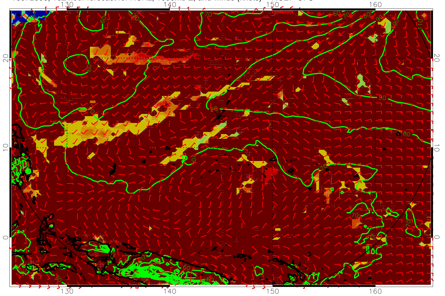
16072306, 102 hour forecast for HCAL, 1000mb Z, and winds (knots) -- NCEP GFS
