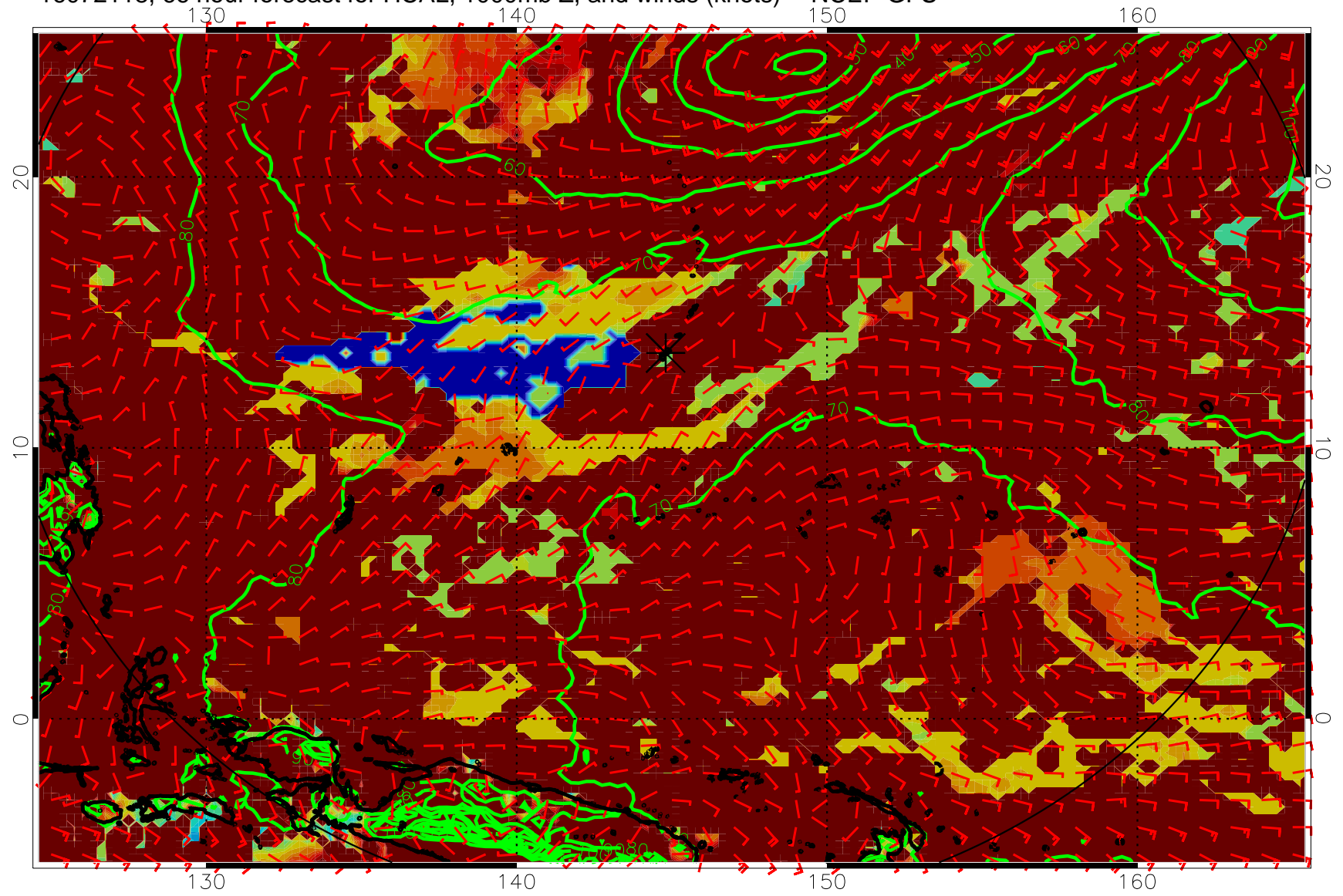
16072118, 66 hour forecast for HCAL, 1000mb Z, and winds (knots) -- NCEP GFS
