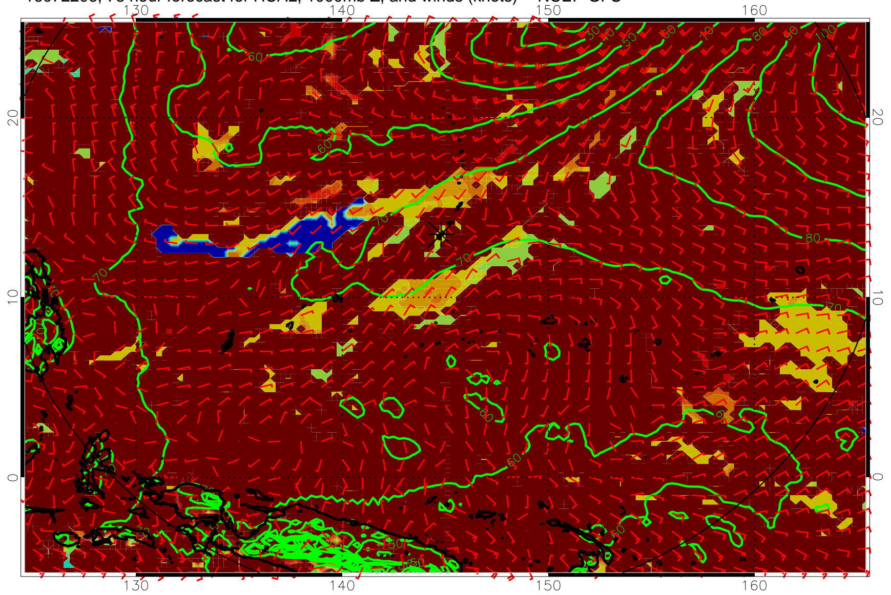
16072206, 78 hour forecast for HCAL, 1000mb Z, and winds (knots) -- NCEP GFS
