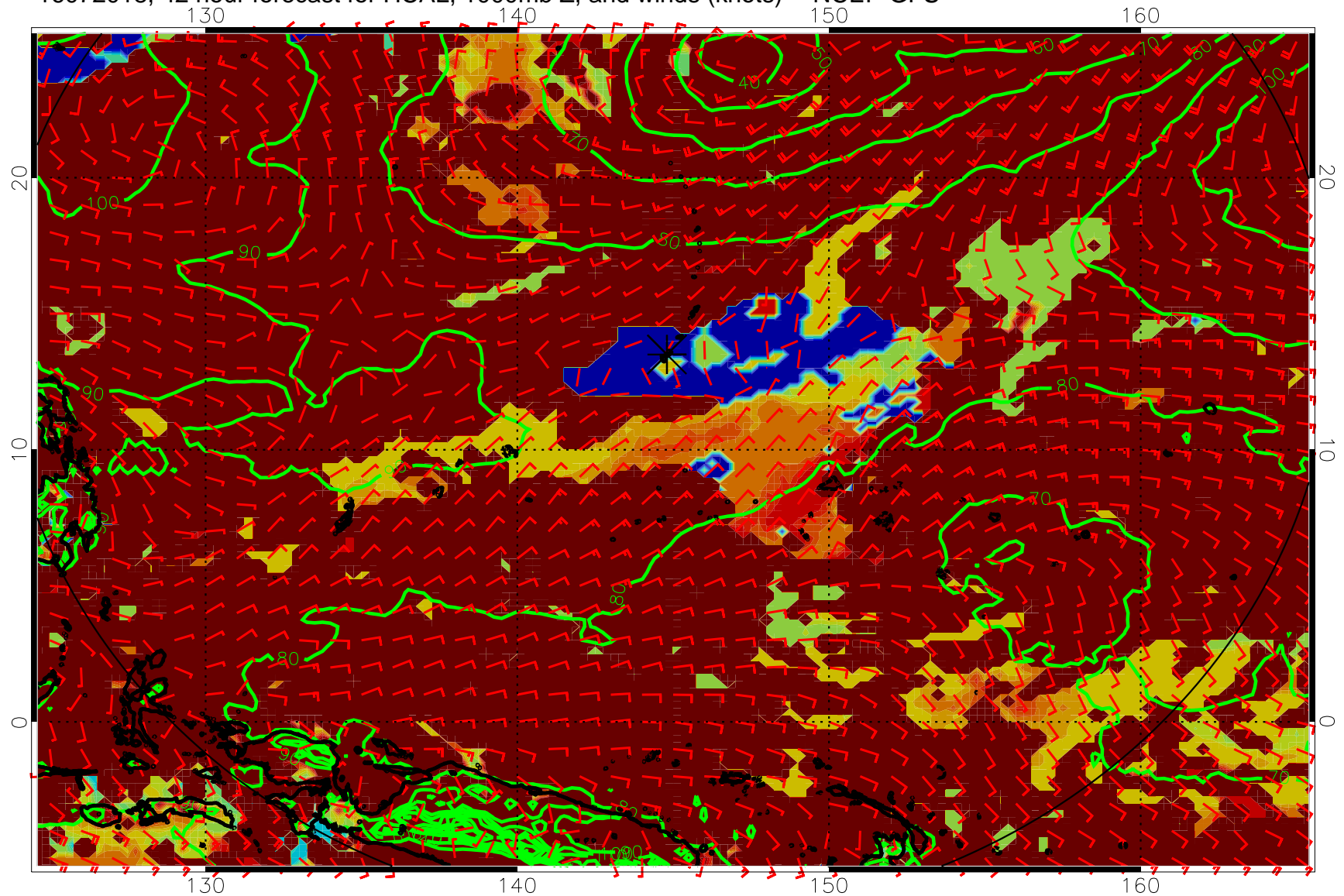
16072018, 42 hour forecast for HCAL, 1000mb Z, and winds (knots) -- NCEP GFS
