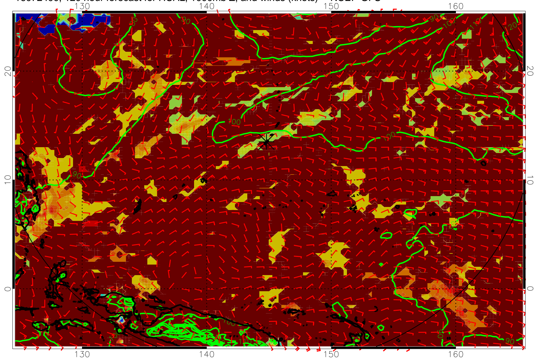
16072400, 120 hour forecast for HCAL, 1000mb Z, and winds (knots) -- NCEP GFS
