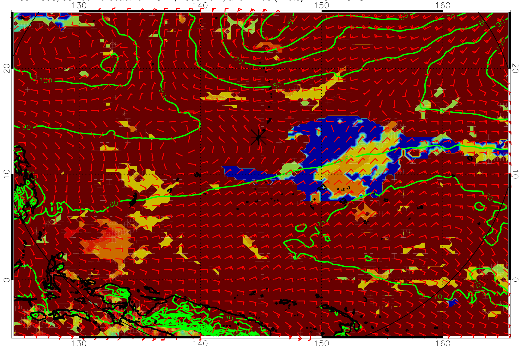
16072006, 30 hour forecast for HCAL, 1000mb Z, and winds (knots) -- NCEP GFS
