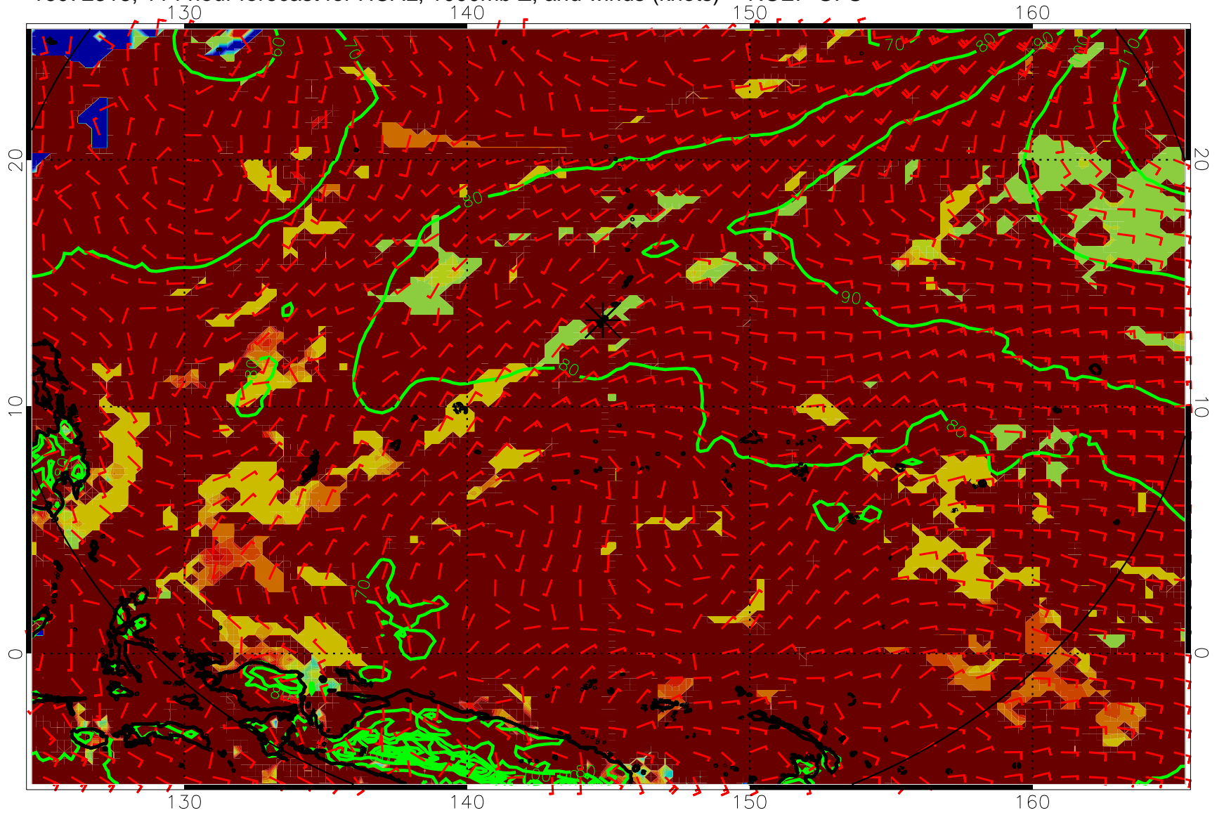
16072318, 114 hour forecast for HCAL, 1000mb Z, and winds (knots) -- NCEP GFS
