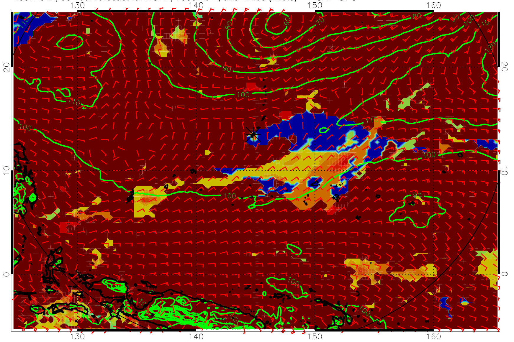
16072012, 36 hour forecast for HCAL, 1000mb Z, and winds (knots) -- NCEP GFS
