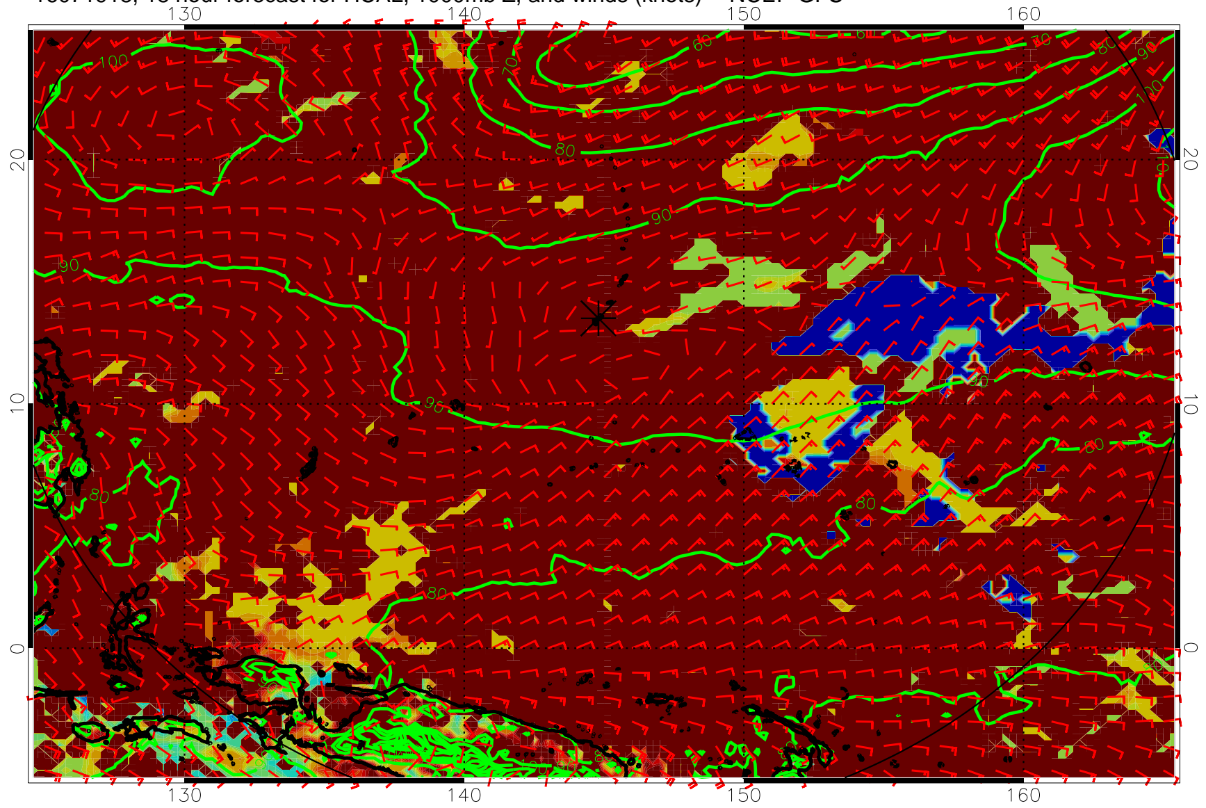
16071918, 18 hour forecast for HCAL, 1000mb Z, and winds (knots) -- NCEP GFS
