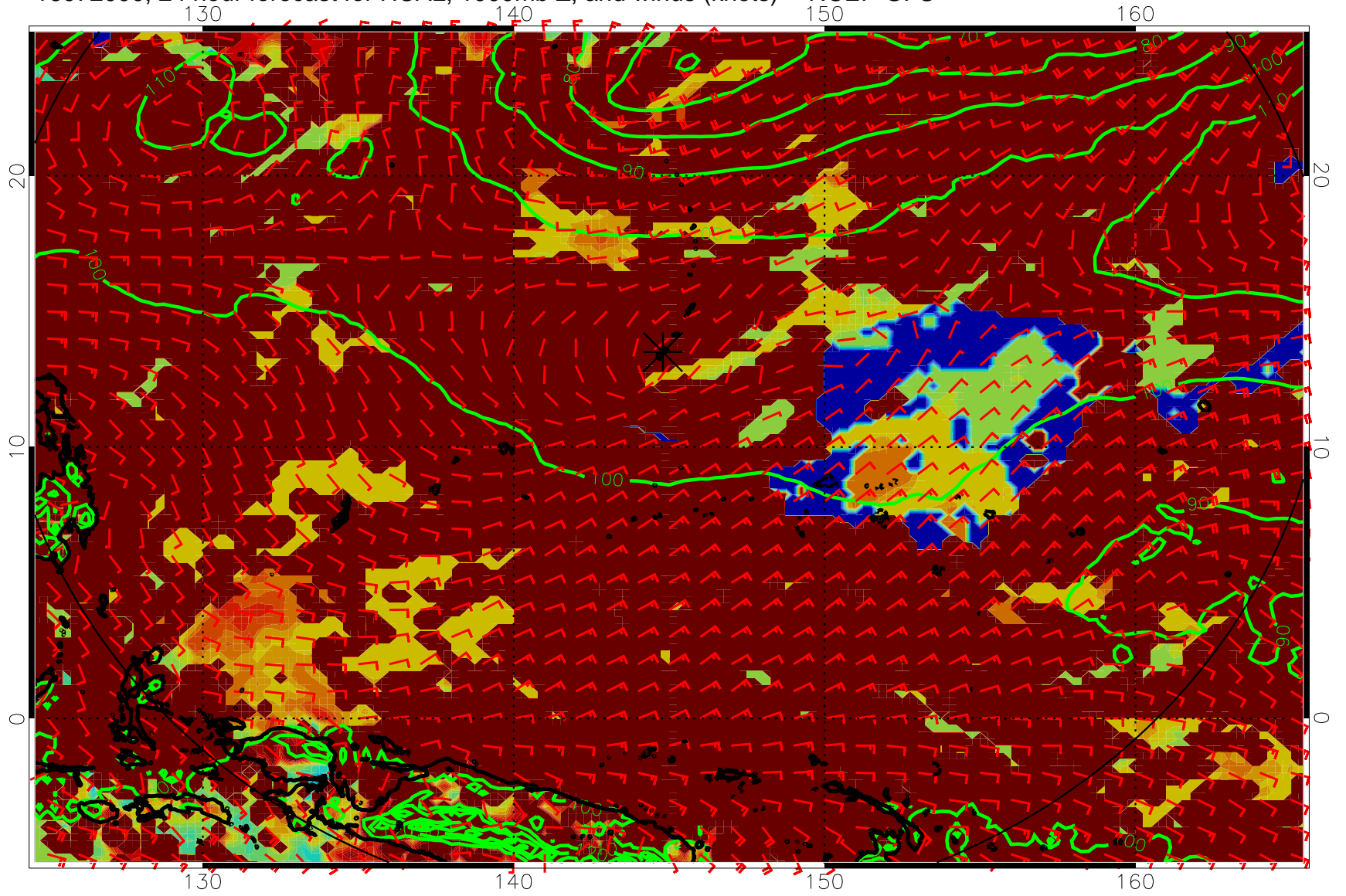
16072000, 24 hour forecast for HCAL, 1000mb Z, and winds (knots) -- NCEP GFS
