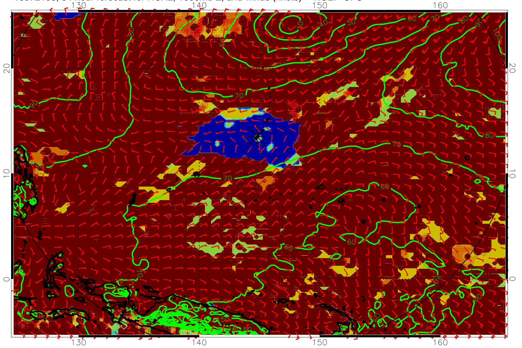
16072106, 54 hour forecast for HCAL, 1000mb Z, and winds (knots) -- NCEP GFS
