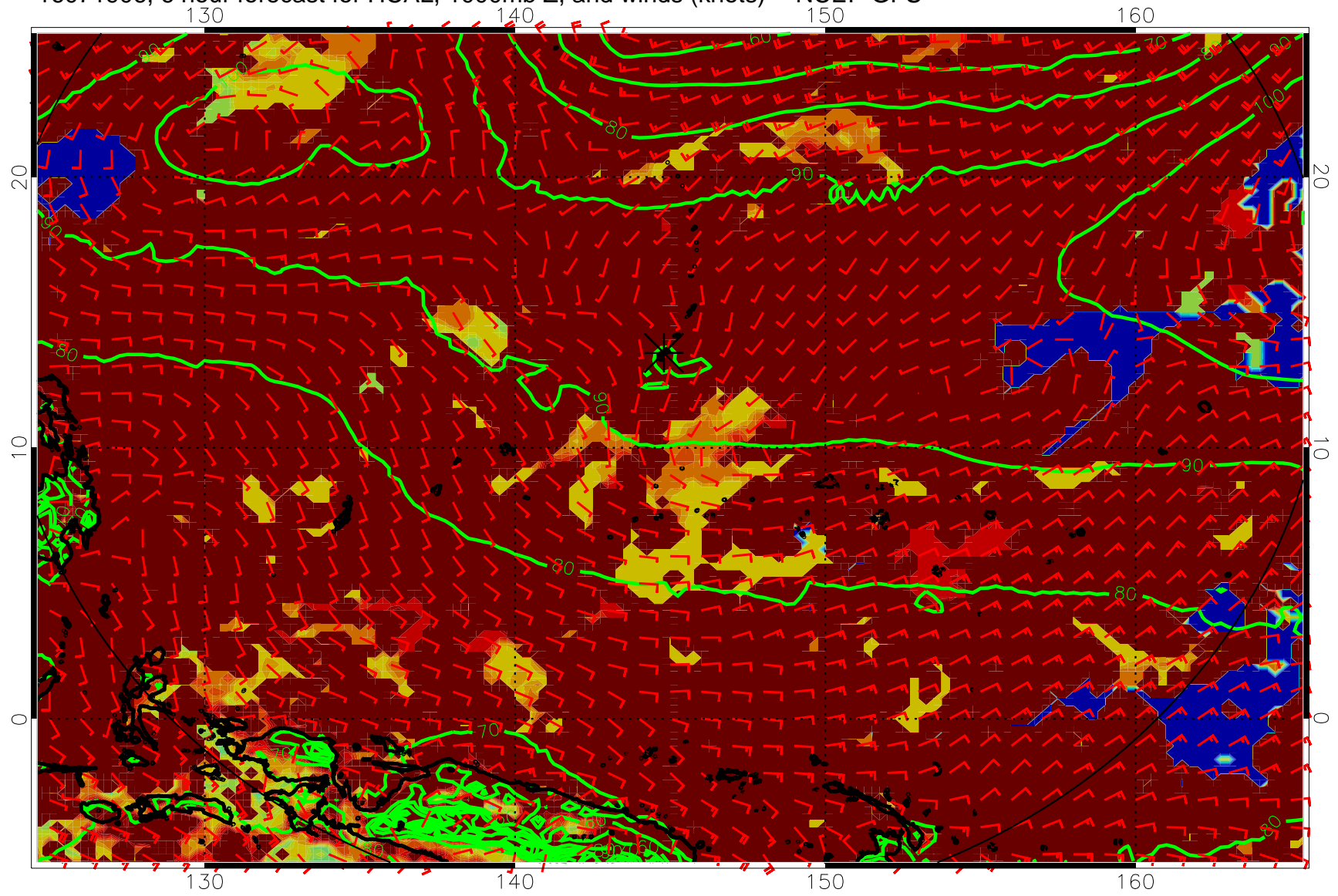
16071906, 6 hour forecast for HCAL, 1000mb Z, and winds (knots) -- NCEP GFS
