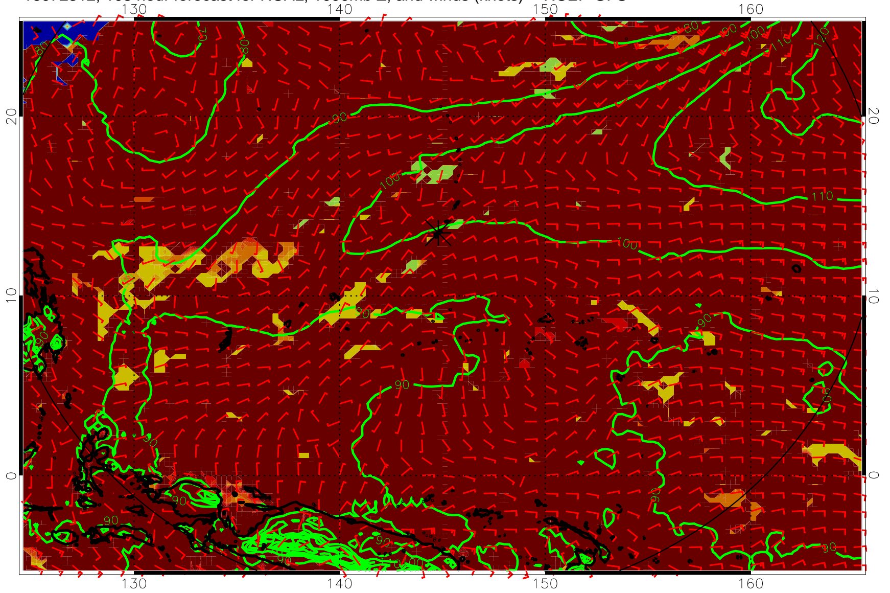
16072312, 108 hour forecast for HCAL, 1000mb Z, and winds (knots) -- NCEP GFS
