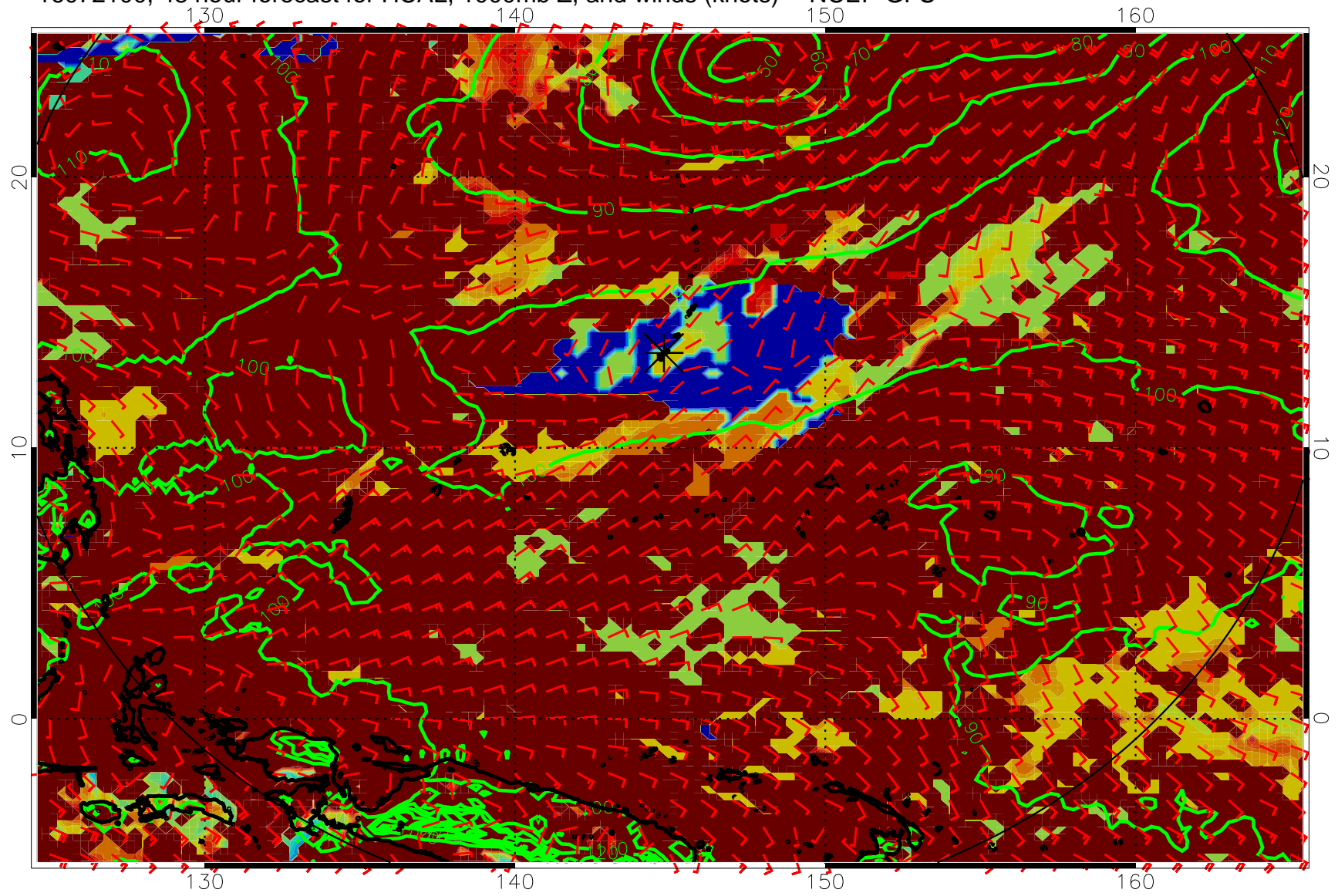
16072100, 48 hour forecast for HCAL, 1000mb Z, and winds (knots) -- NCEP GFS
