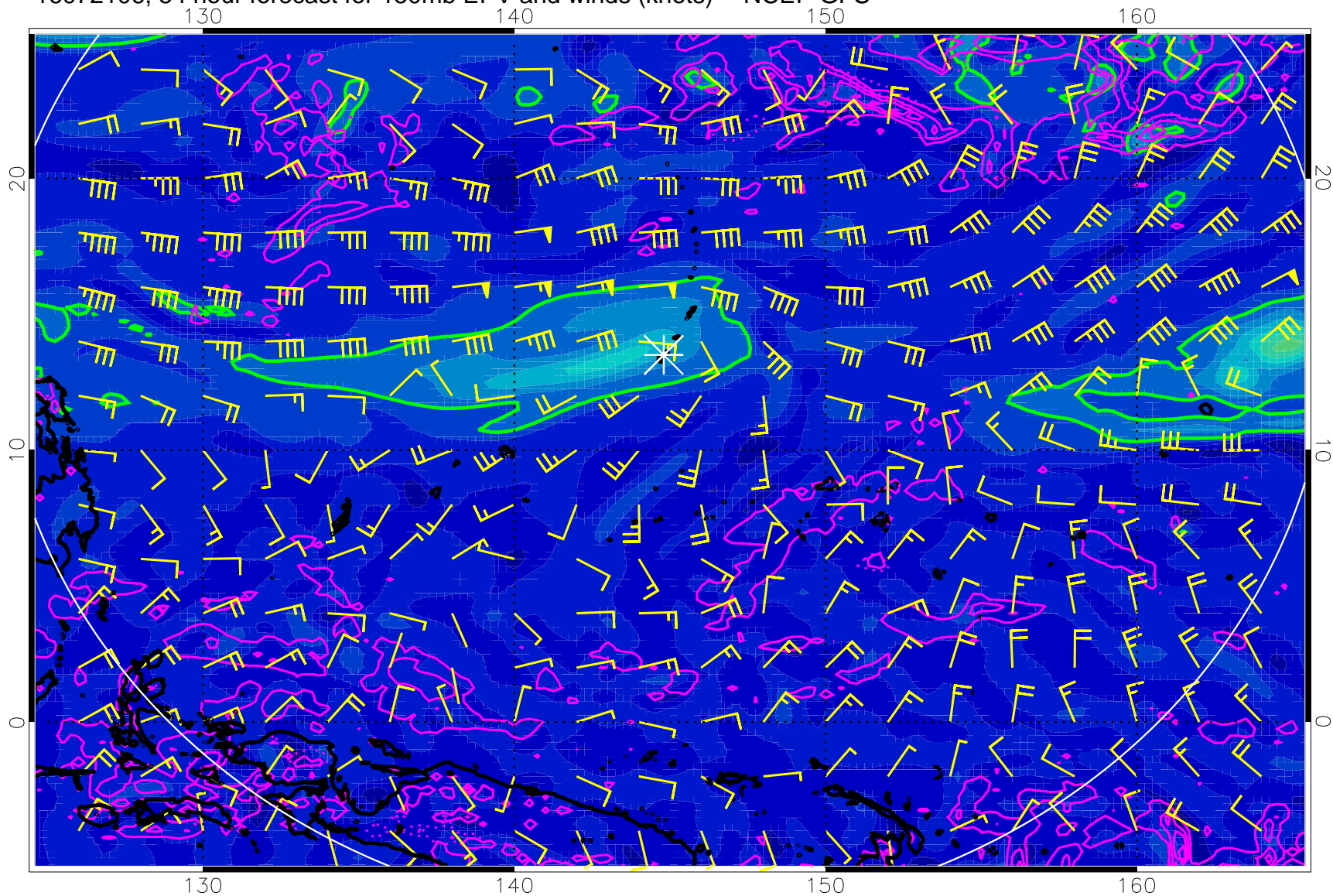
16072106, 54 hour forecast for 150mb EPV and winds (knots) -- NCEP GFS
