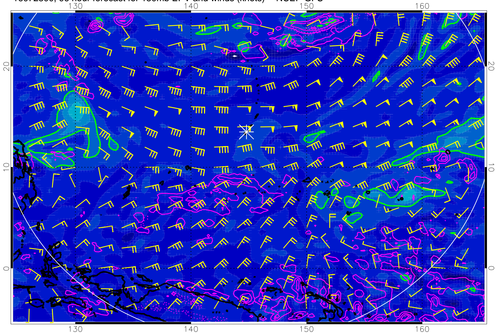
16072300, 96 hour forecast for 150mb EPV and winds (knots) -- NCEP GFS
