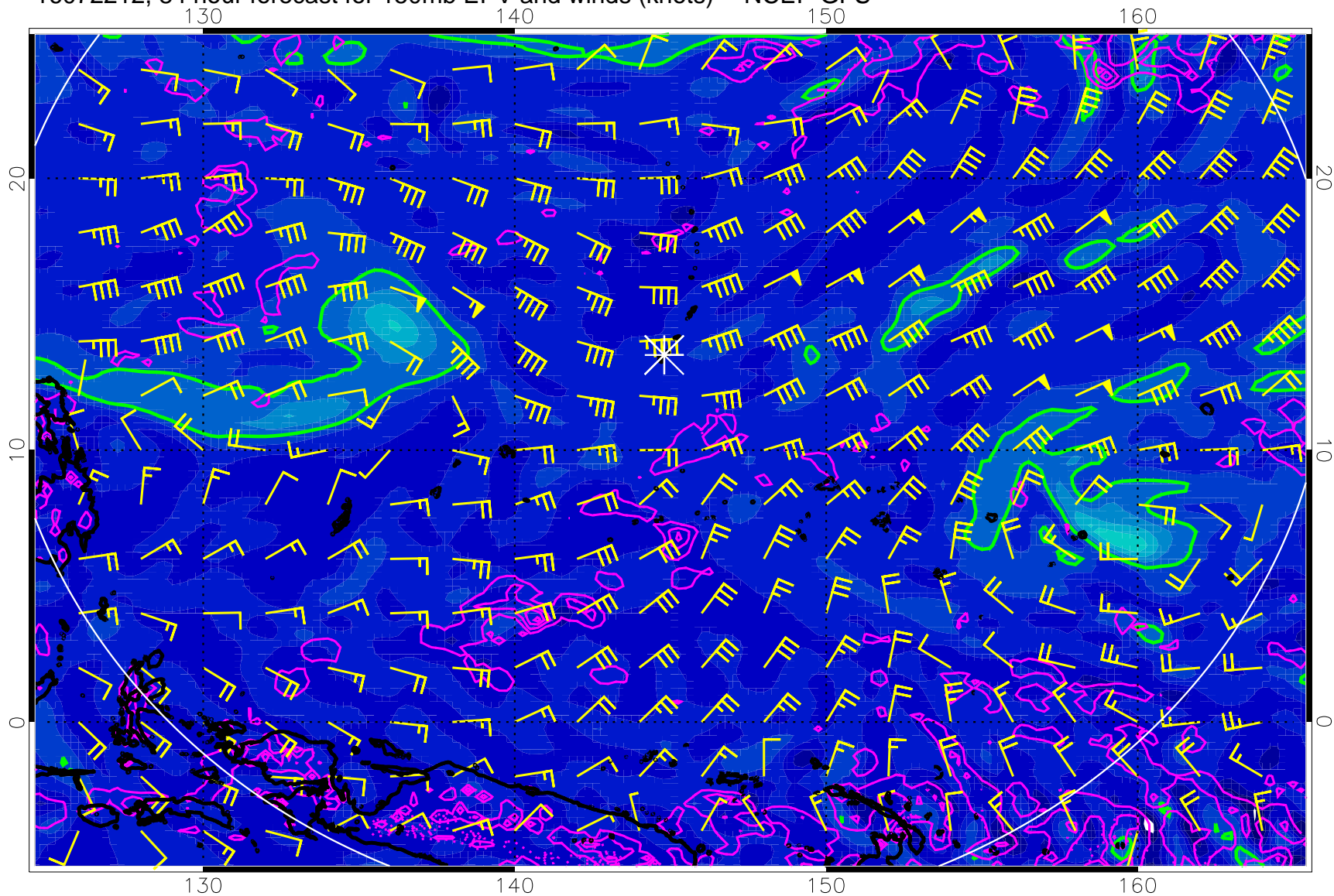
16072212, 84 hour forecast for 150mb EPV and winds (knots) -- NCEP GFS
