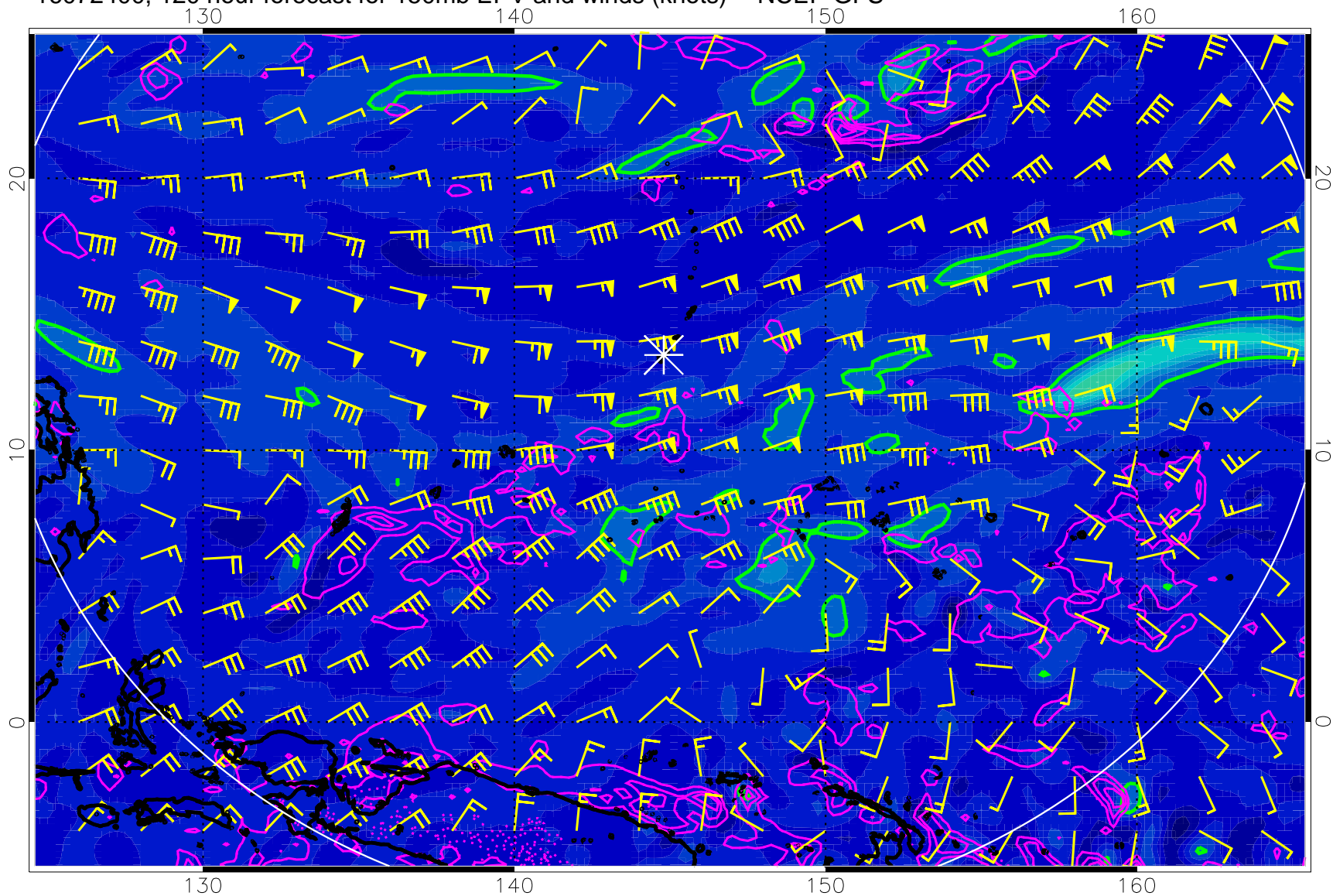
16072400, 120 hour forecast for 150mb EPV and winds (knots) -- NCEP GFS
