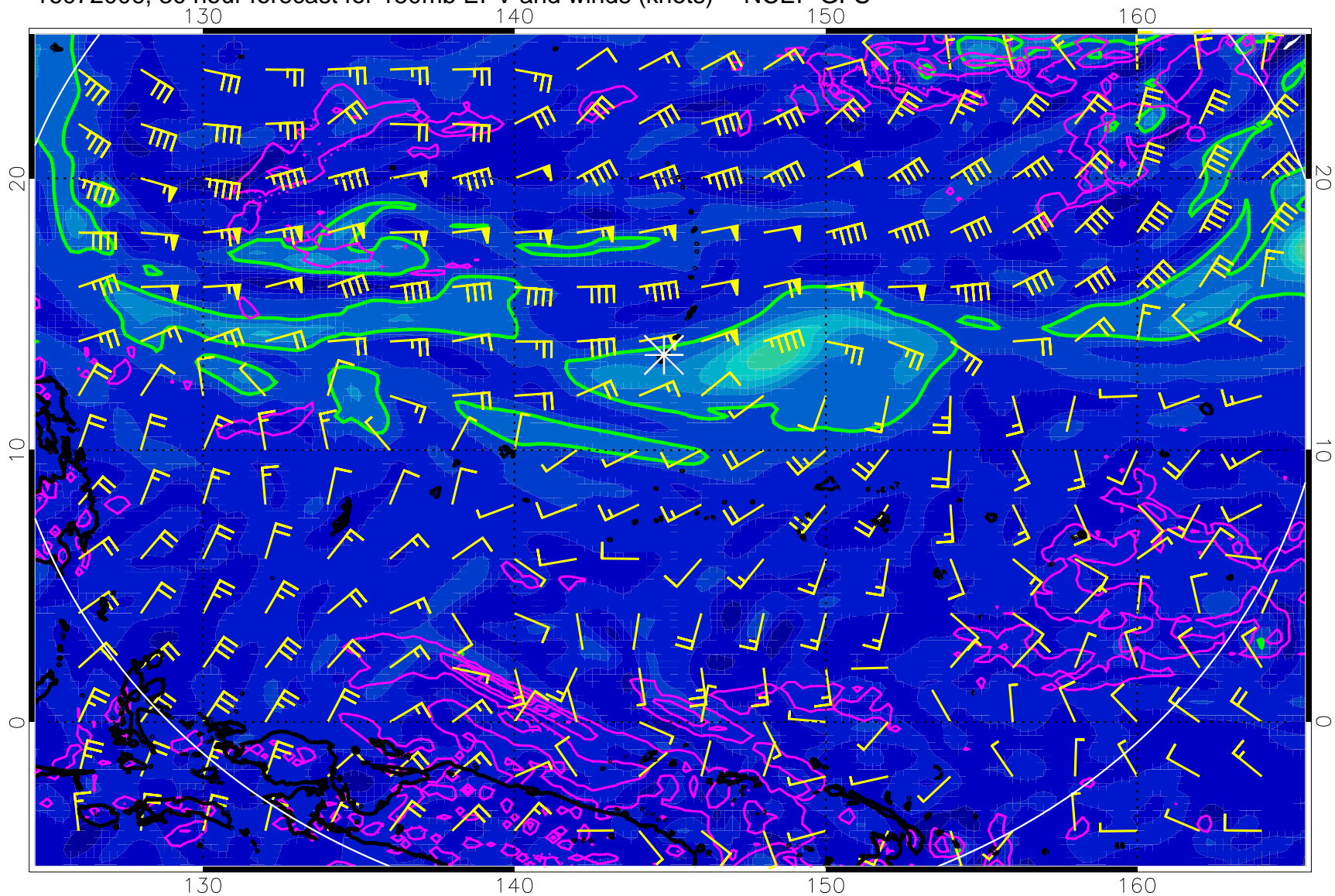
16072006, 30 hour forecast for 150mb EPV and winds (knots) -- NCEP GFS
