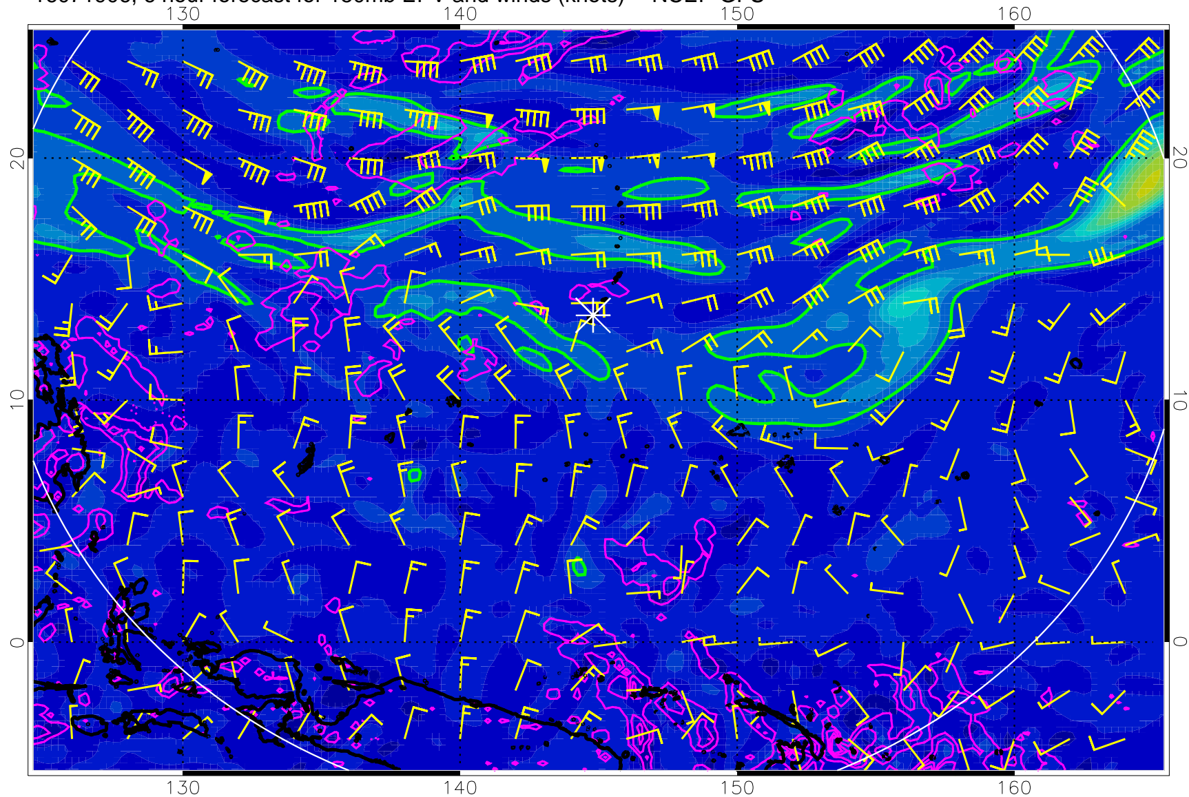
16071906, 6 hour forecast for 150mb EPV and winds (knots) -- NCEP GFS
