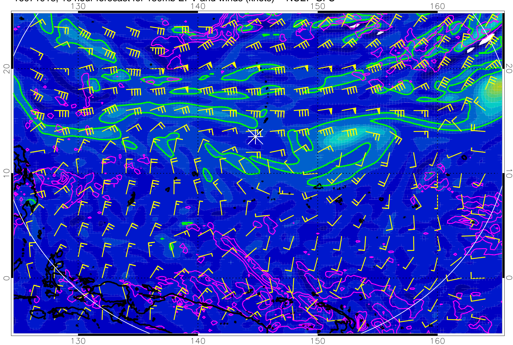
16071918, 18 hour forecast for 150mb EPV and winds (knots) -- NCEP GFS
