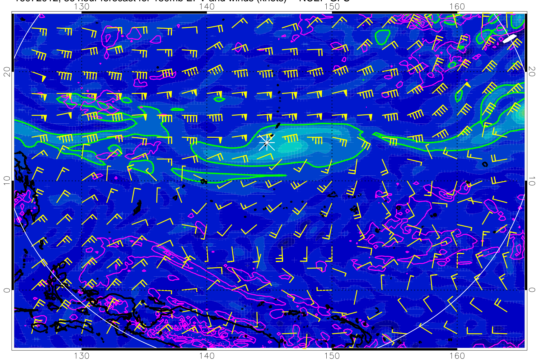
16072012, 36 hour forecast for 150mb EPV and winds (knots) -- NCEP GFS
