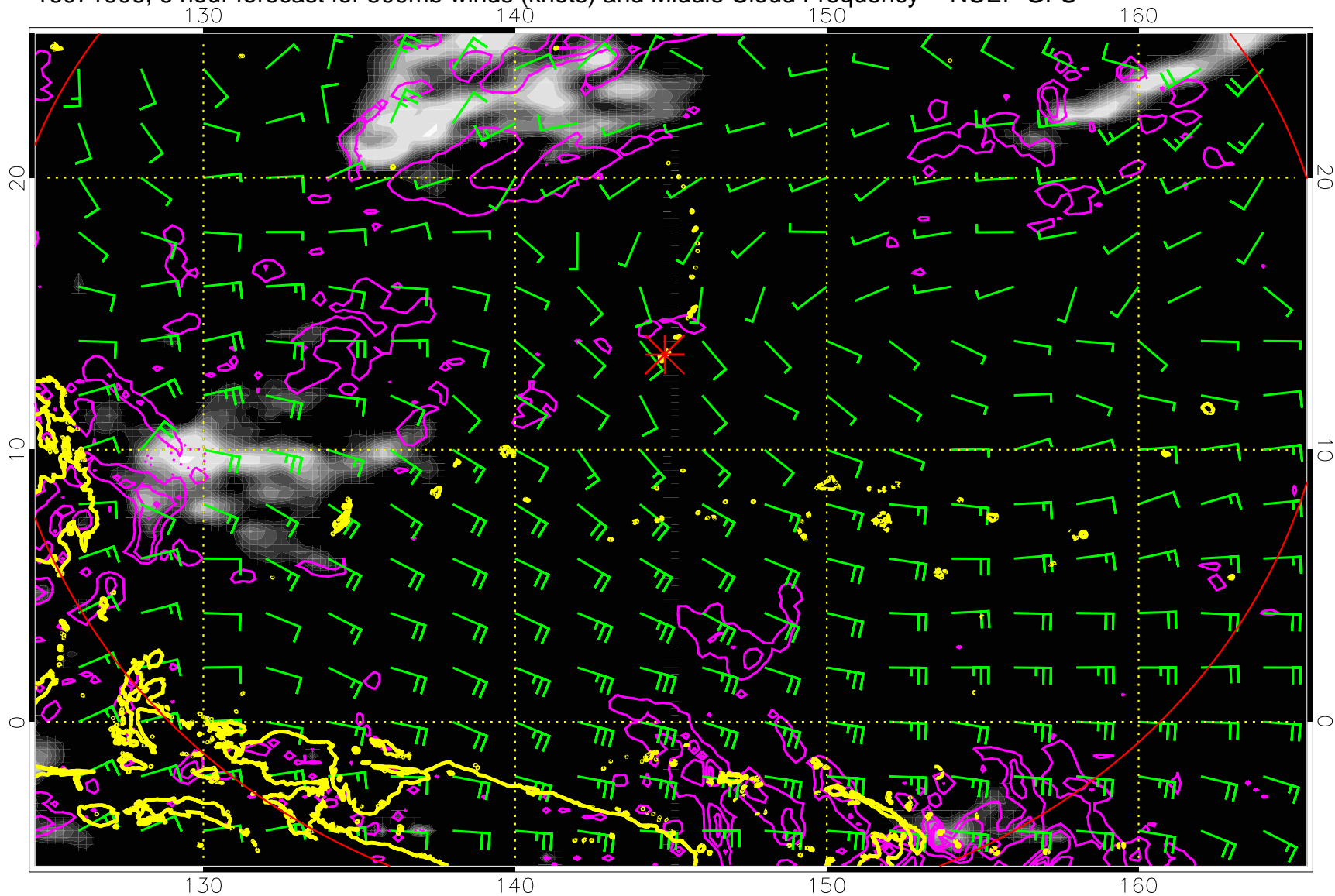
16071906, 6 hour forecast for 500mb winds (knots) and Middle Cloud Frequency -- NCEP GFS
