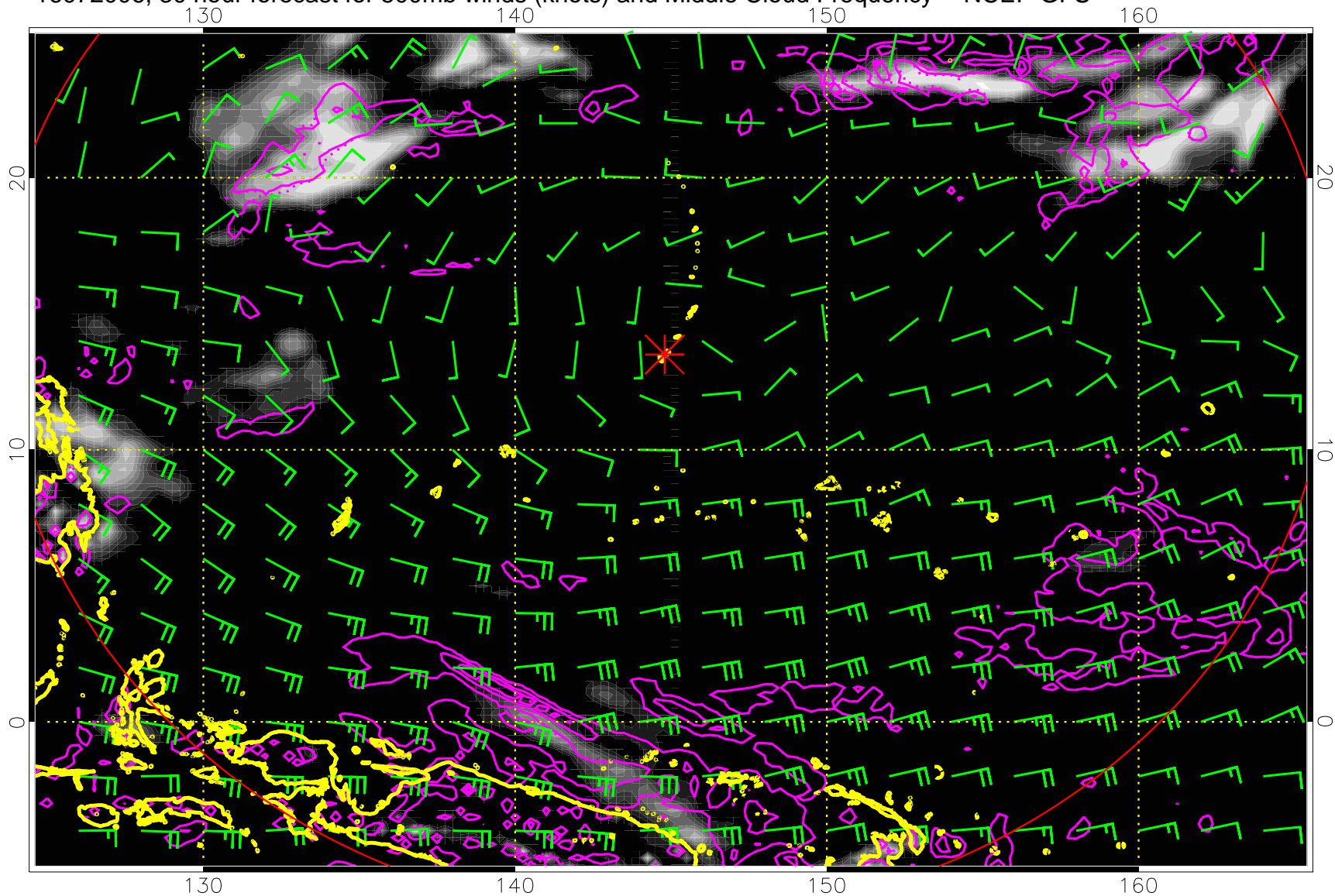
16072006, 30 hour forecast for 500mb winds (knots) and Middle Cloud Frequency -- NCEP GFS
