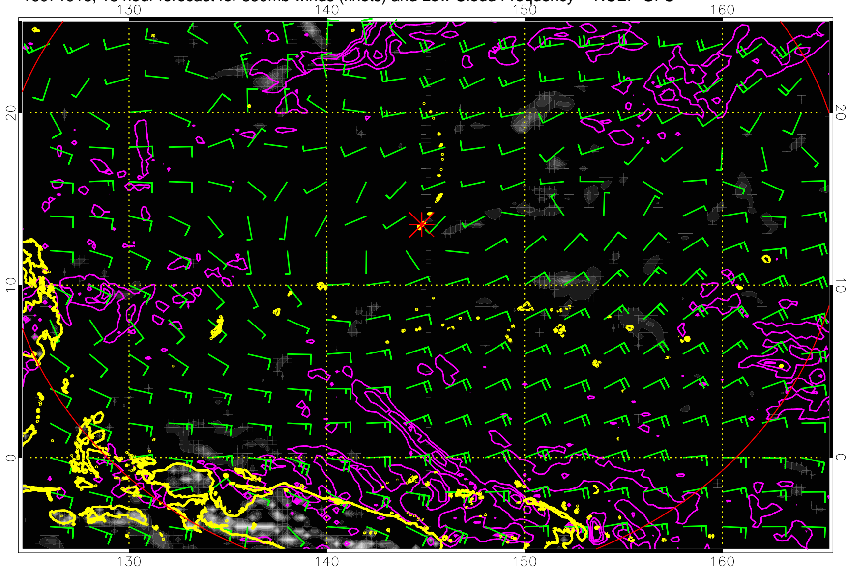
16071918, 18 hour forecast for 850mb winds (knots) and Low Cloud Frequency -- NCEP GFS
