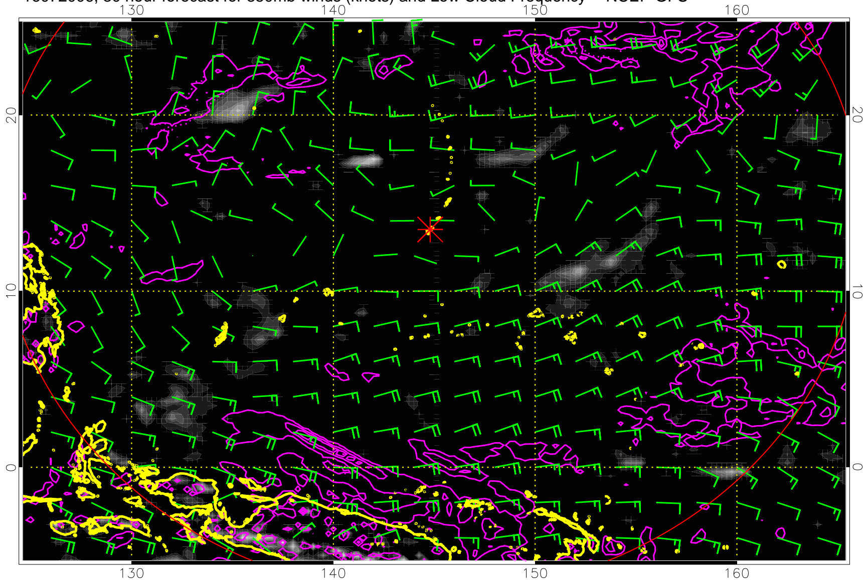
16072006, 30 hour forecast for 850mb winds (knots) and Low Cloud Frequency -- NCEP GFS
