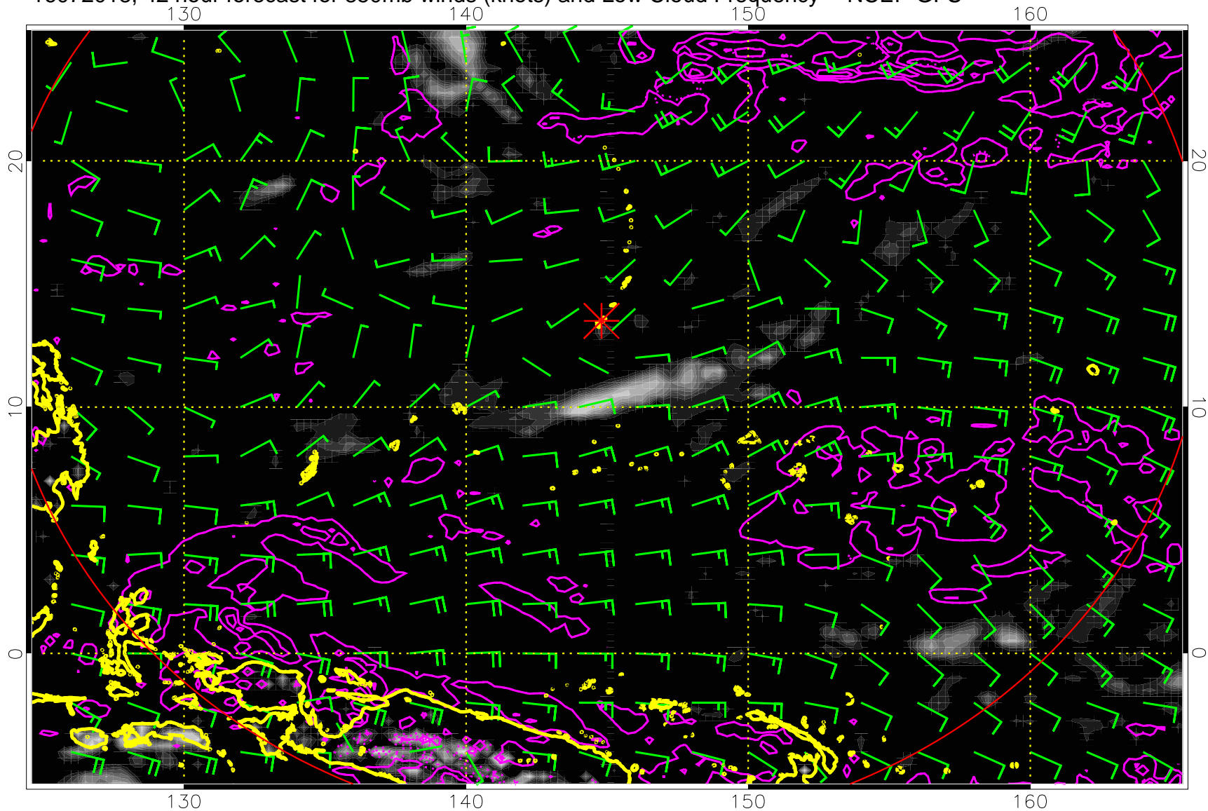
16072018, 42 hour forecast for 850mb winds (knots) and Low Cloud Frequency -- NCEP GFS
