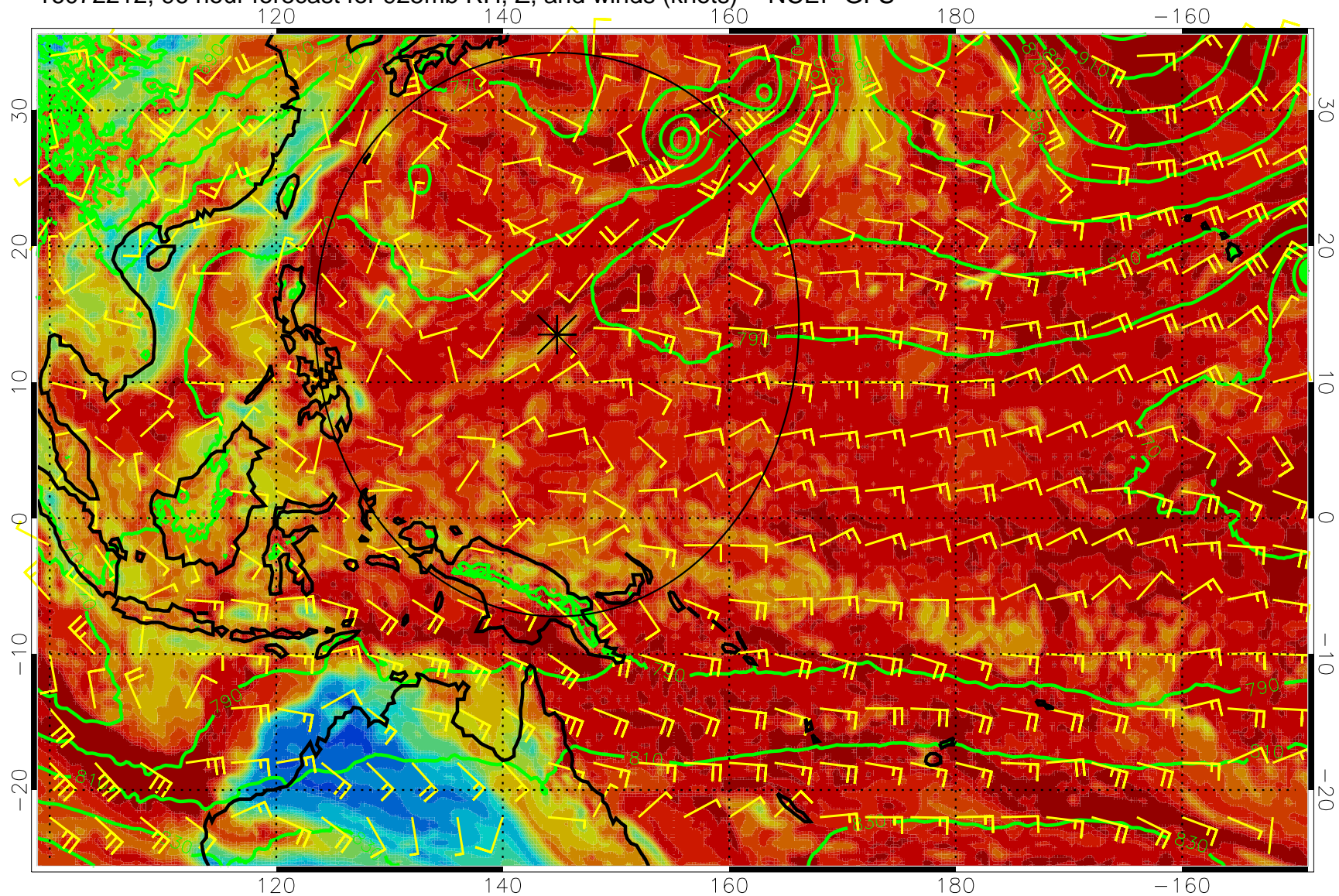
16072212, 96 hour forecast for 925mb RH, Z, and winds (knots) -- NCEP GFS
