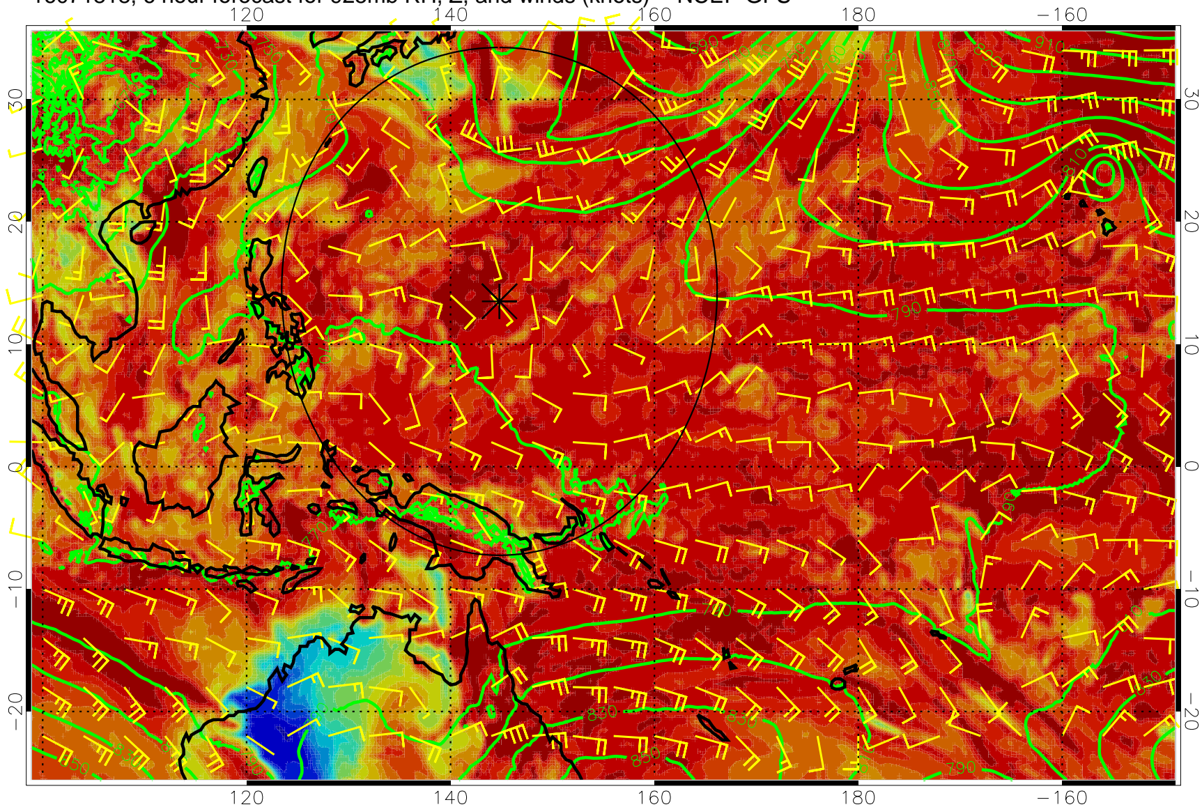
16071818, 6 hour forecast for 925mb RH, Z, and winds (knots) -- NCEP GFS
