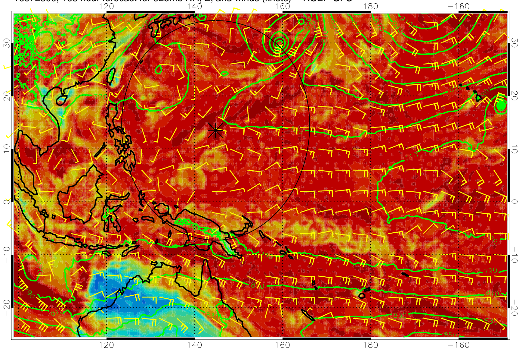
16072300, 108 hour forecast for 925mb RH, Z, and winds (knots) -- NCEP GFS
