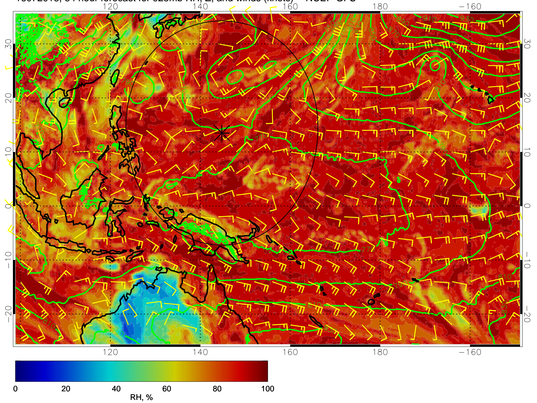
16072018, 54 hour forecast for 925mb RH, Z, and winds (knots) -- NCEP GFS
