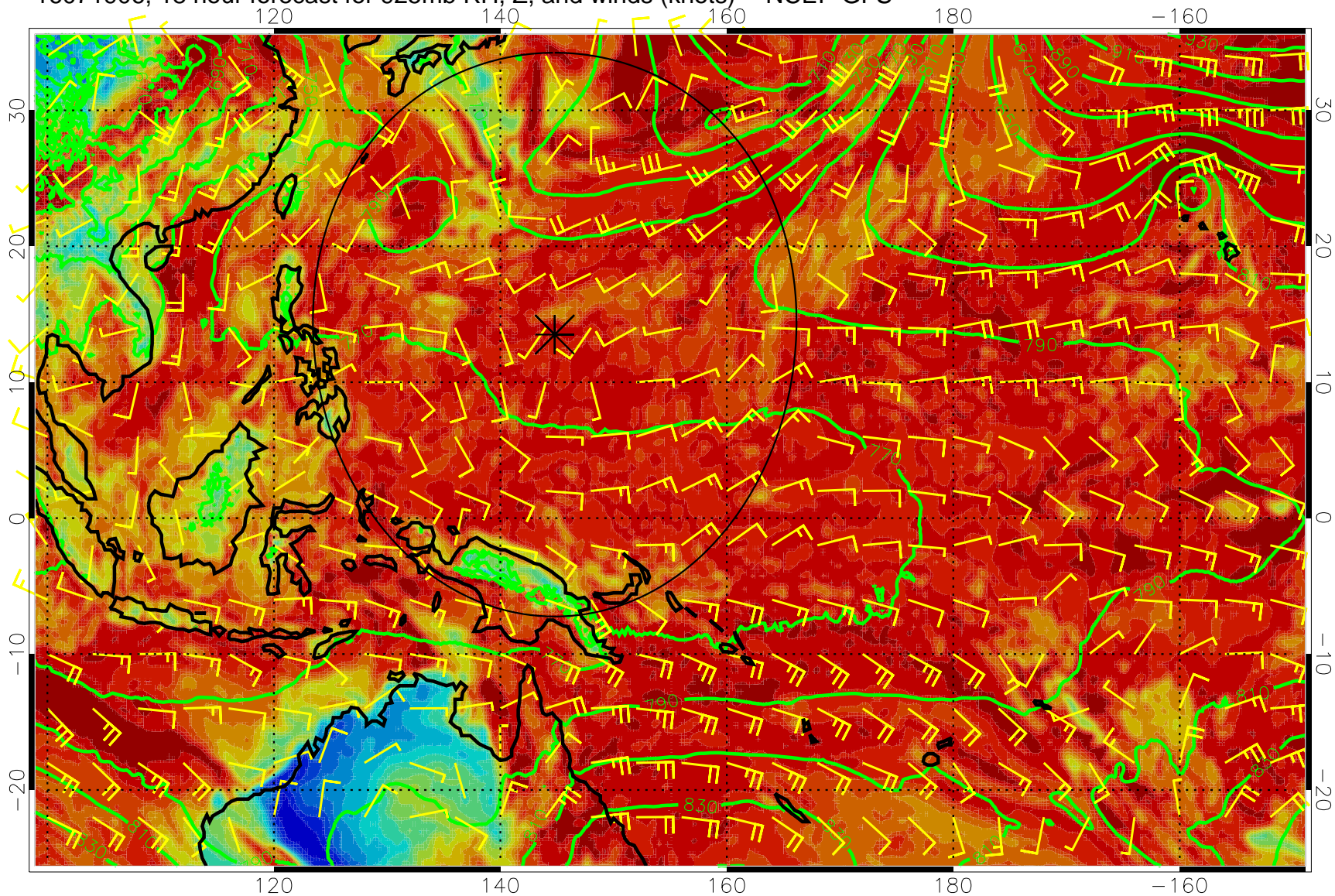
16071906, 18 hour forecast for 925mb RH, Z, and winds (knots) -- NCEP GFS
