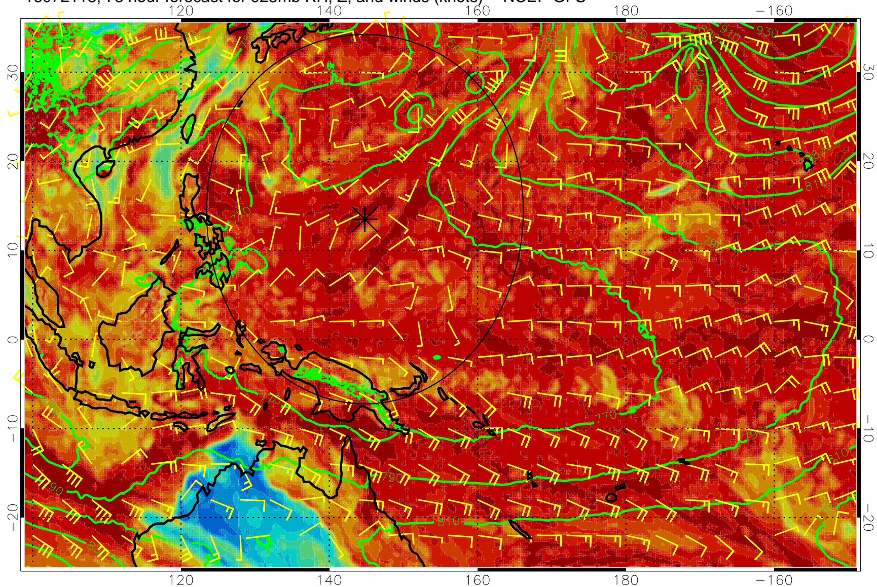
16072118, 78 hour forecast for 925mb RH, Z, and winds (knots) -- NCEP GFS
