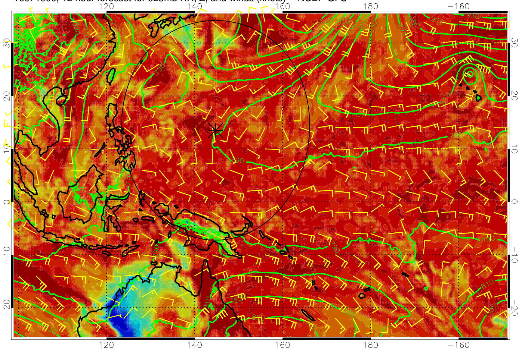
16071900, 12 hour forecast for 925mb RH, Z, and winds (knots) -- NCEP GFS
