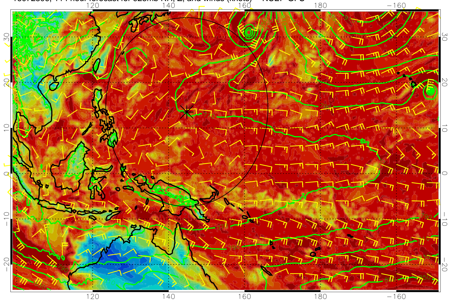
16072306, 114 hour forecast for 925mb RH, Z, and winds (knots) -- NCEP GFS
