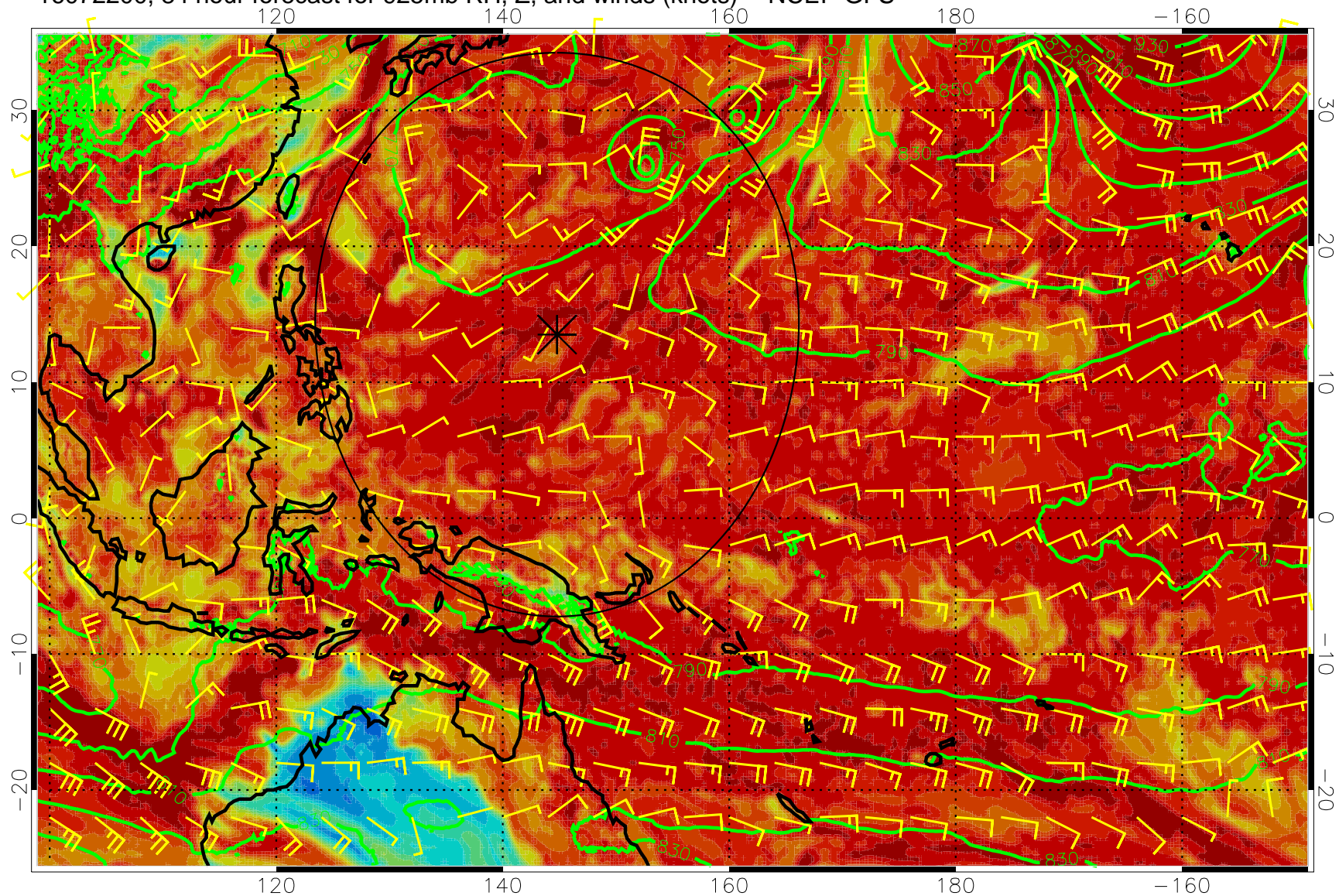
16072200, 84 hour forecast for 925mb RH, Z, and winds (knots) -- NCEP GFS
