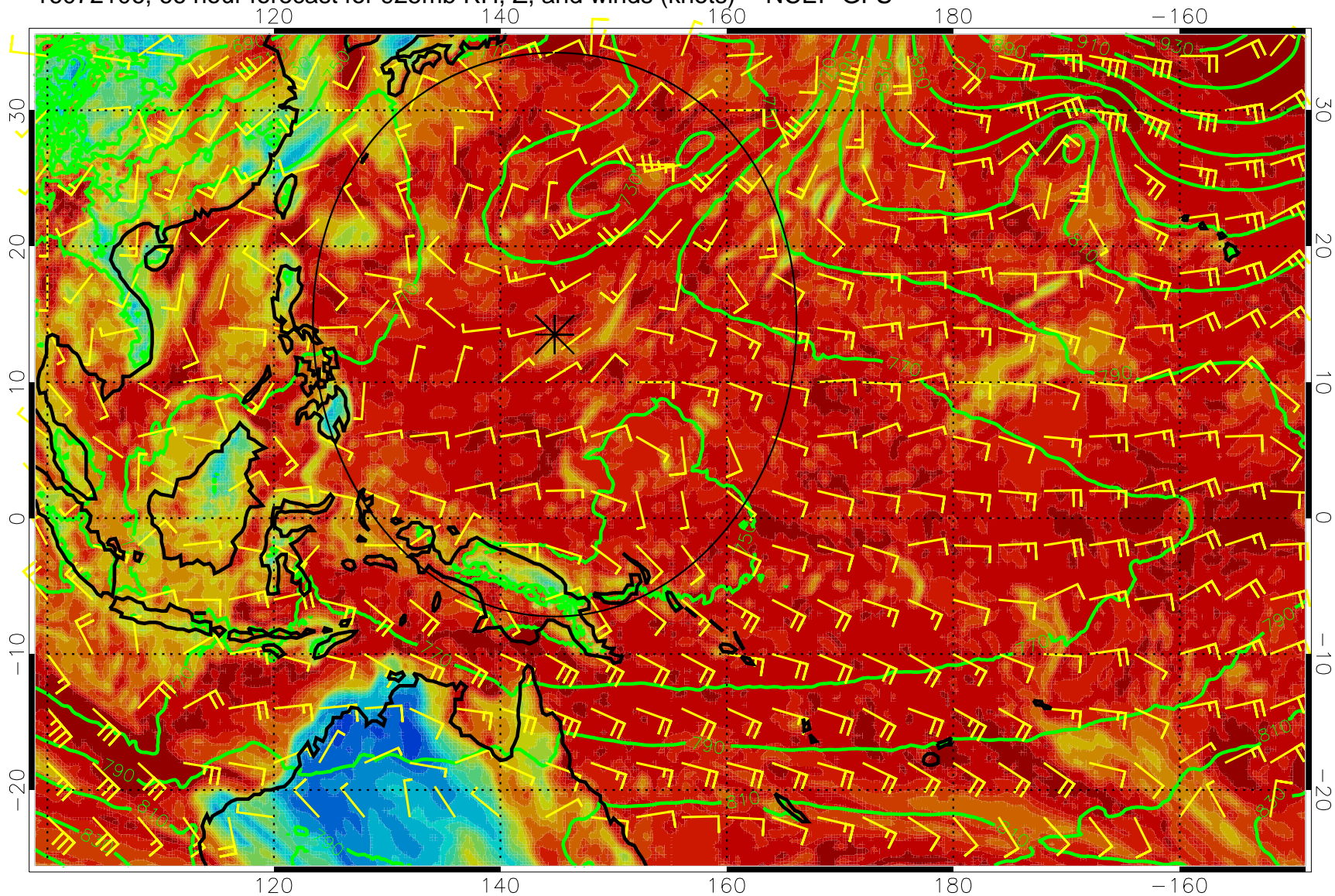
16072106, 66 hour forecast for 925mb RH, Z, and winds (knots) -- NCEP GFS
