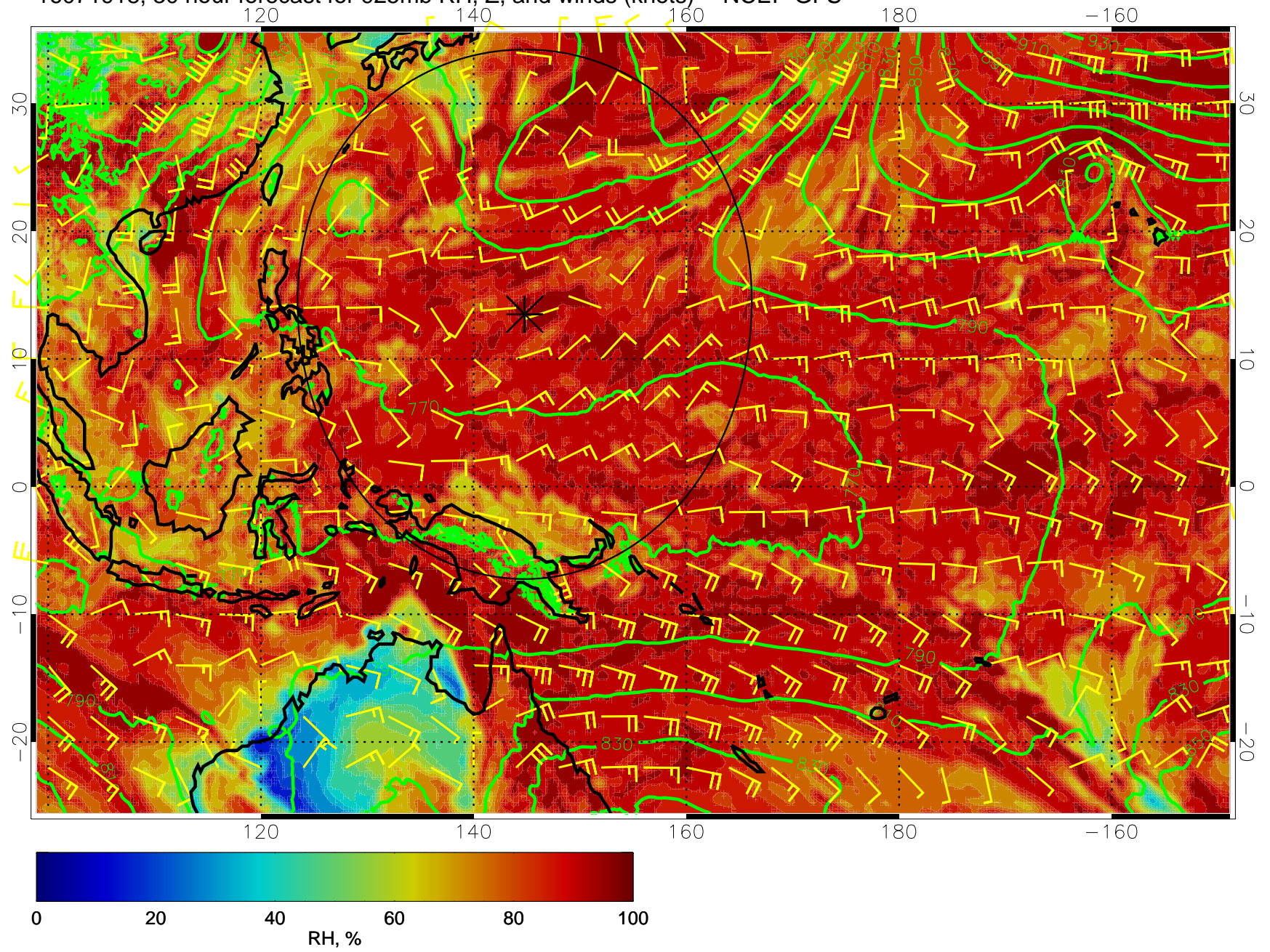
16071918, 30 hour forecast for 925mb RH, Z, and winds (knots) -- NCEP GFS
