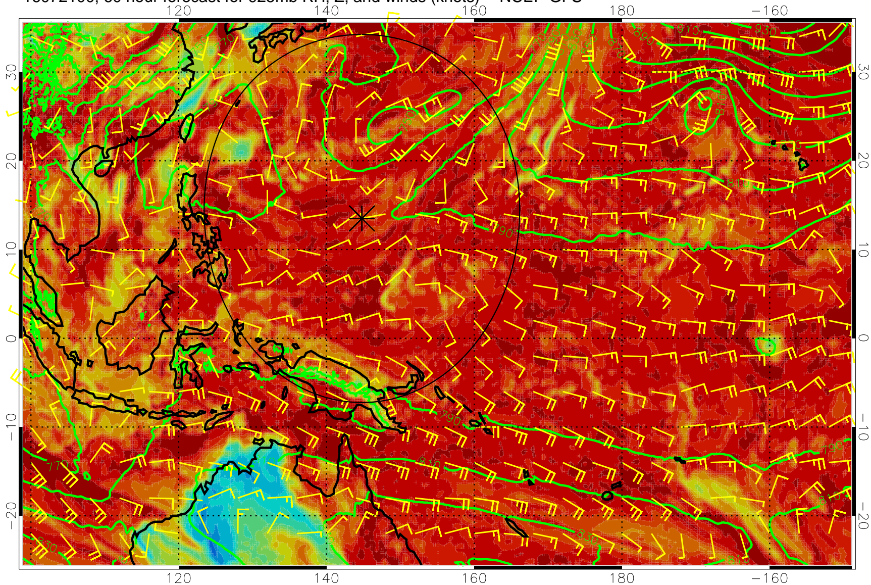
16072100, 60 hour forecast for 925mb RH, Z, and winds (knots) -- NCEP GFS
