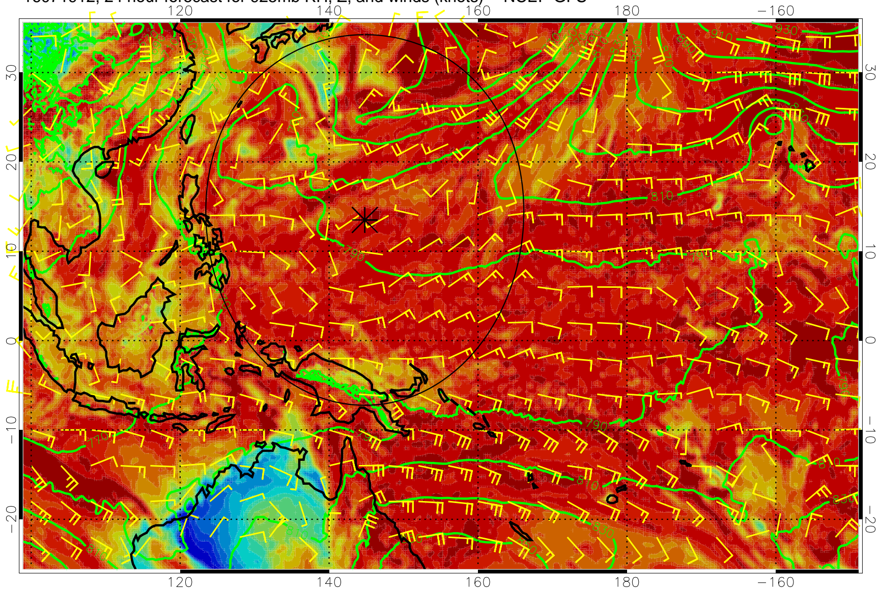
16071912, 24 hour forecast for 925mb RH, Z, and winds (knots) -- NCEP GFS
