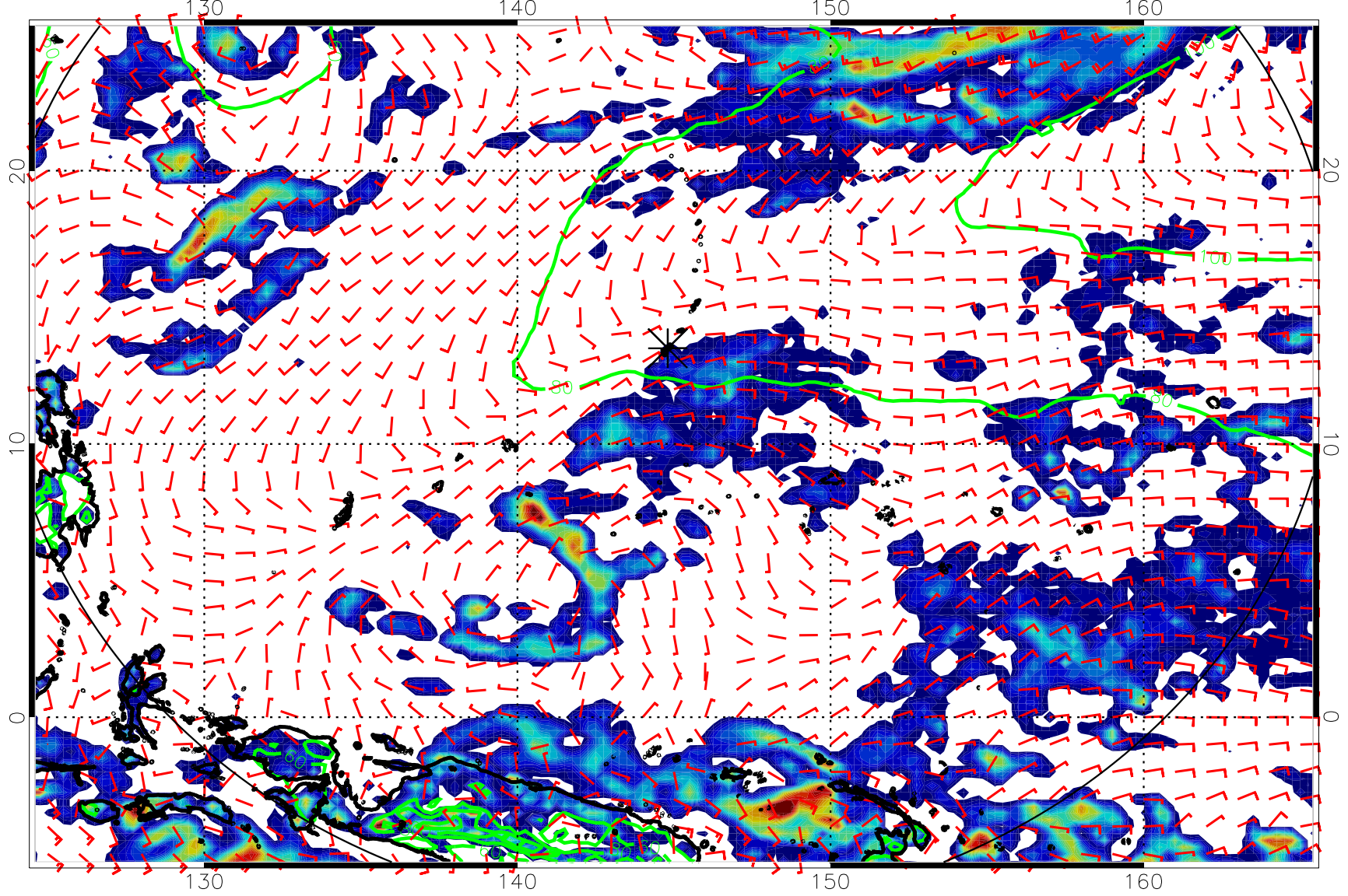
16072306, 114 hour forecast for precip, 1000mb Z, and winds (knots) -- NCEP GFS
