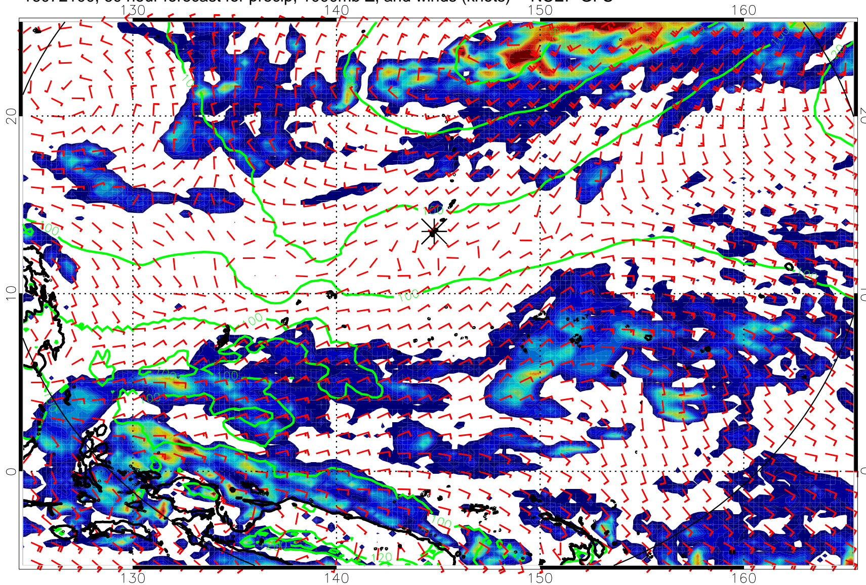
16072100, 60 hour forecast for precip, 1000mb Z, and winds (knots) -- NCEP GFS
