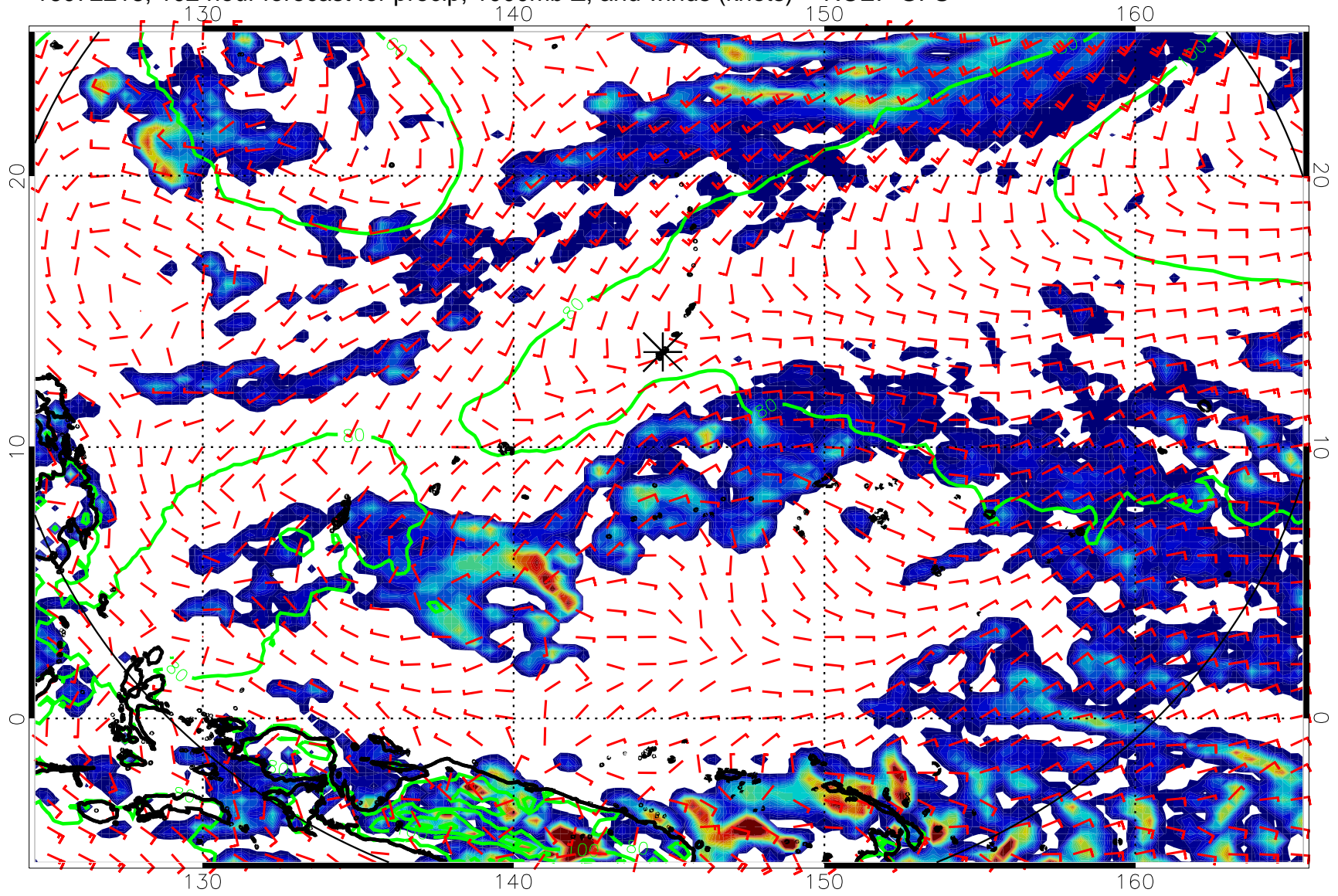
16072218, 102 hour forecast for precip, 1000mb Z, and winds (knots) -- NCEP GFS
