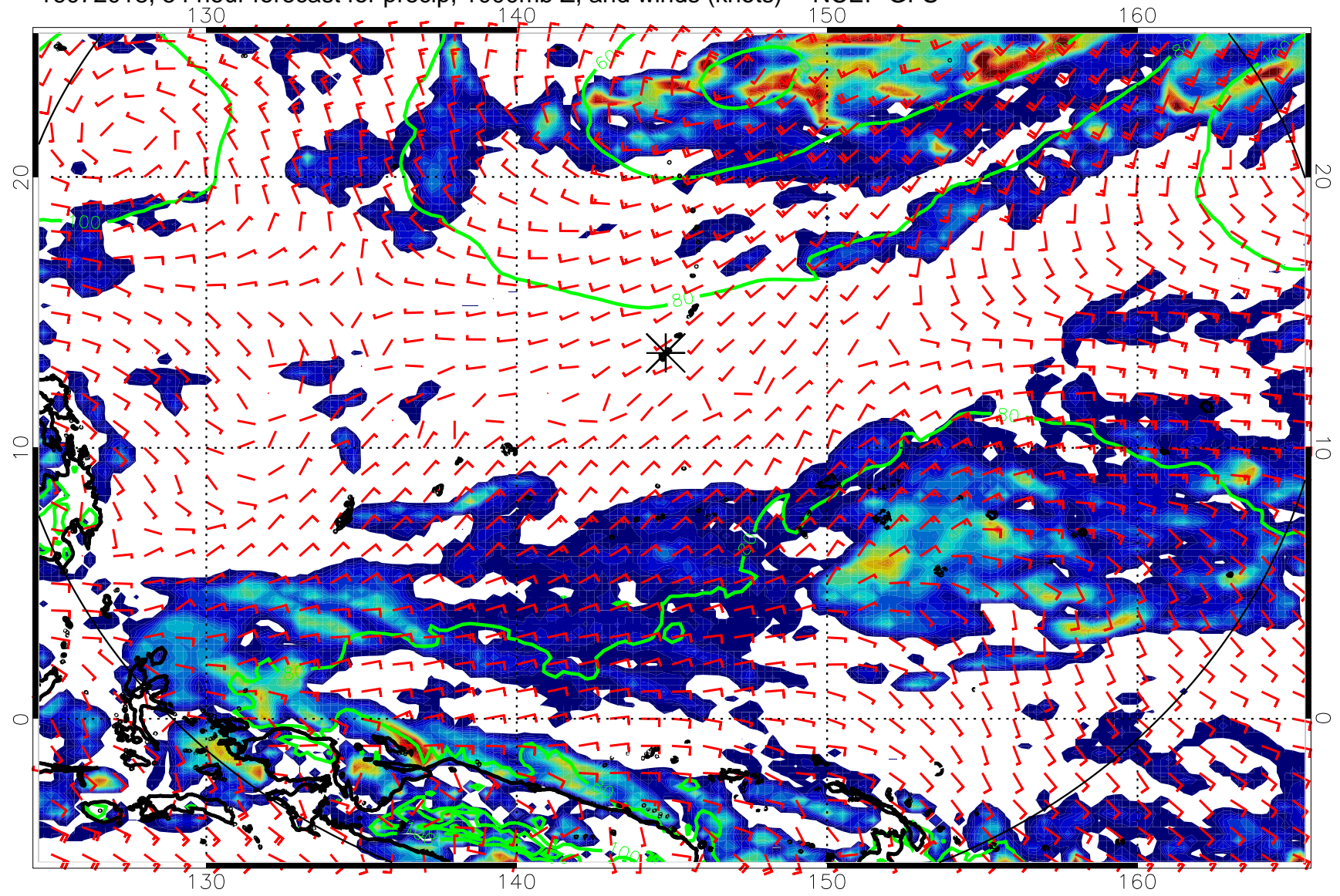
16072018, 54 hour forecast for precip, 1000mb Z, and winds (knots) -- NCEP GFS
