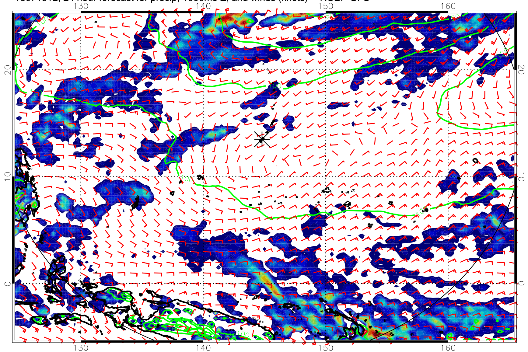
16071912, 24 hour forecast for precip, 1000mb Z, and winds (knots) -- NCEP GFS
