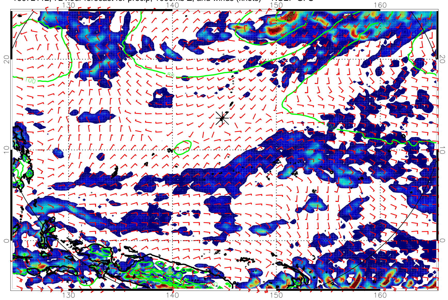
16072112, 72 hour forecast for precip, 1000mb Z, and winds (knots) -- NCEP GFS
