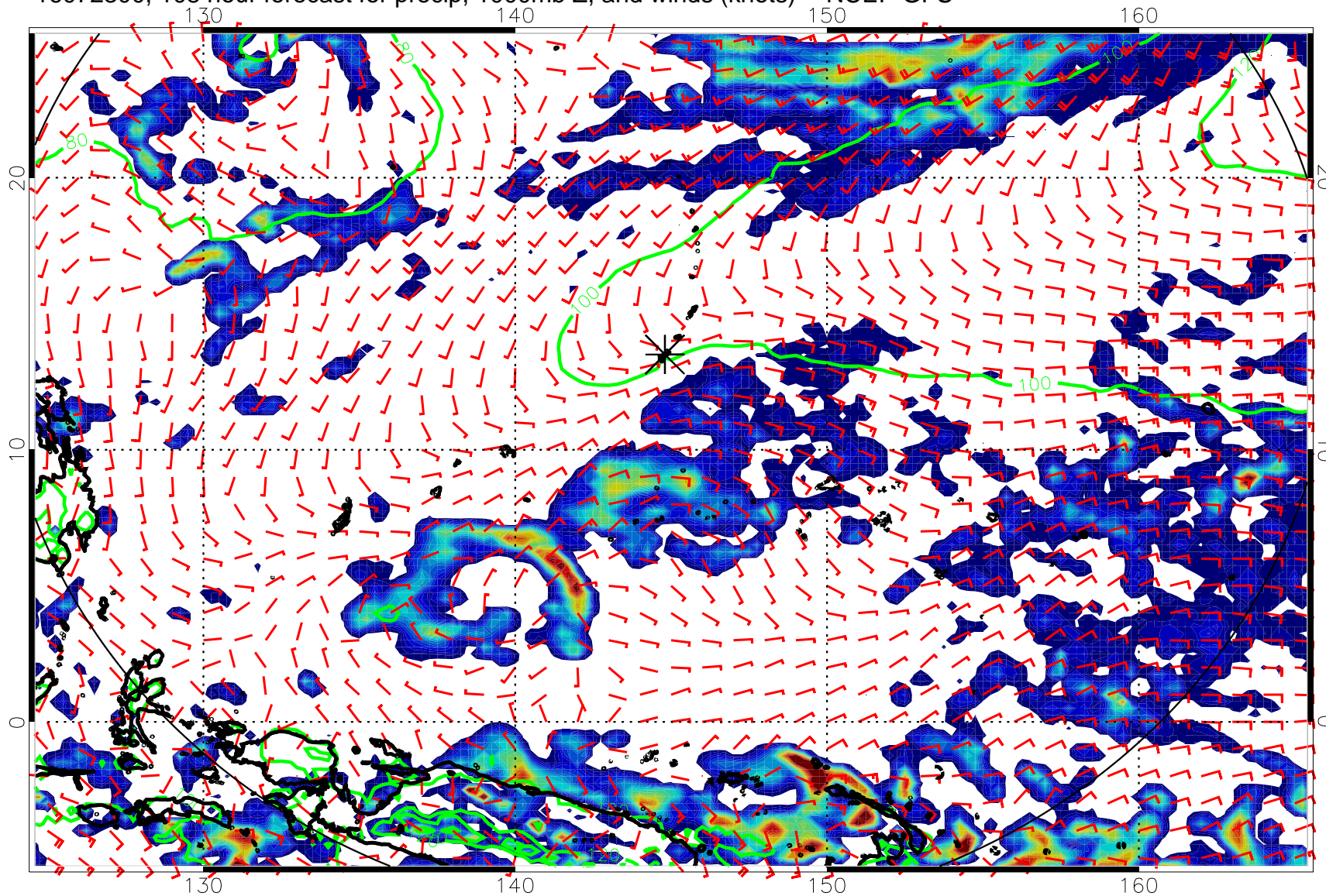
16072300, 108 hour forecast for precip, 1000mb Z, and winds (knots) -- NCEP GFS
