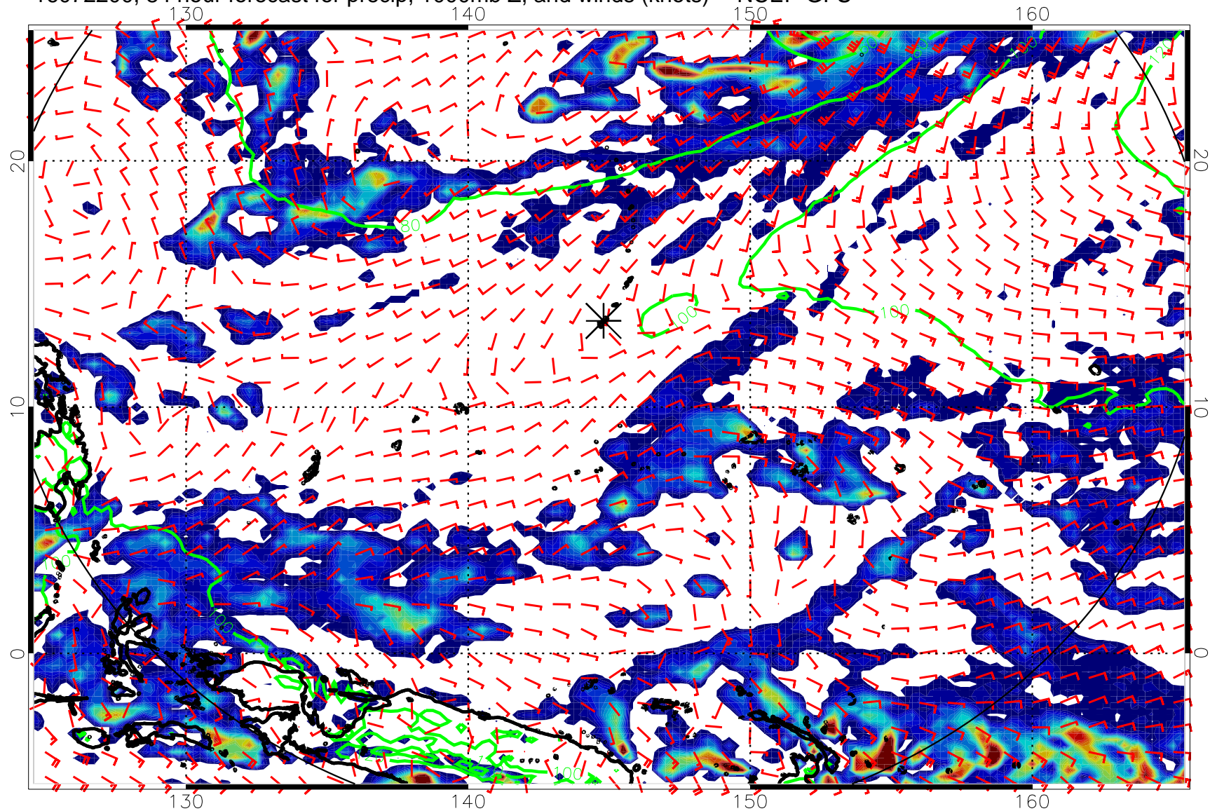
16072200, 84 hour forecast for precip, 1000mb Z, and winds (knots) -- NCEP GFS
