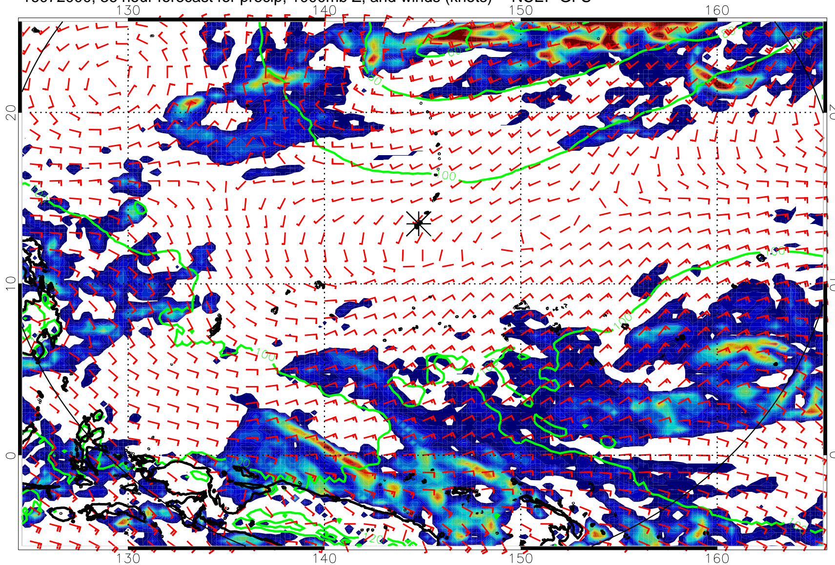
16072000, 36 hour forecast for precip, 1000mb Z, and winds (knots) -- NCEP GFS
