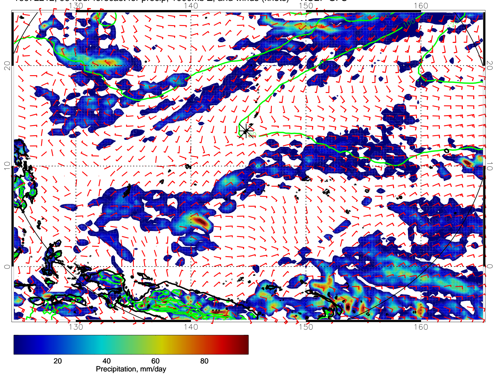
16072212, 96 hour forecast for precip, 1000mb Z, and winds (knots) -- NCEP GFS
