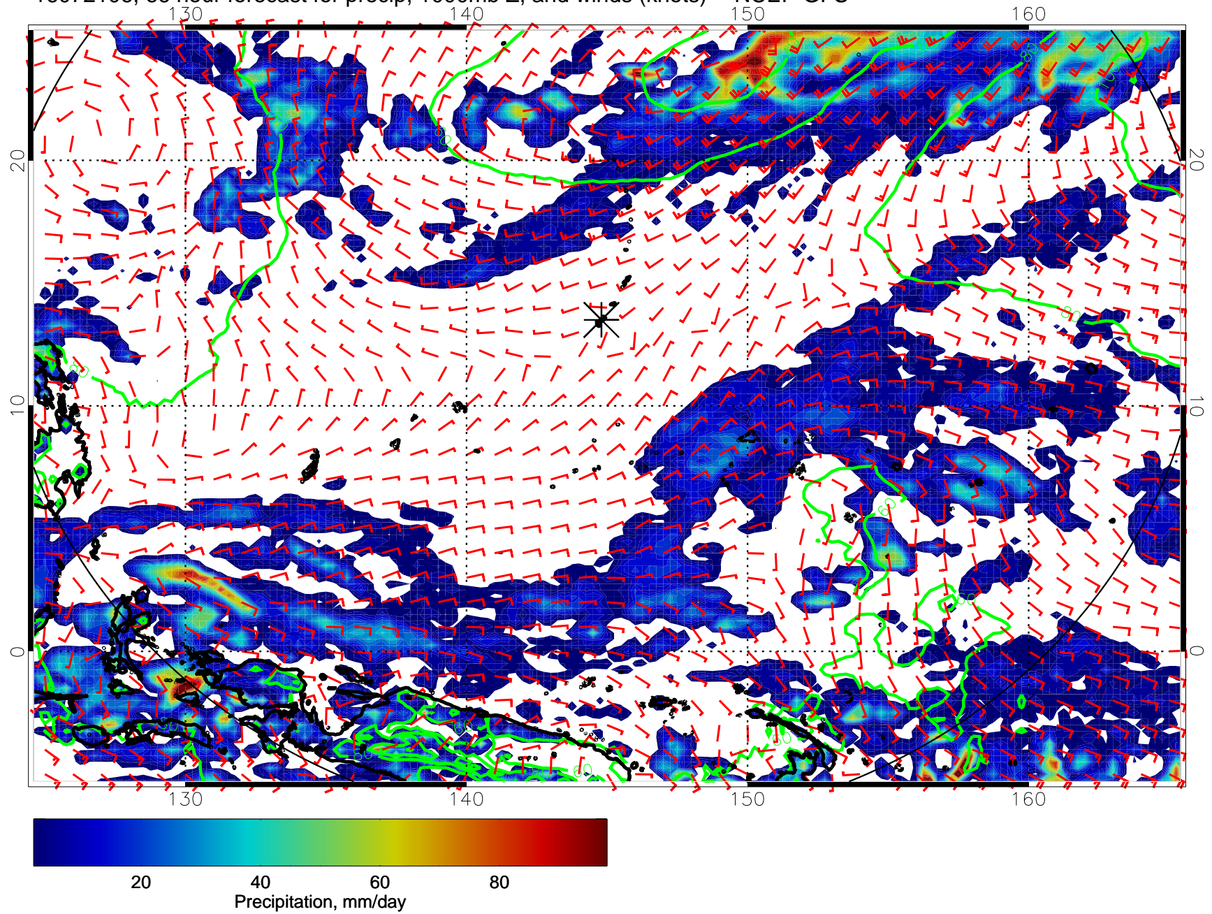
16072106, 66 hour forecast for precip, 1000mb Z, and winds (knots) -- NCEP GFS
