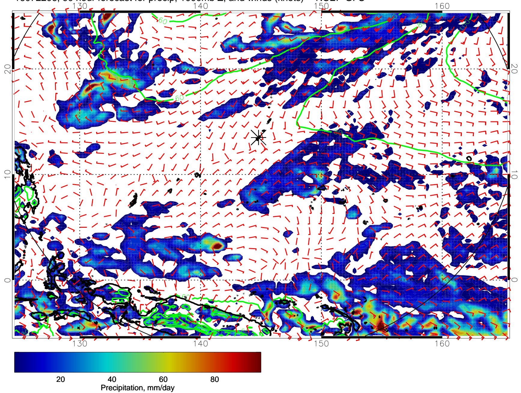
16072206, 90 hour forecast for precip, 1000mb Z, and winds (knots) -- NCEP GFS
