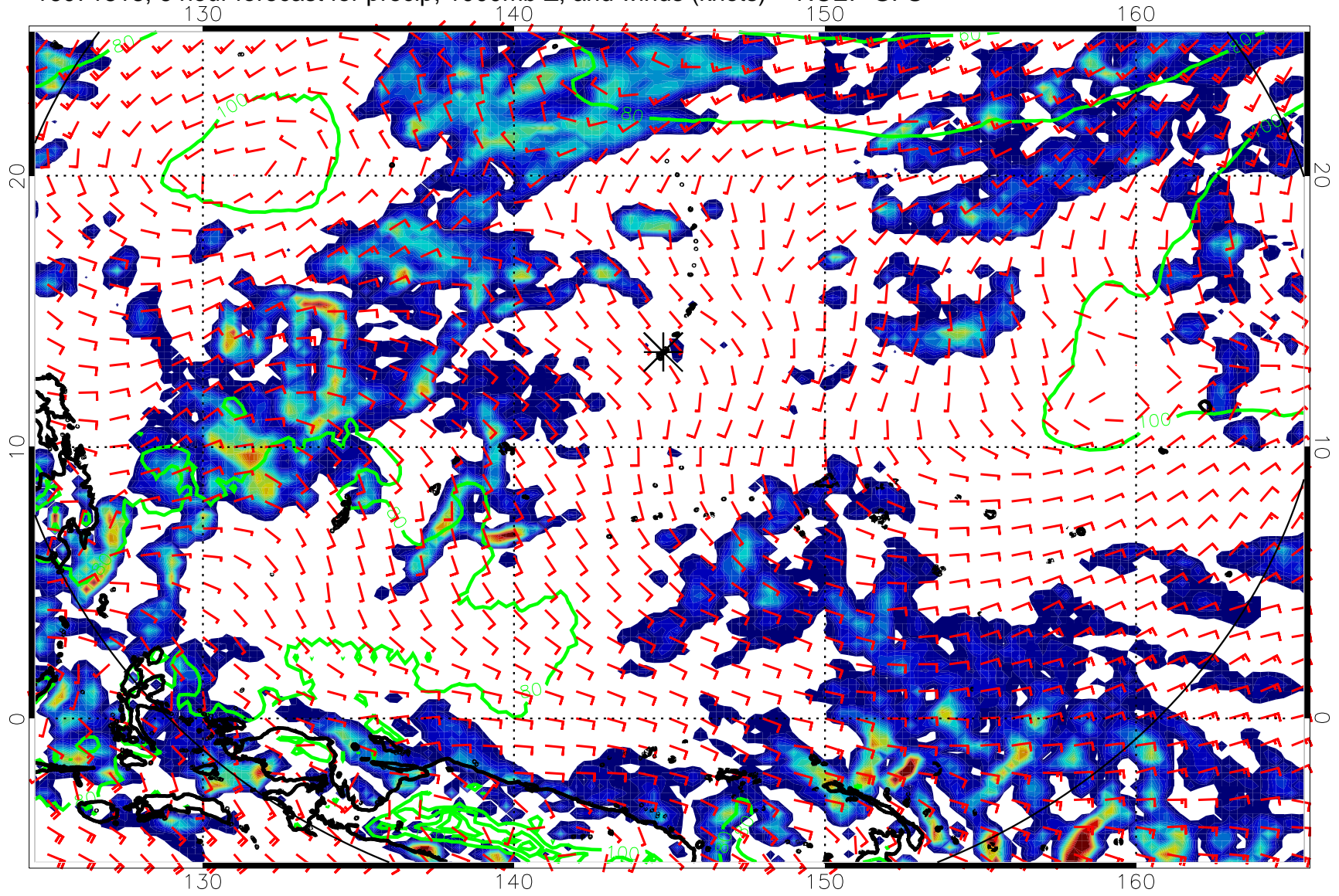
16071818, 6 hour forecast for precip, 1000mb Z, and winds (knots) -- NCEP GFS
