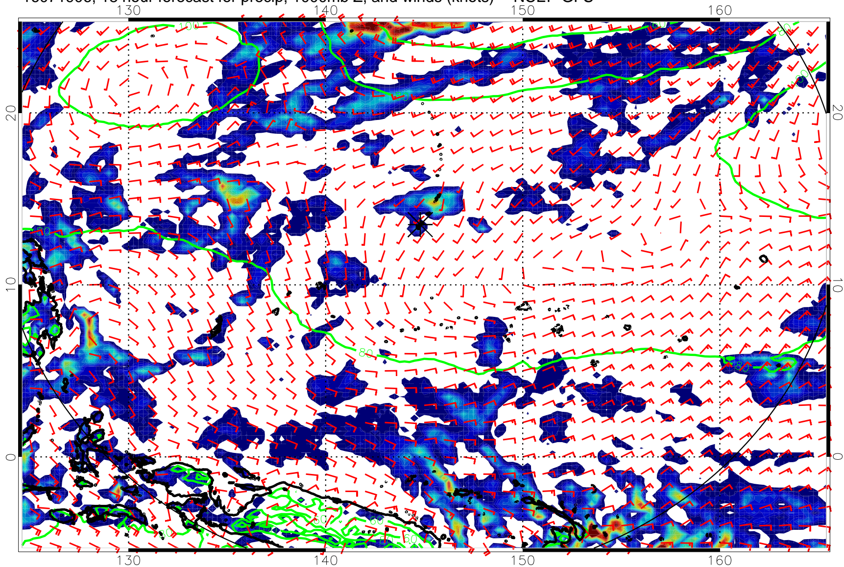
16071906, 18 hour forecast for precip, 1000mb Z, and winds (knots) -- NCEP GFS
