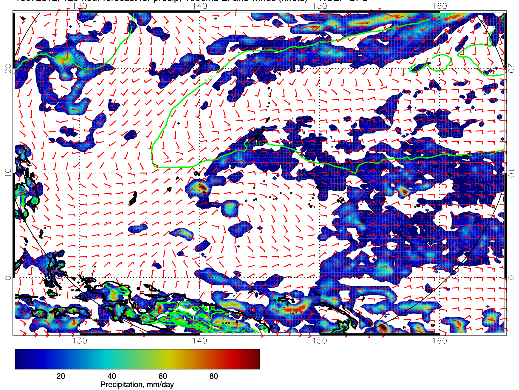
16072312, 120 hour forecast for precip, 1000mb Z, and winds (knots) -- NCEP GFS
