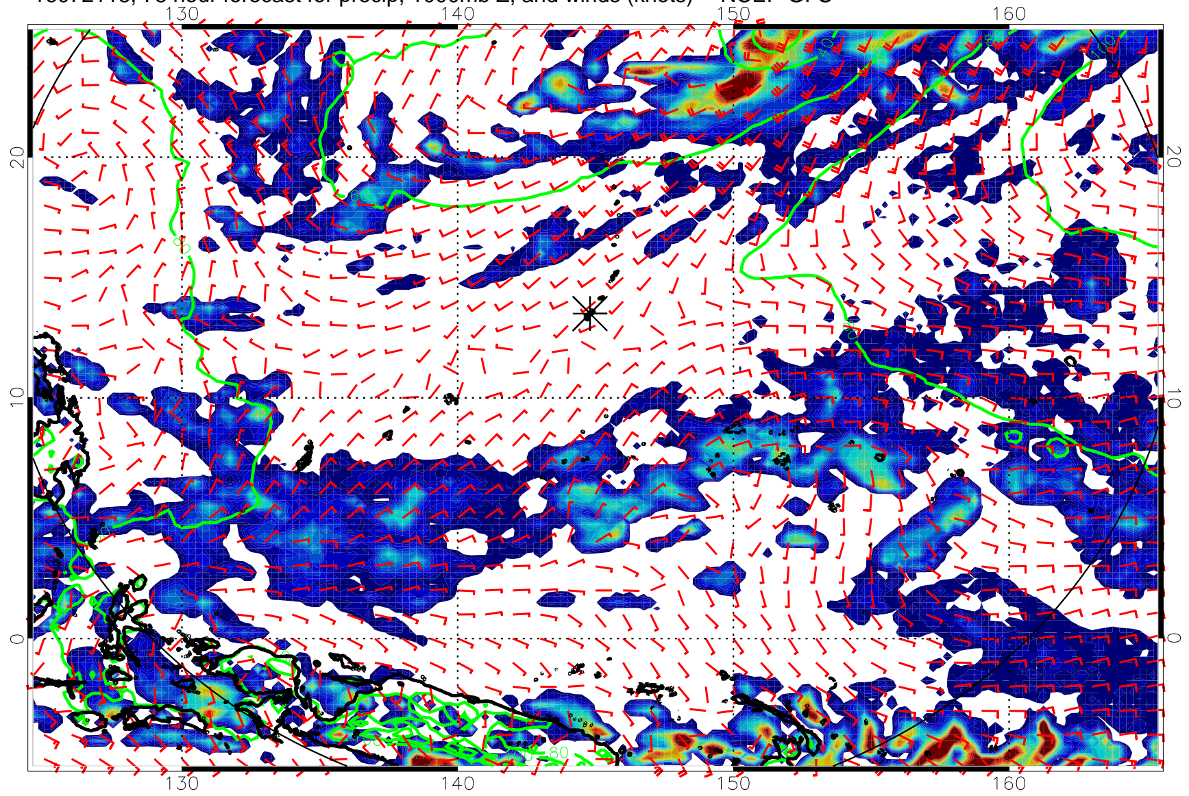
16072118, 78 hour forecast for precip, 1000mb Z, and winds (knots) -- NCEP GFS
