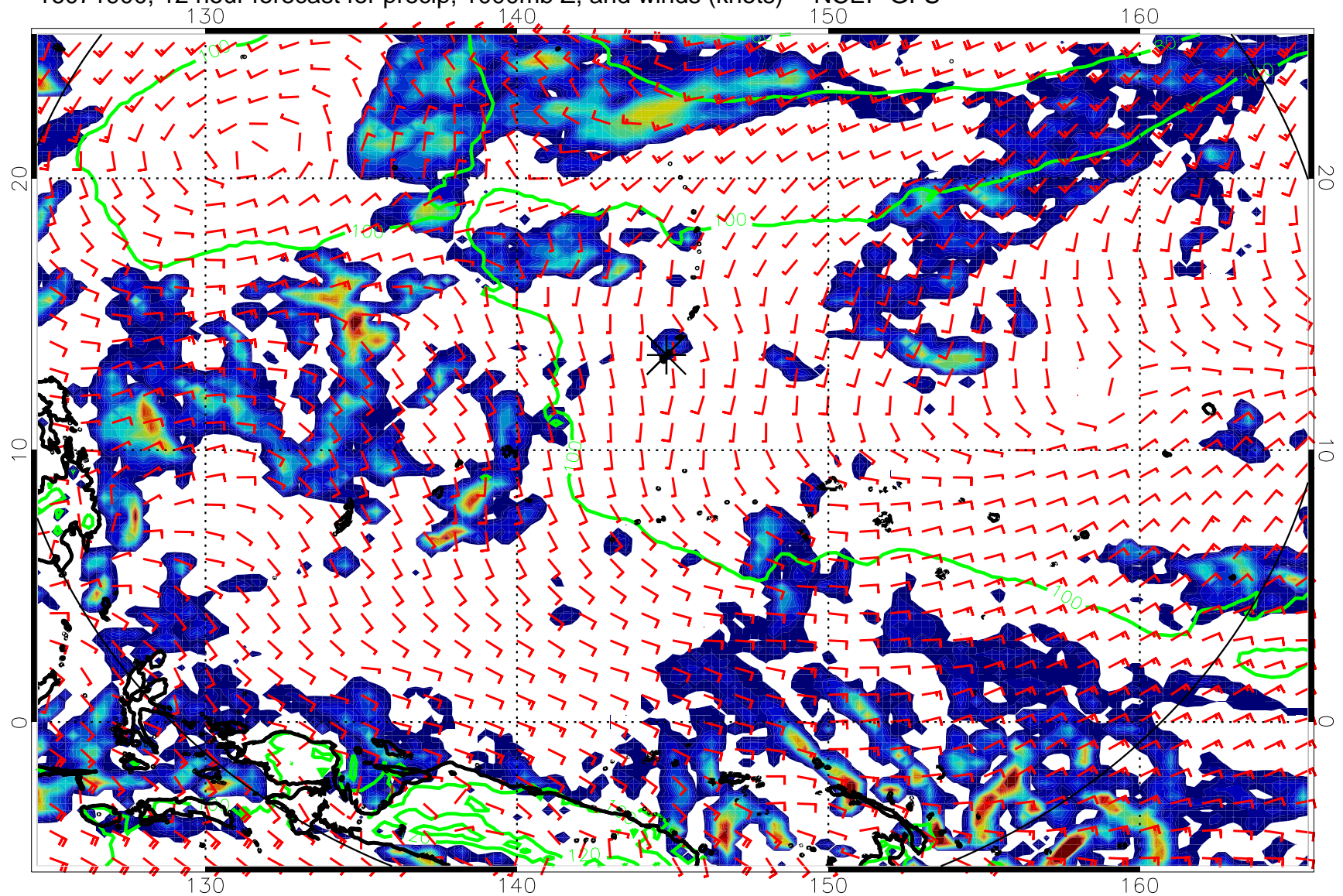
16071900, 12 hour forecast for precip, 1000mb Z, and winds (knots) -- NCEP GFS
