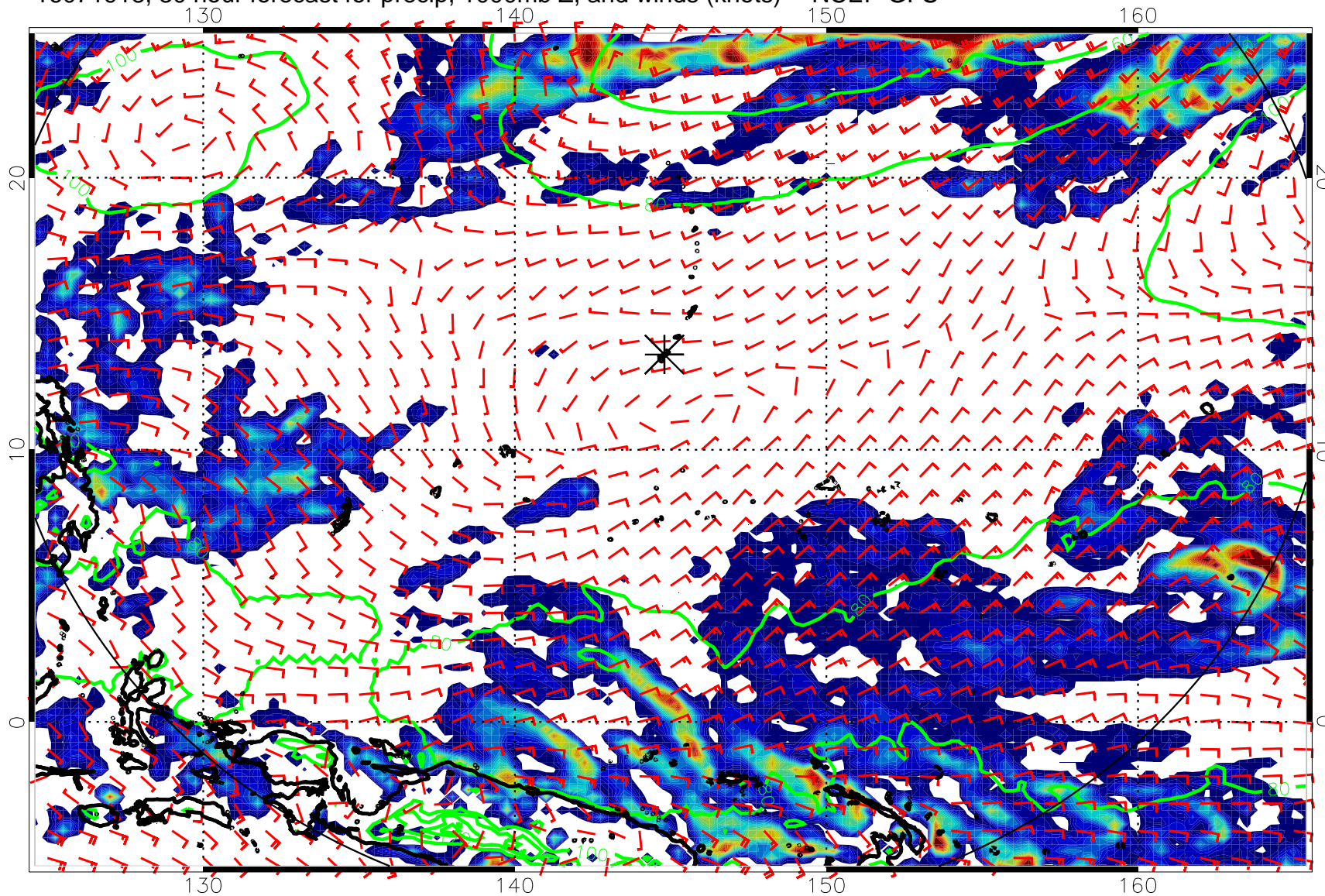
16071918, 30 hour forecast for precip, 1000mb Z, and winds (knots) -- NCEP GFS
