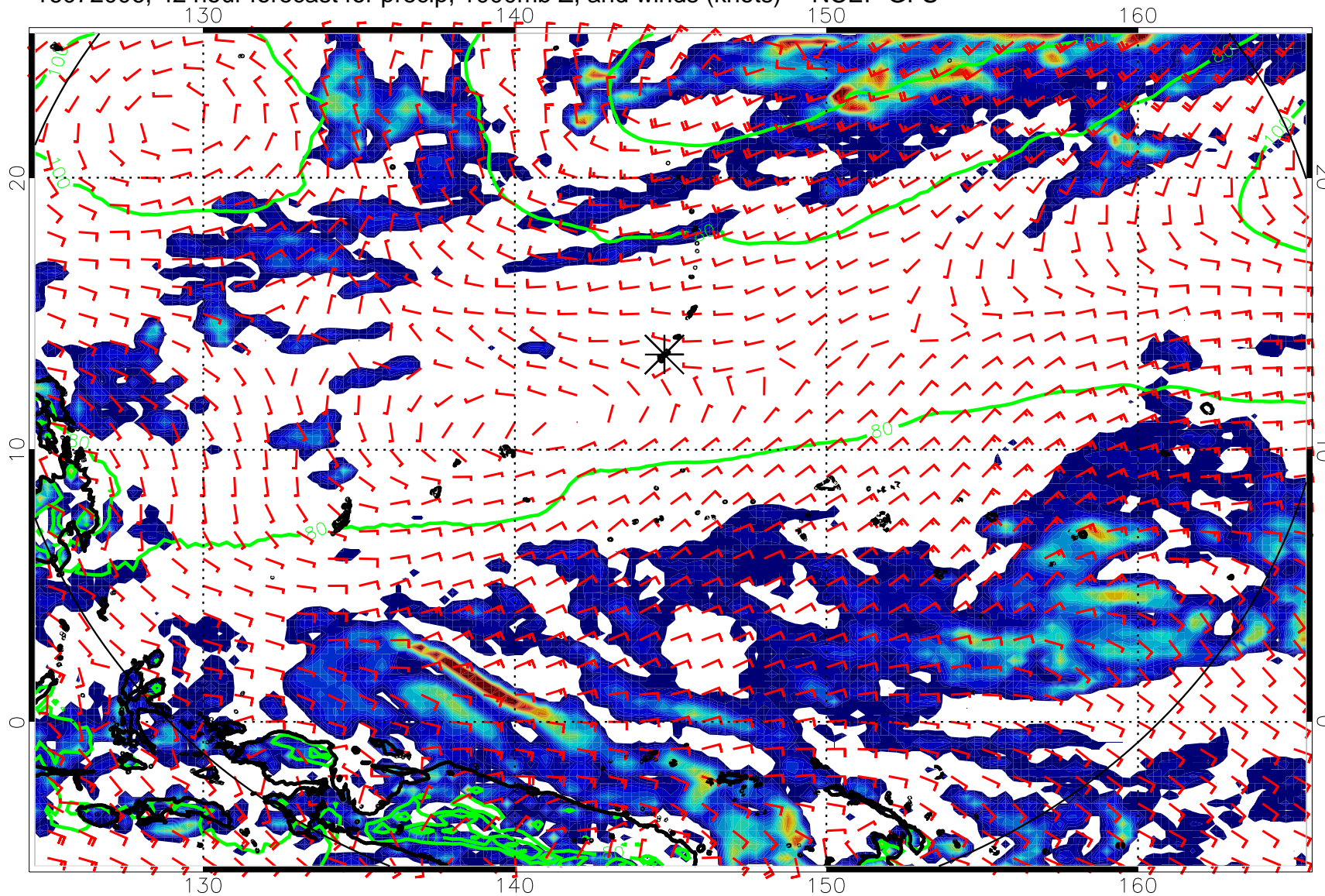
16072006, 42 hour forecast for precip, 1000mb Z, and winds (knots) -- NCEP GFS
