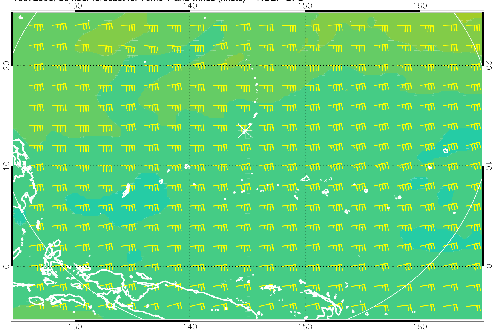
16072000, 36 hour forecast for 70mb T and winds (knots) -- NCEP GFS
