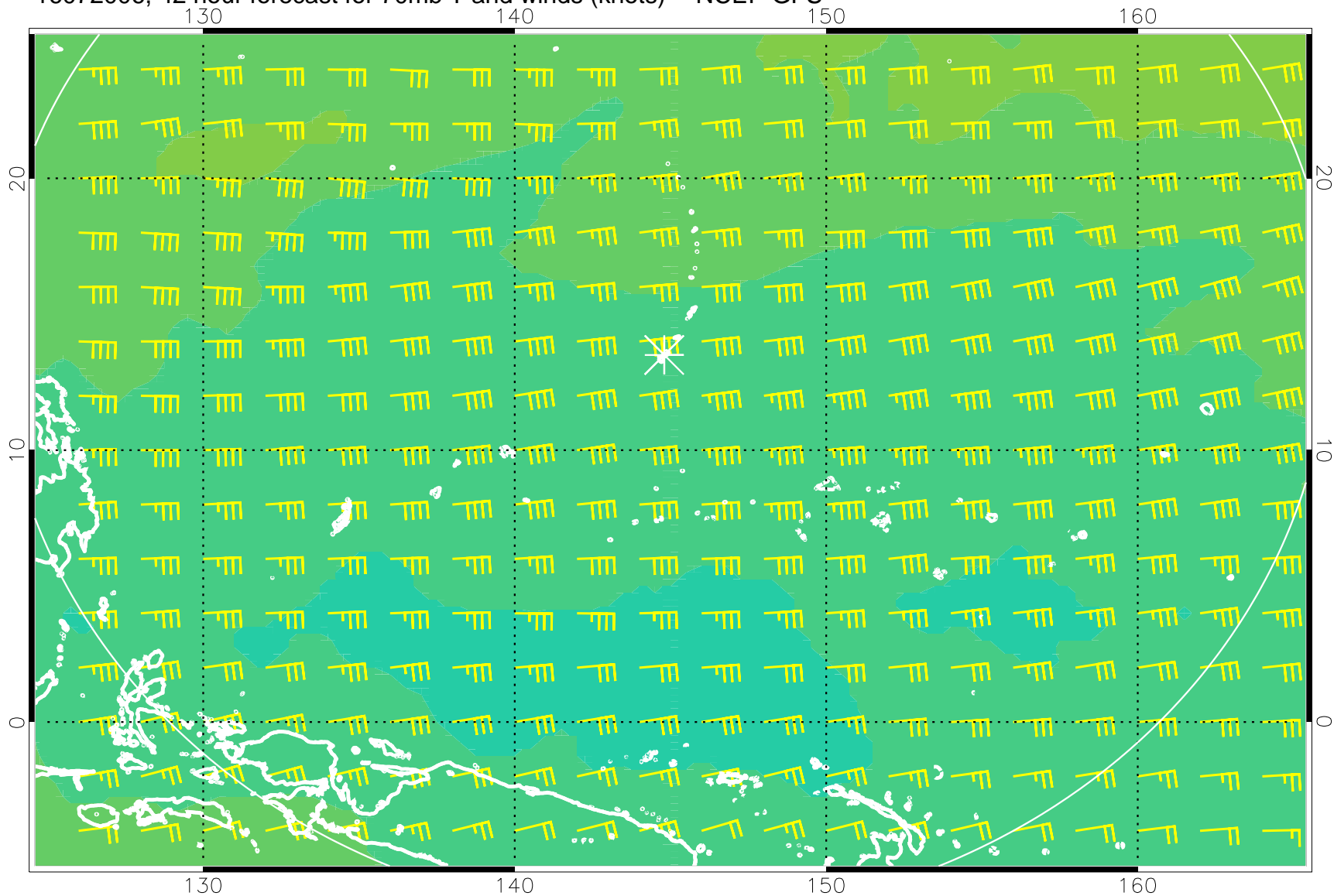
16072006, 42 hour forecast for 70mb T and winds (knots) -- NCEP GFS
