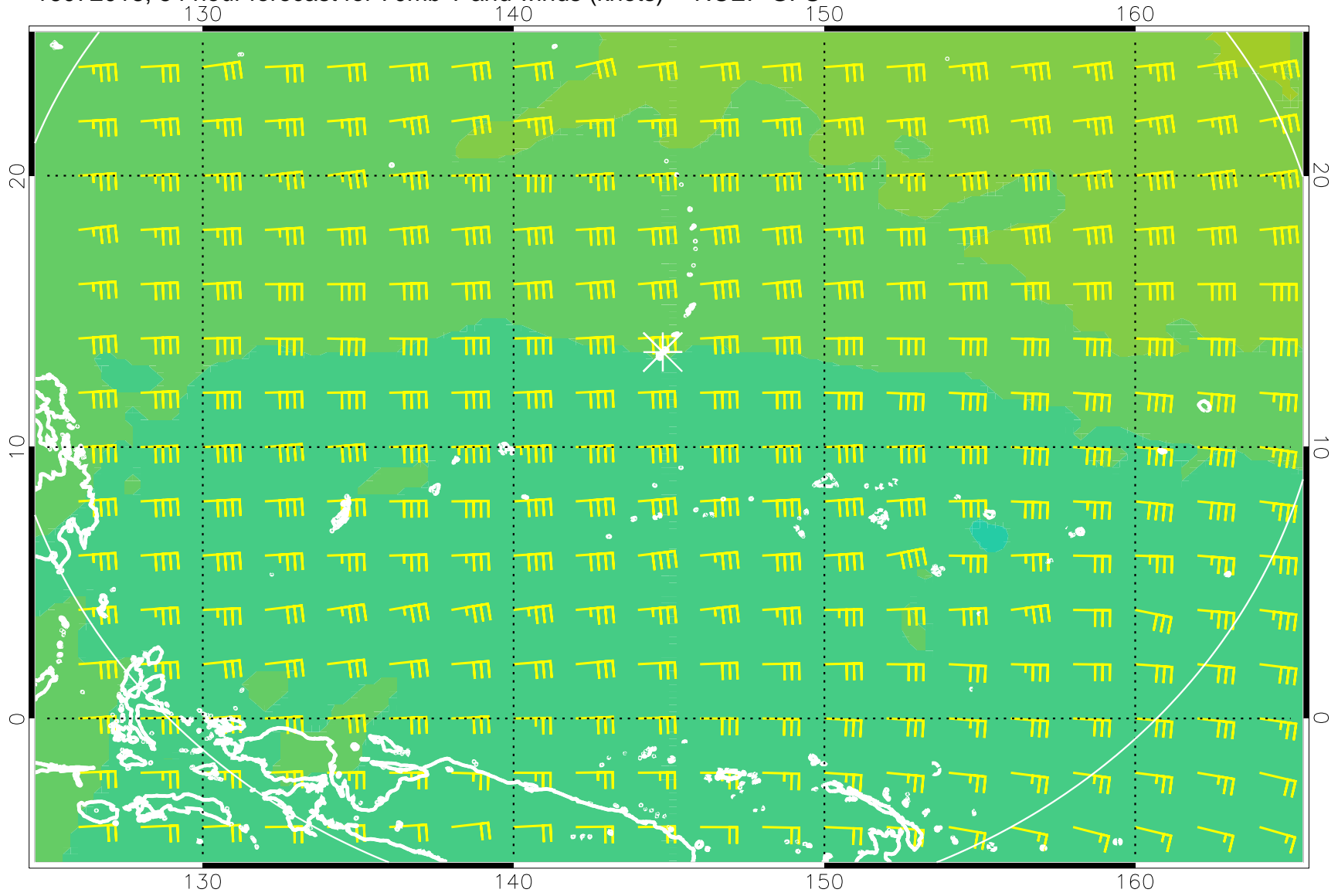
16072018, 54 hour forecast for 70mb T and winds (knots) -- NCEP GFS
