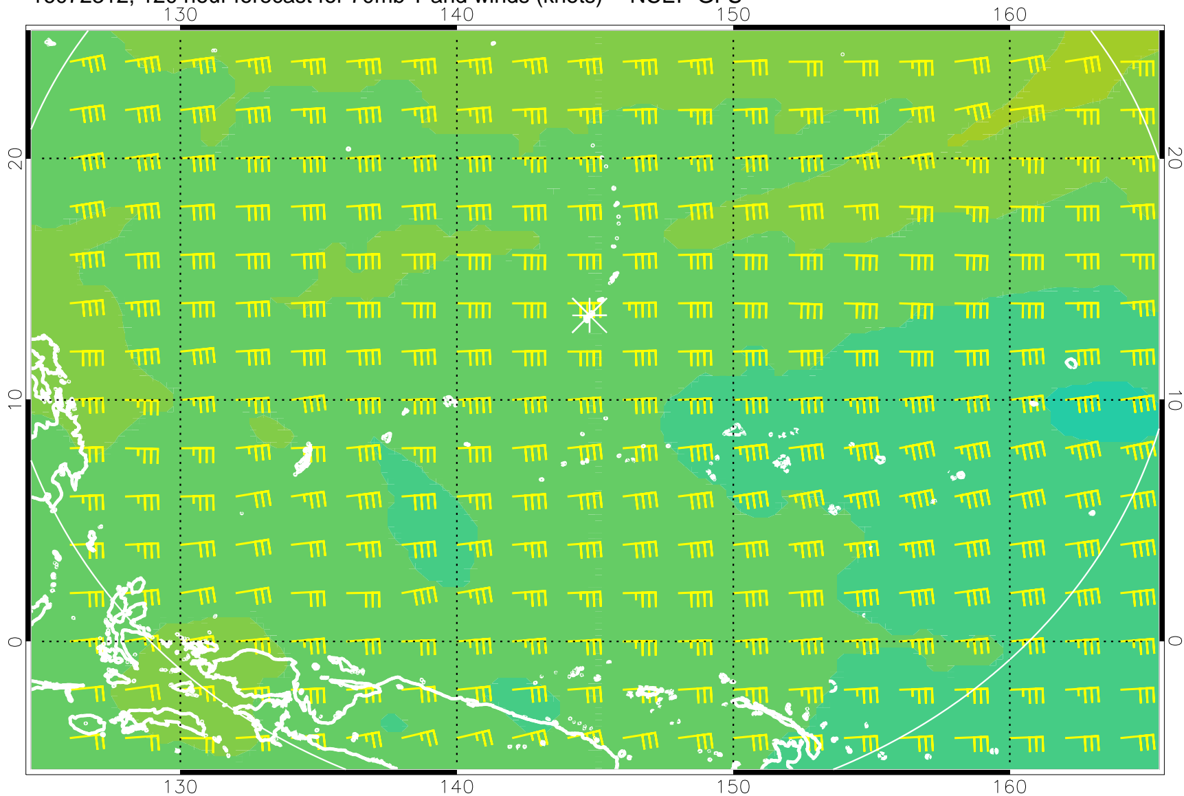
16072312, 120 hour forecast for 70mb T and winds (knots) -- NCEP GFS
