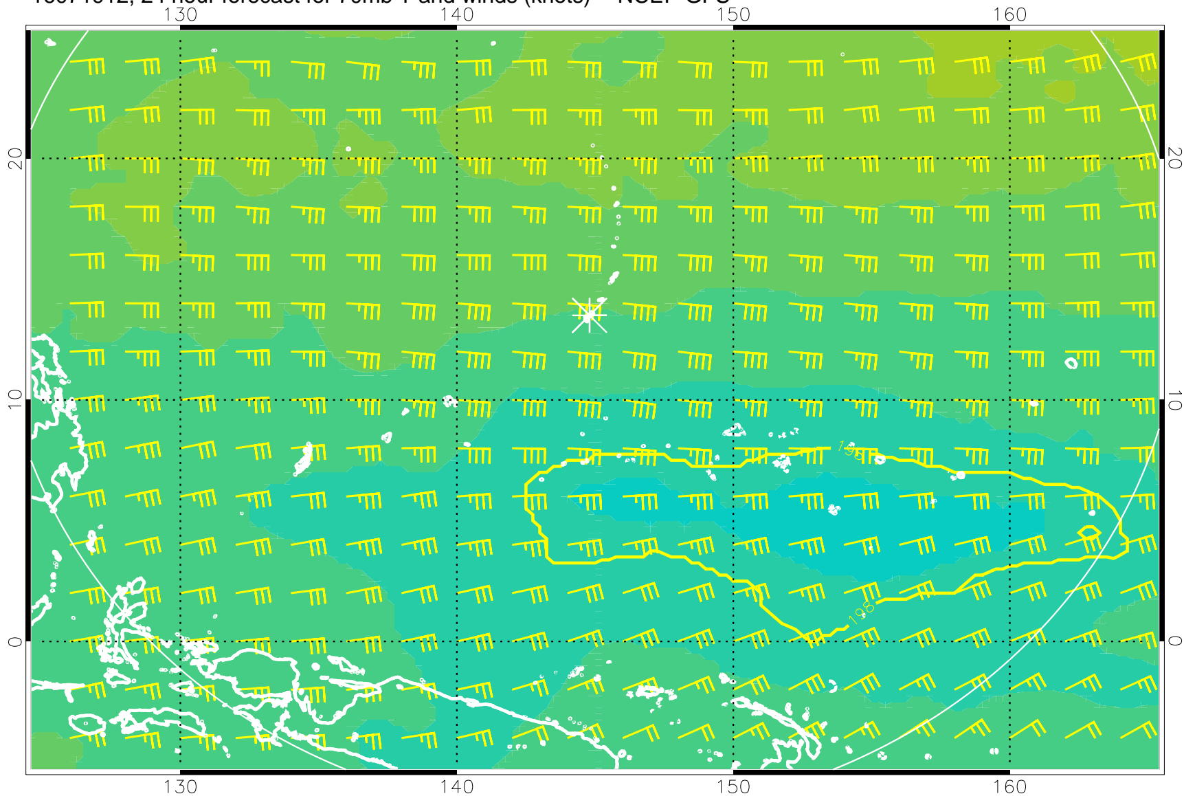
16071912, 24 hour forecast for 70mb T and winds (knots) -- NCEP GFS
