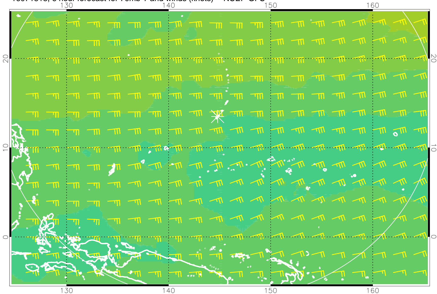
16071818, 6 hour forecast for 70mb T and winds (knots) -- NCEP GFS
