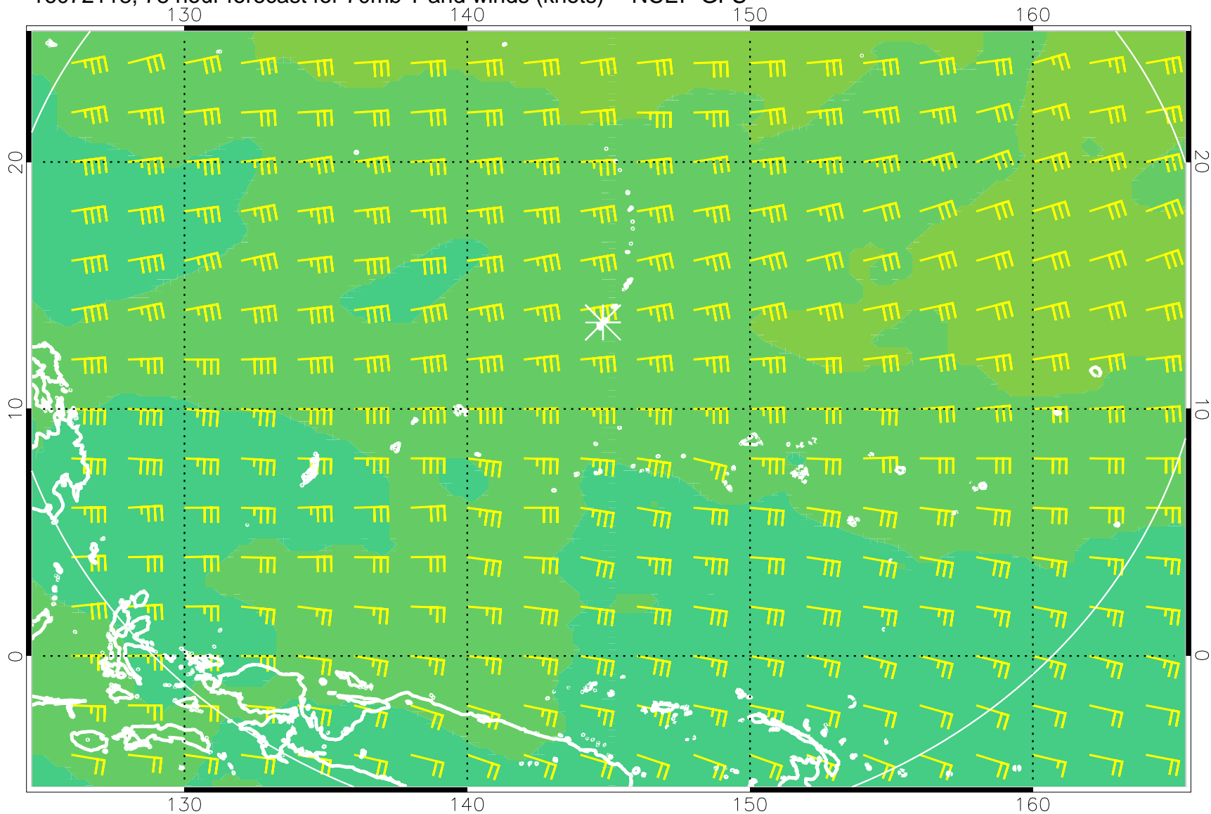
16072118, 78 hour forecast for 70mb T and winds (knots) -- NCEP GFS
