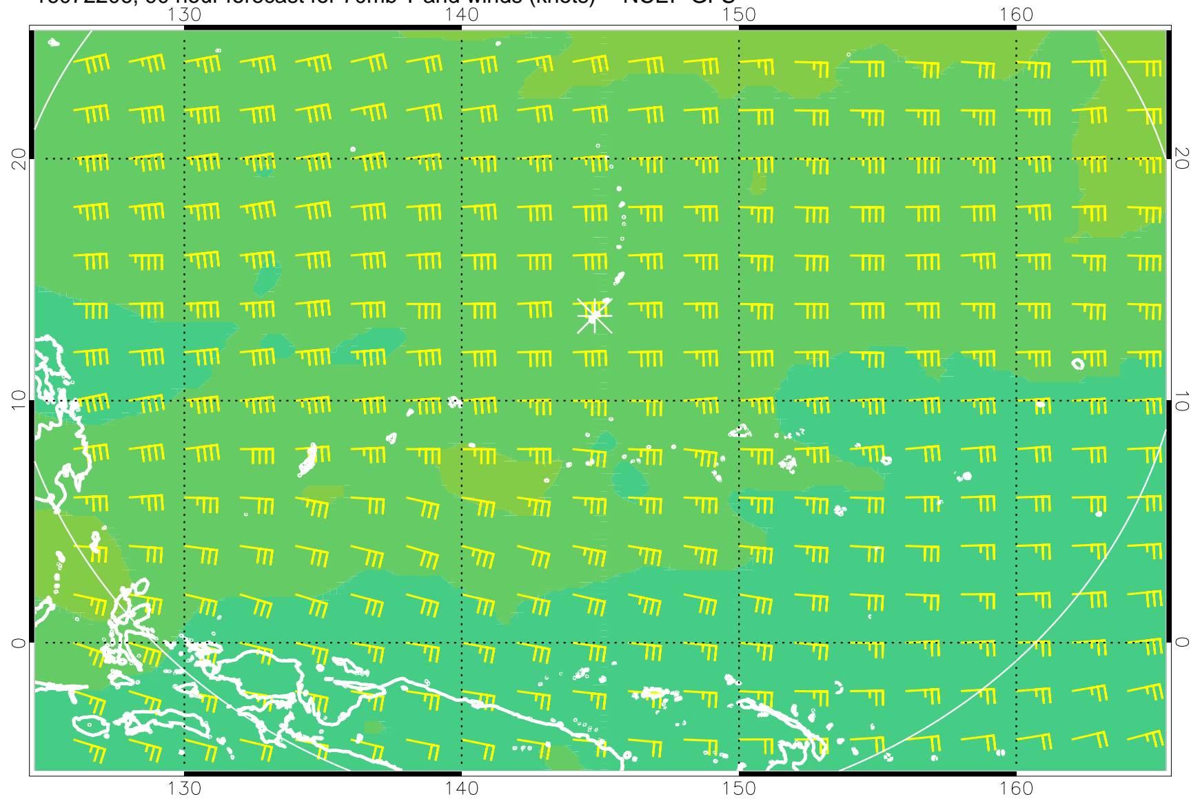
16072206, 90 hour forecast for 70mb T and winds (knots) -- NCEP GFS
