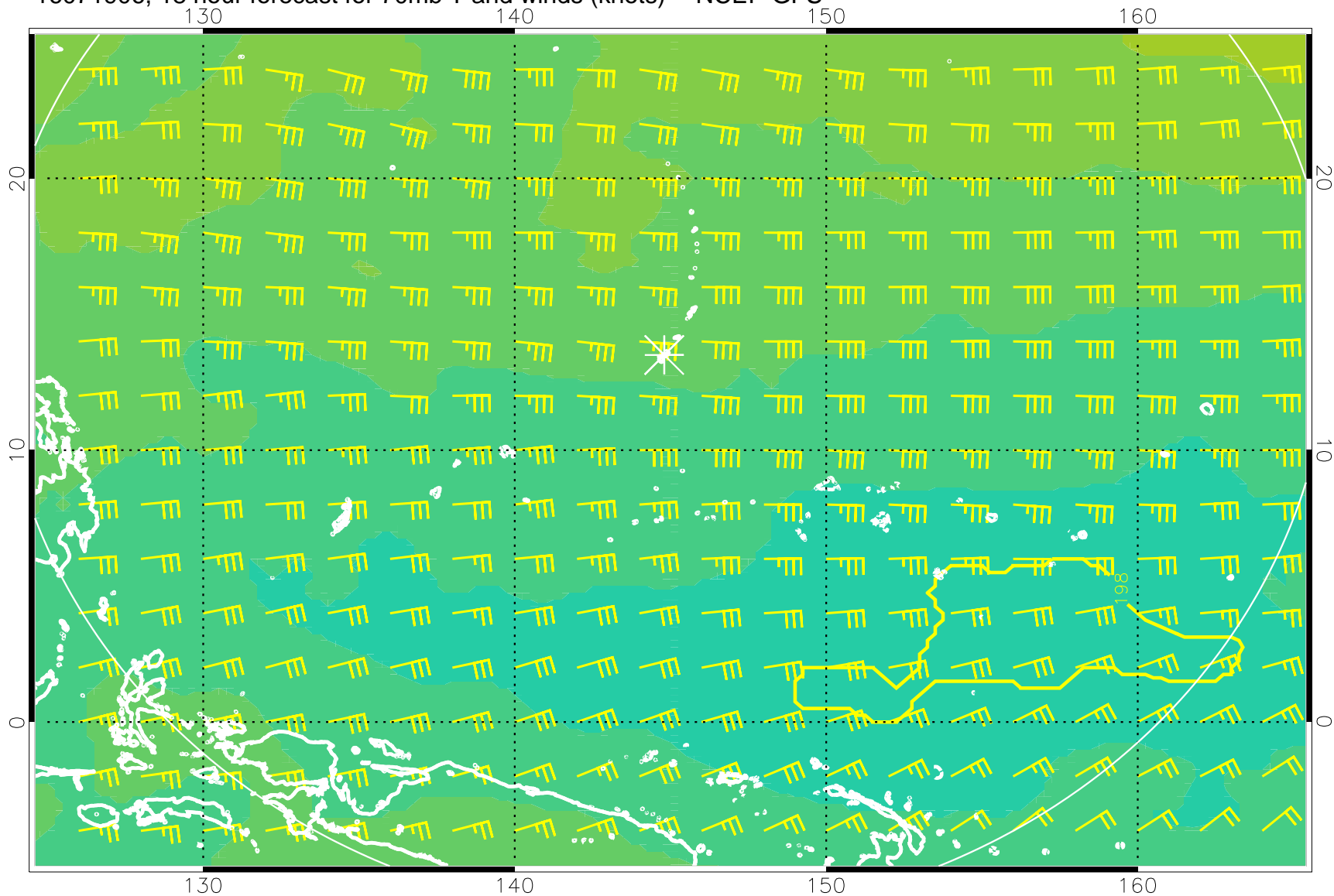
16071906, 18 hour forecast for 70mb T and winds (knots) -- NCEP GFS
