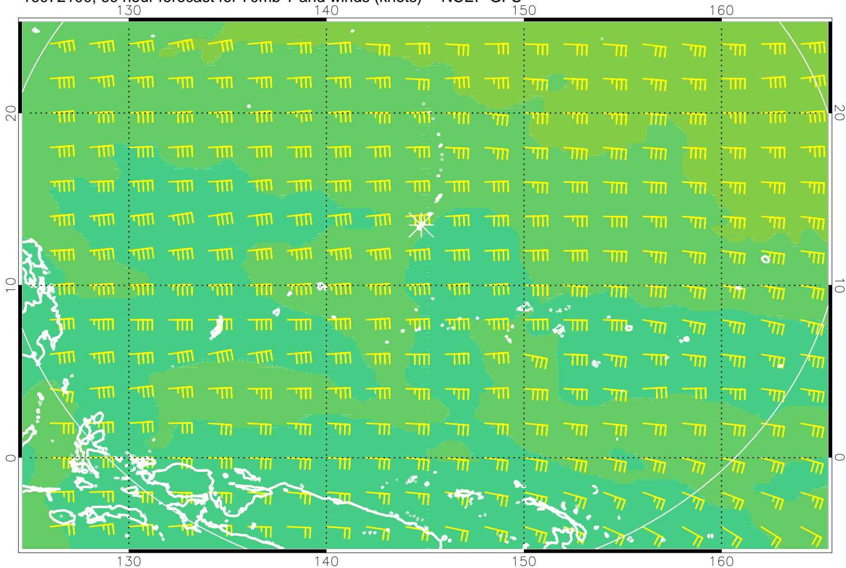
16072100, 60 hour forecast for 70mb T and winds (knots) -- NCEP GFS
