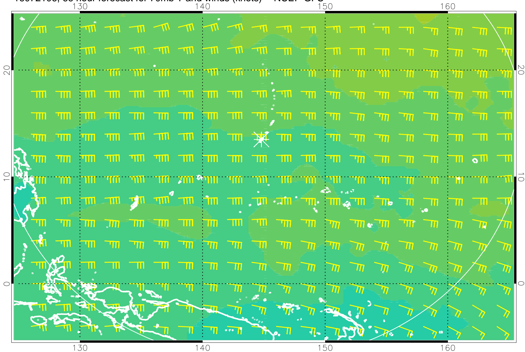
16072106, 66 hour forecast for 70mb T and winds (knots) -- NCEP GFS
