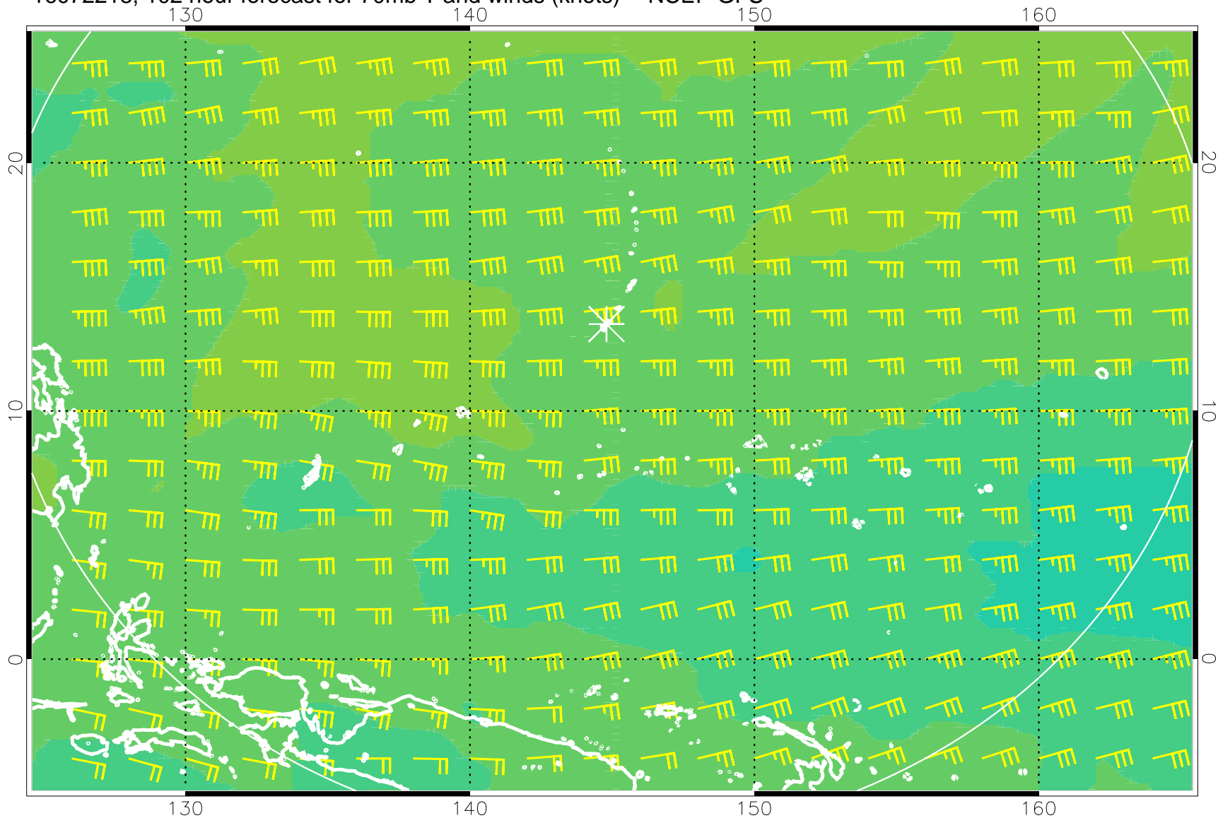
16072218, 102 hour forecast for 70mb T and winds (knots) -- NCEP GFS
