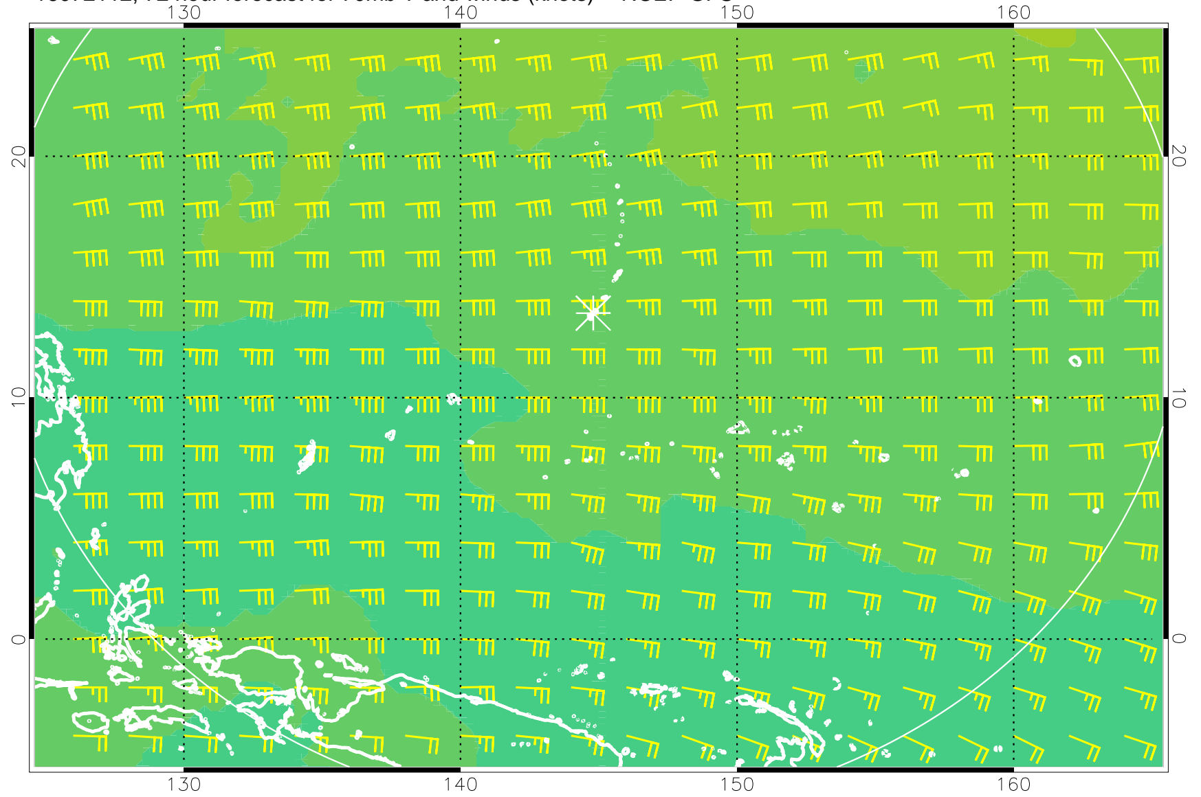
16072112, 72 hour forecast for 70mb T and winds (knots) -- NCEP GFS
