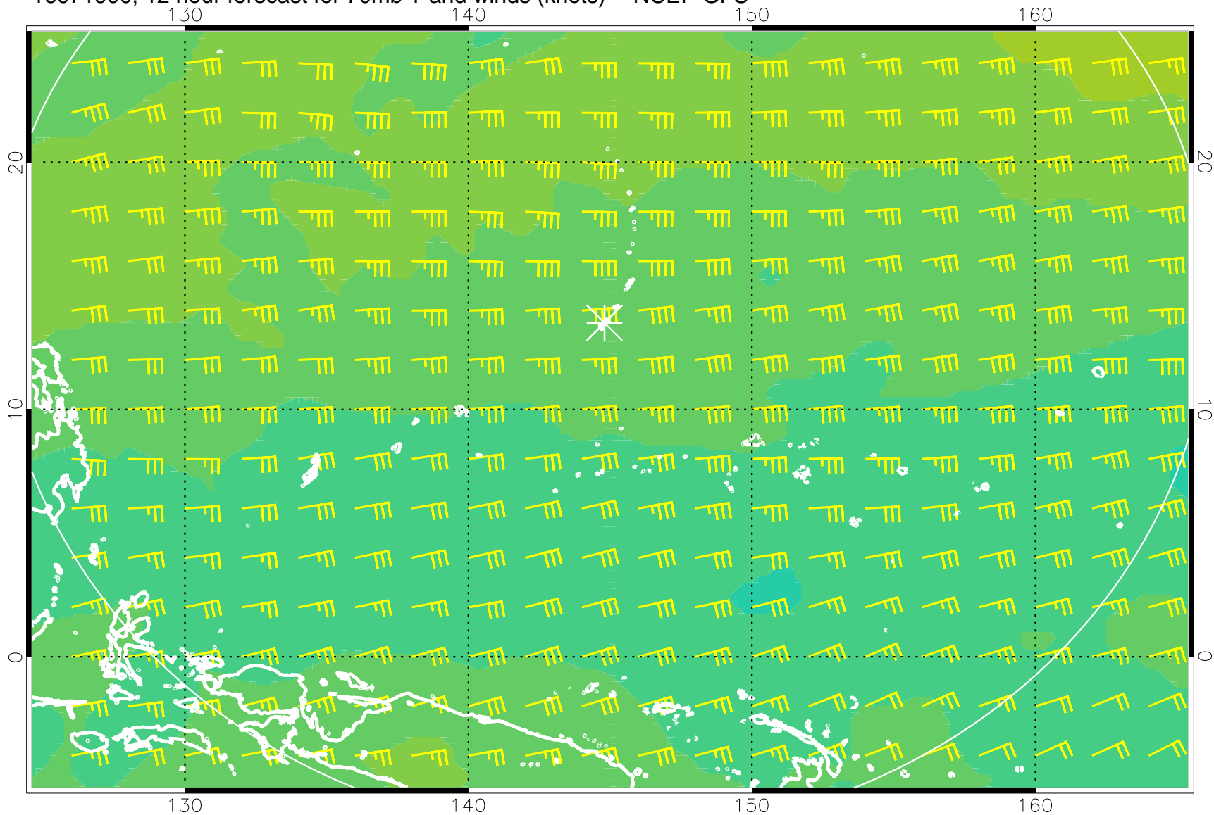
16071900, 12 hour forecast for 70mb T and winds (knots) -- NCEP GFS
