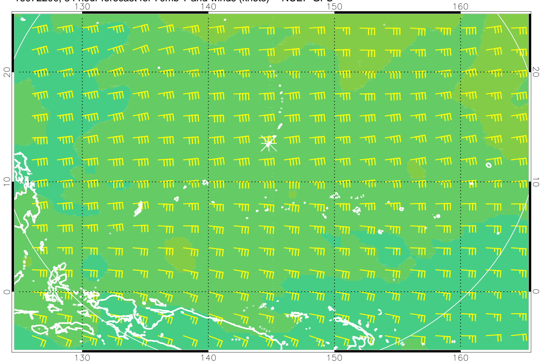
16072200, 84 hour forecast for 70mb T and winds (knots) -- NCEP GFS
