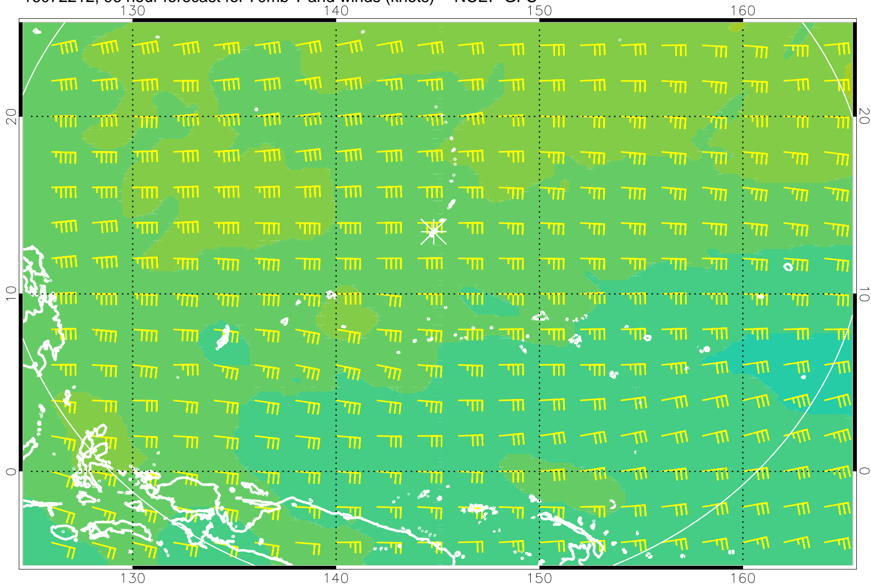
16072212, 96 hour forecast for 70mb T and winds (knots) -- NCEP GFS
