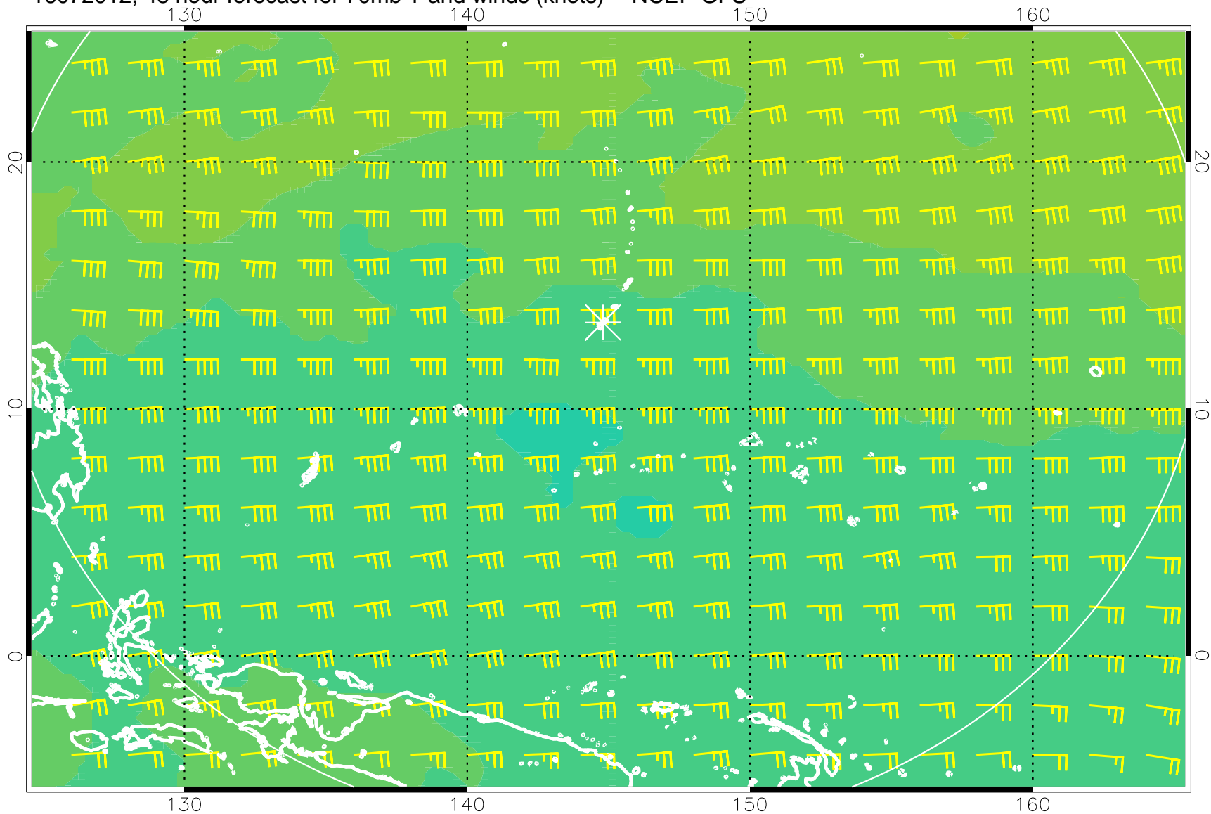
16072012, 48 hour forecast for 70mb T and winds (knots) -- NCEP GFS
