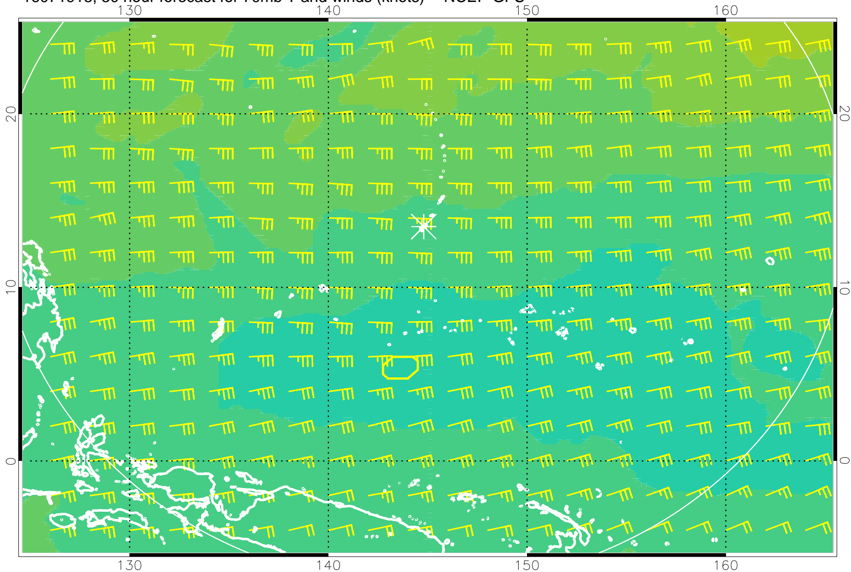
16071918, 30 hour forecast for 70mb T and winds (knots) -- NCEP GFS
