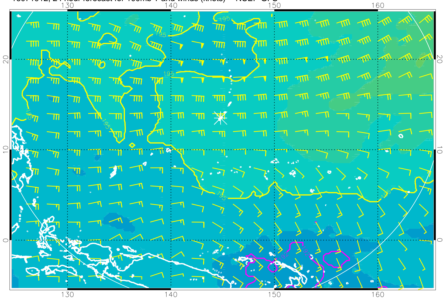
16071912, 24 hour forecast for 100mb T and winds (knots) -- NCEP GFS
