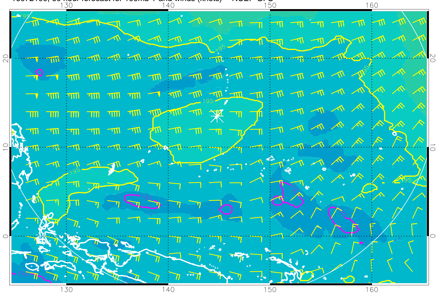
16072100, 60 hour forecast for 100mb T and winds (knots) -- NCEP GFS
