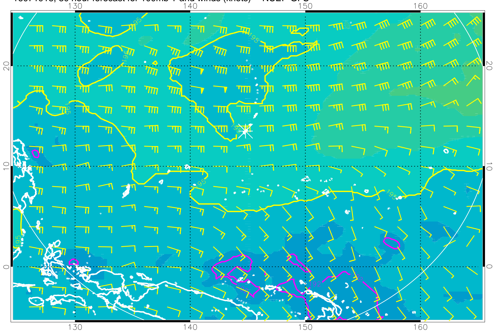
16071918, 30 hour forecast for 100mb T and winds (knots) -- NCEP GFS
