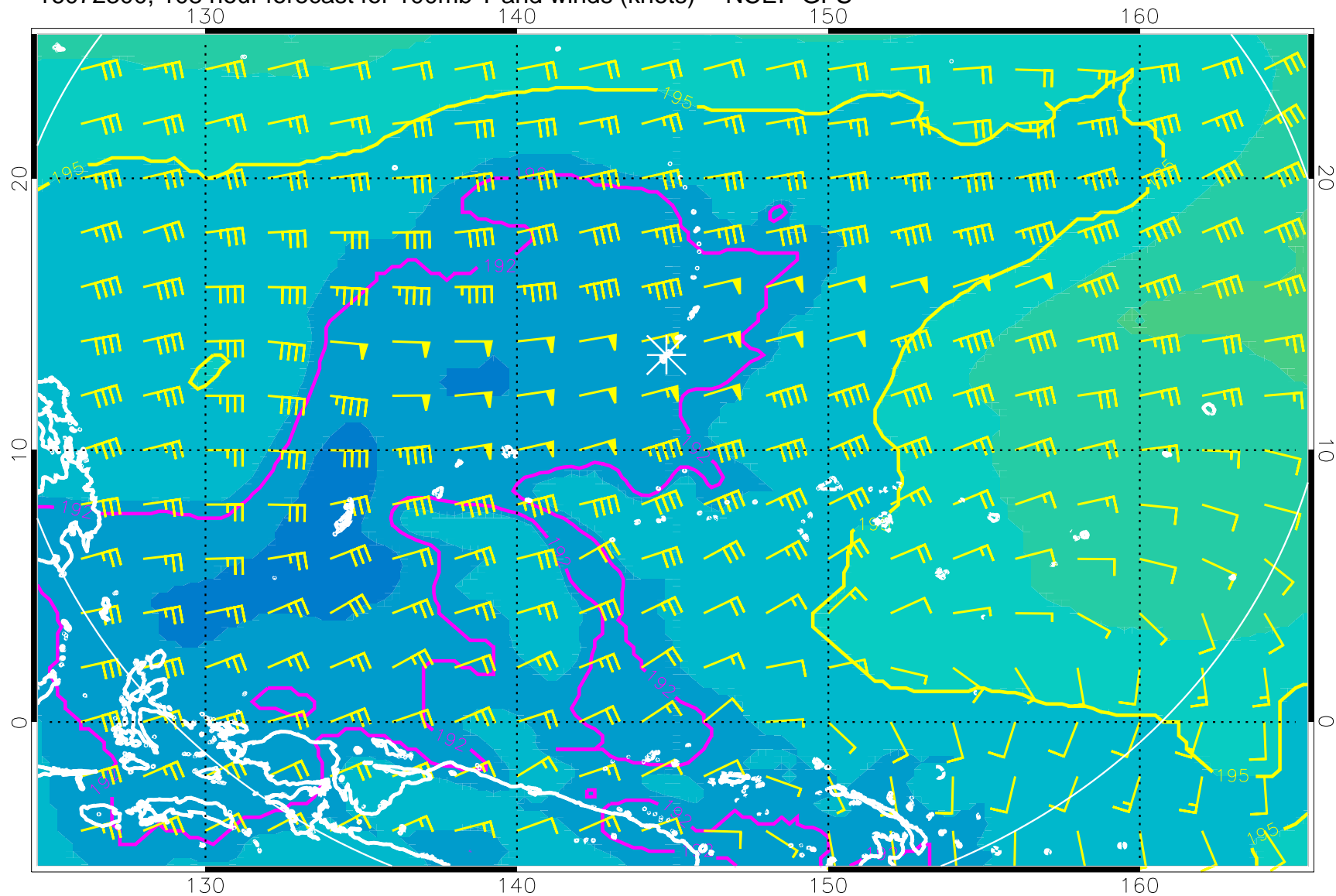
16072300, 108 hour forecast for 100mb T and winds (knots) -- NCEP GFS
