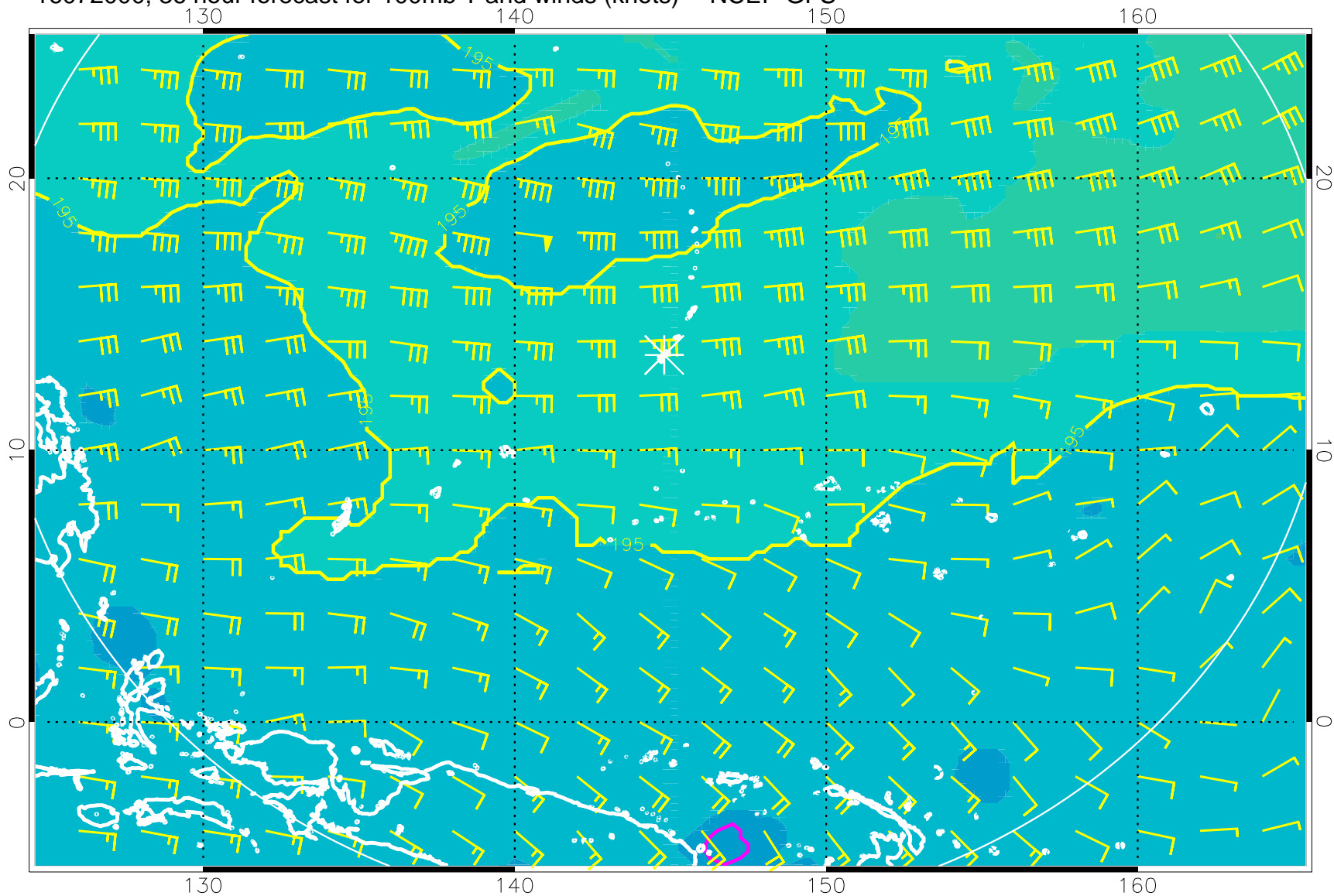
16072000, 36 hour forecast for 100mb T and winds (knots) -- NCEP GFS
