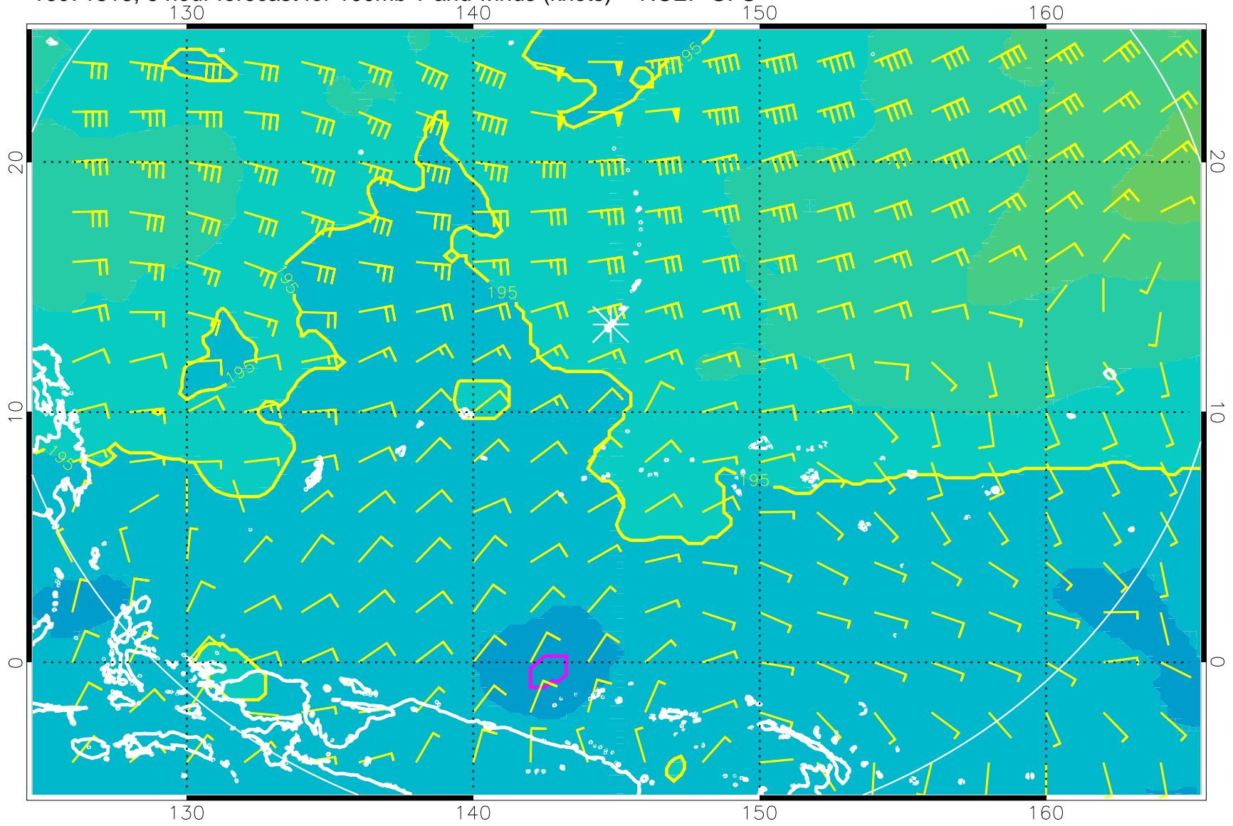
16071818, 6 hour forecast for 100mb T and winds (knots) -- NCEP GFS
