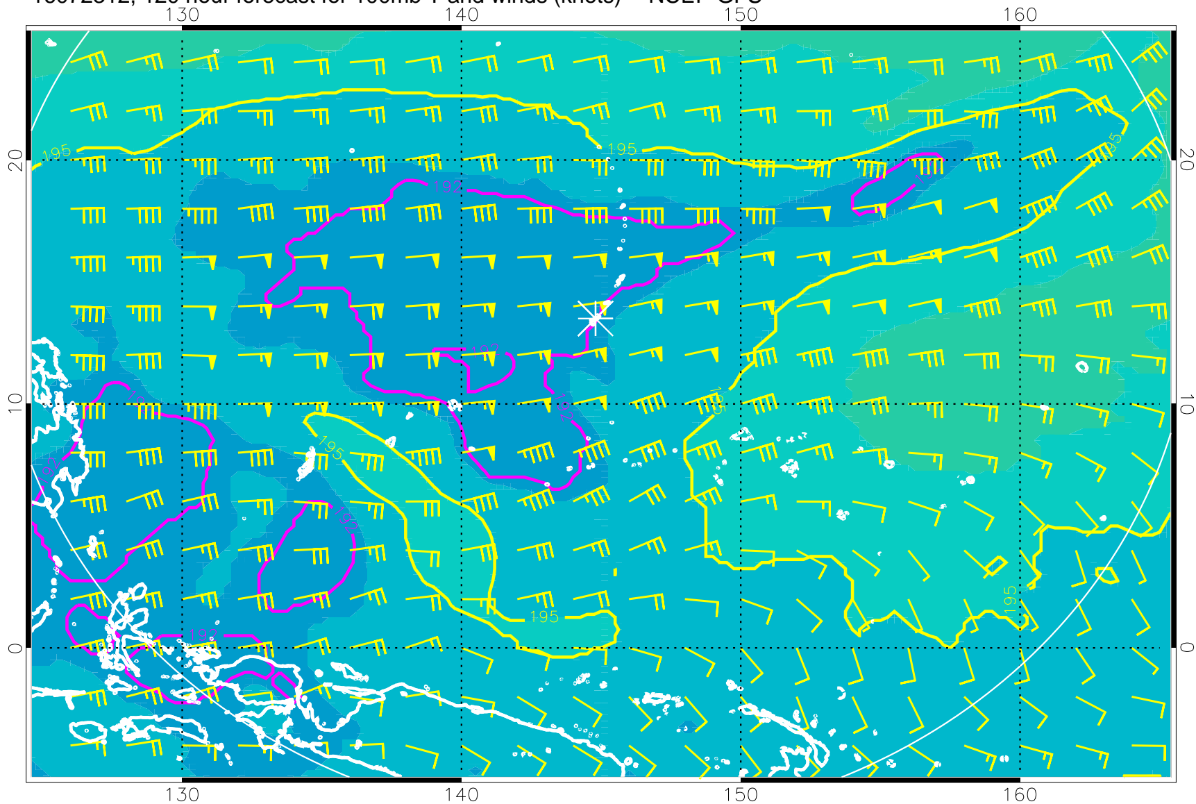
16072312, 120 hour forecast for 100mb T and winds (knots) -- NCEP GFS
