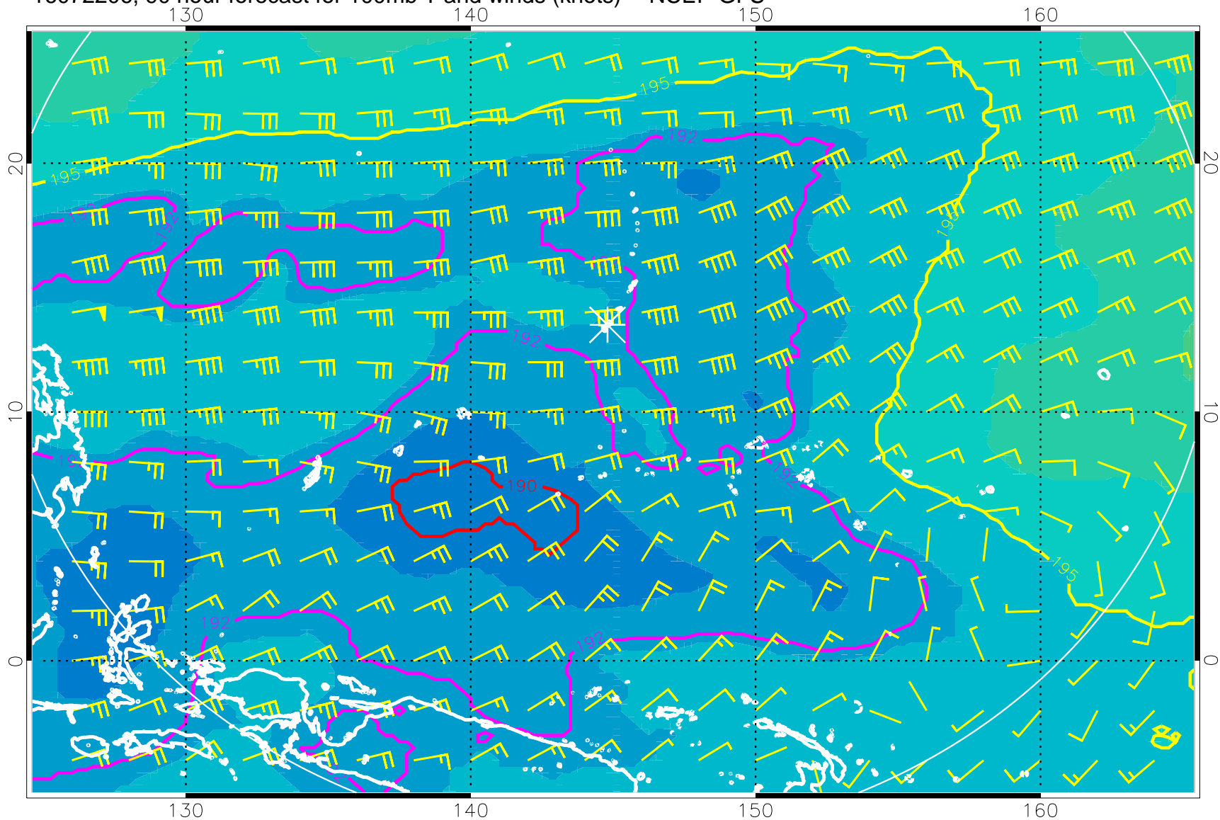
16072206, 90 hour forecast for 100mb T and winds (knots) -- NCEP GFS
