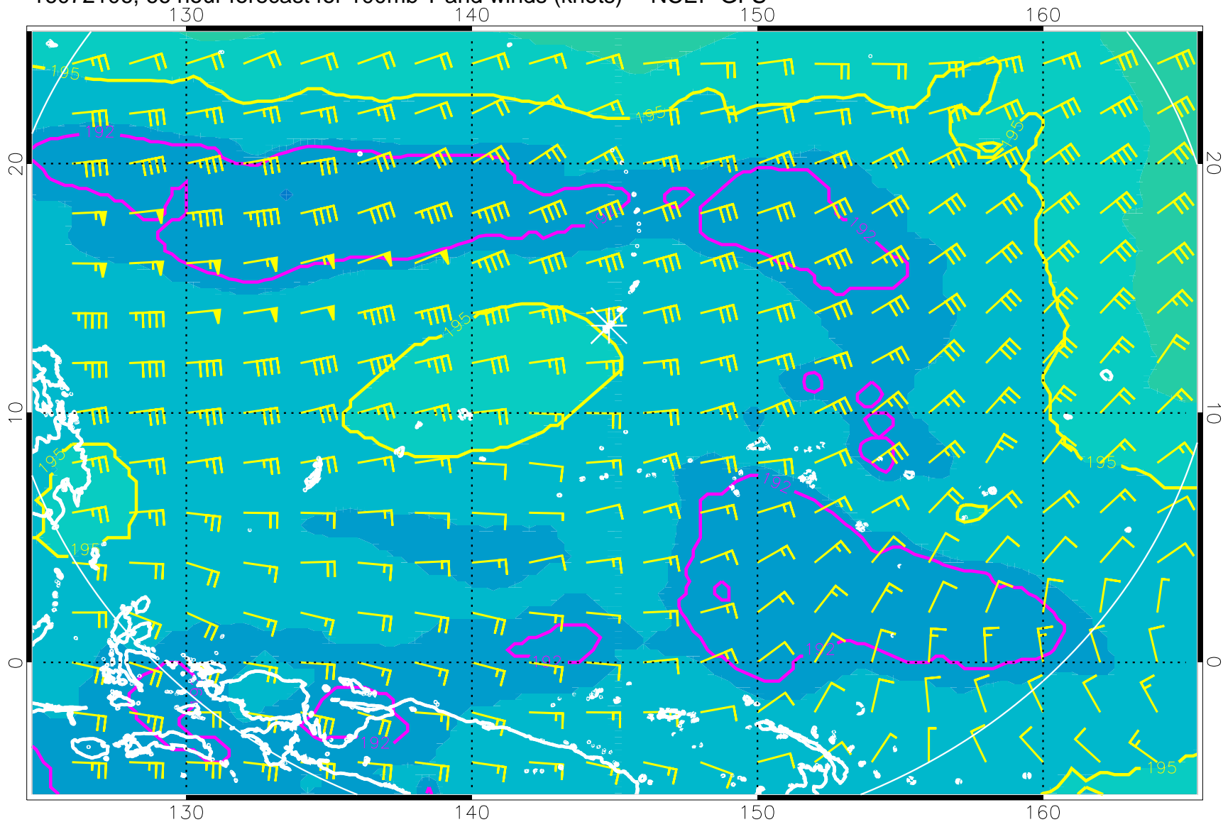
16072106, 66 hour forecast for 100mb T and winds (knots) -- NCEP GFS
