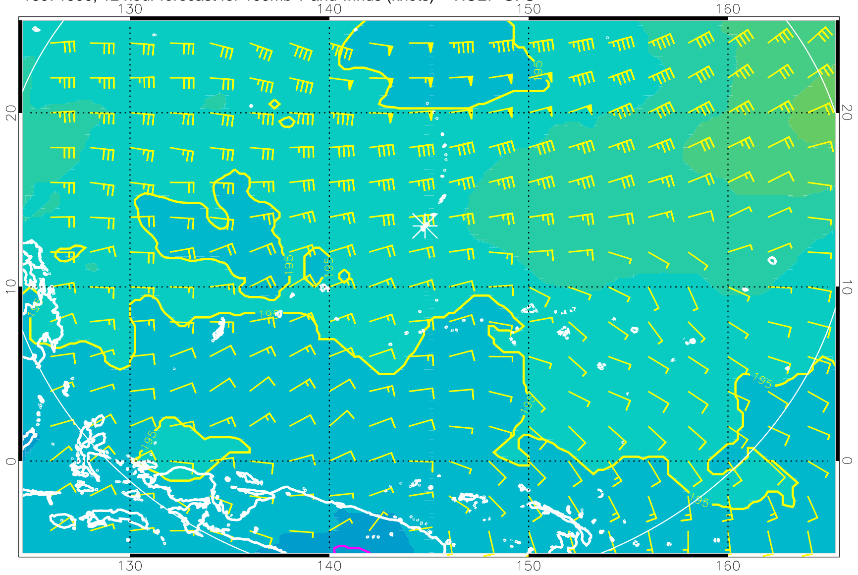
16071900, 12 hour forecast for 100mb T and winds (knots) -- NCEP GFS
