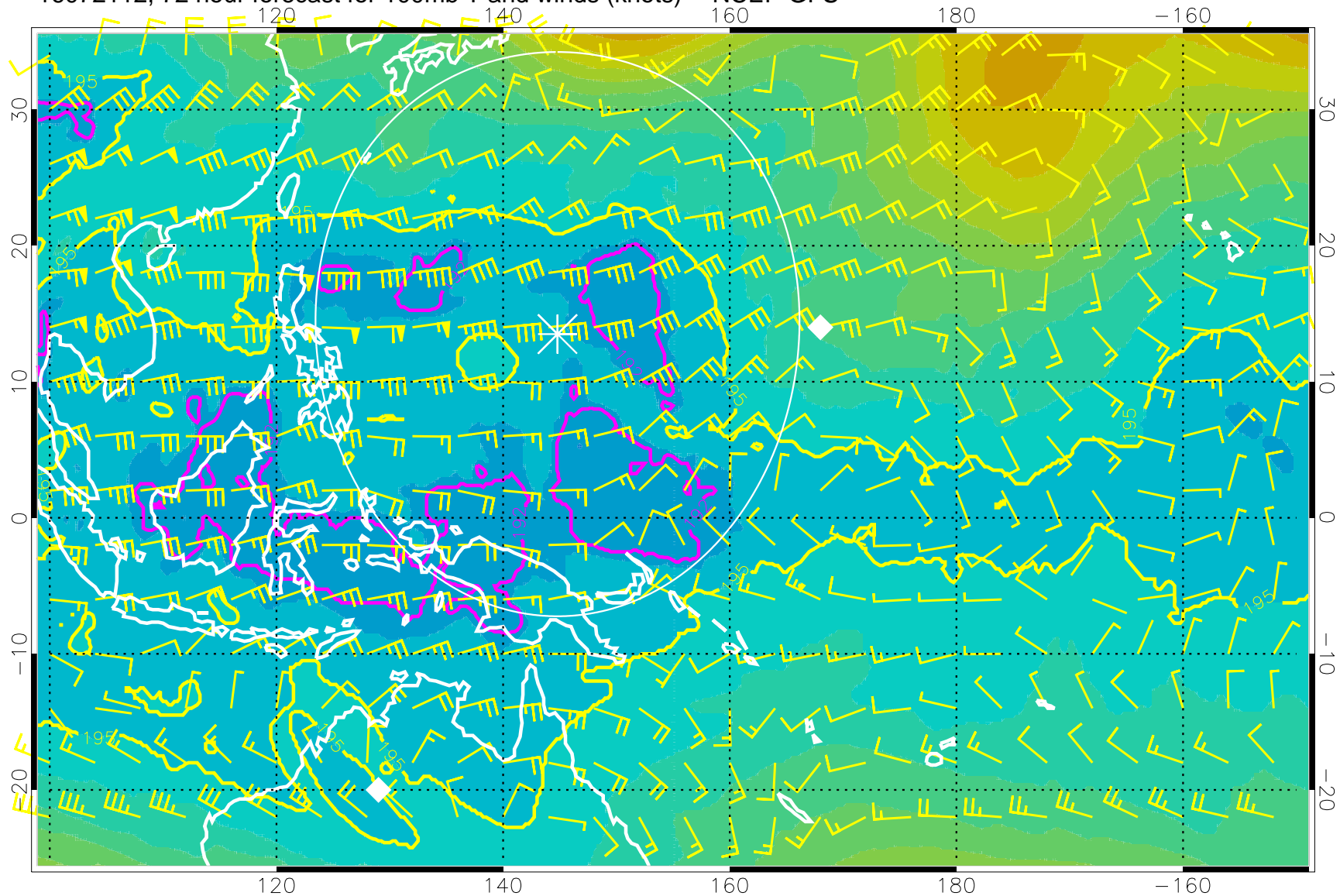
16072112, 72 hour forecast for 100mb T and winds (knots) -- NCEP GFS
