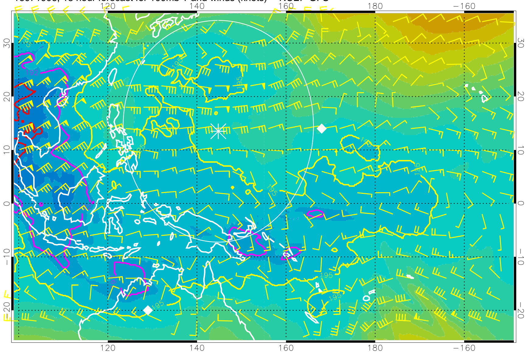
16071906, 18 hour forecast for 100mb T and winds (knots) -- NCEP GFS
