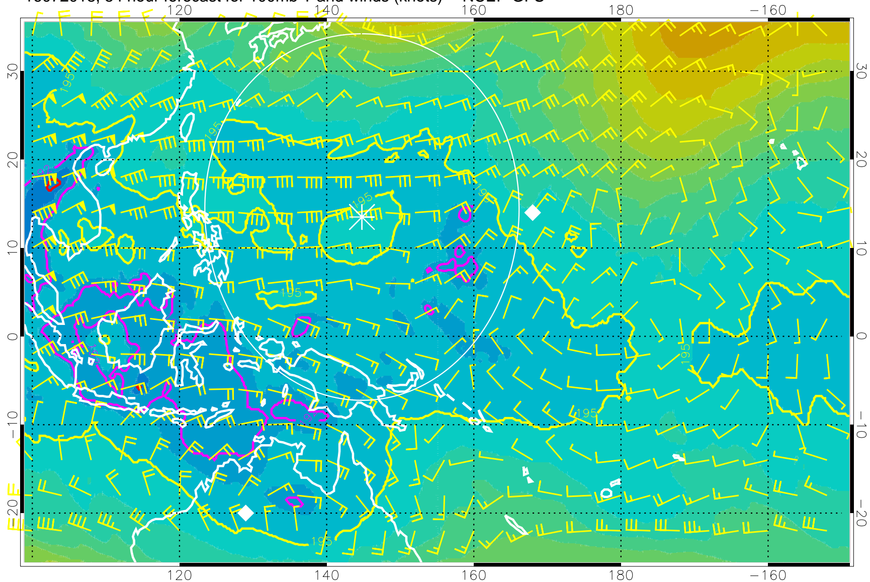
16072018, 54 hour forecast for 100mb T and winds (knots) -- NCEP GFS
