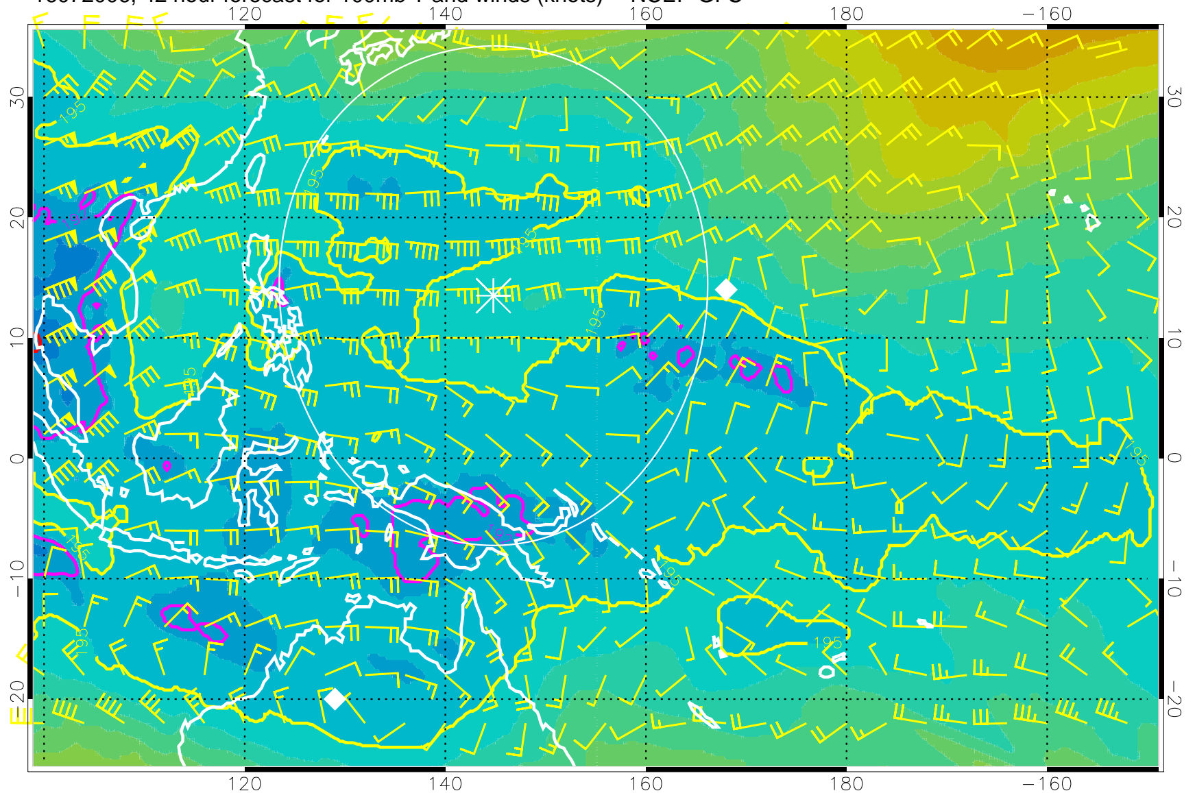
16072006, 42 hour forecast for 100mb T and winds (knots) -- NCEP GFS
