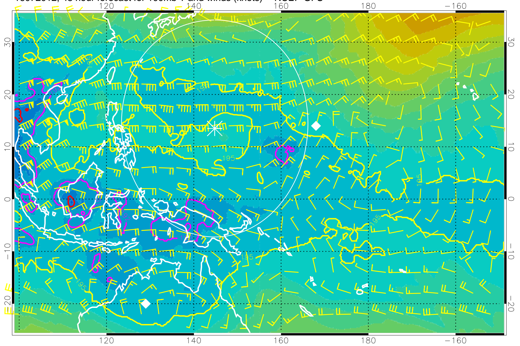
16072012, 48 hour forecast for 100mb T and winds (knots) -- NCEP GFS
