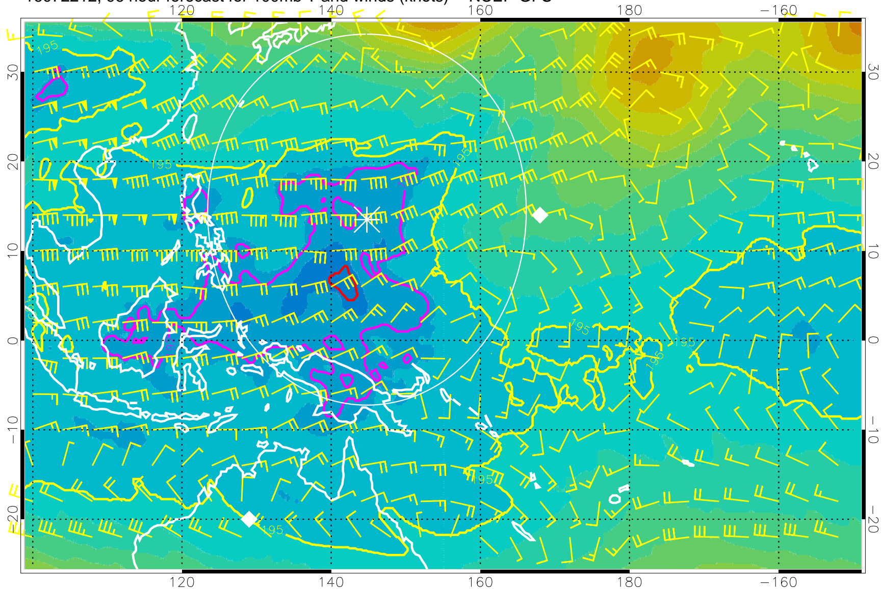
16072212, 96 hour forecast for 100mb T and winds (knots) -- NCEP GFS
