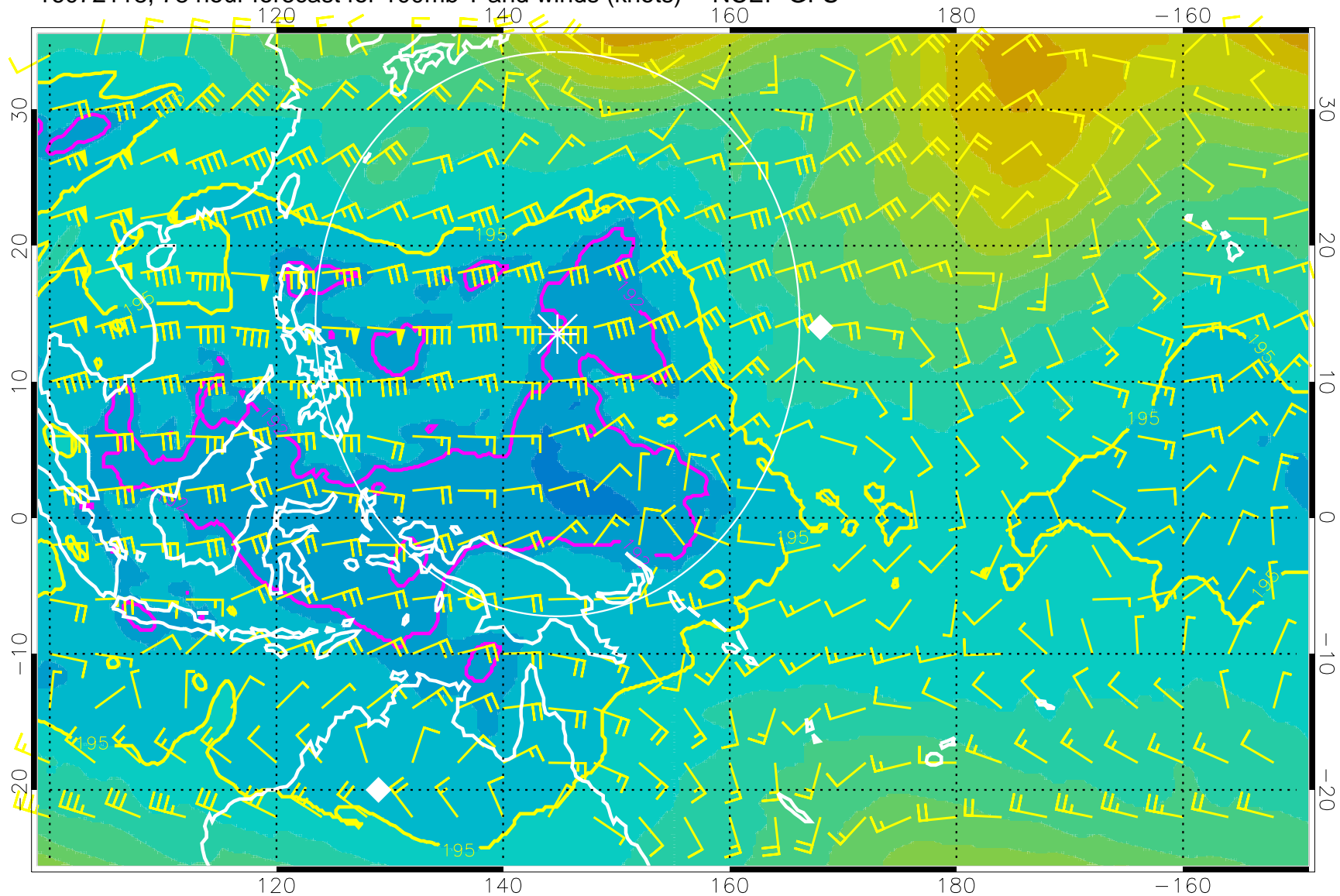
16072118, 78 hour forecast for 100mb T and winds (knots) -- NCEP GFS
