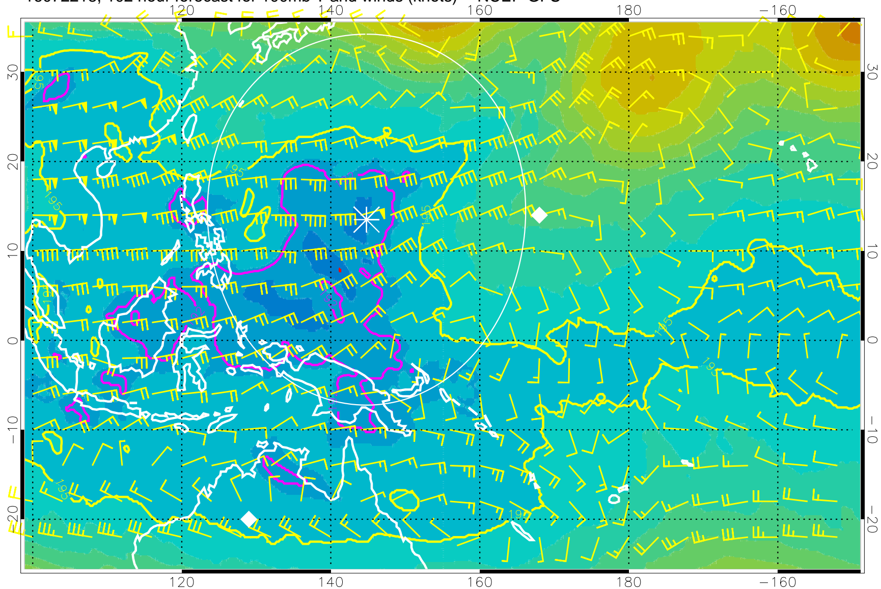
16072218, 102 hour forecast for 100mb T and winds (knots) -- NCEP GFS
