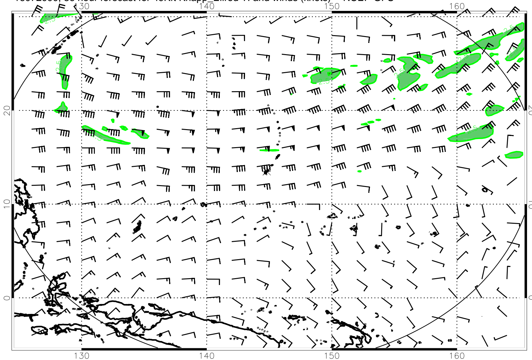
16072000, 36 hour forecast for 49Kft Knapp_Ellrod TI and winds (knots) -- NCEP GFS
