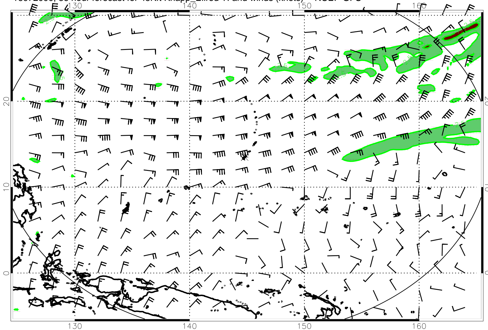
16072000, 36 hour forecast for 45Kft Knapp_Ellrod TI and winds (knots) -- NCEP GFS
