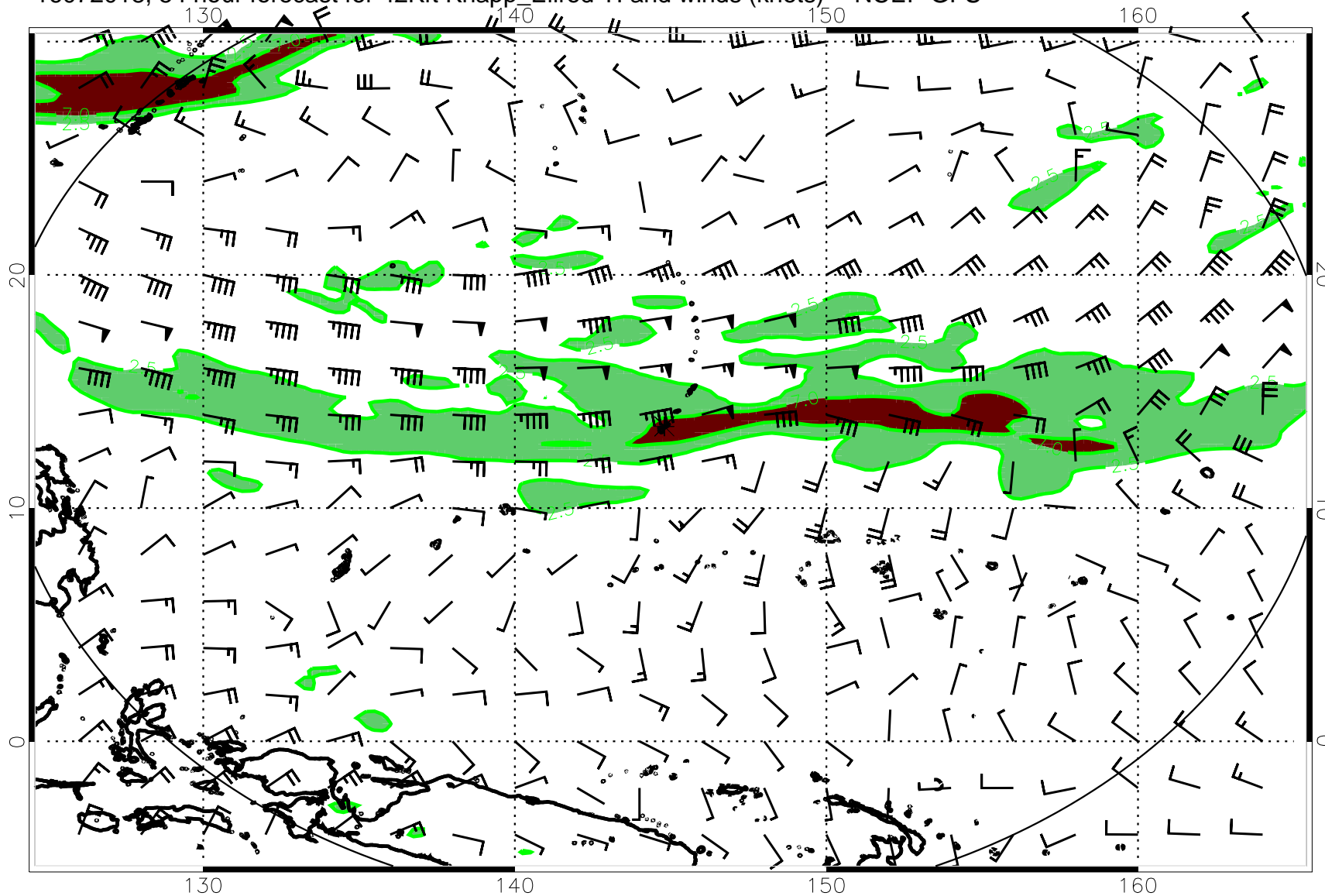
16072018, 54 hour forecast for 42Kft Knapp_Ellrod TI and winds (knots) -- NCEP GFS
