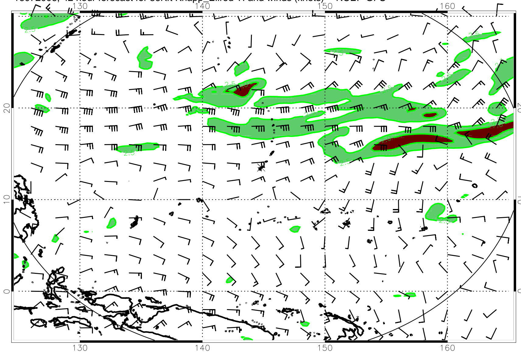
16072006, 42 hour forecast for 36Kft Knapp_Ellrod TI and winds (knots) -- NCEP GFS
