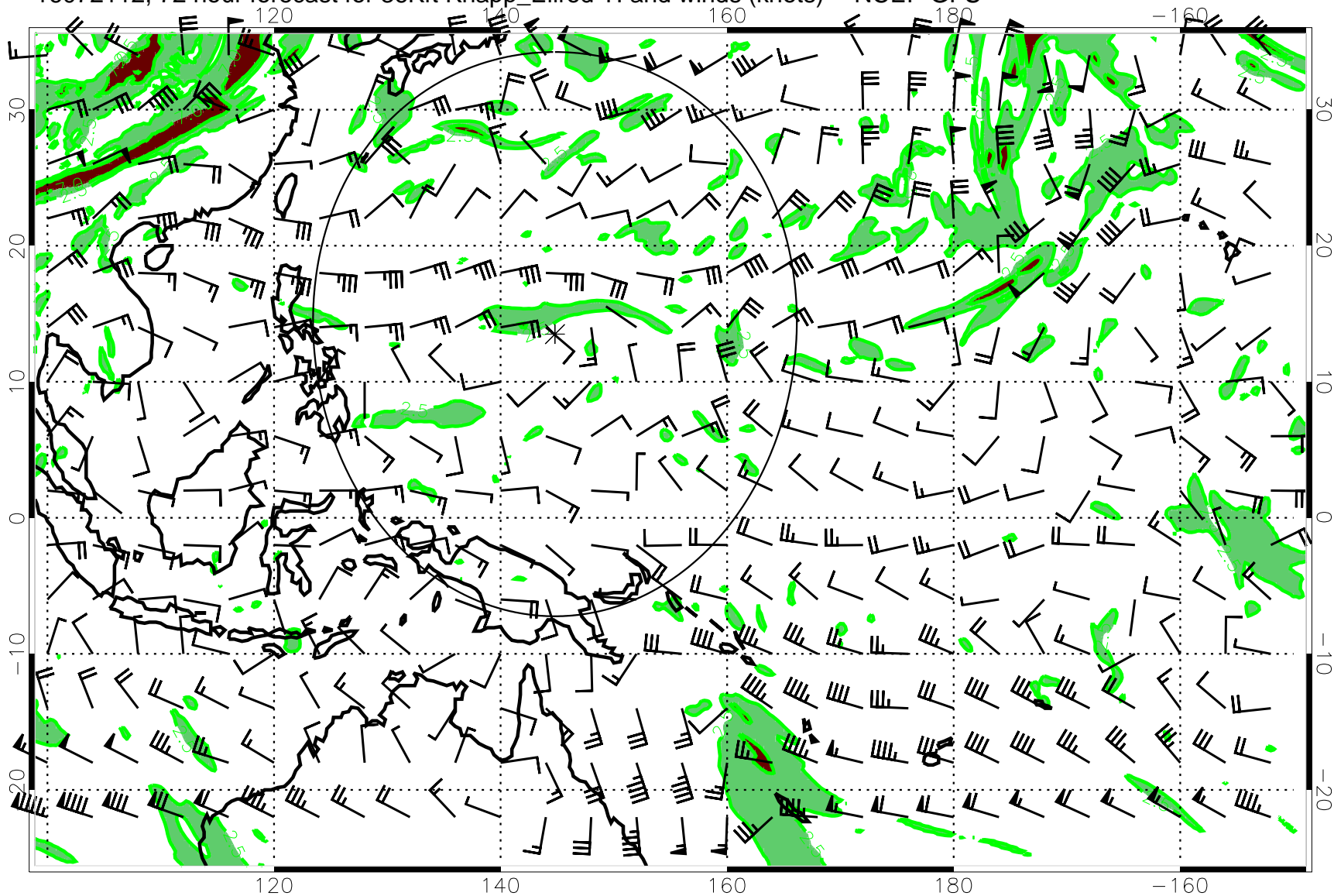
16072112, 72 hour forecast for 36Kft Knapp_Ellrod TI and winds (knots) -- NCEP GFS
