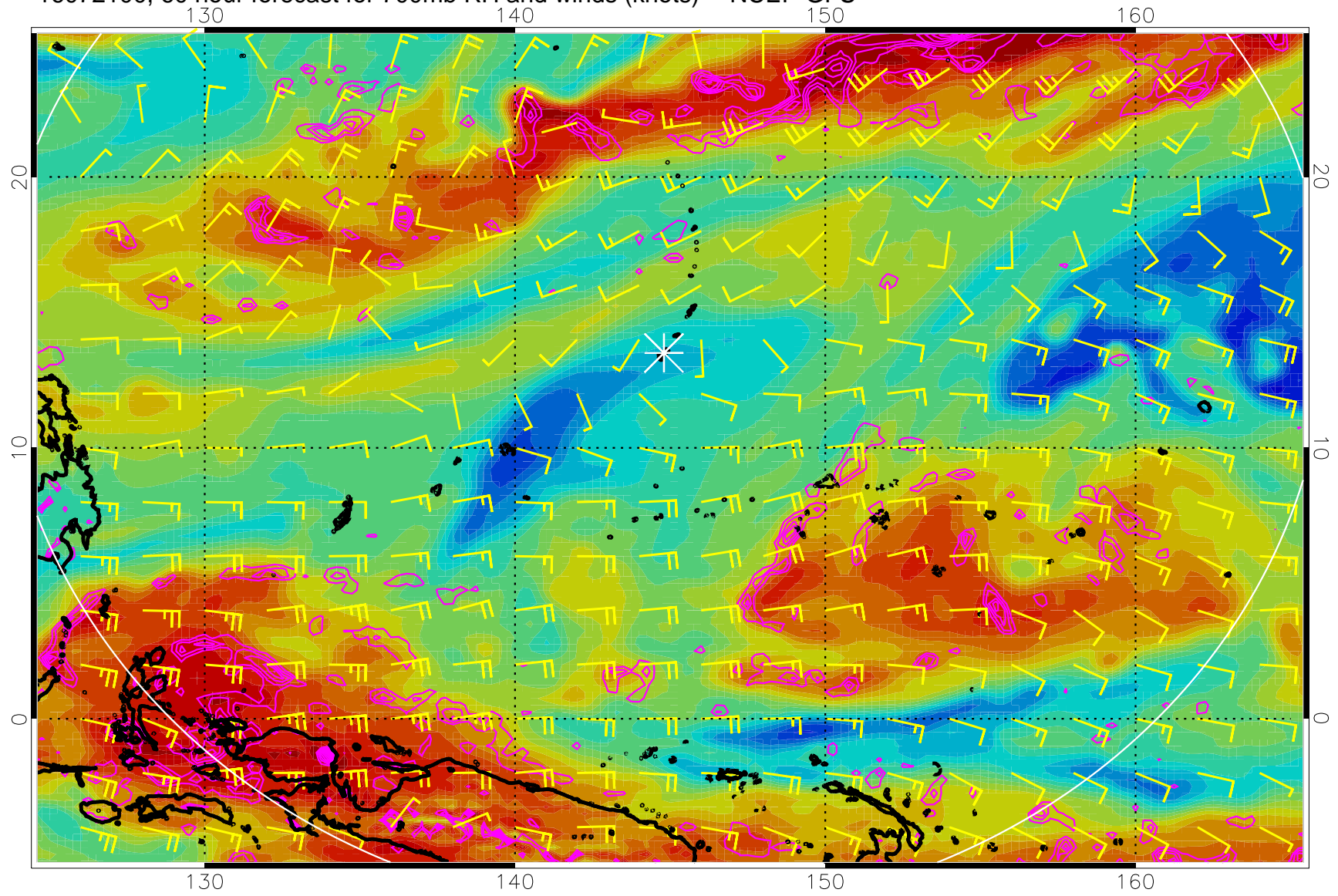
16072100, 60 hour forecast for 700mb RH and winds (knots) -- NCEP GFS
