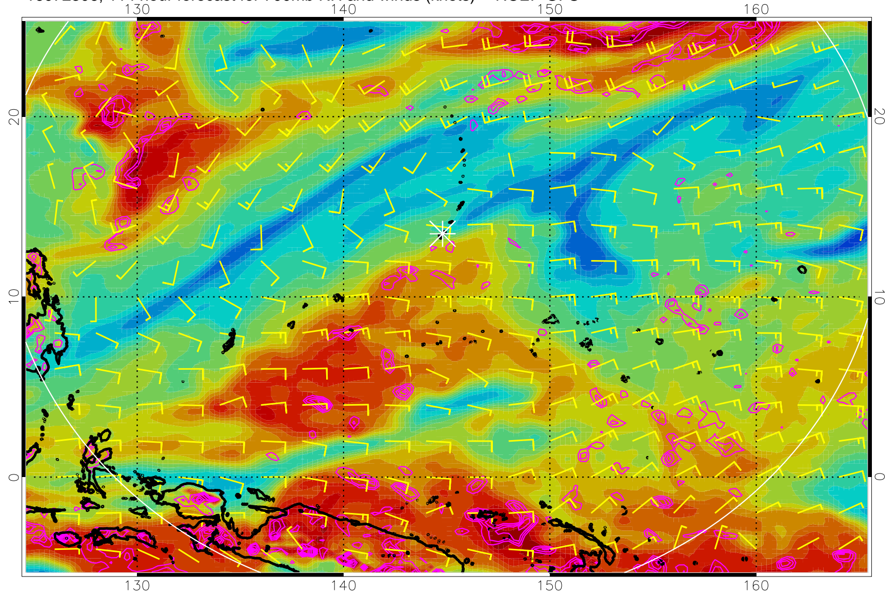
16072306, 114 hour forecast for 700mb RH and winds (knots) -- NCEP GFS
