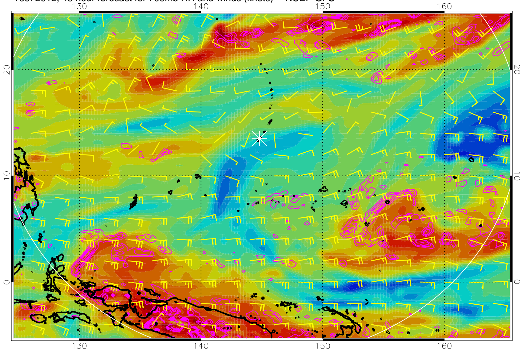
16072012, 48 hour forecast for 700mb RH and winds (knots) -- NCEP GFS
