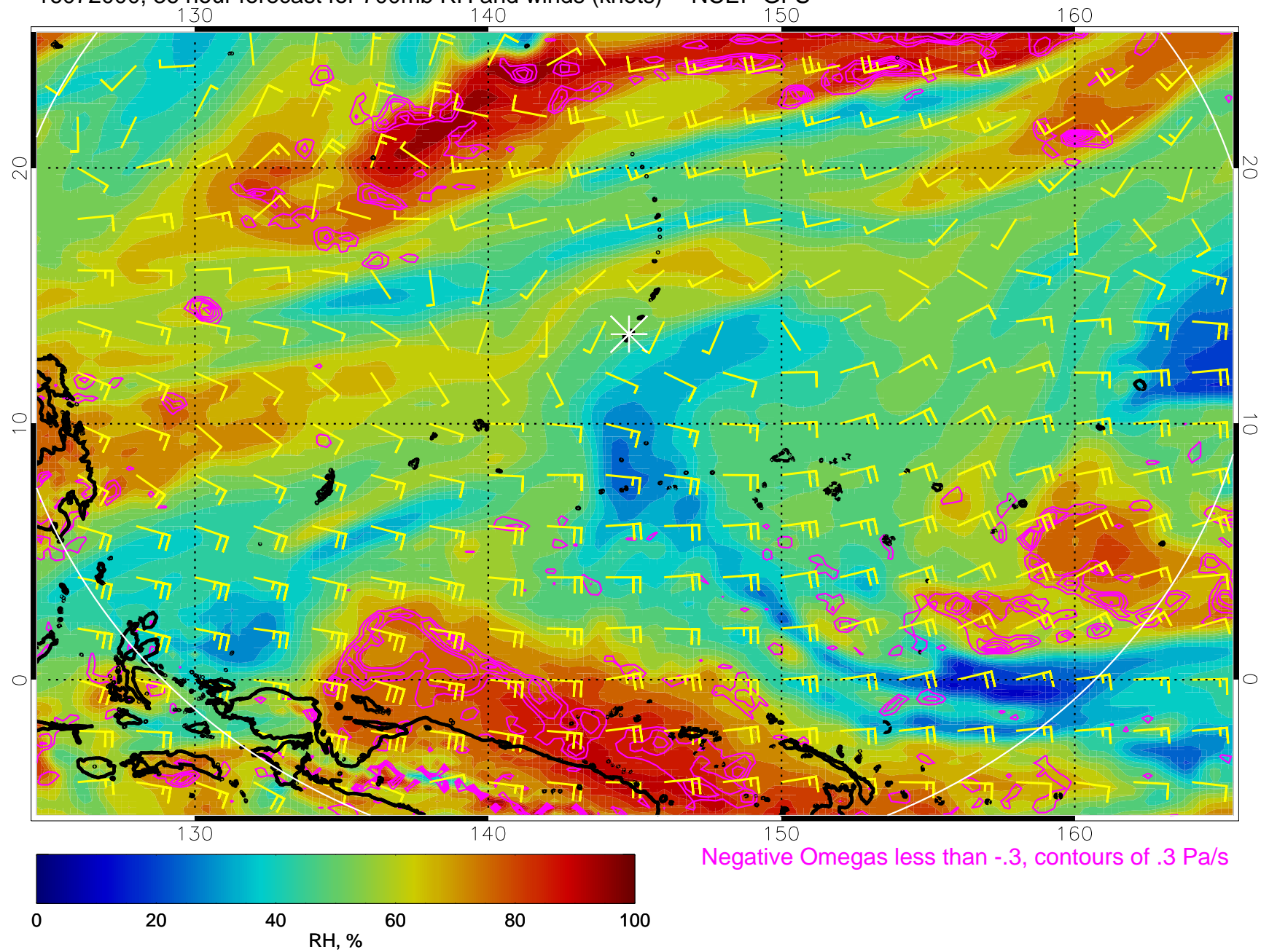
16072000, 36 hour forecast for 700mb RH and winds (knots) -- NCEP GFS
