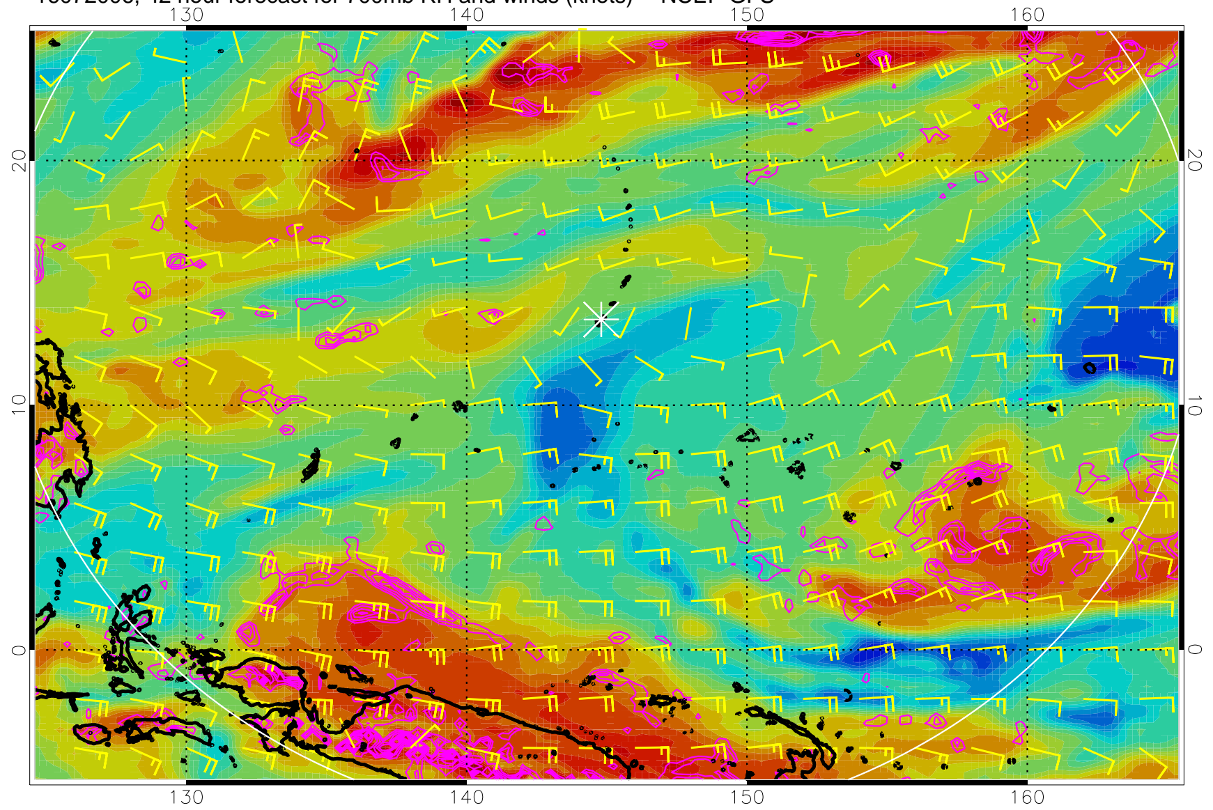
16072006, 42 hour forecast for 700mb RH and winds (knots) -- NCEP GFS
