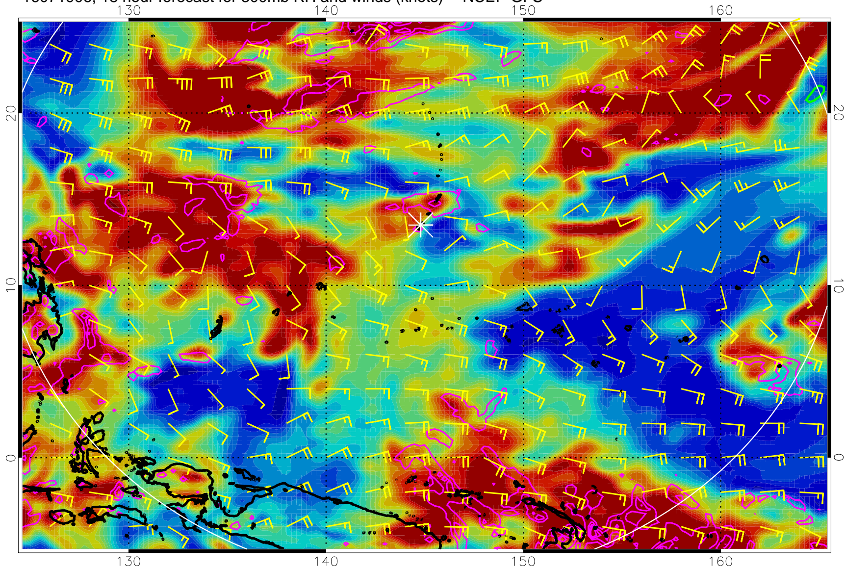
16071906, 18 hour forecast for 300mb RH and winds (knots) -- NCEP GFS
