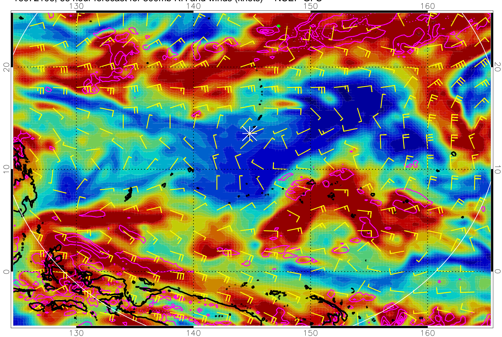
16072106, 66 hour forecast for 300mb RH and winds (knots) -- NCEP GFS
