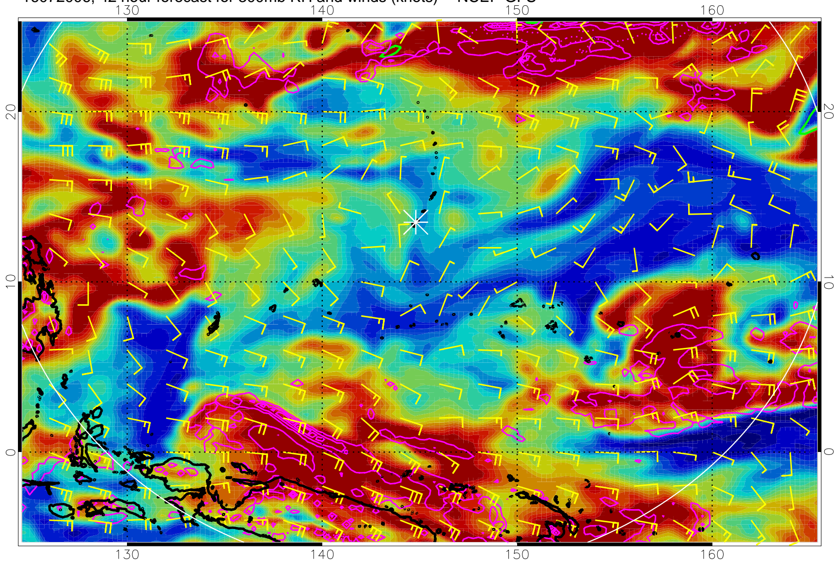
16072006, 42 hour forecast for 300mb RH and winds (knots) -- NCEP GFS
