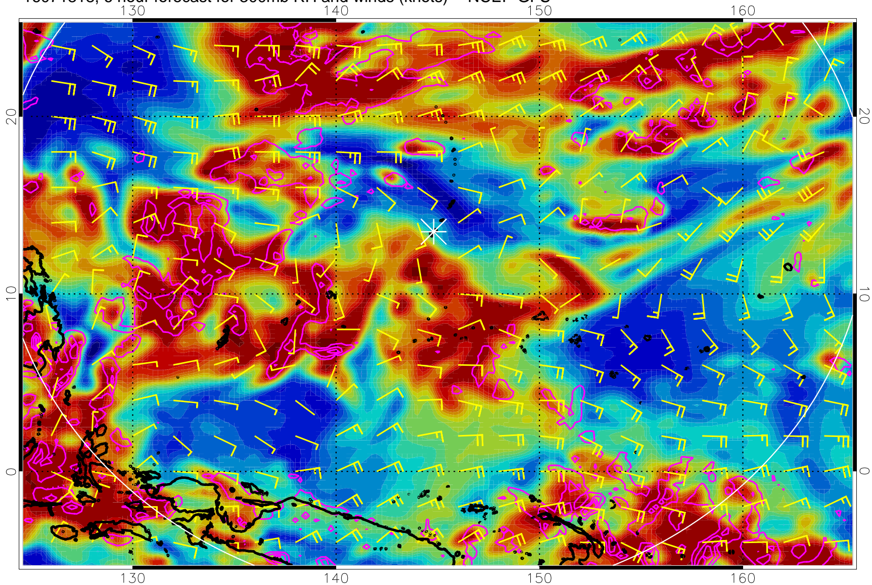
16071818, 6 hour forecast for 300mb RH and winds (knots) -- NCEP GFS
