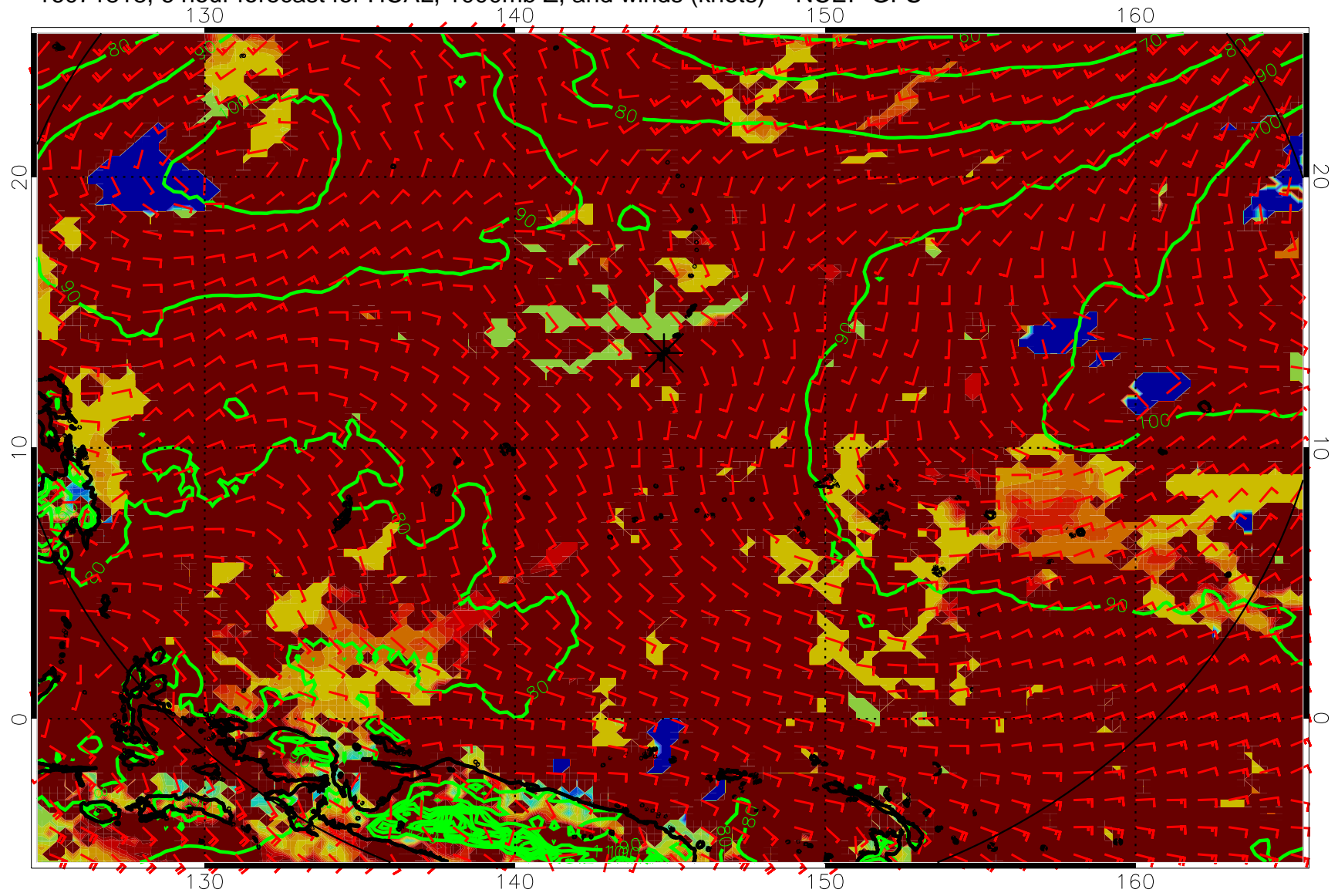
16071818, 6 hour forecast for HCAL, 1000mb Z, and winds (knots) -- NCEP GFS
