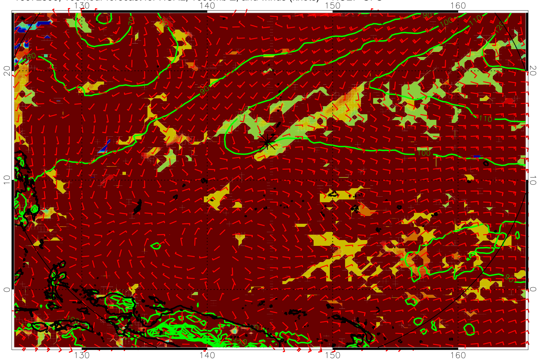
16072300, 108 hour forecast for HCAL, 1000mb Z, and winds (knots) -- NCEP GFS
