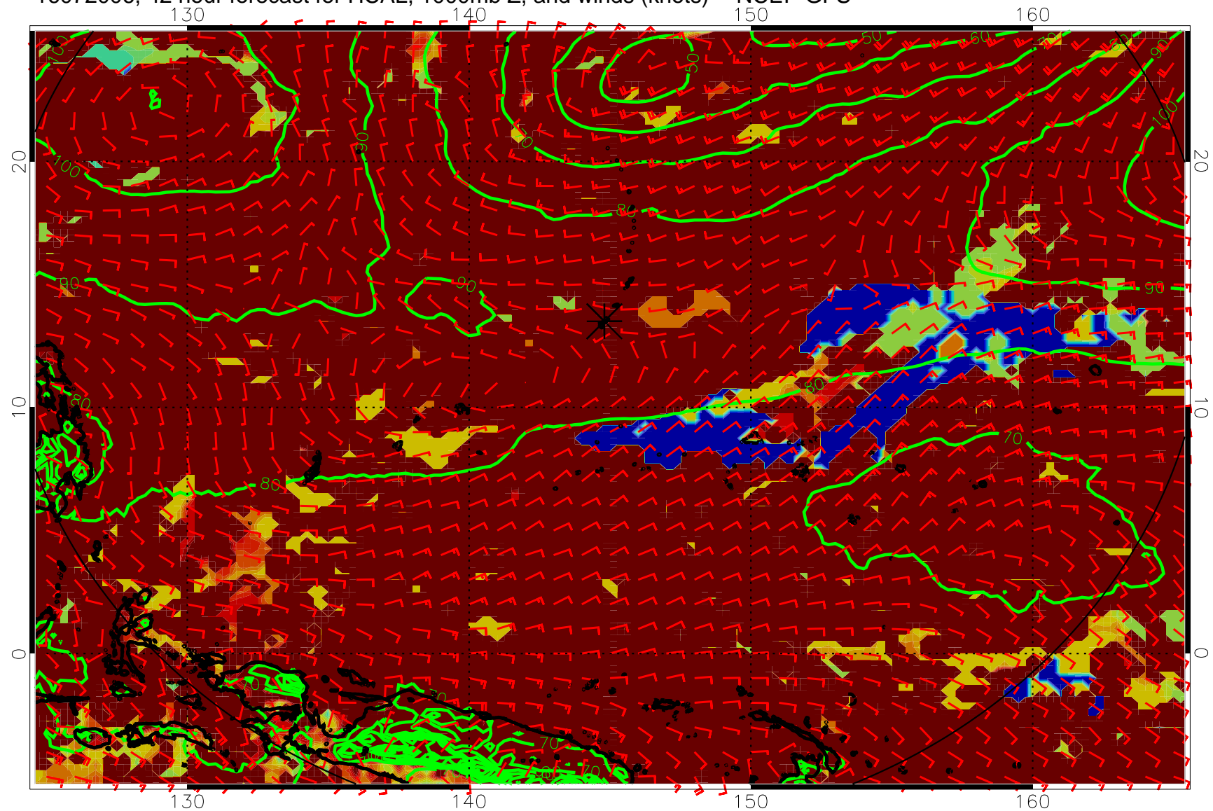
16072006, 42 hour forecast for HCAL, 1000mb Z, and winds (knots) -- NCEP GFS
