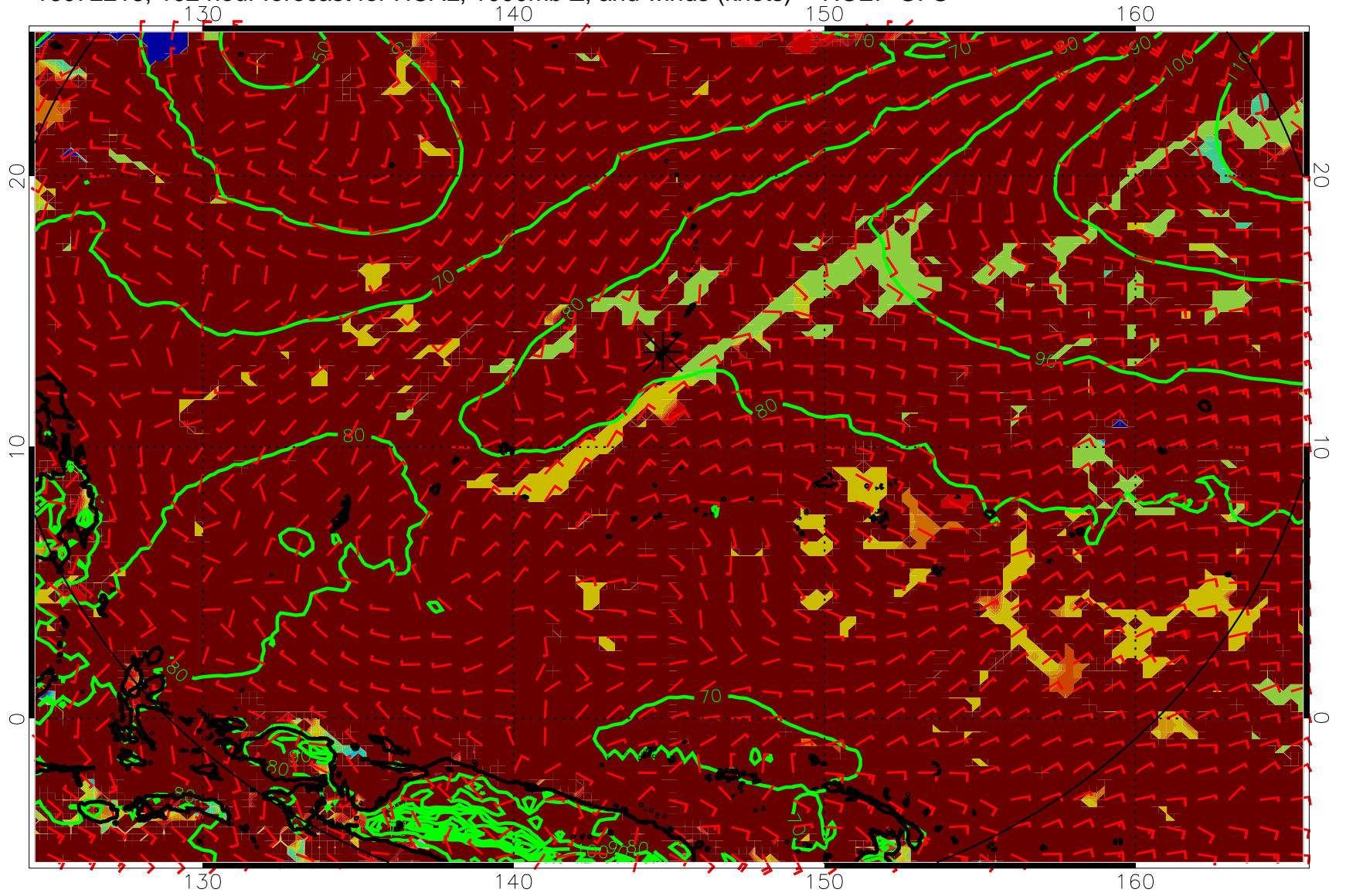
16072218, 102 hour forecast for HCAL, 1000mb Z, and winds (knots) -- NCEP GFS
