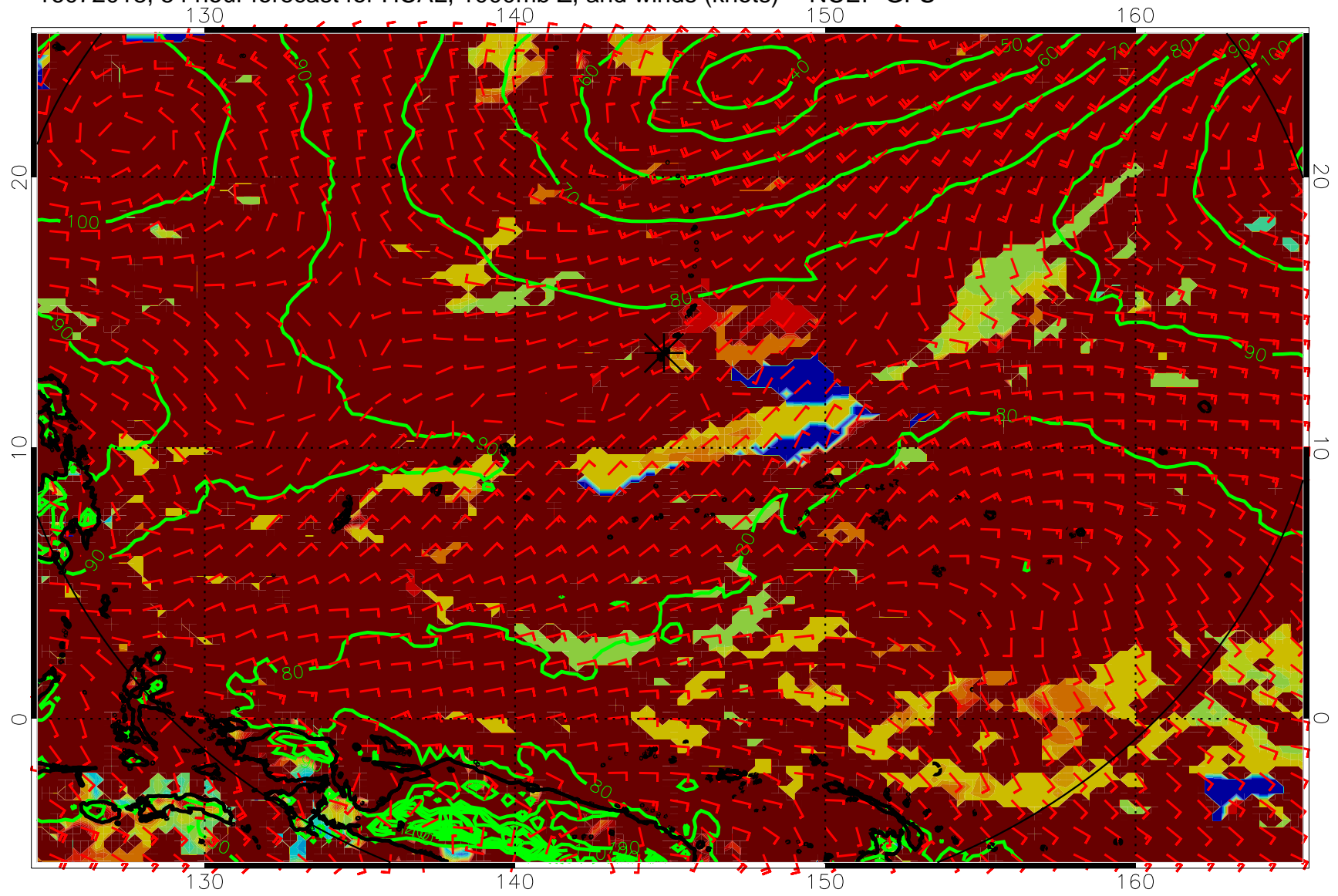
16072018, 54 hour forecast for HCAL, 1000mb Z, and winds (knots) -- NCEP GFS
