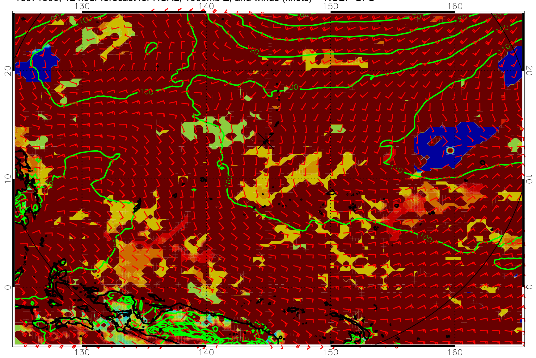
16071900, 12 hour forecast for HCAL, 1000mb Z, and winds (knots) -- NCEP GFS
