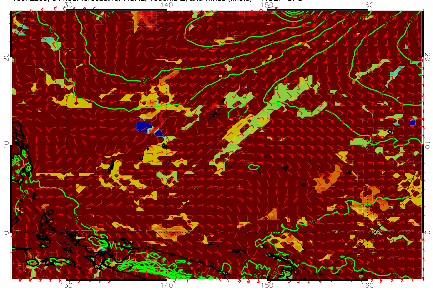
16072200, 84 hour forecast for HCAL, 1000mb Z, and winds (knots) -- NCEP GFS
