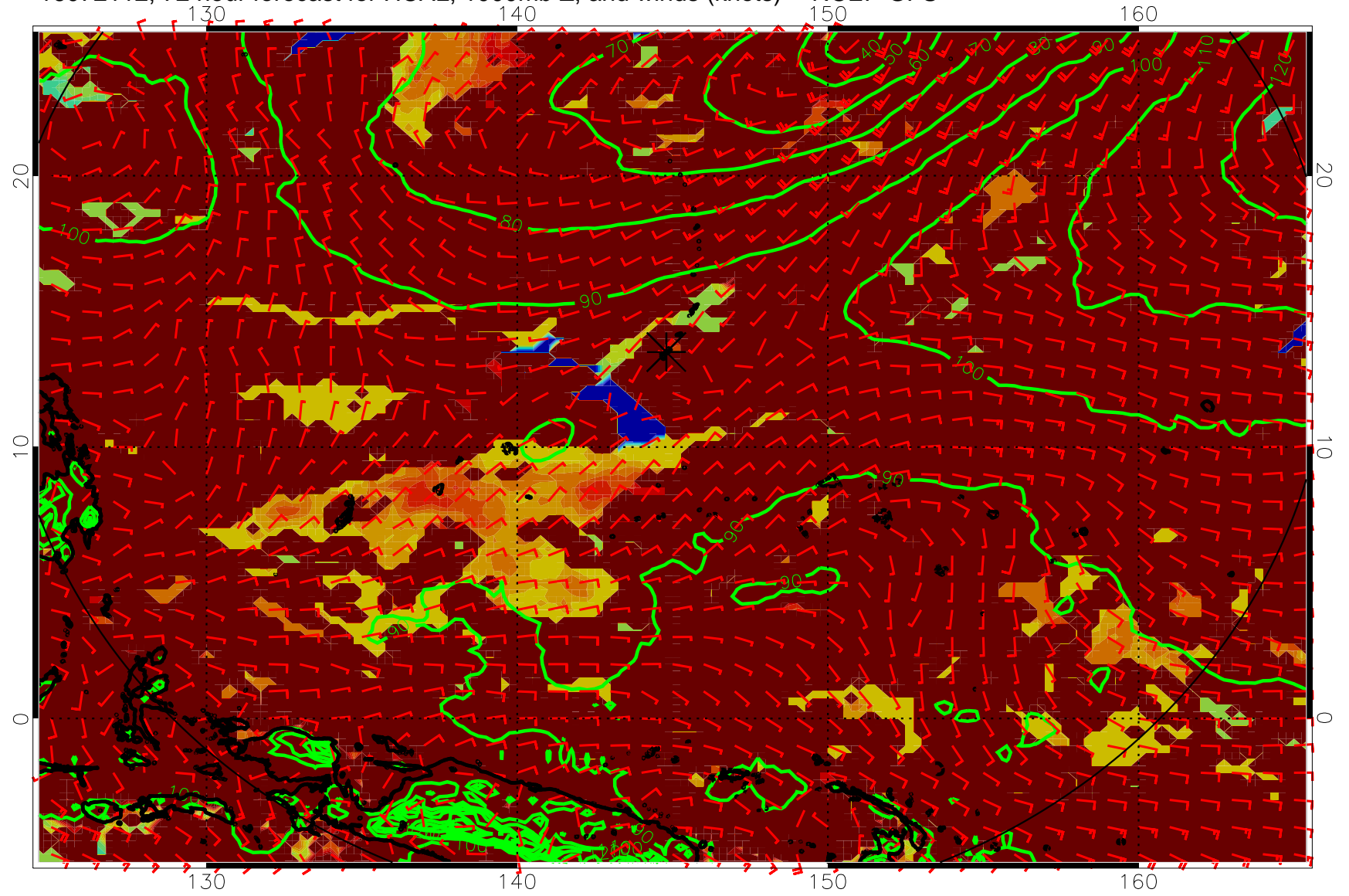
16072112, 72 hour forecast for HCAL, 1000mb Z, and winds (knots) -- NCEP GFS
