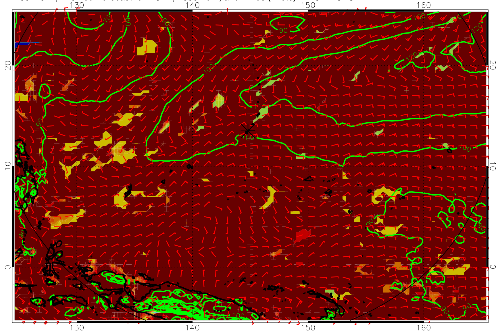
16072312, 120 hour forecast for HCAL, 1000mb Z, and winds (knots) -- NCEP GFS
