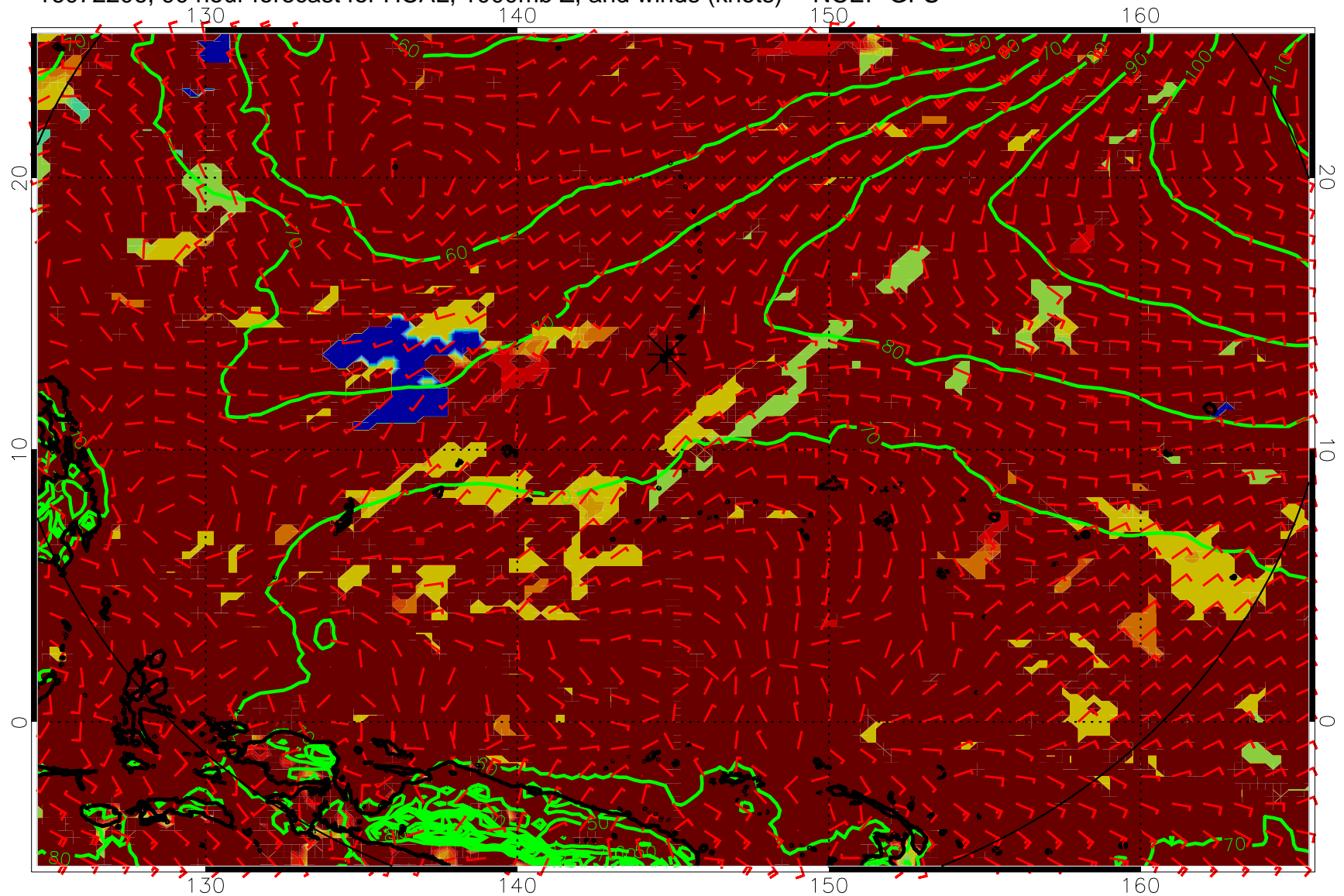
16072206, 90 hour forecast for HCAL, 1000mb Z, and winds (knots) -- NCEP GFS
