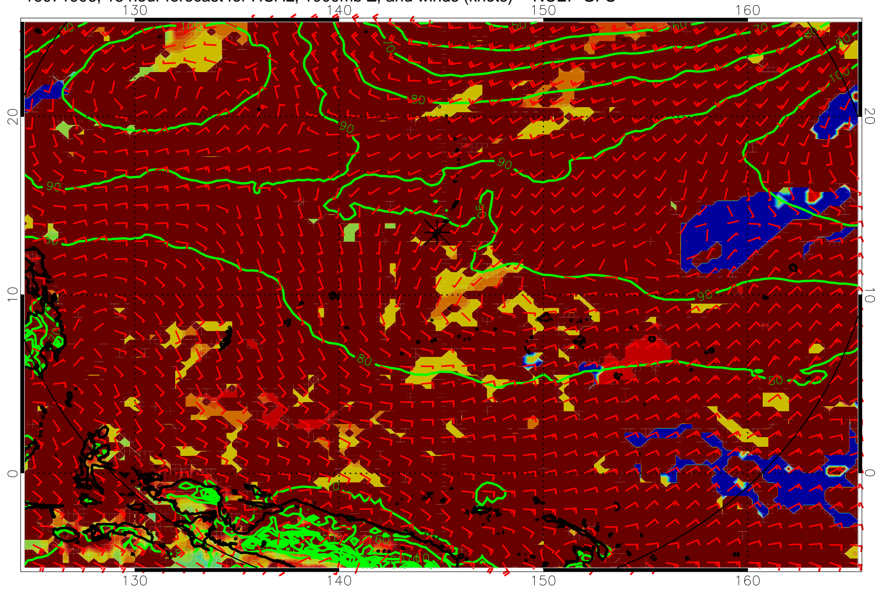
16071906, 18 hour forecast for HCAL, 1000mb Z, and winds (knots) -- NCEP GFS
