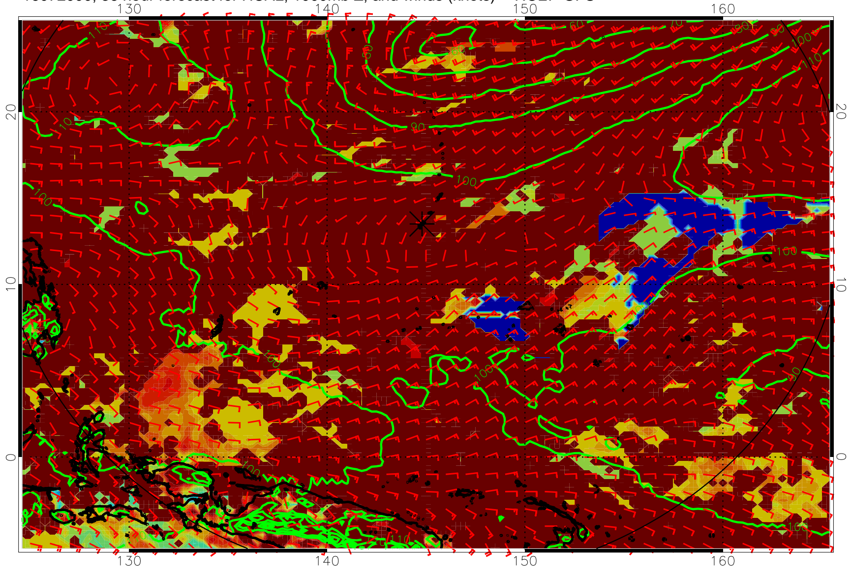
16072000, 36 hour forecast for HCAL, 1000mb Z, and winds (knots) -- NCEP GFS
