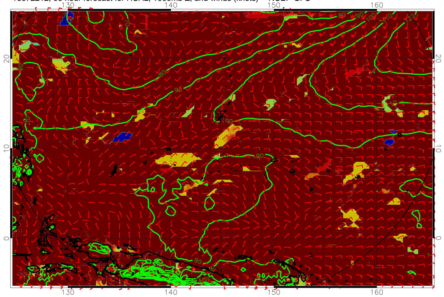
16072212, 96 hour forecast for HCAL, 1000mb Z, and winds (knots) -- NCEP GFS
