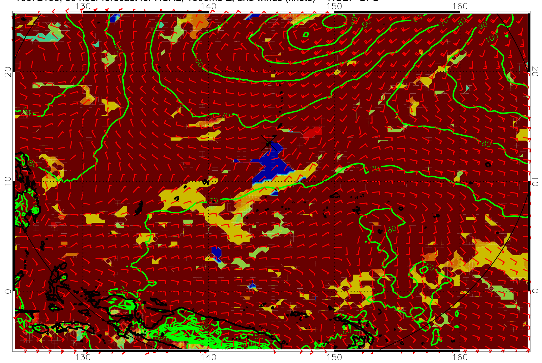
16072106, 66 hour forecast for HCAL, 1000mb Z, and winds (knots) -- NCEP GFS
