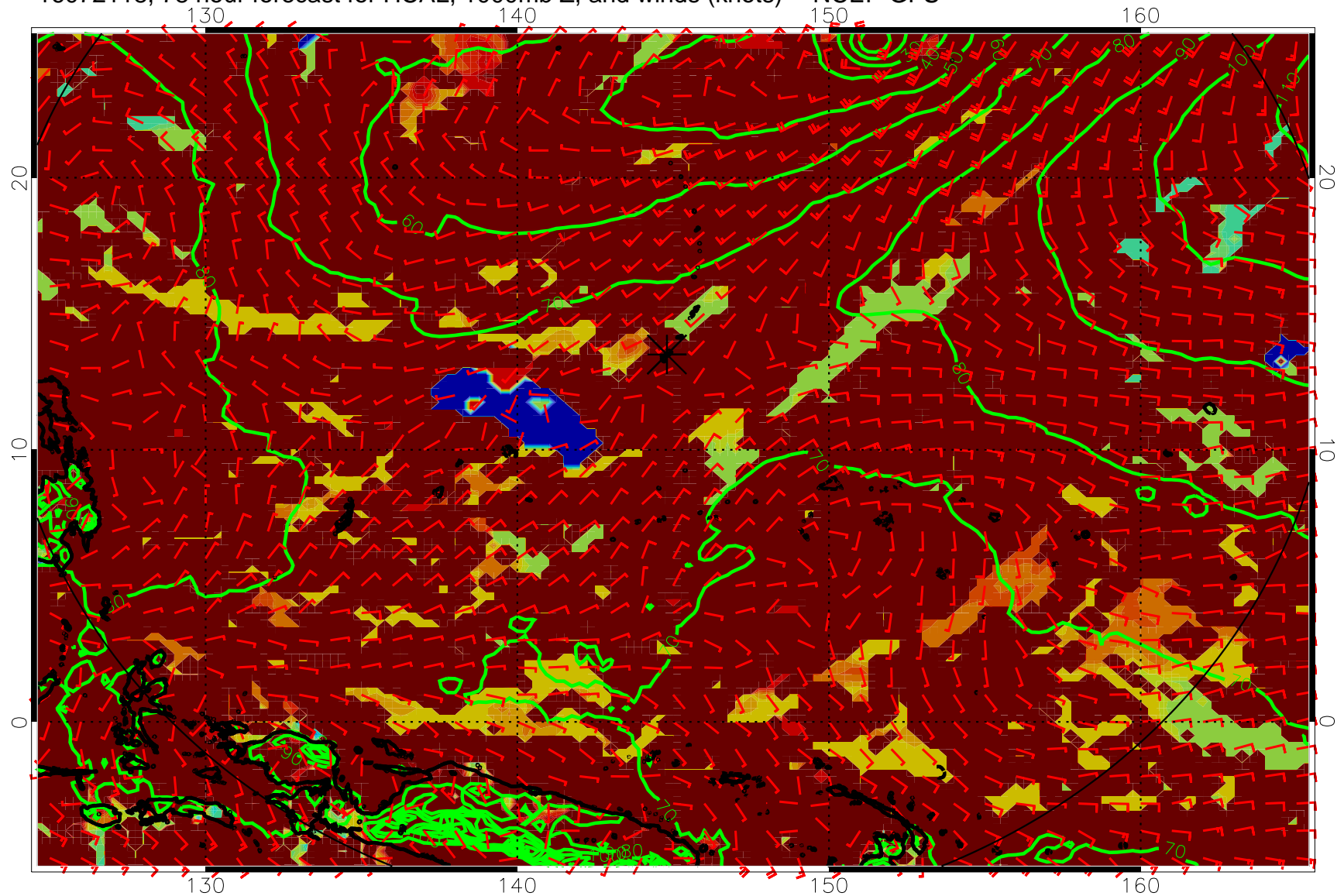
16072118, 78 hour forecast for HCAL, 1000mb Z, and winds (knots) -- NCEP GFS
