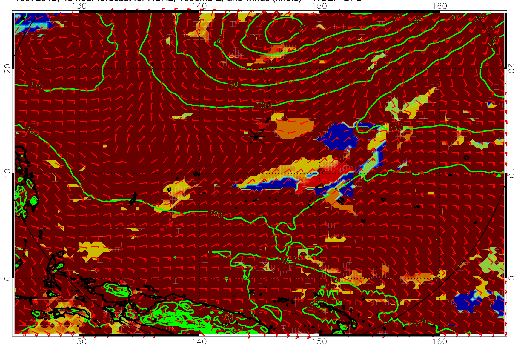
16072012, 48 hour forecast for HCAL, 1000mb Z, and winds (knots) -- NCEP GFS
