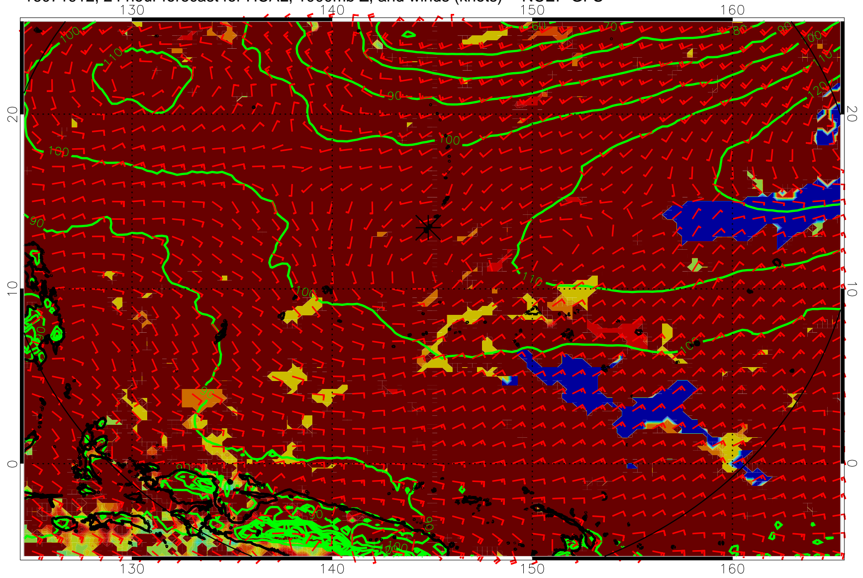
16071912, 24 hour forecast for HCAL, 1000mb Z, and winds (knots) -- NCEP GFS
