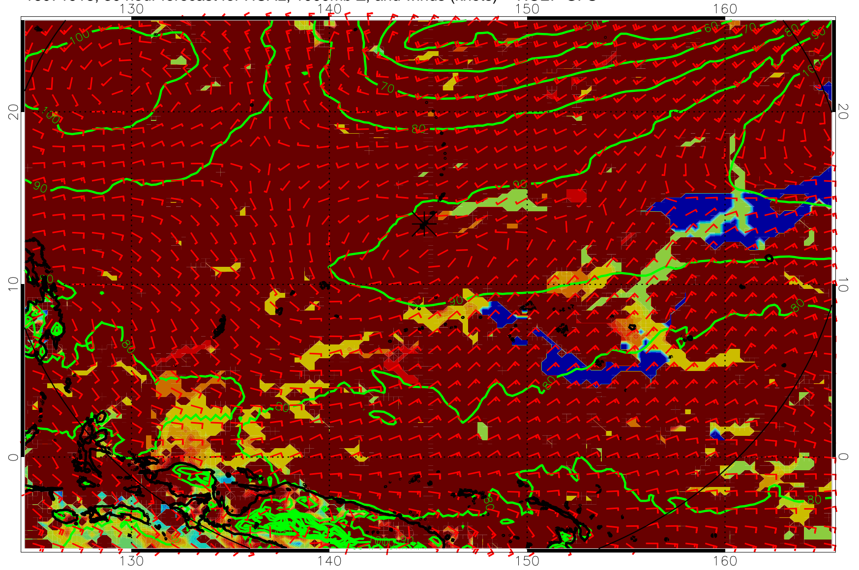
16071918, 30 hour forecast for HCAL, 1000mb Z, and winds (knots) -- NCEP GFS
