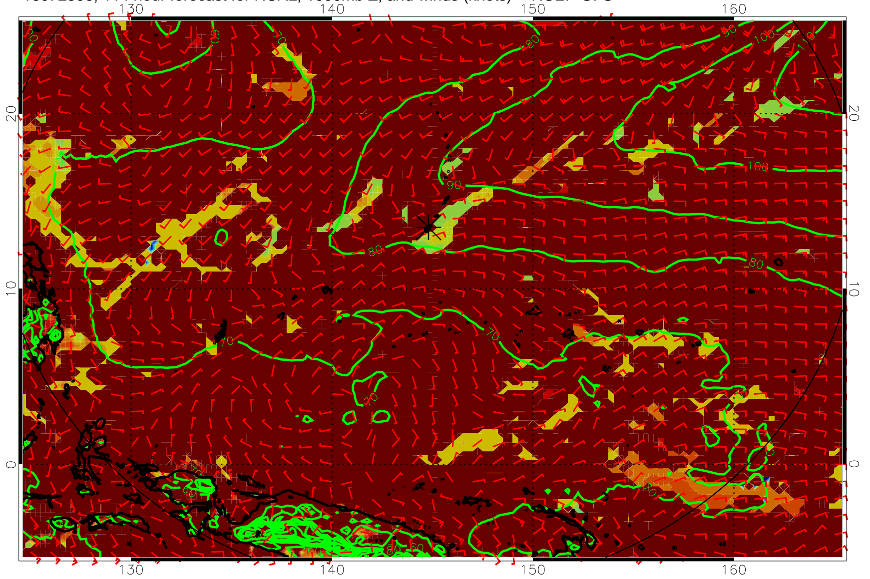
16072306, 114 hour forecast for HCAL, 1000mb Z, and winds (knots) -- NCEP GFS
