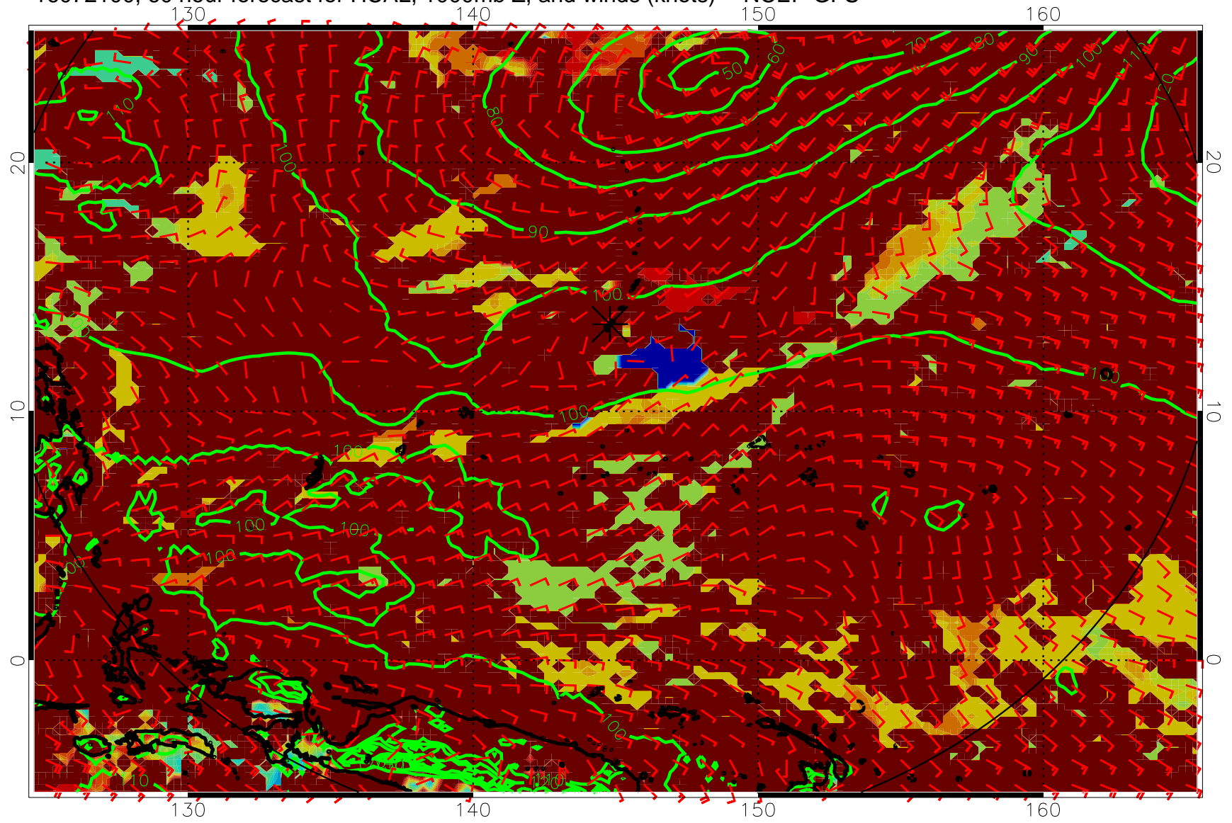
16072100, 60 hour forecast for HCAL, 1000mb Z, and winds (knots) -- NCEP GFS
