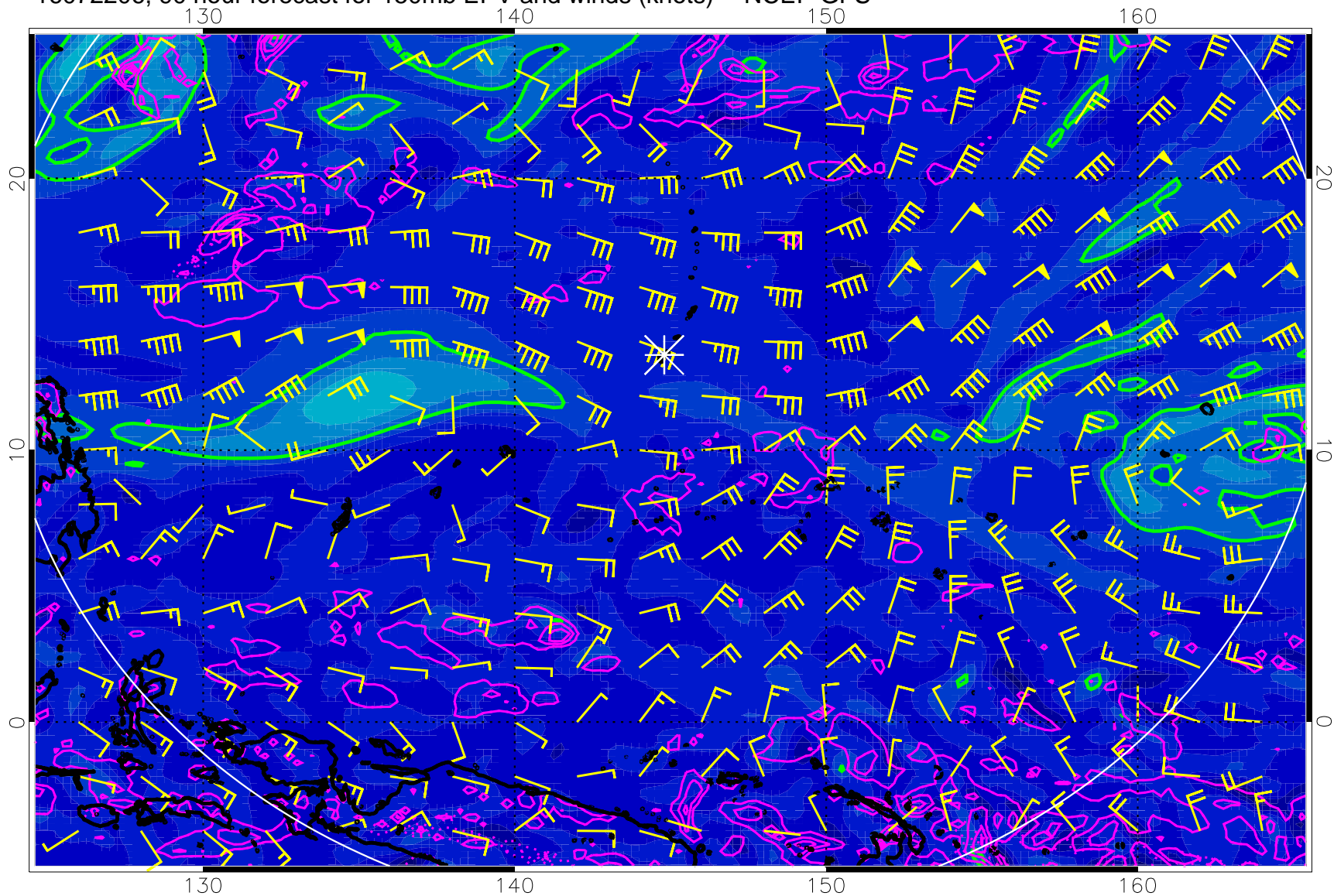
16072206, 90 hour forecast for 150mb EPV and winds (knots) -- NCEP GFS
