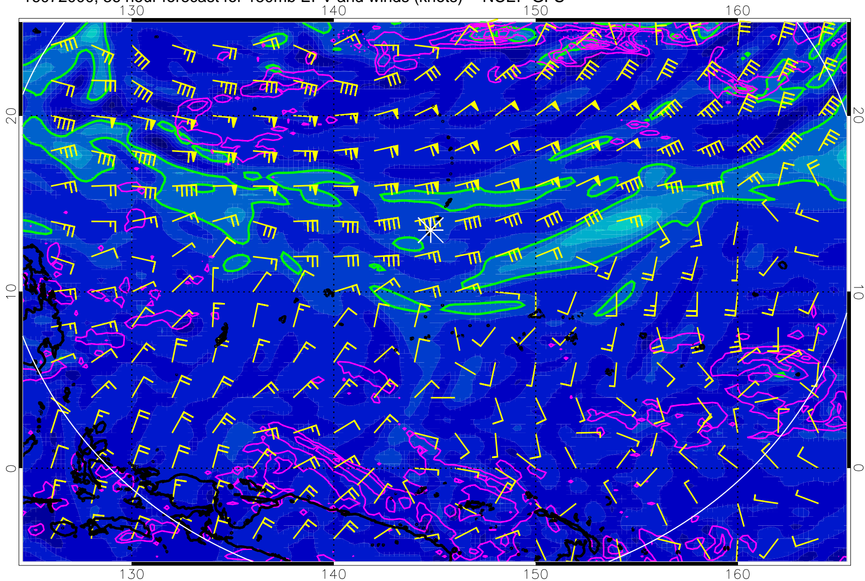
16072000, 36 hour forecast for 150mb EPV and winds (knots) -- NCEP GFS
