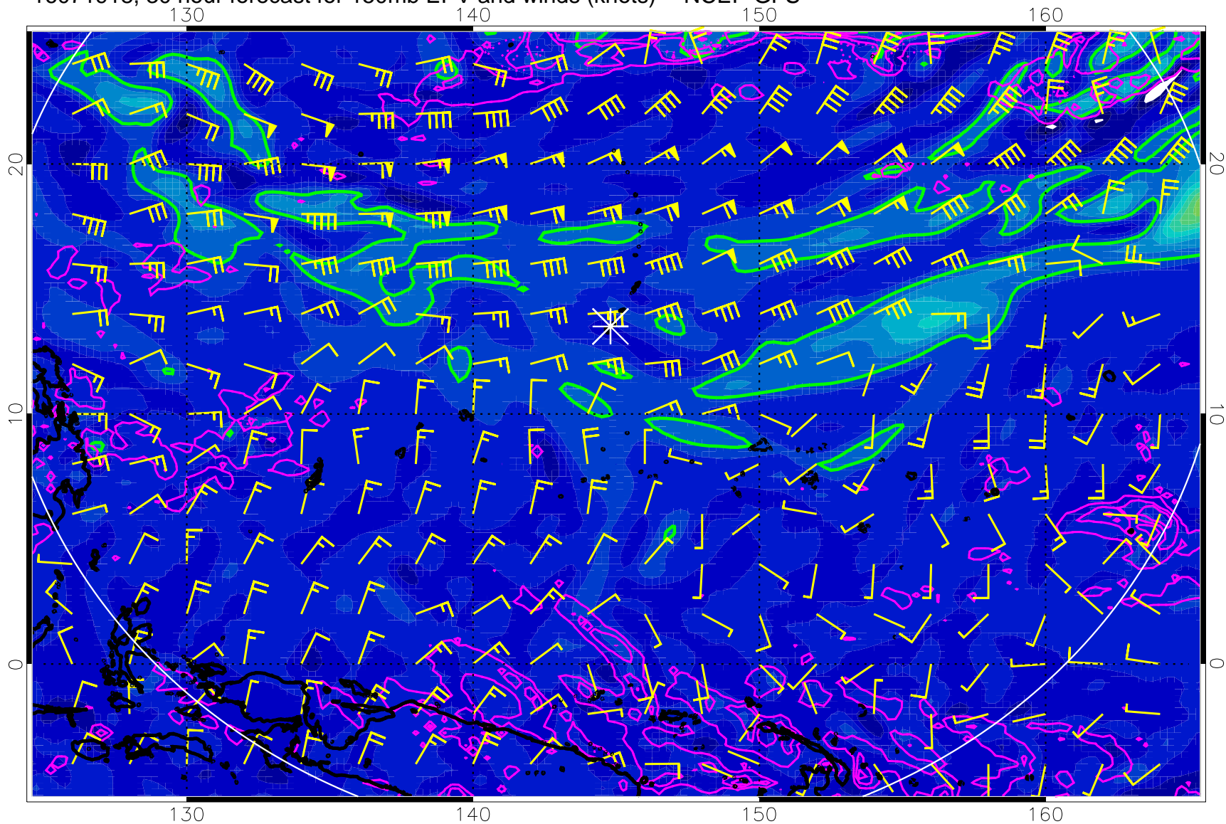
16071918, 30 hour forecast for 150mb EPV and winds (knots) -- NCEP GFS
