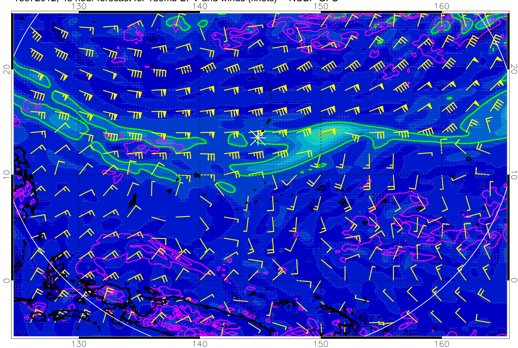
16072012, 48 hour forecast for 150mb EPV and winds (knots) -- NCEP GFS
