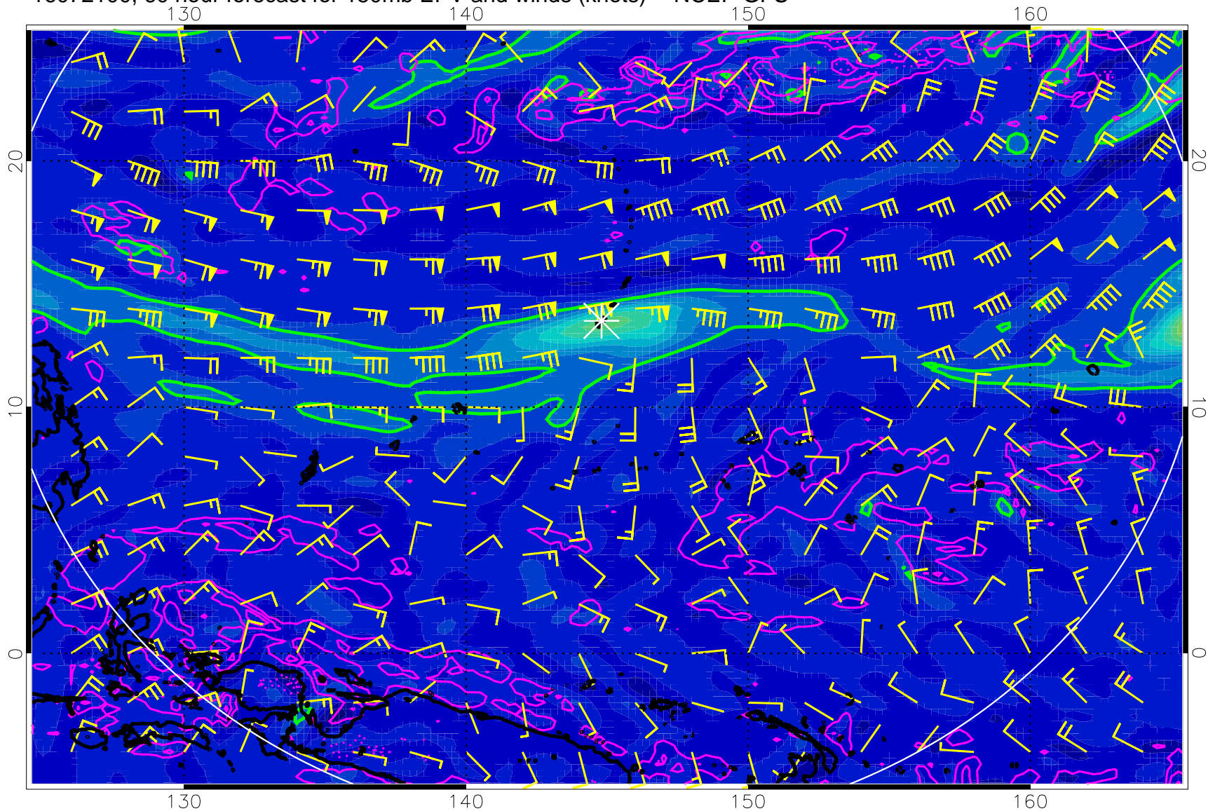
16072100, 60 hour forecast for 150mb EPV and winds (knots) -- NCEP GFS
