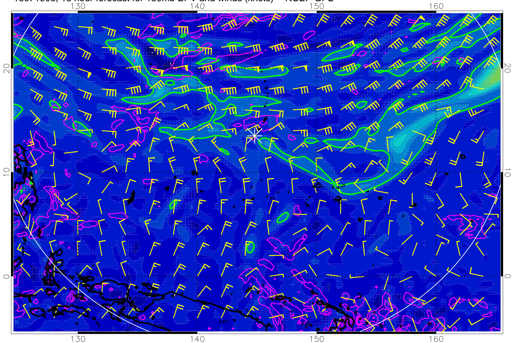
16071906, 18 hour forecast for 150mb EPV and winds (knots) -- NCEP GFS
