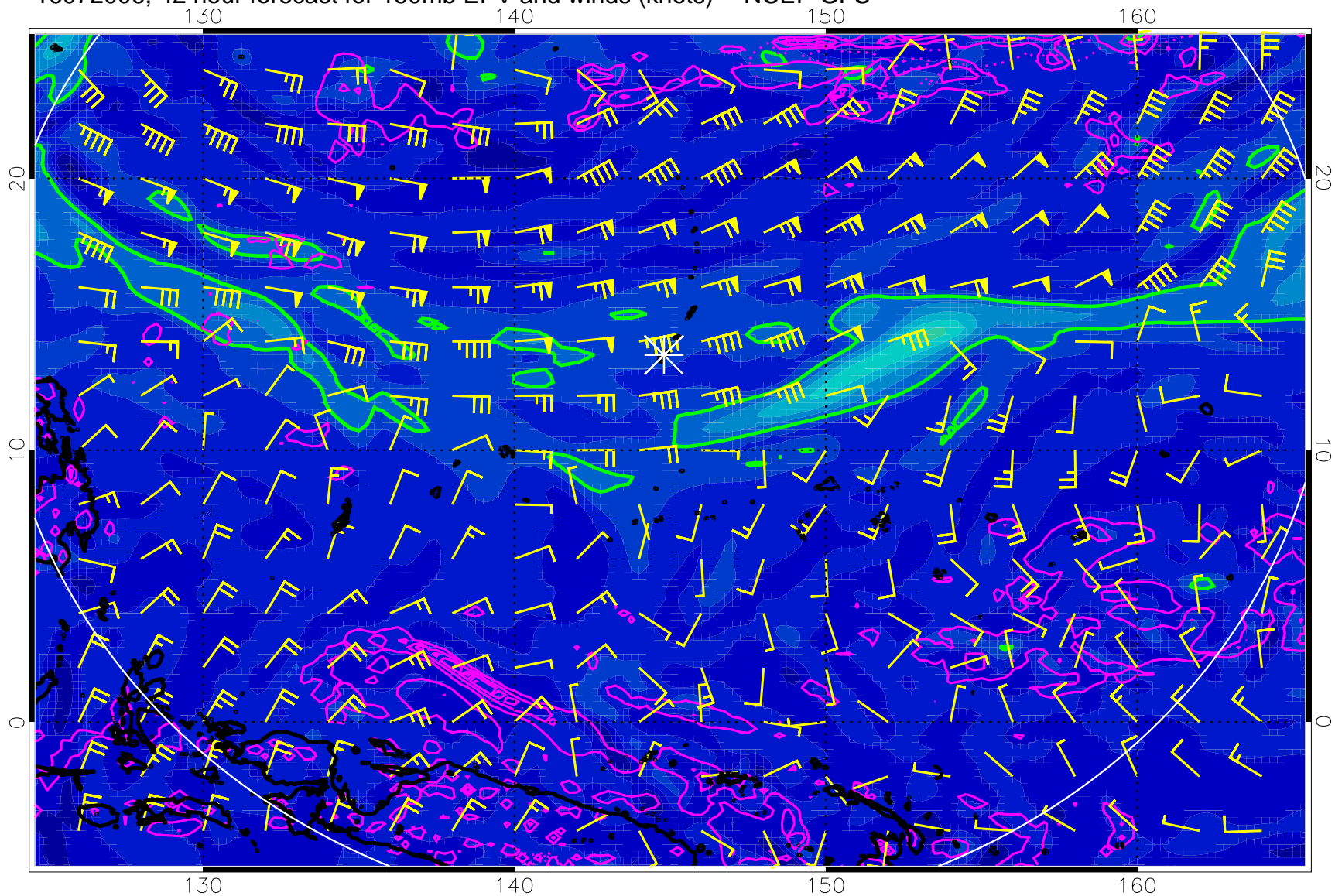
16072006, 42 hour forecast for 150mb EPV and winds (knots) -- NCEP GFS
