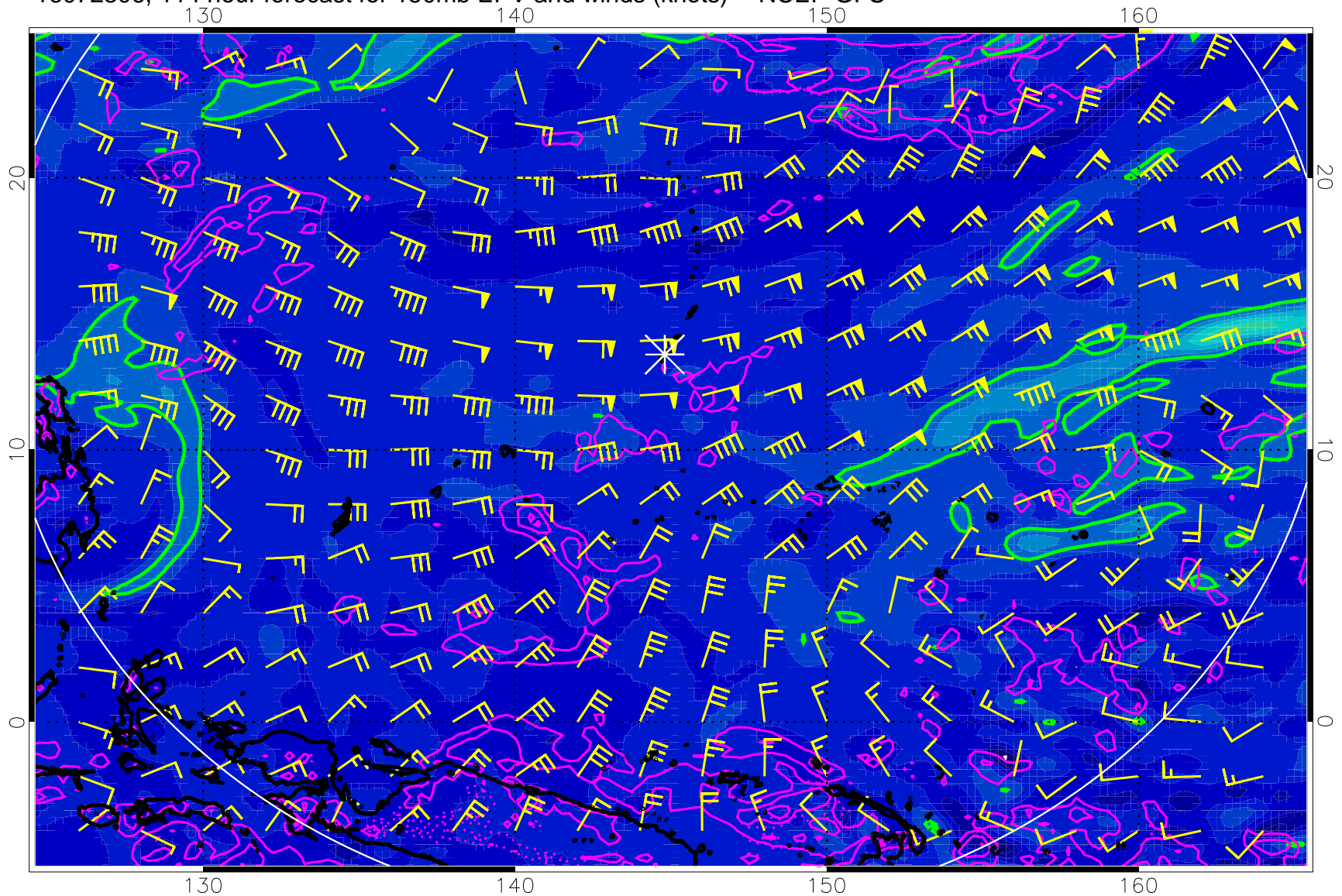
16072306, 114 hour forecast for 150mb EPV and winds (knots) -- NCEP GFS
