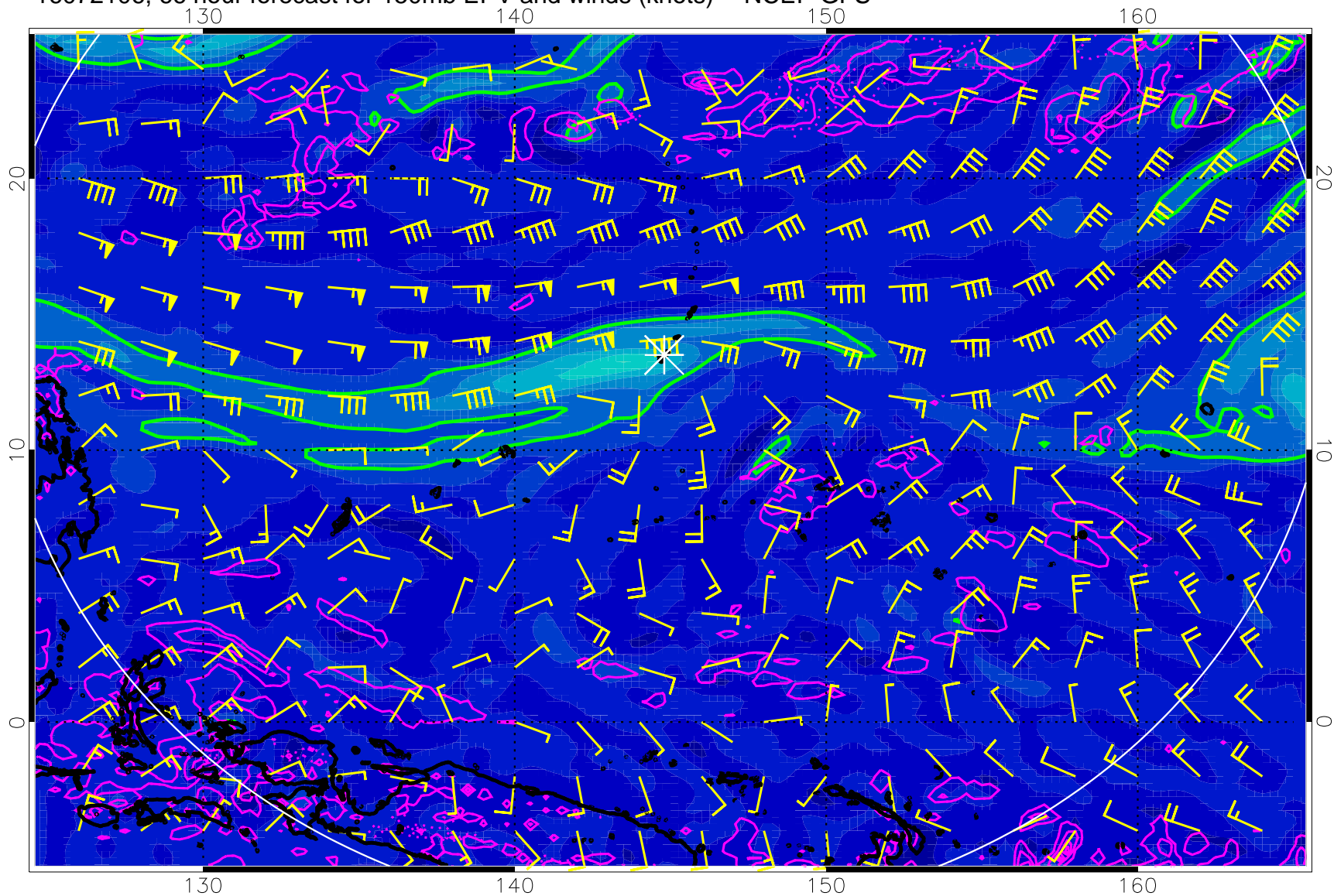
16072106, 66 hour forecast for 150mb EPV and winds (knots) -- NCEP GFS
