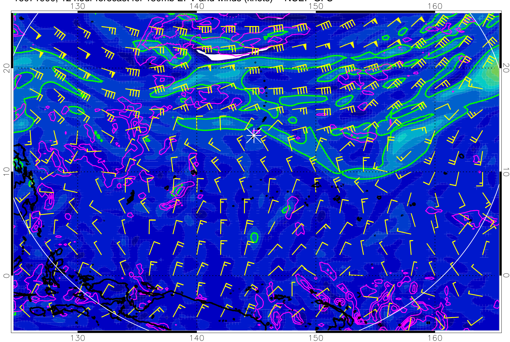
16071900, 12 hour forecast for 150mb EPV and winds (knots) -- NCEP GFS
