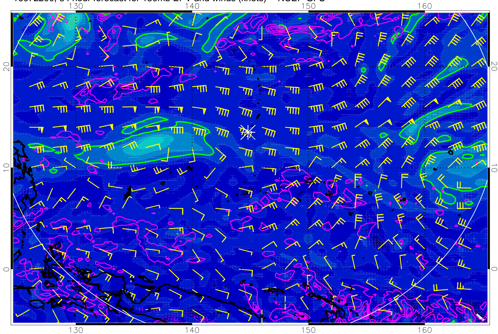
16072200, 84 hour forecast for 150mb EPV and winds (knots) -- NCEP GFS
