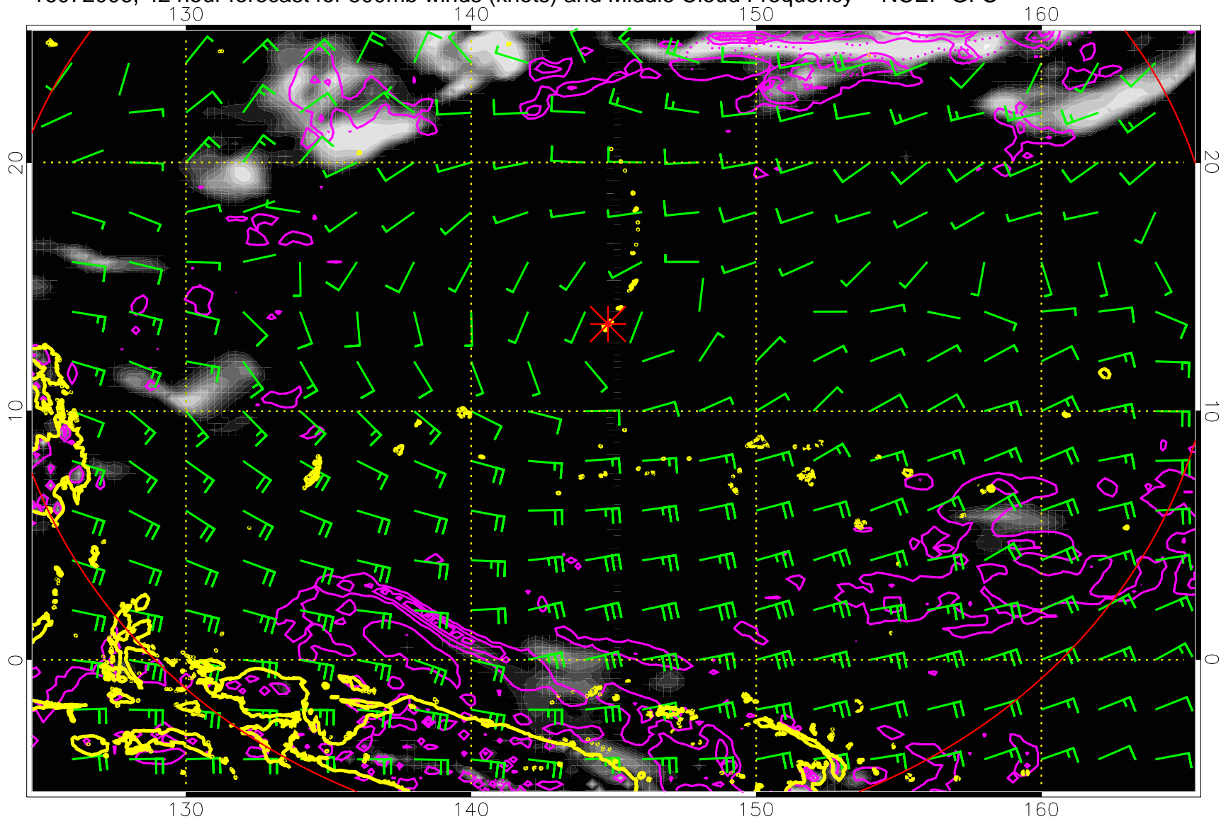
16072006, 42 hour forecast for 500mb winds (knots) and Middle Cloud Frequency -- NCEP GFS
