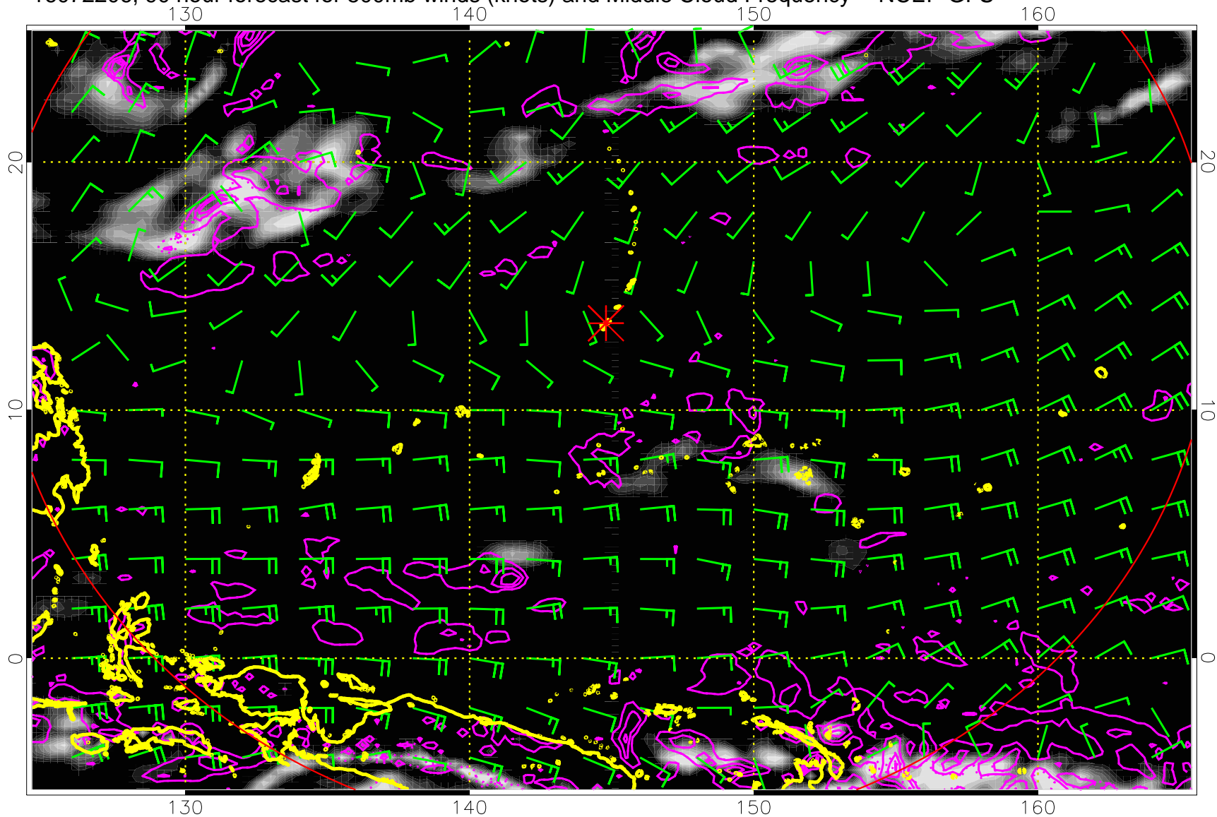
16072206, 90 hour forecast for 500mb winds (knots) and Middle Cloud Frequency -- NCEP GFS
