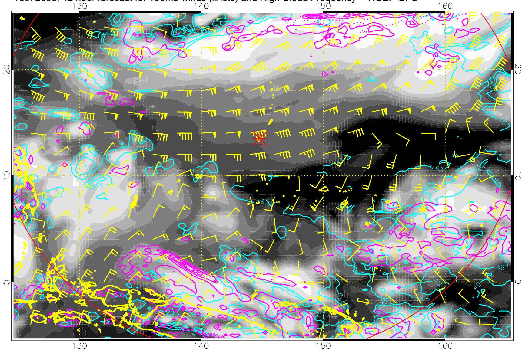
16072006, 42 hour forecast for 150mb winds (knots) and High Cloud Frequency -- NCEP GFS
