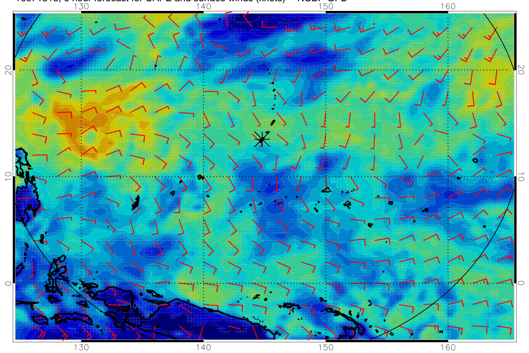
16071818, 6 hour forecast for CAPE and surface winds (knots) -- NCEP GFS
