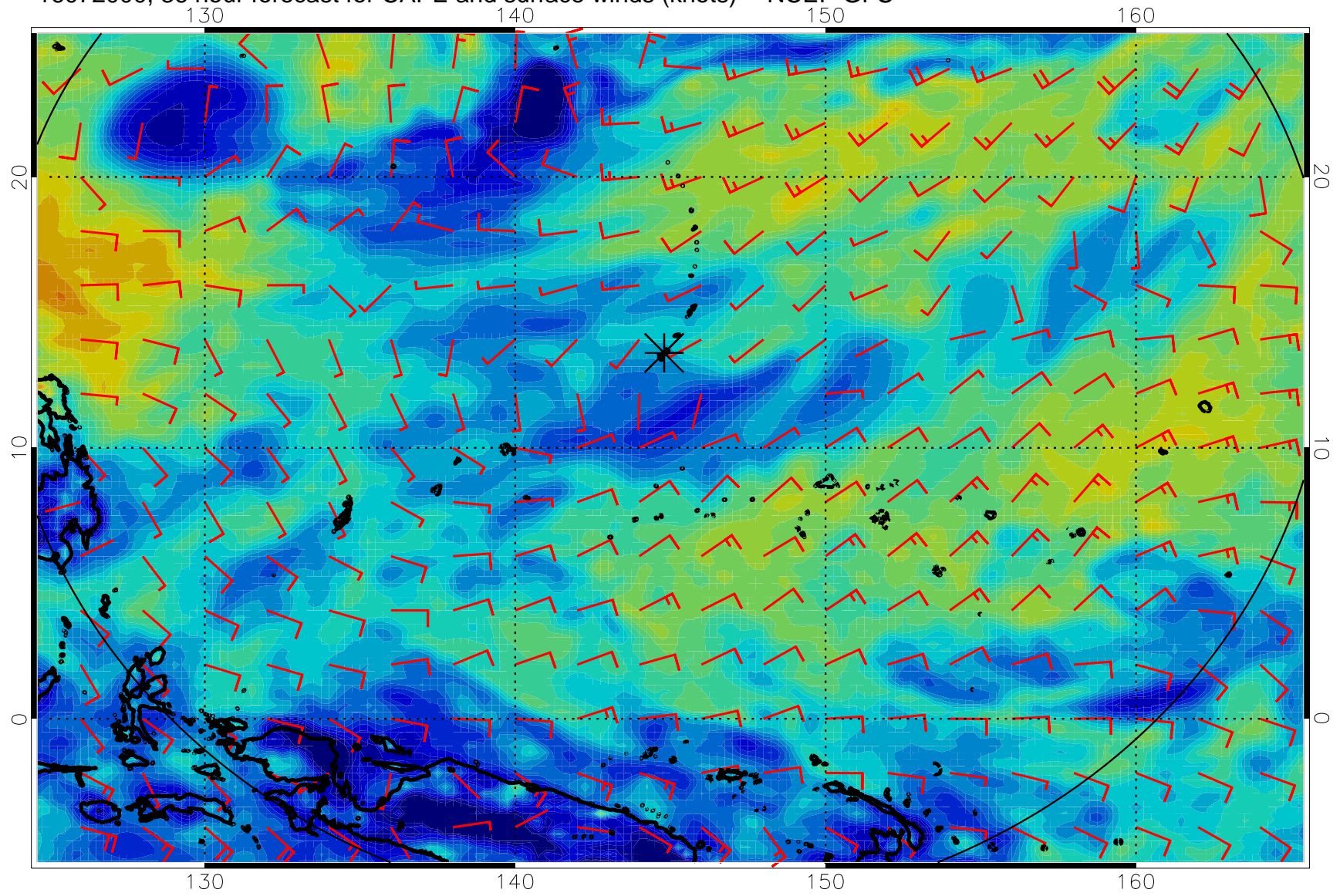
16072000, 36 hour forecast for CAPE and surface winds (knots) -- NCEP GFS
