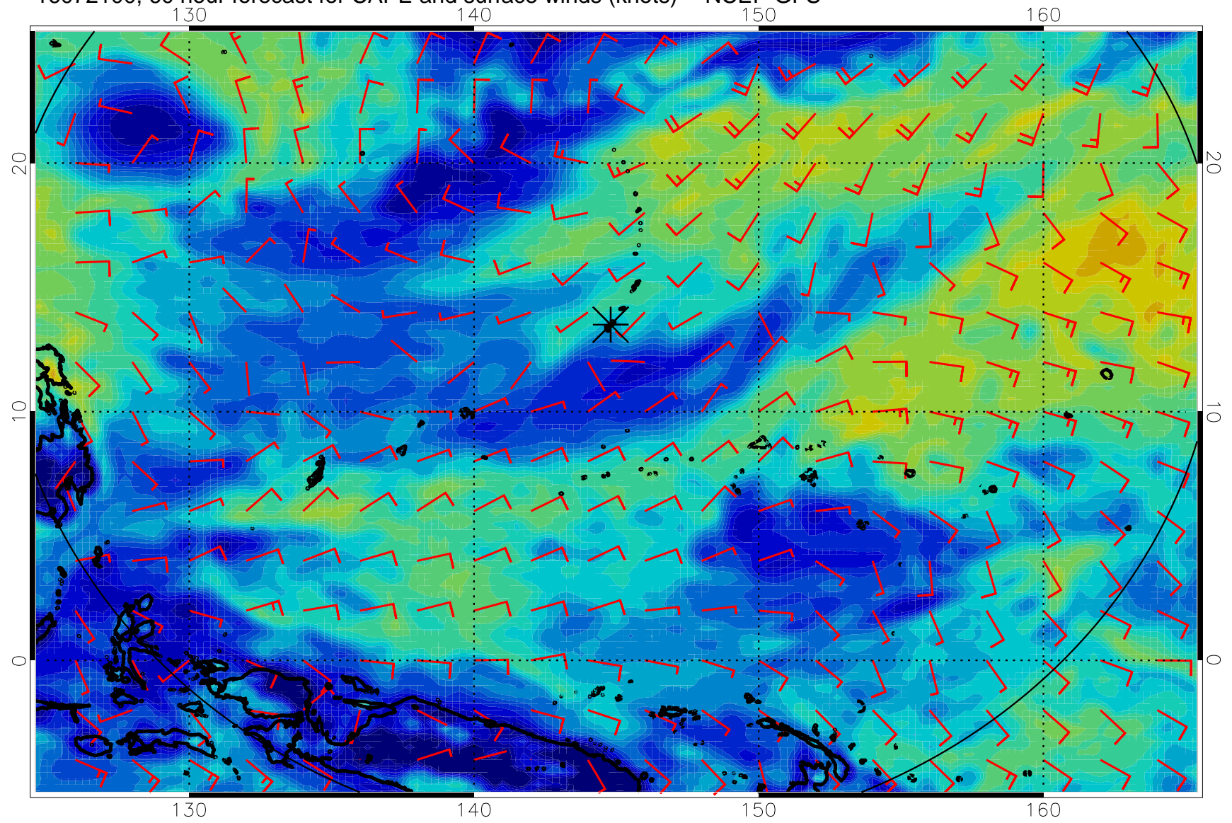
16072100, 60 hour forecast for CAPE and surface winds (knots) -- NCEP GFS
