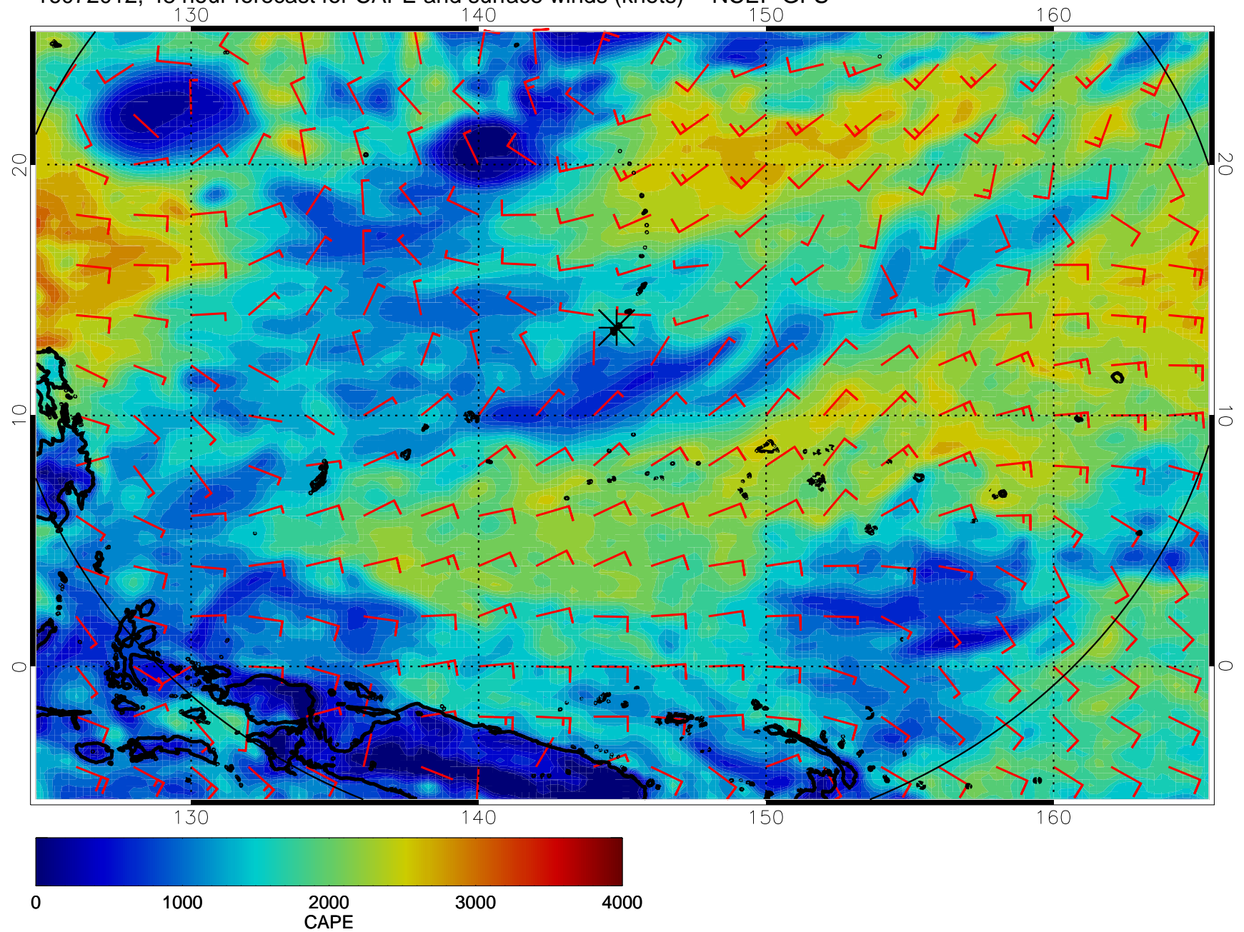
16072012, 48 hour forecast for CAPE and surface winds (knots) -- NCEP GFS
