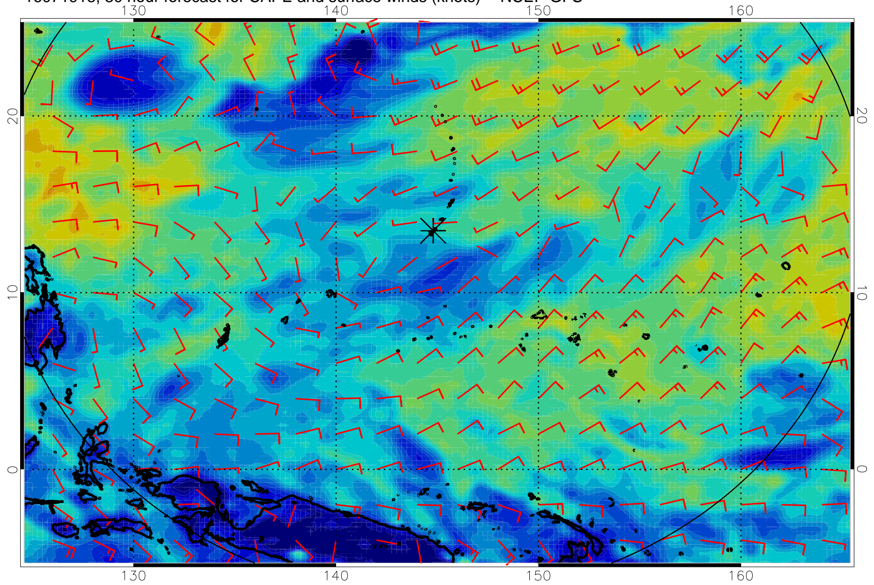
16071918, 30 hour forecast for CAPE and surface winds (knots) -- NCEP GFS
