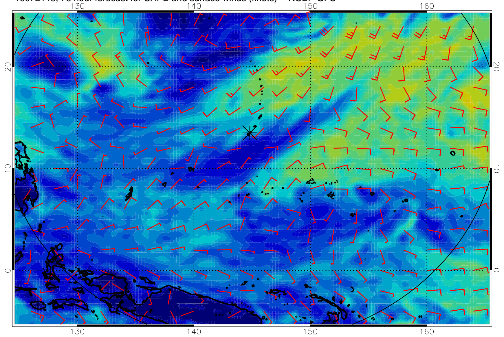
16072118, 78 hour forecast for CAPE and surface winds (knots) -- NCEP GFS
