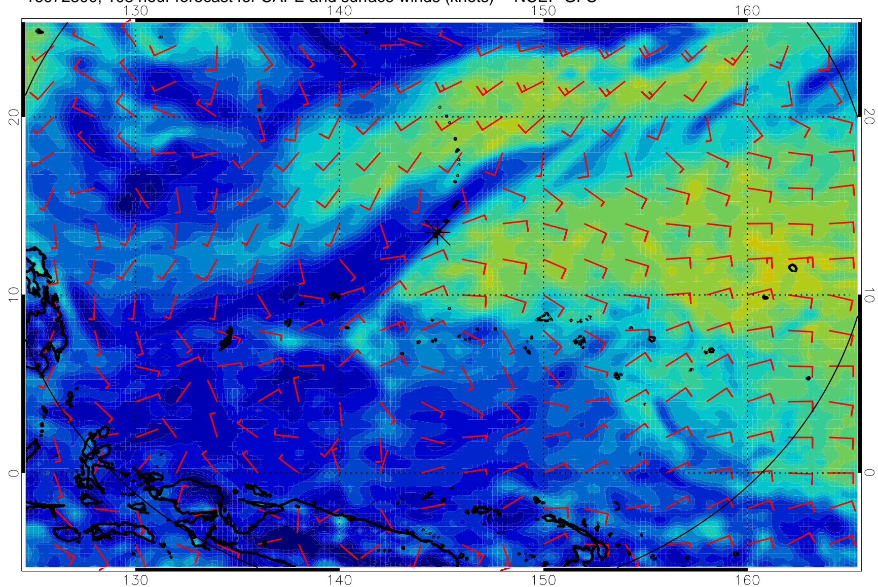
16072300, 108 hour forecast for CAPE and surface winds (knots) -- NCEP GFS
