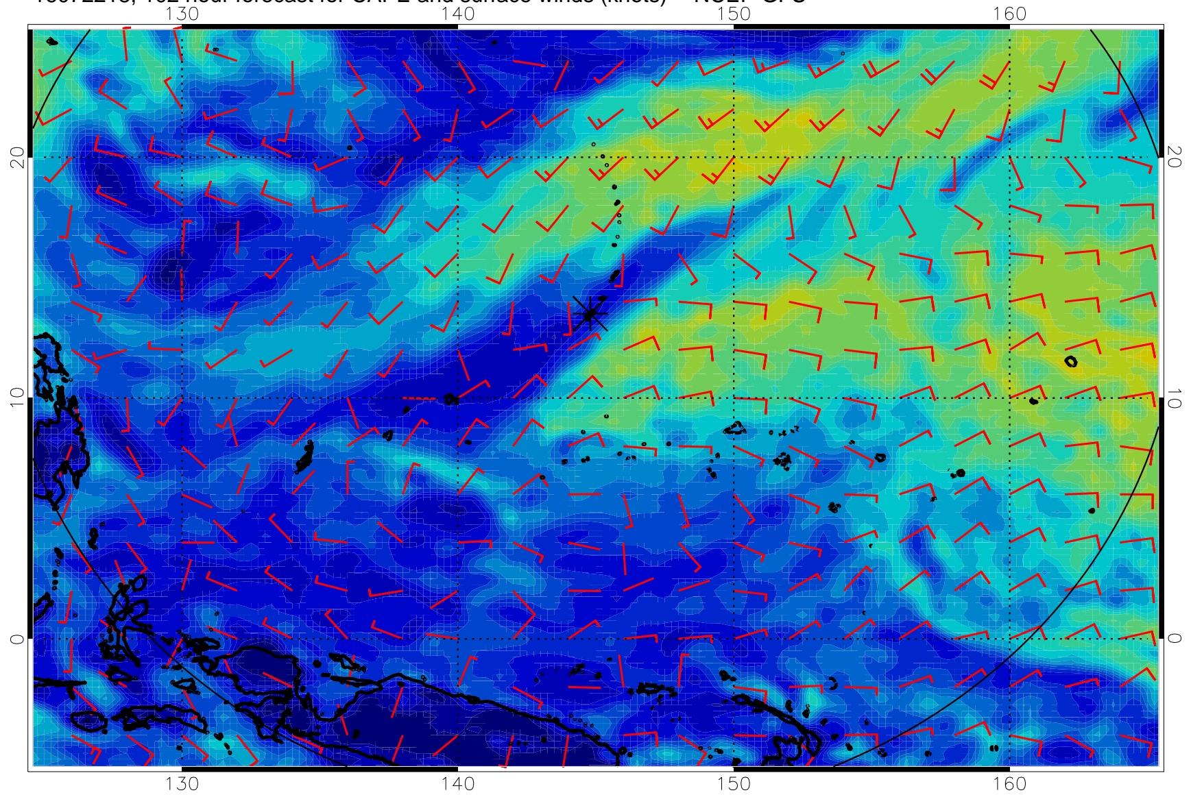
16072218, 102 hour forecast for CAPE and surface winds (knots) -- NCEP GFS
