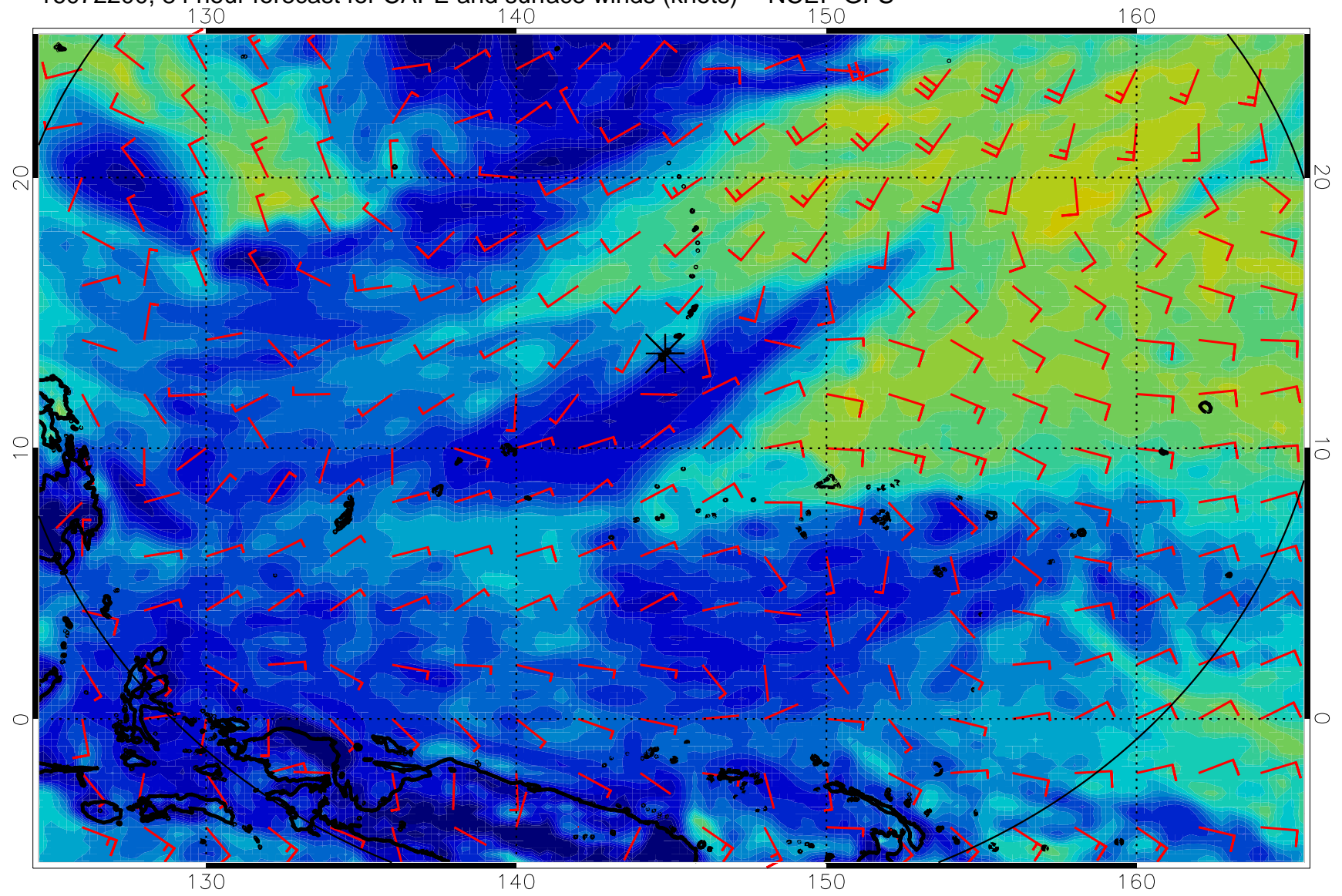
16072200, 84 hour forecast for CAPE and surface winds (knots) -- NCEP GFS
