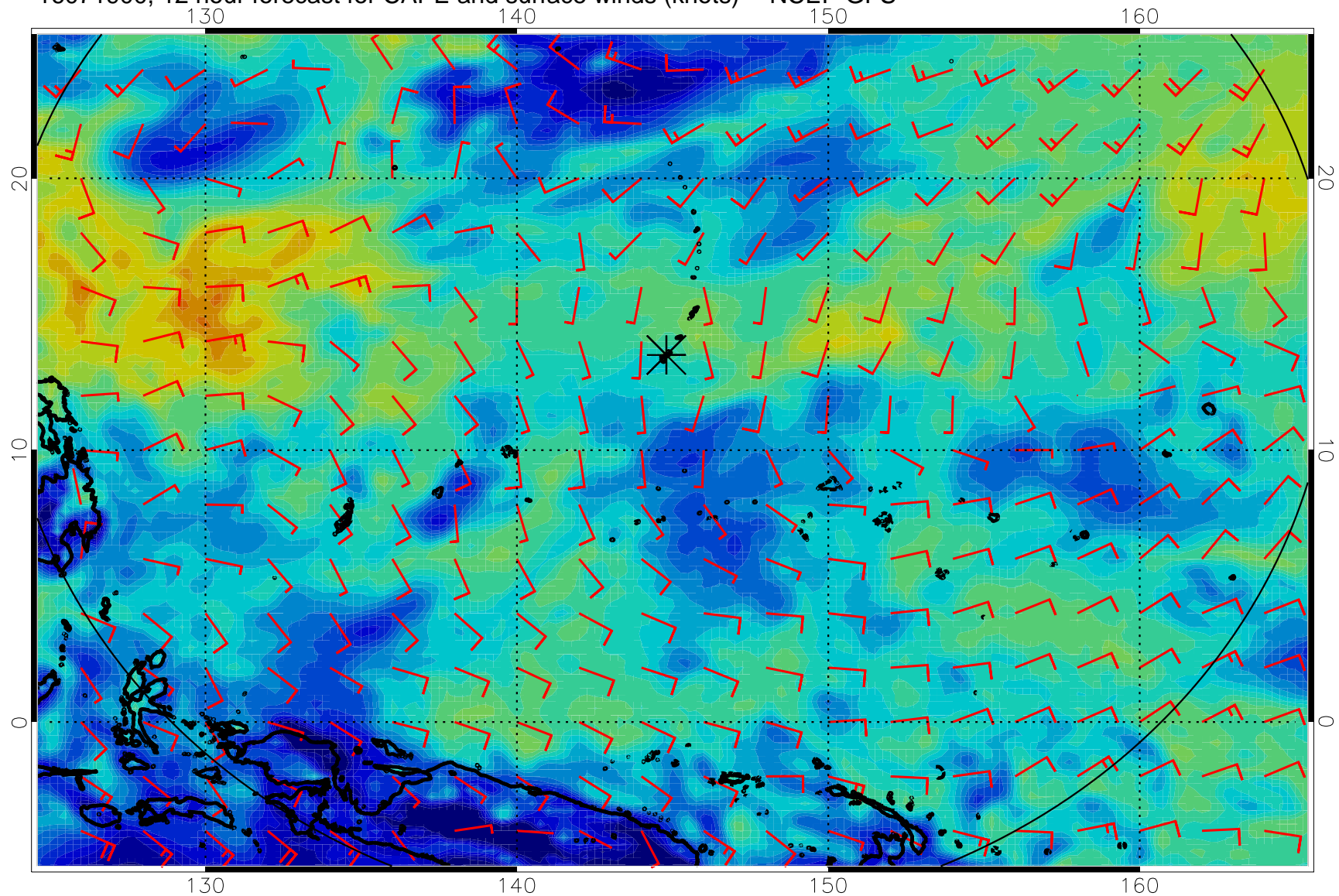
16071900, 12 hour forecast for CAPE and surface winds (knots) -- NCEP GFS
