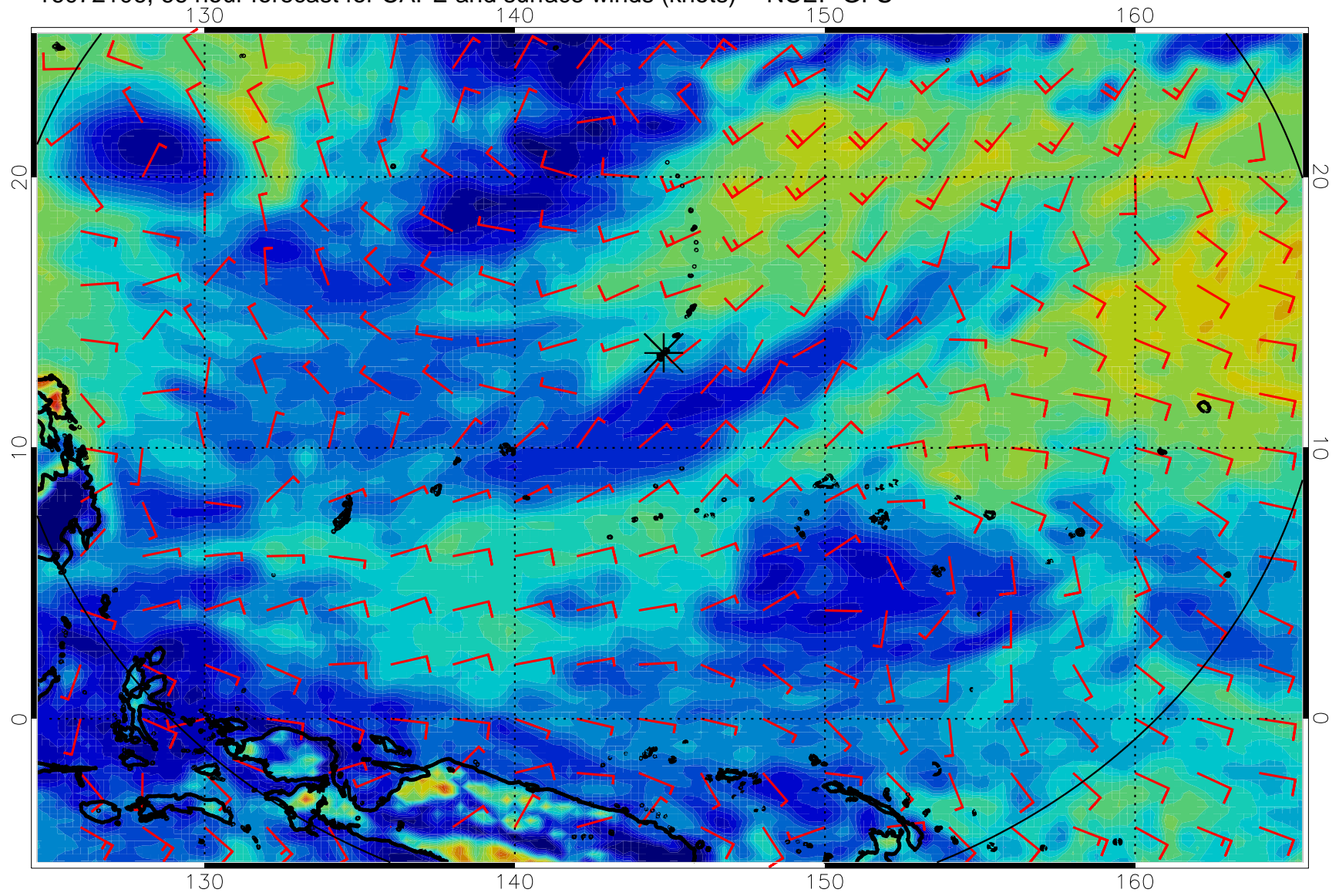
16072106, 66 hour forecast for CAPE and surface winds (knots) -- NCEP GFS
