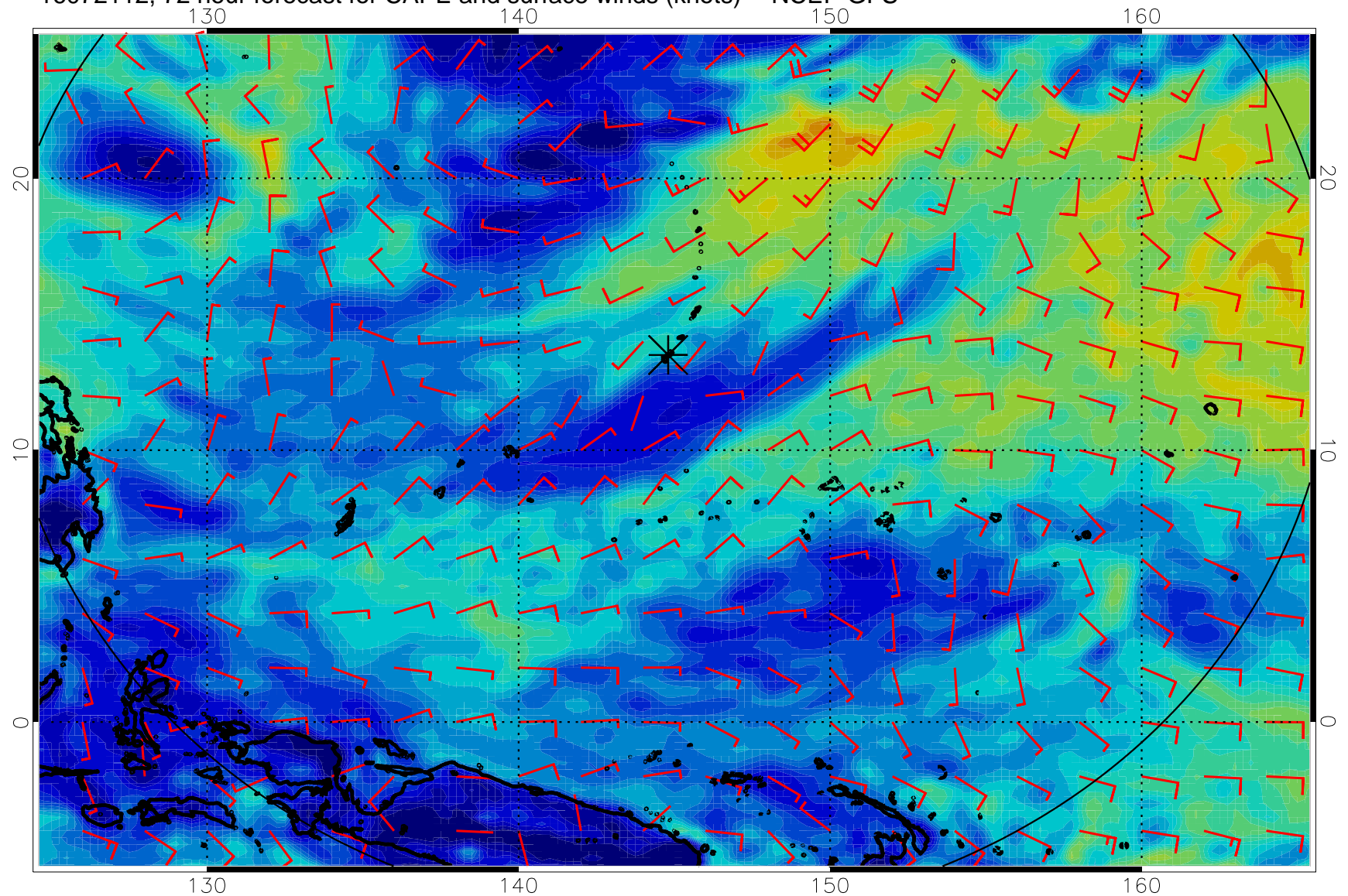
16072112, 72 hour forecast for CAPE and surface winds (knots) -- NCEP GFS
