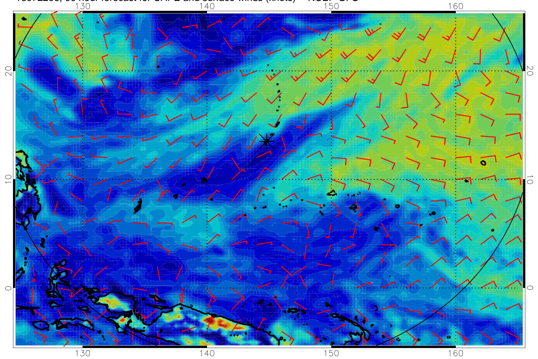
16072206, 90 hour forecast for CAPE and surface winds (knots) -- NCEP GFS
