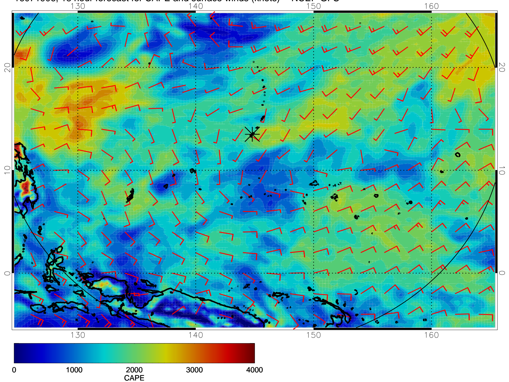
16071906, 18 hour forecast for CAPE and surface winds (knots) -- NCEP GFS
