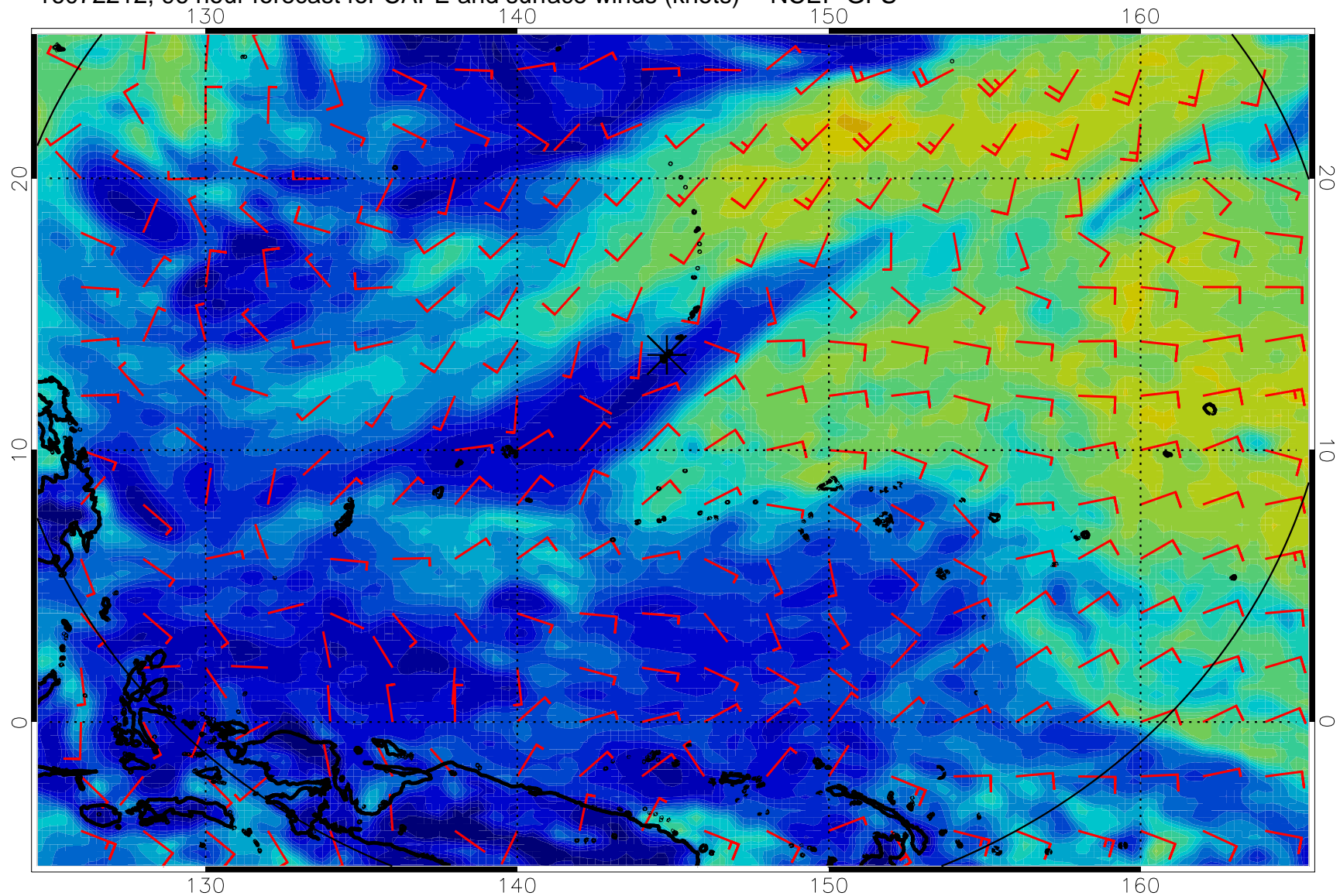
16072212, 96 hour forecast for CAPE and surface winds (knots) -- NCEP GFS
