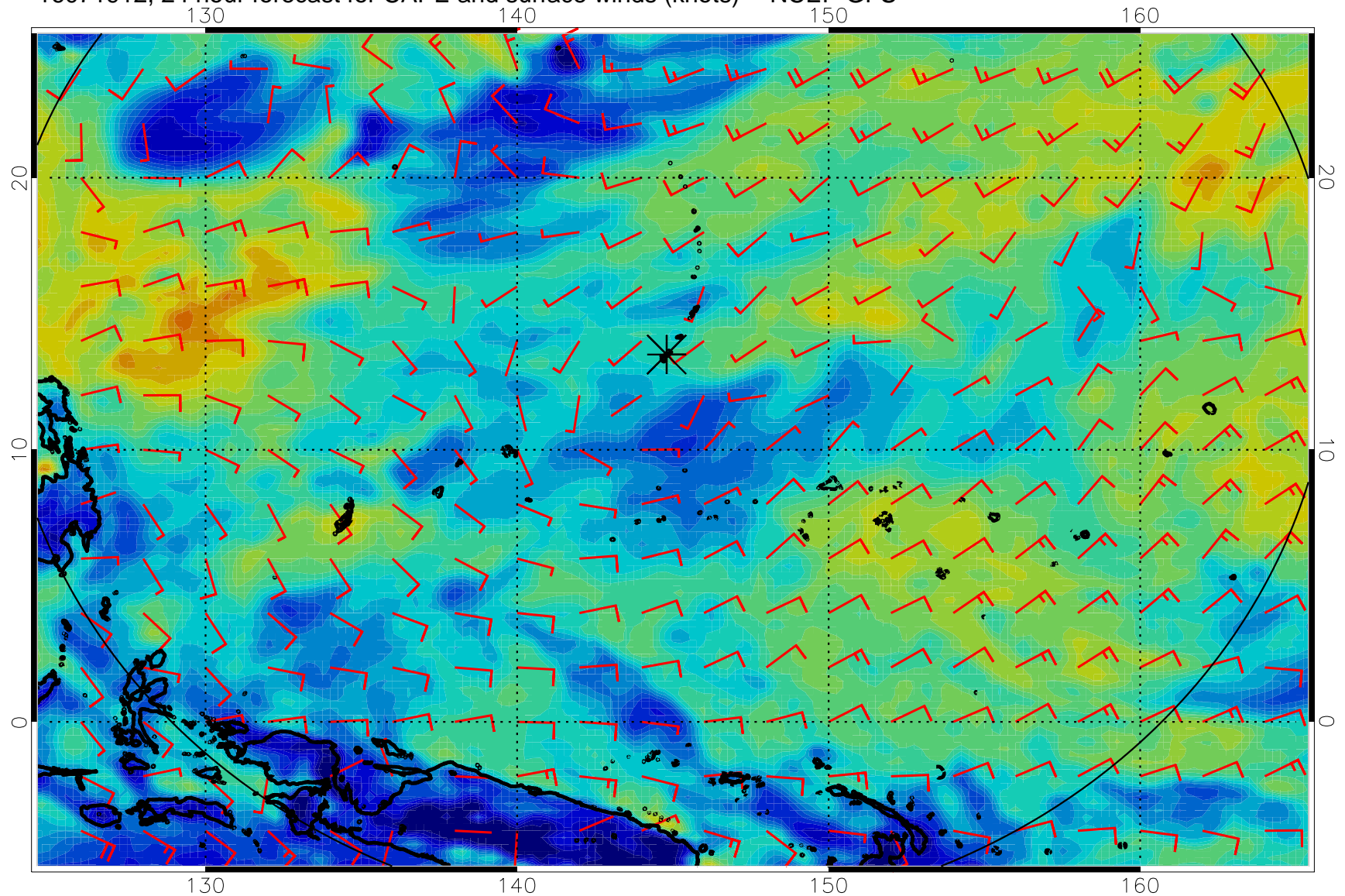
16071912, 24 hour forecast for CAPE and surface winds (knots) -- NCEP GFS
