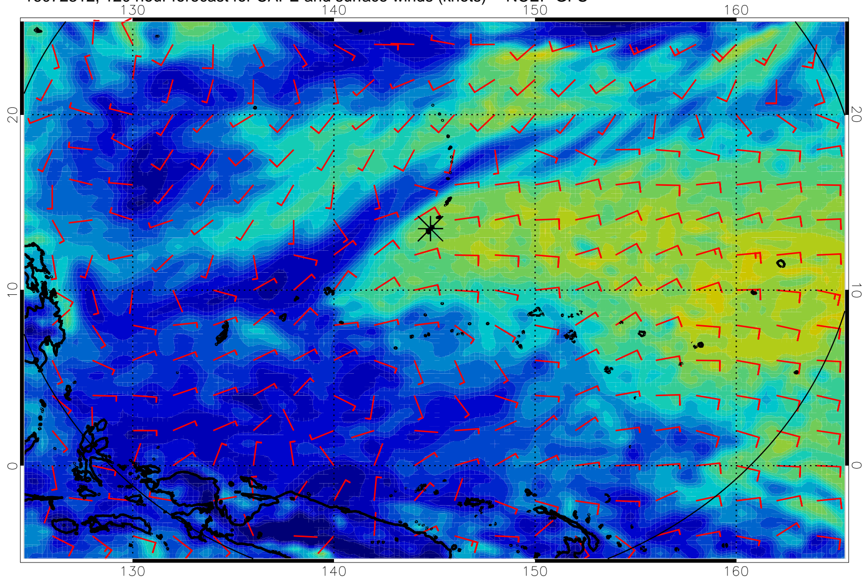
16072312, 120 hour forecast for CAPE and surface winds (knots) -- NCEP GFS
