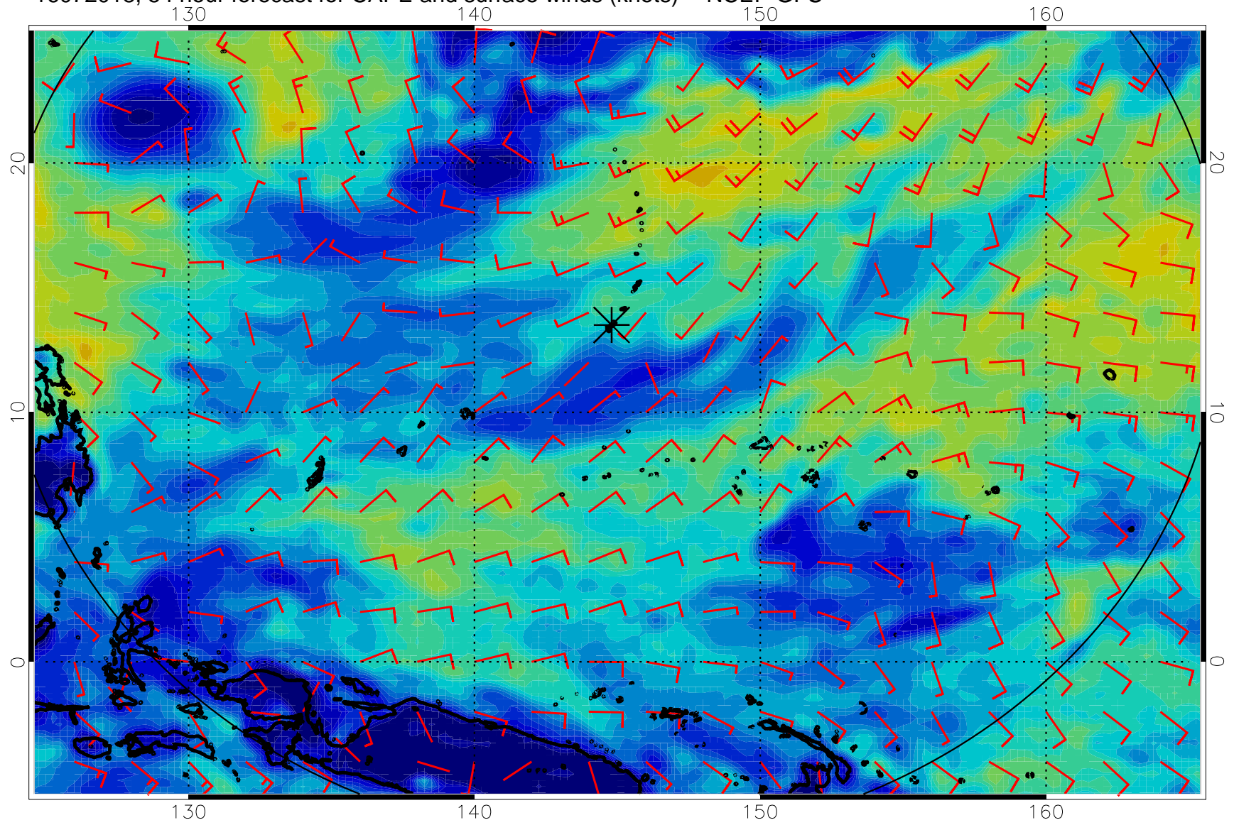
16072018, 54 hour forecast for CAPE and surface winds (knots) -- NCEP GFS
