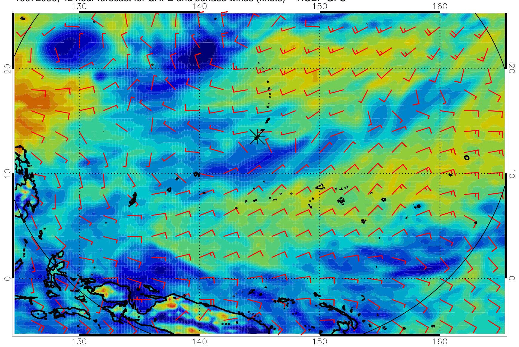
16072006, 42 hour forecast for CAPE and surface winds (knots) -- NCEP GFS
