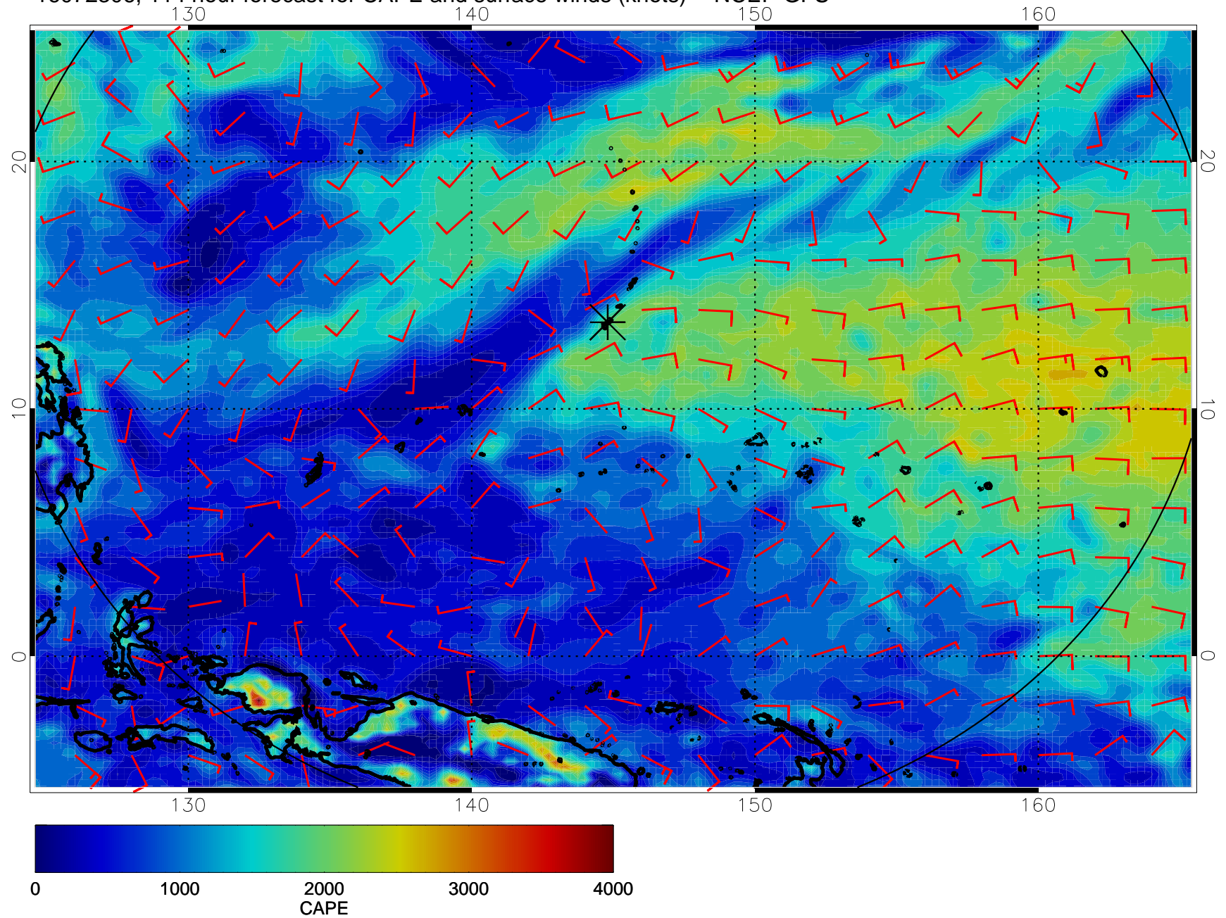
16072306, 114 hour forecast for CAPE and surface winds (knots) -- NCEP GFS
