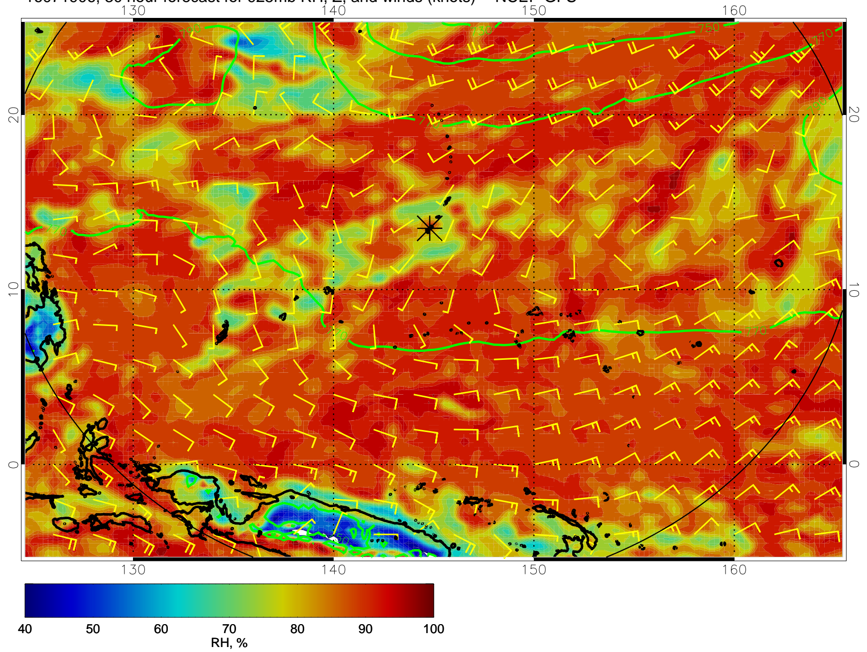
16071906, 30 hour forecast for 925mb RH, Z, and winds (knots) -- NCEP GFS
