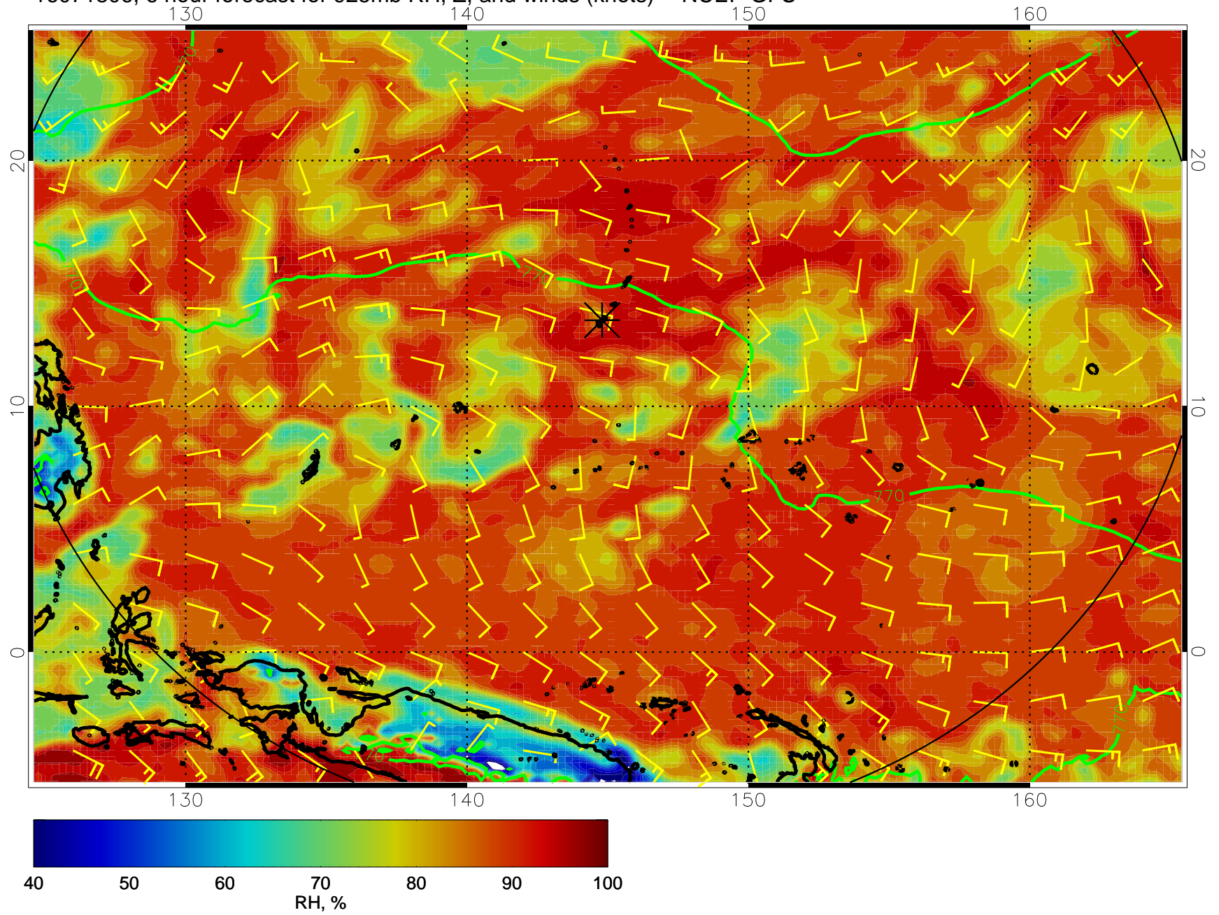
16071806, 6 hour forecast for 925mb RH, Z, and winds (knots) -- NCEP GFS
