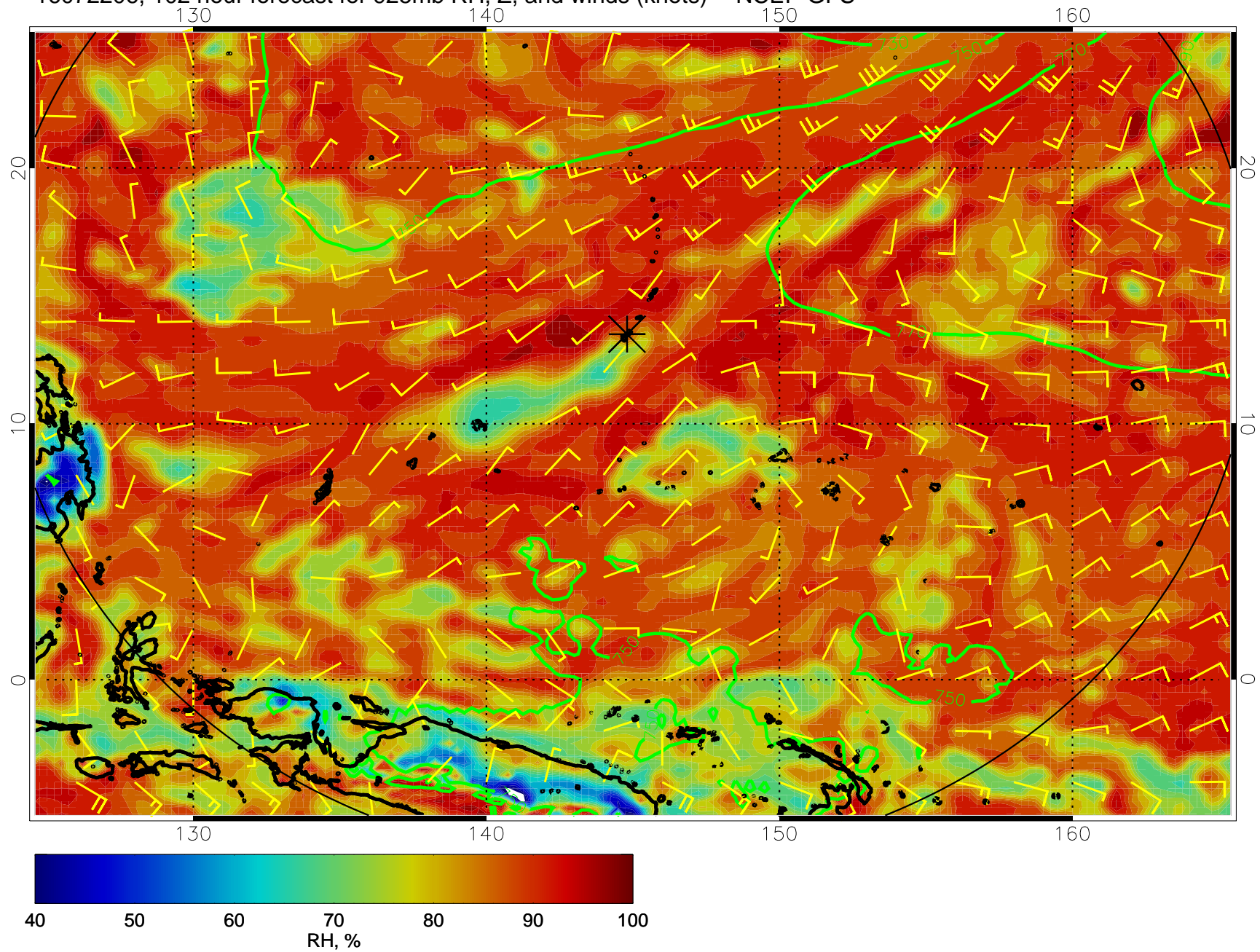
16072206, 102 hour forecast for 925mb RH, Z, and winds (knots) -- NCEP GFS
