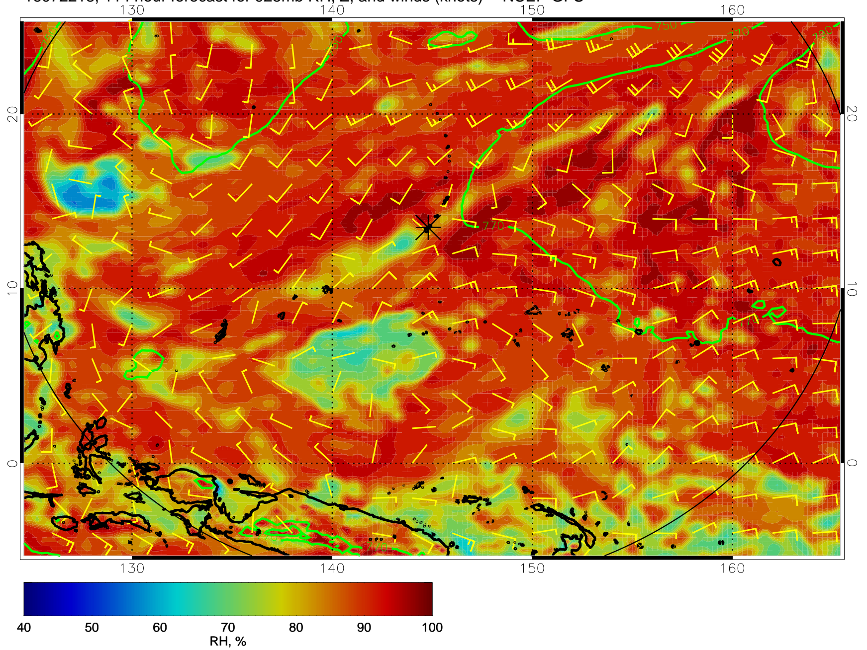
16072218, 114 hour forecast for 925mb RH, Z, and winds (knots) -- NCEP GFS
