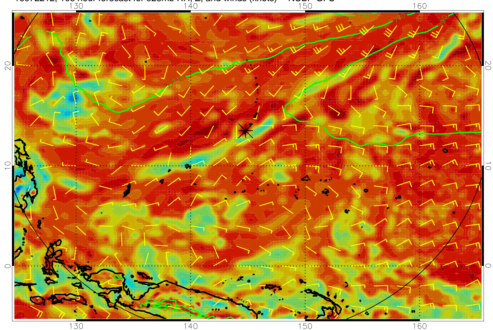
16072212, 108 hour forecast for 925mb RH, Z, and winds (knots) -- NCEP GFS
