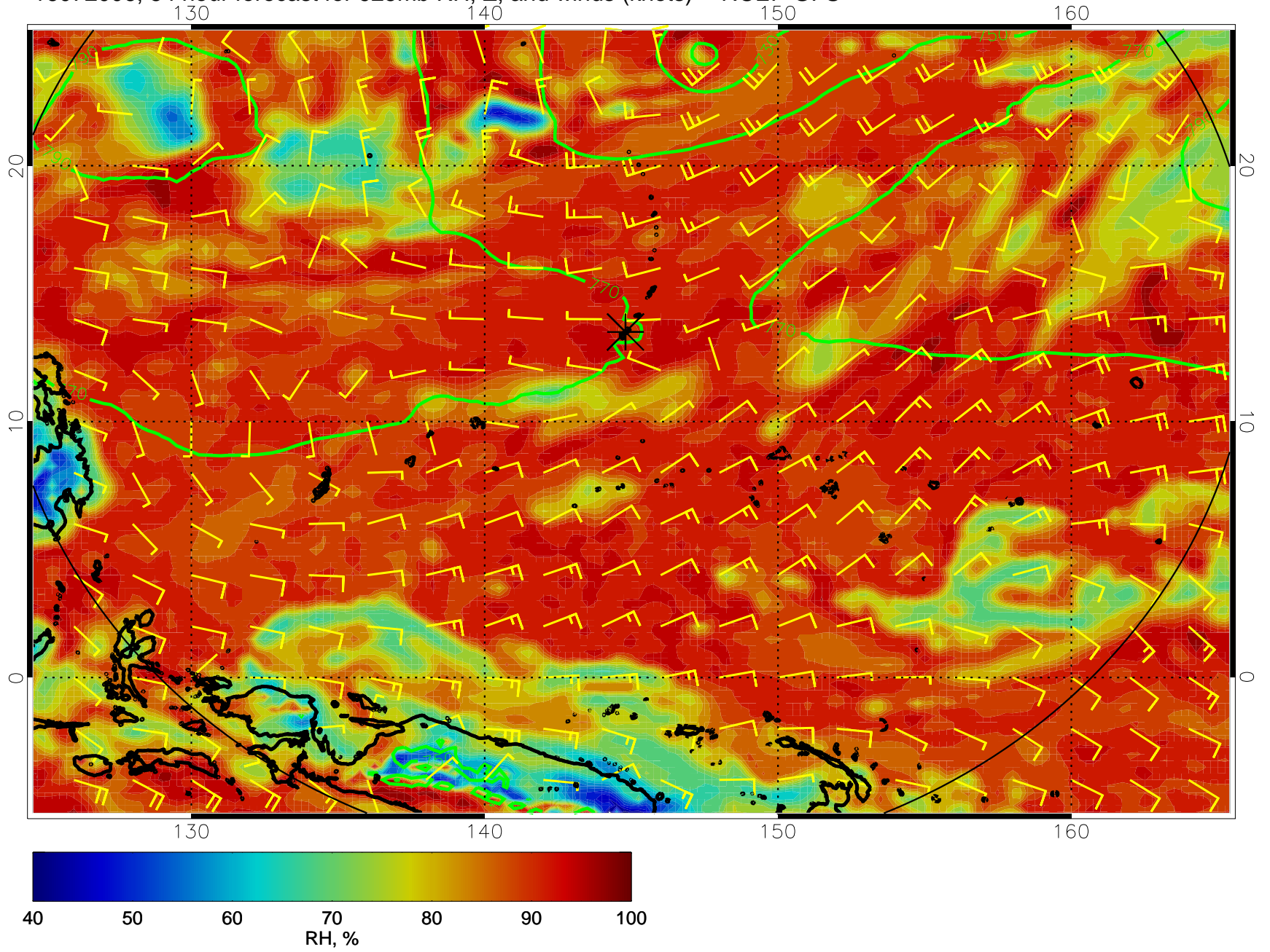
16072006, 54 hour forecast for 925mb RH, Z, and winds (knots) -- NCEP GFS
