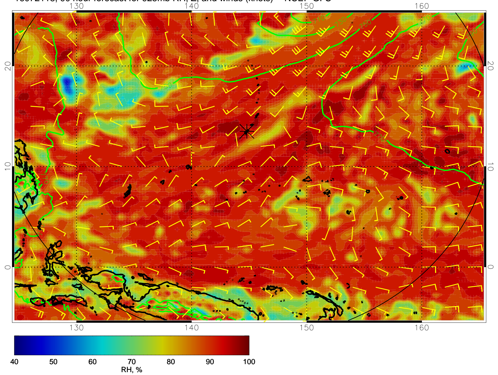
16072118, 90 hour forecast for 925mb RH, Z, and winds (knots) -- NCEP GFS
