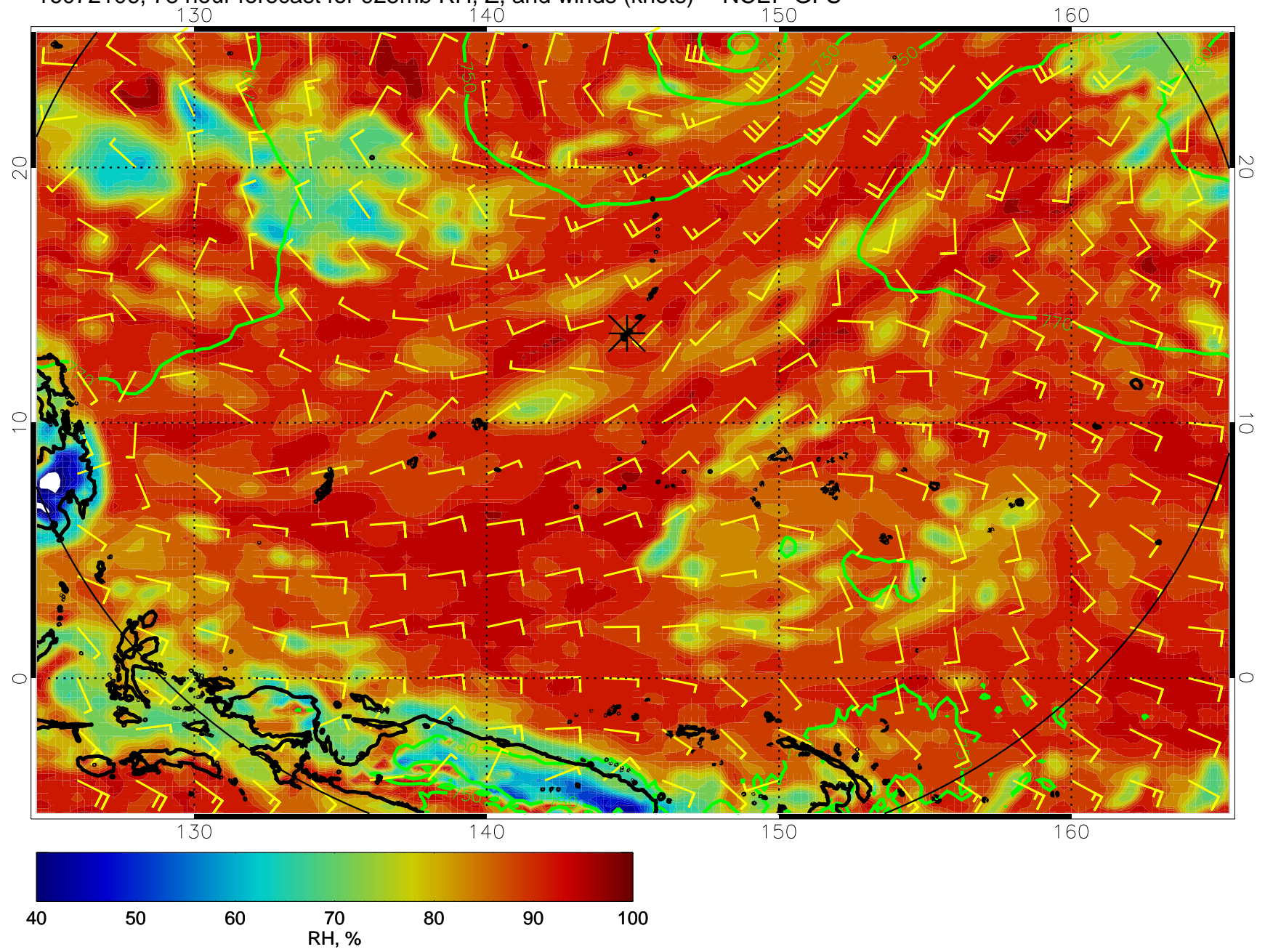
16072106, 78 hour forecast for 925mb RH, Z, and winds (knots) -- NCEP GFS
