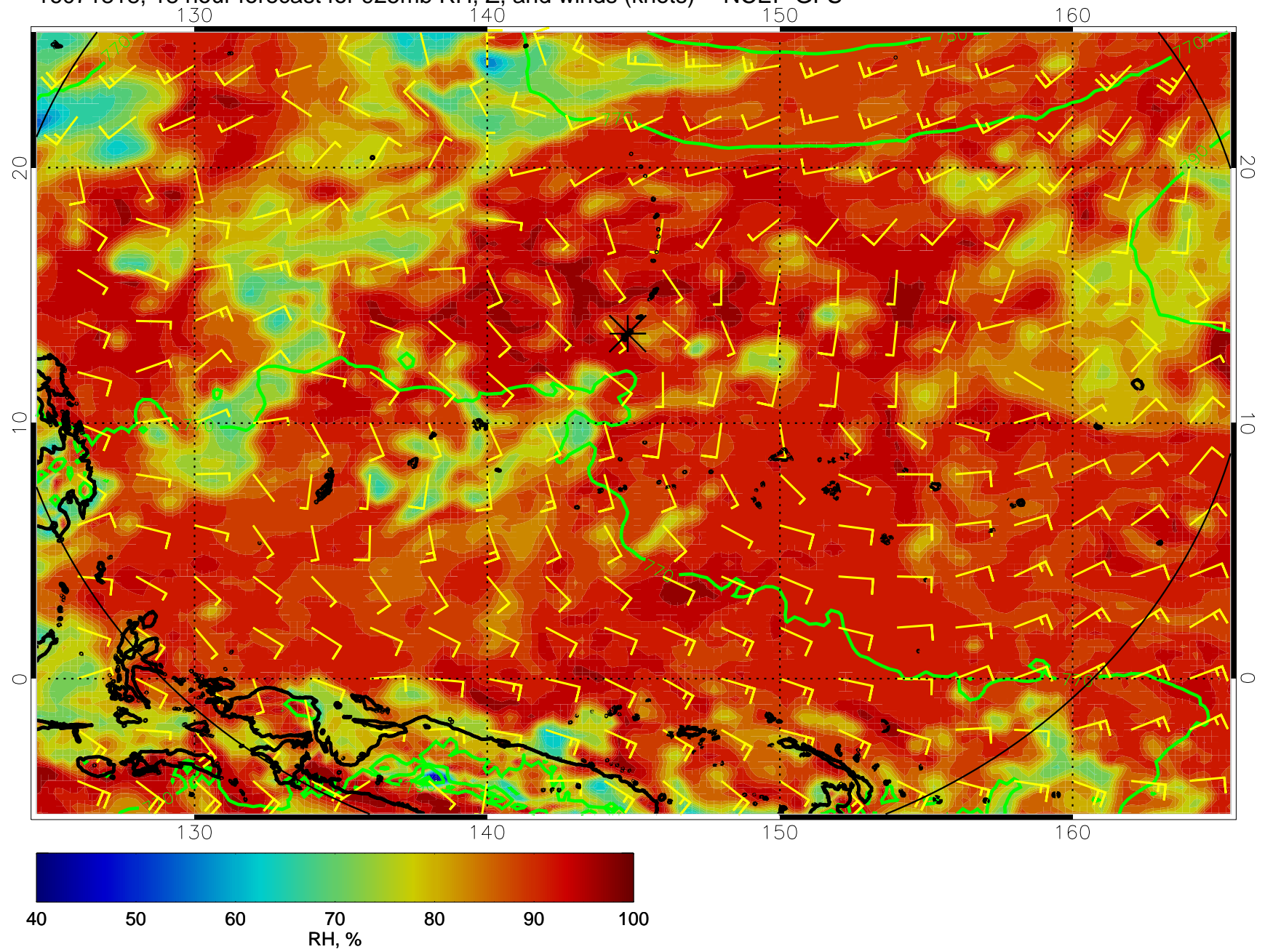
16071818, 18 hour forecast for 925mb RH, Z, and winds (knots) -- NCEP GFS
