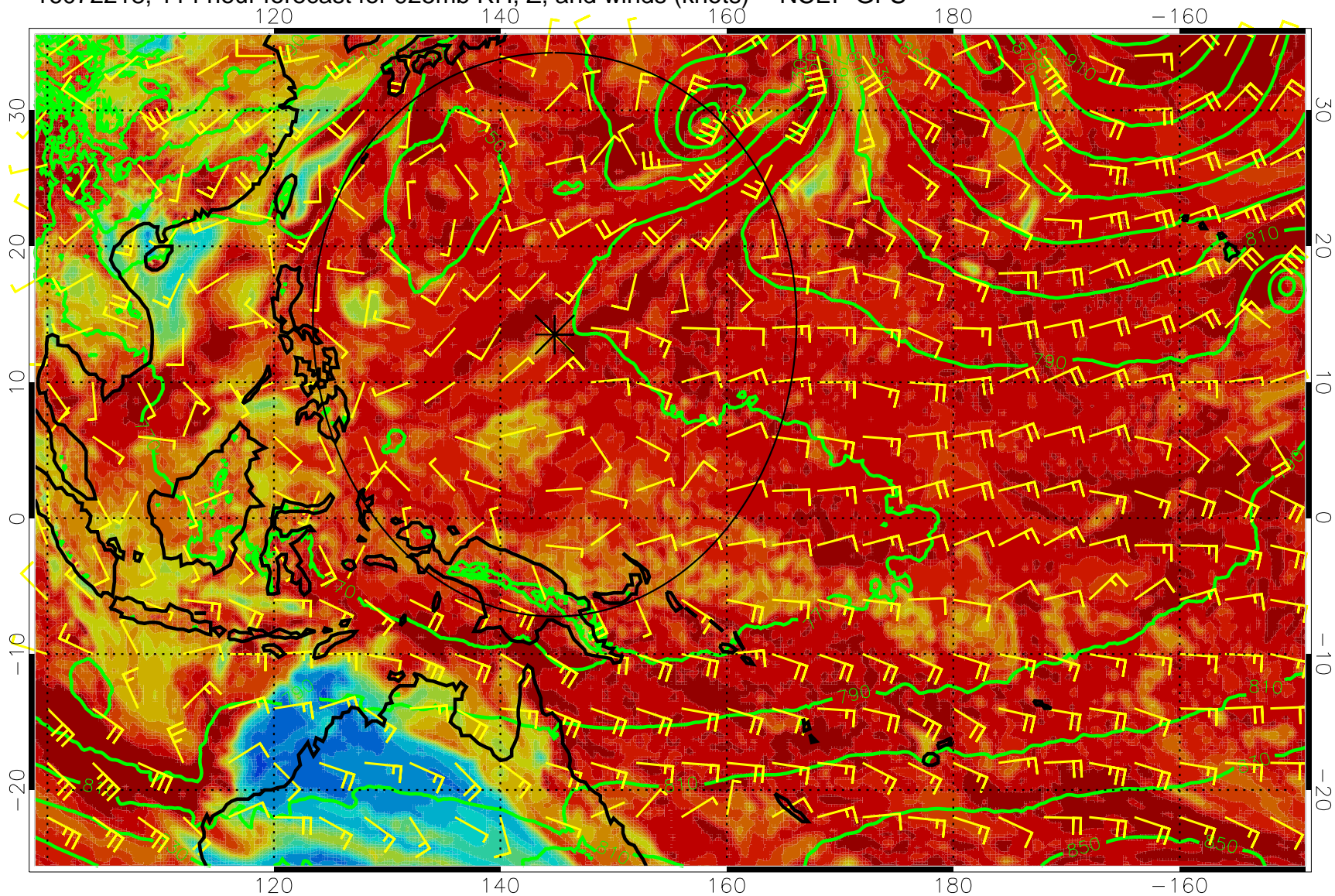
16072218, 114 hour forecast for 925mb RH, Z, and winds (knots) -- NCEP GFS
