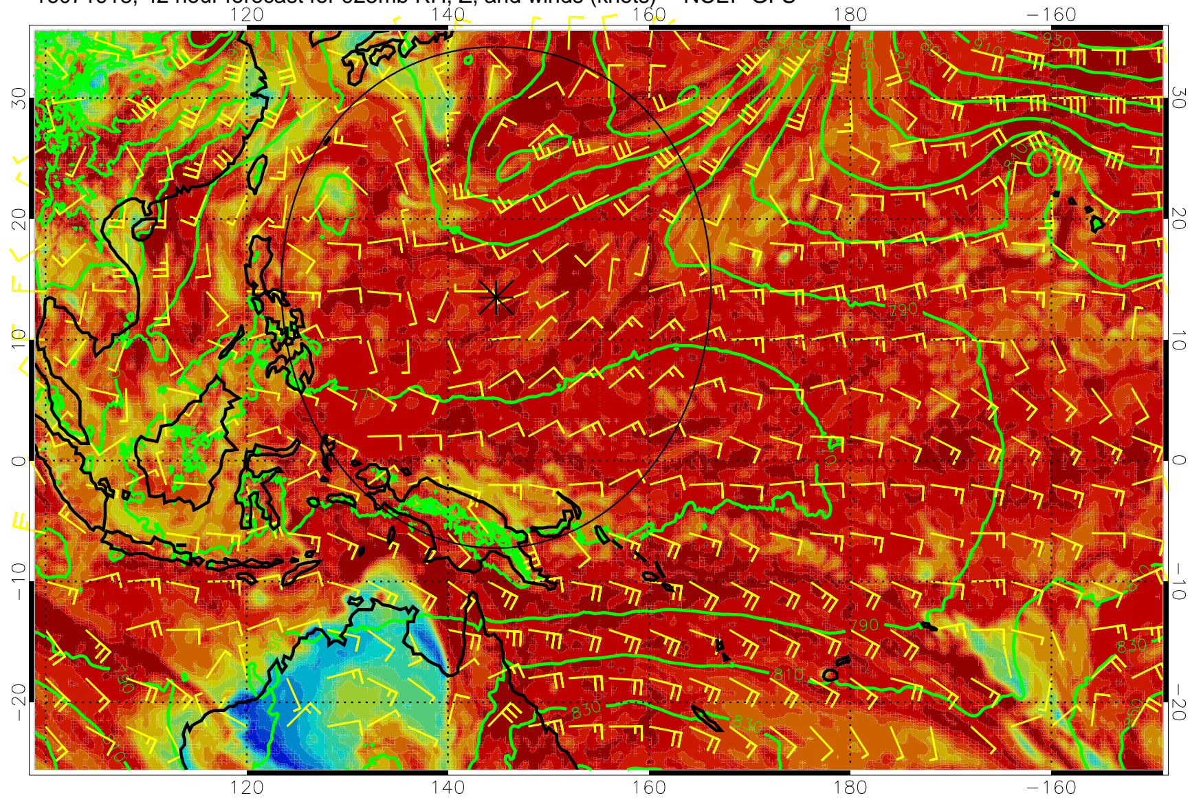
16071918, 42 hour forecast for 925mb RH, Z, and winds (knots) -- NCEP GFS
