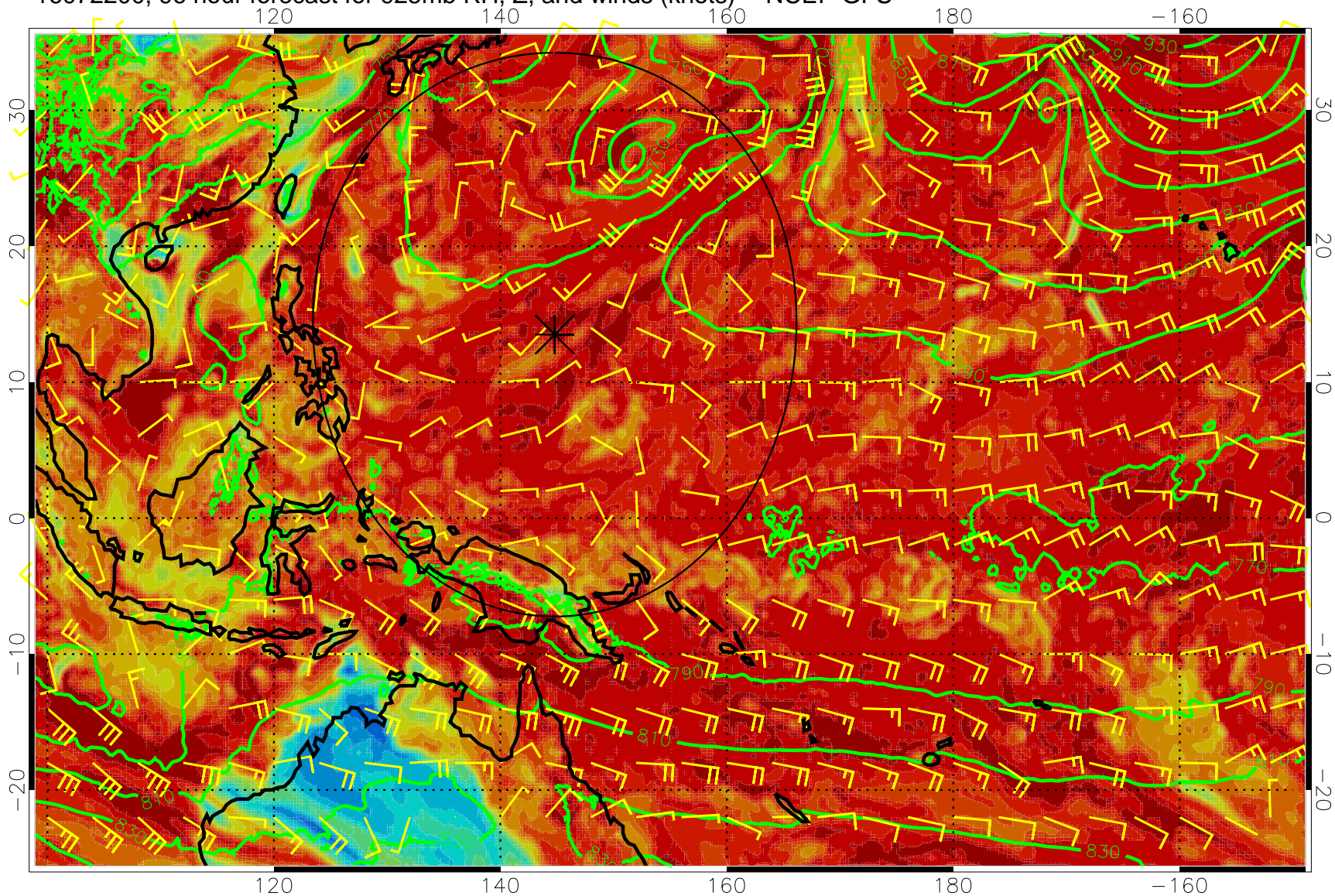
16072200, 96 hour forecast for 925mb RH, Z, and winds (knots) -- NCEP GFS
