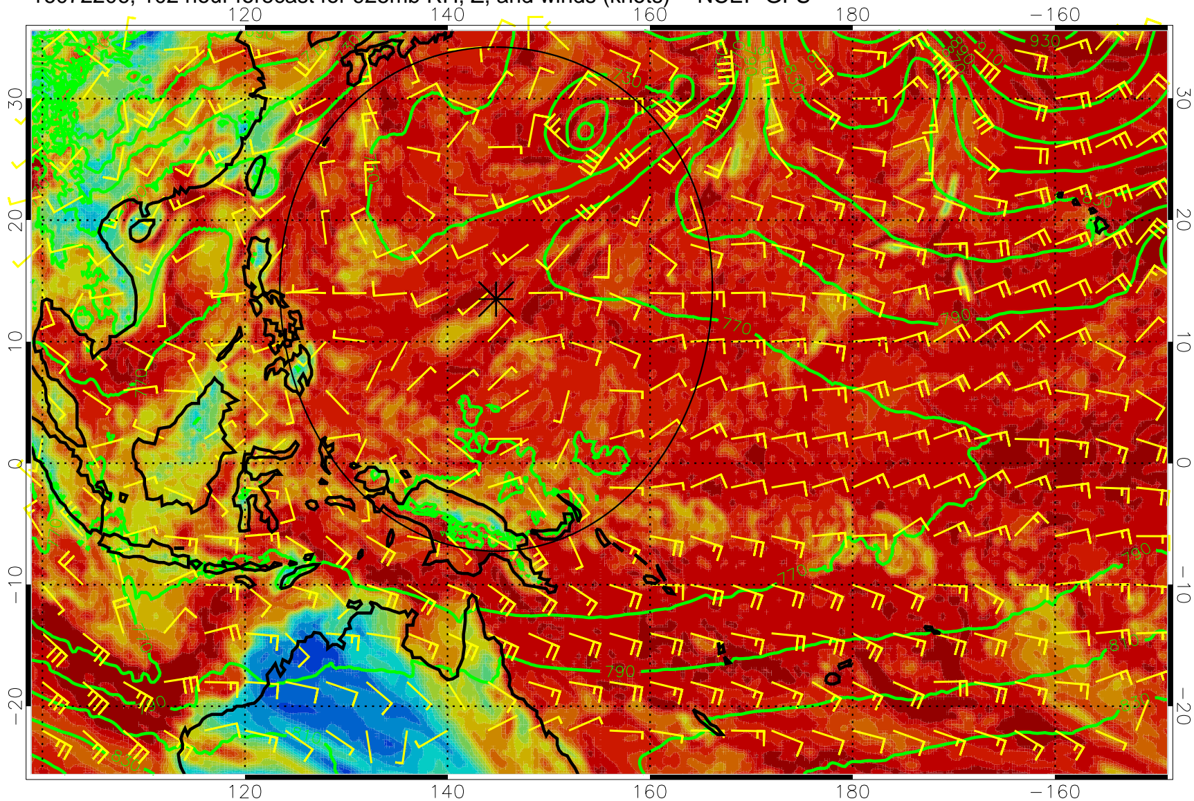
16072206, 102 hour forecast for 925mb RH, Z, and winds (knots) -- NCEP GFS
