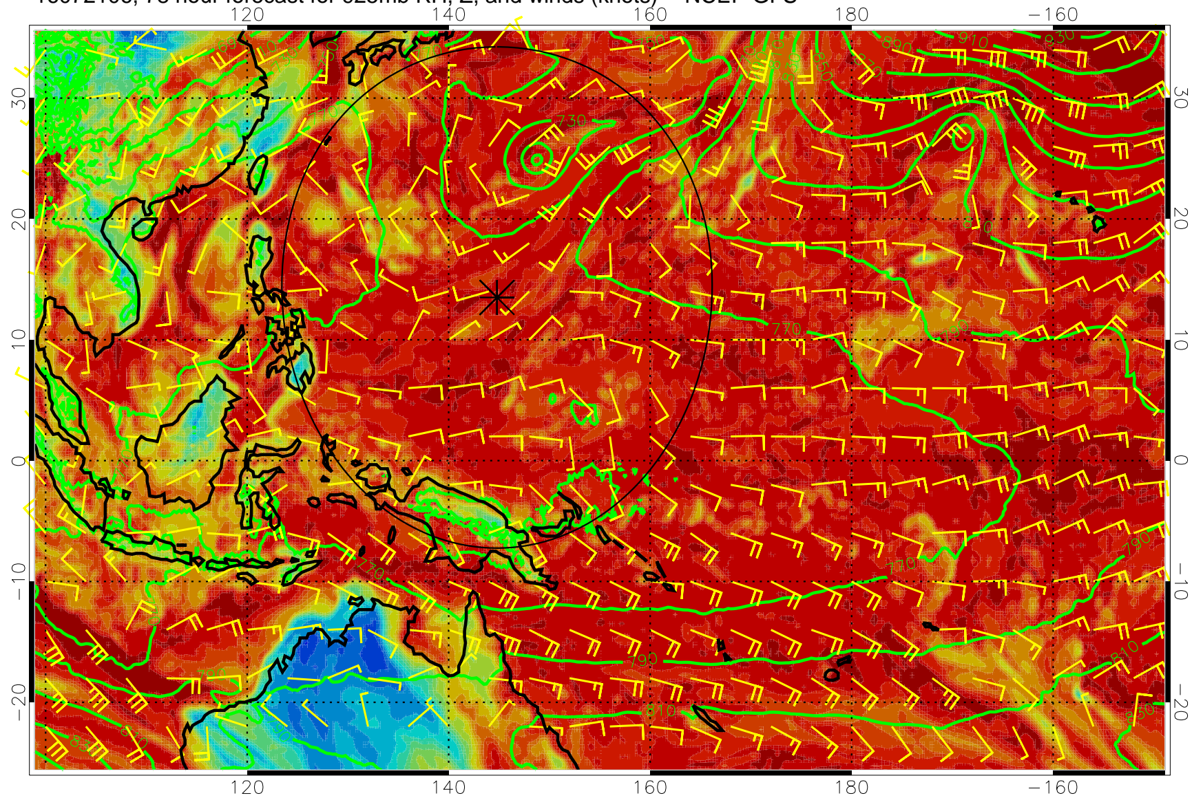
16072106, 78 hour forecast for 925mb RH, Z, and winds (knots) -- NCEP GFS
