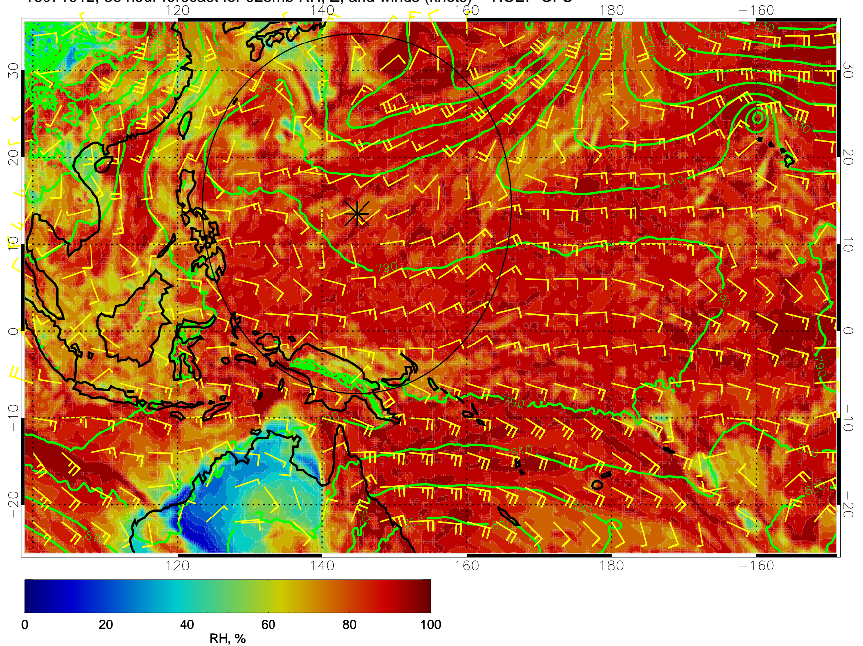
16071912, 36 hour forecast for 925mb RH, Z, and winds (knots) -- NCEP GFS
