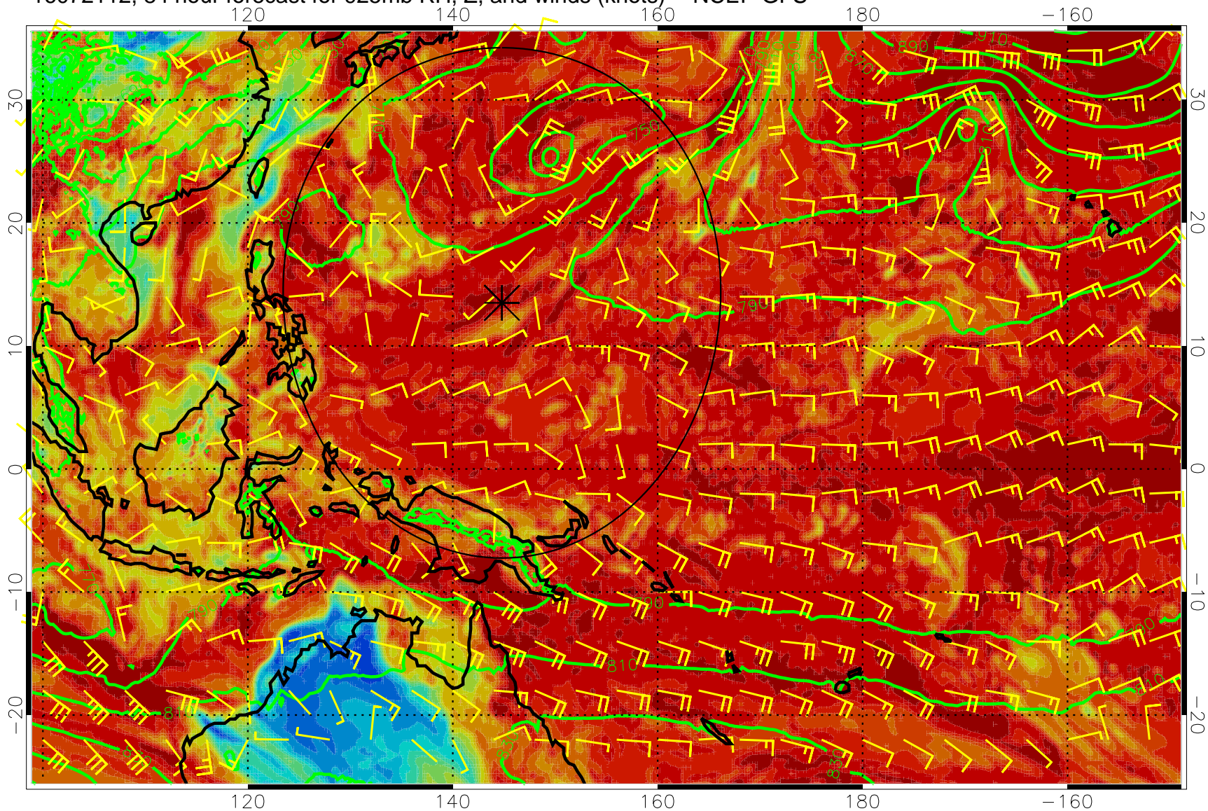
16072112, 84 hour forecast for 925mb RH, Z, and winds (knots) -- NCEP GFS
