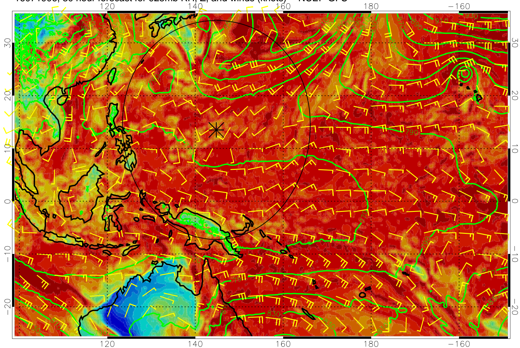
16071906, 30 hour forecast for 925mb RH, Z, and winds (knots) -- NCEP GFS
