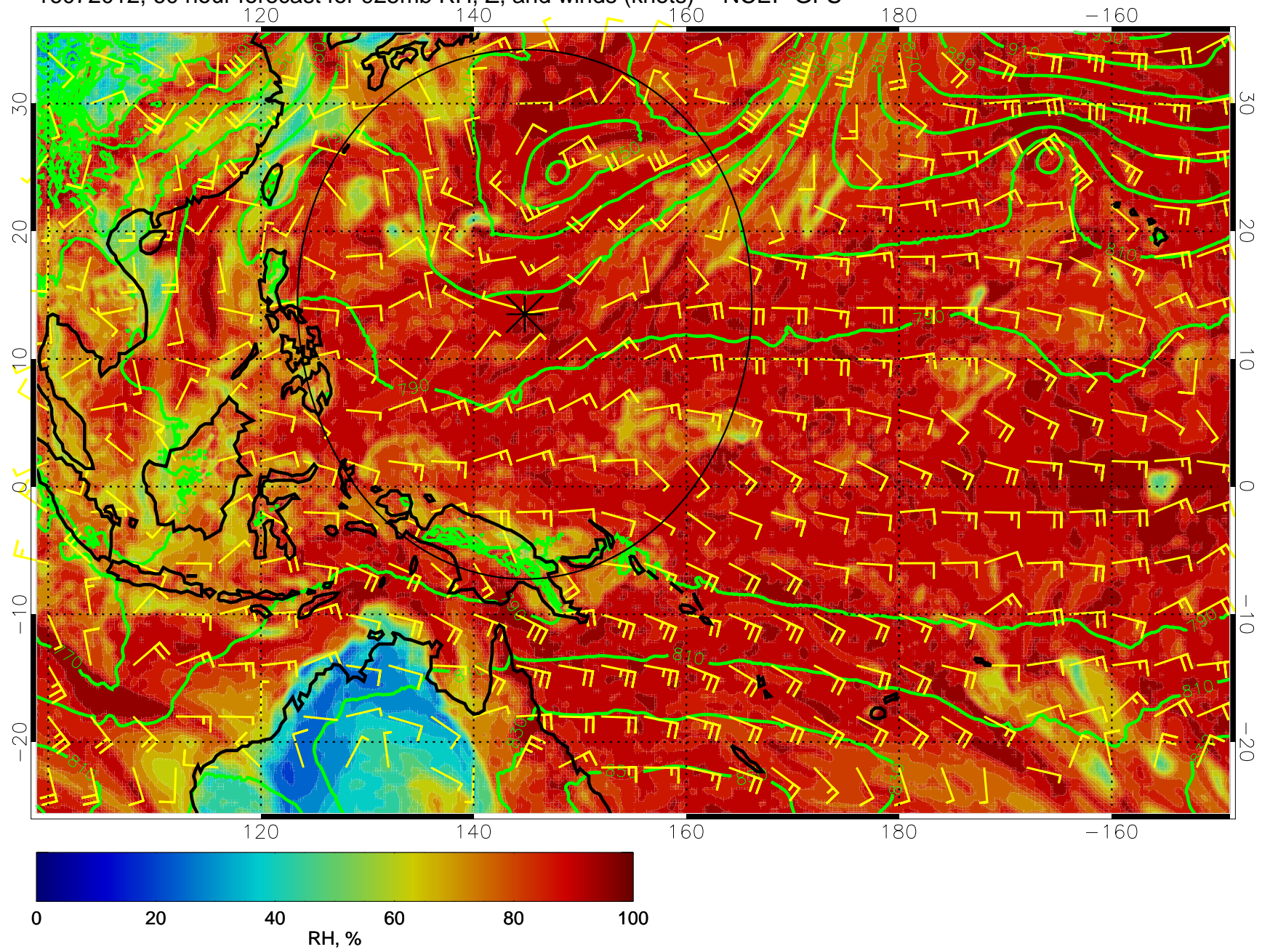
16072012, 60 hour forecast for 925mb RH, Z, and winds (knots) -- NCEP GFS
