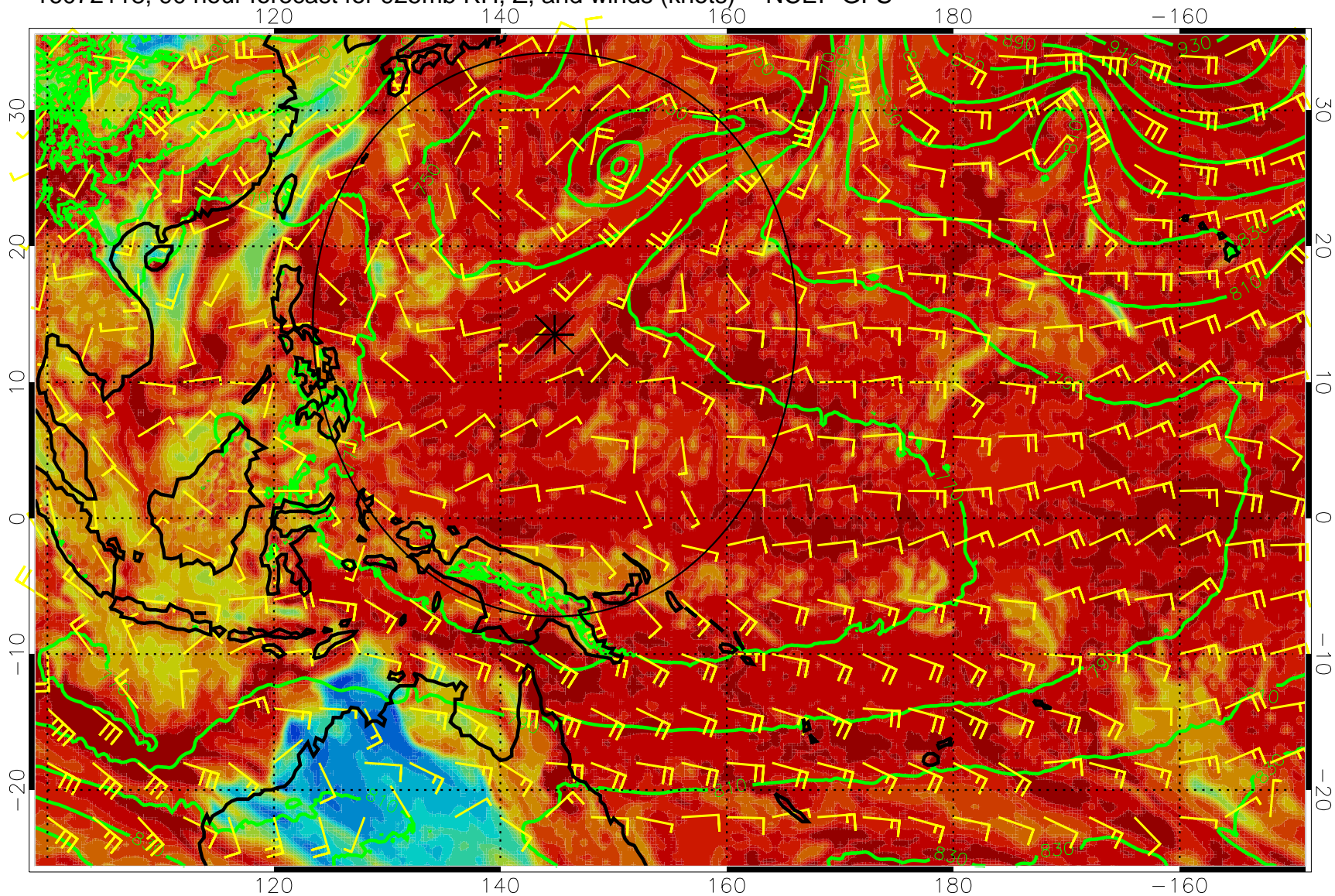
16072118, 90 hour forecast for 925mb RH, Z, and winds (knots) -- NCEP GFS
