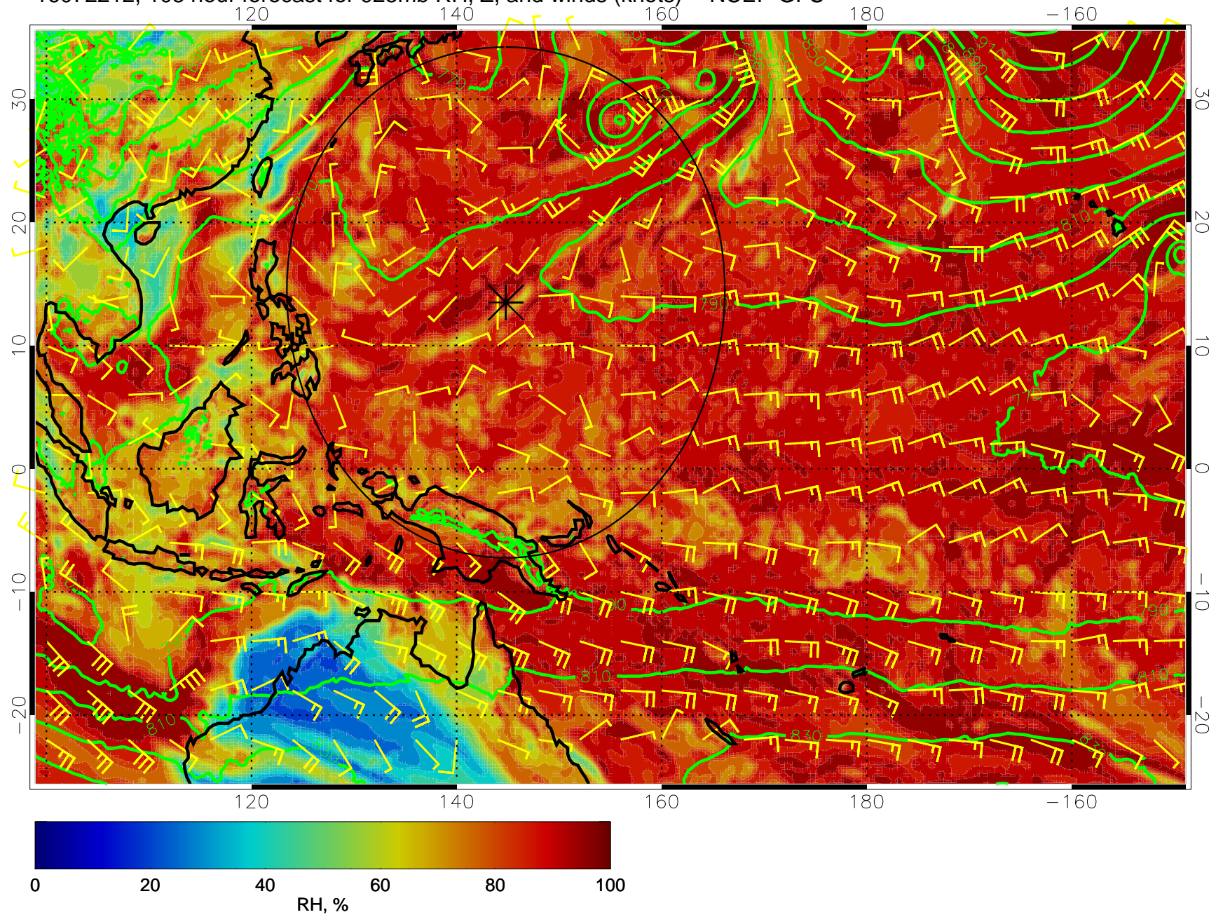
16072212, 108 hour forecast for 925mb RH, Z, and winds (knots) -- NCEP GFS
