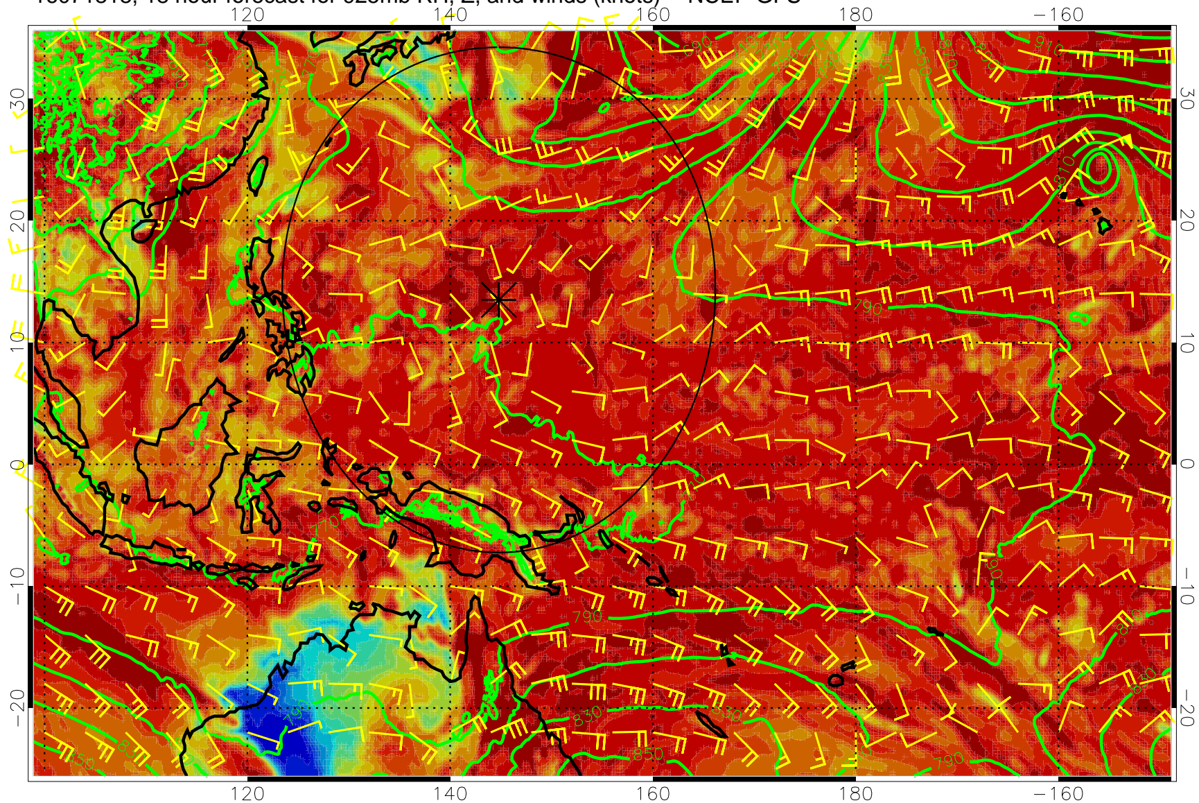
16071818, 18 hour forecast for 925mb RH, Z, and winds (knots) -- NCEP GFS
