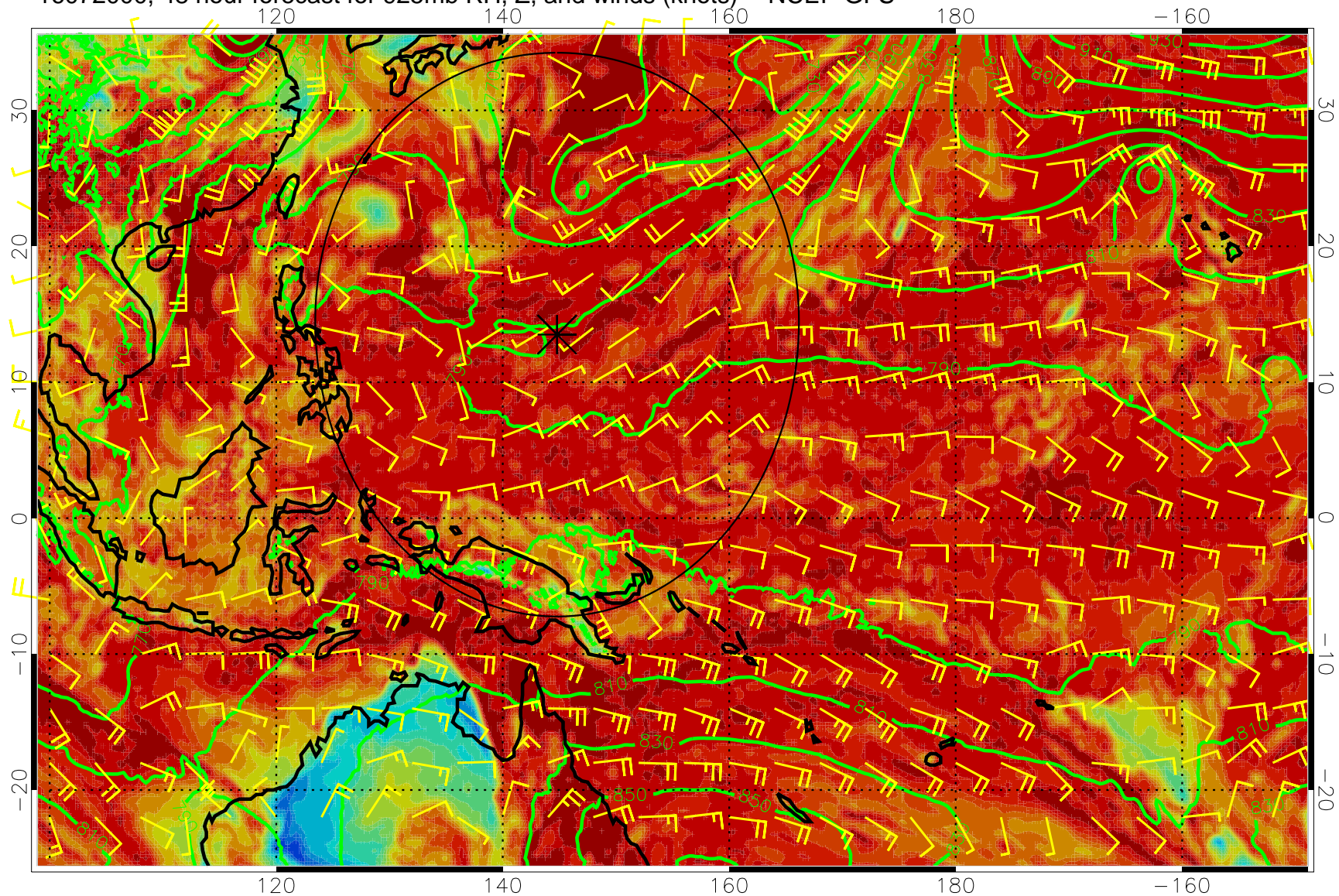
16072000, 48 hour forecast for 925mb RH, Z, and winds (knots) -- NCEP GFS
