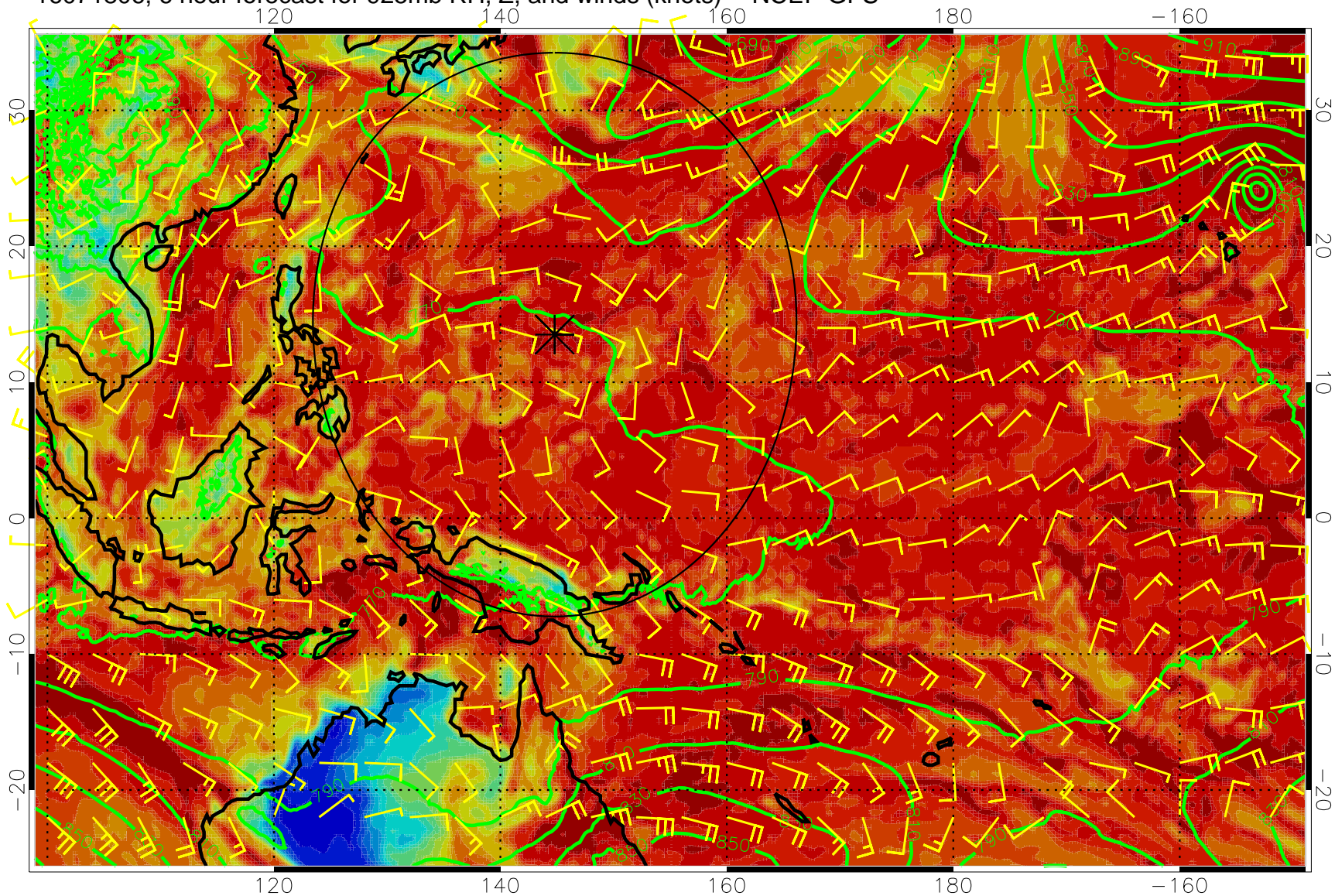
16071806, 6 hour forecast for 925mb RH, Z, and winds (knots) -- NCEP GFS
