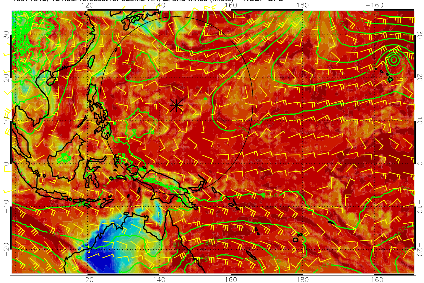
16071812, 12 hour forecast for 925mb RH, Z, and winds (knots) -- NCEP GFS
