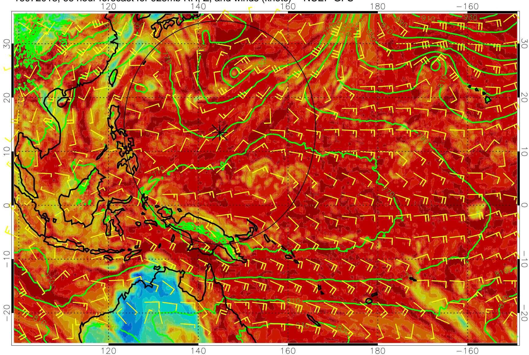
16072018, 66 hour forecast for 925mb RH, Z, and winds (knots) -- NCEP GFS
