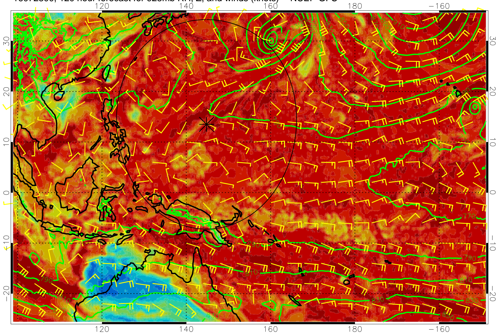
16072300, 120 hour forecast for 925mb RH, Z, and winds (knots) -- NCEP GFS
