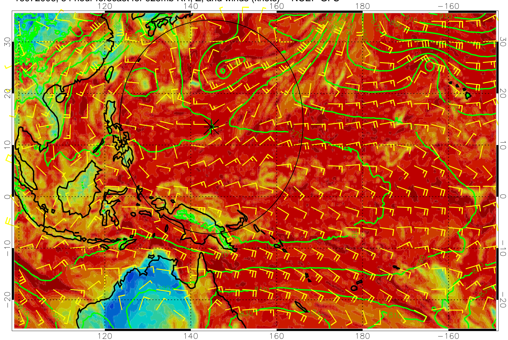
16072006, 54 hour forecast for 925mb RH, Z, and winds (knots) -- NCEP GFS
