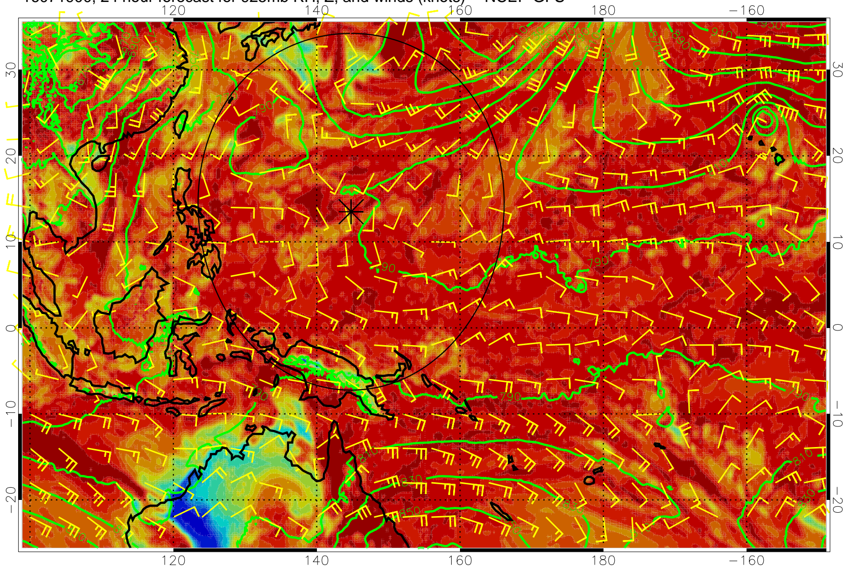
16071900, 24 hour forecast for 925mb RH, Z, and winds (knots) -- NCEP GFS
