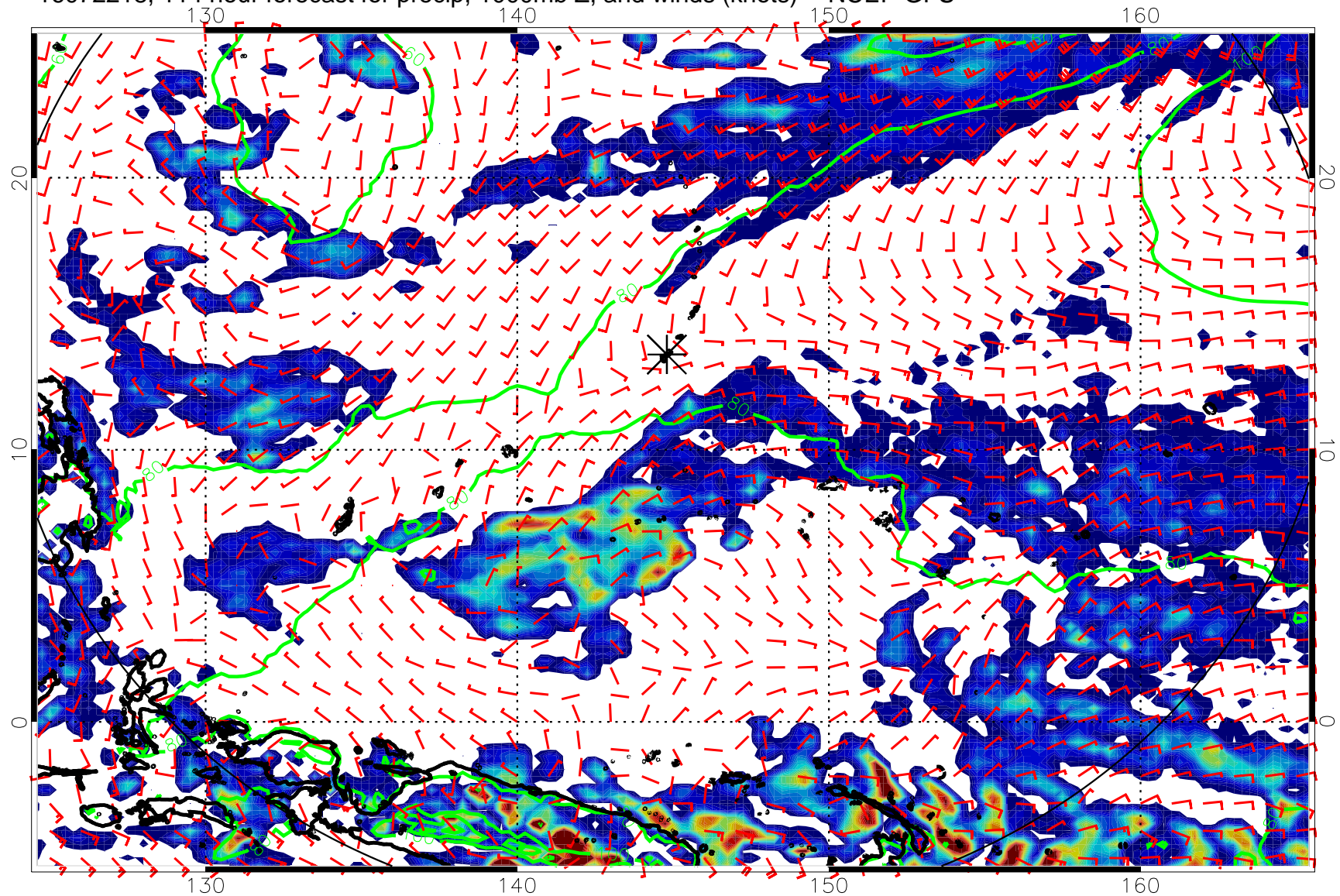
16072218, 114 hour forecast for precip, 1000mb Z, and winds (knots) -- NCEP GFS
