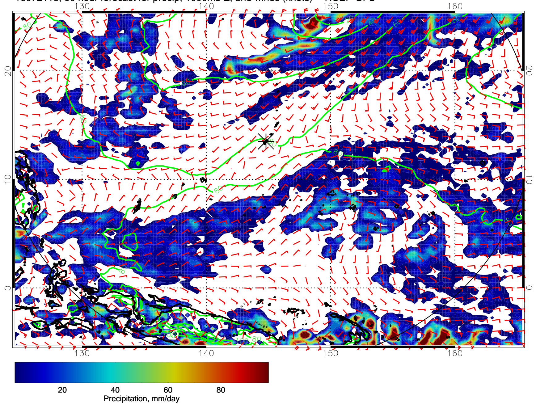
16072118, 90 hour forecast for precip, 1000mb Z, and winds (knots) -- NCEP GFS
