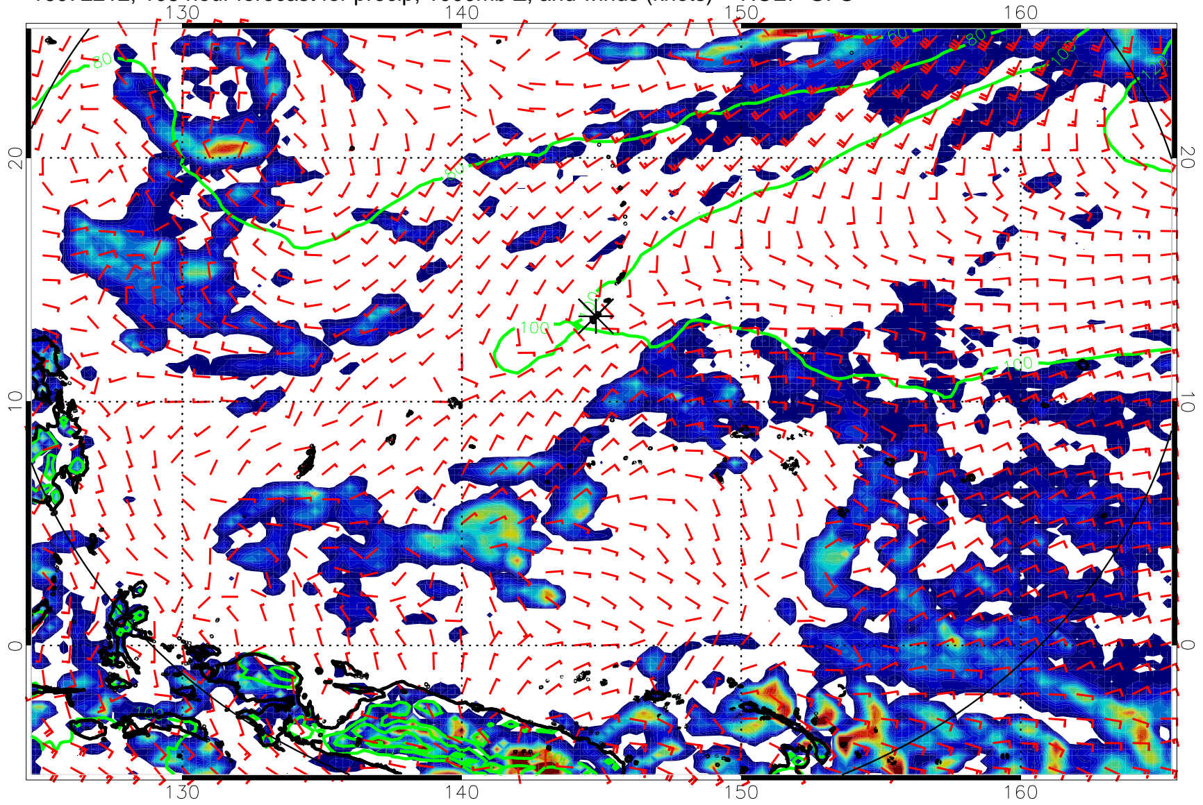
16072212, 108 hour forecast for precip, 1000mb Z, and winds (knots) -- NCEP GFS
