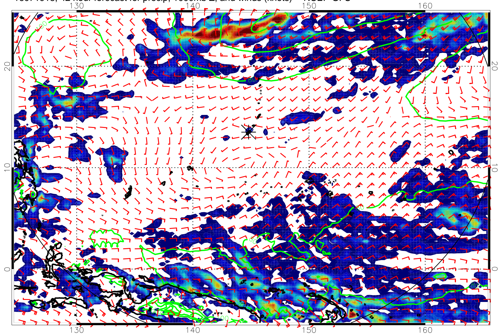
16071918, 42 hour forecast for precip, 1000mb Z, and winds (knots) -- NCEP GFS
