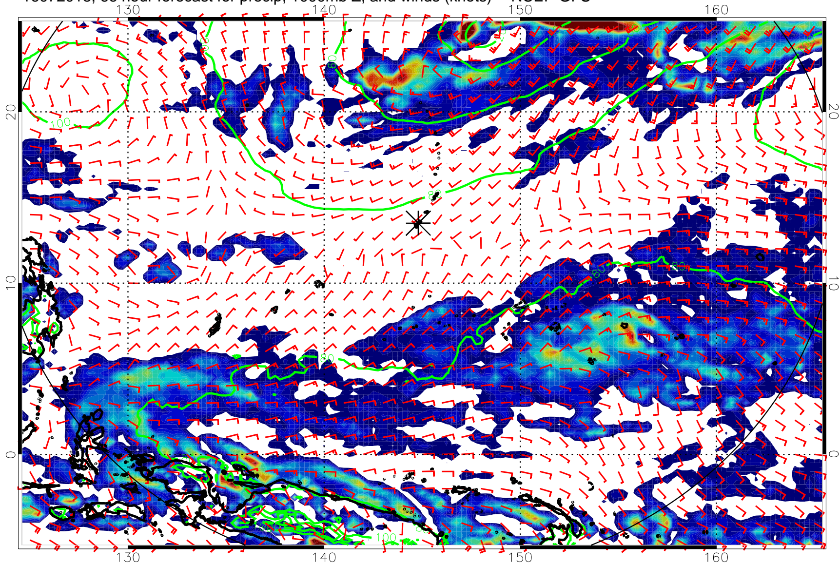
16072018, 66 hour forecast for precip, 1000mb Z, and winds (knots) -- NCEP GFS
