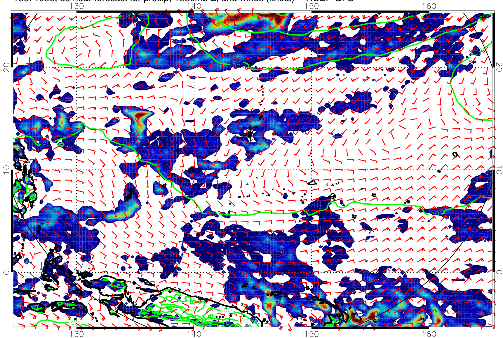
16071906, 30 hour forecast for precip, 1000mb Z, and winds (knots) -- NCEP GFS
