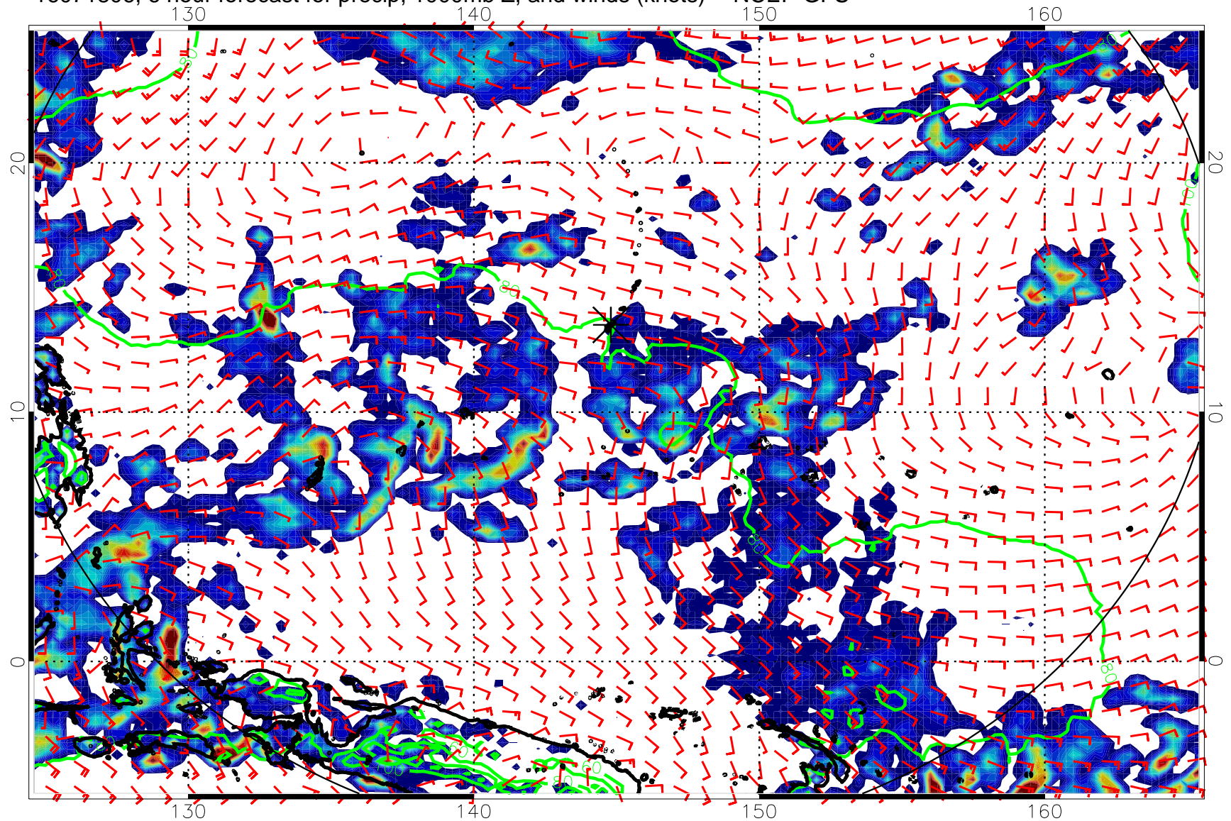
16071806, 6 hour forecast for precip, 1000mb Z, and winds (knots) -- NCEP GFS
