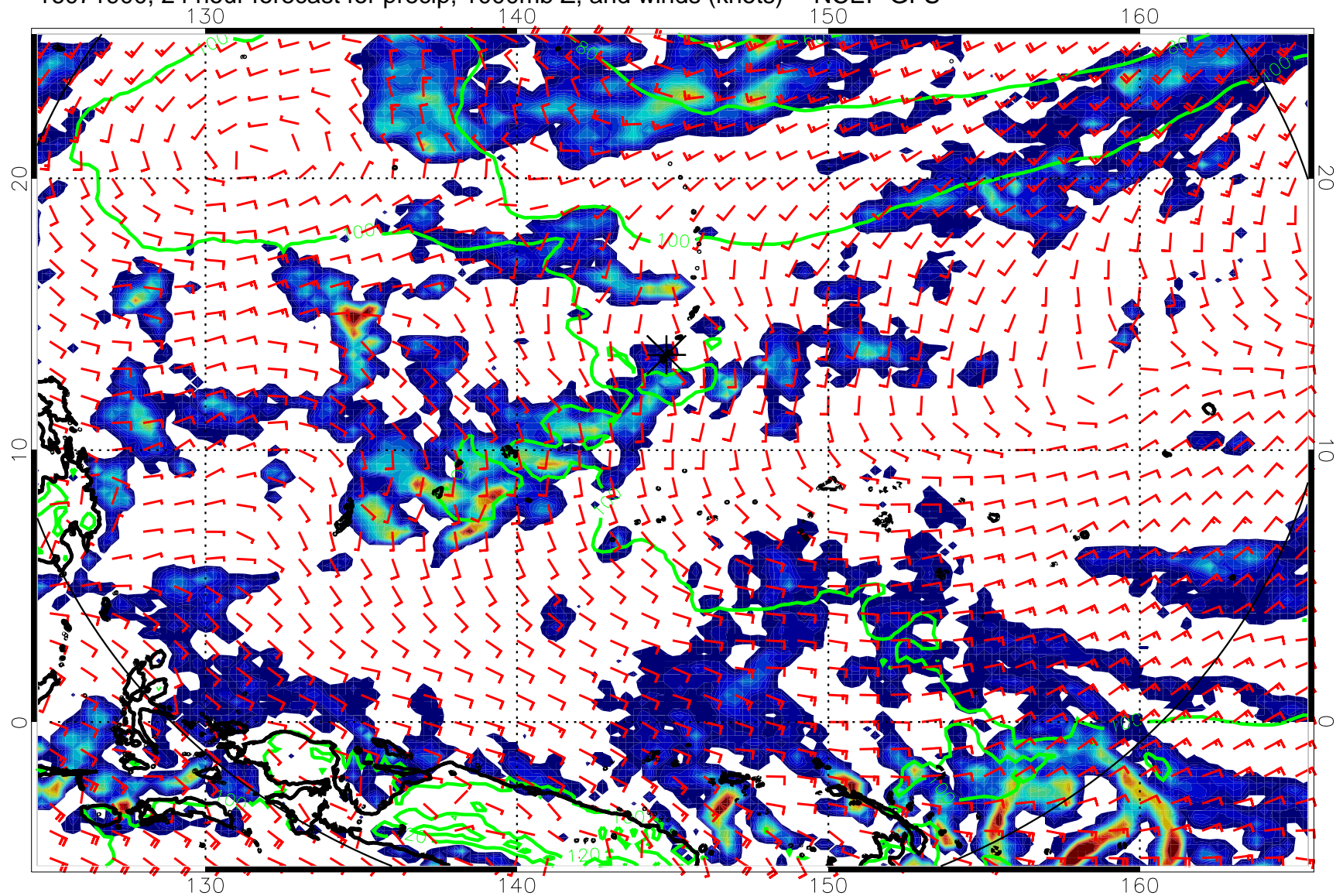
16071900, 24 hour forecast for precip, 1000mb Z, and winds (knots) -- NCEP GFS
