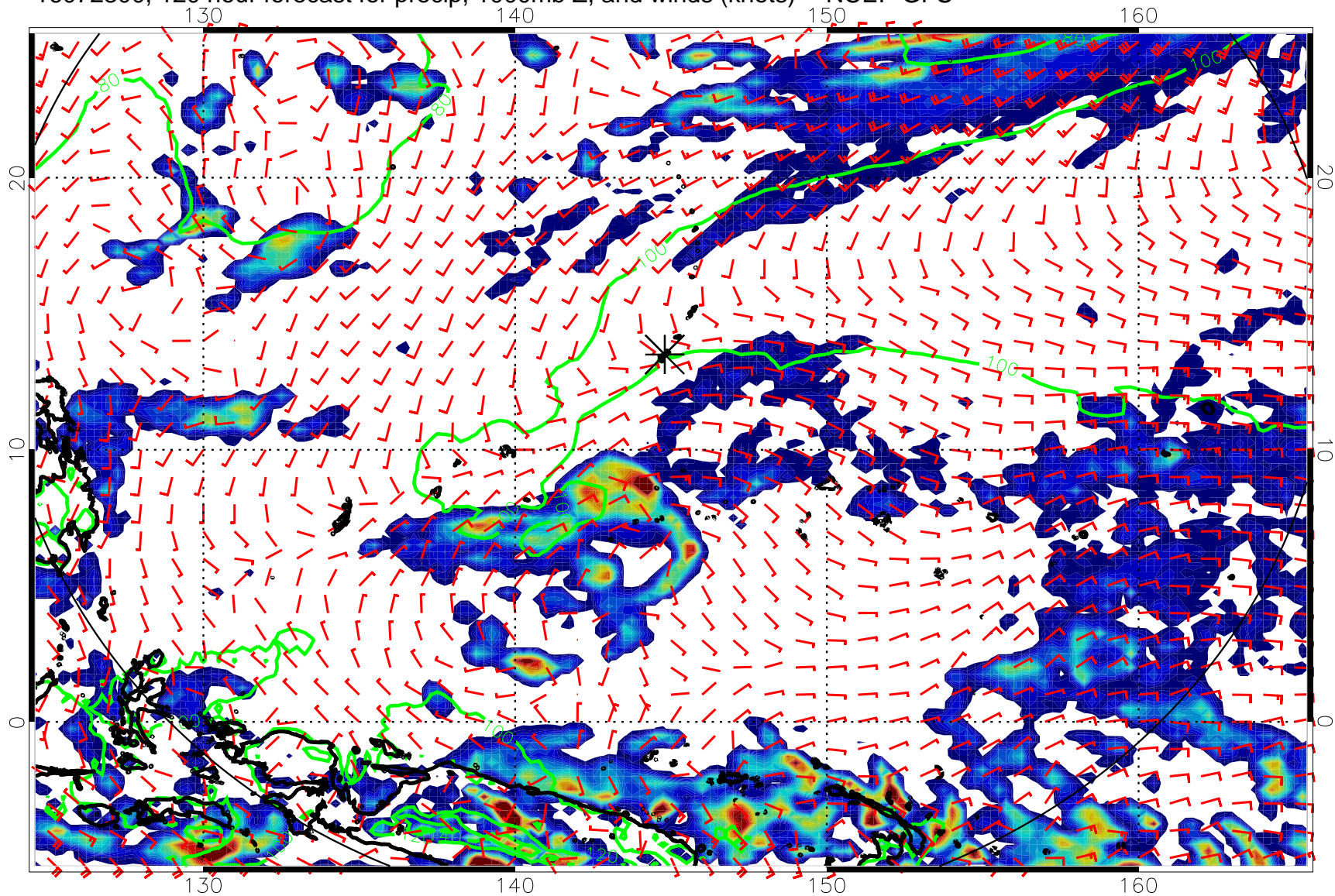
16072300, 120 hour forecast for precip, 1000mb Z, and winds (knots) -- NCEP GFS
