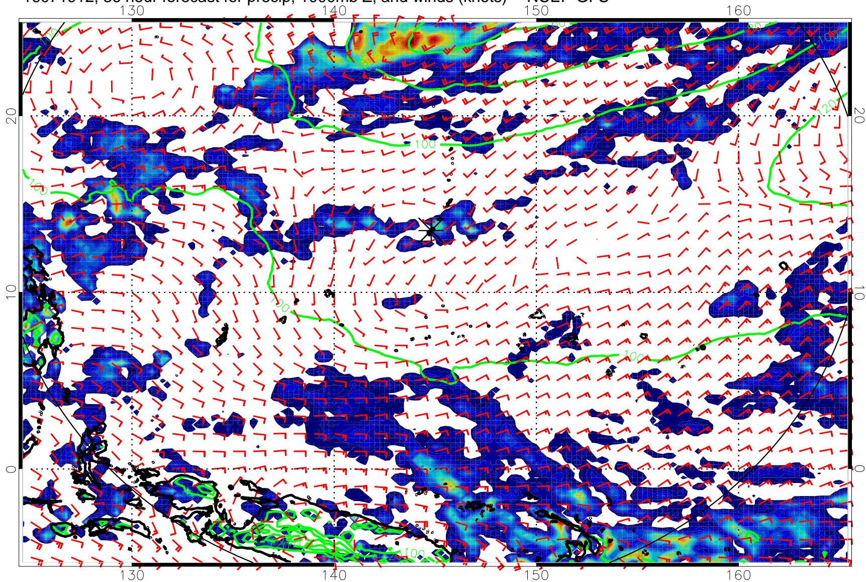
16071912, 36 hour forecast for precip, 1000mb Z, and winds (knots) -- NCEP GFS
