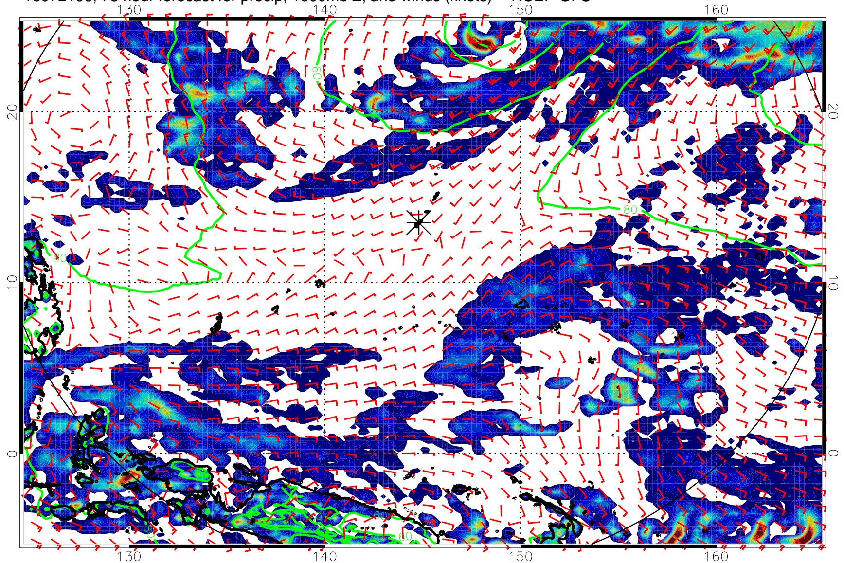
16072106, 78 hour forecast for precip, 1000mb Z, and winds (knots) -- NCEP GFS
