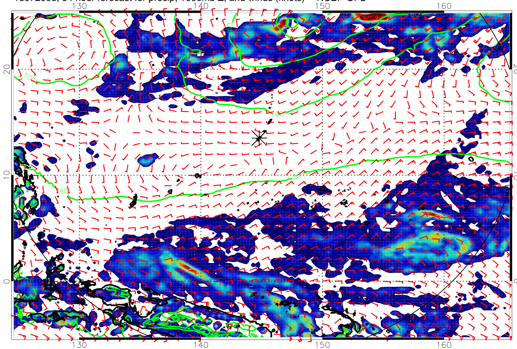
16072006, 54 hour forecast for precip, 1000mb Z, and winds (knots) -- NCEP GFS
