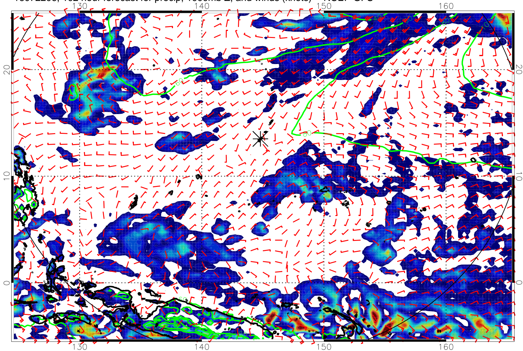
16072206, 102 hour forecast for precip, 1000mb Z, and winds (knots) -- NCEP GFS
