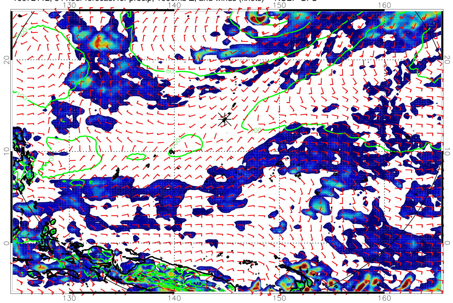
16072112, 84 hour forecast for precip, 1000mb Z, and winds (knots) -- NCEP GFS
