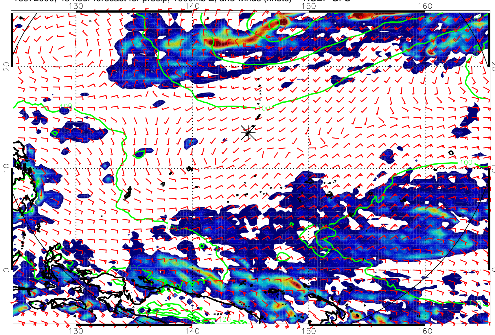
16072000, 48 hour forecast for precip, 1000mb Z, and winds (knots) -- NCEP GFS
