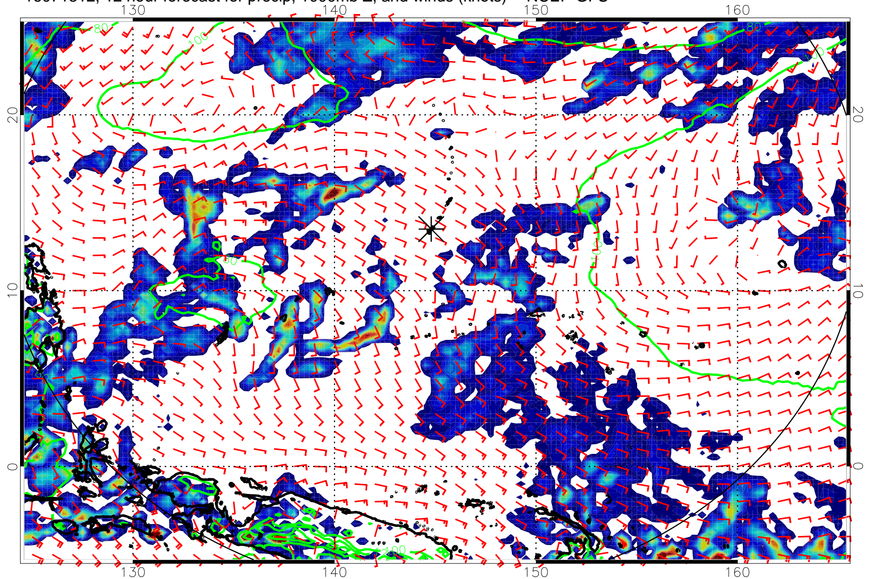
16071812, 12 hour forecast for precip, 1000mb Z, and winds (knots) -- NCEP GFS
