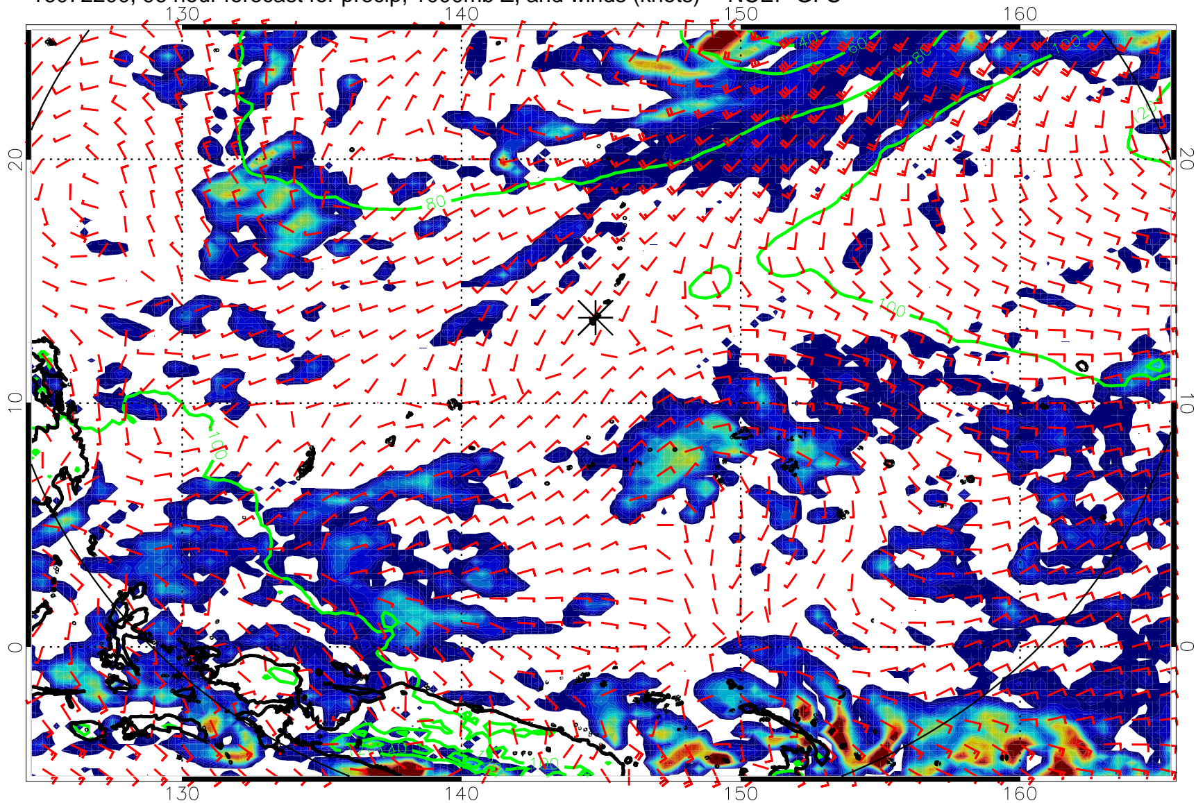
16072200, 96 hour forecast for precip, 1000mb Z, and winds (knots) -- NCEP GFS
