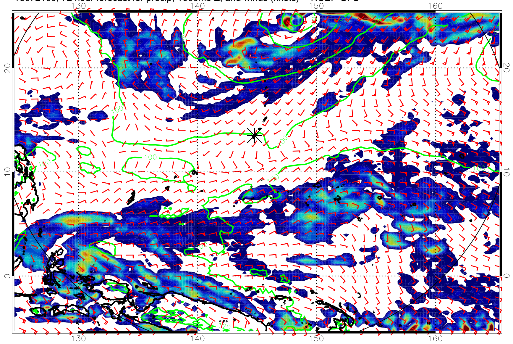
16072100, 72 hour forecast for precip, 1000mb Z, and winds (knots) -- NCEP GFS
