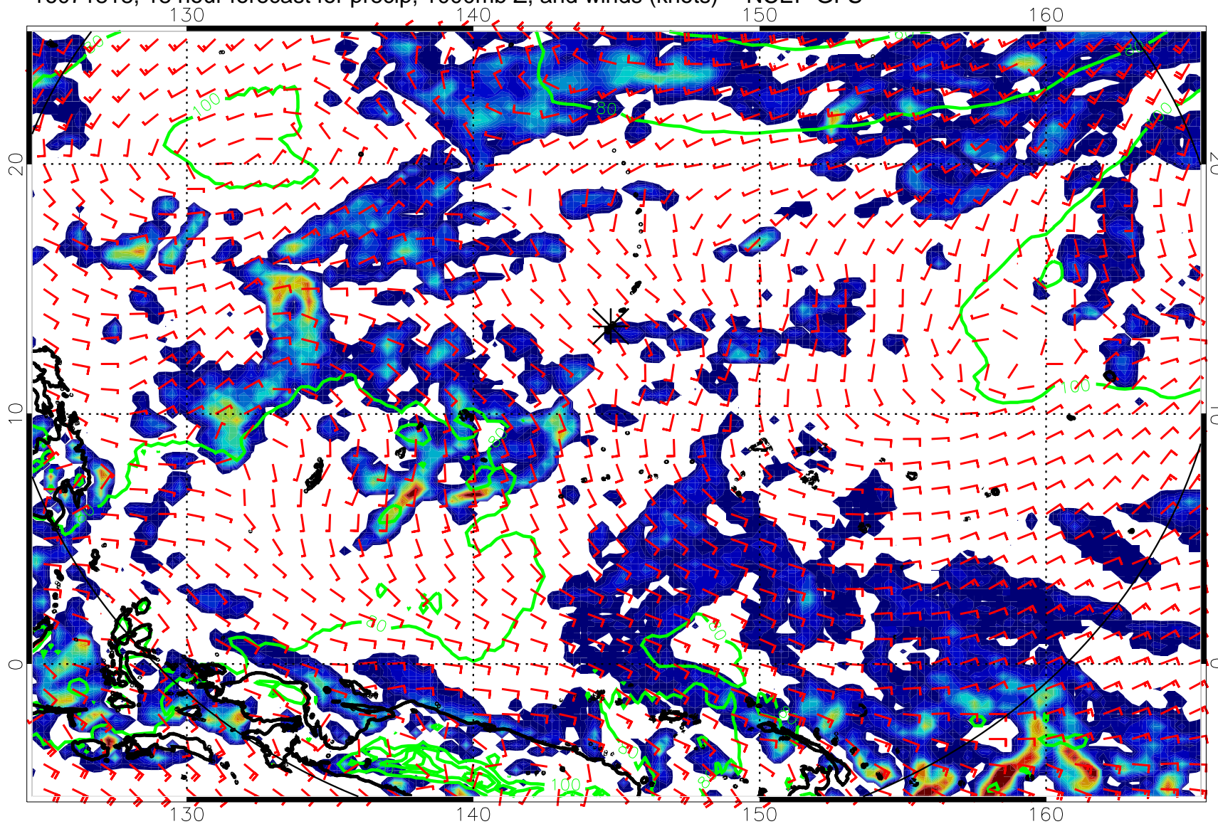
16071818, 18 hour forecast for precip, 1000mb Z, and winds (knots) -- NCEP GFS
