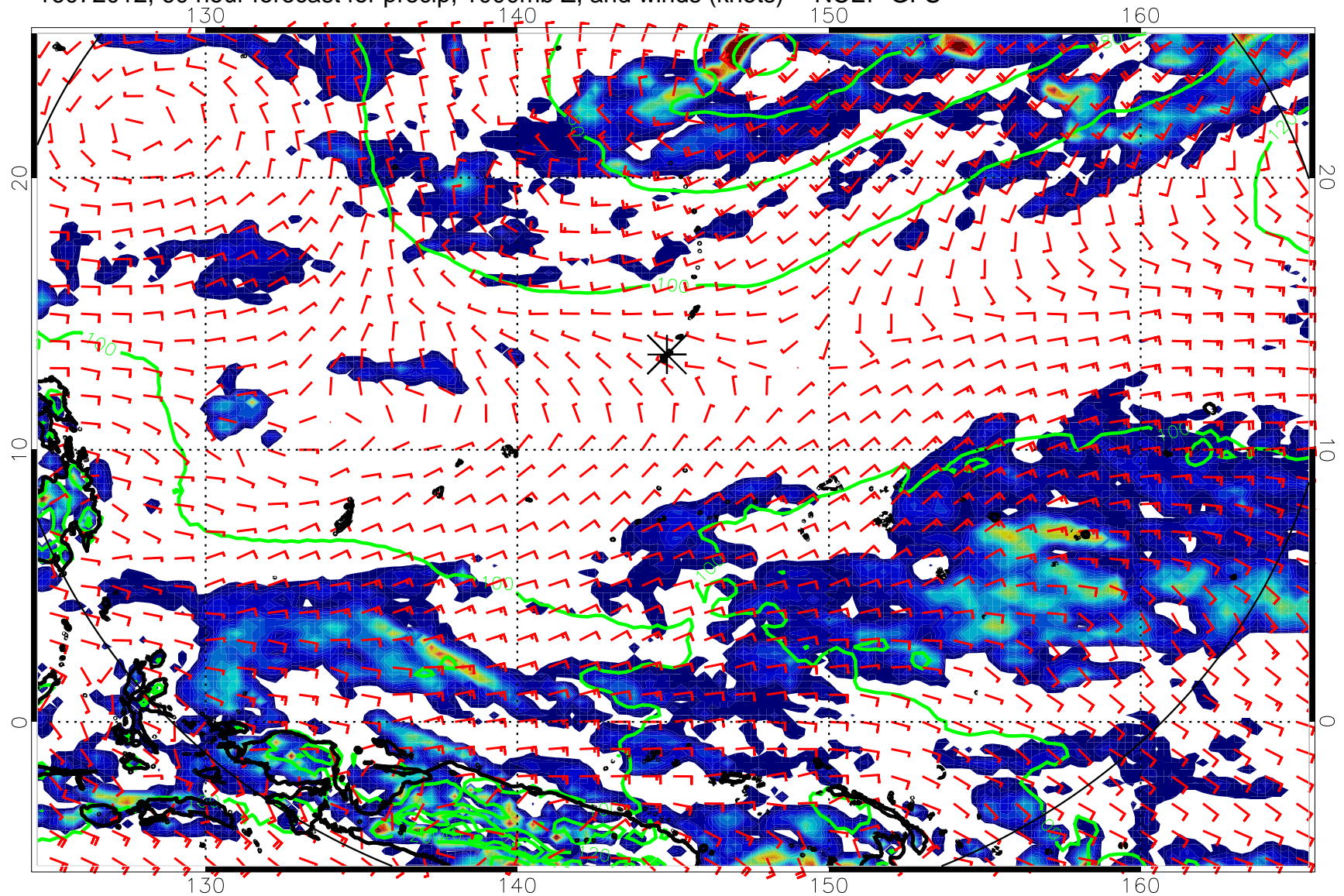
16072012, 60 hour forecast for precip, 1000mb Z, and winds (knots) -- NCEP GFS
