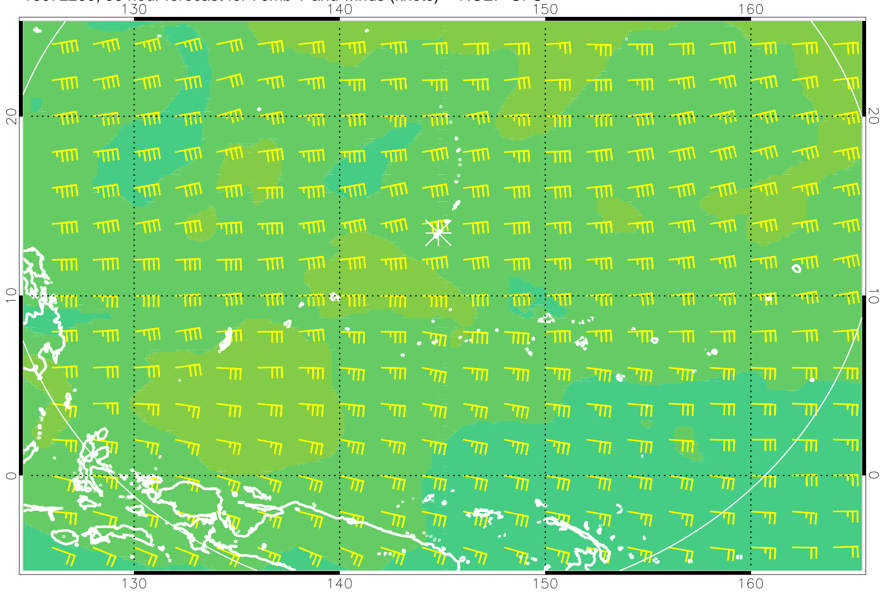
16072200, 96 hour forecast for 70mb T and winds (knots) -- NCEP GFS
