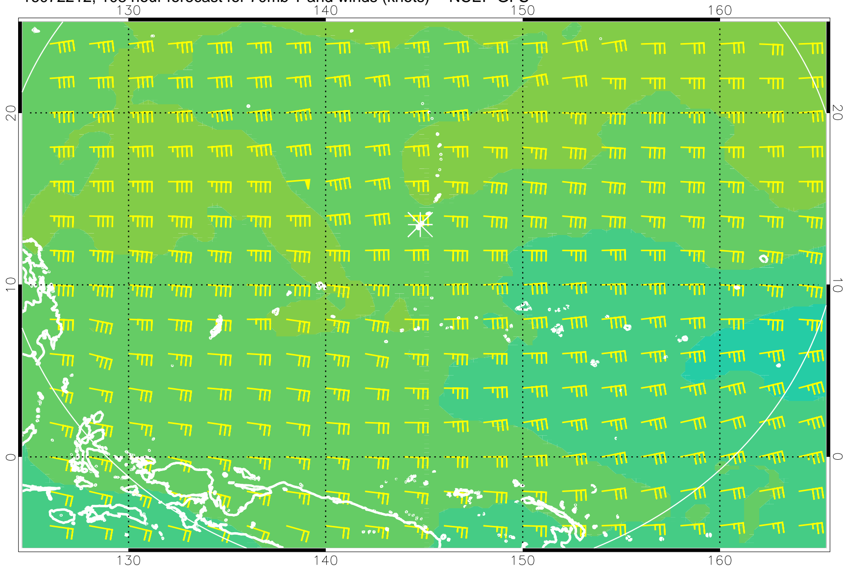
16072212, 108 hour forecast for 70mb T and winds (knots) -- NCEP GFS
