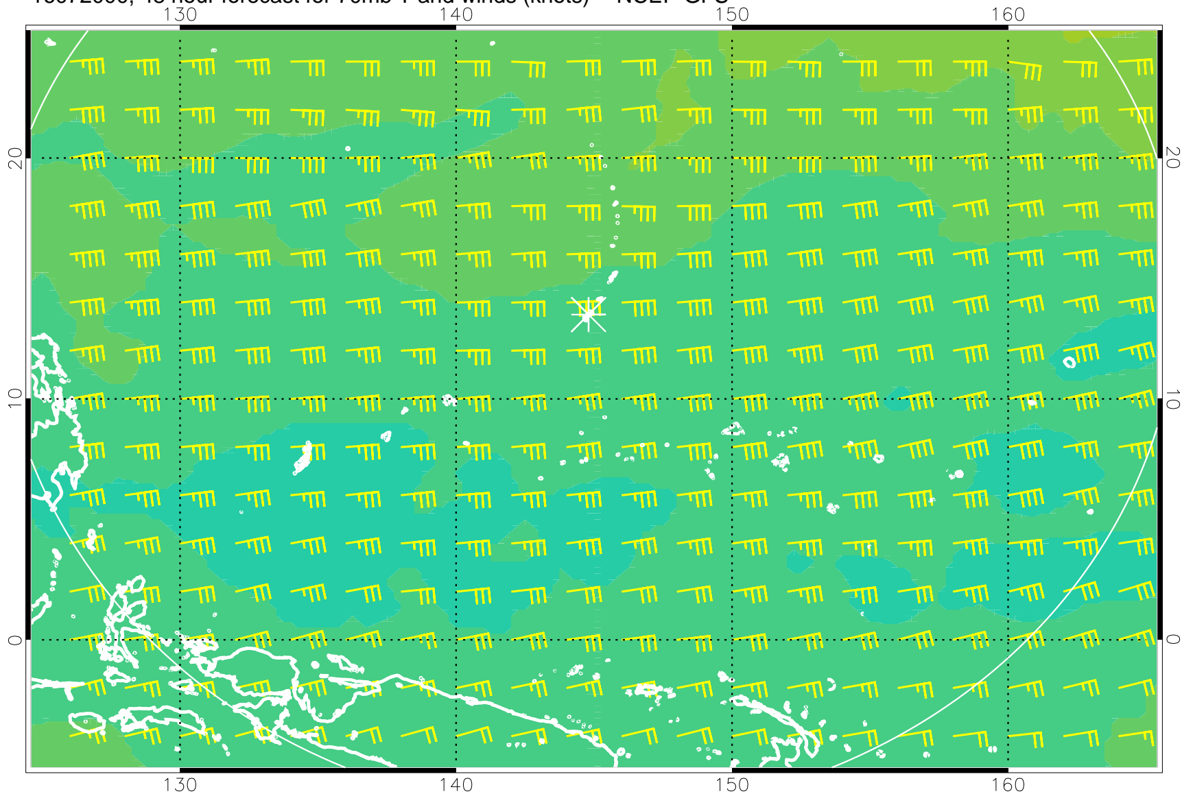
16072000, 48 hour forecast for 70mb T and winds (knots) -- NCEP GFS
