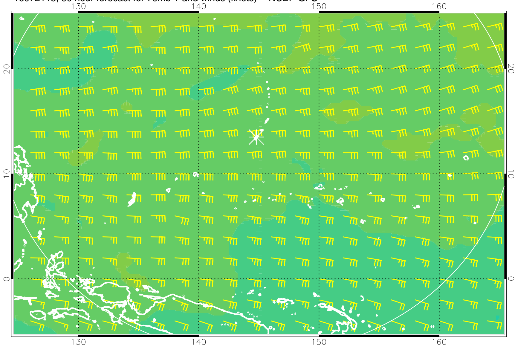
16072118, 90 hour forecast for 70mb T and winds (knots) -- NCEP GFS
