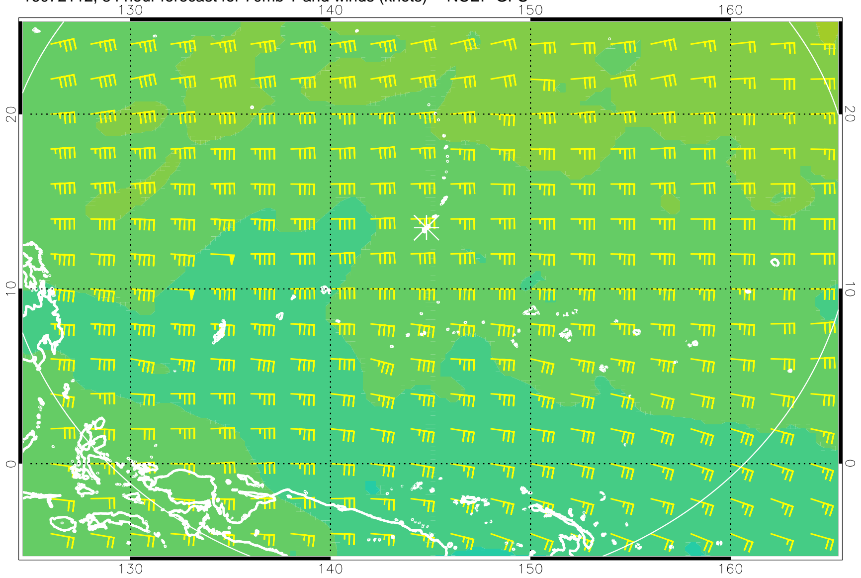
16072112, 84 hour forecast for 70mb T and winds (knots) -- NCEP GFS
