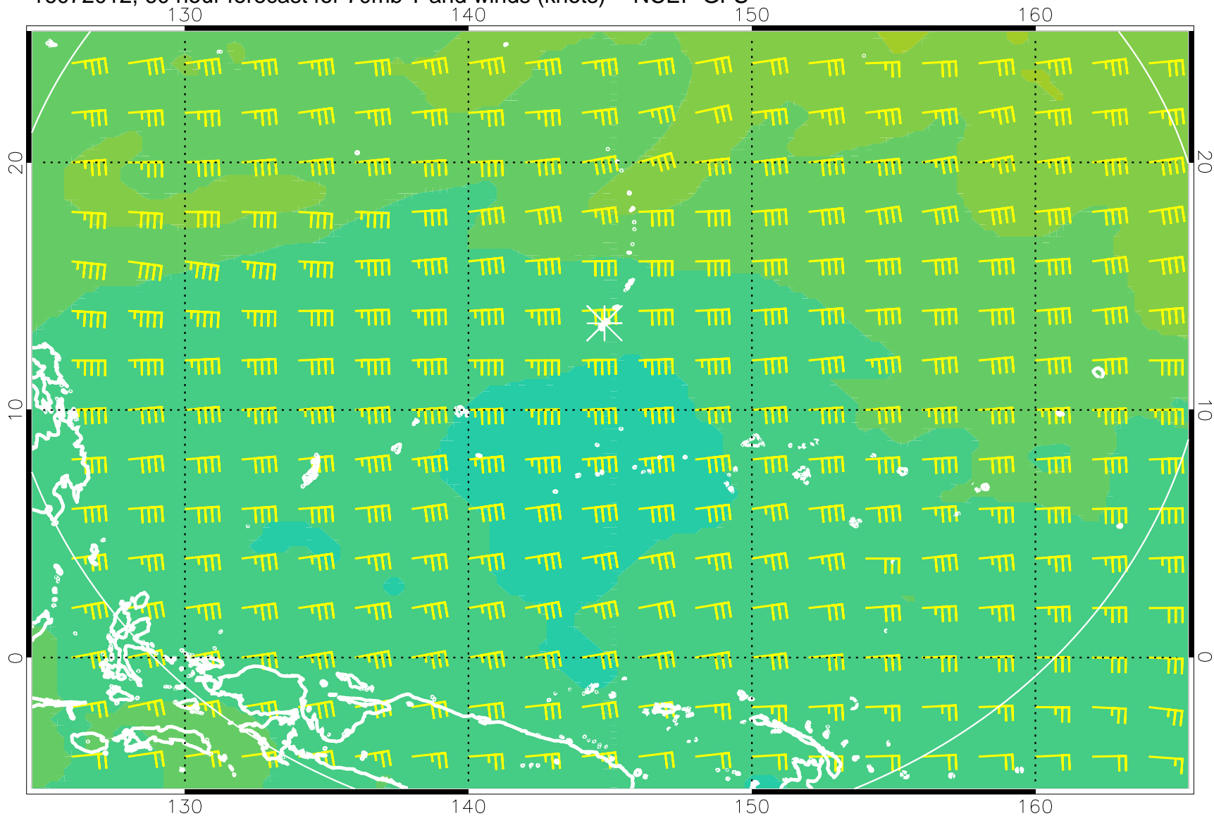
16072012, 60 hour forecast for 70mb T and winds (knots) -- NCEP GFS
