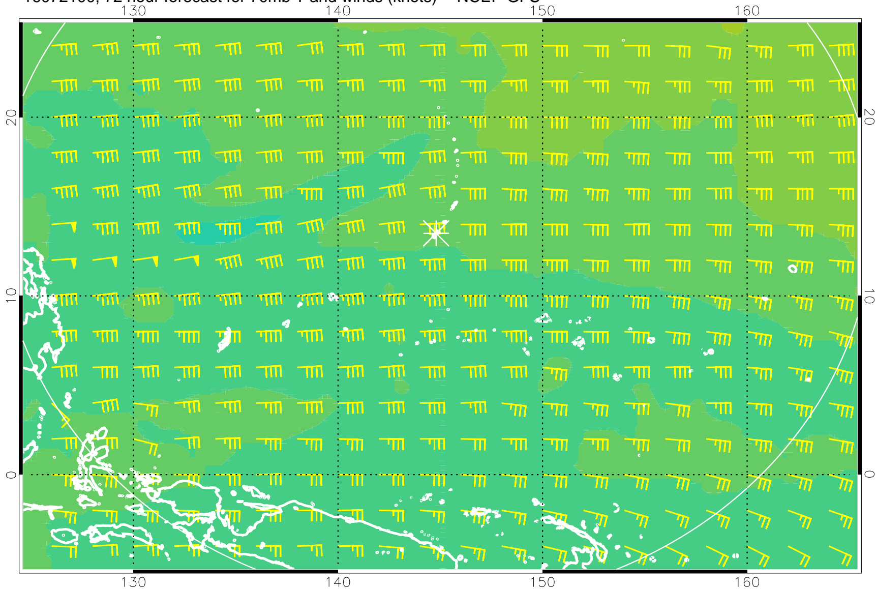
16072100, 72 hour forecast for 70mb T and winds (knots) -- NCEP GFS
