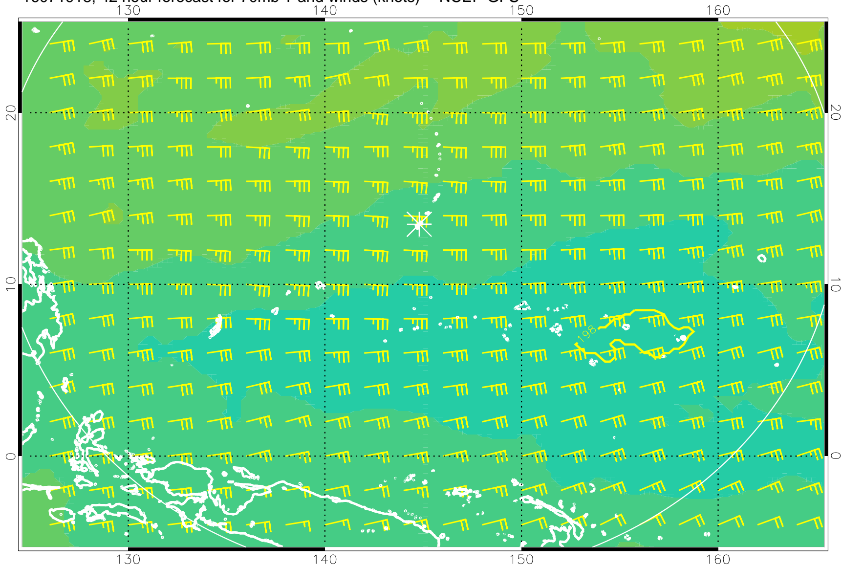
16071918, 42 hour forecast for 70mb T and winds (knots) -- NCEP GFS
