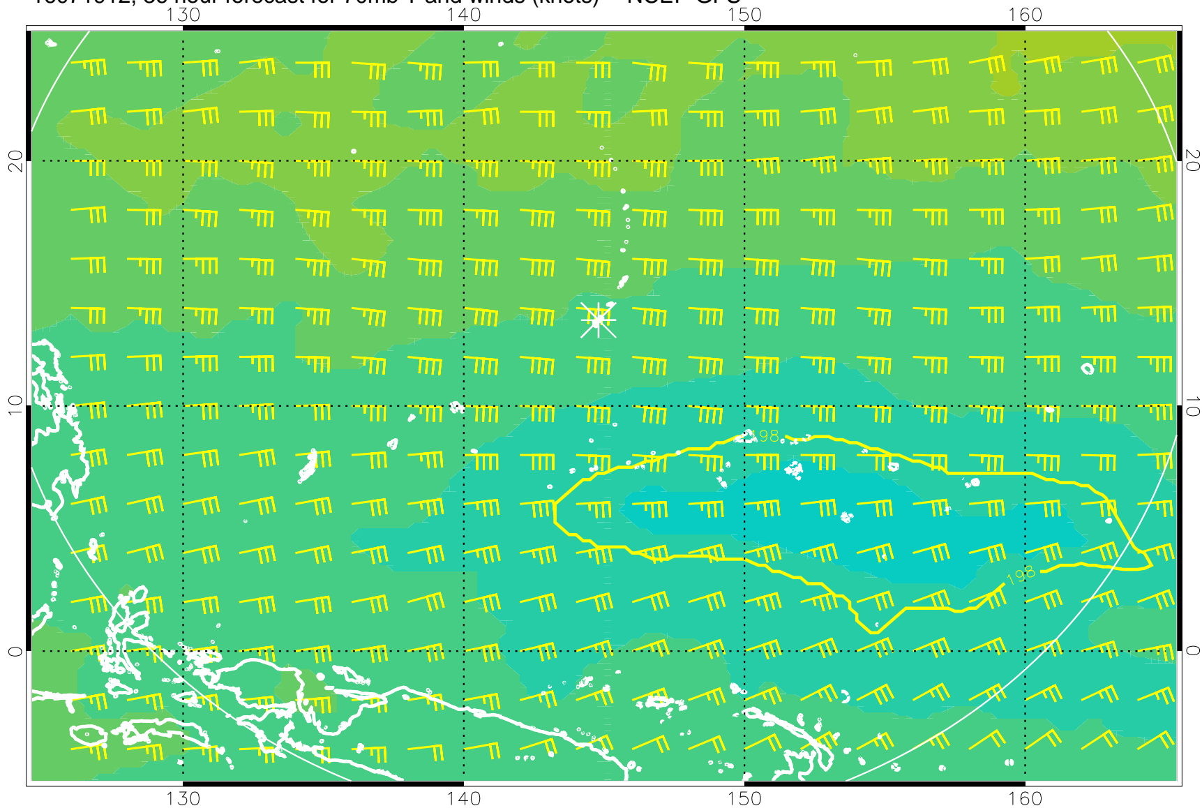
16071912, 36 hour forecast for 70mb T and winds (knots) -- NCEP GFS
