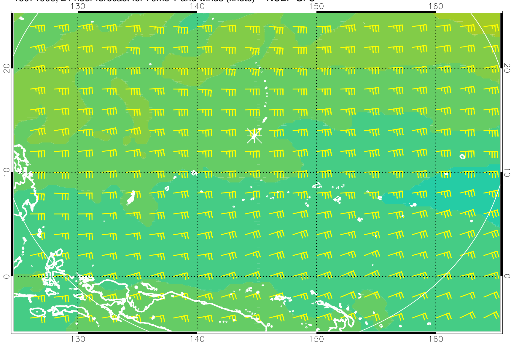
16071900, 24 hour forecast for 70mb T and winds (knots) -- NCEP GFS
