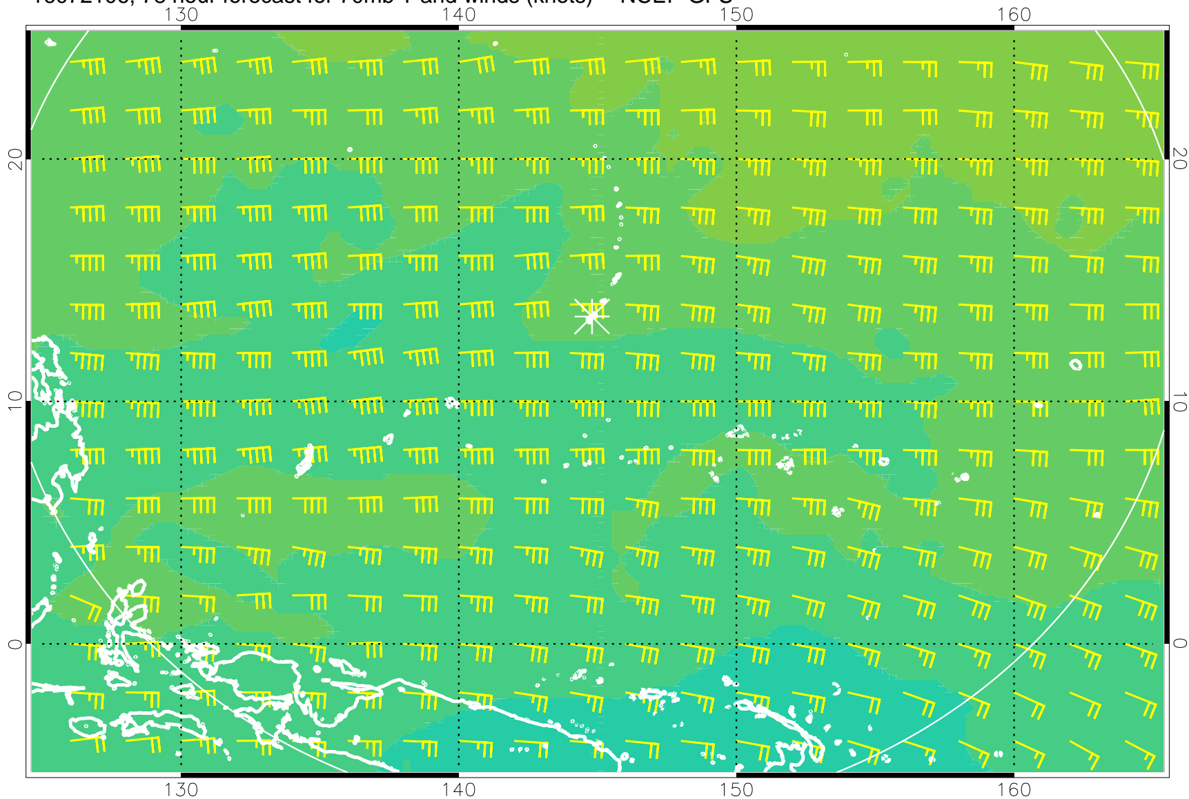
16072106, 78 hour forecast for 70mb T and winds (knots) -- NCEP GFS
