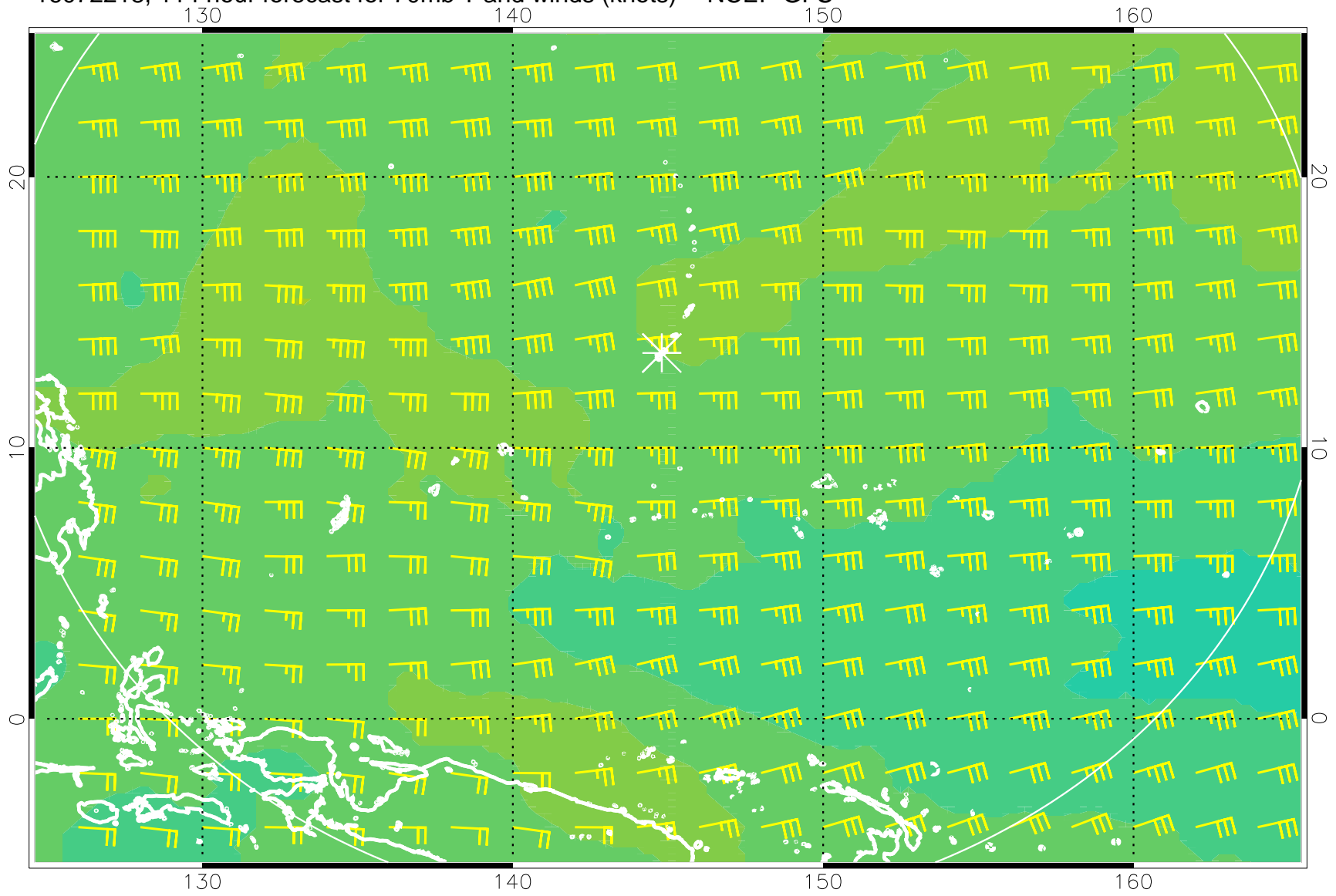
16072218, 114 hour forecast for 70mb T and winds (knots) -- NCEP GFS
