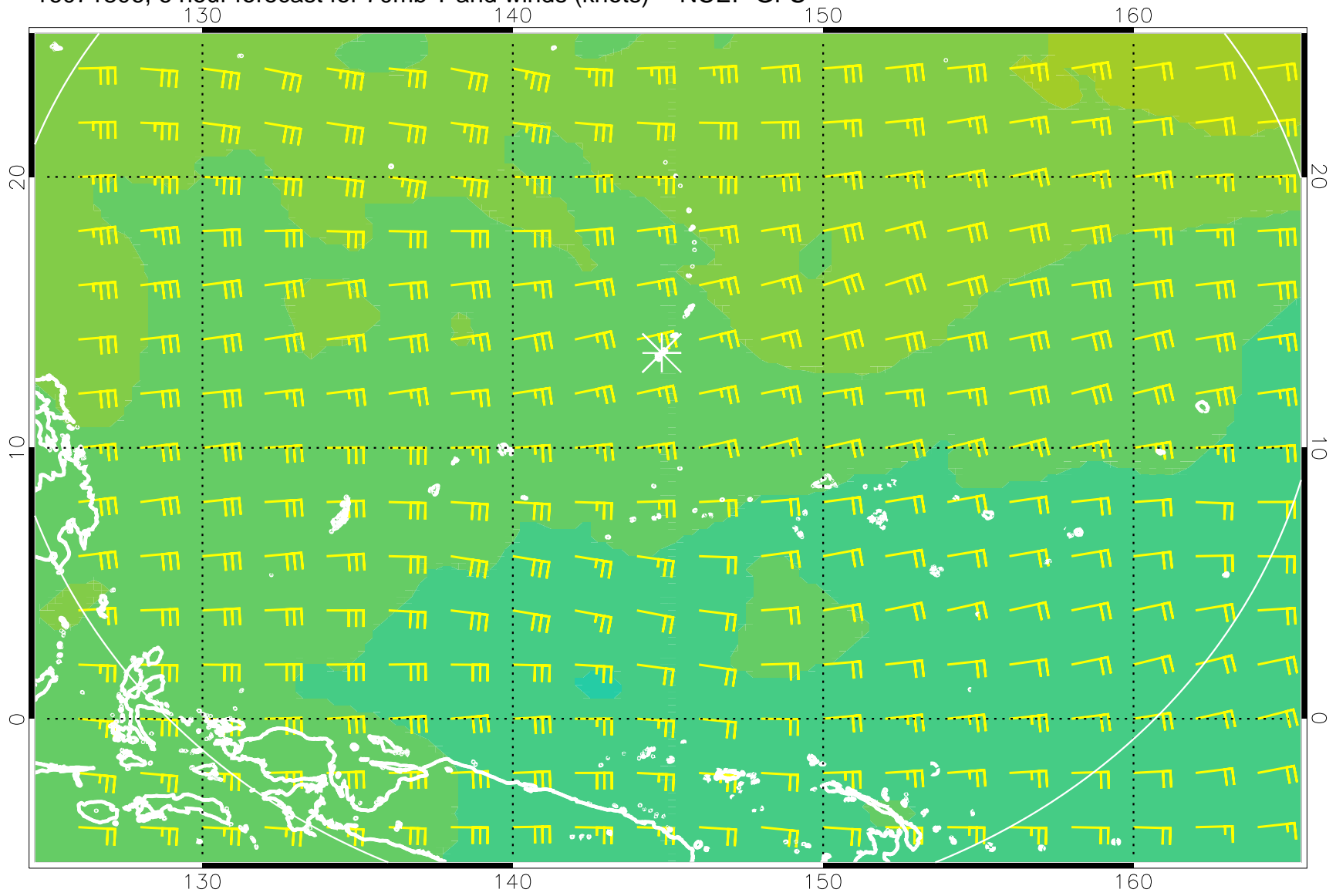
16071806, 6 hour forecast for 70mb T and winds (knots) -- NCEP GFS
