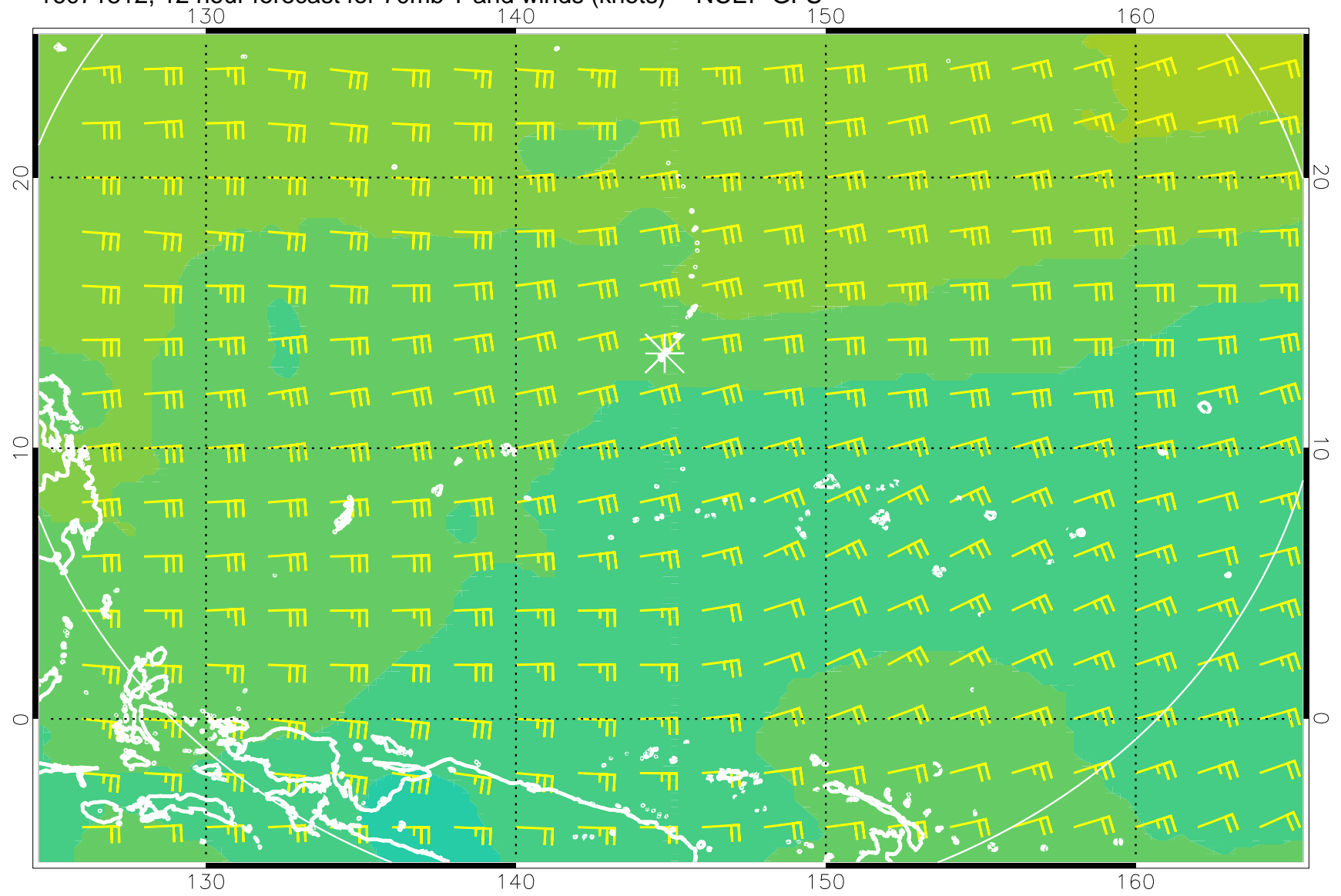
16071812, 12 hour forecast for 70mb T and winds (knots) -- NCEP GFS
