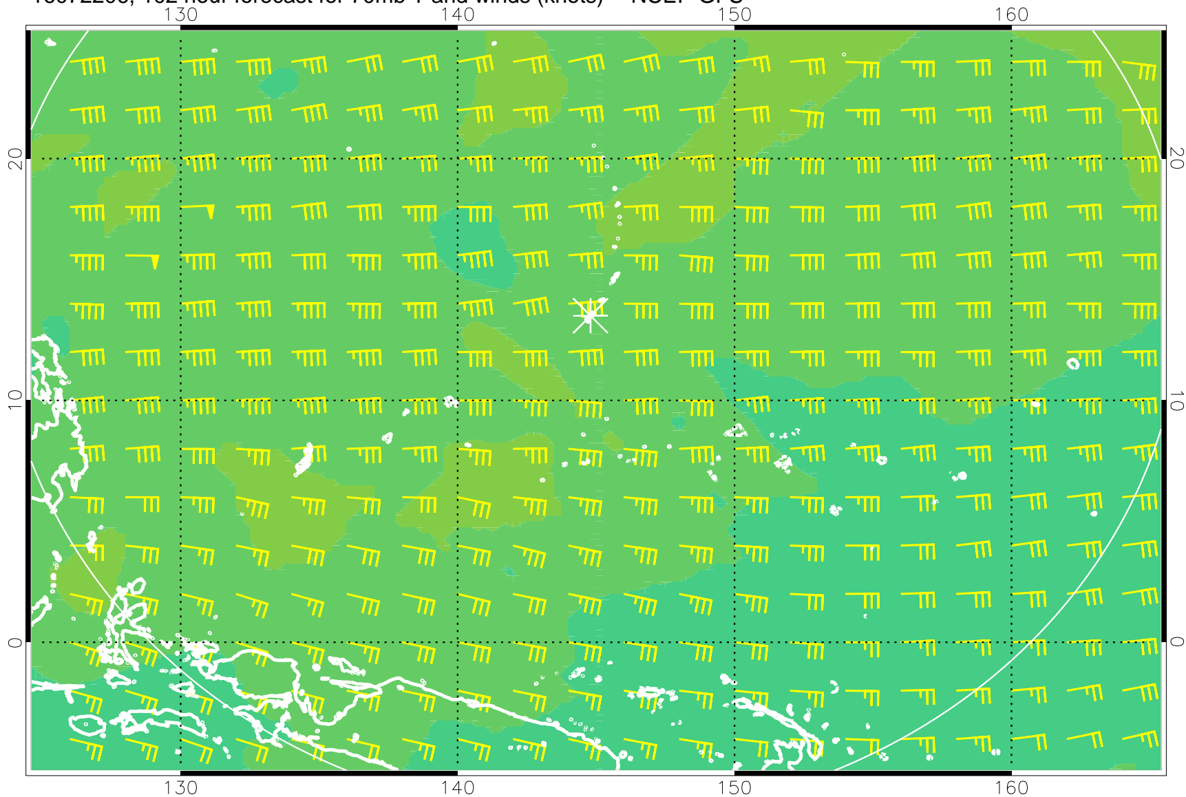
16072206, 102 hour forecast for 70mb T and winds (knots) -- NCEP GFS
