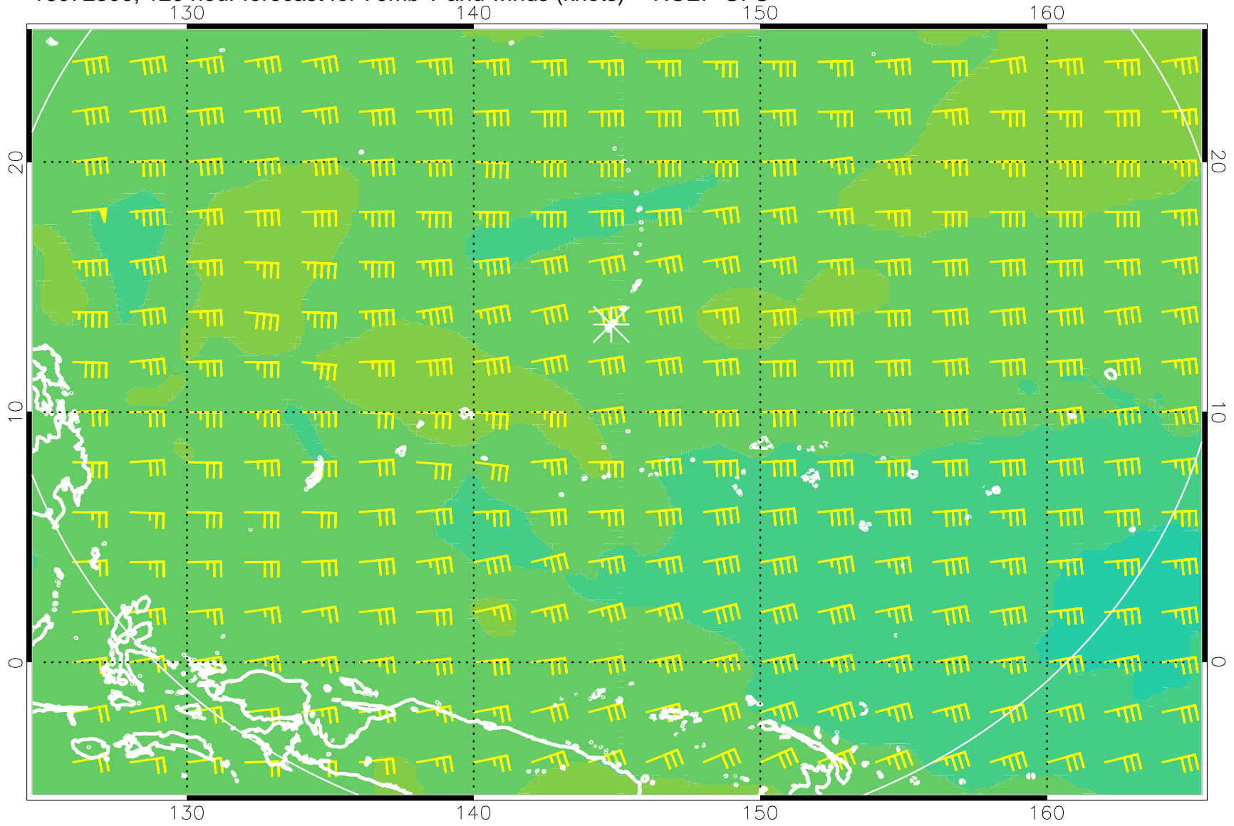
16072300, 120 hour forecast for 70mb T and winds (knots) -- NCEP GFS
