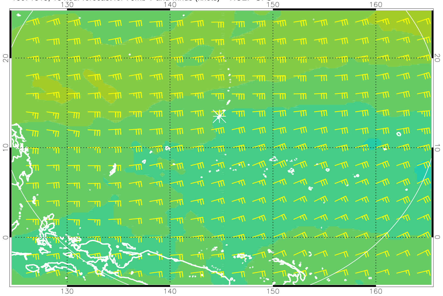
16071818, 18 hour forecast for 70mb T and winds (knots) -- NCEP GFS
