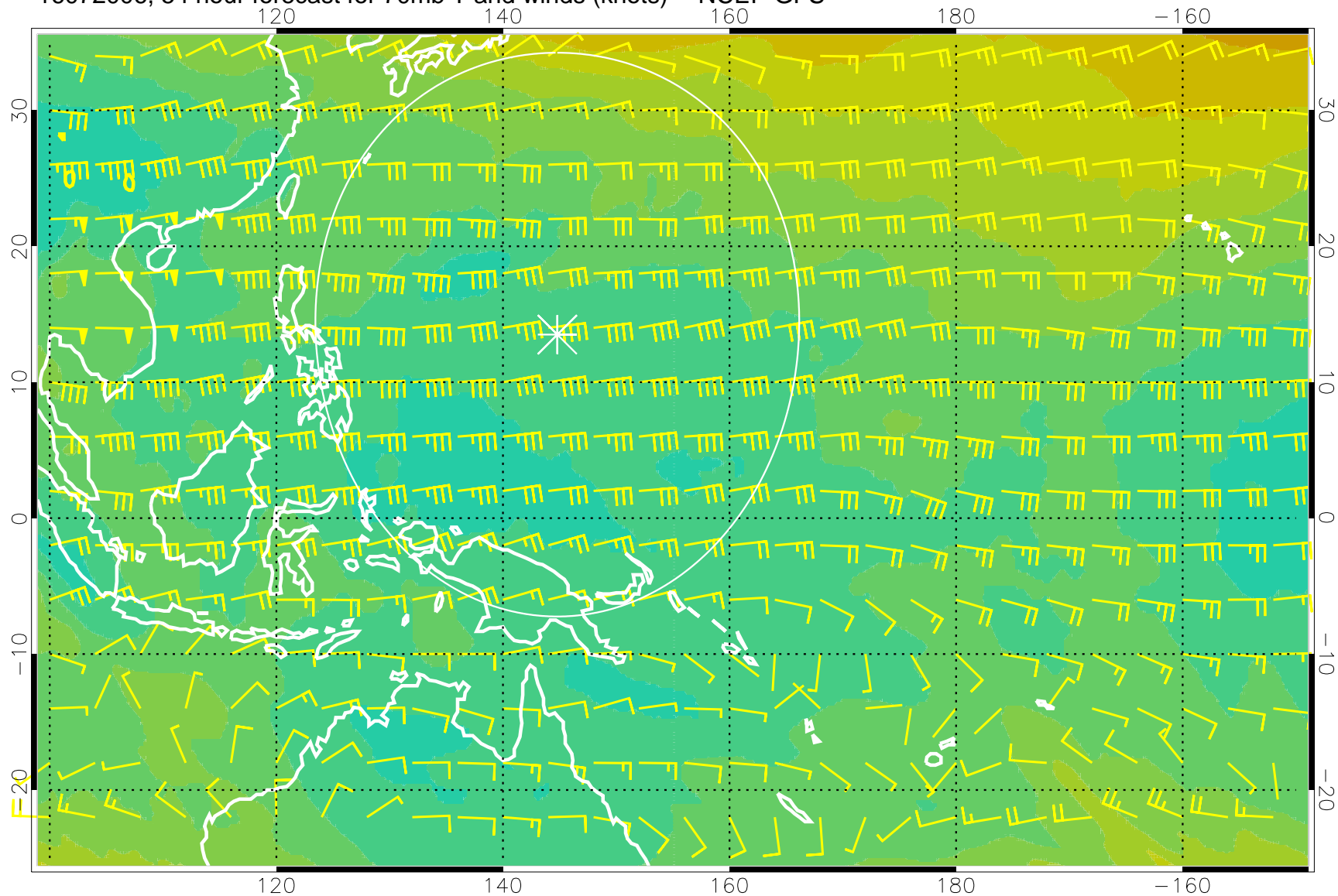
16072006, 54 hour forecast for 70mb T and winds (knots) -- NCEP GFS
