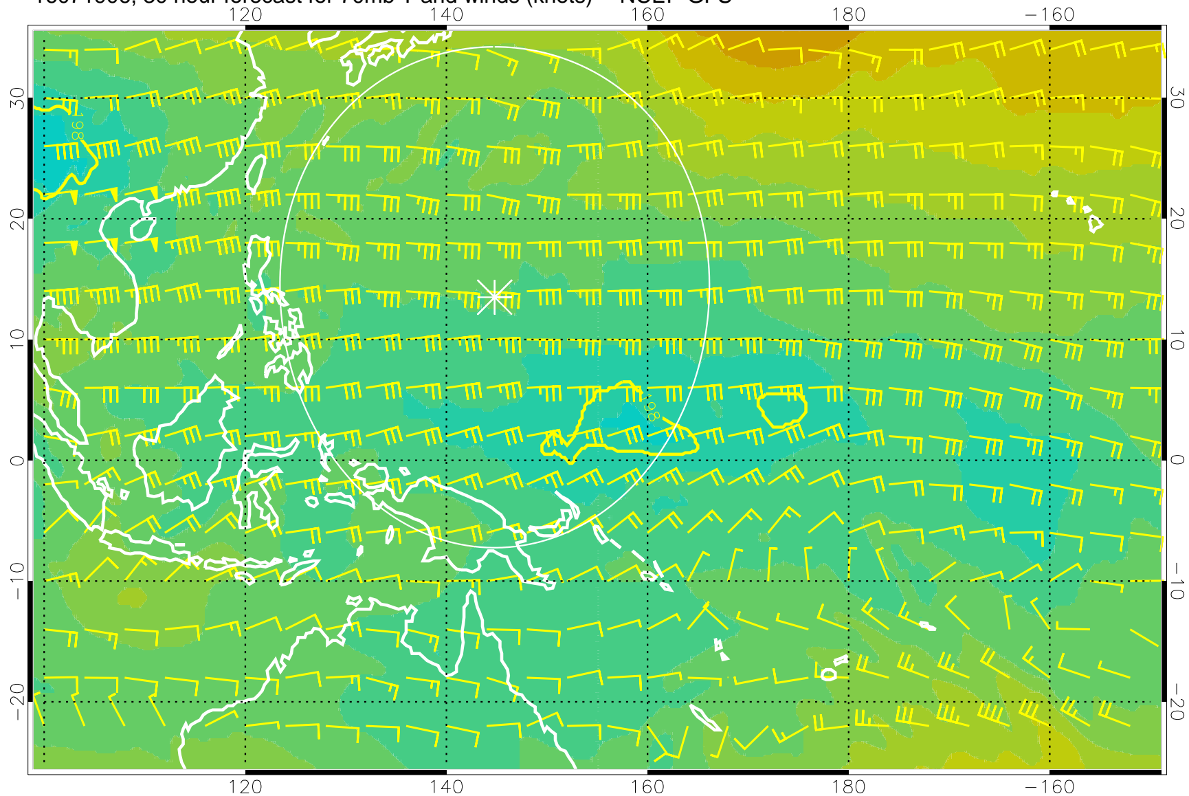
16071906, 30 hour forecast for 70mb T and winds (knots) -- NCEP GFS
