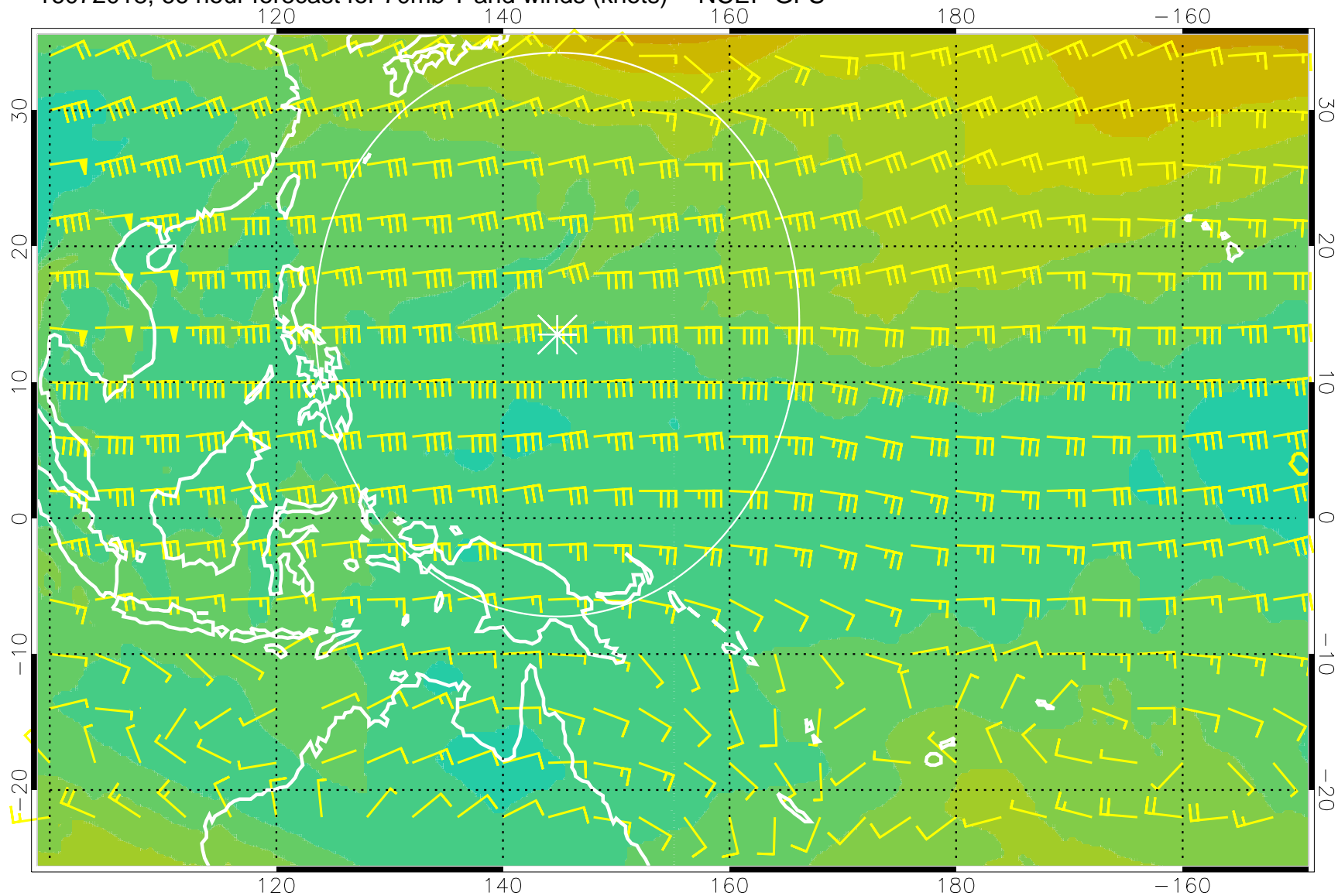
16072018, 66 hour forecast for 70mb T and winds (knots) -- NCEP GFS
