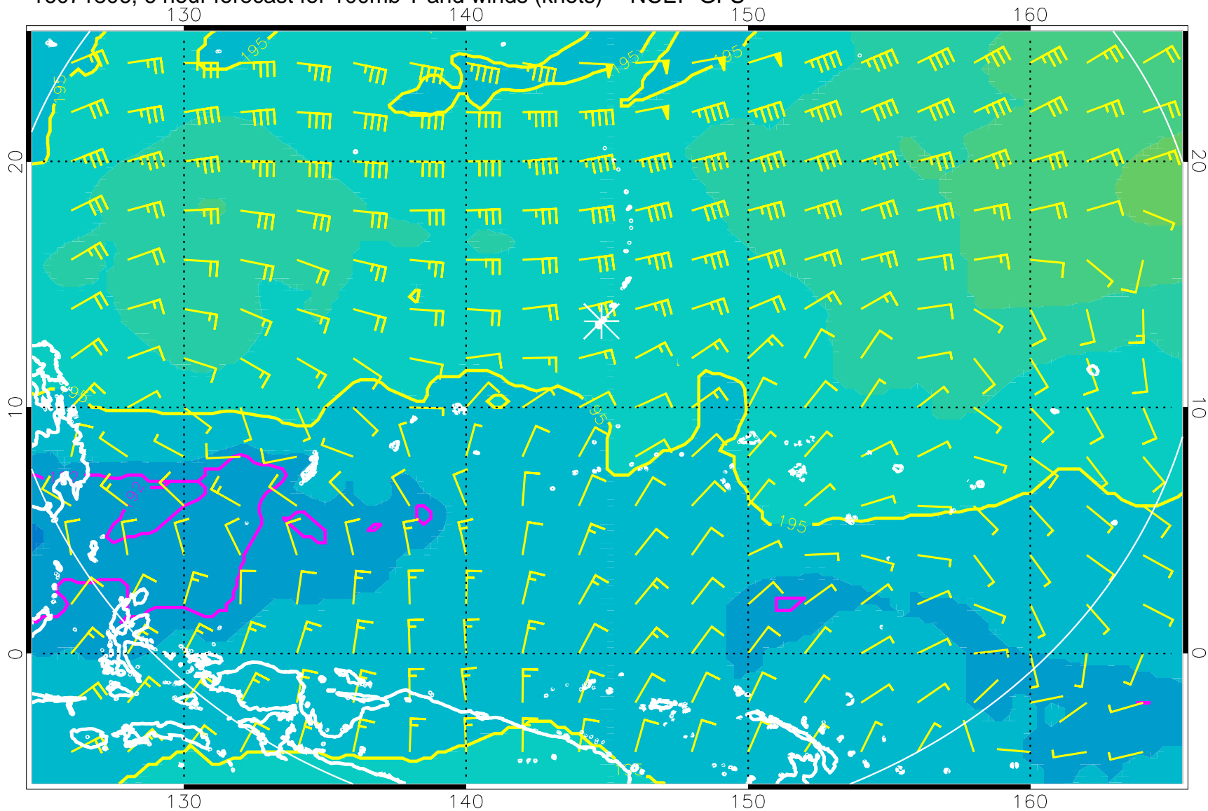
16071806, 6 hour forecast for 100mb T and winds (knots) -- NCEP GFS
