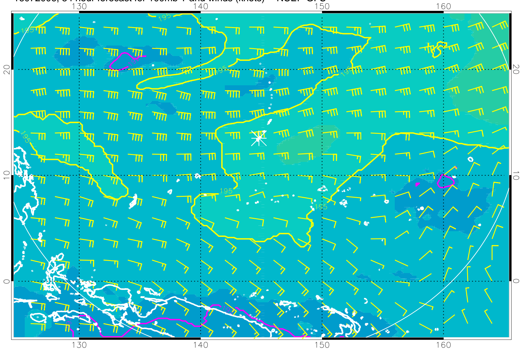
16072006, 54 hour forecast for 100mb T and winds (knots) -- NCEP GFS
