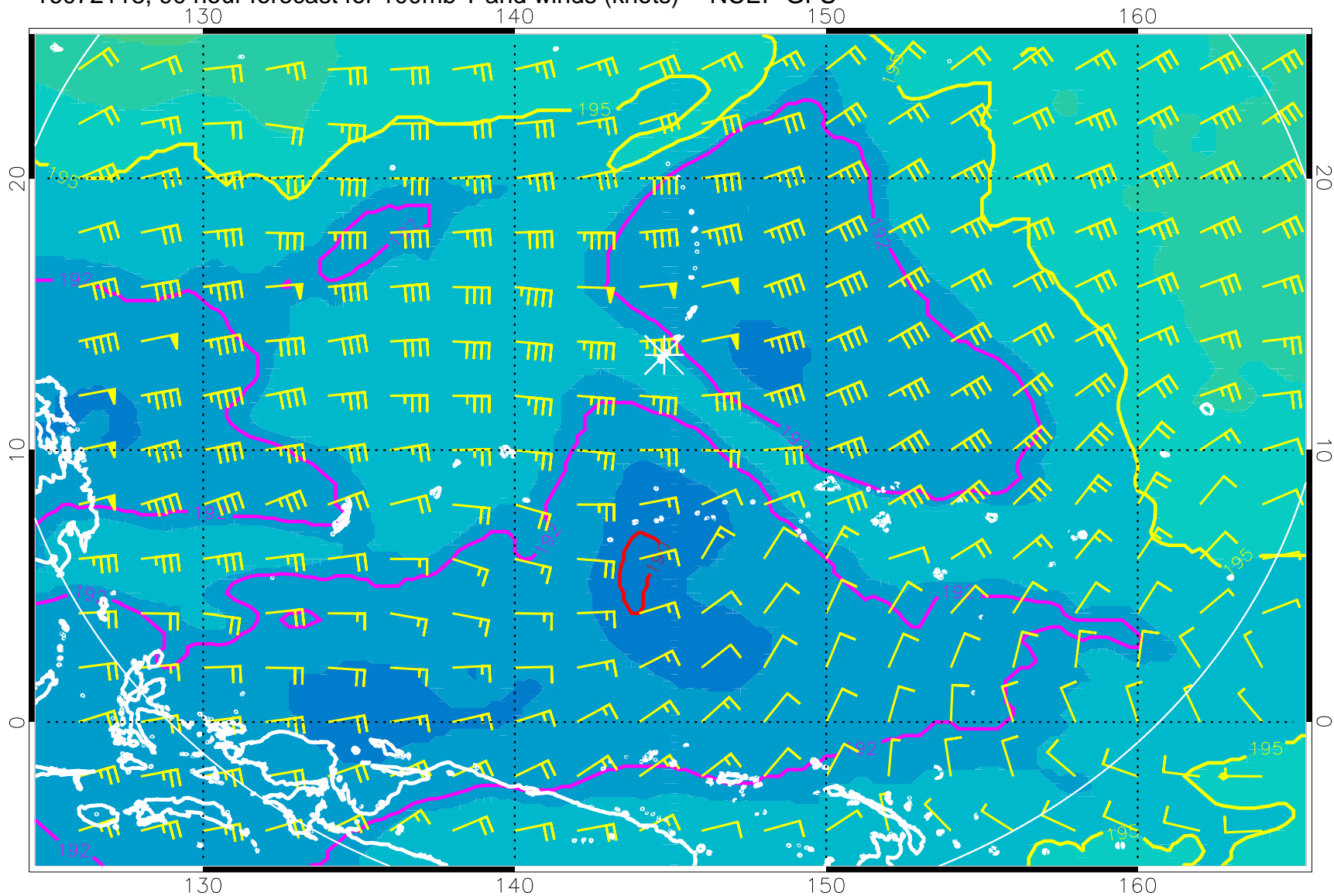
16072118, 90 hour forecast for 100mb T and winds (knots) -- NCEP GFS
