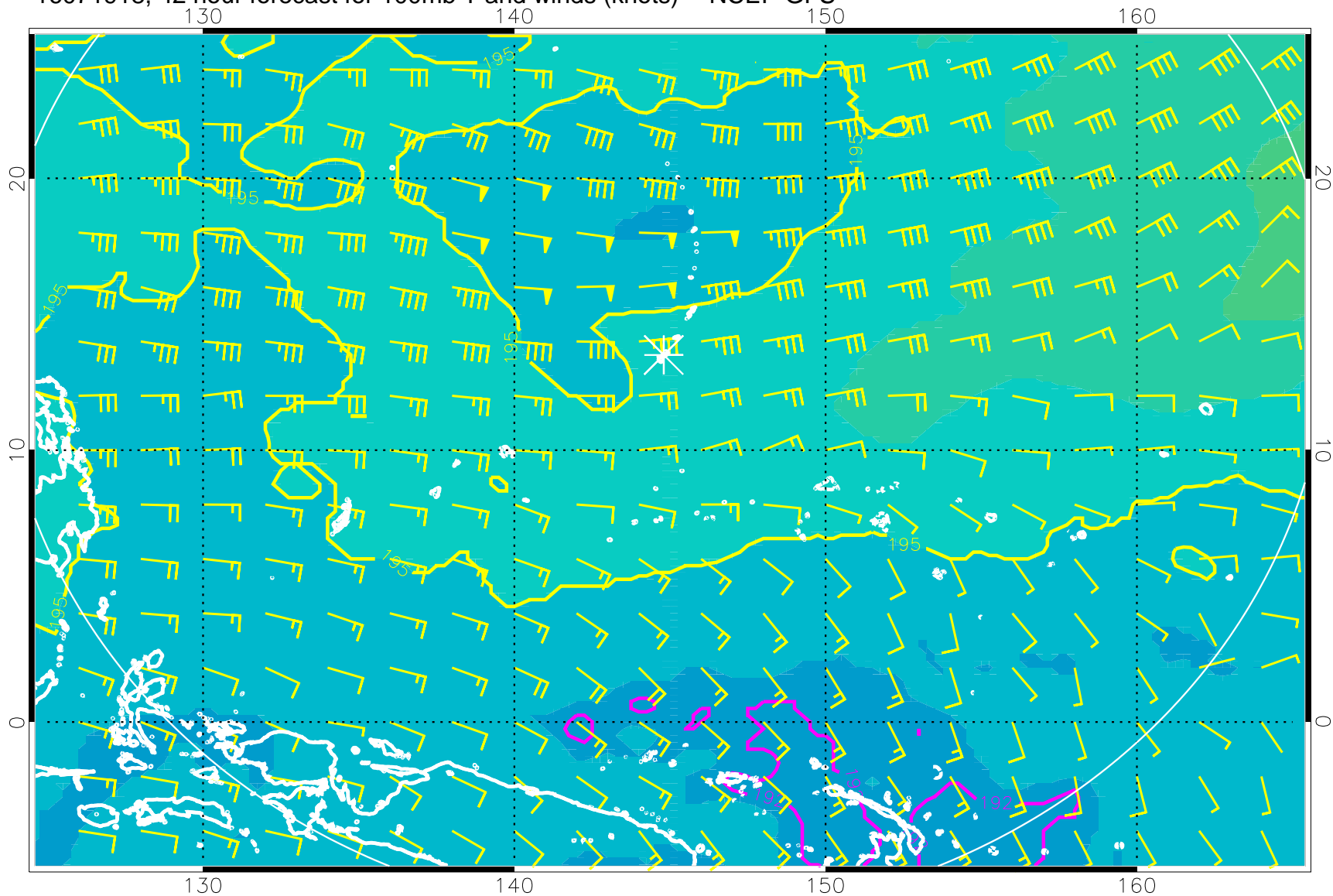
16071918, 42 hour forecast for 100mb T and winds (knots) -- NCEP GFS
