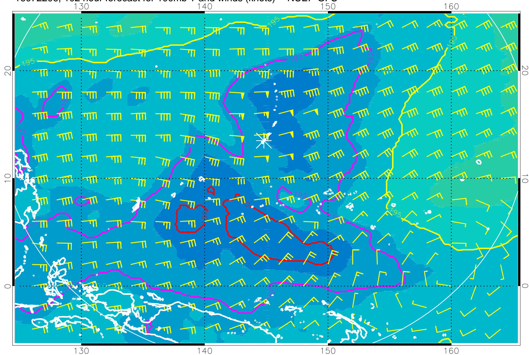
16072206, 102 hour forecast for 100mb T and winds (knots) -- NCEP GFS
