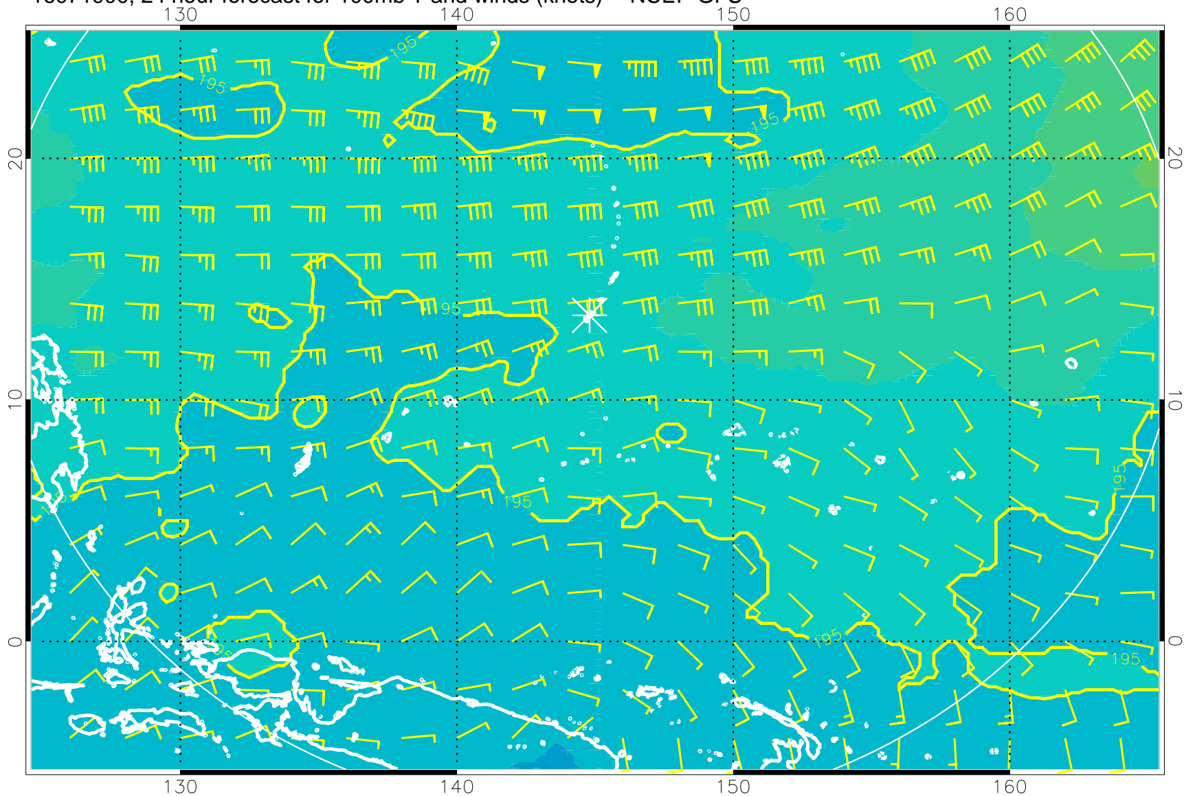
16071900, 24 hour forecast for 100mb T and winds (knots) -- NCEP GFS
