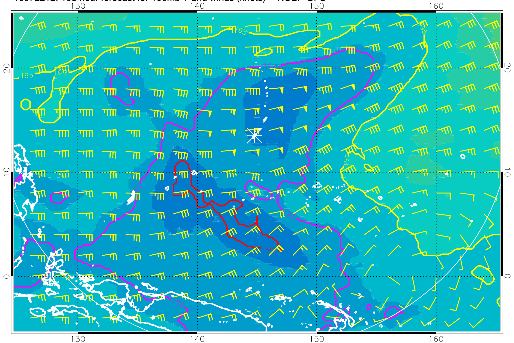
16072212, 108 hour forecast for 100mb T and winds (knots) -- NCEP GFS
