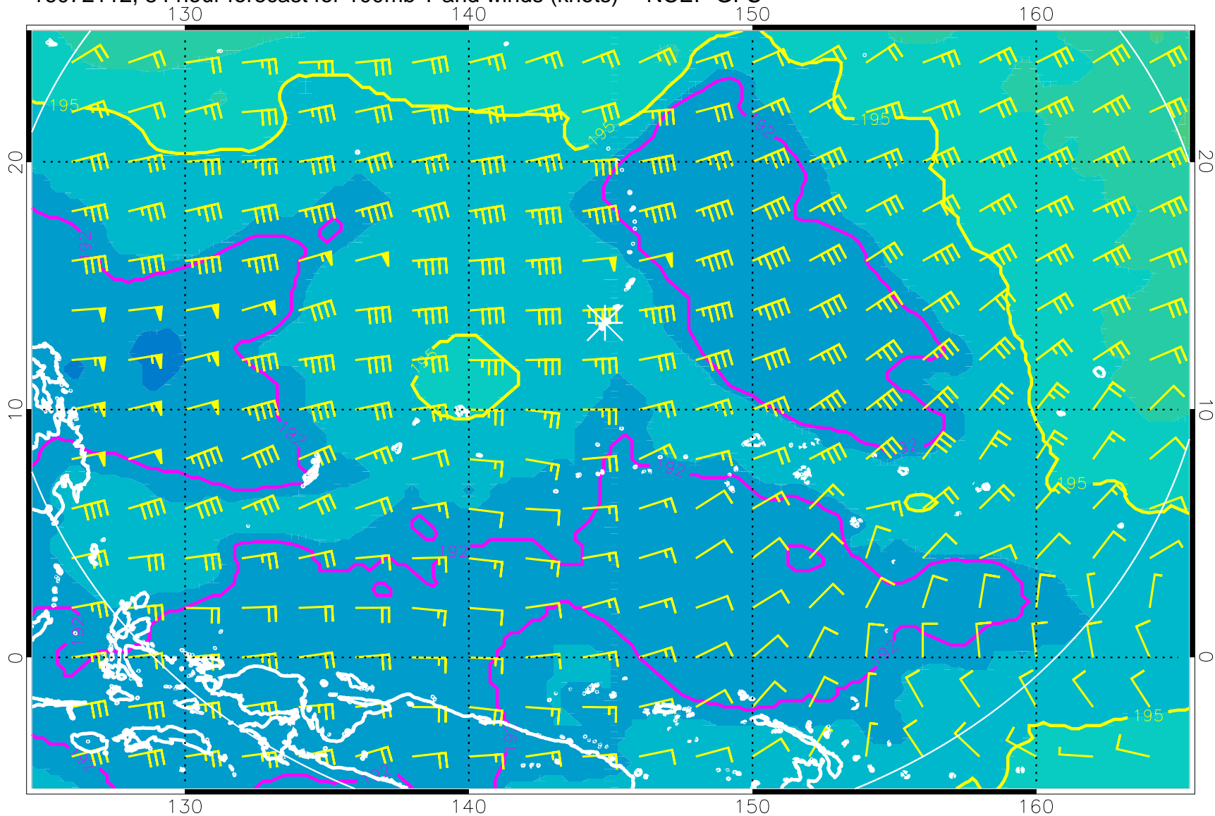
16072112, 84 hour forecast for 100mb T and winds (knots) -- NCEP GFS
