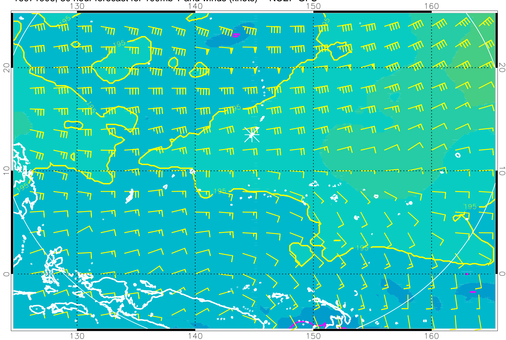
16071906, 30 hour forecast for 100mb T and winds (knots) -- NCEP GFS
