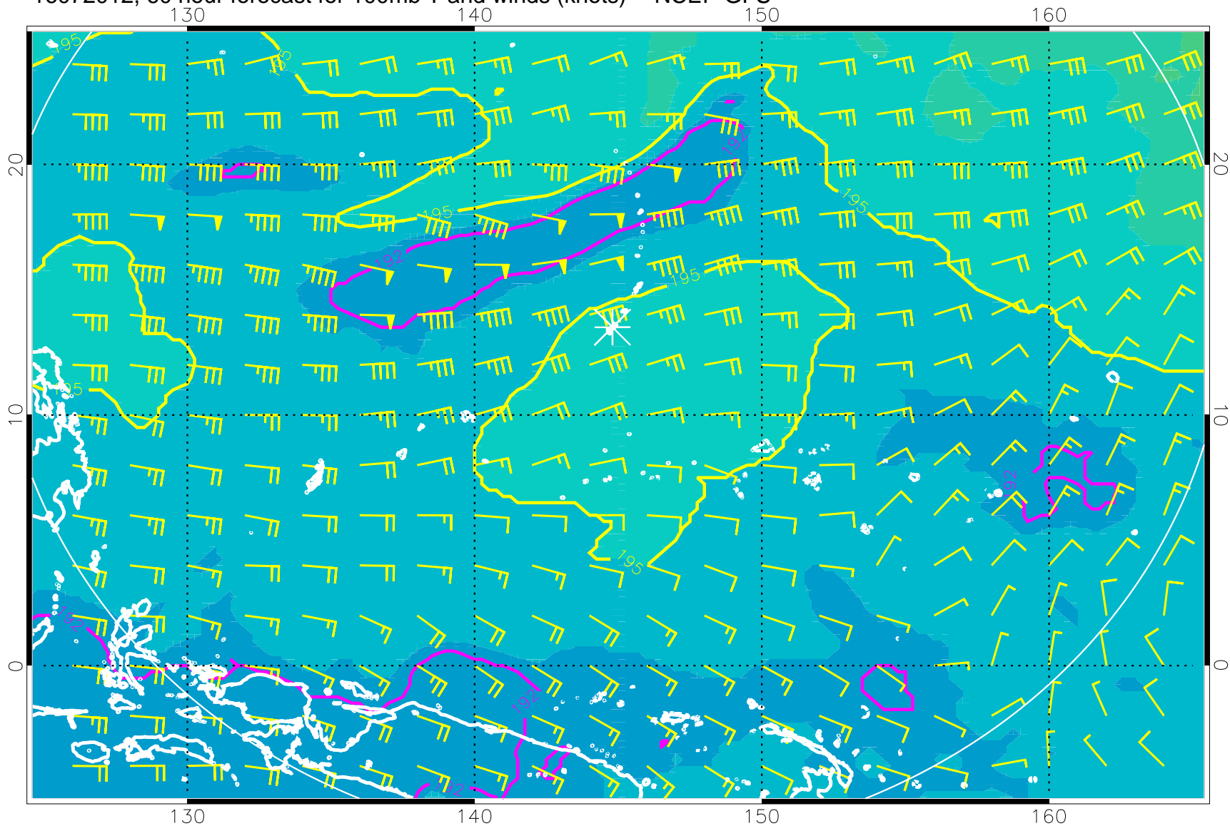
16072012, 60 hour forecast for 100mb T and winds (knots) -- NCEP GFS
