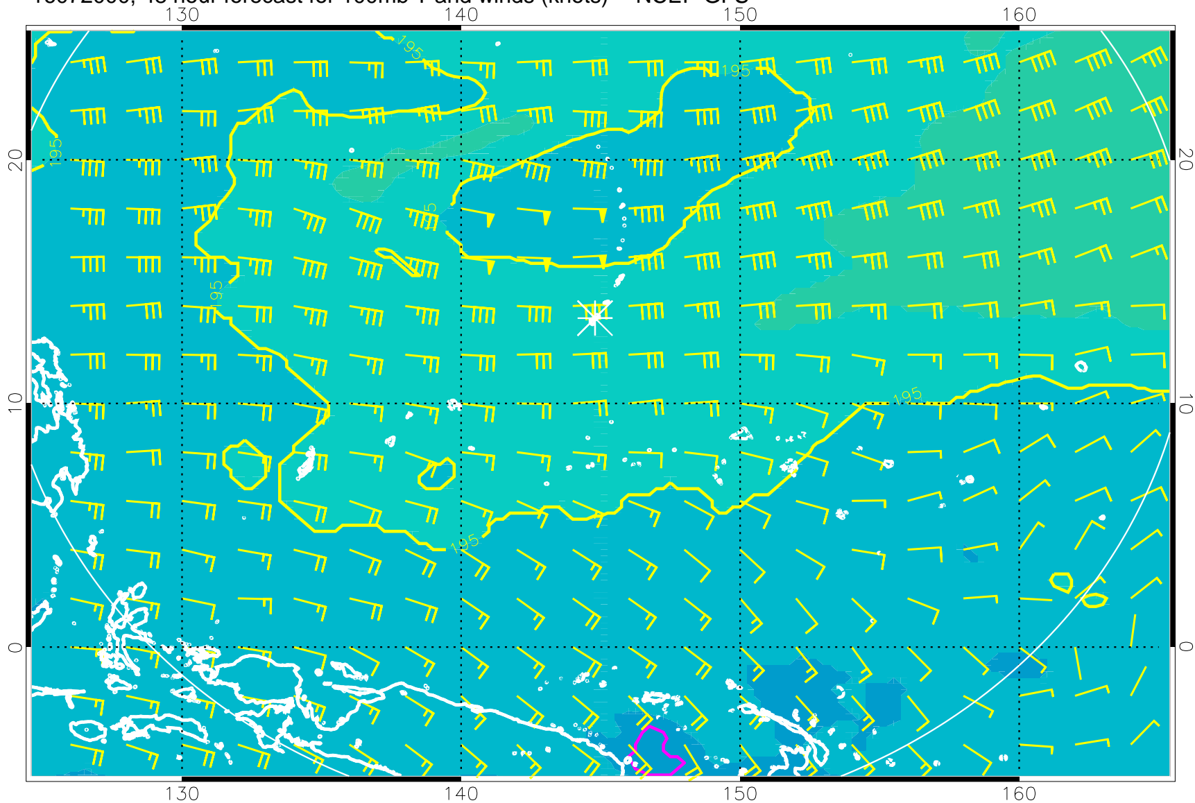
16072000, 48 hour forecast for 100mb T and winds (knots) -- NCEP GFS
