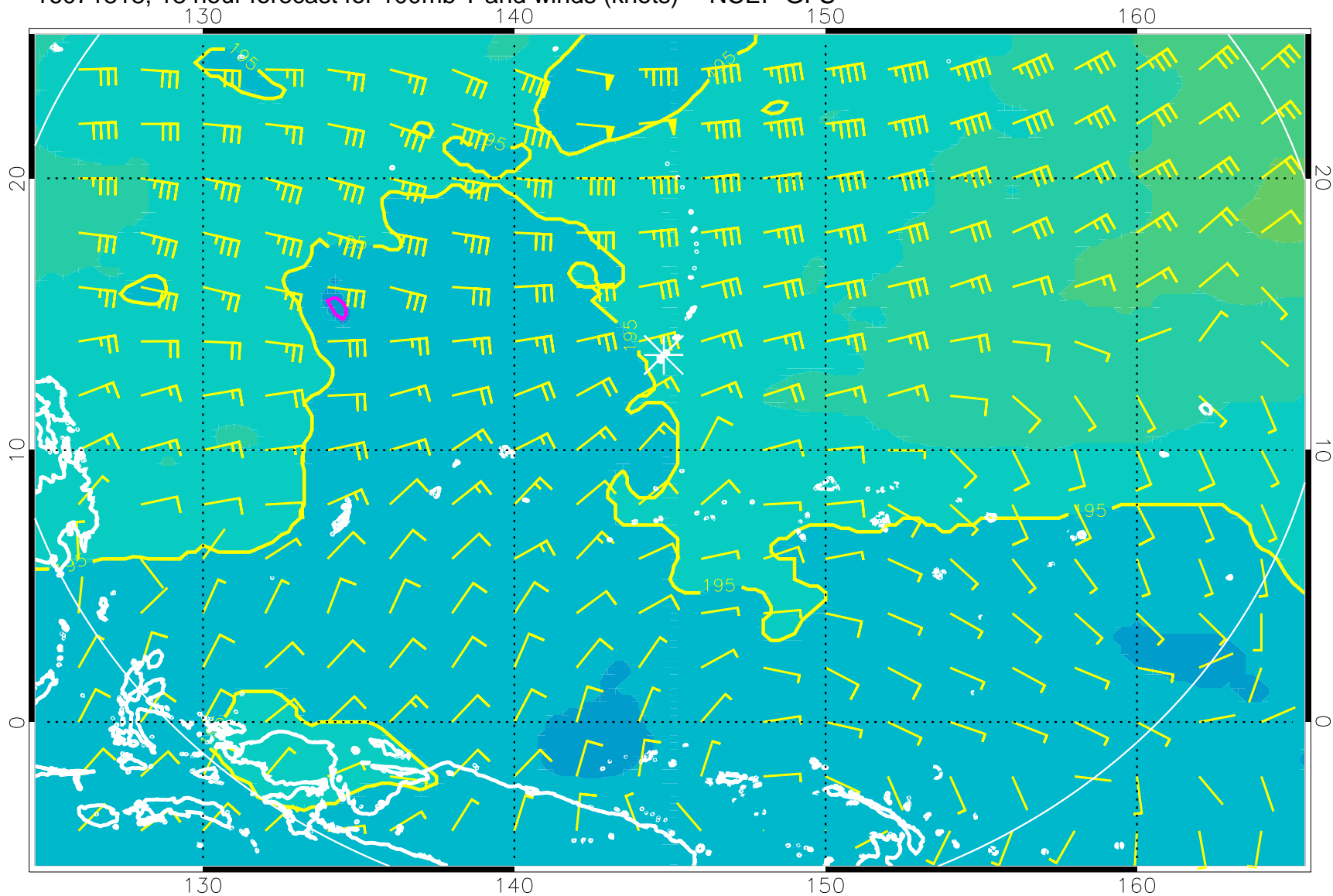
16071818, 18 hour forecast for 100mb T and winds (knots) -- NCEP GFS
