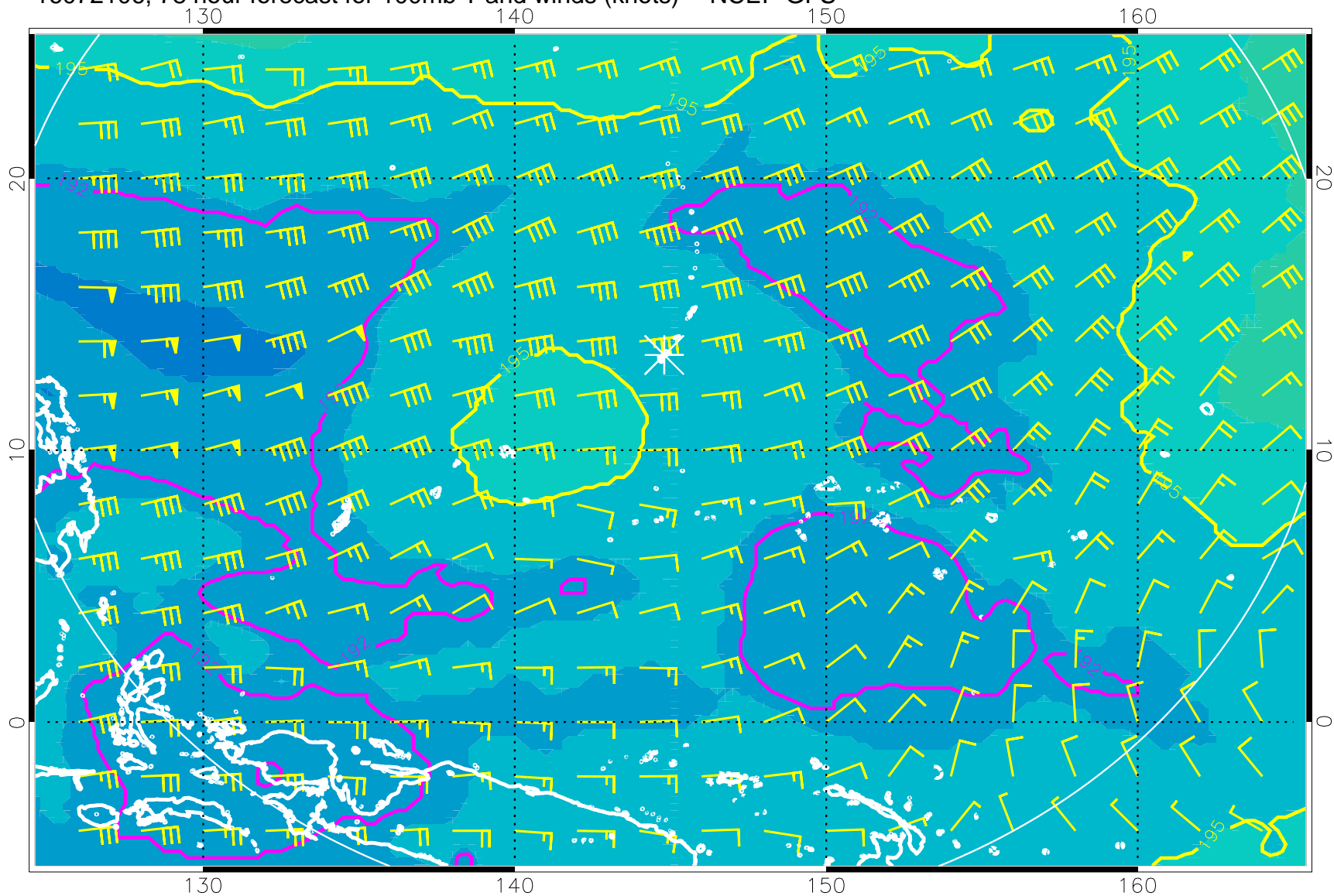
16072106, 78 hour forecast for 100mb T and winds (knots) -- NCEP GFS
