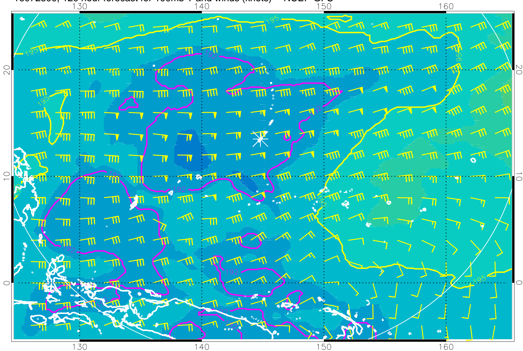
16072300, 120 hour forecast for 100mb T and winds (knots) -- NCEP GFS
