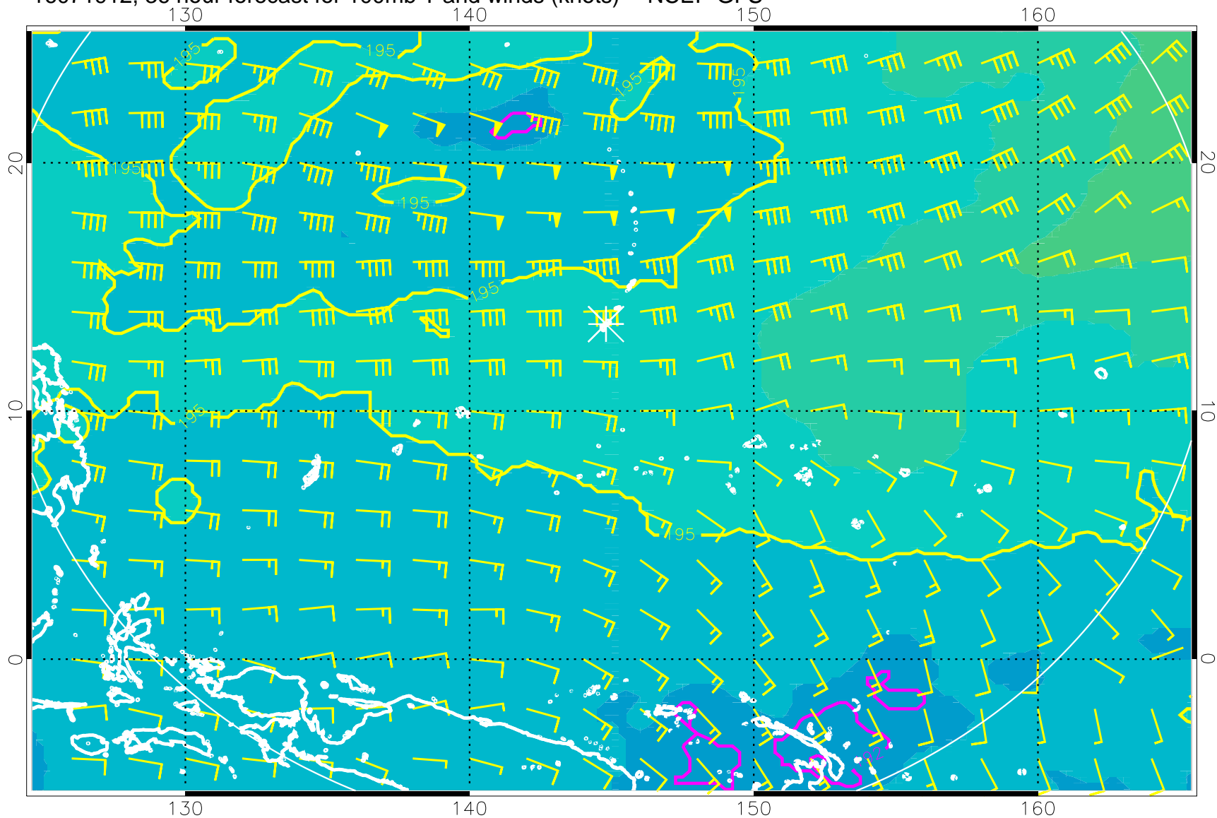
16071912, 36 hour forecast for 100mb T and winds (knots) -- NCEP GFS
