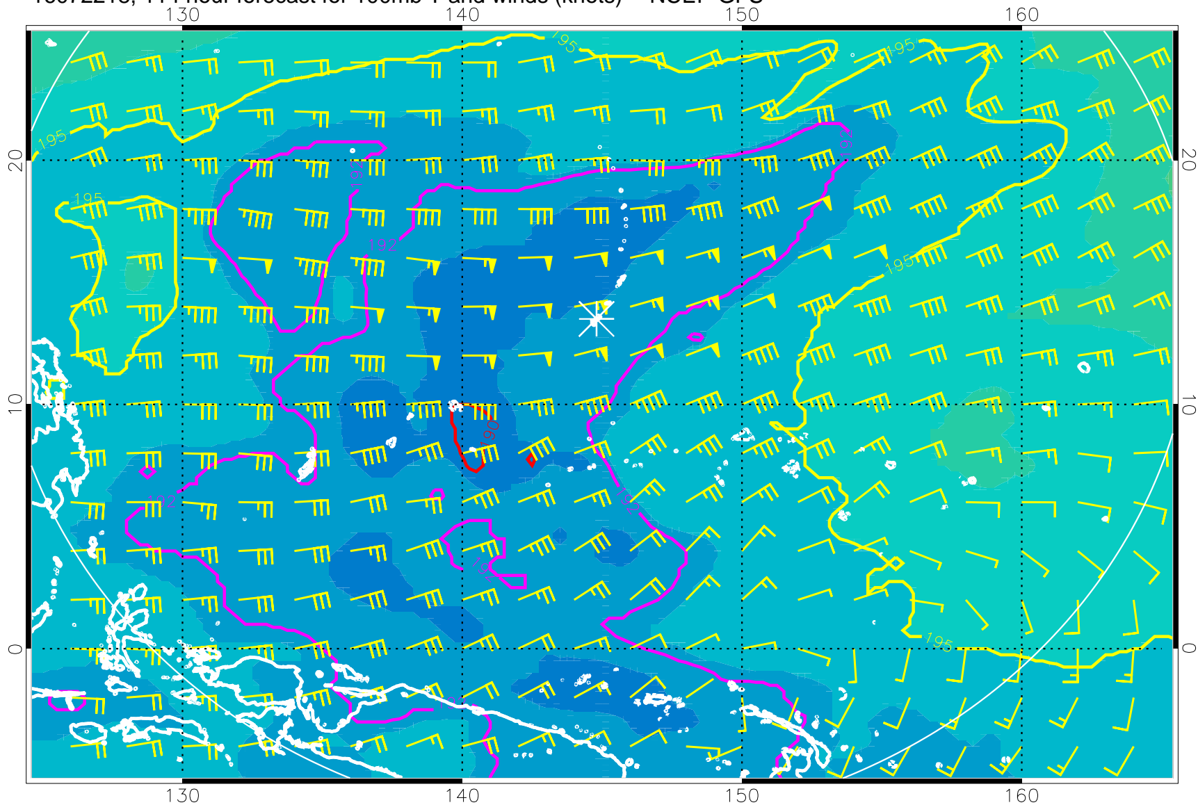
16072218, 114 hour forecast for 100mb T and winds (knots) -- NCEP GFS
