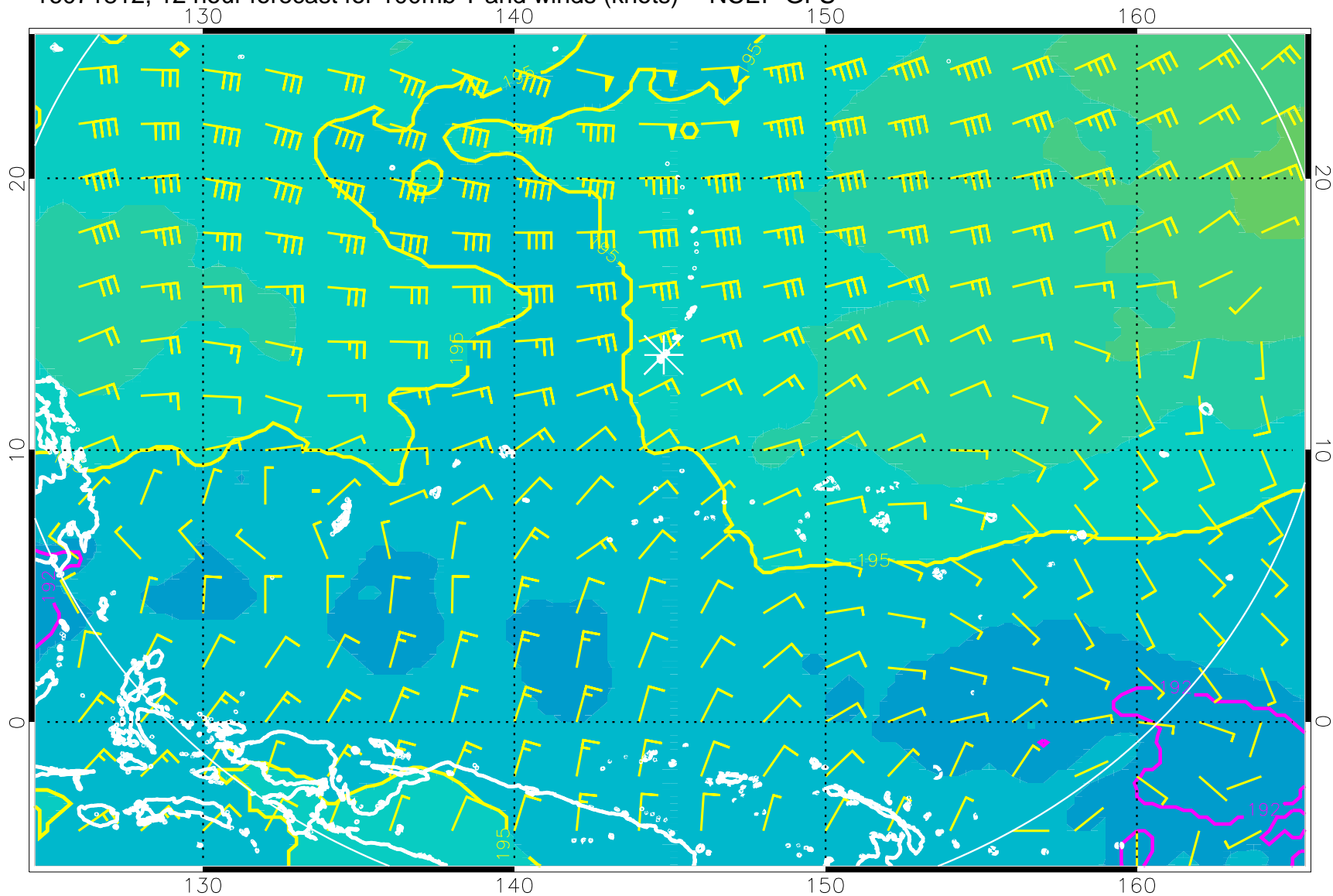
16071812, 12 hour forecast for 100mb T and winds (knots) -- NCEP GFS
