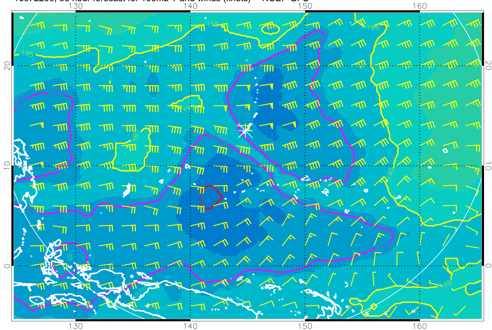
16072200, 96 hour forecast for 100mb T and winds (knots) -- NCEP GFS
