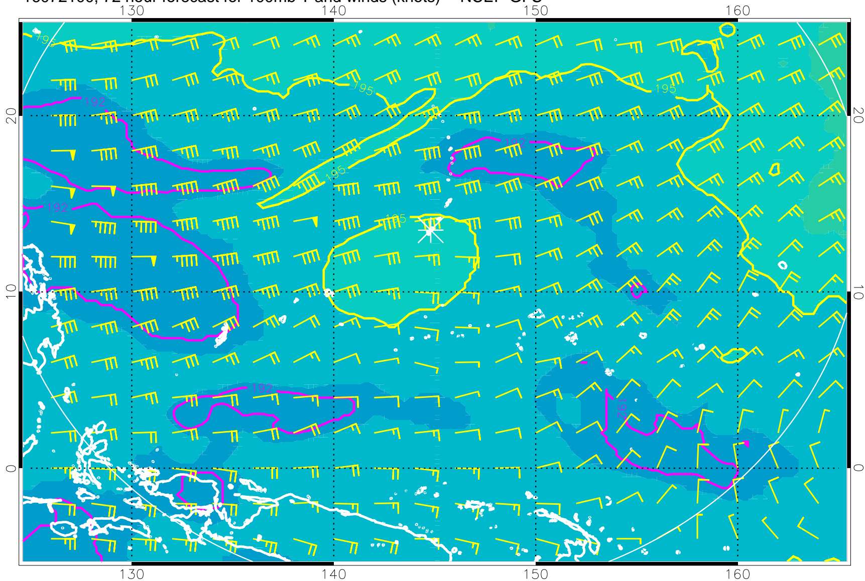
16072100, 72 hour forecast for 100mb T and winds (knots) -- NCEP GFS
