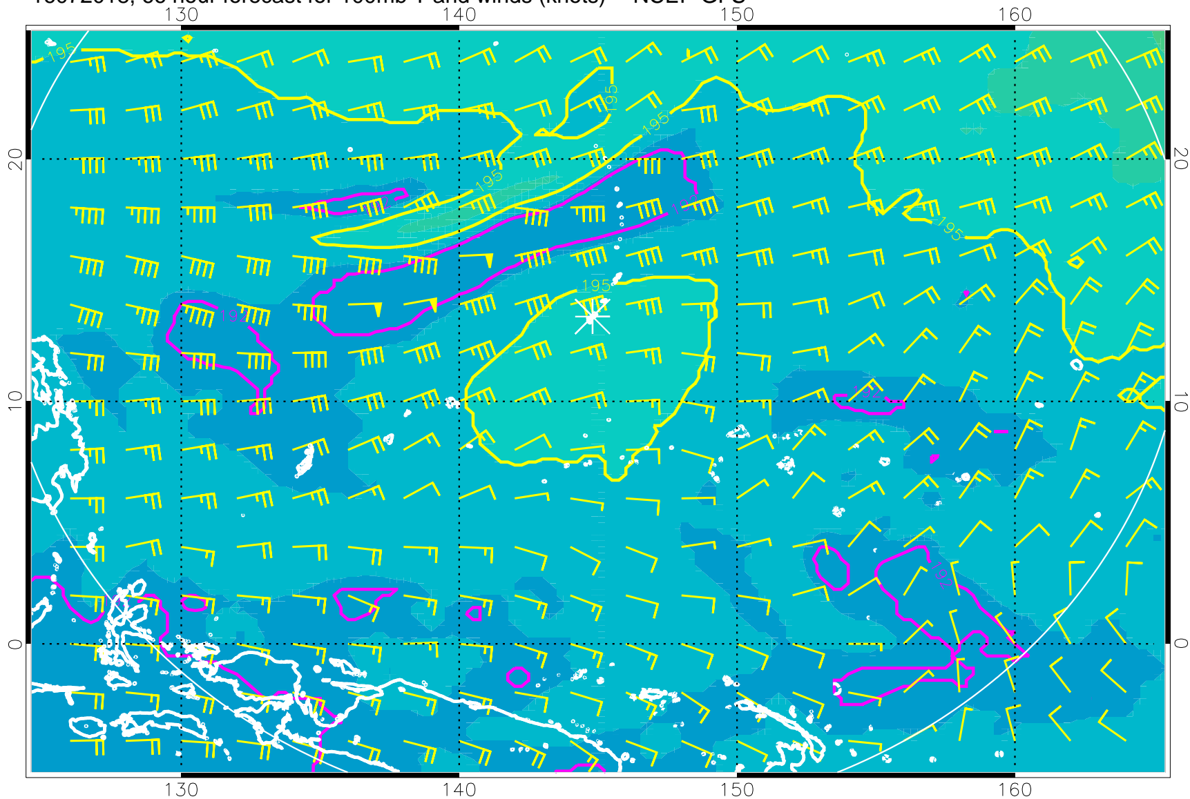
16072018, 66 hour forecast for 100mb T and winds (knots) -- NCEP GFS
